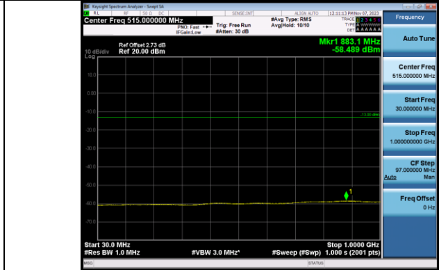
Band2_20MHz_QPSK_19100_1RB#0_30~1000_30~1000
