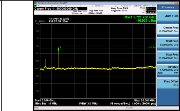
Band2 3MHz_QPSK_19185_1RB#0_3000~20000_3000~20000
