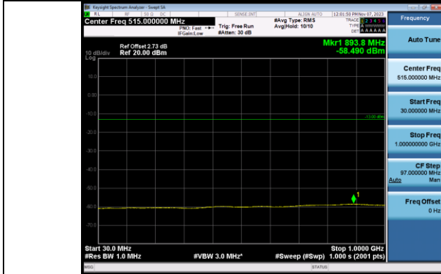
Band2_15MHz_QPSK_18675_1RB#0_30~1000_30~1000
