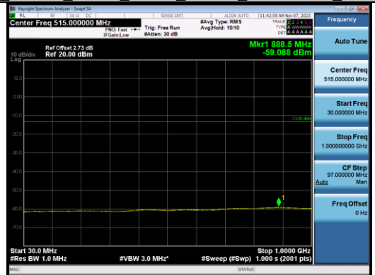
Band2_10MHz_QPSK_19150_1RB#0_30~1000_30~1000
