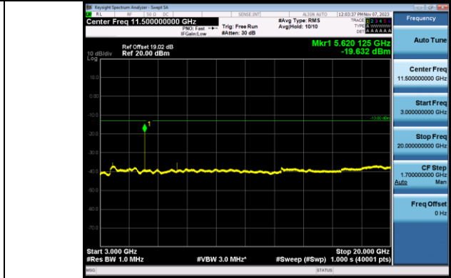
Band2_15MHz_QPSK_18900_1RB#0_3000-20000_3000-20000
