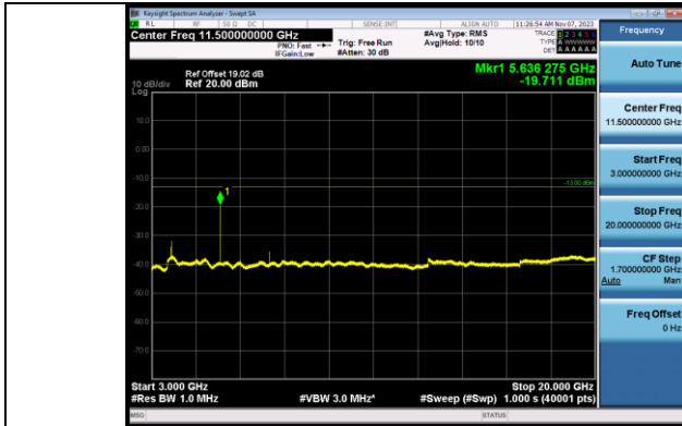
Band2 3MHz_QPSK_1890_1RB#0_3000~20000_3000~20000
