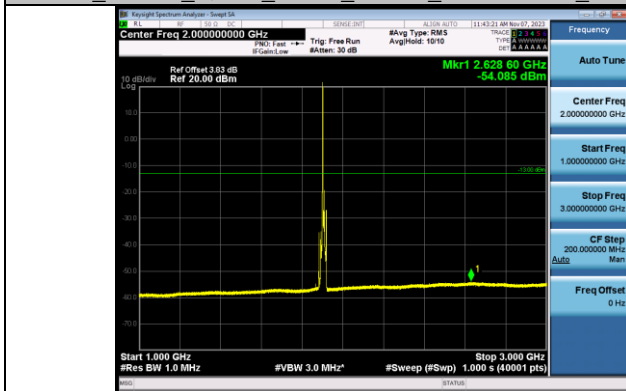
Band2_10MHz_QPSK_19150_1RB#0_1000~3000_1000~3000
