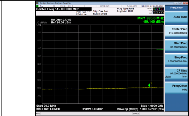
Band2 5MHz_QPSK_1890_1RB#0_30~1000_30~1000
