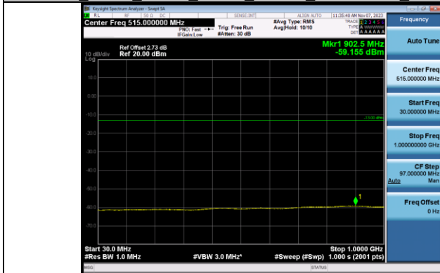
Band2_5MHz_QPSK_19175_1RB#0_30~1000_30~1000
