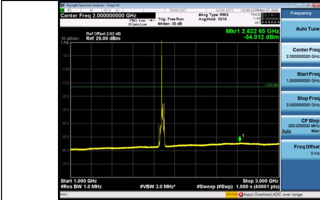
Band2_15MHz_QPSK_18900_1RB#0_1000-3000_1000-3000
