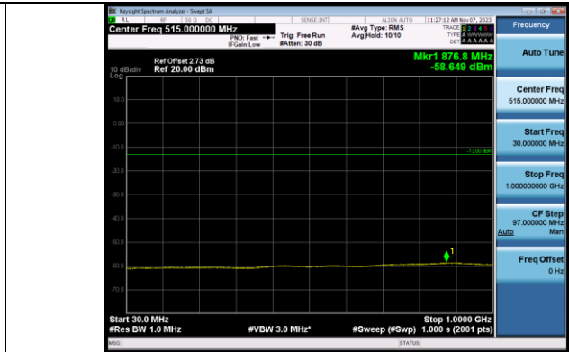
Band2 3MHz_QPSK_19185_1RB#0_30~1000_30~1000
