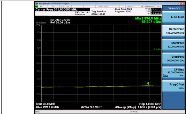
Band2_15MHz_QPSK_18900_1RB#0_30-1000_30-1000
