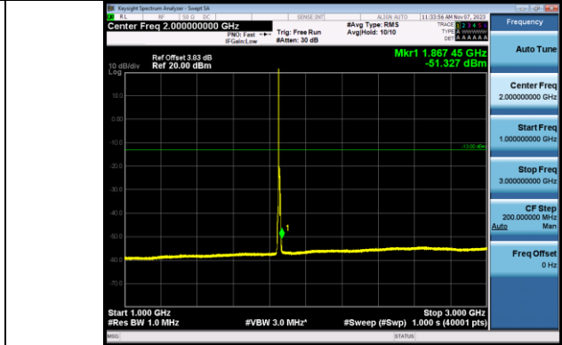
Band2 5MHz_QPSK_18625_1RB#0_1000~3000_1000~3000
