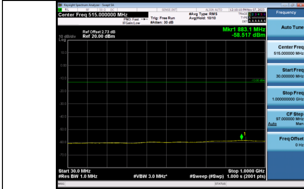
Band2_20MHz_QPSK_18900_1RB#0_30~1000_30~1000
