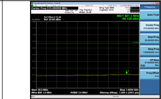
Band2_10MHz_QPSK_18650_1RB#0_30~1000_30~1000
