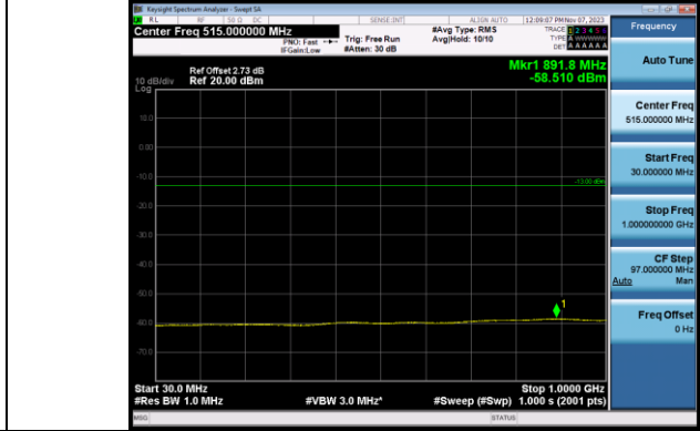
Band2_20MHz_QPSK_18700_1RB#0_30-1000_30-1000
