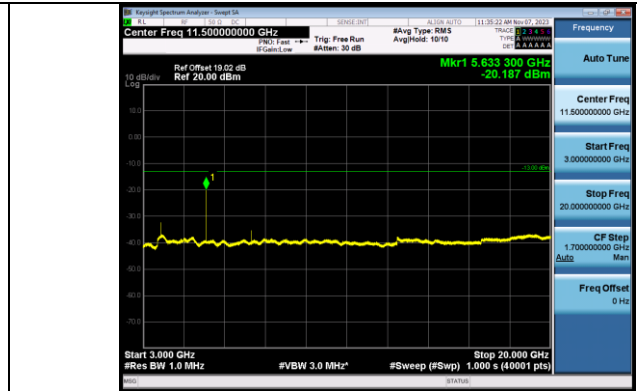
Band2_5MHz_QPSK_18900_1RB#0_3000~20000_3000~20000
