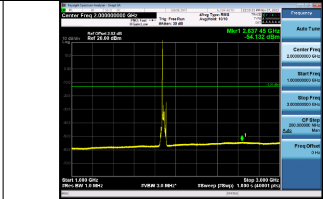
Band2_20MHz_QPSK_18900_1RB#0_1000~3000_1000~3000
