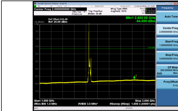
Band2_20MHz_QPSK_18700_1RB#0_1000~3000_1000~3000
