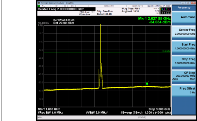
Band2_15MHz_QPSK_19125_1RB#0_1000-3000_1000-3000
