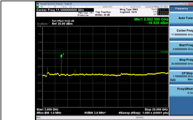
Band2_15MHz_QPSK_18675_1RB#0_3000-20000_3000-20000
