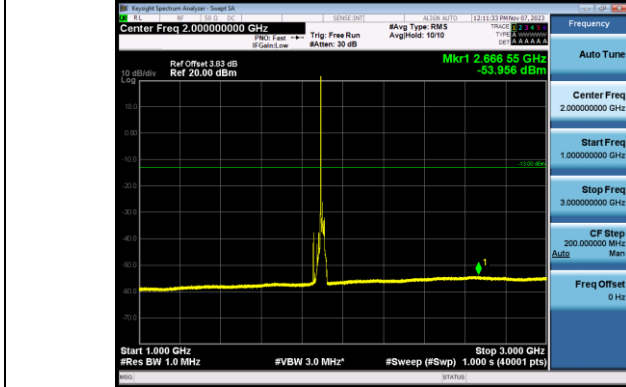
Band2_20MHz_QPSK_19100_1RB#0_1000~3000_1000~3000
