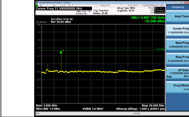
Band2_15MHz_QPSK_19125_1RB#0_3000-20000_3000-20000
