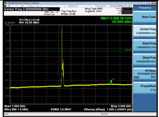
Band2_15MHz_QPSK_18675_1RB#0_1000~3000_1000~3000
