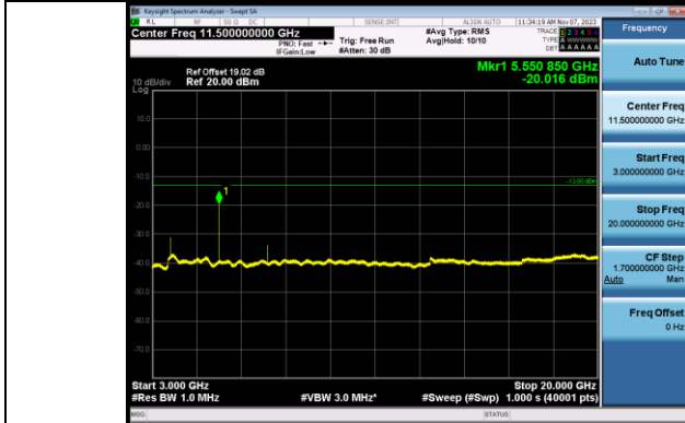
Band2 5MHz_QPSK_18625_1RB#0_3000~20000_3000~20000
