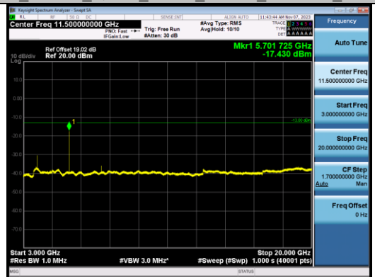
Band2_10MHz_QPSK_19150_1RB#0_3000~20000_3000~20000
