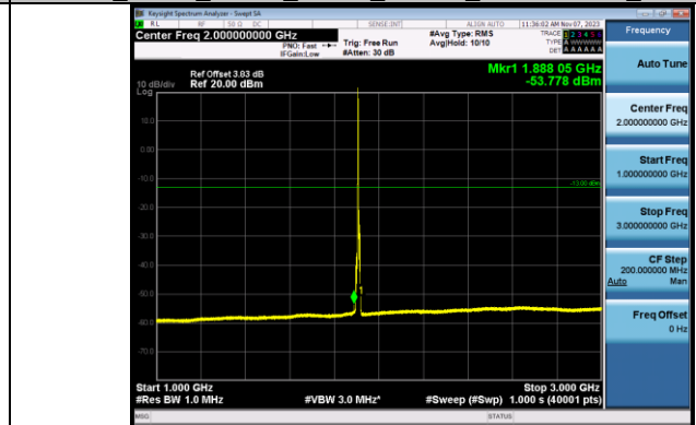
Band2_5MHz_QPSK_19175_1RB#0_1000~3000_1000~3000
