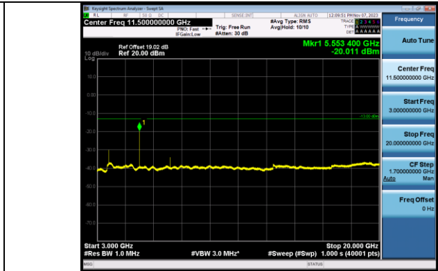
Band2_20MHz_QPSK_18700_1RB#0_3000~20000_3000~20000
