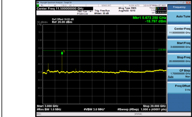
Band2_20MHz_QPSK_19100_1RB#0_3000~20000_3000~20000
