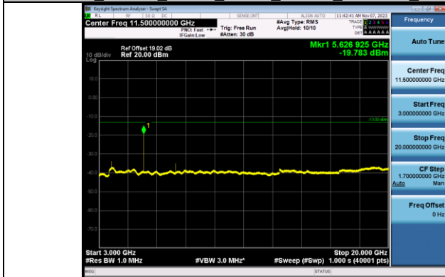
Band2_10MHz_QPSK_18900_1RB#0_3000~20000_3000~20000
