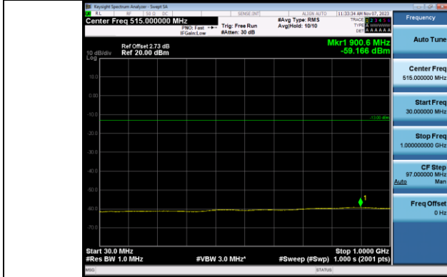
Band2 5MHz_QPSK_18625_1RB#0_30~1000_30~1000
