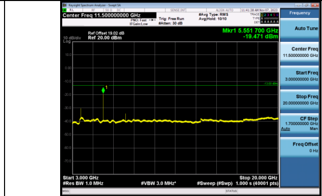
Band2_10MHz_QPSK_18650_1RB#0_3000~20000_3000~20000
