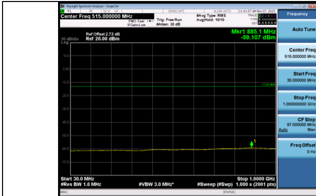
Band2_10MHz_QPSK_18900_1RB#0_30~1000_30~1000
