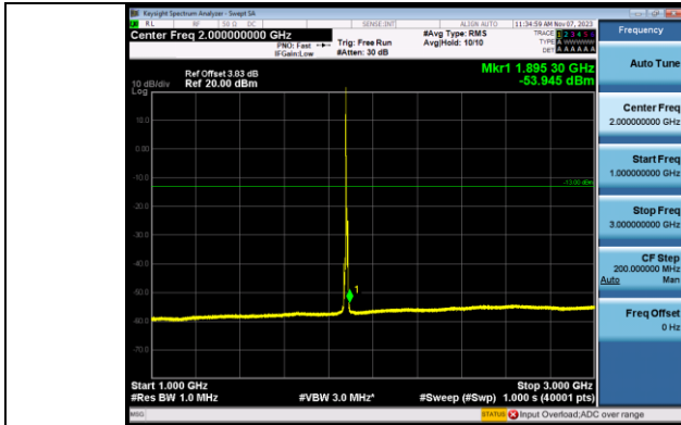
Band2_5MHz_QPSK_18900_1RB#0_1000~3000_1000~3000
