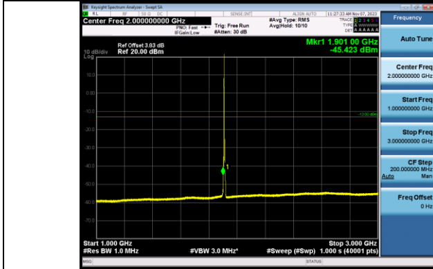
Band2 3MHz_QPSK_19185_1RB#0_1000~3000_1000~3000
