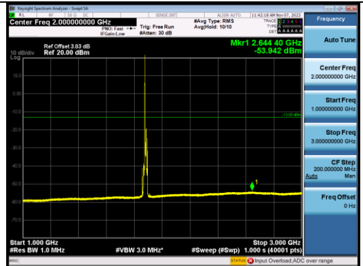
Band2_10MHz_QPSK_18900_1RB#0_1000~3000_1000~3000
