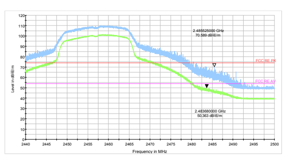
802.11g-Channel 10 Peak+ Average
