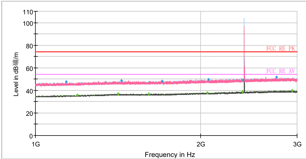
Note: The signal beyond the limit is carrier. Radiates Emission from 1GHz to 3GHz
