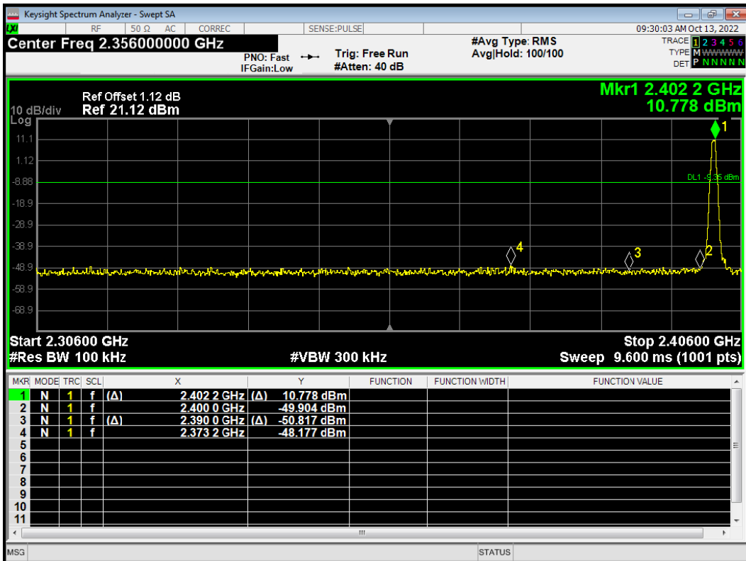
Band Edge 1-DH5 2402MHz No-Hopping Emission
