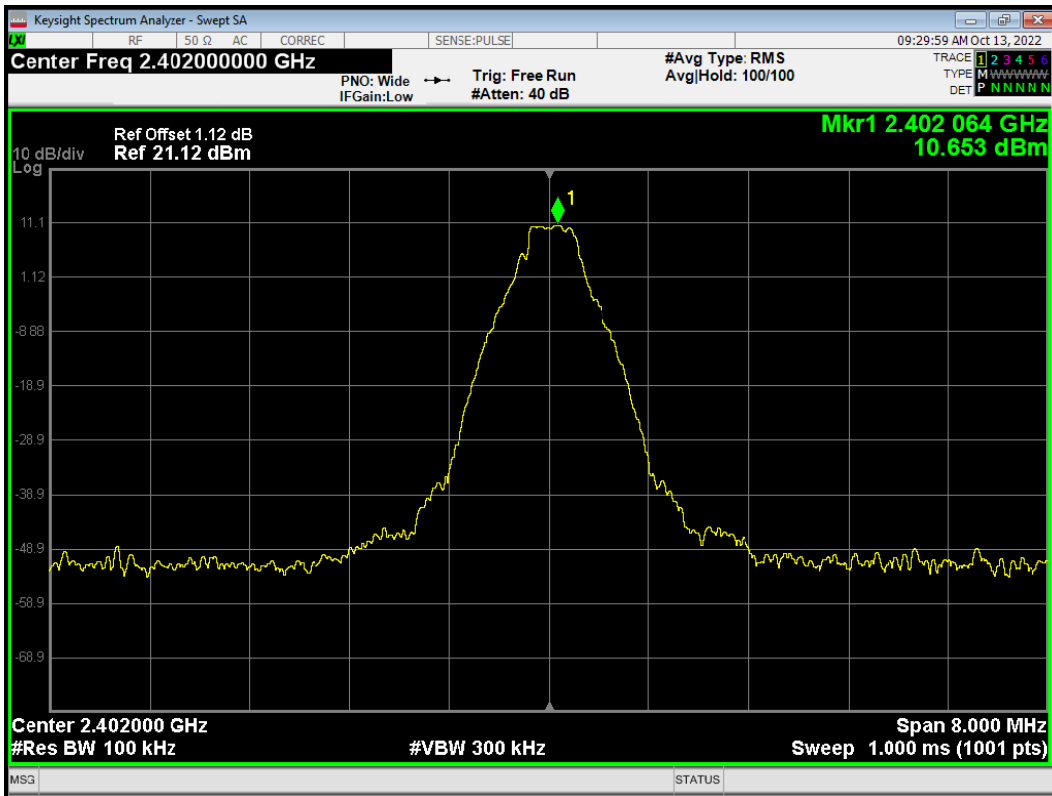
Band Edge 1-DH5 2402MHz No-Hopping Ref
