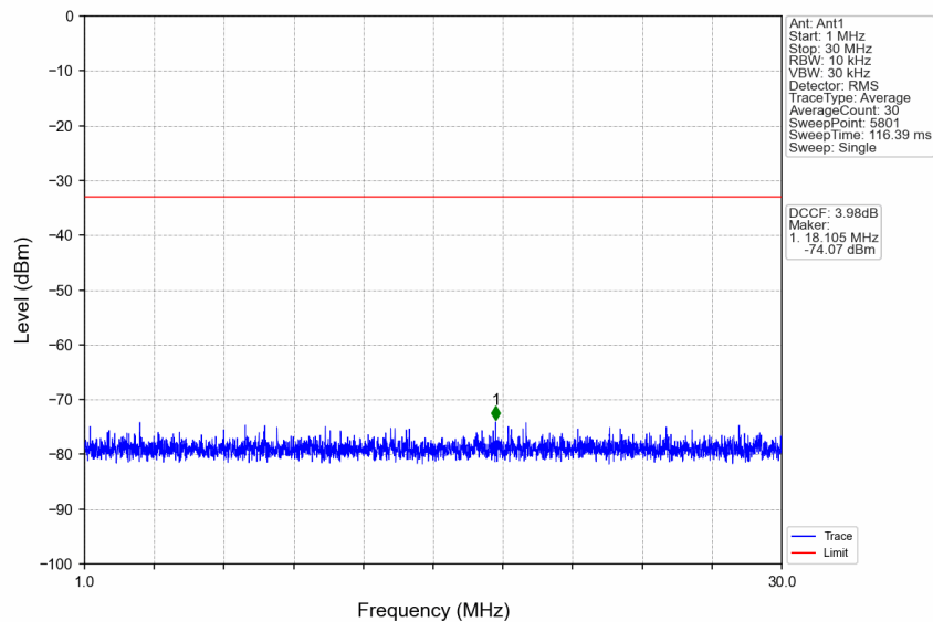
n77a_30kHz_SISO_NTNV_100MHz_CP-OFDM QPSK_3840MHz_Edge_1RB_Left
