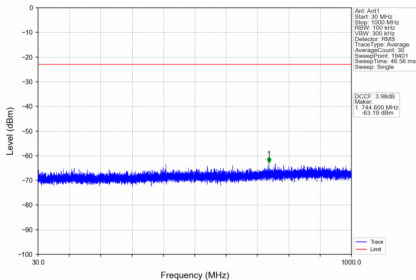
n77a_30kHz_SISO_NTNV_100MHz_CP-OFDM QPSK_3840MHz_Edge_1RB_Left
