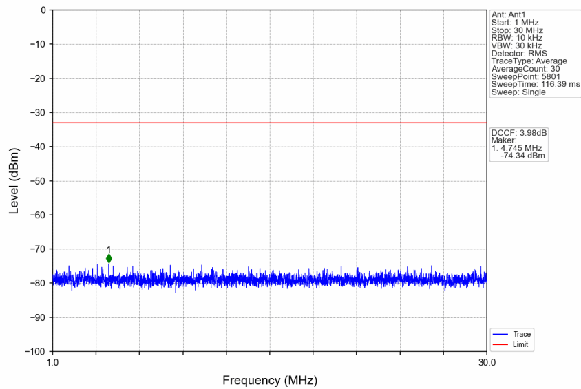
n77a_30kHz_SISO_NTNV_100MHz_DFT-s-OFDM QPSK_3840MHz_Edge_1RB_Left
