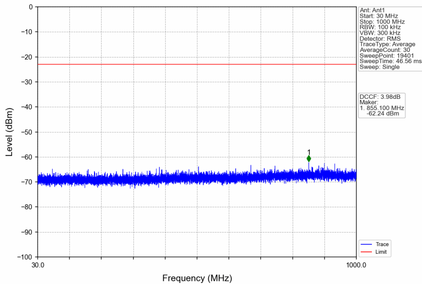
n77a_30kHz_SISO_NTNV_90MHz_CP-OFDM QPSK_3840MHz_Edge_1RB_Left
