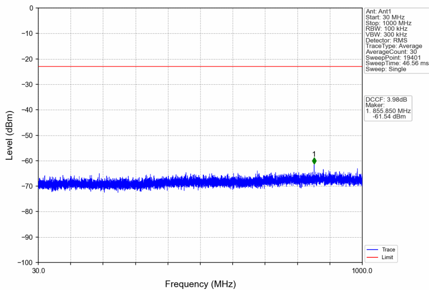
n77a_30kHz_SISO_NTNV_90MHz_DFT-s-OFDM_QPSK_3745.02MHz_Edge_1RB_Left
