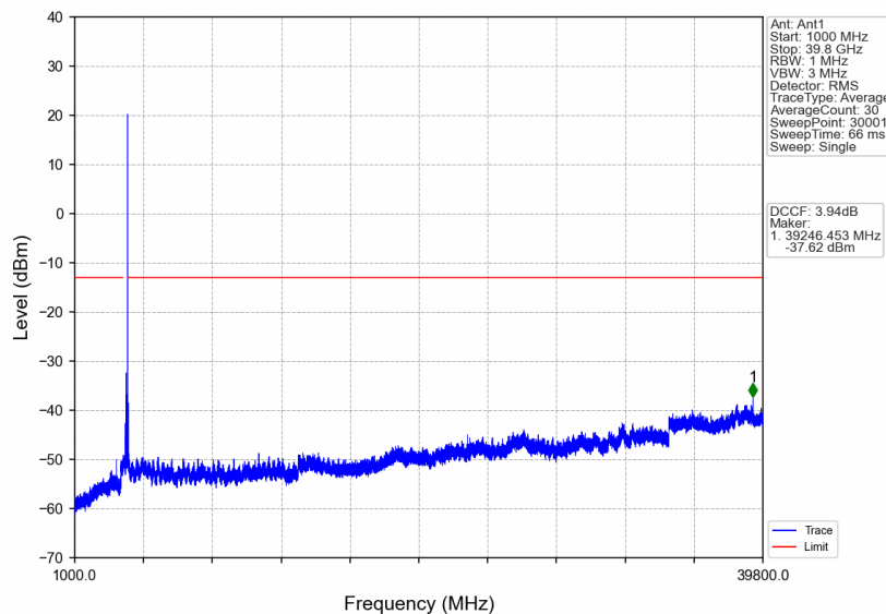
n77a_30kHz_SISO_NTNV_90MHz_CP-OFDM QPSK_3934.98MHz_Edge_1RB_Right
