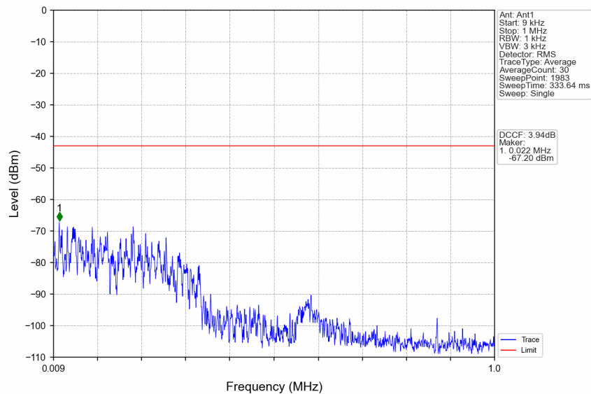
n77a_30kHz_SISO_NTNV_90MHz_CP-OFDM_QPSK_3934.98MHz_Edge_1RB_Right
