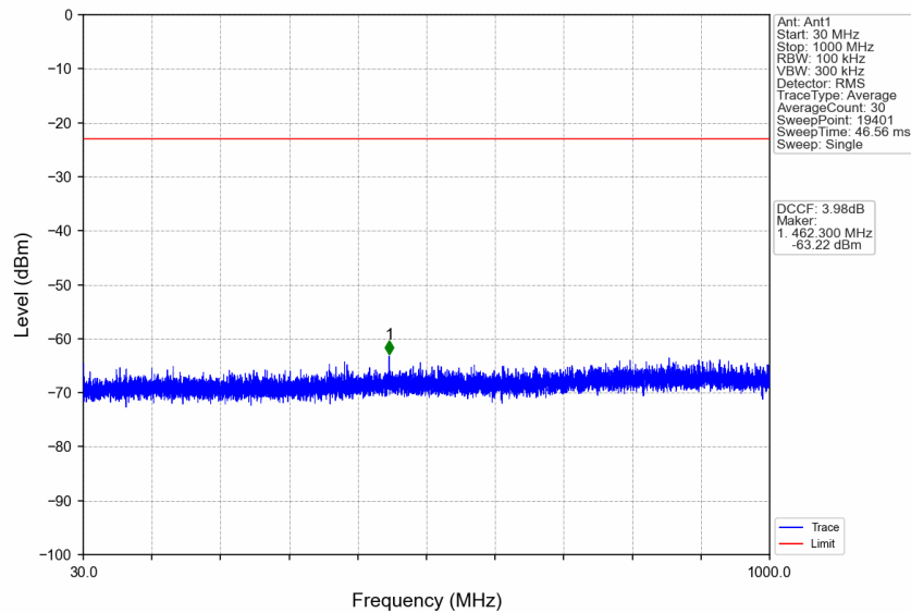
n77a_30kHz_SISO_NTNV_100MHz_DFT-s-OFDM QPSK_3750MHz_Edge_1RB_Left
