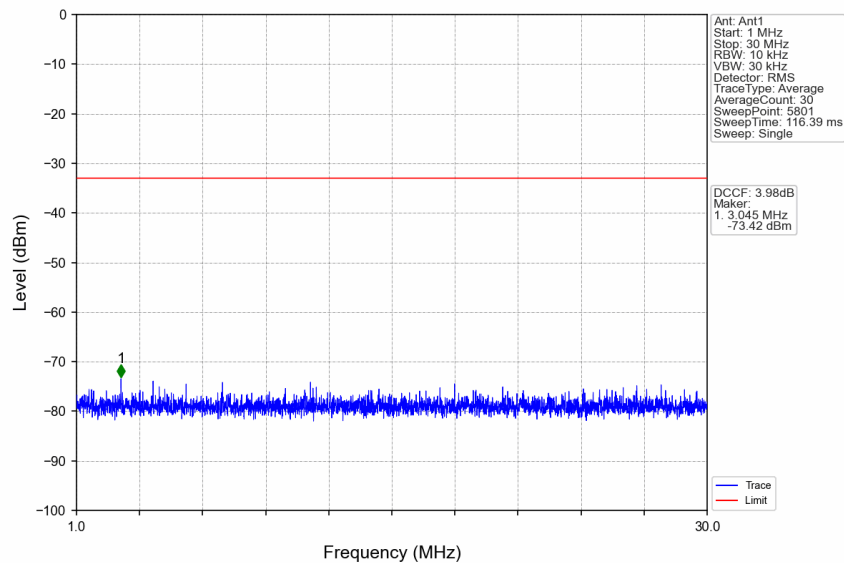
n77a_30kHz_SISO_NTNV_100MHz_DFT-s-OFDM PI/2 BPSK_3840MHz_Edge_1RB_Left
