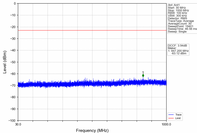
n77a_30kHz_SISO_NTNV_90MHz_CP-OFDM QPSK_3934.98MHz_Edge_1RB_Right
