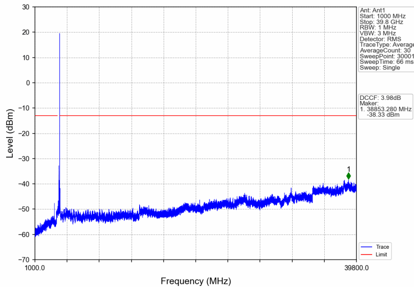
n77a_30kHz_SISO_NTNV_100MHz_DFT-s-OFDM PI/2 BPSK_3930MHz_Edge_1RB_Right
