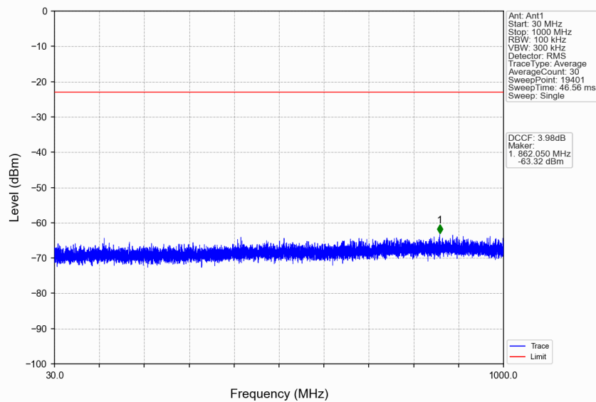
n77a_30kHz_SISO_NTNV_100MHz_DFT-s-OFDM QPSK_3840MHz_Edge_1RB_Left
