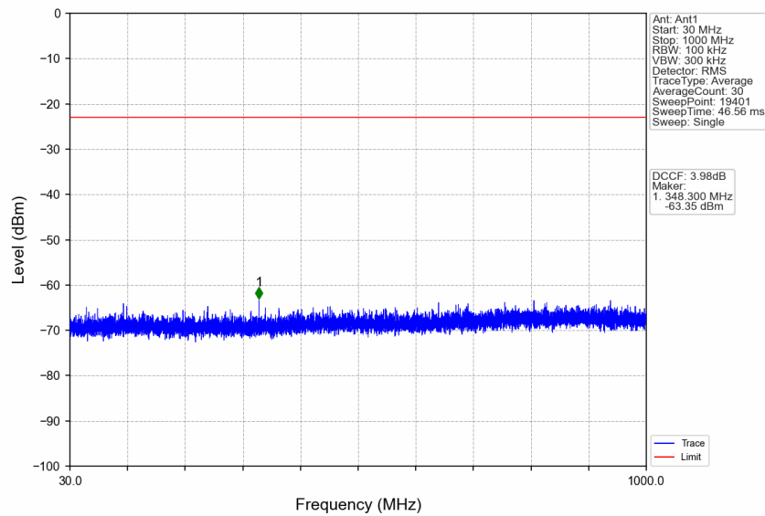
n77a_30kHz_SISO_NTNV_90MHz_DFT-s-OFDM PI/2 BPSK_3934.98MHz_Edge_1RB_Right
