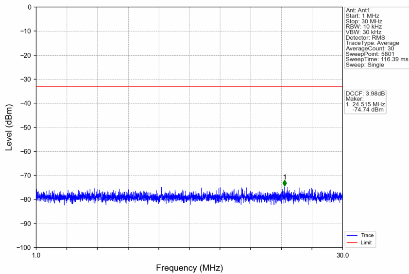
n77a_30kHz_SISO_NTNV_90MHz_DFT-s-OFDM_QPSK_3745.02MHz_Edge_1RB_Left
