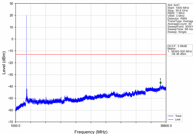
n77a_30kHz_SISO_NTNV_90MHz_CP-OFDM QPSK_3934.98MHz_Edge_1RB_Right
