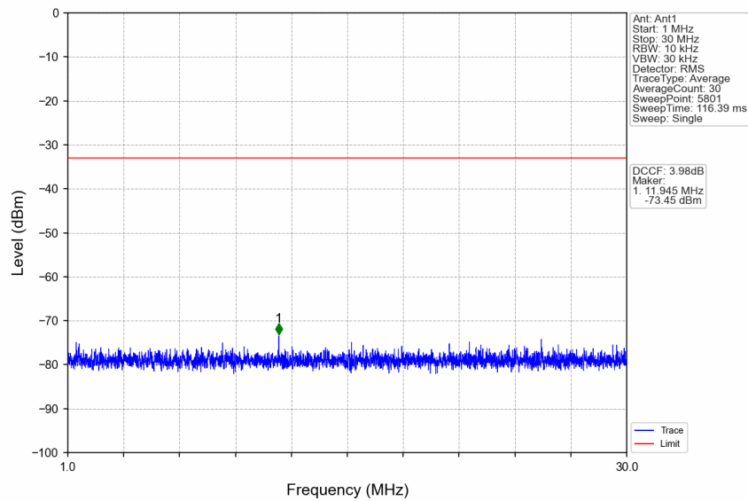
n77a_30kHz_SISO_NTNV_100MHz_DFT-s-OFDM PI/2 BPSK_3750MHz_Edge_1RB_Left
