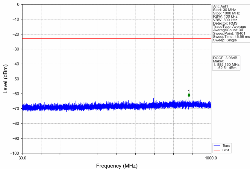
n77a_30kHz_SISO_NTNV_90MHz_DFT-s-OFDM QPSK_3934.98MHz_Edge_1RB_Right
