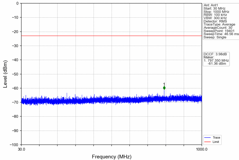
n77a_30kHz_SISO_NTNV_90MHz_DFT-s-OFDM_QPSK_3840MHz_Edge_1RB_Left
