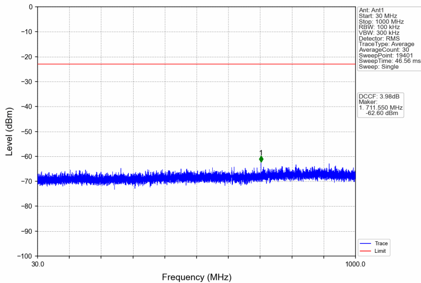
n77a_30kHz_SISO_NTNV_90MHz_CP-OFDM QPSK_3745.02MHz_Edge_1RB_Left
