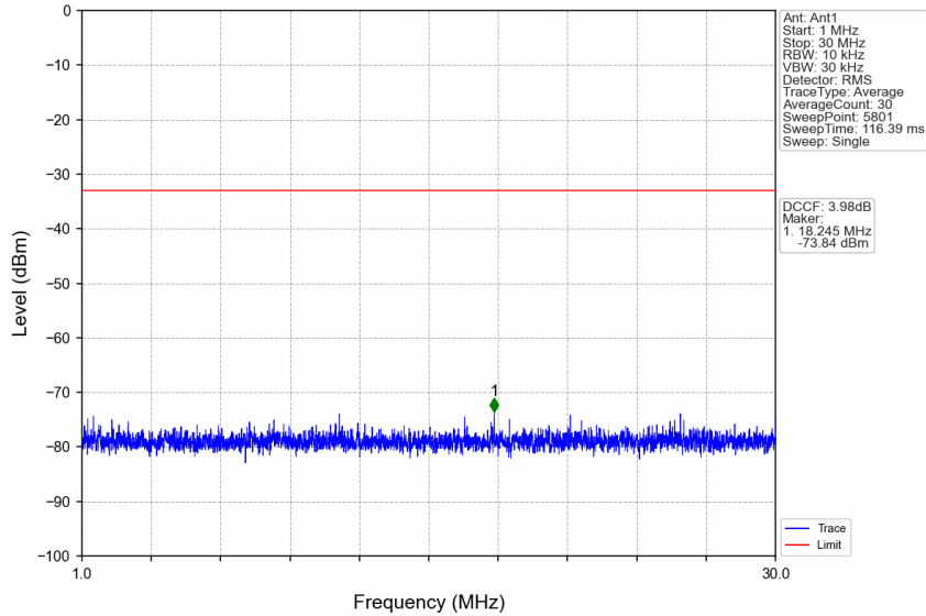
n77a_30kHz_SISO_NTNV_90MHz_DFT-s-OFDM_QPSK_3840MHz_Edge_1RB_Left
