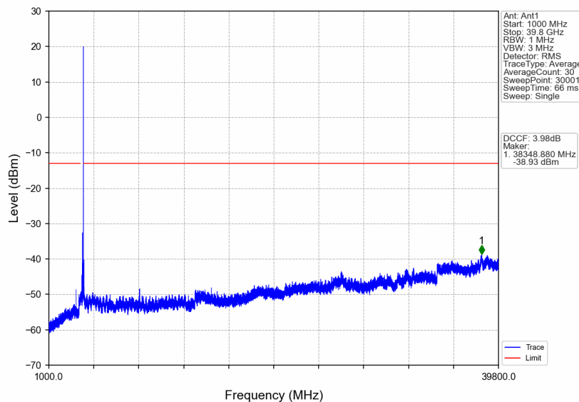
n77a_30kHz_SISO_NTNV_90MHz_DFT-s-OFDM QPSK_3934.98MHz_Edge_1RB_Right
