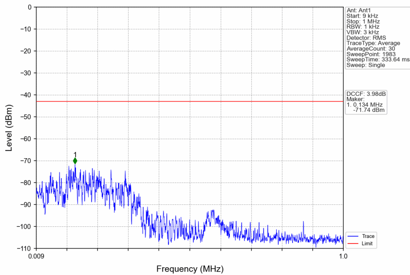
n77a_30kHz_SISO_NTNV_100MHz_DFT-s-OFDM_QPSK_3930MHz_Edge_1RB_Right
