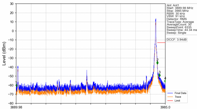
n77a_30kHz_SISO_NTNV_90MHz_CP-OFDM QPSK_3934.98MHz_Edge_1RB_Right
