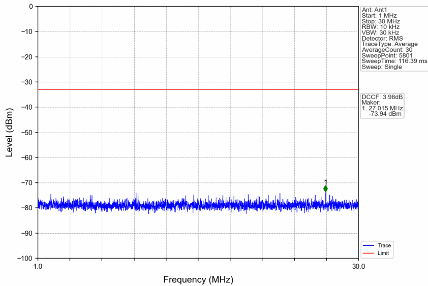
n77a_30kHz_SISO_NTNV_90MHz_CP-OFDM QPSK_3840MHz_Edge_1RB_Left
