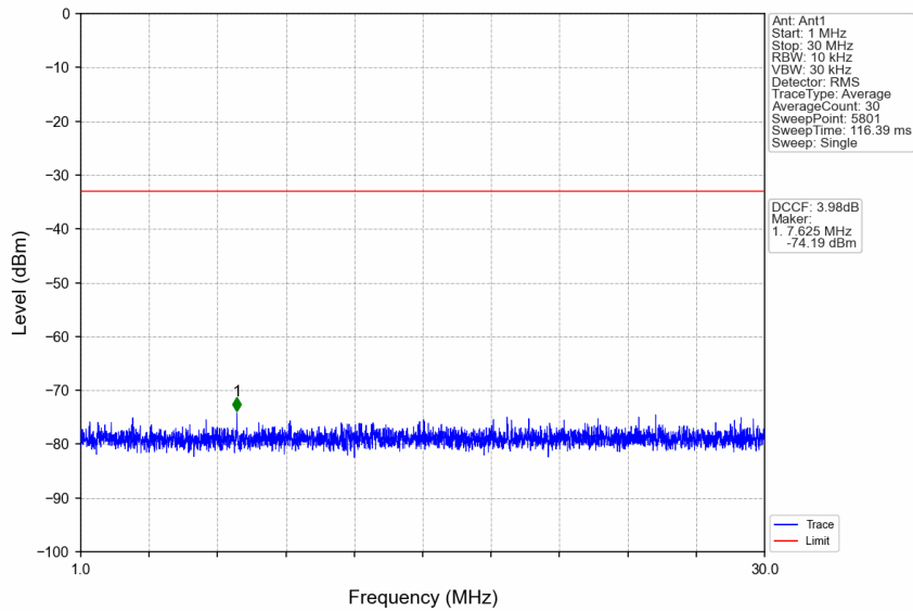
n77a_30kHz_SISO_NTNV_90MHz_CP-OFDM QPSK_3745.02MHz_Edge_1RB_Left
