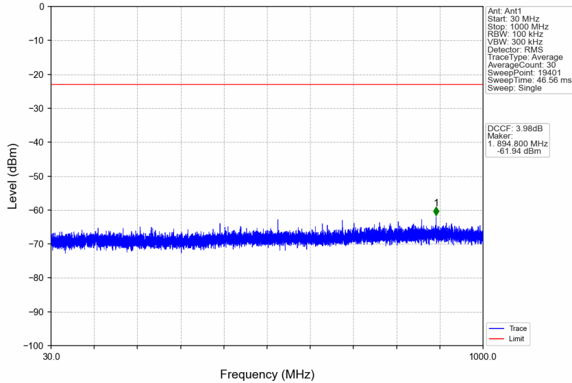
n77a_30kHz_SISO_NTNV_80MHz_DFT-s-OFDM PI/2 BPSK_3939.99MHz_Edge_1RB_Right
