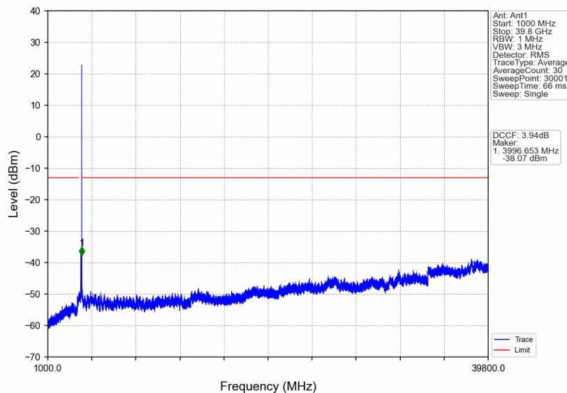
n77a_30kHz_SISO_NTNV_70MHz_DFT-s-OFDM_QPSK_3945MHz_Edge_1RB_Right
