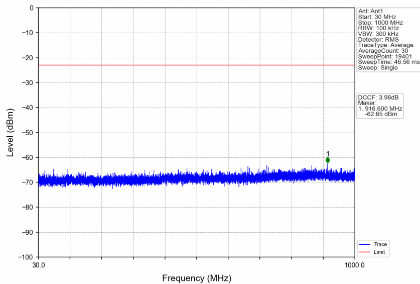
n77a_30kHz_SISO_NTNV_80MHz_DFT-s-OFDM_QPSK_3840MHz_Edge_1RB_Left
