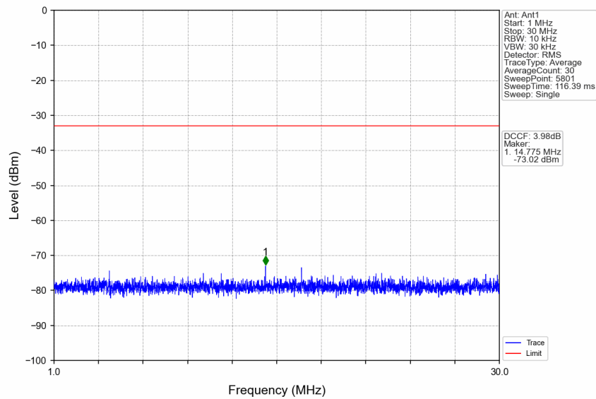
n77a_30kHz_SISO_NTNV_70MHz_CP-OFDM QPSK_3735MHz_Edge_1RB_Left
