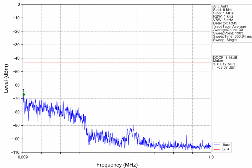
n77a_30kHz_SISO_NTNV_80MHz_CP-OFDM QPSK_3939.99MHz_Edge_1RB_Right
