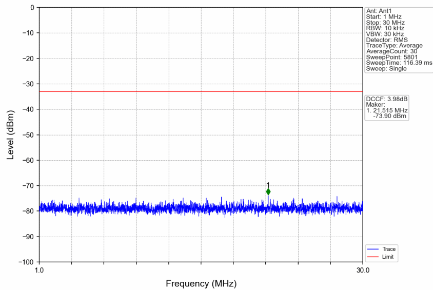
n77a_30kHz_SISO_NTNV_80MHz_CP-OFDM QPSK_3840MHz_Edge_1RB_Left
