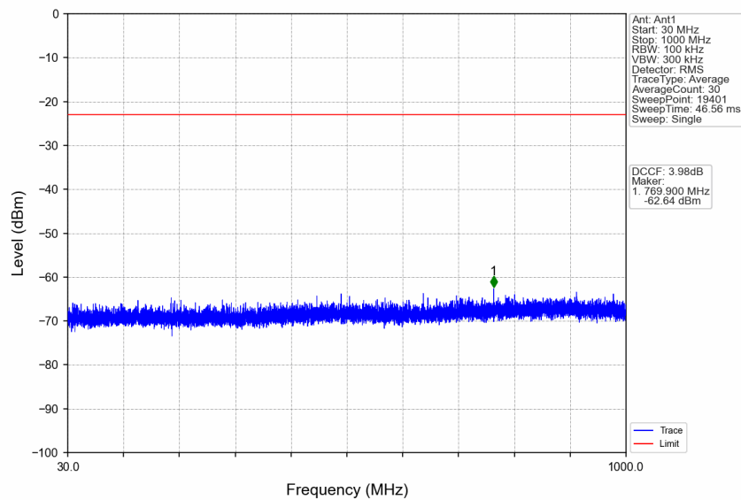
n77a_30kHz_SISO_NTNV_80MHz_CP-OFDM QPSK_3840MHz_Edge_1RB_Left
