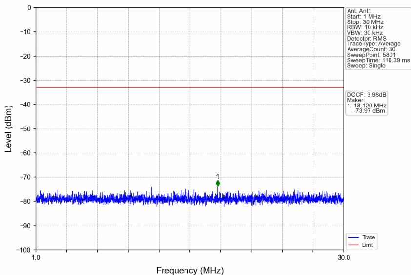
n77a_30kHz_SISO_NTNV_80MHz_DFT-s-OFDM QPSK_3939.99MHz_Edge_1RB_Right
