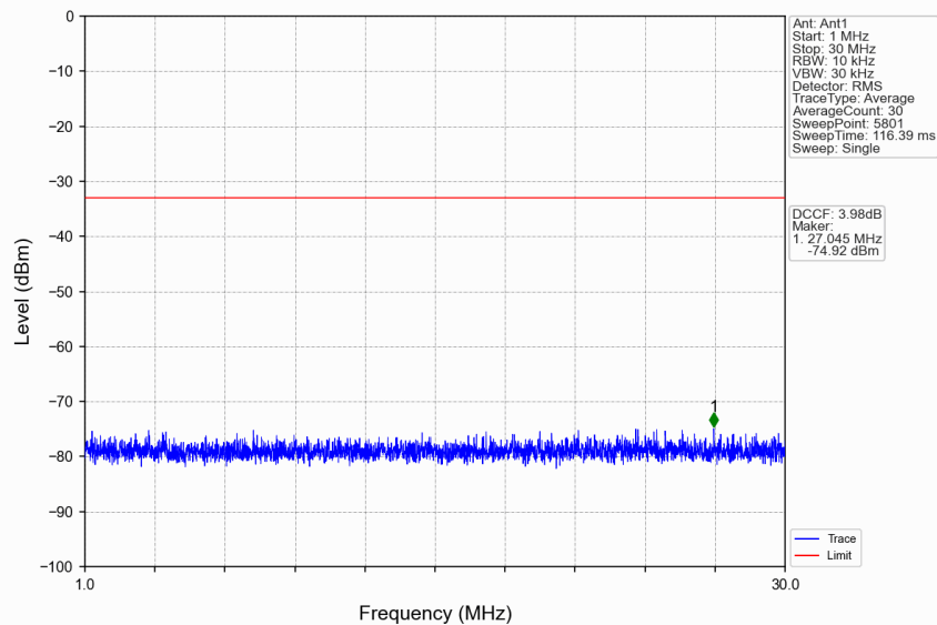
n77a_30kHz_SISO_NTNV_70MHz_CP-OFDM QPSK_3840MHz_Edge_1RB_Left
