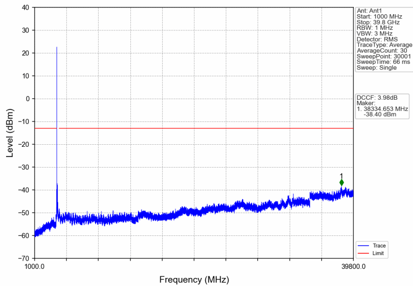
n77a_30kHz_SISO_NTNV_70MHz_CP-OFDM QPSK_3735MHz_Outer_Full
