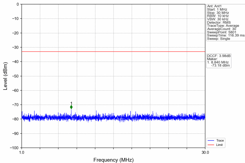
n77a_30kHz_SISO_NTNV_80MHz_DFT-s-OFDM_QPSK_3740.01MHz_Edge_1RB_Left
