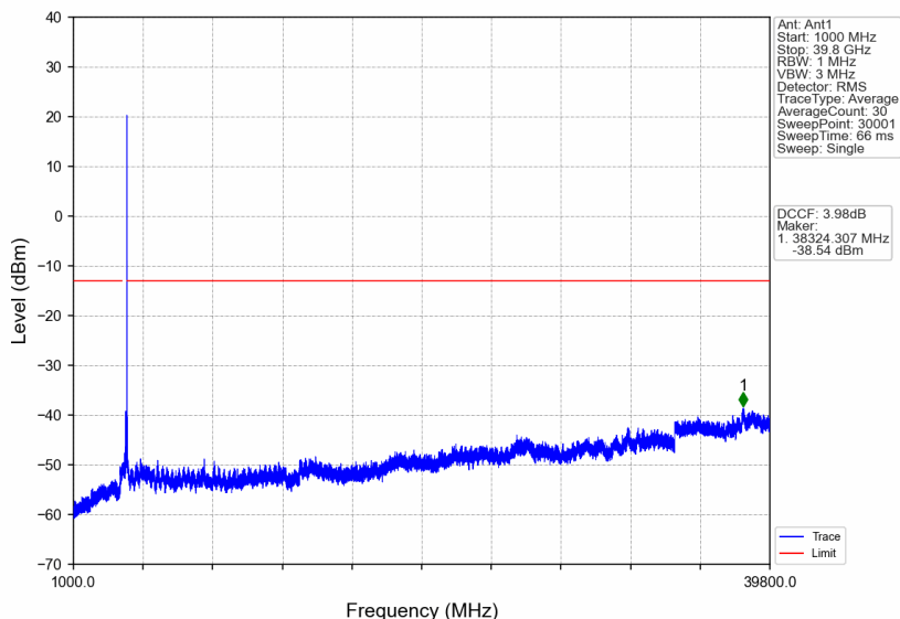
n77a_30kHz_SISO_NTNV_70MHz_CP-OFDM QPSK_3945MHz_Edge_1RB_Right
