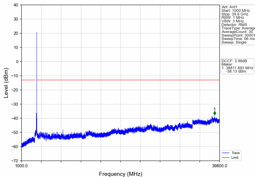
n77a_30kHz_SISO_NTNV_80MHz_CP-OFDM QPSK_3939.99MHz_Edge_1RB_Right
