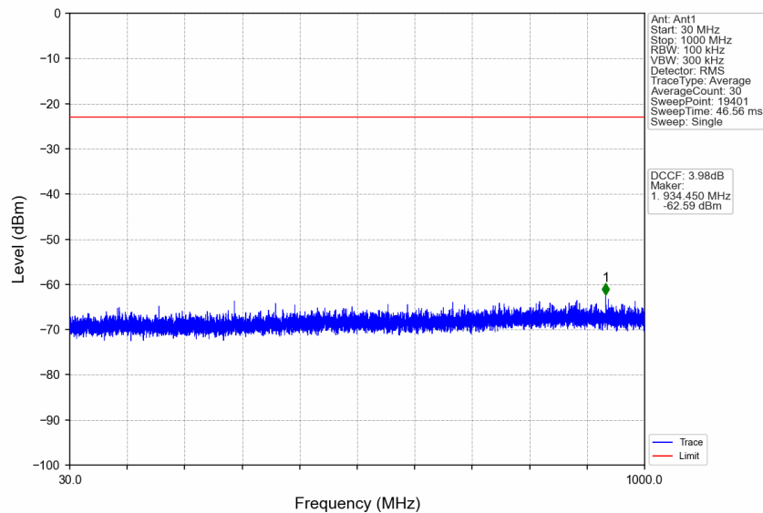
n77a_30kHz_SISO_NTNV_80MHz_CP-OFDM QPSK_3939.99MHz_Edge_1RB_Right
