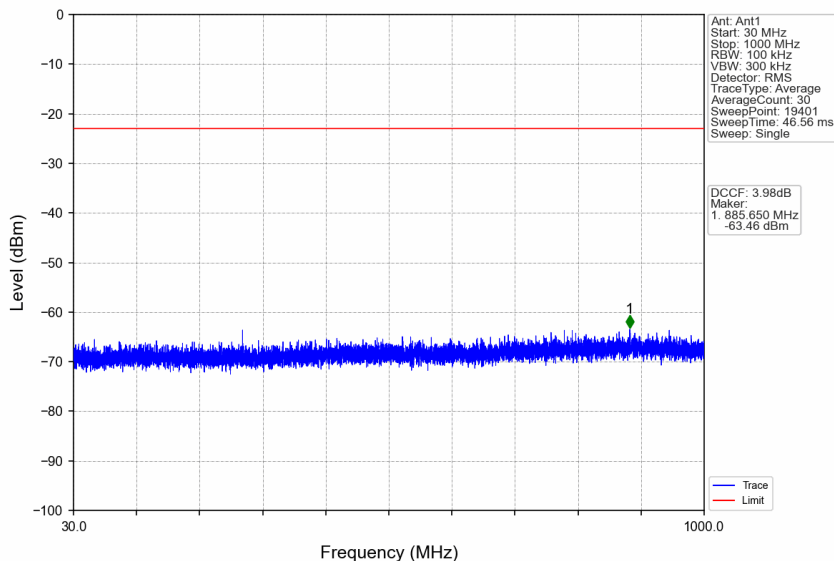
n77a_30kHz_SISO_NTNV_70MHz_CP-OFDM QPSK_3945MHz_Edge_1RB_Right
