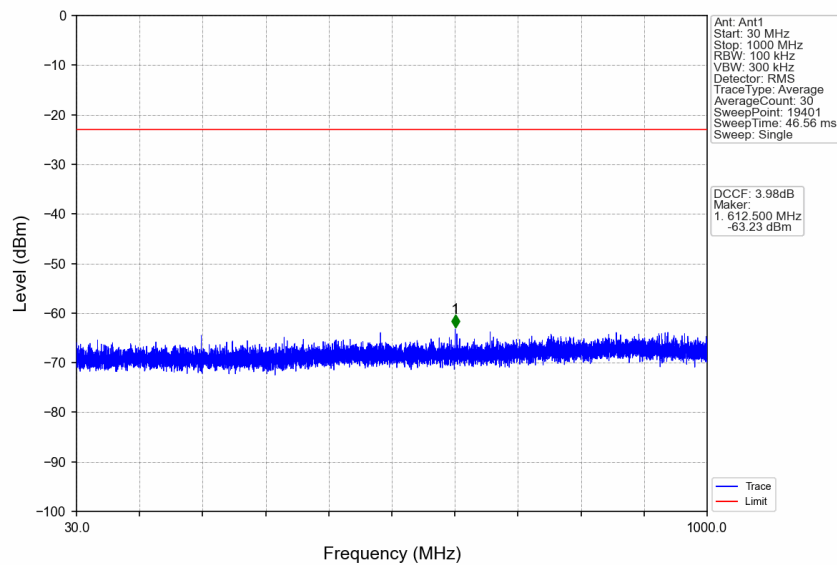
n77a_30kHz_SISO_NTNV_80MHz_CP-OFDM_QPSK_3740.01MHz_Edge_1RB_Left
