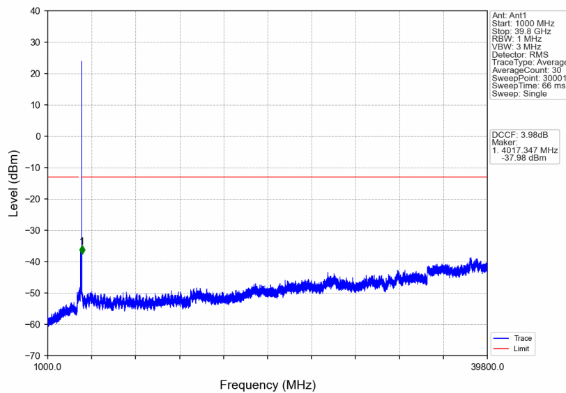
n77a_30kHz_SISO_NTNV_80MHz_DFT-s-OFDM QPSK_3939.99MHz_Edge_1RB_Right
