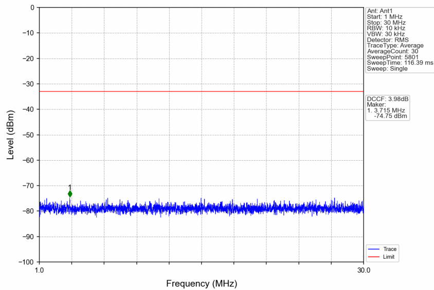
n77a_30kHz_SISO_NTNV_80MHz_DFT-s-OFDM_QPSK_3840MHz_Edge_1RB_Left
