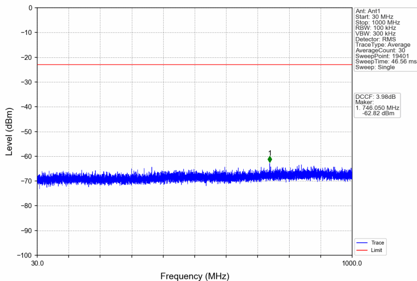
n77a_30kHz_SISO_NTNV_80MHz_DFT-s-OFDM_QPSK_3740.01MHz_Edge_1RB_Left
