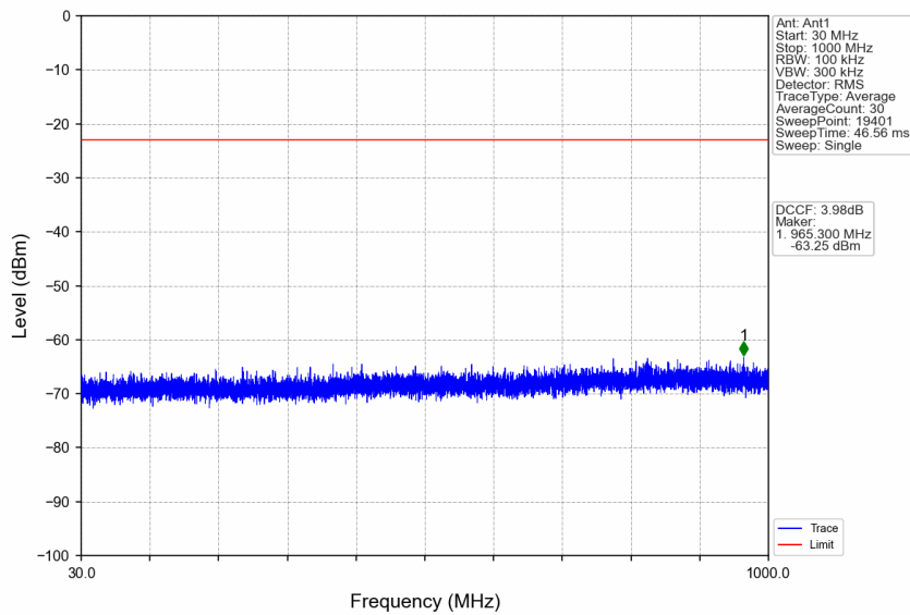
n77a_30kHz_SISO_NTNV_80MHz_DFT-s-OFDM QPSK_3939.99MHz_Edge_1RB_Right
