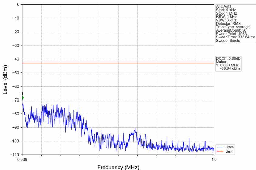
n77a_30kHz_SISO_NTNV_80MHz_DFT-s-OFDM QPSK_3939.99MHz_Edge_1RB_Right
