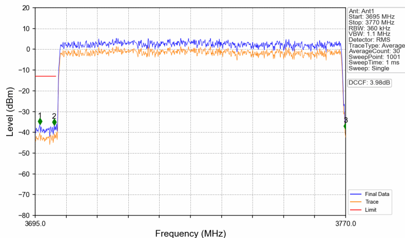
n77a_30kHz_SISO_NTNV_70MHz_CP-OFDM QPSK_3735MHz_Outer_Full
