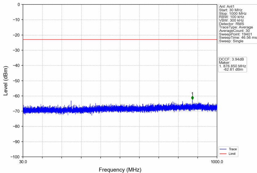
n77a_30kHz_SISO_NTNV_70MHz_DFT-s-OFDM_QPSK_3945MHz_Edge_1RB_Right
