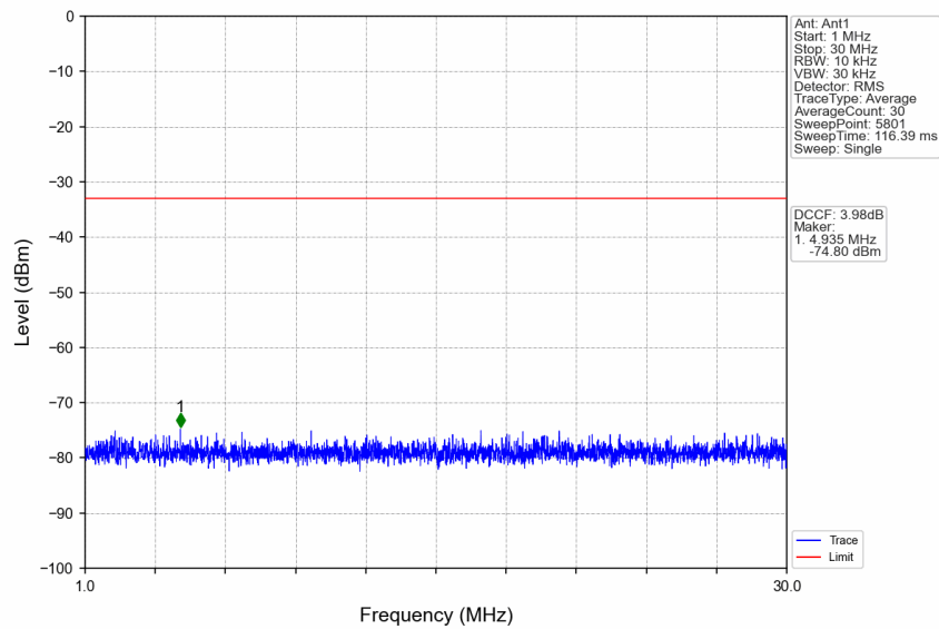
n77a_30kHz_SISO_NTNV_80MHz_CP-OFDM_QPSK_3740.01MHz_Edge_1RB_Left
