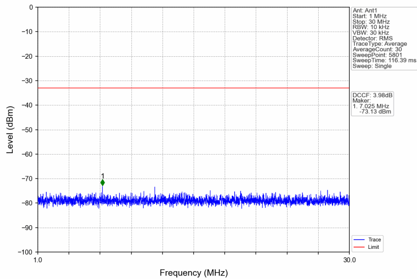
n77a_30kHz_SISO_NTNV_70MHz_DFT-s-OFDM_QPSK_3840MHz_Edge_1RB_Left
