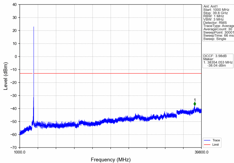
n77a_30kHz_SISO_NTNV_60MHz_DFT-s-OFDM QPSK_3949.98MHz_Edge_1RB_Right
