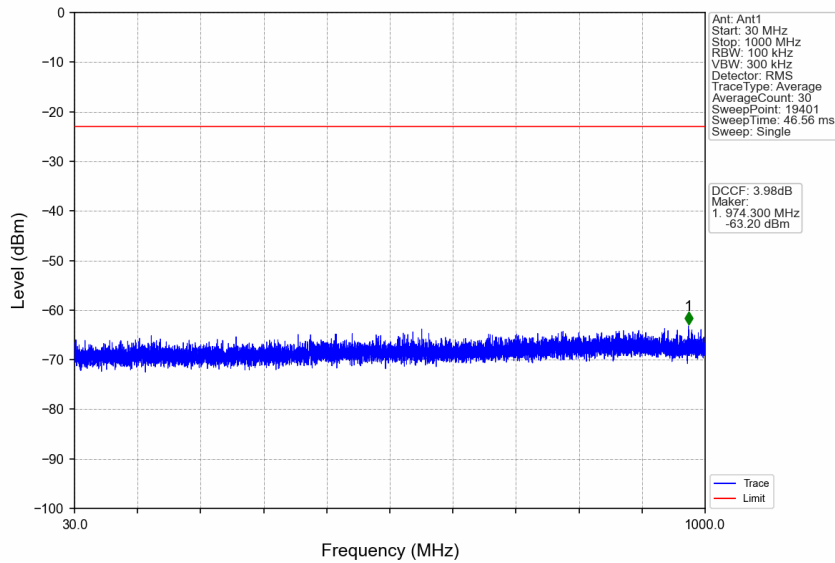
n77a_30kHz_SISO_NTNV_60MHz_CP-OFDM QPSK_3949.98MHz_Edge_1RB_Right
