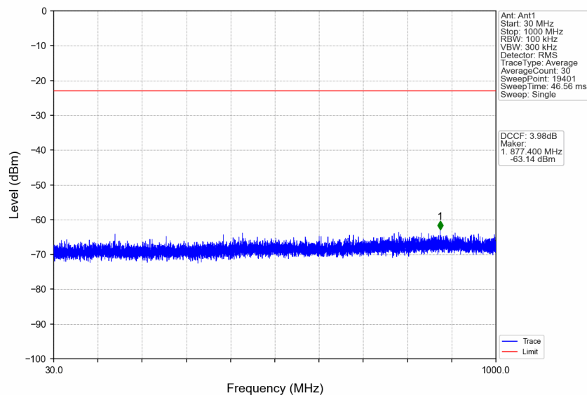
n77a_30kHz_SISO_NTNV_60MHz_CP-OFDM QPSK_3840MHz_Edge_1RB_Left
