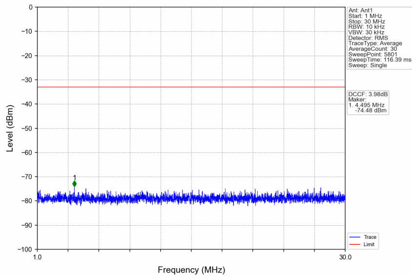
n77a_30kHz_SISO_NTNV_60MHz_DFT-s-OFDM_QPSK_3730.02MHz_Edge_1RB_Left
