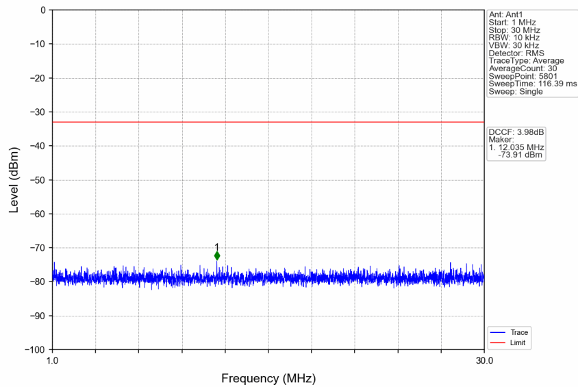
n77a_30kHz_SISO_NTNV_60MHz_CP-OFDM QPSK_3730.02MHz_Edge_1RB_Left
