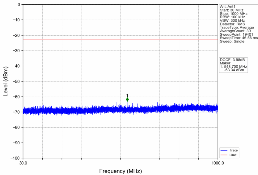
n77a_30kHz_SISO_NTNV_70MHz_DFT-s-OFDM PI/2 BPSK_3945MHz_Edge_1RB_Right
