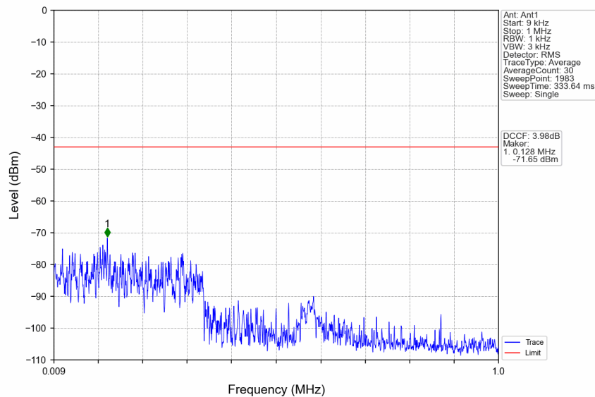
n77a_30kHz_SISO_NTNV_60MHz_DFT-s-OFDM PI/2 BPSK_3949.98MHz_Edge_1RB_Right
