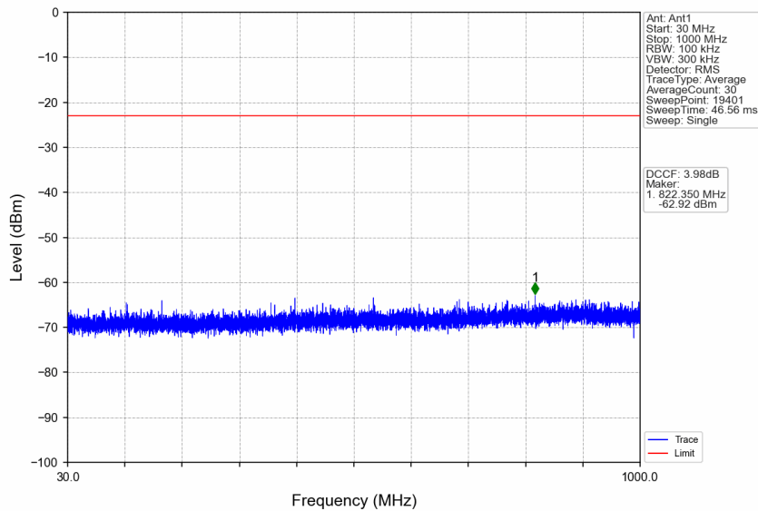
n77a_30kHz_SISO_NTNV_70MHz_DFT-s-OFDM_QPSK_3735MHz_Edge_1RB_Left
