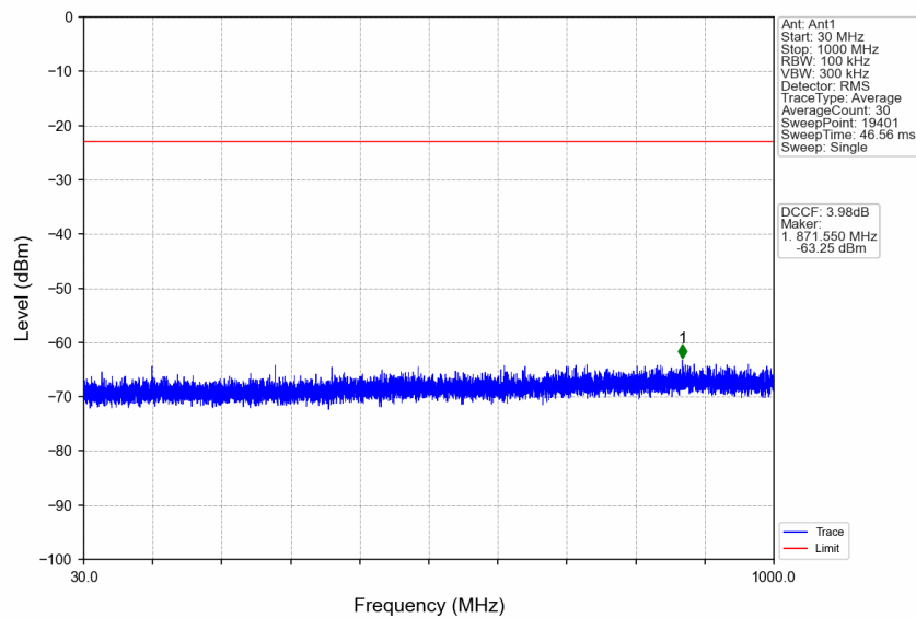
n77a_30kHz_SISO_NTNV_60MHz_DFT-s-OFDM_QPSK_3730.02MHz_Edge_1RB_Left
