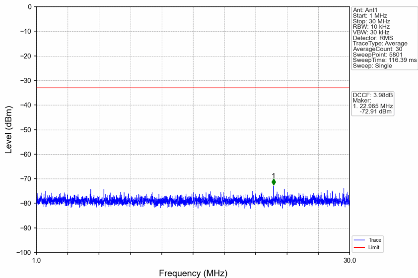
n77a_30kHz_SISO_NTNV_60MHz_DFT-s-OFDM QPSK_3949.98MHz_Edge_1RB_Right
