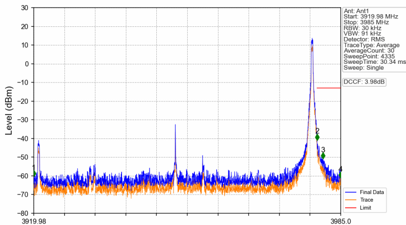
n77a_30kHz_SISO_NTNV_60MHz_CP-OFDM QPSK_3949.98MHz_Edge_1RB_Right
