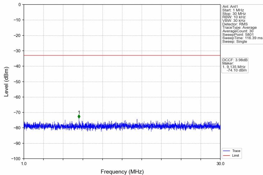
n77a_30kHz_SISO_NTNV_60MHz_CP-OFDM QPSK_3840MHz_Edge_1RB_Left
