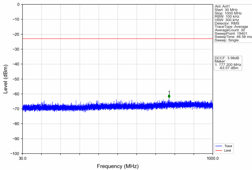
n77a_30kHz_SISO_NTNV_60MHz_DFT-s-OFDM QPSK_3949.98MHz_Edge_1RB_Right
