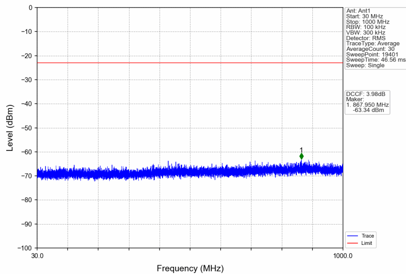
n77a_30kHz_SISO_NTNV_60MHz_DFT-s-OFDM_QPSK_3840MHz_Edge_1RB_Left
