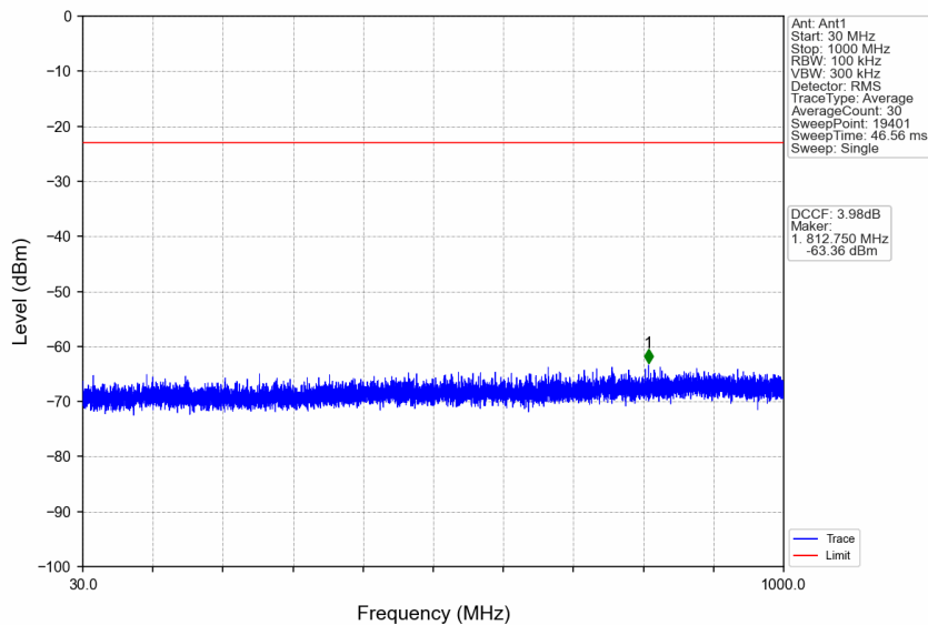
n77a_30kHz_SISO_NTNV_50MHz_CP-OFDM QPSK_3954.99MHz_Edge_1RB_Right
