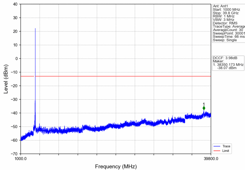
n77a_30kHz_SISO_NTNV_60MHz_CP-OFDM QPSK_3949.98MHz_Edge_1RB_Right
