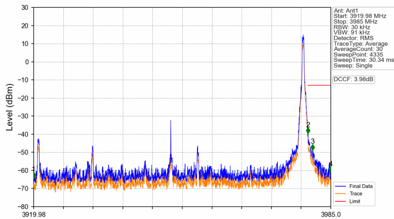
n77a_30kHz_SISO_NTNV_60MHz_DFT-s-OFDM PI/2 BPSK_3949.98MHz_Edge_1RB_Right
