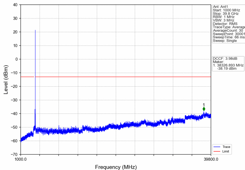
n77a_30kHz_SISO_NTNV_70MHz_DFT-s-OFDM PI/2 BPSK_3945MHz_Edge_1RB_Right
