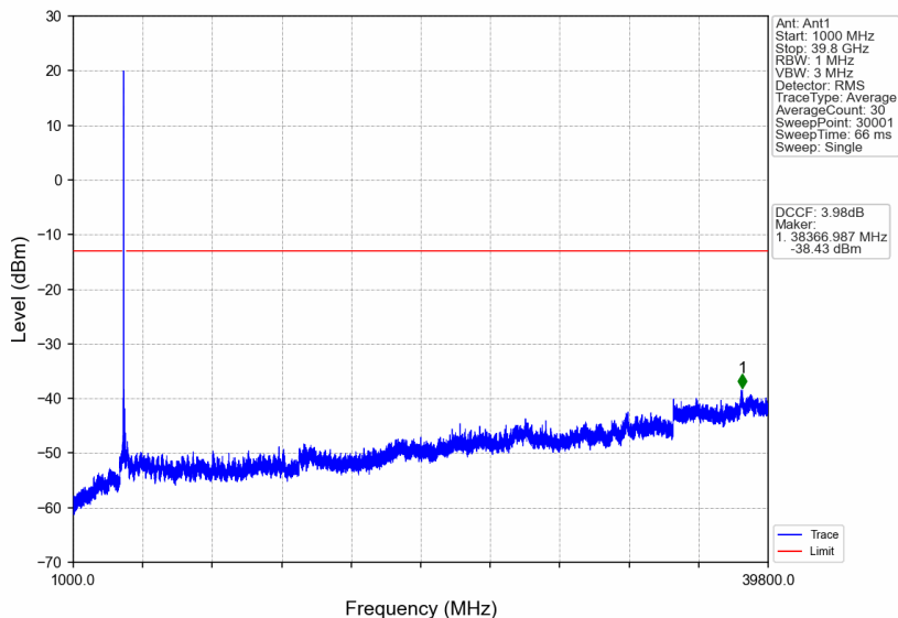
n77a_30kHz_SISO_NTNV_60MHz_CP-OFDM QPSK_3949.98MHz_Edge_1RB_Right
