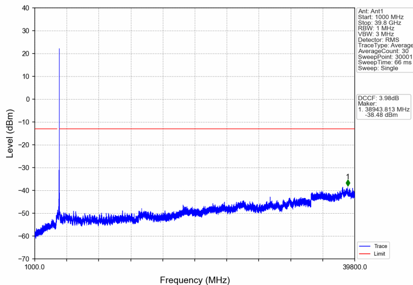
n77a_30kHz_SISO_NTNV_50MHz_CP-OFDM QPSK_3954.99MHz_Edge_1RB_Right
