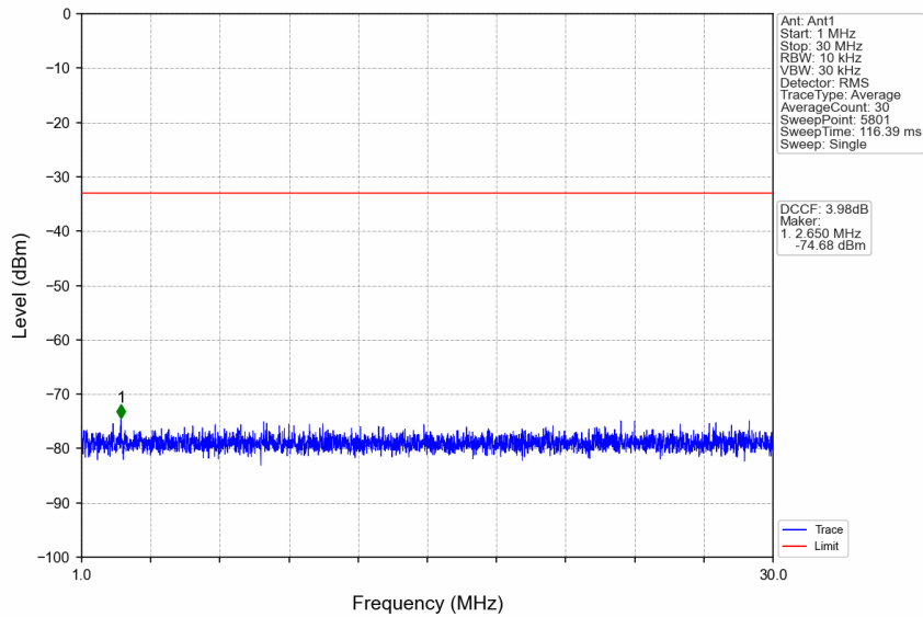
n77a_30kHz_SISO_NTNV_70MHz_DFT-s-OFDM_QPSK_3735MHz_Edge_1RB_Left
