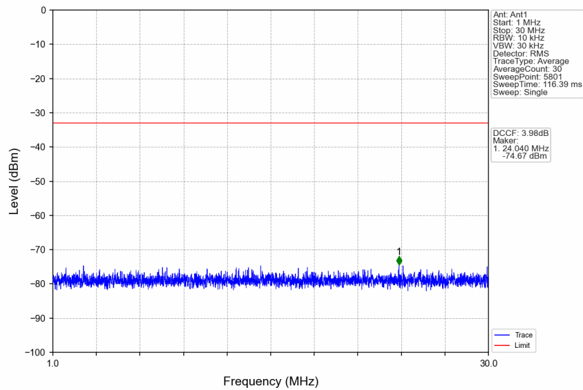
n77a_30kHz_SISO_NTNV_60MHz_DFT-s-OFDM_QPSK_3840MHz_Edge_1RB_Left
