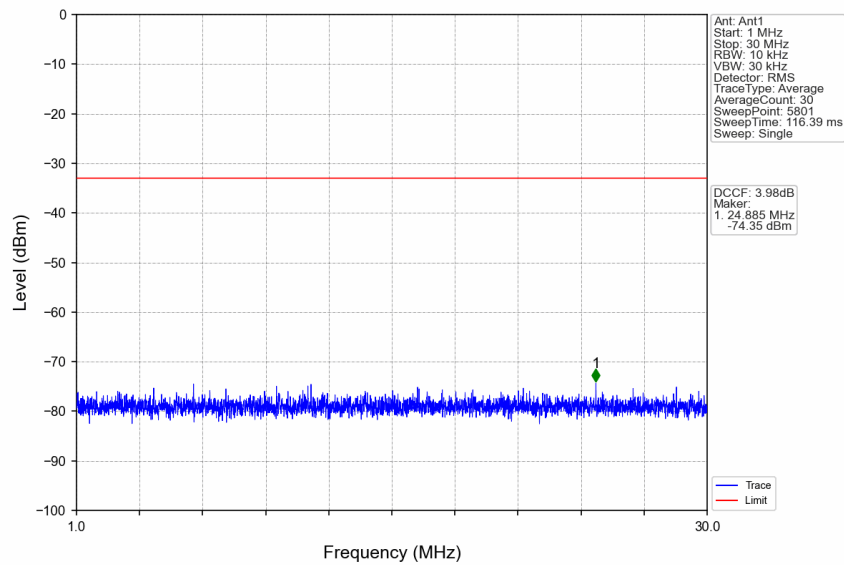
n77a_30kHz_SISO_NTNV_50MHz_CP-OFDM QPSK_3840MHz_Edge_1RB_Left
