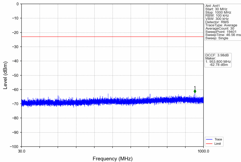
n77a_30kHz_SISO_NTNV_50MHz_DFT-s-OFDM_QPSK_3725.01MHz_Edge_1RB_Left
