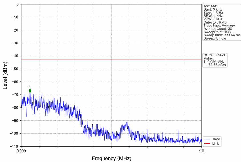
n77a_30kHz_SISO_NTNV_40MHz_CP-OFDM QPSK_3960MHz_Edge_1RB_Right
