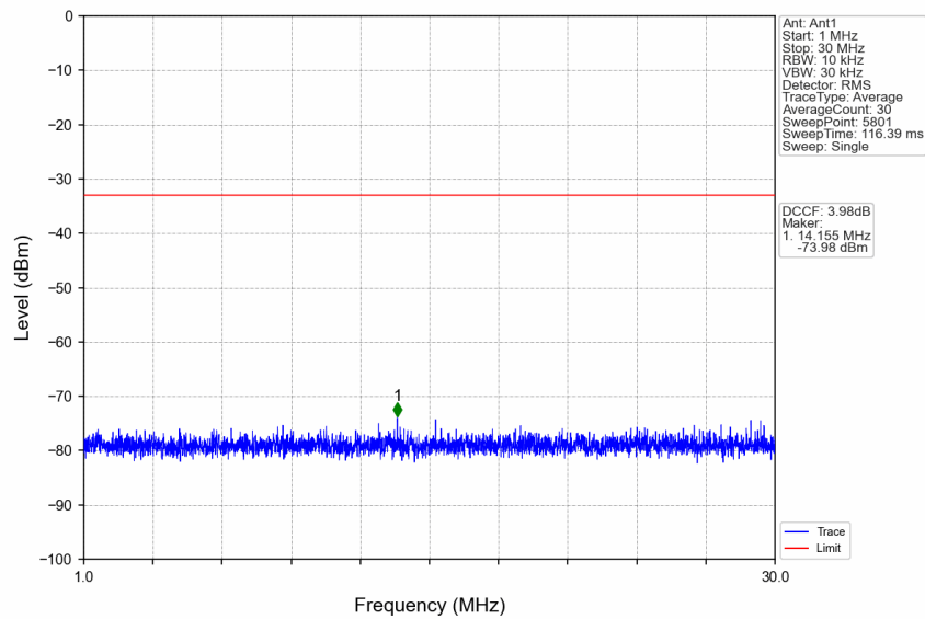
n77a_30kHz_SISO_NTNV_40MHz_CP-OFDM QPSK_3720MHz_Edge_1RB_Left
