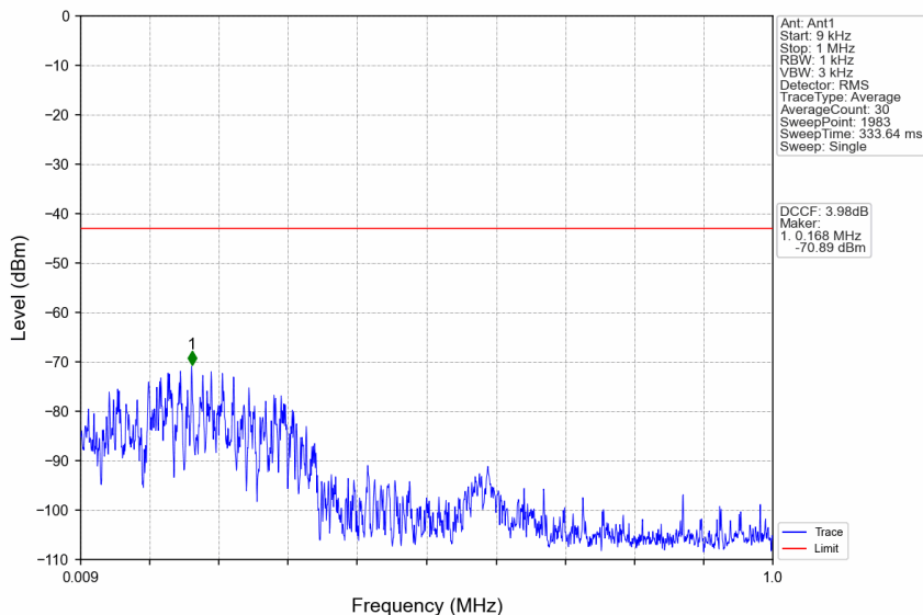
n77a_30kHz_SISO_NTNV_40MHz_DFT-s-OFDM_QPSK_3960MHz_Edge_1RB_Right
