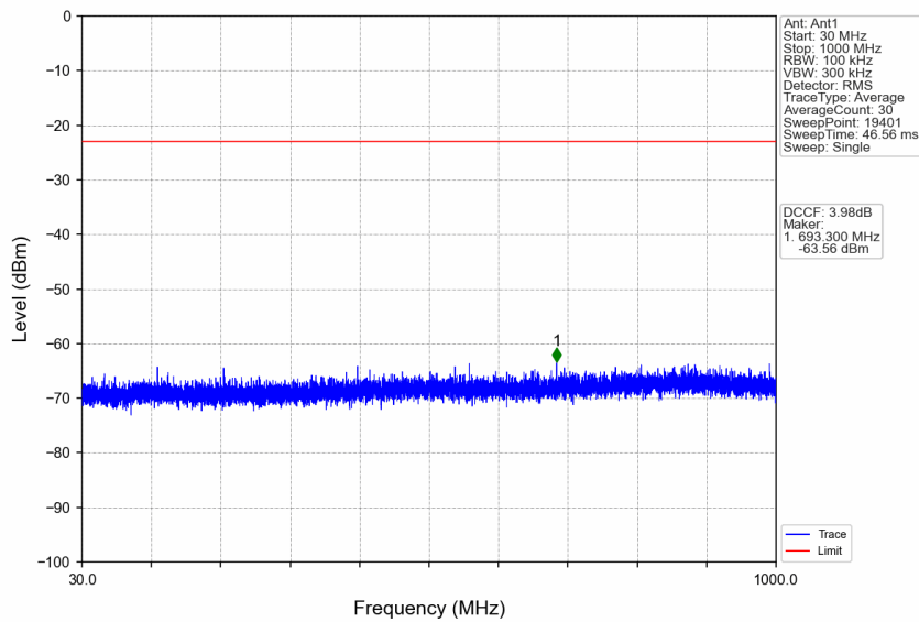
n77a_30kHz_SISO_NTNV_50MHz_DFT-s-OFDM QPSK_3954.99MHz_Edge_1RB_Right
