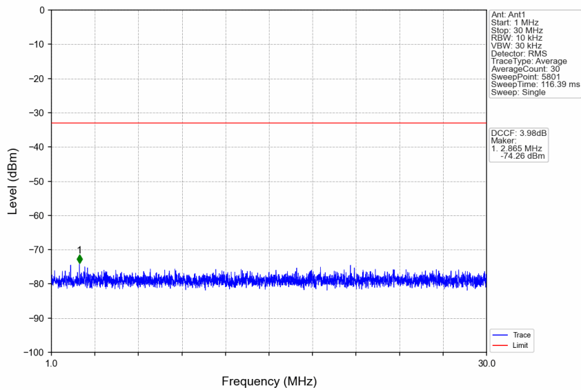
n77a_30kHz_SISO_NTNV_50MHz_CP-OFDM QPSK_3725.01MHz_Edge_1RB_Left
