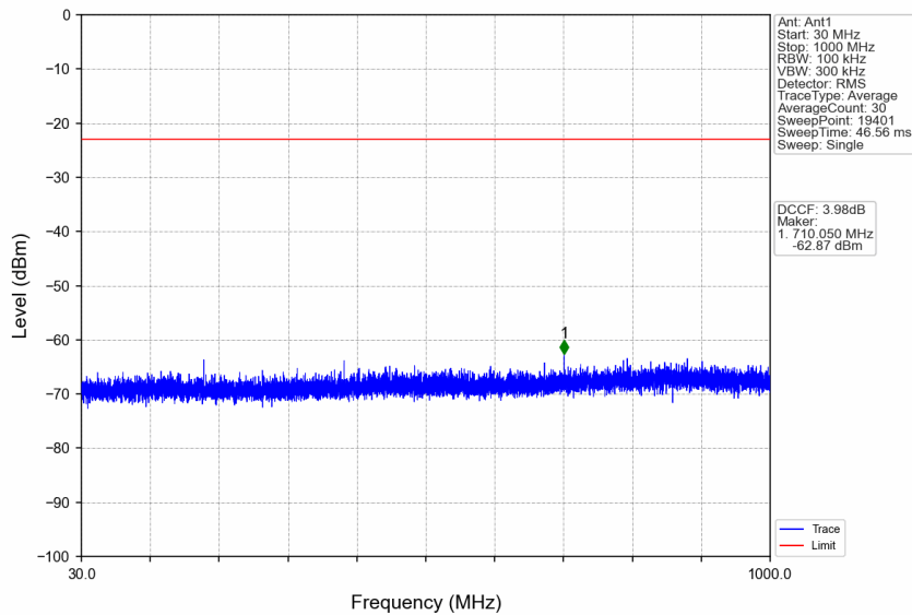
n77a_30kHz_SISO_NTNV_40MHz_DFT-s-OFDM_QPSK_3840MHz_Edge_1RB_Left
