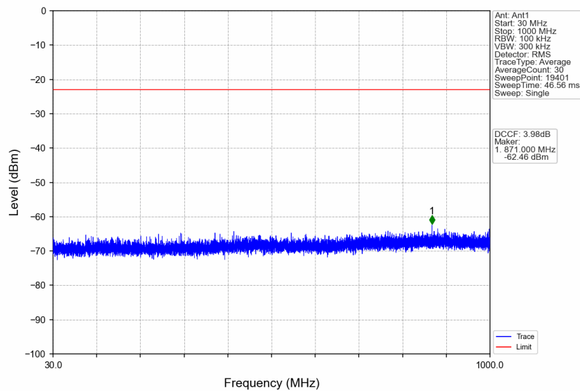
n77a_30kHz_SISO_NTNV_40MHz_CP-OFDM QPSK_3840MHz_Edge_1RB_Left
