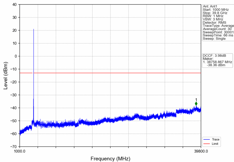
n77a_30kHz_SISO_NTNV_50MHz_DFT-s-OFDM QPSK_3954.99MHz_Edge_1RB_Right
