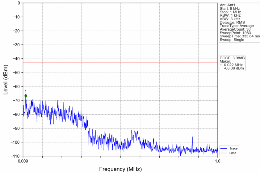
n77a_30kHz_SISO_NTNV_50MHz_CP-OFDM QPSK_3954.99MHz_Edge_1RB_Right
