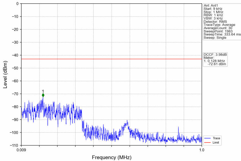
n77a_30kHz_SISO_NTNV_50MHz_DFT-s-OFDM PI/2 BPSK_3954.99MHz_Edge_1RB_Right
