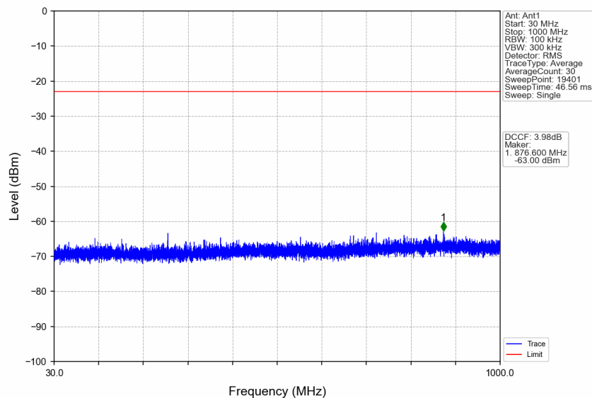
n77a_30kHz_SISO_NTNV_50MHz_DFT-s-OFDM_QPSK_3840MHz_Edge_1RB_Left
