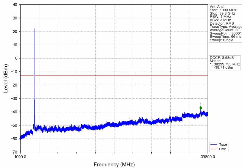
n77a_30kHz_SISO_NTNV_40MHz_CP-OFDM QPSK_3960MHz_Edge_1RB_Right
