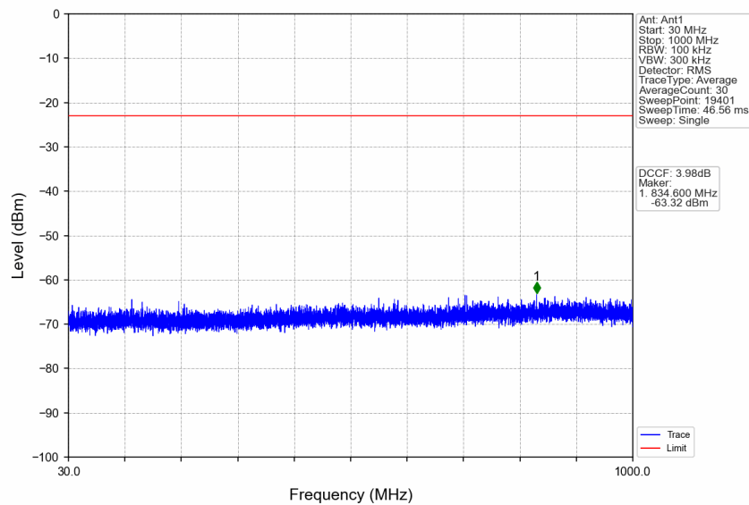
n77a_30kHz_SISO_NTNV_40MHz_CP-OFDM QPSK_3720MHz_Edge_1RB_Left
