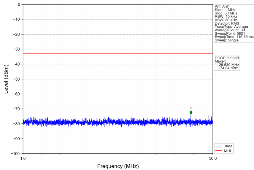
n77a_30kHz_SISO_NTNV_40MHz_CP-OFDM QPSK_3840MHz_Edge_1RB_Left
