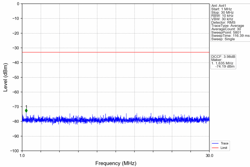
n77a_30kHz_SISO_NTNV_50MHz_DFT-s-OFDM_QPSK_3725.01MHz_Edge_1RB_Left
