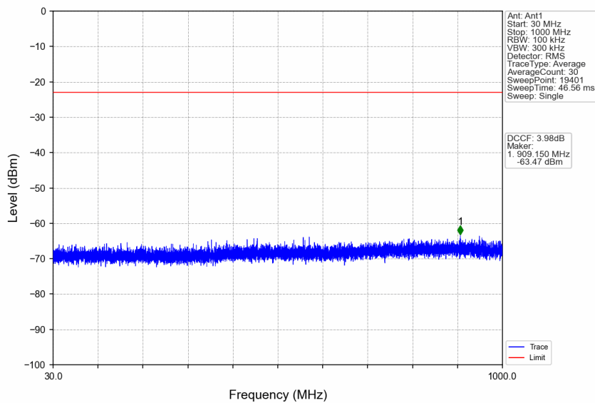
n77a_30kHz_SISO_NTNV_50MHz_CP-OFDM QPSK_3725.01MHz_Edge_1RB_Left
