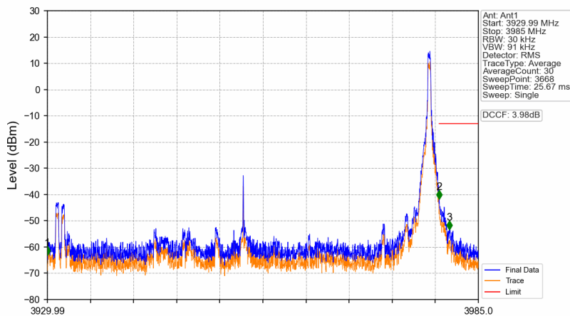
n77a_30kHz_SISO_NTNV_50MHz_CP-OFDM QPSK_3954.99MHz_Edge_1RB_Right
