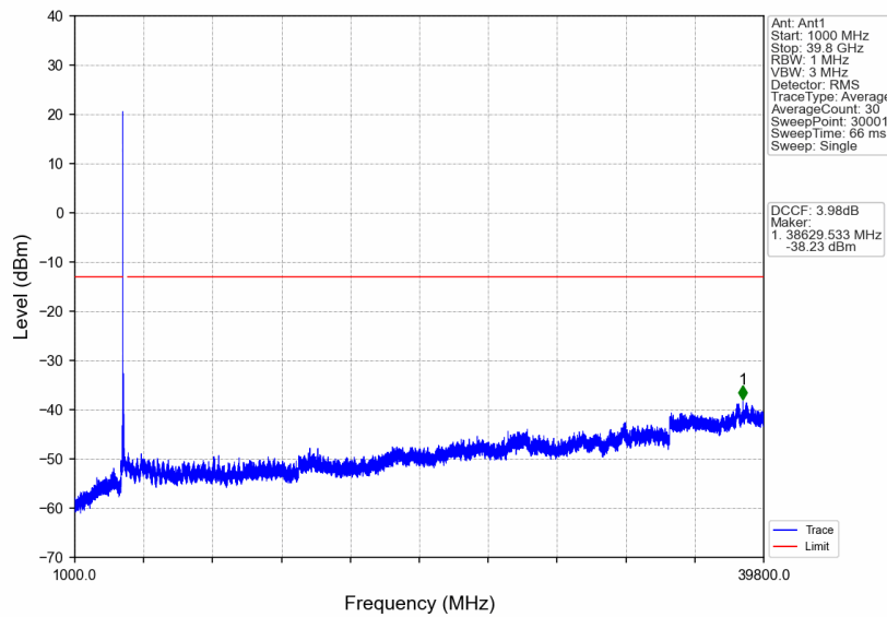
n77a_30kHz_SISO_NTNV_40MHz_CP-OFDM QPSK_3720MHz_Outer_Full
