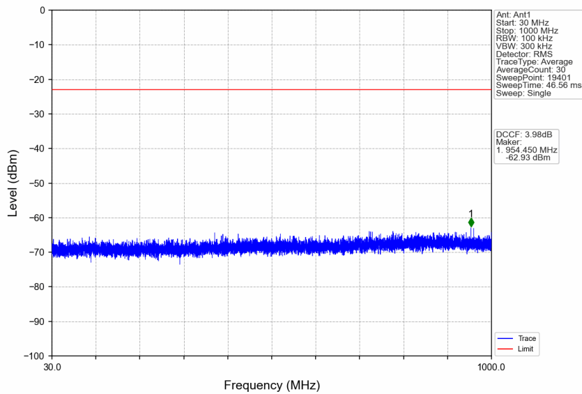
n77a_30kHz_SISO_NTNV_40MHz_CP-OFDM QPSK_3960MHz_Edge_1RB_Right
