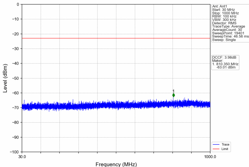
n77a_30kHz_SISO_NTNV_40MHz_DFT-s-OFDM_QPSK_3960MHz_Edge_1RB_Right
