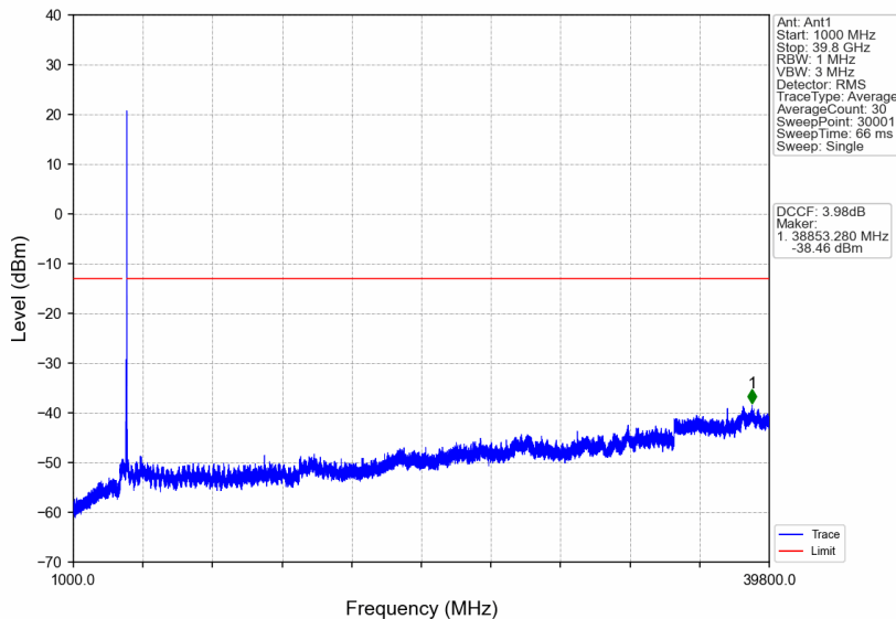
n77a_30kHz_SISO_NTNV_40MHz_DFT-s-OFDM_QPSK_3960MHz_Edge_1RB_Right
