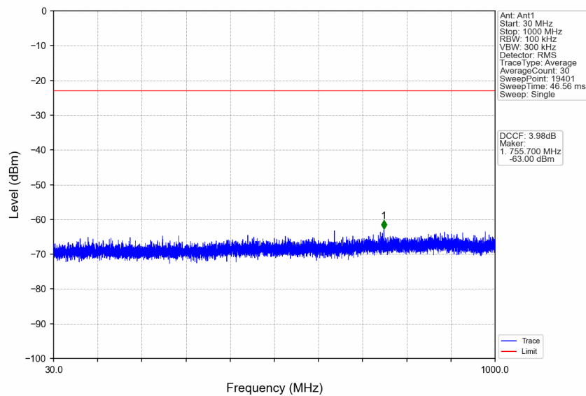
n77a_30kHz_SISO_NTNV_50MHz_CP-OFDM QPSK_3840MHz_Edge_1RB_Left
