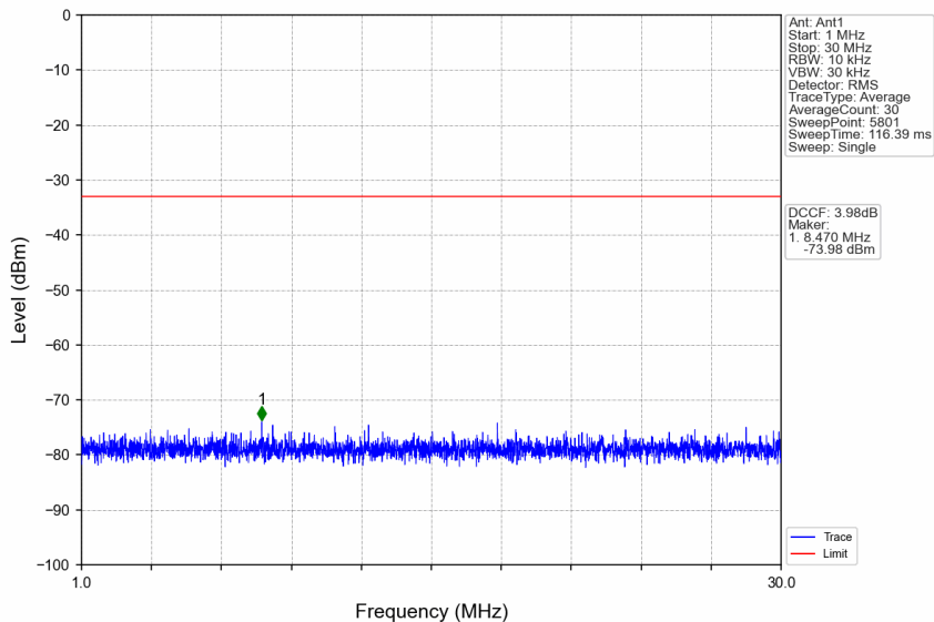
n77a_30kHz_SISO_NTNV_50MHz_DFT-s-OFDM QPSK_3954.99MHz_Edge_1RB_Right
