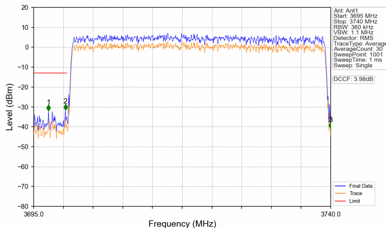
n77a_30kHz_SISO_NTNV_40MHz_CP-OFDM QPSK_3720MHz_Outer_Full
