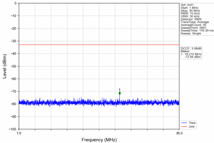
n77a_30kHz_SISO_NTNV_40MHz_DFT-s-OFDM_QPSK_3840MHz_Edge_1RB_Left
