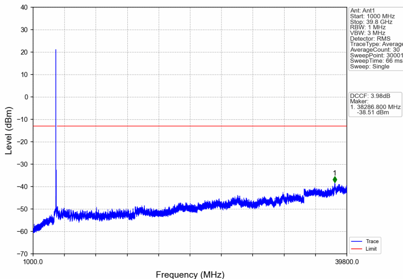
n77a_30kHz_SISO_NTNV_50MHz_CP-OFDM QPSK_3954.99MHz_Edge_1RB_Right
