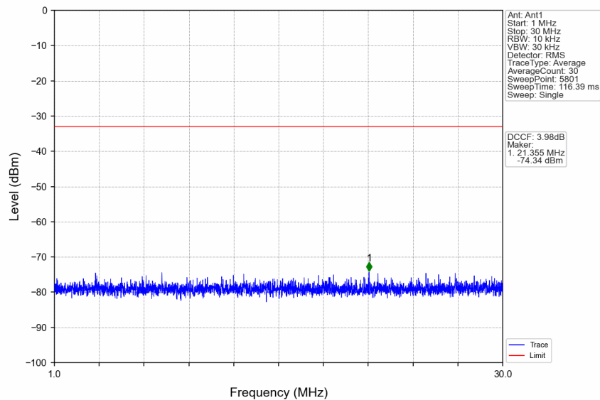
n77a_30kHz_SISO_NTNV_50MHz_DFT-s-OFDM_QPSK_3840MHz_Edge_1RB_Left
