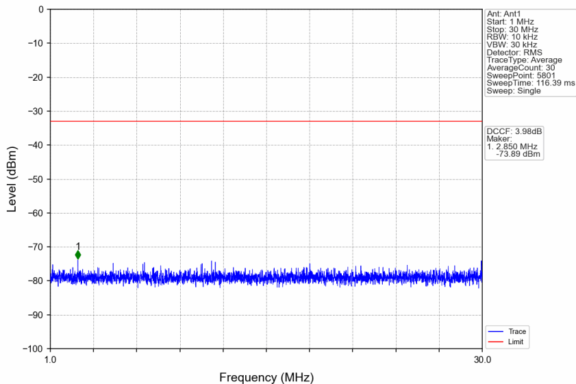
n77a_30kHz_SISO_NTNV_25MHz_CP-OFDM QPSK_3967.5MHz_Edge_1RB_Right
