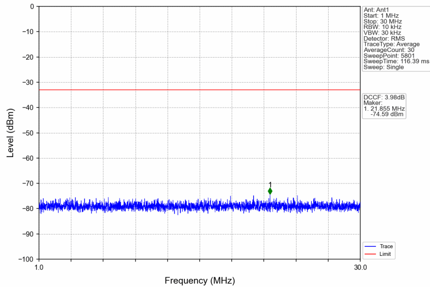
n77a_30kHz_SISO_NTNV_30MHz_DFT-s-OFDM_QPSK_3840MHz_Edge_1RB_Left
