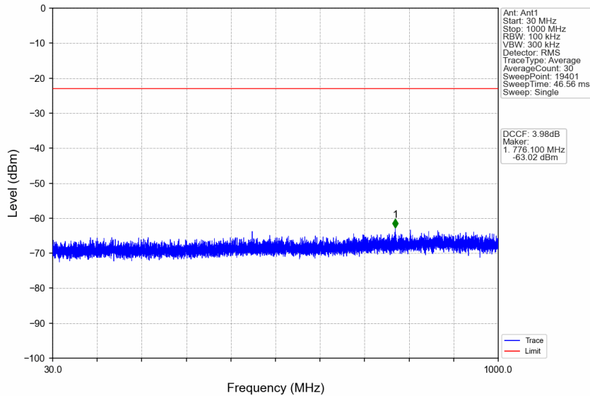
n77a_30kHz_SISO_NTNV_30MHz_DFT-s-OFDM_QPSK_3715.02MHz_Edge_1RB_Left
