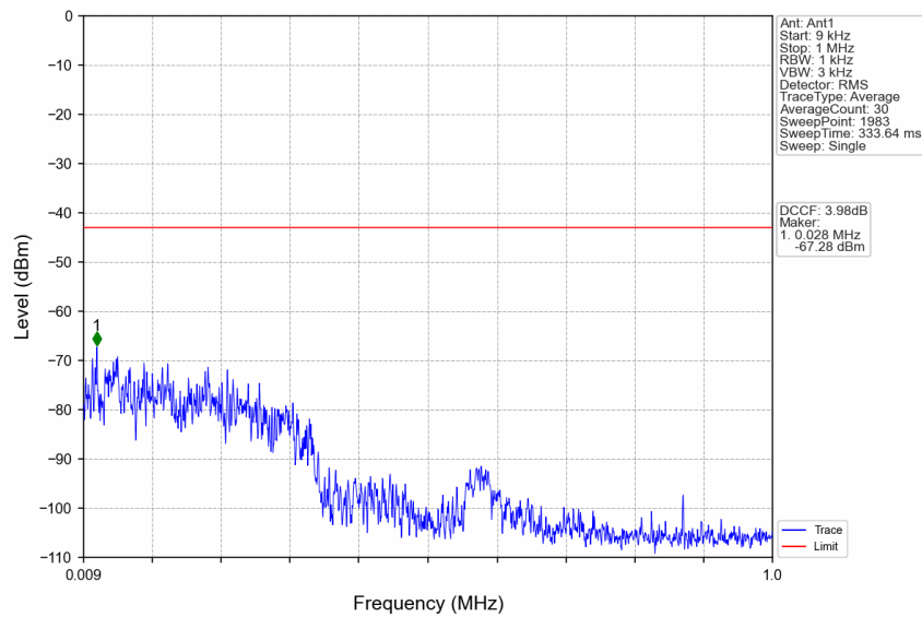
n77a_30kHz_SISO_NTNV_30MHz_CP-OFDM_QPSK_3964.98MHz_Edge_1RB_Right
