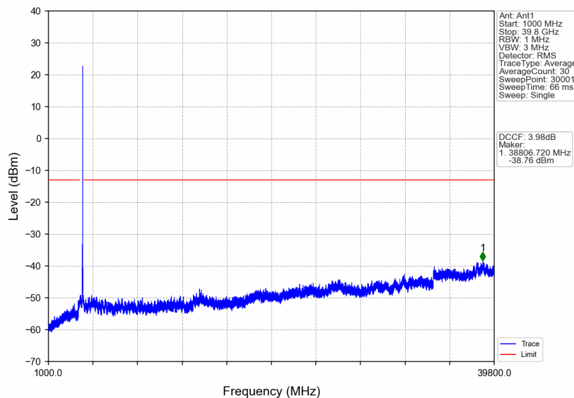
n77a_30kHz_SISO_NTNV_25MHz_CP-OFDM QPSK_3967.5MHz_Edge_1RB_Right
