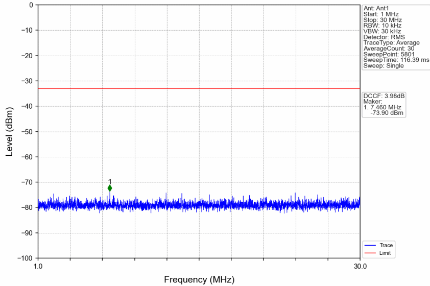
n77a_30kHz_SISO_NTNV_30MHz_DFT-s-OFDM_QPSK_3715.02MHz_Edge_1RB_Left
