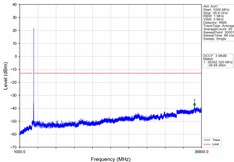
n77a_30kHz_SISO_NTNV_30MHz_DFT-s-OFDM QPSK_3964.98MHz_Edge_1RB_Right
