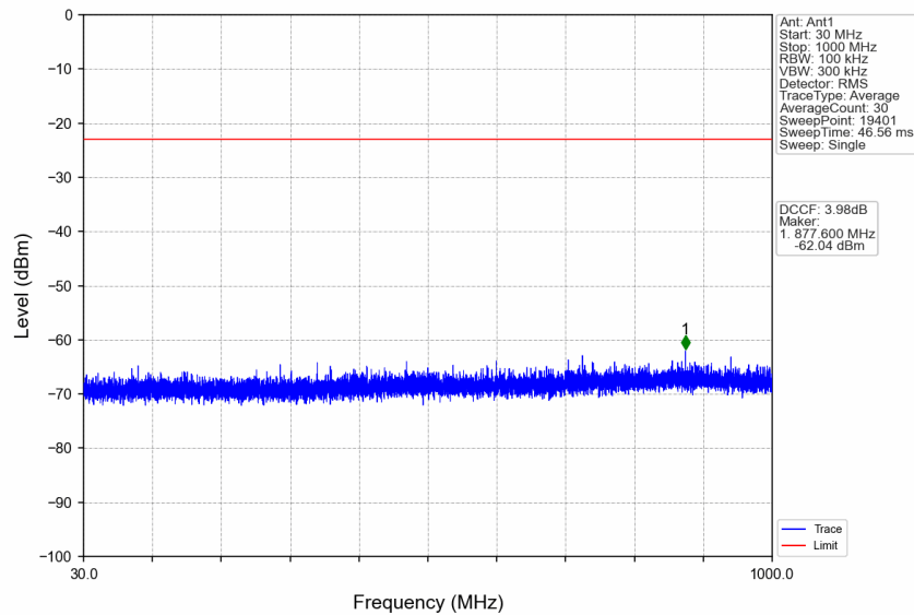
n77a_30kHz_SISO_NTNV_30MHz_DFT-s-OFDM_QPSK_3840MHz_Edge_1RB_Left
