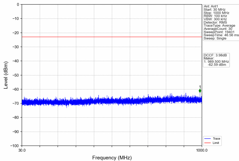
n77a_30kHz_SISO_NTNV_40MHz_DFT-s-OFDM_QPSK_3720MHz_Edge_1RB_Left
