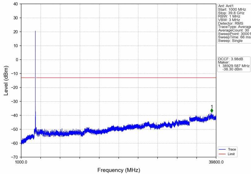
n77a_30kHz_SISO_NTNV_30MHz_CP-OFDM QPSK_3964.98MHz_Edge_1RB_Right
