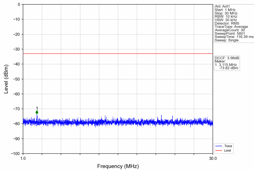
n77a_30kHz_SISO_NTNV_30MHz_CP-OFDM QPSK_3840MHz_Edge_1RB_Left
