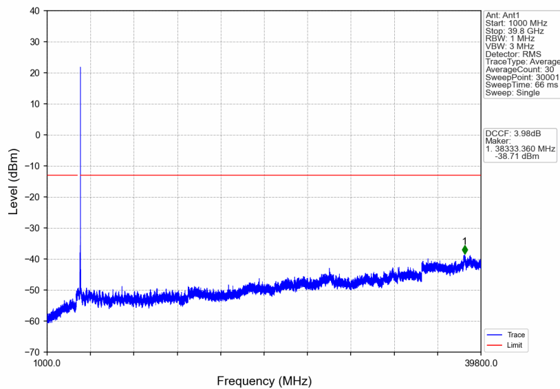
n77a_30kHz_SISO_NTNV_30MHz_CP-OFDM QPSK_3964.98MHz_Edge_1RB_Right
