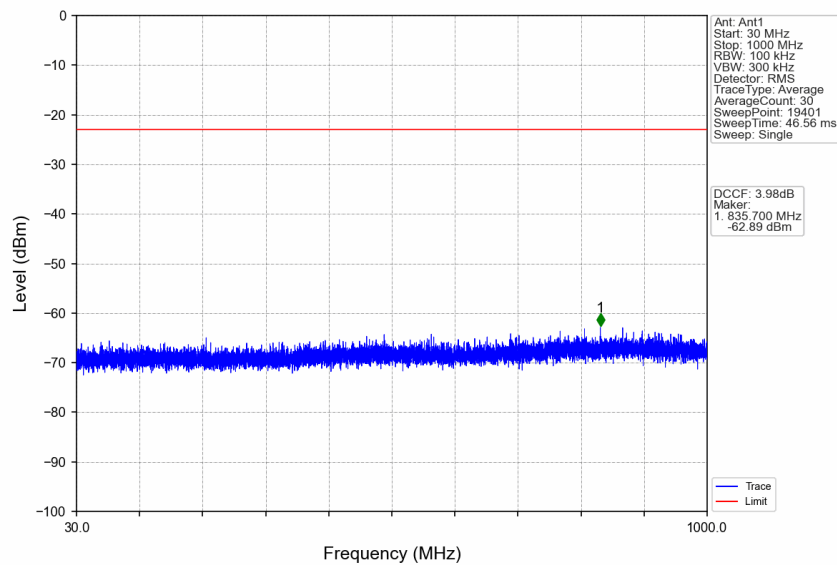
n77a_30kHz_SISO_NTNV_30MHz_CP-OFDM QPSK_3840MHz_Edge_1RB_Left
