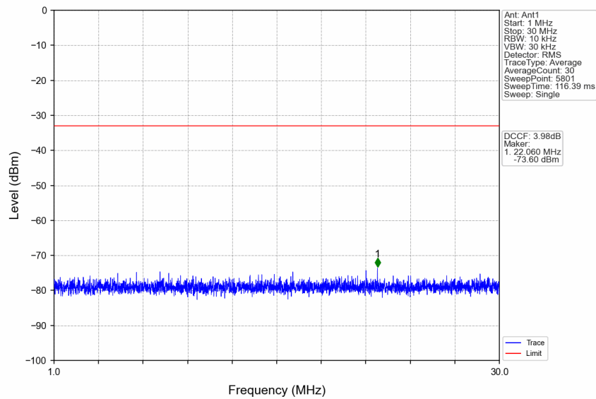
n77a_30kHz_SISO_NTNV_40MHz_DFT-s-OFDM_QPSK_3720MHz_Edge_1RB_Left
