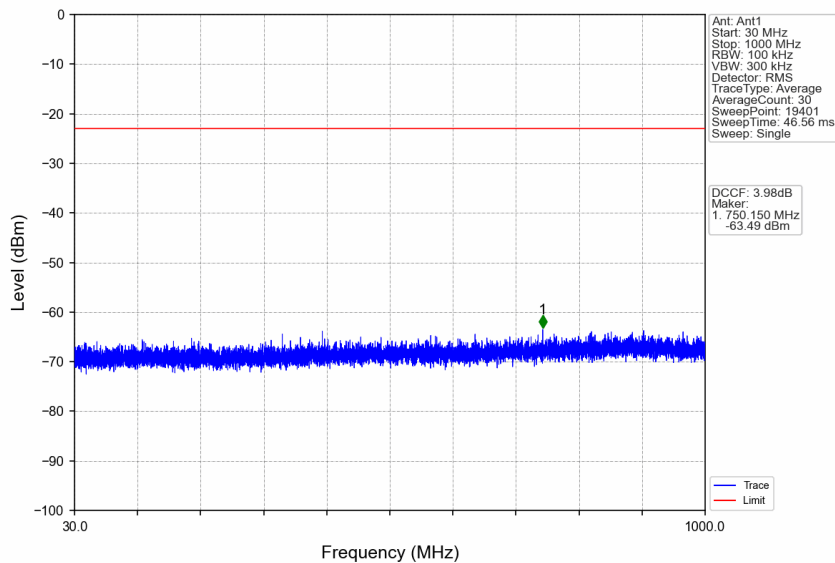
n77a_30kHz_SISO_NTNV_25MHz_CP-OFDM QPSK_3967.5MHz_Edge_1RB_Right
