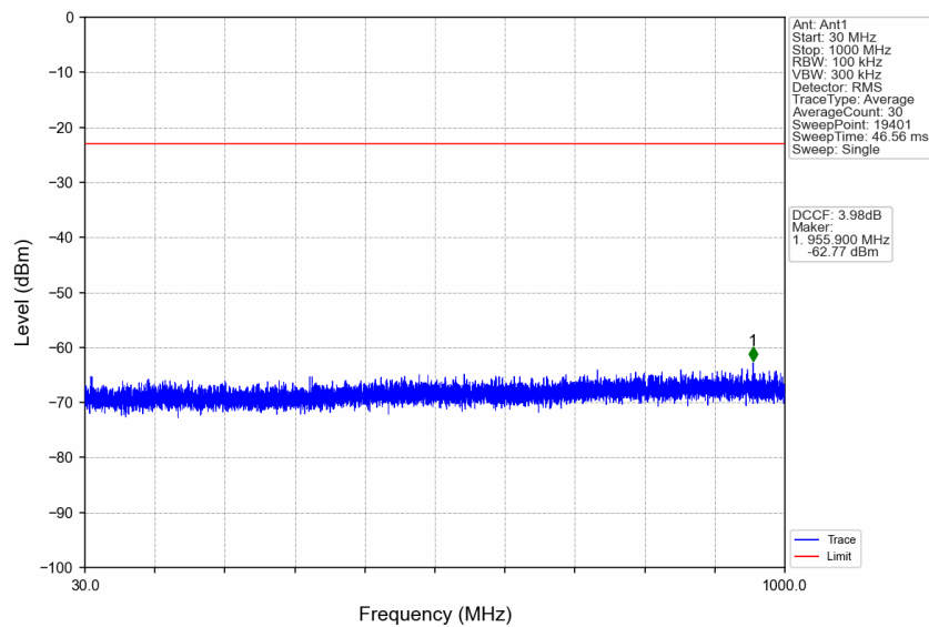
n77a_30kHz_SISO_NTNV_30MHz_CP-OFDM_QPSK_3715.02MHz_Edge_1RB_Left
