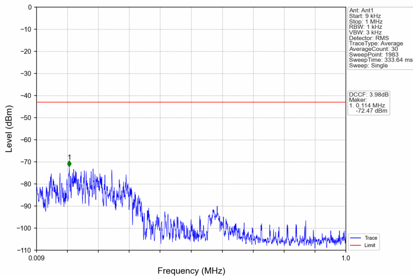
n77a_30kHz_SISO_NTNV_30MHz_DFT-s-OFDM QPSK_3964.98MHz_Edge_1RB_Right
