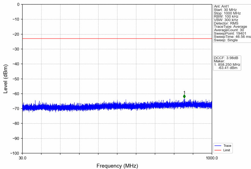
n77a_30kHz_SISO_NTNV_30MHz_DFT-s-OFDM QPSK_3964.98MHz_Edge_1RB_Right
