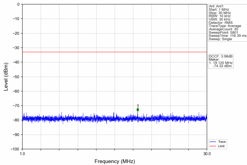
n77a_30kHz_SISO_NTNV_30MHz_CP-OFDM_QPSK_3715.02MHz_Edge_1RB_Left
