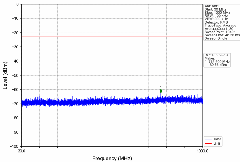
n77a_30kHz_SISO_NTNV_30MHz_CP-OFDM QPSK_3964.98MHz_Edge_1RB_Right
