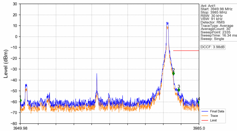
n77a_30kHz_SISO_NTNV_30MHz_CP-OFDM QPSK_3964.98MHz_Edge_1RB_Right
