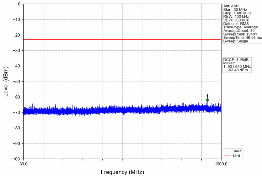
n77a_30kHz_SISO_NTNV_10MHz_CP-OFDM QPSK_3975MHz_Edge_1RB_Right
