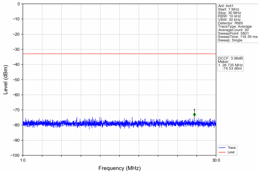
n77a_30kHz_SISO_NTNV_15MHz_CP-OFDM QPSK_3707.52MHz_Edge_1RB_Left
