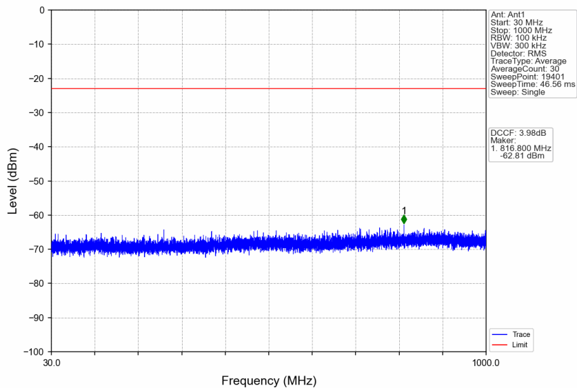
n77a_30kHz_SISO_NTNV_15MHz_DFT-s-OFDM QPSK_3972.48MHz_Edge_1RB_Right
