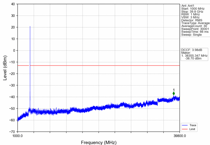
n77a_30kHz_SISO_NTNV_15MHz_DFT-s-OFDM QPSK_3972.48MHz_Edge_1RB_Right
