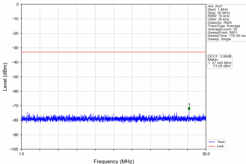
n77a_30kHz_SISO_NTNV_15MHz_DFT-s-OFDM_QPSK_3707.52MHz_Edge_1RB_Left
