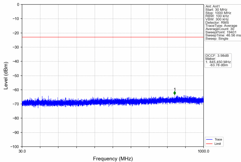
n77a_30kHz_SISO_NTNV_15MHz_DFT-s-OFDM PI/2 BPSK_3707.52MHz_Edge_1RB_Left
