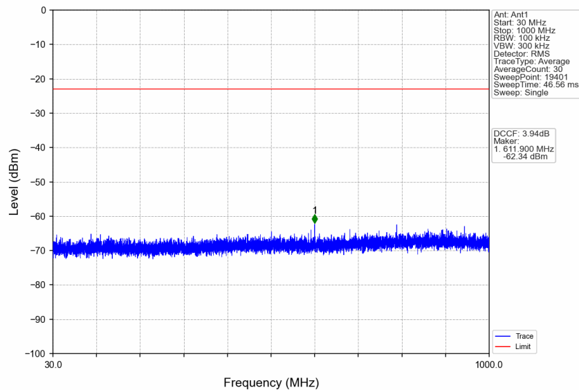
n77a_30kHz_SISO_NTNV_15MHz_CP-OFDM_QPSK_3972.48MHz_Edge_1RB_Right
