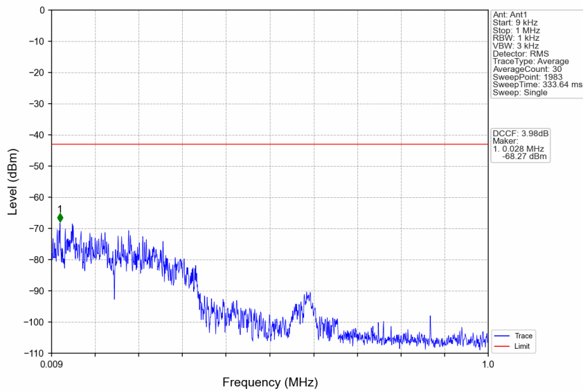
n77a_30kHz_SISO_NTNV_10MHz_CP-OFDM QPSK_3975MHz_Edge_1RB_Right
