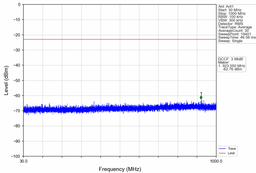
n77a_30kHz_SISO_NTNV_15MHz_DFT-s-OFDM PI/2 BPSK_3972.48MHz_Edge_1RB_Right
