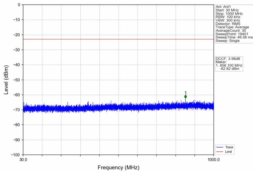
n77a_30kHz_SISO_NTNV_15MHz_CP-OFDM QPSK_3840MHz_Edge_1RB_Left
