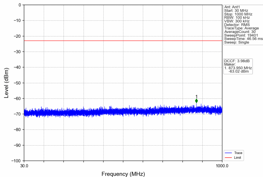
n77a_30kHz_SISO_NTNV_20MHz_DFT-s-OFDM Pi/2 BPSK_3710.01MHz_Edge_1RB_Left
