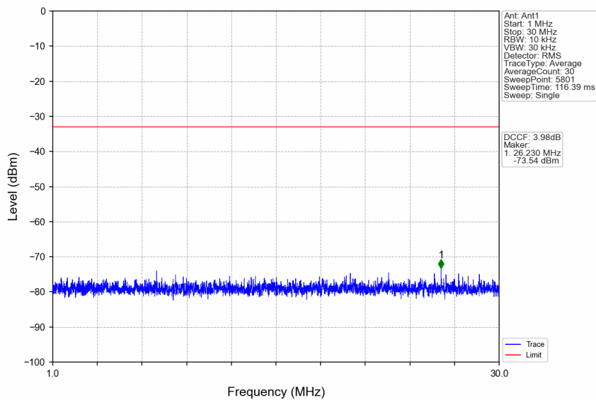
n77a_30kHz_SISO_NTNV_15MHz_DFT-s-OFDM QPSK_3972.48MHz_Edge_1RB_Right
