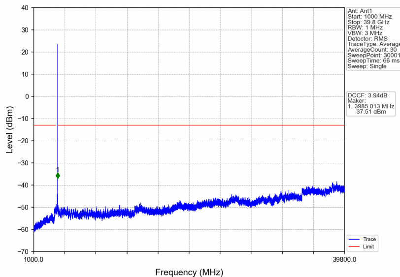
n77a_30kHz_SISO_NTNV_15MHz_CP-OFDM_QPSK_3972.48MHz_Edge_1RB_Right
