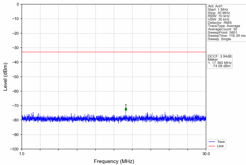
n77a_30kHz_SISO_NTNV_15MHz_DFT-s-OFDM_QPSK_3840MHz_Edge_1RB_Left
