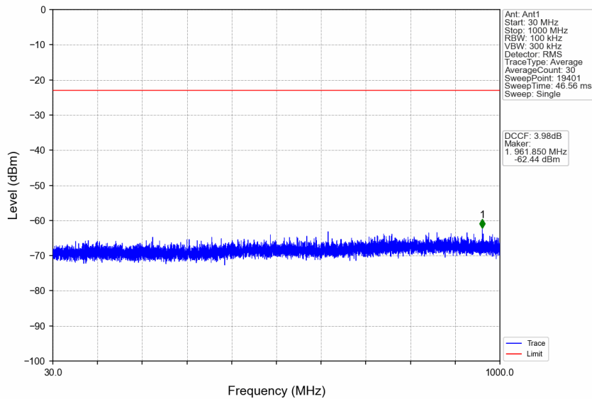
n77a_30kHz_SISO_NTNV_15MHz_CP-OFDM QPSK_3707.52MHz_Edge_1RB_Left
