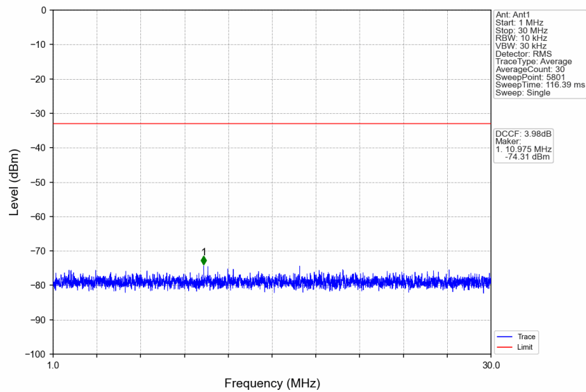
n77a_30kHz_SISO_NTNV_15MHz_CP-OFDM QPSK_3840MHz_Edge_1RB_Left
