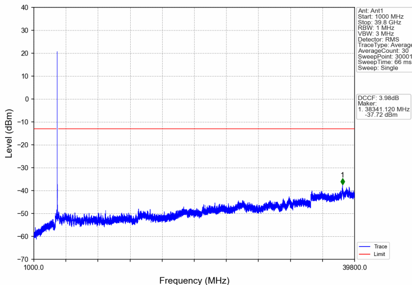
n77a_30kHz_SISO_NTNV_15MHz_CP-OFDM QPSK_3972.48MHz_Edge_1RB_Right
