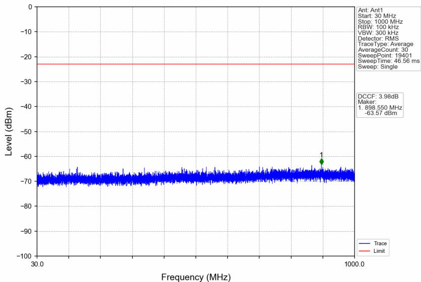
n77a_30kHz_SISO_NTNV_15MHz_DFT-s-OFDM_QPSK_3707.52MHz_Edge_1RB_Left
