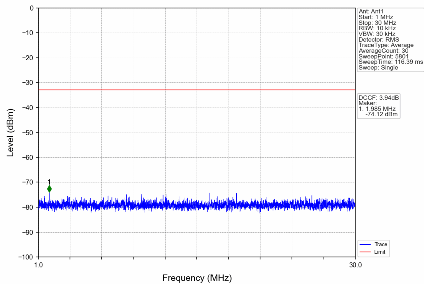
n77a_30kHz_SISO_NTNV_15MHz_CP-OFDM QPSK_3972.48MHz_Edge_1RB_Right
