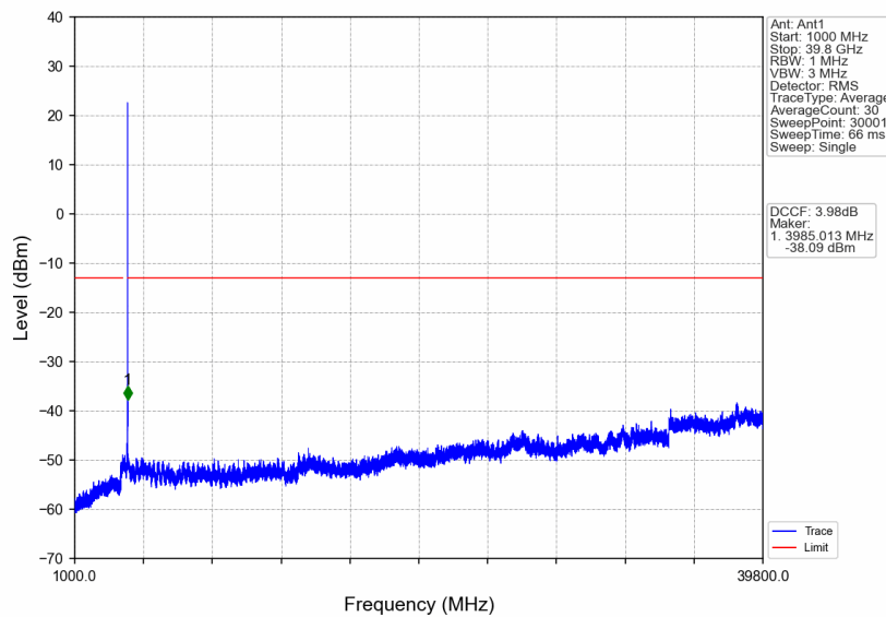
n77a_30kHz_SISO_NTNV_15MHz_DFT-s-OFDM PI/2 BPSK_3972.48MHz_Edge_1RB_Right
