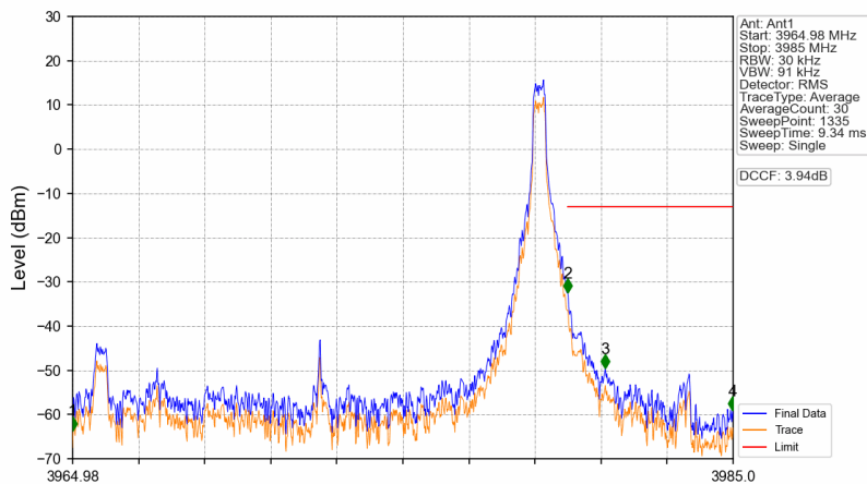
n77a_30kHz_SISO_NTNV_15MHz_CP-OFDM QPSK_3972.48MHz_Edge_1RB_Right
