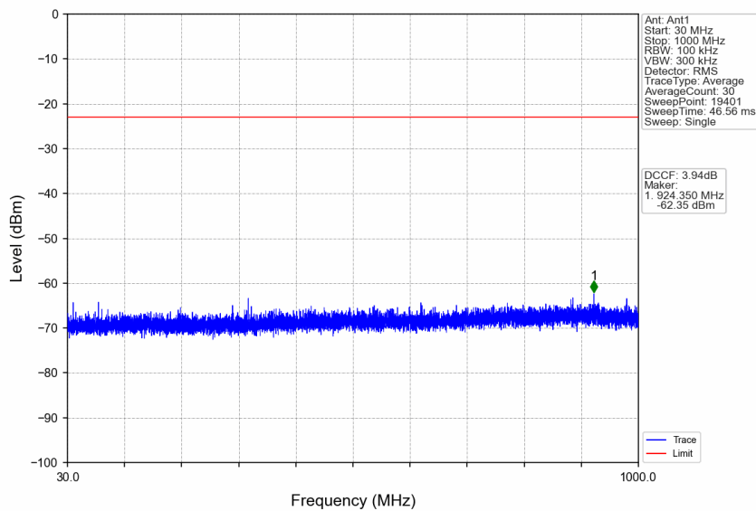
n77a_30kHz_SISO_NTNV_15MHz_DFT-s-OFDM_QPSK_3840MHz_Edge_1RB_Left
