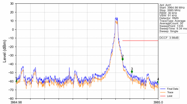
n77a_30kHz_SISO_NTNV_15MHz_DFT-s-OFDM PI/2 BPSK_3972.48MHz_Edge_1RB_Right
