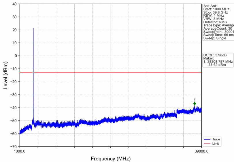
n77a_30kHz_SISO_NTNV_10MHz_CP-OFDM QPSK_3975MHz_Edge_1RB_Right
