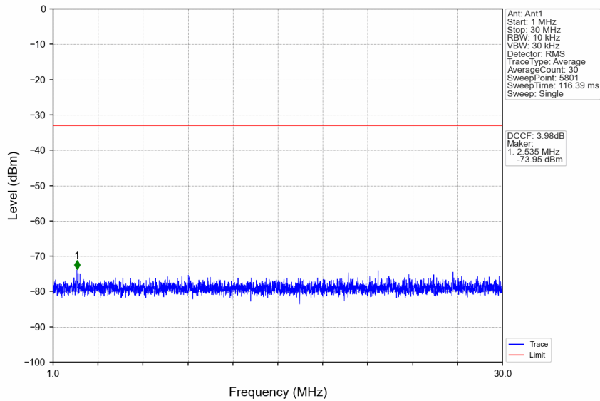
n77a_30kHz_SISO_NTNV_15MHz_DFT-s-OFDM PI/2 BPSK_3840MHz_Edge_1RB_Left
