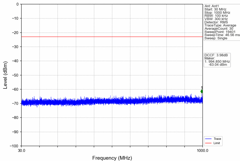
n77a_30kHz_SISO_NTNV_20MHz_DFT-s-OFDM PI/2 BPSK_3969.99MHz_Edge_1RB_Right
