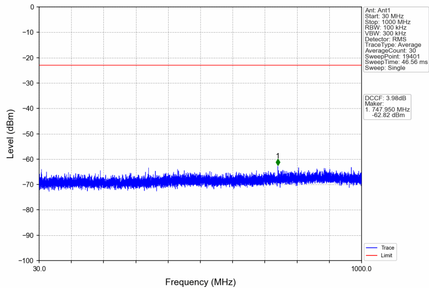
n77a_30kHz_SISO_NTNV_10MHz_DFT-s-OFDM PI/2 BPSK_3840MHz_Edge_1RB_Left
