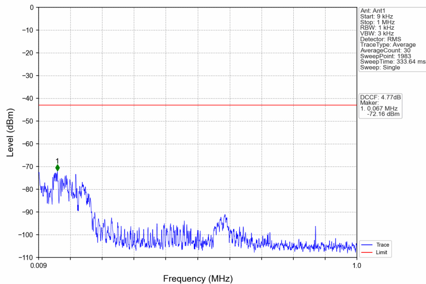
n77a_15kHz_SISO_NTNV_50MHz_DFT-s-OFDM QPSK_3954.99MHz_Edge_1RB_Right
