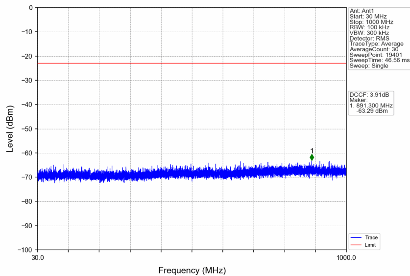
n77a_15kHz_SISO_NTNV_50MHz_CP-OFDM QPSK_3725.01MHz_Edge_1RB_Left
