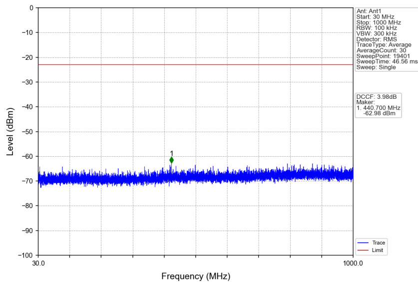
n77a_30kHz_SISO_NTNV_10MHz_DFT-s-OFDM_QPSK_3705MHz_Edge_1RB_Left
