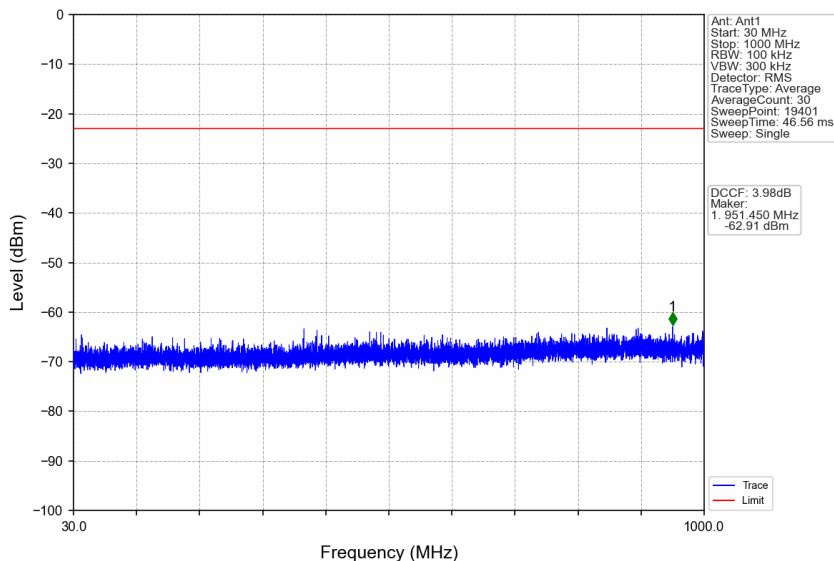
n77a_30kHz_SISO_NTNV_10MHz_DFT-s-OFDM PI/2 BPSK_3975MHz_Edge_1RB_Right
