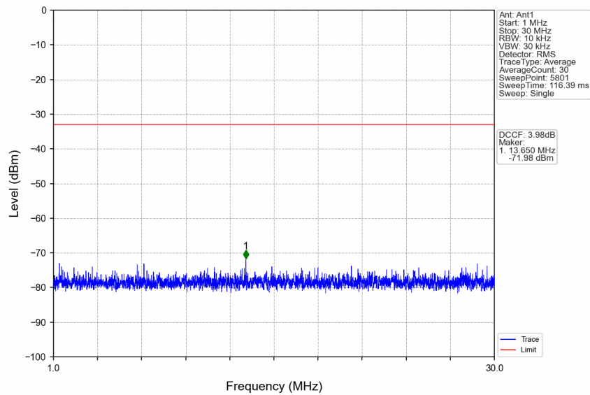
n77a_30kHz_SISO_NTNV_10MHz_DFT-s-OFDM_QPSK_3705MHz_Edge_1RB_Left
