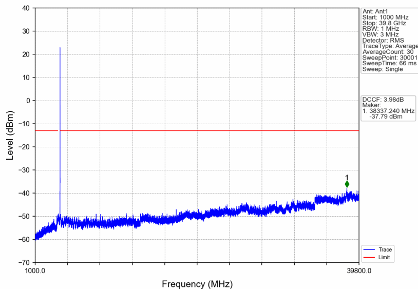
n77a_30kHz_SISO_NTNV_10MHz_DFT-s-OFDM_QPSK_3975MHz_Edge_1RB_Right
