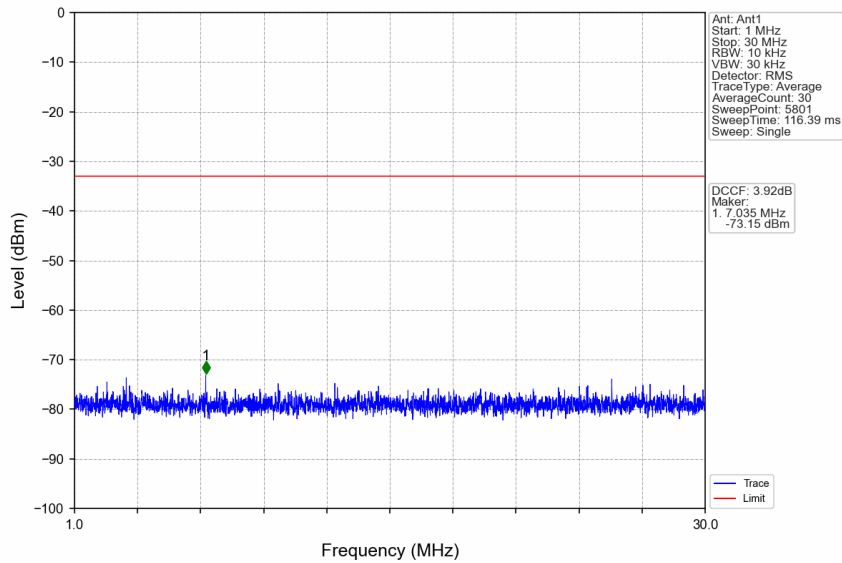
n77a_15kHz_SISO_NTNV_50MHz_DFT-s-OFDM_QPSK_3840MHz_Edge_1RB_Left
