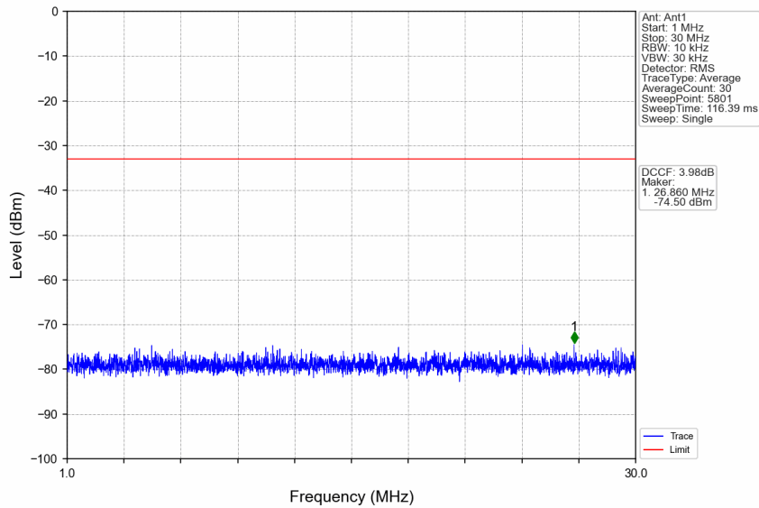
n77a_30kHz_SISO_NTNV_10MHz_DFT-s-OFDM PI/2 BPSK_3705MHz_Edge_1RB_Left
