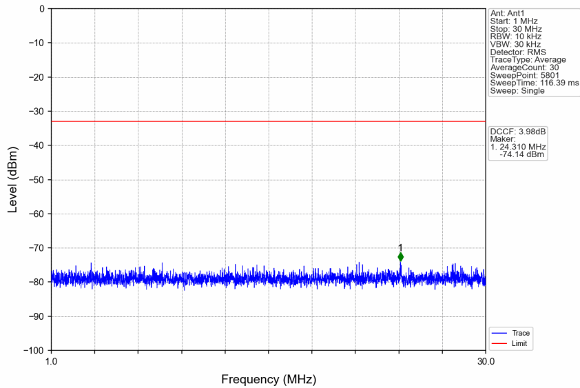
n77a_30kHz_SISO_NTNV_10MHz_CP-OFDM QPSK_3840MHz_Edge_1RB_Left
