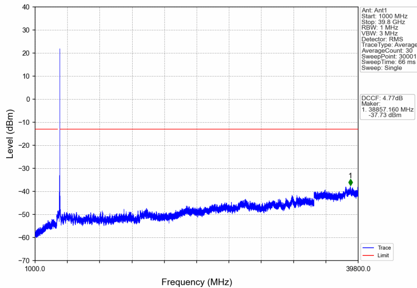
n77a_15kHz_SISO_NTNV_50MHz_CP-OFDM QPSK_3954.99MHz_Edge_1RB_Right
