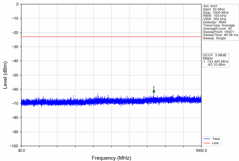
n77a_30kHz_SISO_NTNV_10MHz_DFT-s-OFDM_QPSK_3975MHz_Edge_1RB_Right
