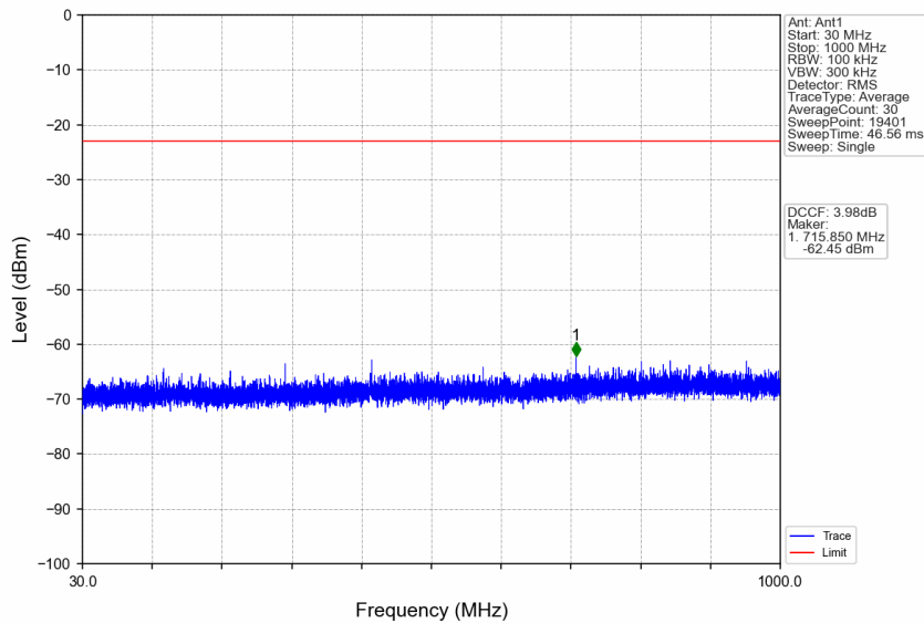
n77a_30kHz_SISO_NTNV_10MHz_CP-OFDM QPSK_3840MHz_Edge_1RB_Left
