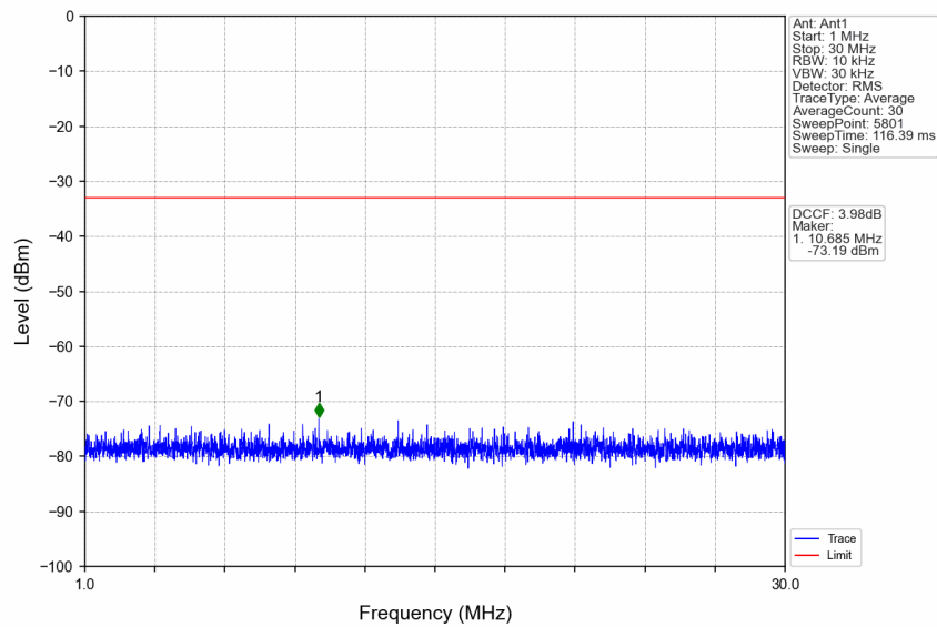
n77a_30kHz_SISO_NTNV_10MHz_DFT-s-OFDM_QPSK_3840MHz_Edge_1RB_Left
