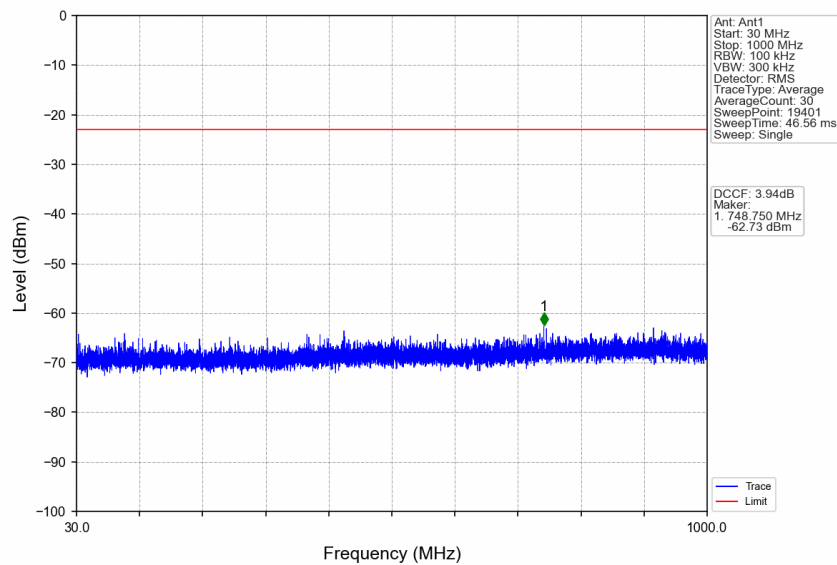
n77a_30kHz_SISO_NTNV_10MHz_CP-OFDM QPSK_3705MHz_Edge_1RB_Left
