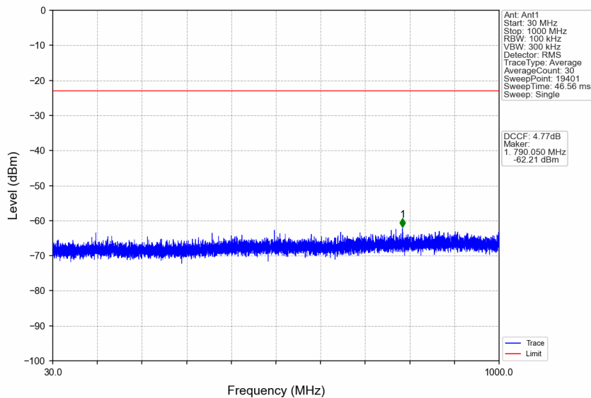
n77a_15kHz_SISO_NTNV_50MHz_DFT-s-OFDM QPSK_3954.99MHz_Edge_1RB_Right
