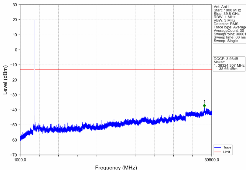
n77a_30kHz_SISO_NTNV_10MHz_DFT-s-OFDM PI/2 BPSK_3975MHz_Edge_1RB_Right
