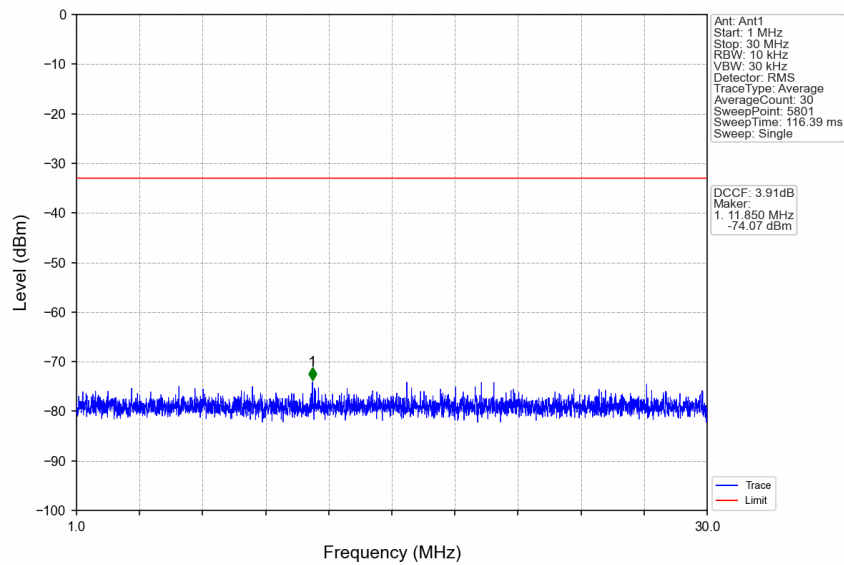
n77a_15kHz_SISO_NTNV_50MHz_CP-OFDM QPSK_3725.01MHz_Edge_1RB_Left
