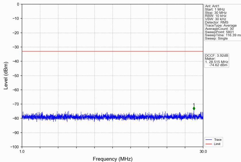
n77a_15kHz_SISO_NTNV_50MHz_CP-OFDM QPSK_3840MHz_Edge_1RB_Left
