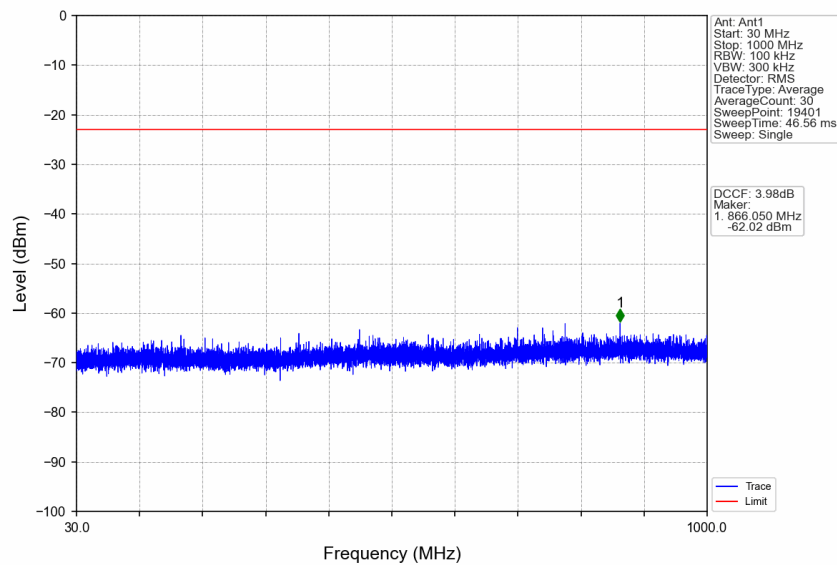
n77a_30kHz_SISO_NTNV_10MHz_DFT-s-OFDM_QPSK_3840MHz_Edge_1RB_Left
