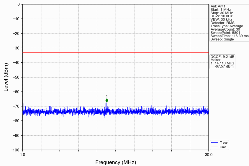
n77a_15kHz_SISO_NTNV_50MHz_DFT-s-OFDM_QPSK_3725.01MHz_Edge_1RB_Left
