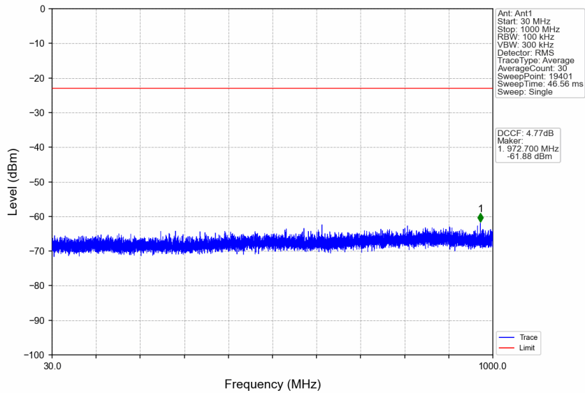
n77a_15kHz_SISO_NTNV_50MHz_CP-OFDM QPSK_3954.99MHz_Edge_1RB_Right
