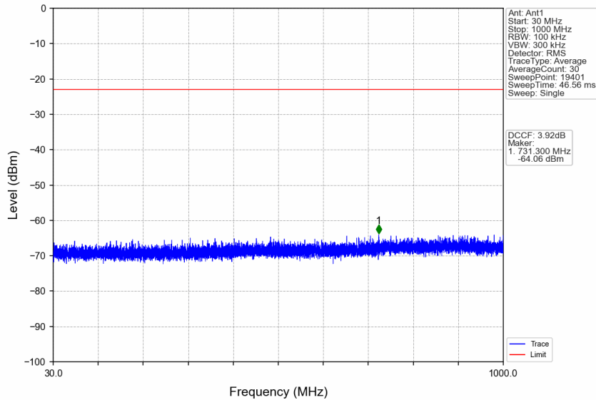
n77a_15kHz_SISO_NTNV_50MHz_DFT-s-OFDM_QPSK_3840MHz_Edge_1RB_Left
