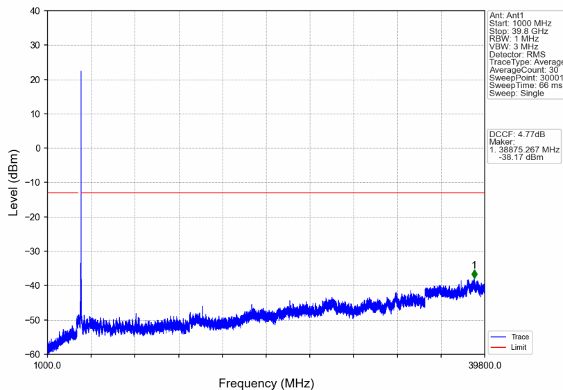
n77a_15kHz_SISO_NTNV_50MHz_DFT-s-OFDM QPSK_3954.99MHz_Edge_1RB_Right
