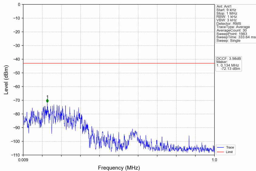
n77a_30kHz_SISO_NTNV_10MHz_DFT-s-OFDM QPSK_3975MHz_Edge_1RB_Right
