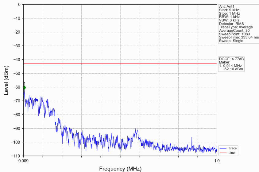
n77a_15kHz_SISO_NTNV_50MHz_CP-OFDM QPSK_3954.99MHz_Edge_1RB_Right
