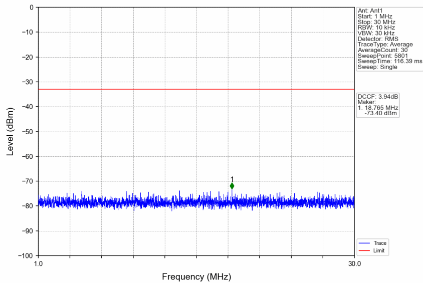
n77a_30kHz_SISO_NTNV_10MHz_CP-OFDM QPSK_3705MHz_Edge_1RB_Left
