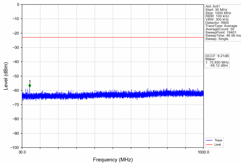
n77a_15kHz_SISO_NTNV_50MHz_DFT-s-OFDM_QPSK_3725.01MHz_Edge_1RB_Left
