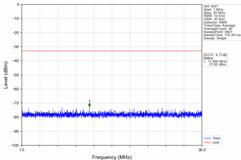
n77a_15kHz_SISO_NTNV_30MHz_DFT-s-OFDM PI/2 BPSK_3964.995MHz_Edge_1RB_Right
