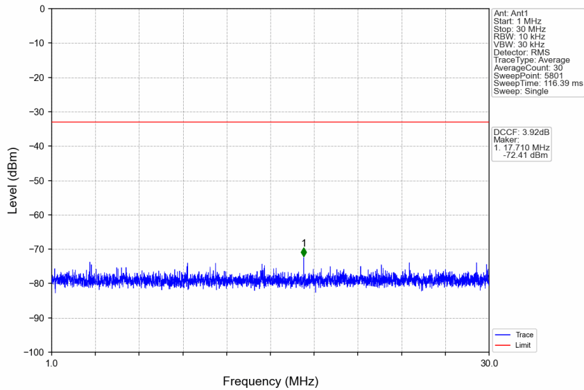
n77a_15kHz_SISO_NTNV_30MHz_DFT-s-OFDM PI/2 BPSK_3840MHz_Edge_1RB_Left
