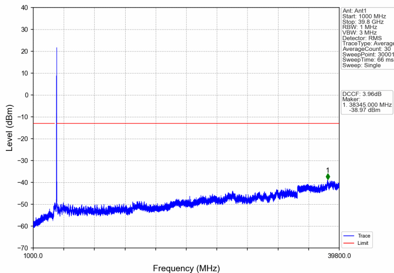
n77a_15kHz_SISO_NTNV_30MHz_DFT-s-OFDM_QPSK_3964.995MHz_Edge_1RB_Right
