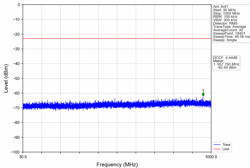
n77a_15kHz_SISO_NTNV_25MHz_CP-OFDM QPSK_3712.5MHz_Edge_1RB_Left
