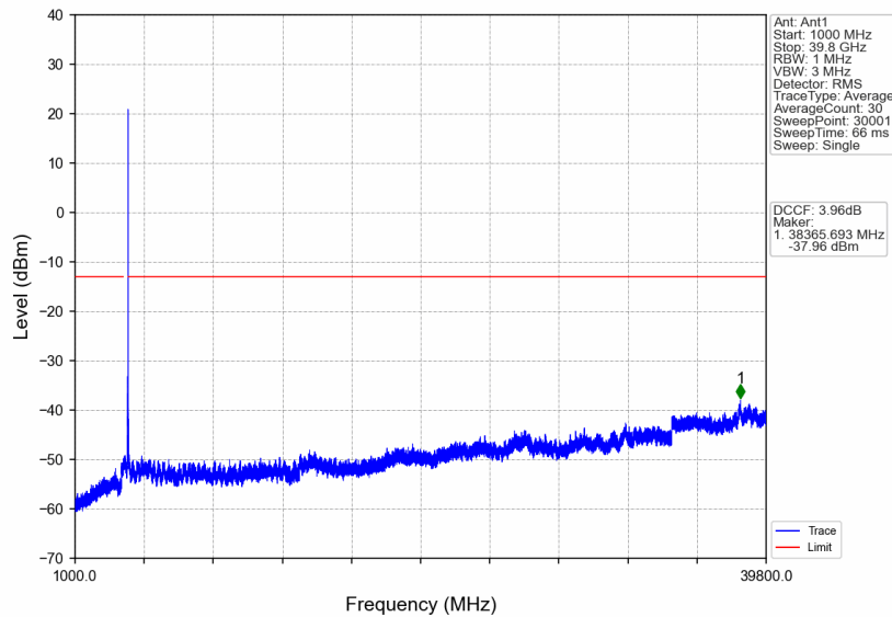
n77a_15kHz_SISO_NTNV_25MHz_DFT-s-OFDM PI/2 BPSK_3967.5MHz_Edge_1RB_Right
