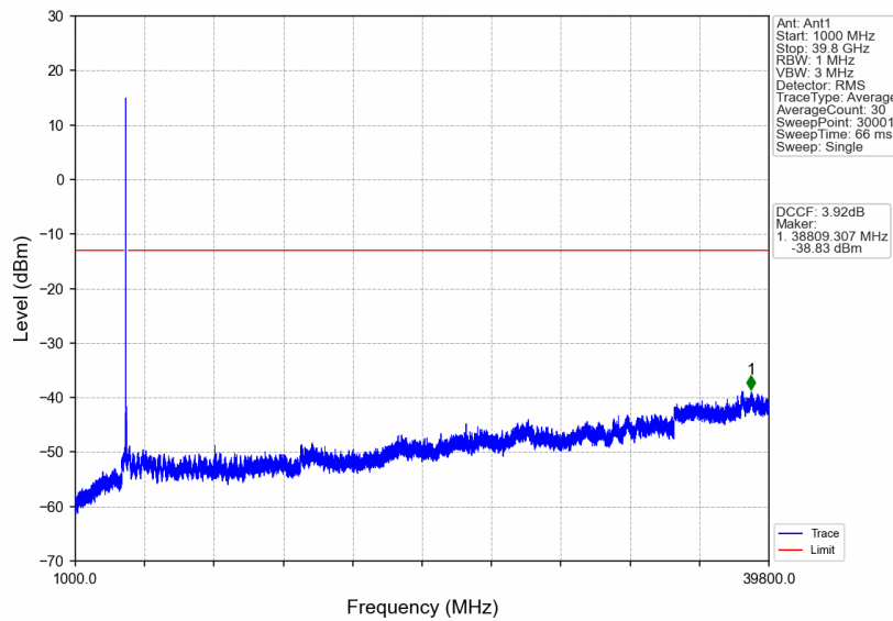
n77a_15kHz_SISO_NTNV_30MHz_DFT-s-OFDM PI/2 BPSK_3964.995MHz_Edge_1RB_Right
