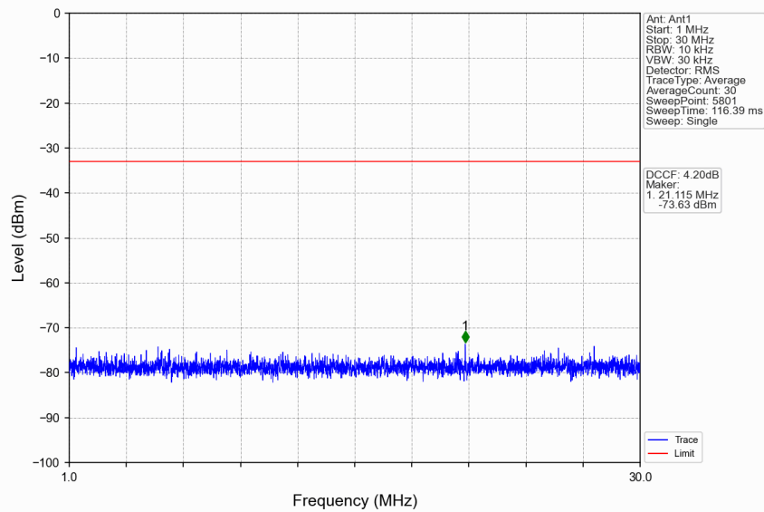
n77a_15kHz_SISO_NTNV_30MHz_CP-OFDM QPSK_3715.005MHz_Edge_1RB_Left
