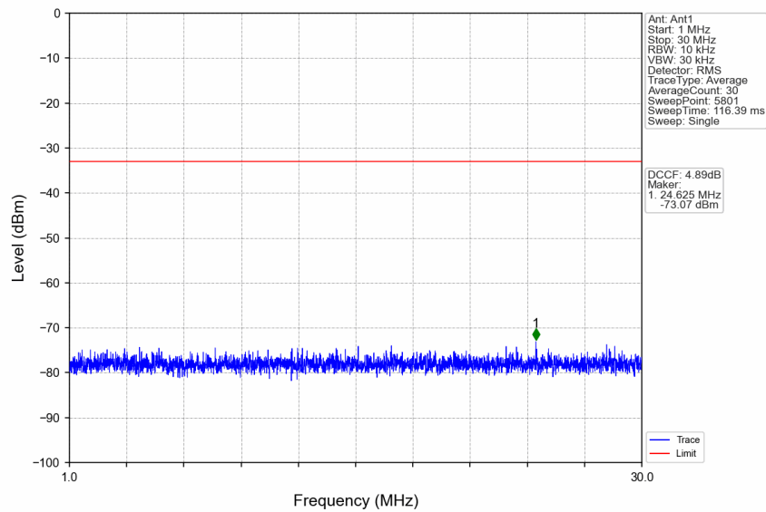
n77a_15kHz_SISO_NTNV_25MHz_CP-OFDM QPSK_3840MHz_Edge_1RB_Left
