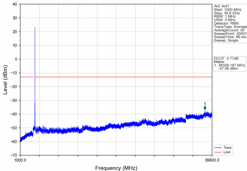
n77a_15kHz_SISO_NTNV_25MHz_DFT-s-OFDM QPSK_3967.5MHz_Edge_1RB_Right
