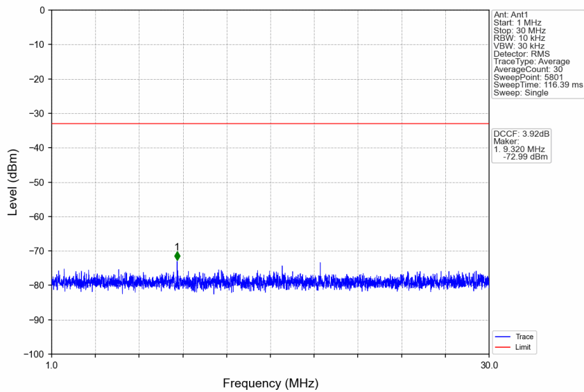
n77a_15kHz_SISO_NTNV_30MHz_DFT-s-OFDM_QPSK_3840MHz_Edge_1RB_Left
