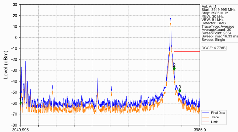
n77a_15kHz_SISO_NTNV_30MHz_DFT-s-OFDM PI/2 BPSK_3964.995MHz_Edge_1RB_Right
