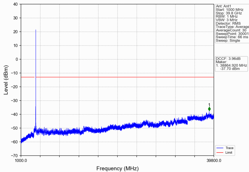
n77a_15kHz_SISO_NTNV_25MHz_CP-OFDM QPSK_3967.5MHz_Edge_1RB_Right
