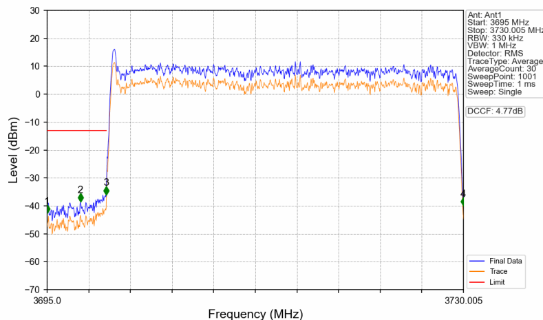
n77a_15kHz_SISO_NTNV_30MHz_DFT-s-OFDM PI/2 BPSK_3715.005MHz_Outer_Full
