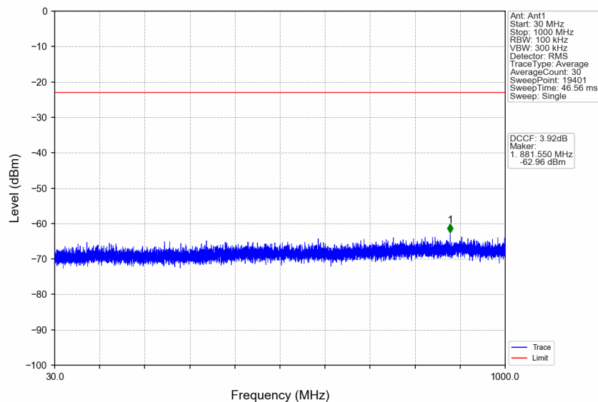
n77a_15kHz_SISO_NTNV_25MHz_DFT-s-OFDM QPSK_3840MHz_Edge_1RB_Left
