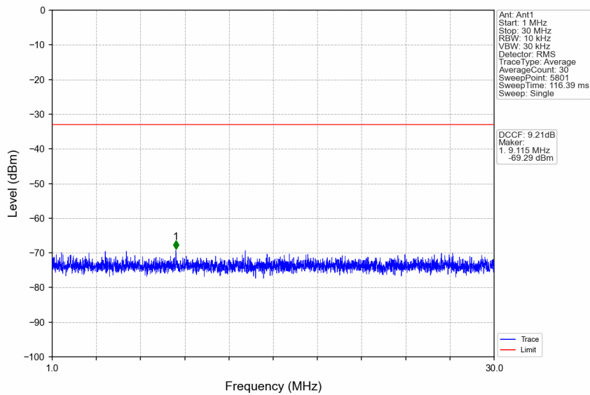
n77a_15kHz_SISO_NTNV_30MHz_DFT-s-OFDM QPSK_3715.005MHz_Edge_1RB_Left
