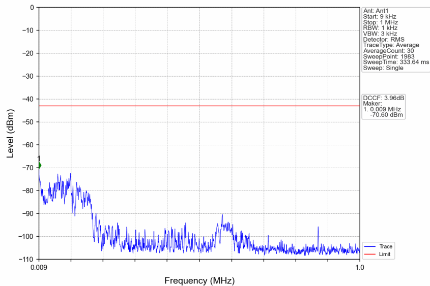
n77a_15kHz_SISO_NTNV_30MHz_DFT-s-OFDM_QPSK_3964.995MHz_Edge_1RB_Right
