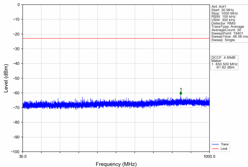
n77a_15kHz_SISO_NTNV_25MHz_CP-OFDM QPSK_3840MHz_Edge_1RB_Left
