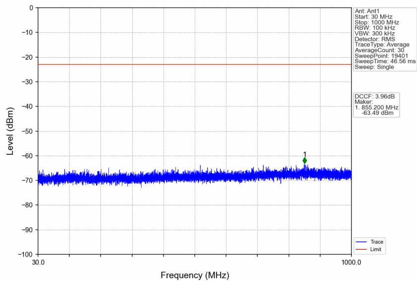
n77a_15kHz_SISO_NTNV_30MHz_DFT-s-OFDM PI/2 BPSK_3715.005MHz_Edge_1RB_Left
