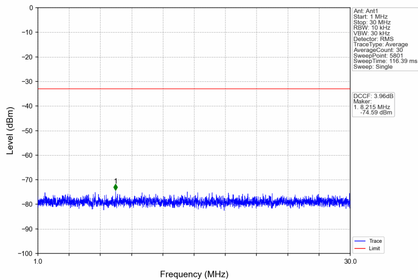
n77a_15kHz_SISO_NTNV_25MHz_CP-OFDM QPSK_3967.5MHz_Edge_1RB_Right
