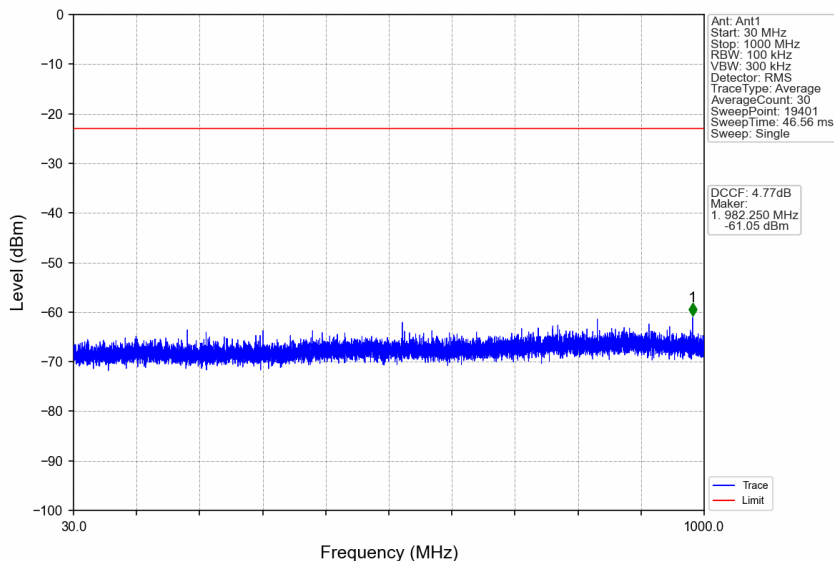
n77a_15kHz_SISO_NTNV_25MHz_DFT-s-OFDM QPSK_3967.5MHz_Edge_1RB_Right
