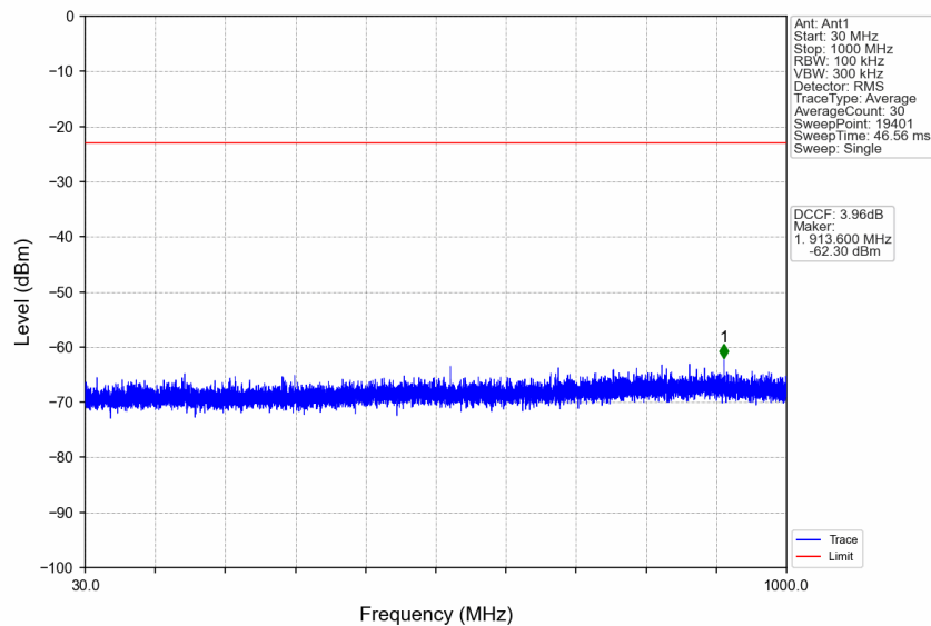
n77a_15kHz_SISO_NTNV_30MHz_DFT-s-OFDM_QPSK_3964.995MHz_Edge_1RB_Right
