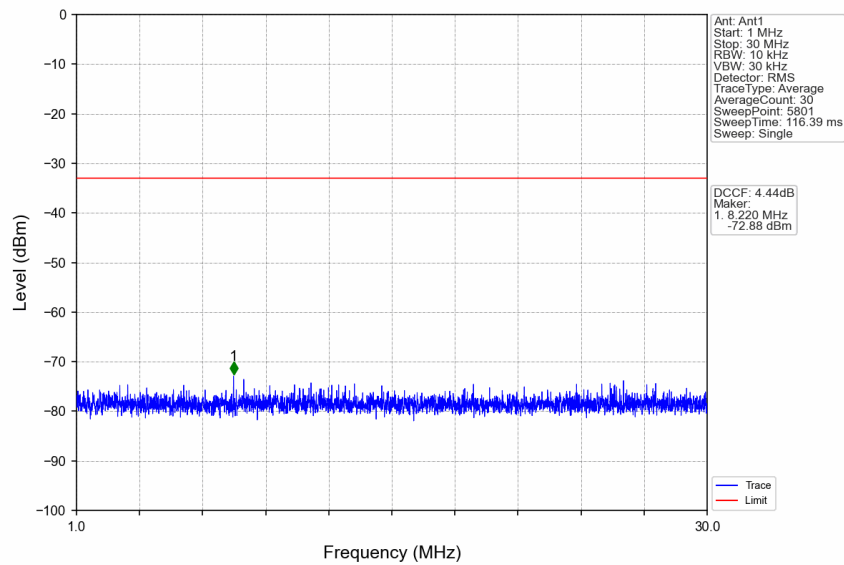
n77a_15kHz_SISO_NTNV_25MHz_CP-OFDM QPSK_3712.5MHz_Edge_1RB_Left
