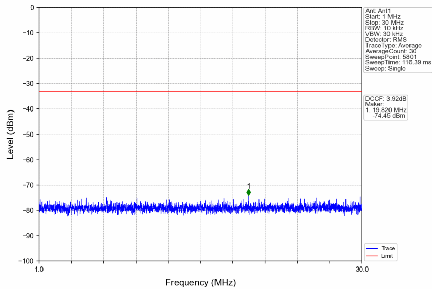
n77a_15kHz_SISO_NTNV_25MHz_DFT-s-OFDM QPSK_3840MHz_Edge_1RB_Left
