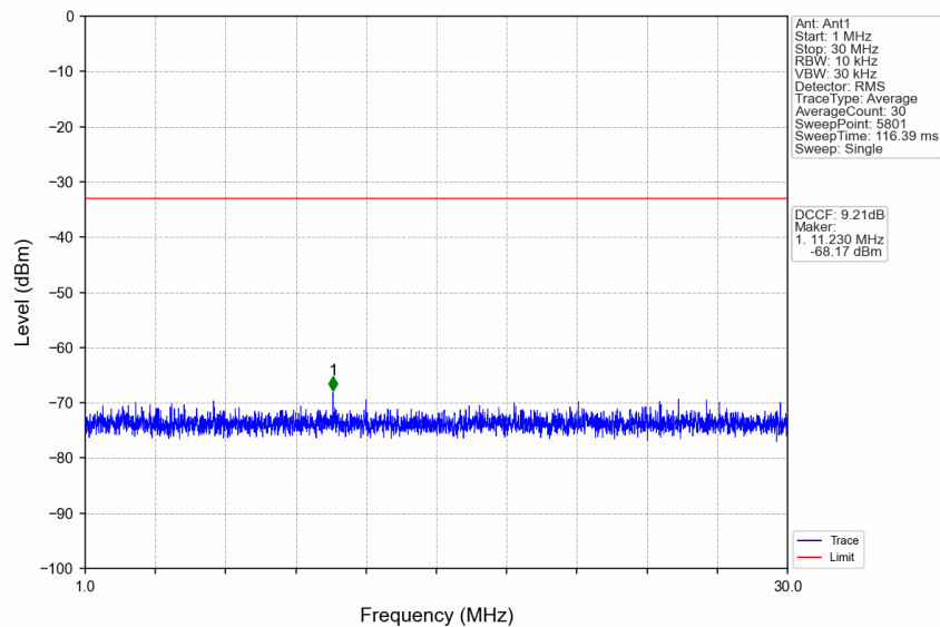
n77a_15kHz_SISO_NTNV_25MHz_DFT-s-OFDM QPSK_3712.5MHz_Edge_1RB_Left
