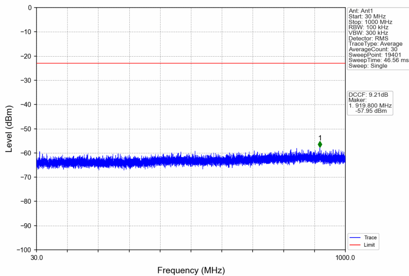
n77a_15kHz_SISO_NTNV_30MHz_DFT-s-OFDM QPSK_3715.005MHz_Edge_1RB_Left
