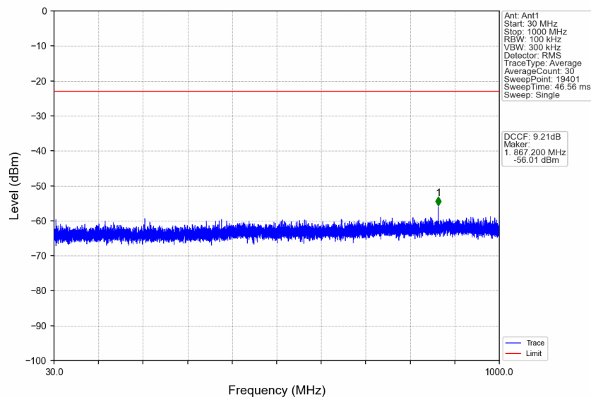
n77a_15kHz_SISO_NTNV_25MHz_DFT-s-OFDM QPSK_3712.5MHz_Edge_1RB_Left
