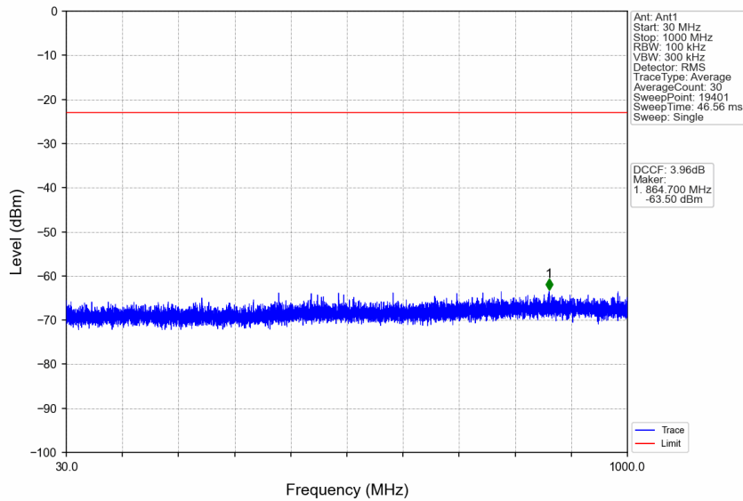
n77a_15kHz_SISO_NTNV_25MHz_CP-OFDM QPSK_3967.5MHz_Edge_1RB_Right
