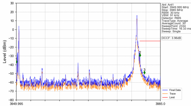
n77a_15kHz_SISO_NTNV_30MHz_DFT-s-OFDM_QPSK_3964.995MHz_Edge_1RB_Right
