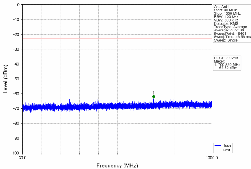
n77a_15kHz_SISO_NTNV_30MHz_DFT-s-OFDM_QPSK_3840MHz_Edge_1RB_Left
