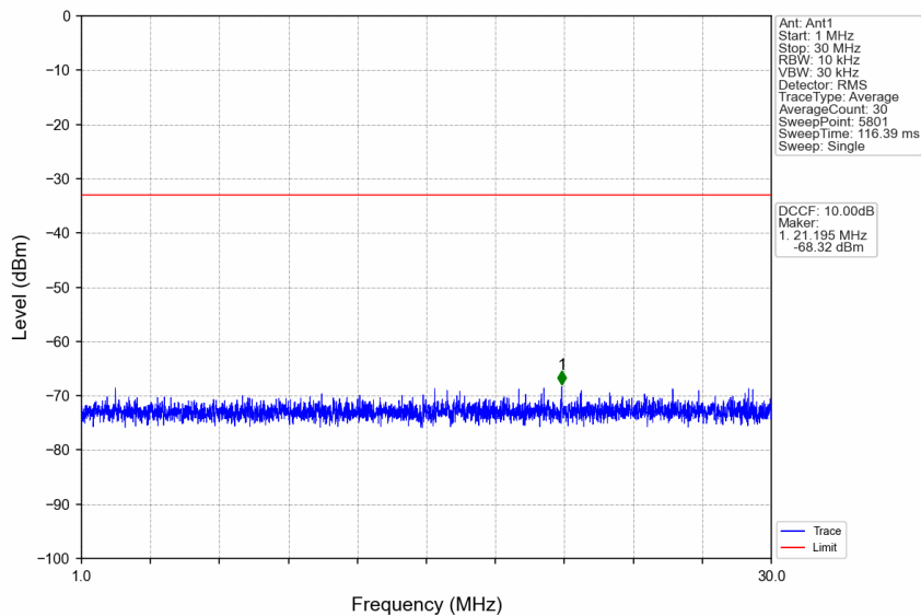
n77a_15kHz_SISO_NTNV_20MHz_DFT-s-OFDM_QPSK_3710.01MHz_Edge_1RB_Left
