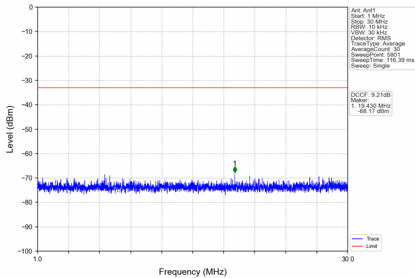
n77a_15kHz_SISO_NTNV_20MHz_CP-OFDM_QPSK_3840MHz_Edge_1RB_Left
