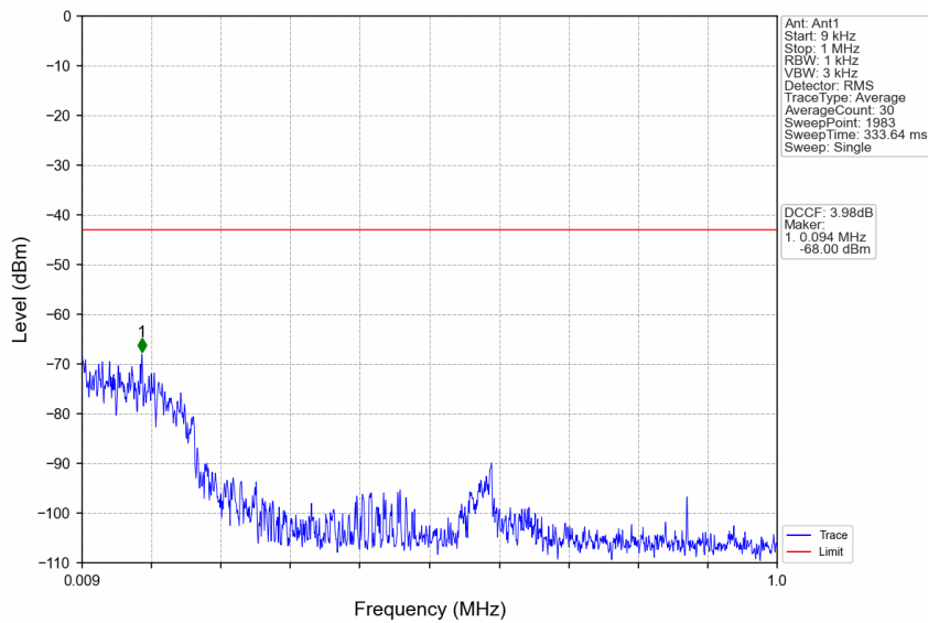
n77a_15kHz_SISO_NTNV_15MHz_CP-OFDM QPSK_3972.495MHz_Edge_1RB_Right
