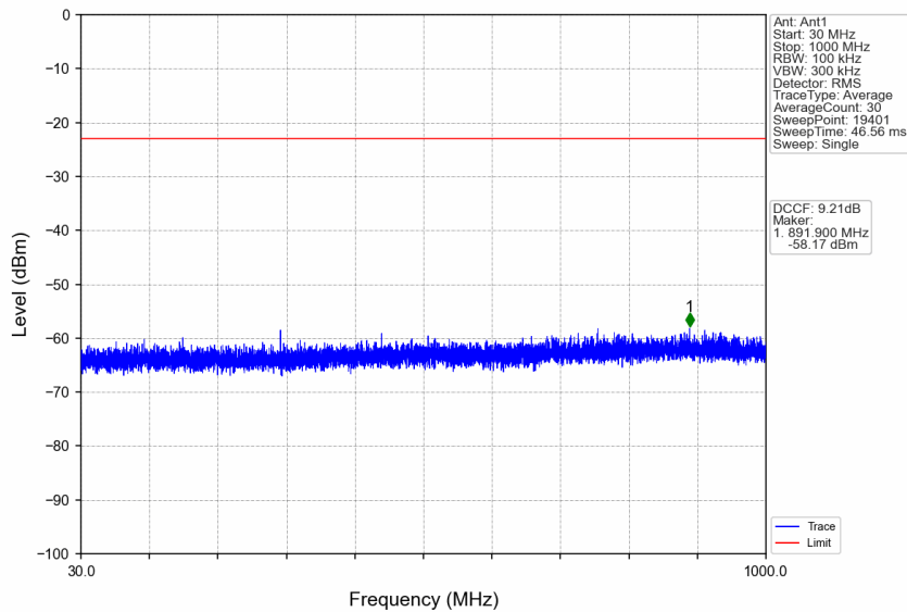
n77a_15kHz_SISO_NTNV_20MHz_CP-OFDM QPSK_3710.01MHz_Edge_1RB_Left
