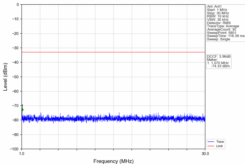
n77a_15kHz_SISO_NTNV_25MHz_DFT-s-OFDM PI/2 BPSK_3967.5MHz_Edge_1RB_Right
