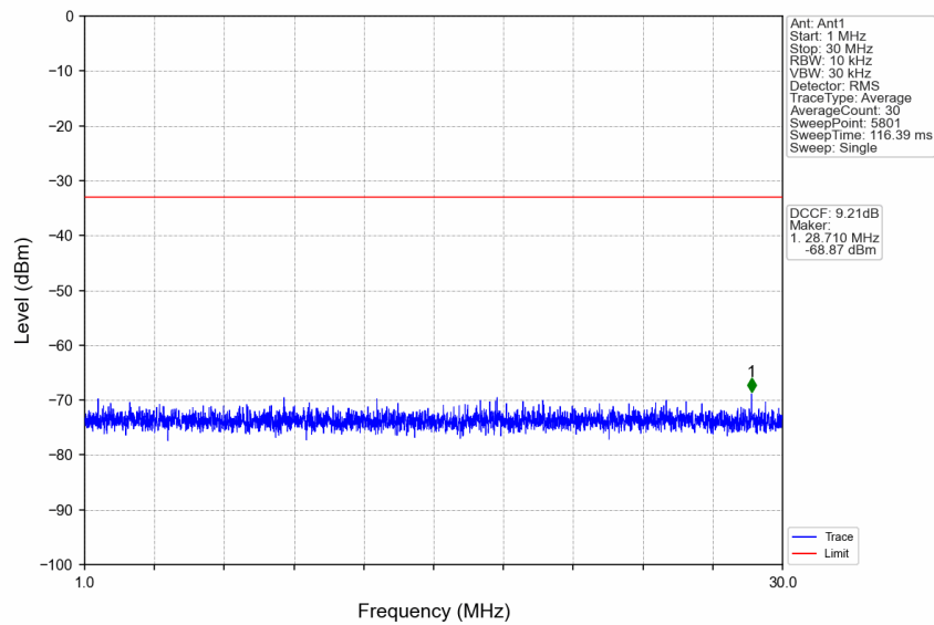
n77a_15kHz_SISO_NTNV_20MHz_DFT-s-OFDM_QPSK_3840MHz_Edge_1RB_Left
