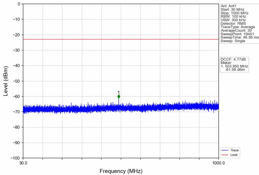
n77a_15kHz_SISO_NTNV_20MHz_CP-OFDM_QPSK_3969.99MHz_Edge_1RB_Right
