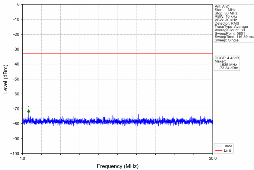
n77a_15kHz_SISO_NTNV_20MHz_DFT-s-OFDM PI/2 BPSK_3840MHz_Edge_1RB_Left
