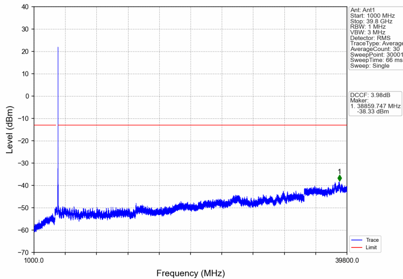
n77a_15kHz_SISO_NTNV_20MHz_DFT-s-OFDM PI/2 BPSK_3969.99MHz_Edge_1RB_Right
