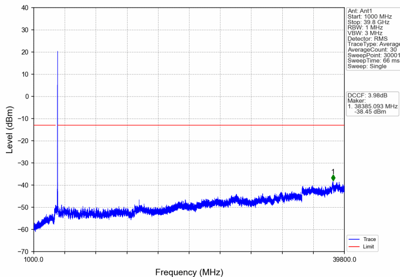
n77a_15kHz_SISO_NTNV_20MHz_DFT-s-OFDM QPSK_3969.99MHz_Edge_1RB_Right
