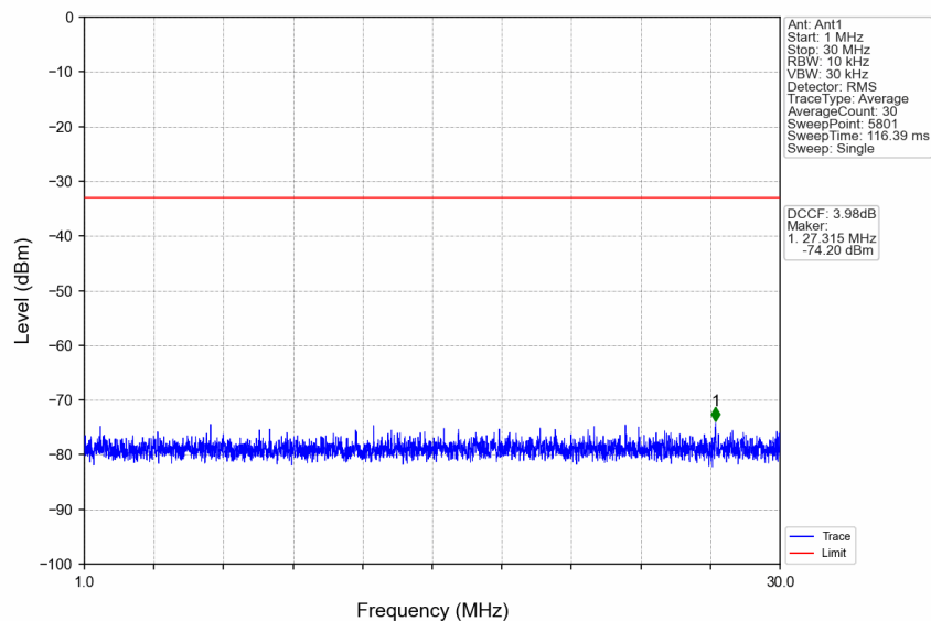
n77a_15kHz_SISO_NTNV_20MHz_DFT-s-OFDM QPSK_3969.99MHz_Edge_1RB_Right
