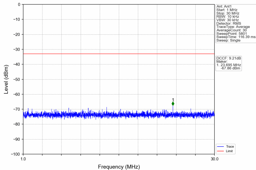
n77a_15kHz_SISO_NTNV_15MHz_CP-OFDM QPSK_3840MHz_Edge_1RB_Left
