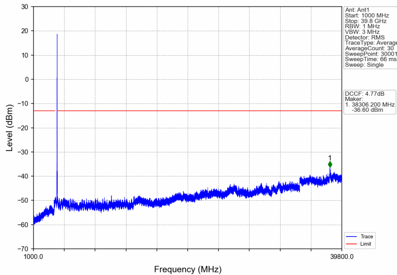
n77a_15kHz_SISO_NTNV_20MHz_CP-OFDM_QPSK_3969.99MHz_Edge_1RB_Right
