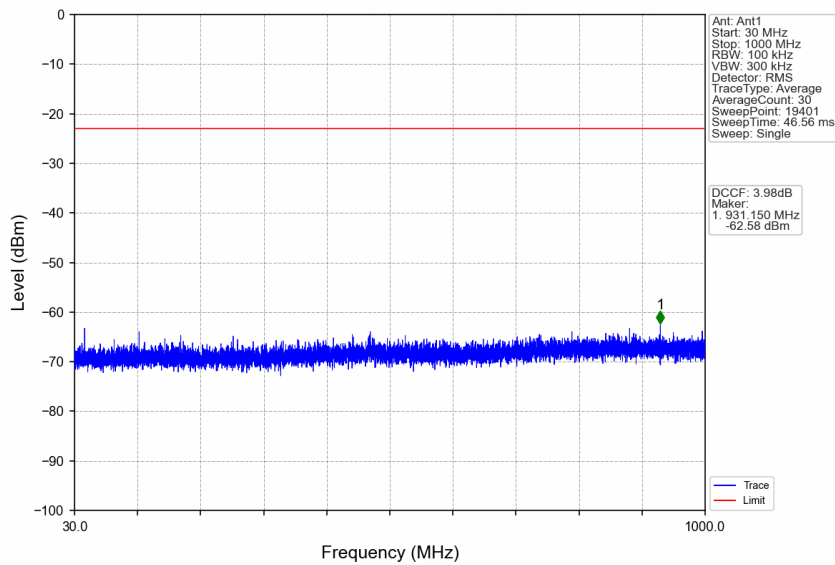
n77a_15kHz_SISO_NTNV_20MHz_DFT-s-OFDM QPSK_3969.99MHz_Edge_1RB_Right
