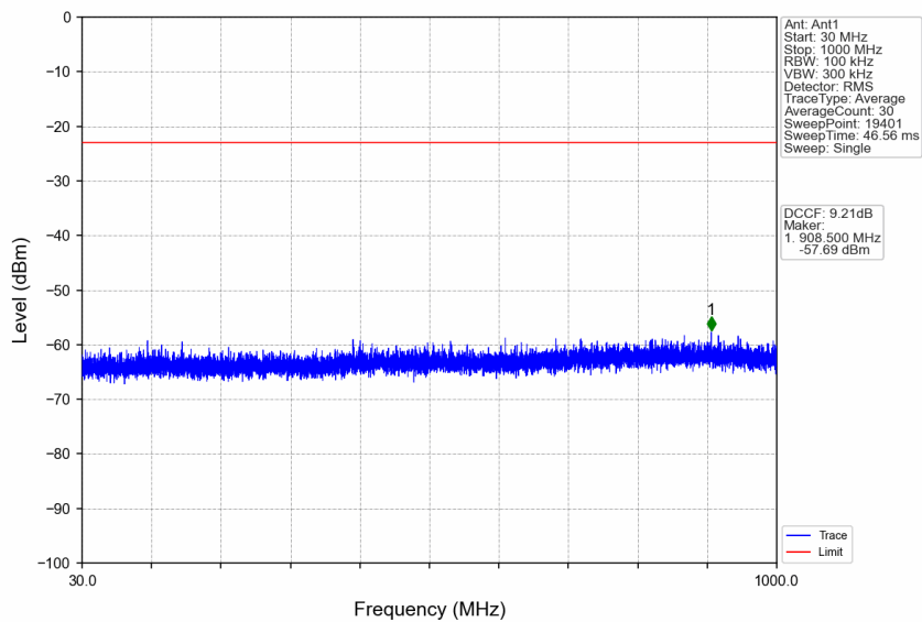
n77a_15kHz_SISO_NTNV_25MHz_DFT-s-OFDM PI/2 BPSK_3840MHz_Edge_1RB_Left
