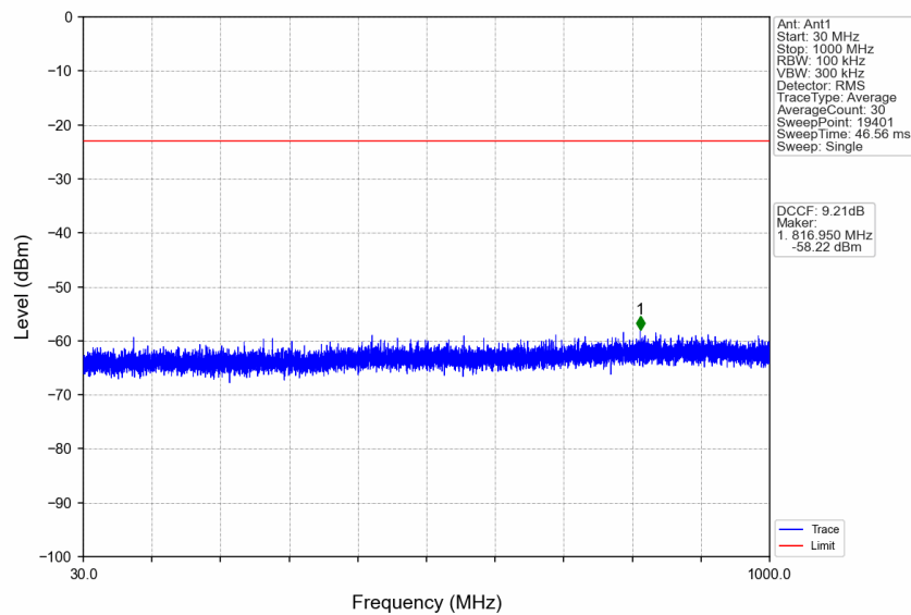
n77a_15kHz_SISO_NTNV_20MHz_DFT-s-OFDM_QPSK_3840MHz_Edge_1RB_Left
