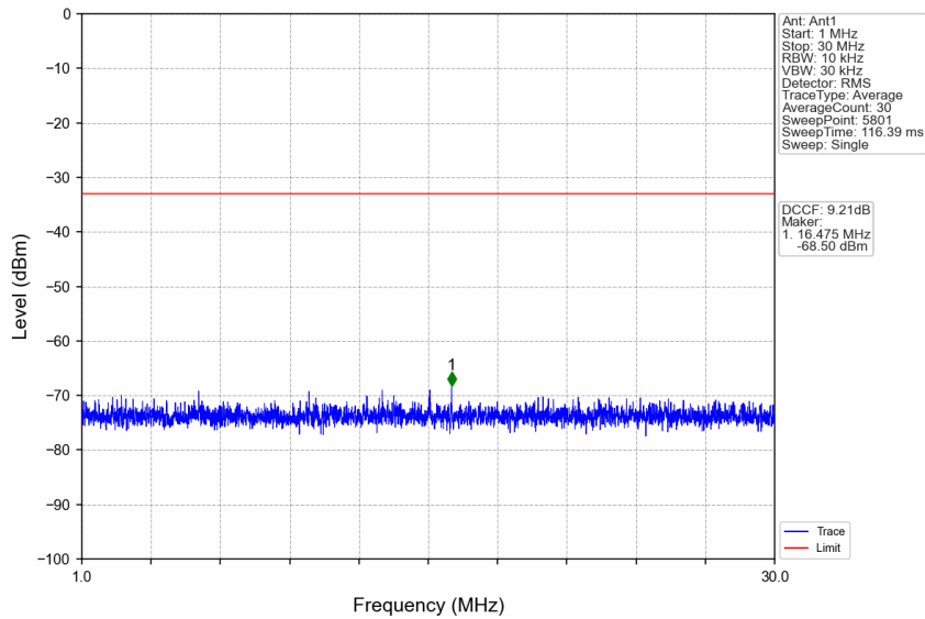
n77a_15kHz_SISO_NTNV_20MHz_CP-OFDM QPSK_3710.01MHz_Edge_1RB_Left
