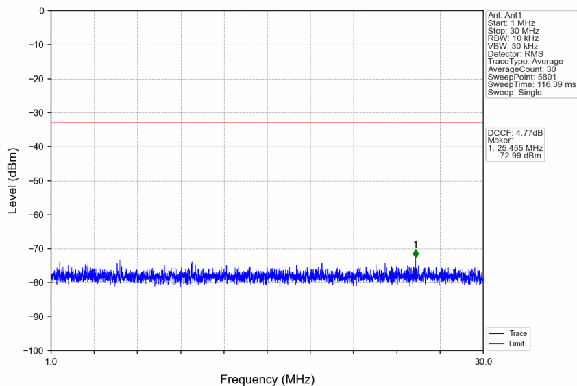
n77a_15kHz_SISO_NTNV_20MHz_CP-OFDM QPSK_3969.99MHz_Edge_1RB_Right
