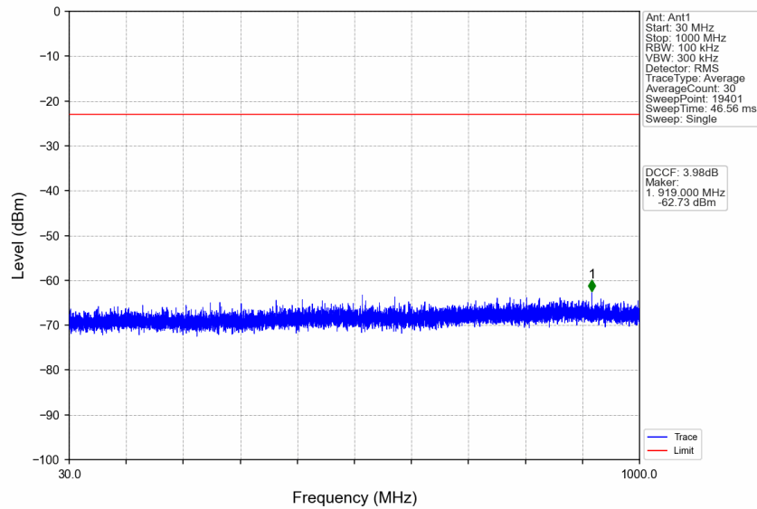
n77a_15kHz_SISO_NTNV_20MHz_DFT-s-OFDM PI/2 BPSK_3969.99MHz_Edge_1RB_Right
