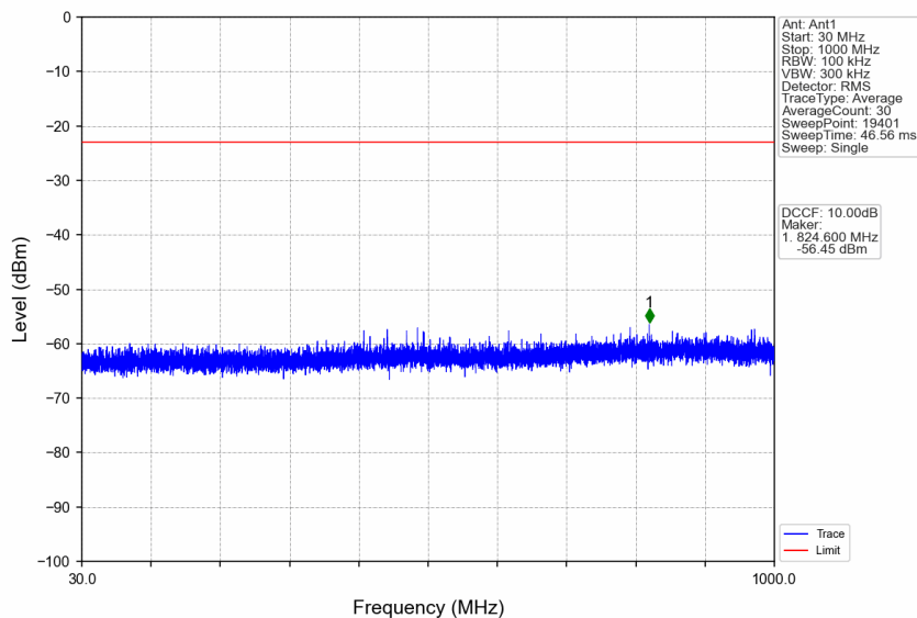
n77a_15kHz_SISO_NTNV_20MHz_DFT-s-OFDM_QPSK_3710.01MHz_Edge_1RB_Left
