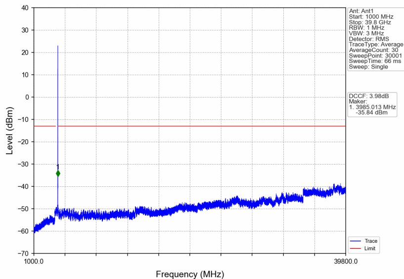
n77a_15kHz_SISO_NTNV_15MHz_CP-OFDM QPSK_3972.495MHz_Edge_1RB_Right
