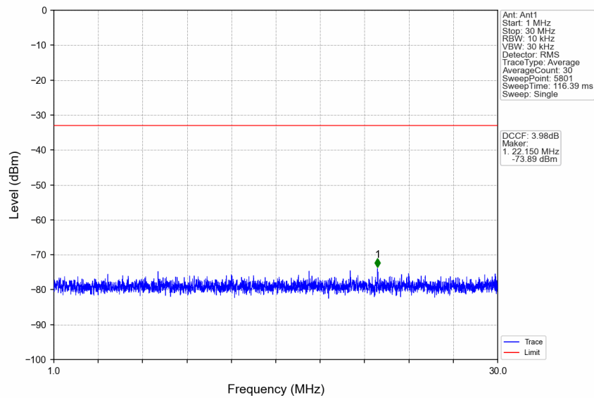
n77a_15kHz_SISO_NTNV_25MHz_DFT-s-OFDM PI/2 BPSK_3712.5MHz_Edge_1RB_Left
