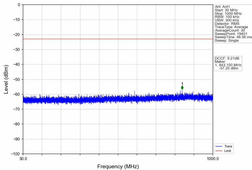
n77a_15kHz_SISO_NTNV_20MHz_CP-OFDM_QPSK_3840MHz_Edge_1RB_Left
