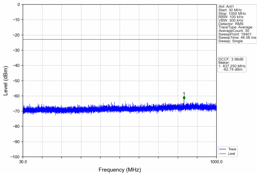
n77a_15kHz_SISO_NTNV_15MHz_CP-OFDM QPSK_3972.495MHz_Edge_1RB_Right
