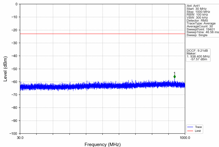
n77a_15kHz_SISO_NTNV_15MHz_CP-OFDM QPSK_3840MHz_Edge_1RB_Left
