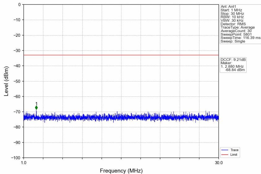
n77a_15kHz_SISO_NTNV_15MHz_DFT-s-OFDM QPSK_3707.505MHz_Edge_1RB_Left
