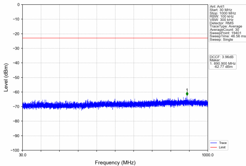
n77a_15kHz_SISO_NTNV_10MHz_DFT-s-OFDM QPSK_3840MHz_Edge_1RB_Left
