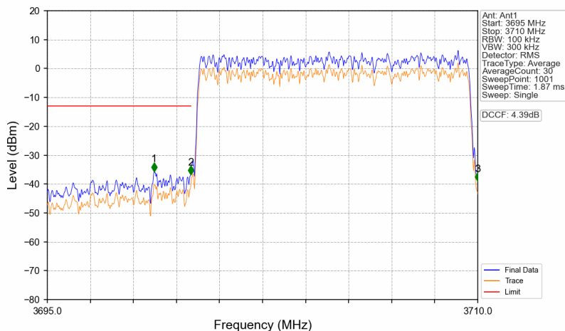
n77a_15kHz_SISO_NTNV_10MHz_CP-OFDM QPSK_3705MHz_Outer_Full
