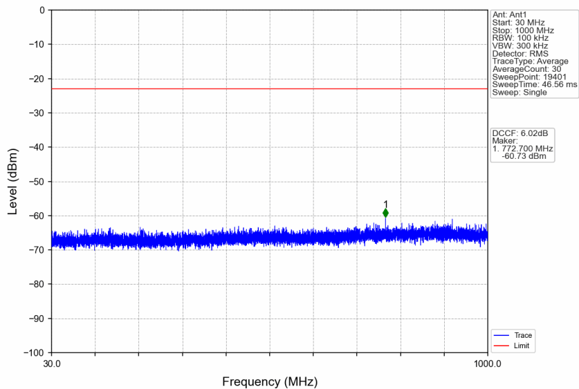
n77a_15kHz_SISO_NTNV_10MHz_DFT-s-OFDM PI/2 BPSK_3975MHz_Edge_1RB_Right
