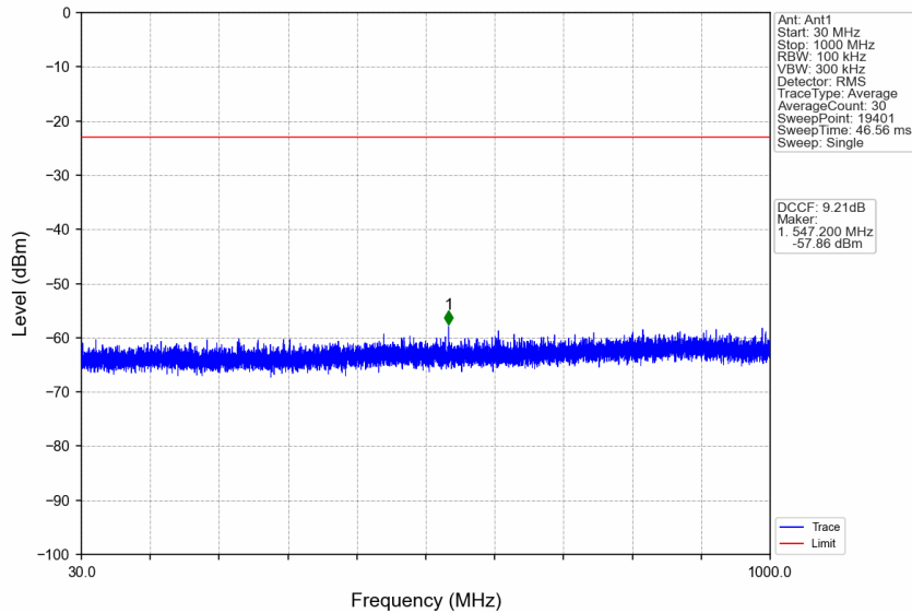
n77a_15kHz_SISO_NTNV_15MHz_DFT-s-OFDM_QPSK_3840MHz_Edge_1RB_Left
