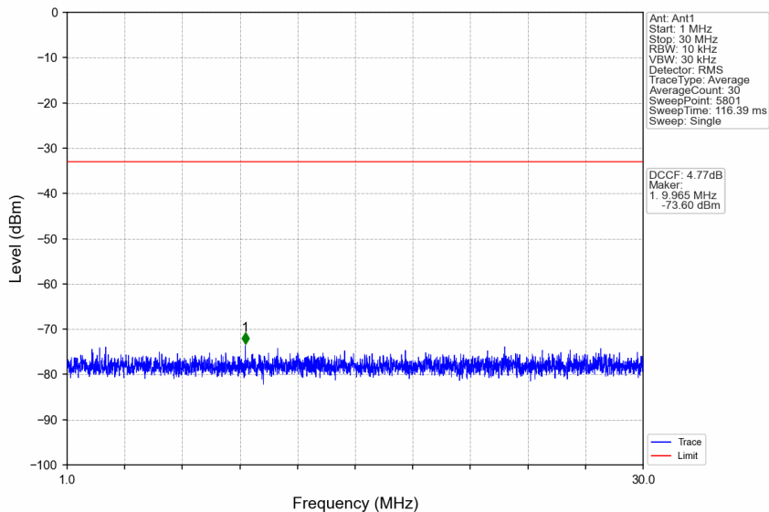
n77a_15kHz_SISO_NTNV_10MHz_CP-OFDM QPSK_3975MHz_Edge_1RB_Right
