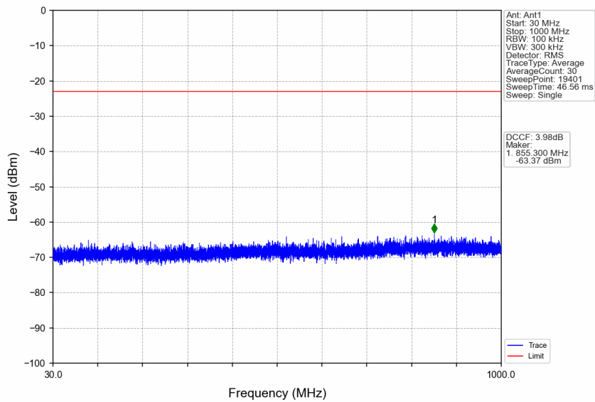
n77a_15kHz_SISO_NTNV_15MHz_DFT-s-OFDM_QPSK_3972.495MHz_Edge_1RB_Right
