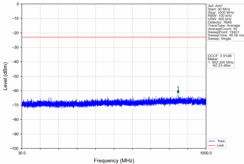
n77a_15kHz_SISO_NTNV_15MHz_DFT-s-OFDM PI/2 BPSK_3840MHz_Edge_1RB_Left
