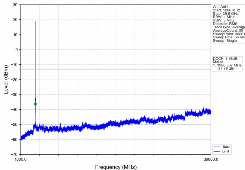
n77a_15kHz_SISO_NTNV_15MHz_DFT-s-OFDM PI/2 BPSK_3972.495MHz_Edge_1RB_Right
