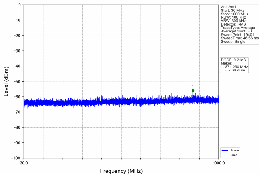
n77a_15kHz_SISO_NTNV_15MHz_DFT-s-OFDM QPSK_3707.505MHz_Edge_1RB_Left
