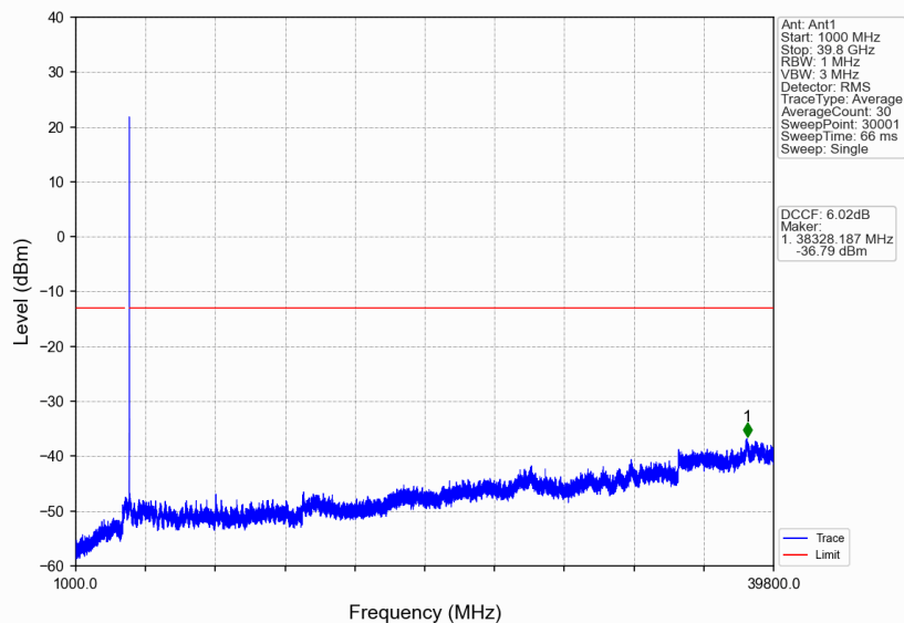
n77a_15kHz_SISO_NTNV_10MHz_DFT-s-OFDM PI/2 BPSK_3975MHz_Edge_1RB_Right
