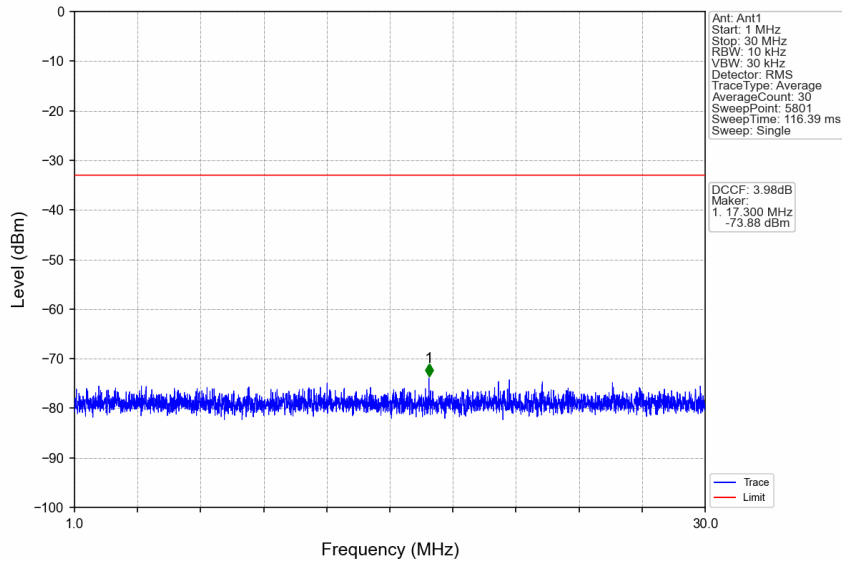
n77a_15kHz_SISO_NTNV_15MHz_DFT-s-OFDM_QPSK_3972.495MHz_Edge_1RB_Right
