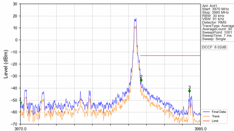
n77a_15kHz_SISO_NTNV_10MHz_DFT-s-OFDM PI/2 BPSK_3975MHz_Edge_1RB_Right
