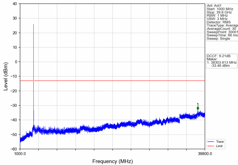
n77a_15kHz_SISO_NTNV_15MHz_DFT-s-OFDM QPSK_3972.495MHz_Edge_1RB_Right
