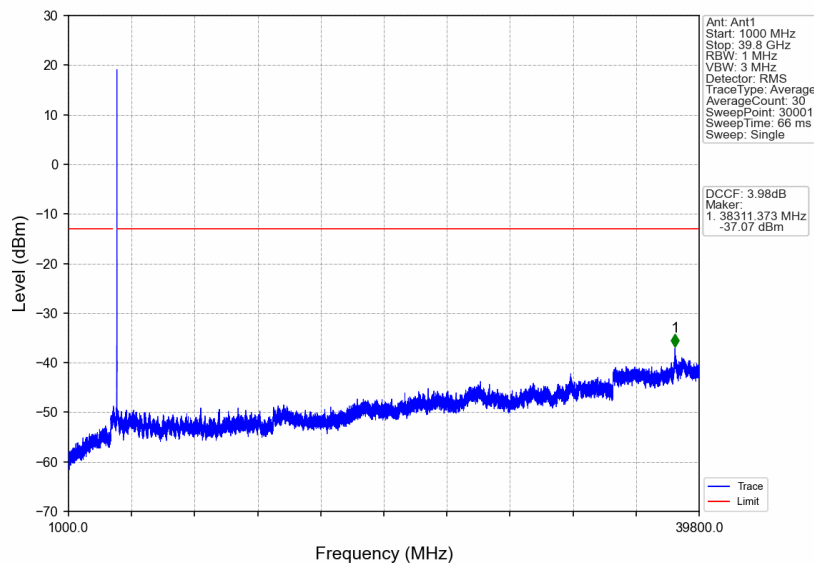
n77a_15kHz_SISO_NTNV_15MHz_DFT-s-OFDM_QPSK_3972.495MHz_Edge_1RB_Right
