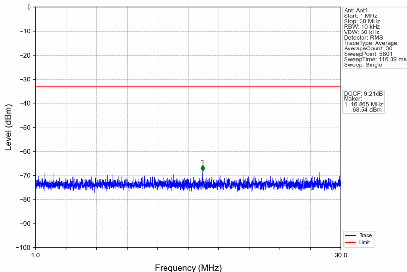
n77a_15kHz_SISO_NTNV_15MHz_CP-OFDM QPSK_3707.505MHz_Edge_1RB_Left
