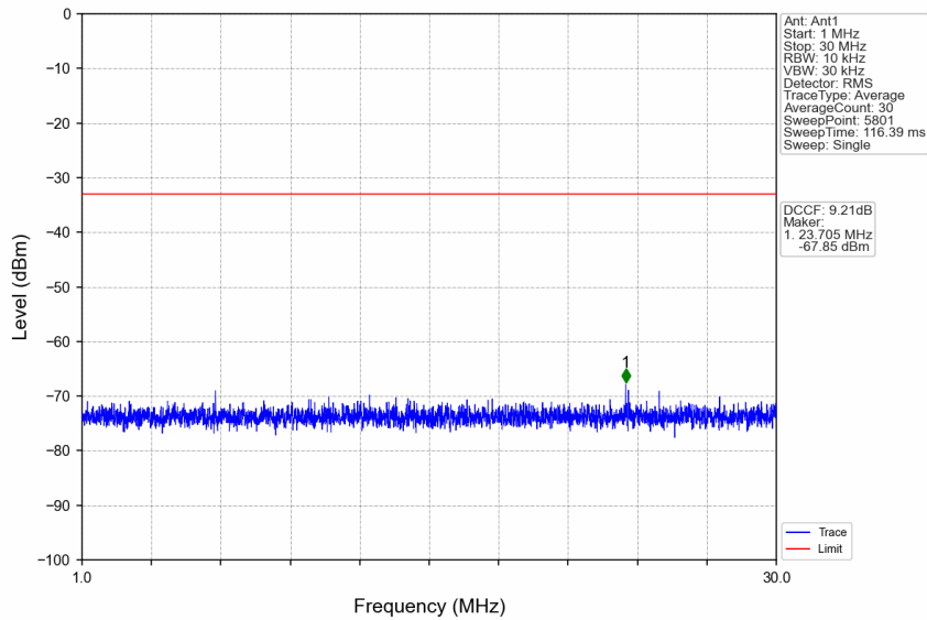
n77a_15kHz_SISO_NTNV_15MHz_DFT-s-OFDM_QPSK_3840MHz_Edge_1RB_Left
