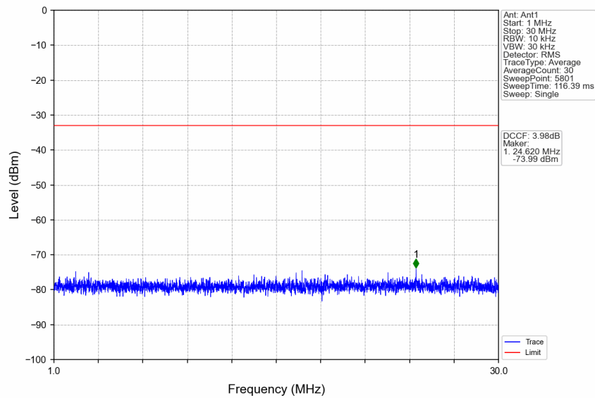
n77a_15kHz_SISO_NTNV_10MHz_CP-OFDM QPSK_3840MHz_Edge_1RB_Left
