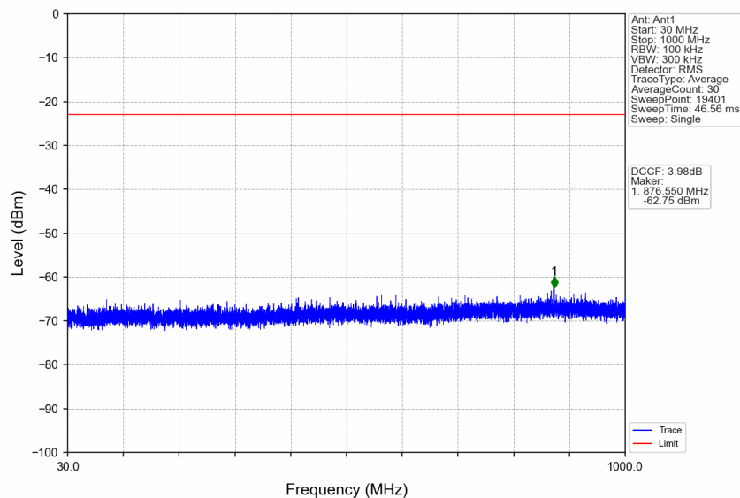
n77a_15kHz_SISO_NTNV_10MHz_CP-OFDM QPSK_3705MHz_Edge_1RB_Left
