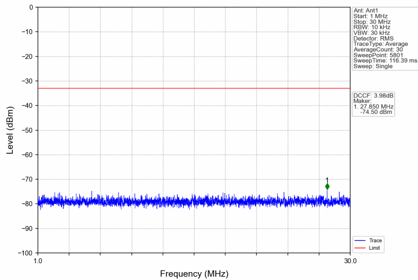
n77a_15kHz_SISO_NTNV_10MHz_DFT-s-OFDM QPSK_3705MHz_Edge_1RB_Left
