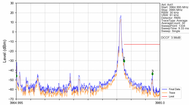
n77a_15kHz_SISO_NTNV_15MHz_DFT-s-OFDM QPSK_3972.495MHz_Edge_1RB_Right
