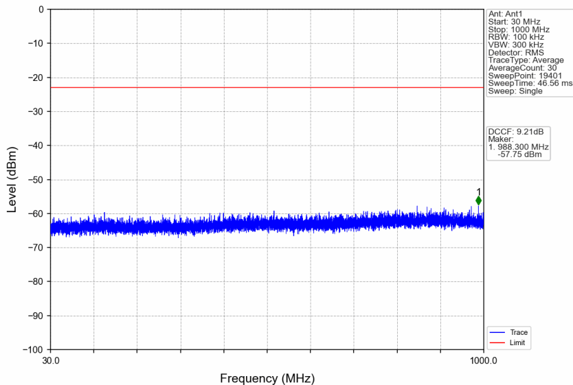
n77a_15kHz_SISO_NTNV_15MHz_CP-OFDM QPSK_3707.505MHz_Edge_1RB_Left
