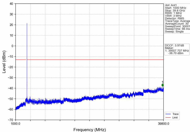
n77a_15kHz_SISO_NTNV_10MHz_DFT-s-OFDM QPSK_3975MHz_Edge_1RB_Right
