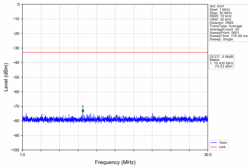
n77a_15kHz_SISO_NTNV_10MHz_CP-OFDM QPSK_3705MHz_Edge_1RB_Left
