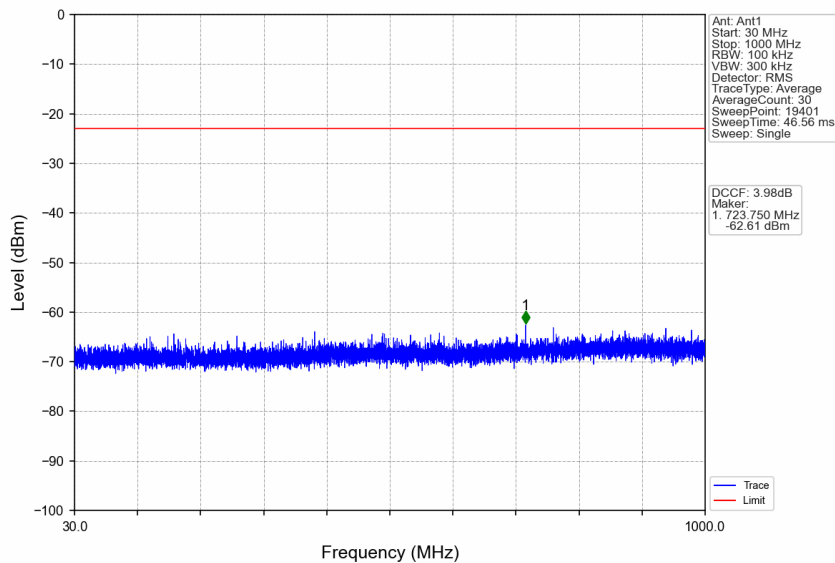
n77a_15kHz_SISO_NTNV_15MHz_DFT-s-OFDM PI/2 BPSK_3972.495MHz_Edge_1RB_Right
