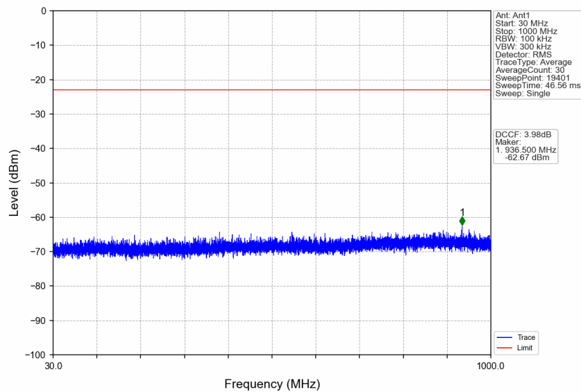
n77a_15kHz_SISO_NTNV_10MHz_DFT-s-OFDM QPSK_3705MHz_Edge_1RB_Left
