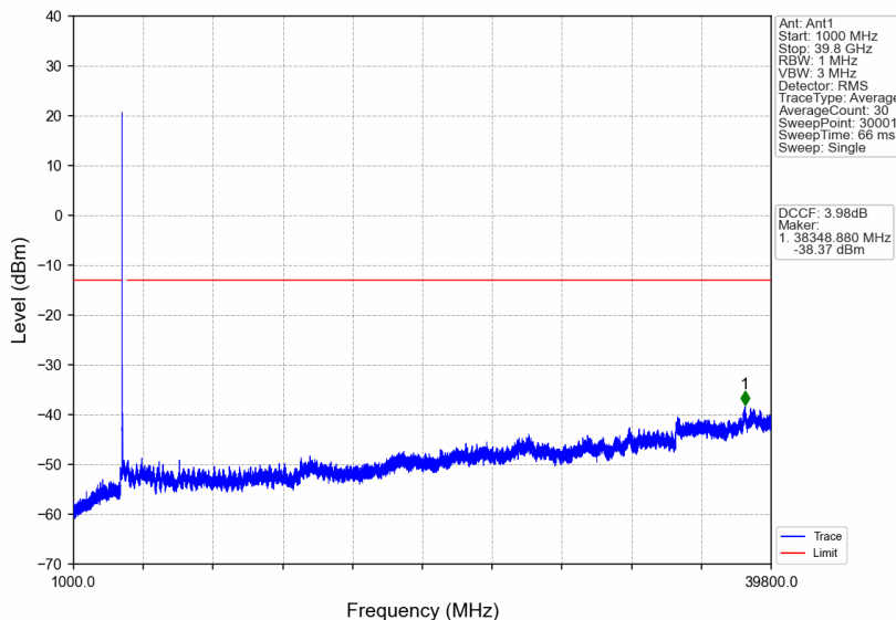
n77a_15kHz_SISO_NTNV_10MHz_CP-OFDM QPSK_3705MHz_Outer_Full
