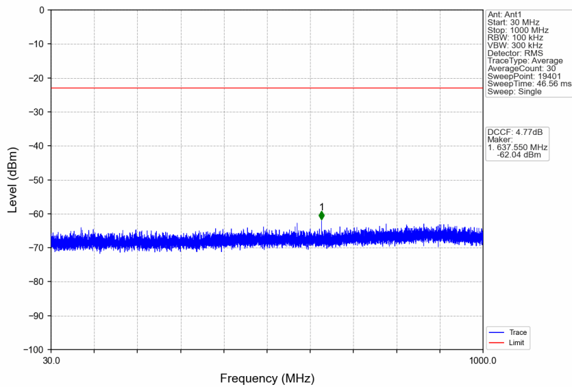
n77a_15kHz_SISO_NTNV_10MHz_CP-OFDM QPSK_3975MHz_Edge_1RB_Right
