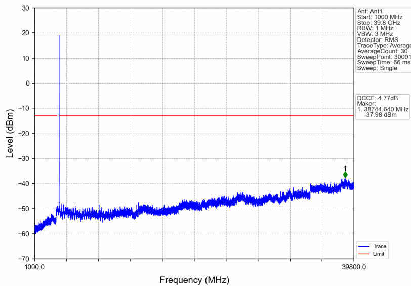
n77a_15kHz_SISO_NTNV_10MHz_CP-OFDM QPSK_3975MHz_Edge_1RB_Right
