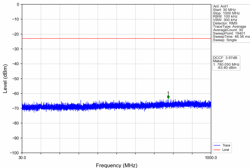
n77a_15kHz_SISO_NTNV_10MHz_DFT-s-OFDM QPSK_3975MHz_Edge_1RB_Right
