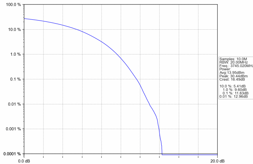
n77a_30kHz_SISO_NTNV_90MHz_CP-OFDM 16 QAM_3745.02MHz_Outer_Full
