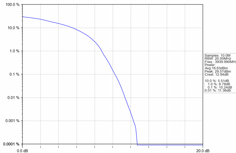
n77a_30kHz_SISO_NTNV_80MHz_DFT-s-OFDM QPSK_3939.99MHz_Outer_Full
