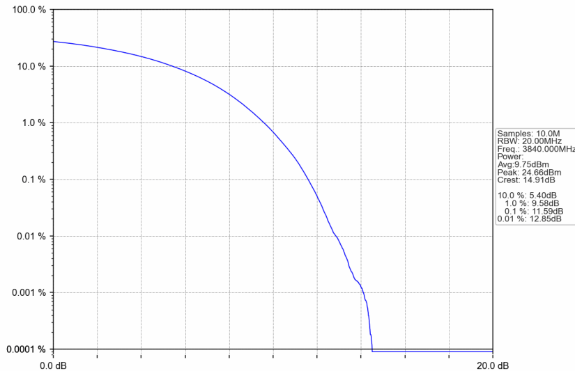
n77a_30kHz_SISO_NTNV_100MHz_CP-OFDM 256 QAM_3840MHz_Outer_Full
