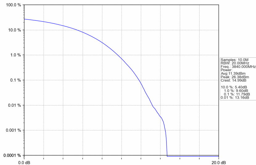
n77a_30kHz_SISO_NTNV_70MHz_CP-OFDM 256 QAM_3840MHz_Outer_Full
