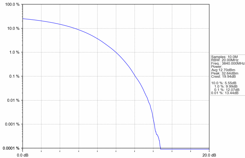
n77a_30kHz_SISO_NTNV_100MHz_CP-OFDM QPSK_3840MHz_Outer_Full
