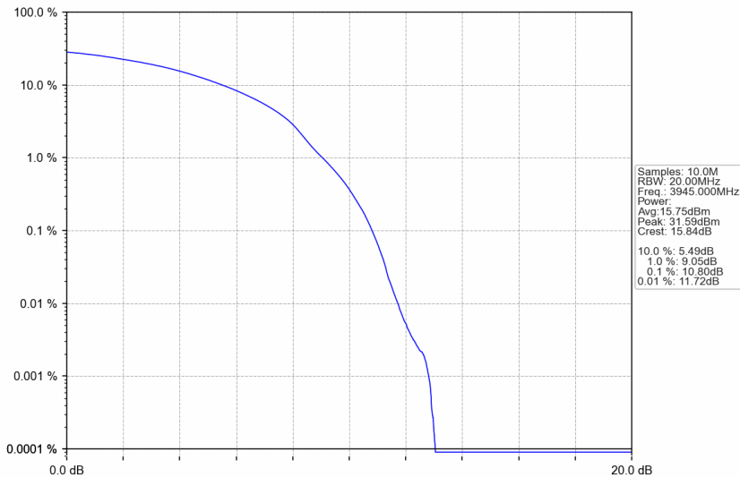
n77a_30kHz_SISO_NTNV_70MHz_DFT-s-OFDM 64 QAM_3945MHz_Outer_Full
