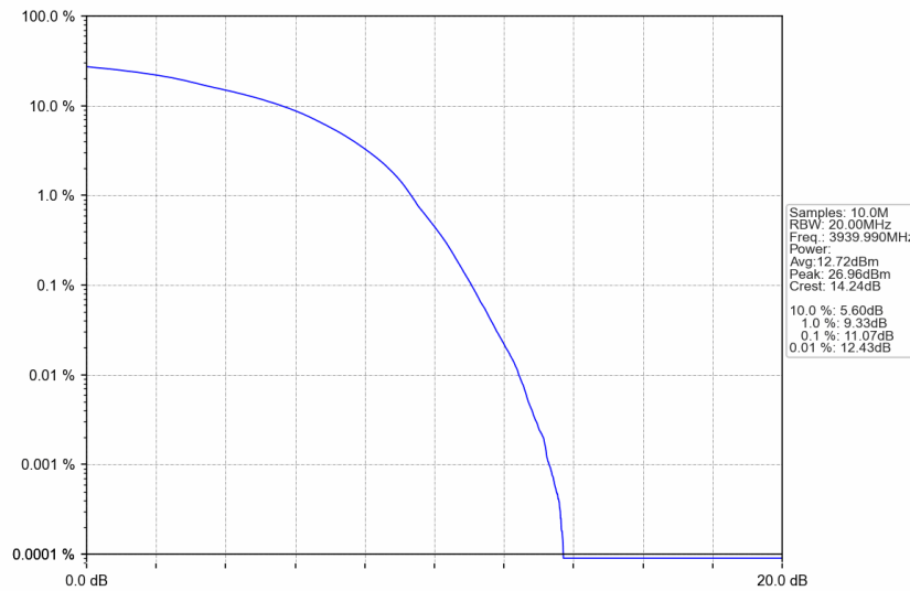
n77a_30kHz_SISO_NTNV_80MHz_DFT-s-OFDM 256 QAM_3939.99MHz_Outer_Full
