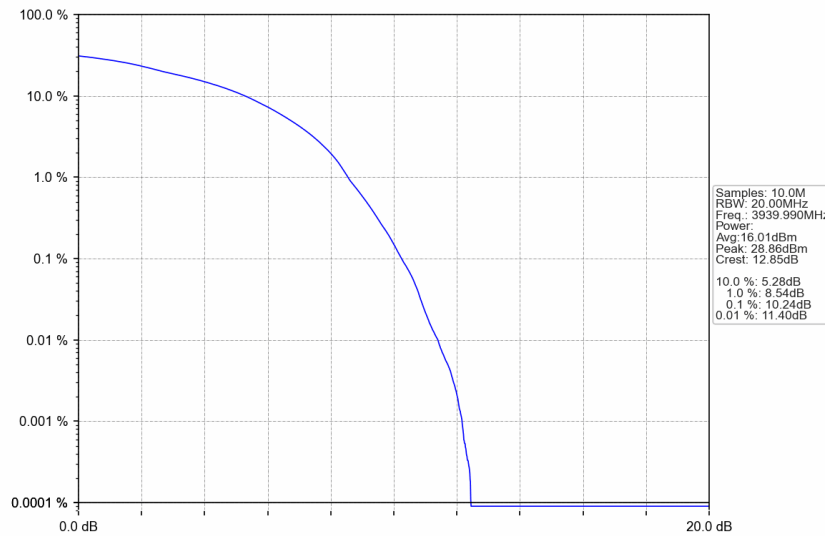
n77a_30kHz_SISO_NTNV_80MHz_DFT-s-OFDM 16 QAM_3939.99MHz_Outer_Full
