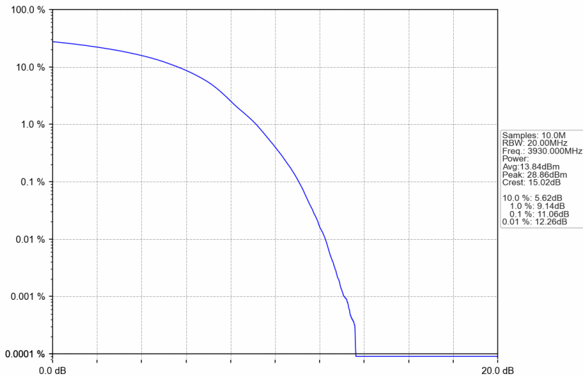
n77a_30kHz_SISO_NTNV_100MHz_DFT-s-OFDM 64 QAM_3930MHz_Outer_Full
