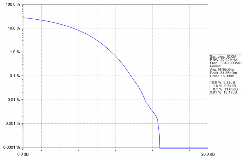
n77a_30kHz_SISO_NTNV_70MHz_CP-OFDM QPSK_3840MHz_Outer_Full
