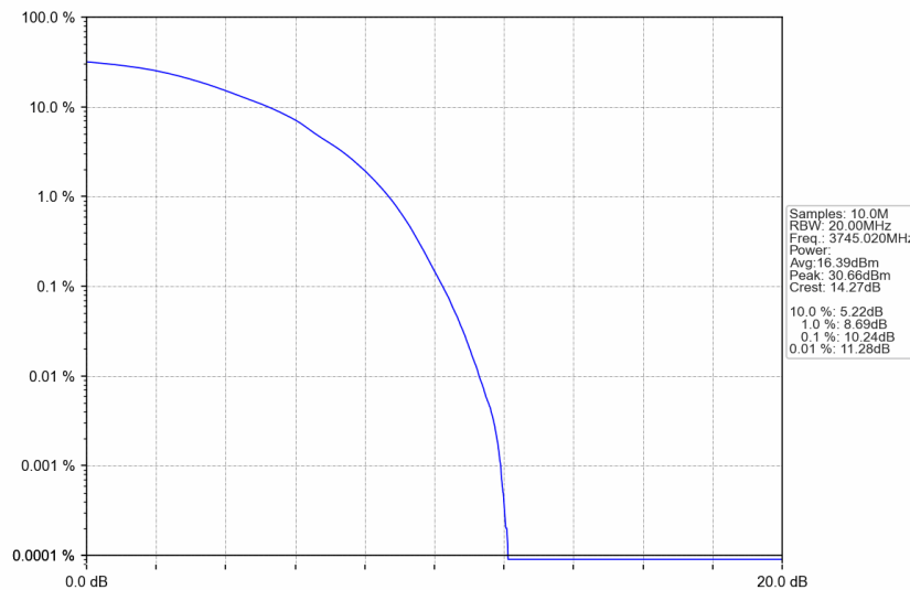
n77a_30kHz_SISO_NTNV_90MHz_DFT-s-OFDM QPSK_3745.02MHz_Outer_Full
