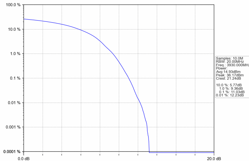
n77a_30kHz_SISO_NTNV_100MHz_DFT-s-OFDM QPSK_3930MHz_Outer_Full
