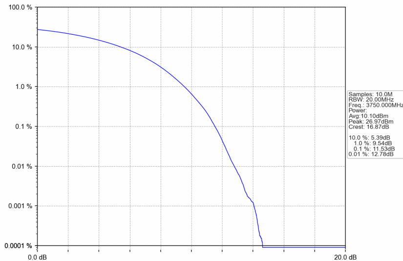
n77a_30kHz_SISO_NTNV_100MHz_CP-OFDM 256 QAM_3750MHz_Outer_Full
