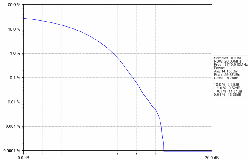
n77a_30kHz_SISO_NTNV_80MHz_CP-OFDM 64 QAM_3740.01MHz_Outer_Full
