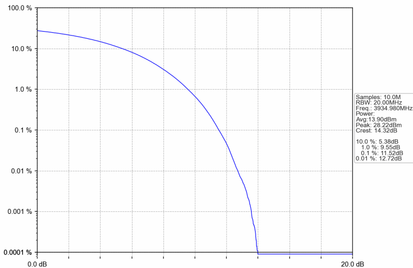
n77a_30kHz_SISO_NTNV_90MHz_CP-OFDM QPSK_3934.98MHz_Outer_Full
