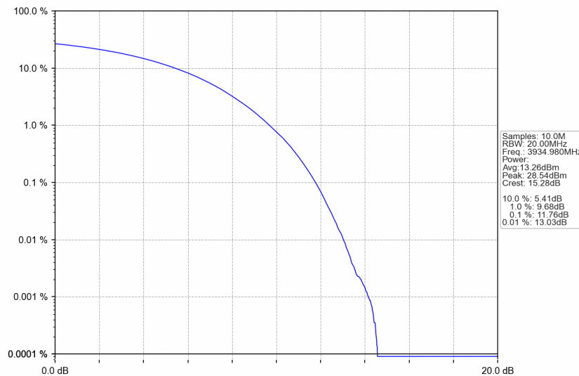
n77a_30kHz_SISO_NTNV_90MHz_CP-OFDM 64 QAM_3934.98MHz_Outer_Full
