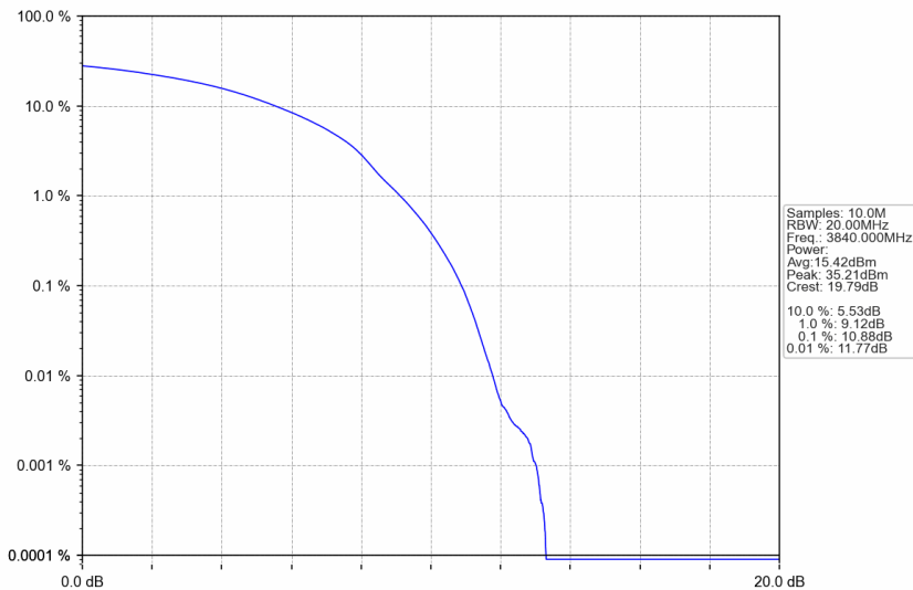
n77a_30kHz_SISO_NTNV_70MHz_DFT-s-OFDM 64 QAM_3840MHz_Outer_Full
