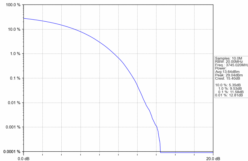
n77a_30kHz_SISO_NTNV_90MHz_CP-OFDM 64 QAM_3745.02MHz_Outer_Full
