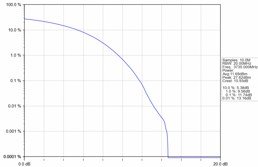
n77a_30kHz_SISO_NTNV_70MHz_CP-OFDM 256 QAM_3735MHz_Outer_Full
