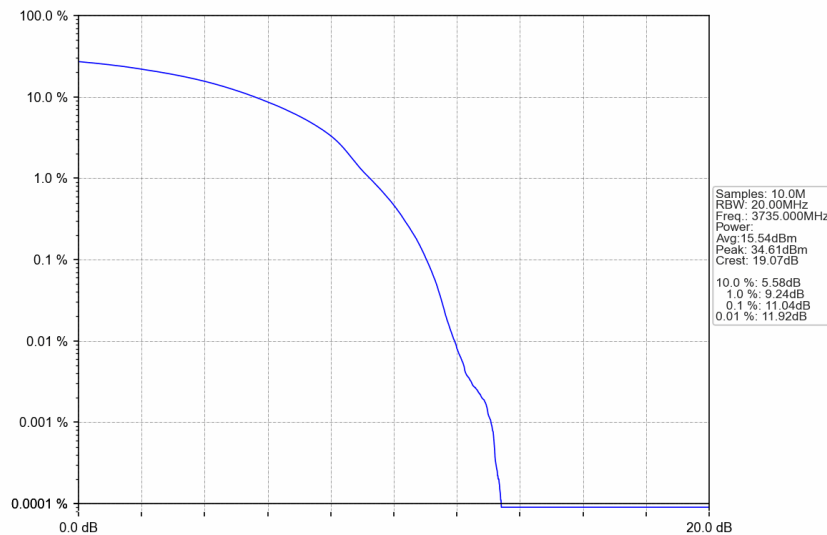
n77a_30kHz_SISO_NTNV_70MHz_DFT-s-OFDM 64 QAM_3735MHz_Outer_Full
