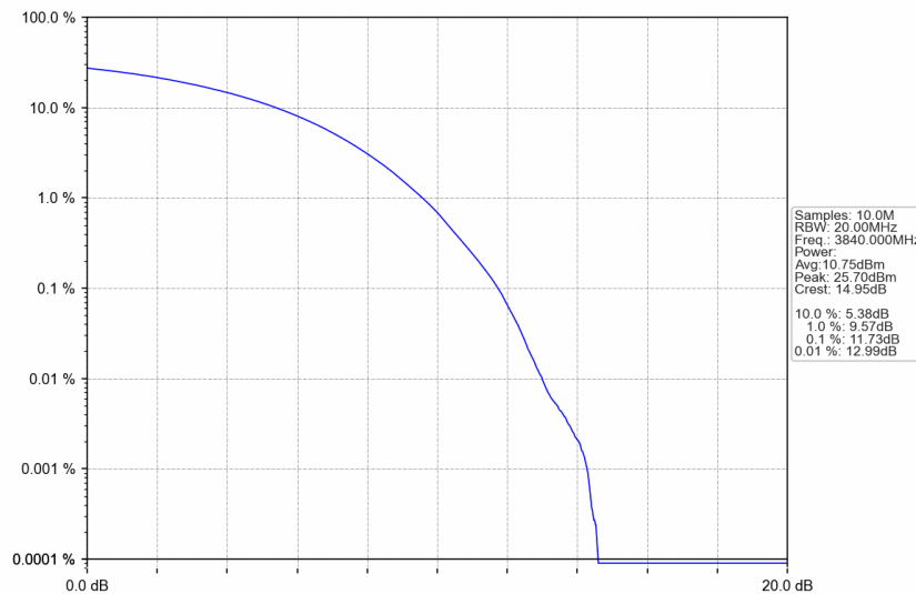
n77a_30kHz_SISO_NTNV_80MHz_CP-OFDM 256 QAM_3840MHz_Outer_Full
