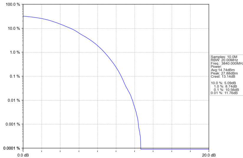
n77a_30kHz_SISO_NTNV_90MHz_DFT-s-OFDM 64 QAM_3840MHz_Outer_Full
