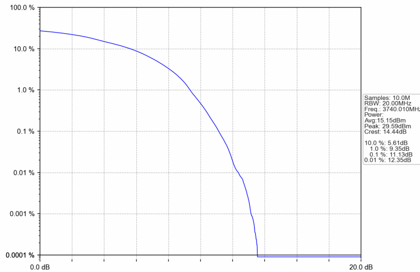
n77a_30kHz_SISO_NTNV_80MHz_DFT-s-OFDM 16 QAM_3740.01MHz_Outer_Full
