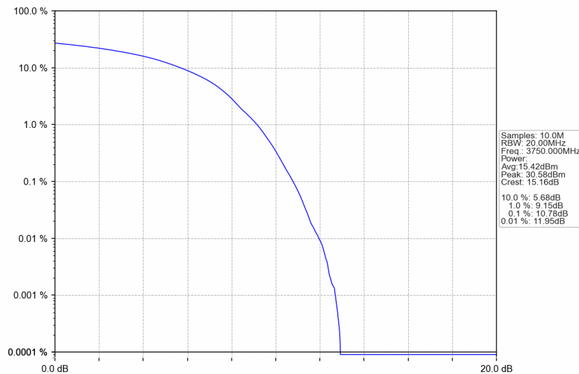
n77a_30kHz_SISO_NTNV_100MHz_DFT-s-OFDM QPSK_3750MHz_Outer_Full
