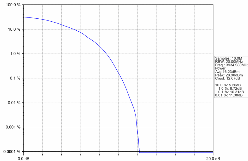
n77a_30kHz_SISO_NTNV_90MHz_DFT-s-OFDM QPSK_3934.98MHz_Outer_Full
