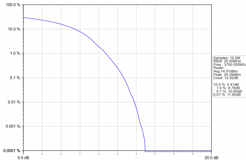
n77a_30kHz_SISO_NTNV_100MHz_DFT-s-OFDM 64 QAM_3750MHz_Outer_Full
