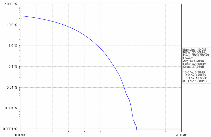
n77a_30kHz_SISO_NTNV_80MHz_CP-OFDM QPSK_3939.99MHz_Outer_Full
