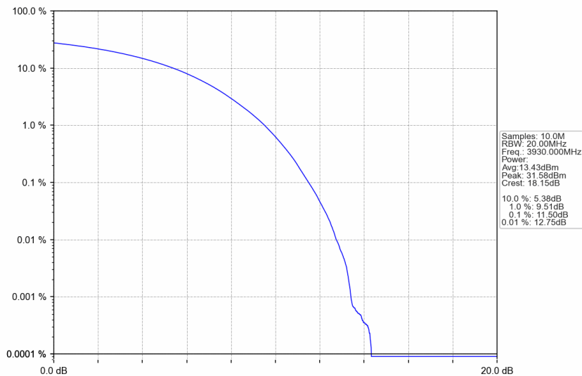
n77a_30kHz_SISO_NTNV_100MHz_CP-OFDM QPSK_3930MHz_Outer_Full
