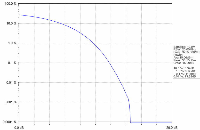
n77a_30kHz_SISO_NTNV_70MHz_CP-OFDM 16 QAM_3735MHz_Outer_Full
