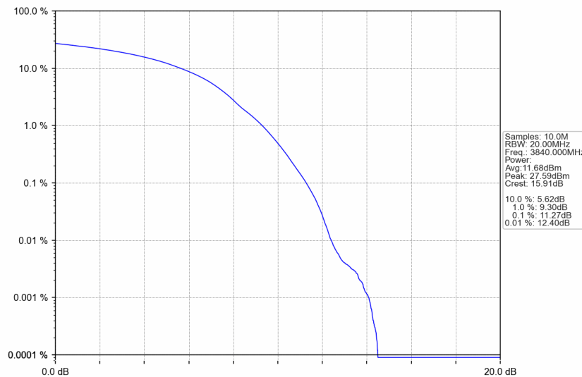
n77a_30kHz_SISO_NTNV_100MHz_DFT-s-OFDM 256 QAM_3840MHz_Outer_Full
