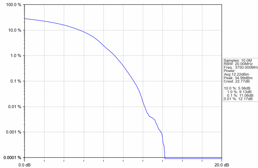
n77a_30kHz_SISO_NTNV_100MHz_DFT-s-OFDM 256 QAM_3750MHz_Outer_Full
