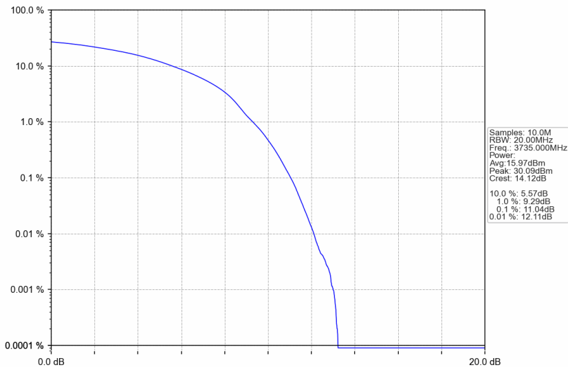
n77a_30kHz_SISO_NTNV_70MHz_DFT-s-OFDM 16 QAM_3735MHz_Outer_Full
