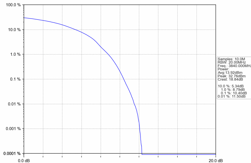
n77a_30kHz_SISO_NTNV_70MHz_DFT-s-OFDM 256 QAM_3840MHz_Outer_Full
