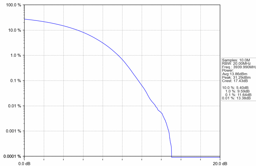
n77a_30kHz_SISO_NTNV_80MHz_CP-OFDM 64 QAM_3939.99MHz_Outer_Full
