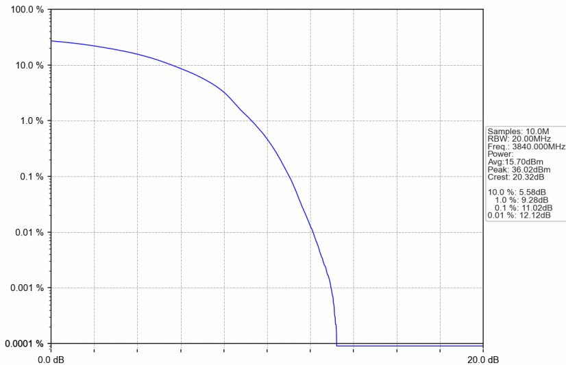
n77a_30kHz_SISO_NTNV_70MHz_DFT-s-OFDM 16 QAM_3840MHz_Outer_Full
