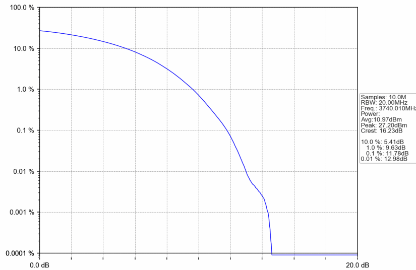
n77a_30kHz_SISO_NTNV_80MHz_CP-OFDM 256 QAM_3740.01MHz_Outer_Full
