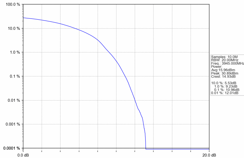
n77a_30kHz_SISO_NTNV_70MHz_DFT-s-OFDM 16 QAM_3945MHz_Outer_Full
