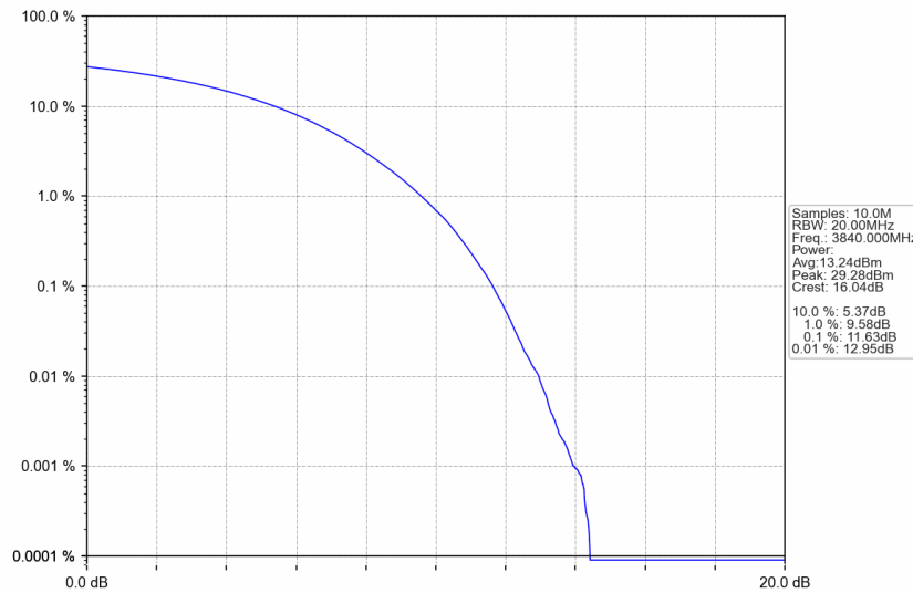
n77a_30kHz_SISO_NTNV_90MHz_CP-OFDM 64 QAM_3840MHz_Outer_Full
