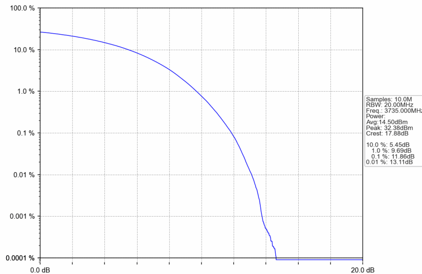
n77a_30kHz_SISO_NTNV_70MHz_CP-OFDM 64 QAM_3735MHz_Outer_Full
