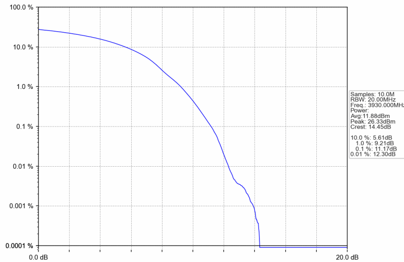
n77a_30kHz_SISO_NTNV_100MHz_DFT-s-OFDM 256 QAM_3930MHz_Outer_Full
