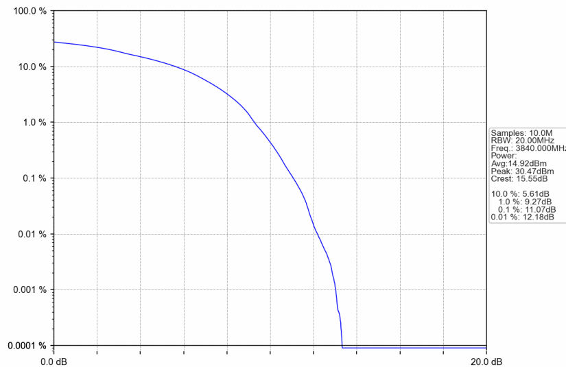
n77a_30kHz_SISO_NTNV_80MHz_DFT-s-OFDM 16 QAM_3840MHz_Outer_Full
