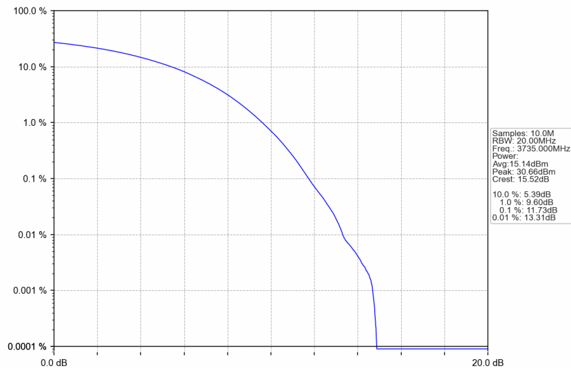
n77a_30kHz_SISO_NTNV_70MHz_CP-OFDM QPSK_3735MHz_Outer_Full
