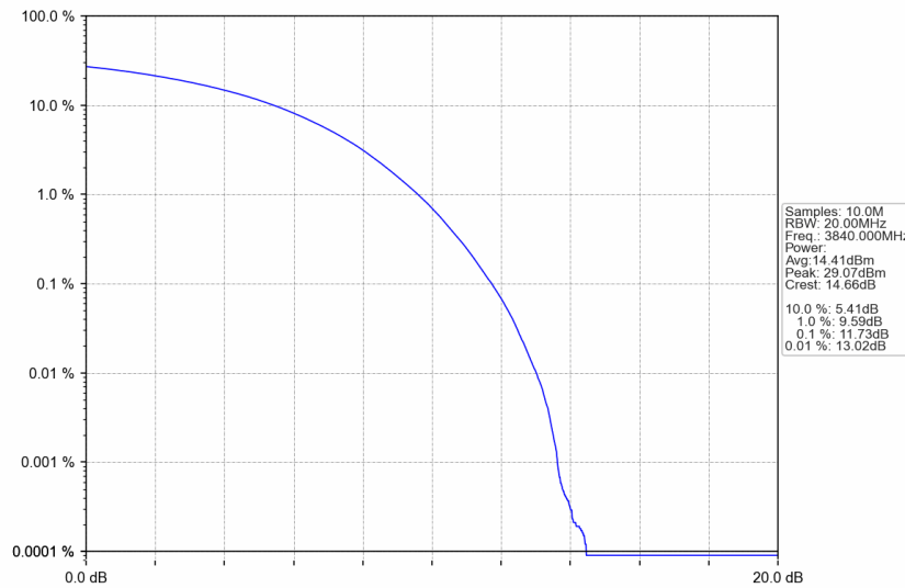
n77a_30kHz_SISO_NTNV_70MHz_CP-OFDM 64 QAM_3840MHz_Outer_Full
