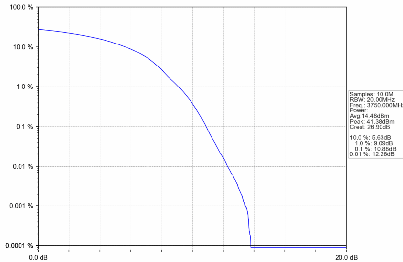
n77a_30kHz_SISO_NTNV_100MHz_DFT-s-OFDM 16 QAM_3750MHz_Outer_Full
