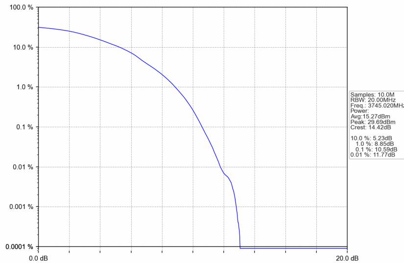
n77a_30kHz_SISO_NTNV_90MHz_DFT-s-OFDM 16 QAM_3745.02MHz_Outer_Full
