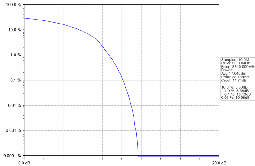
n77a_30kHz_SISO_NTNV_70MHz_DFT-s-OFDM QPSK_3840MHz_Outer_Full
