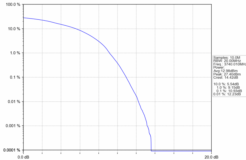
n77a_30kHz_SISO_NTNV_80MHz_DFT-s-OFDM 256 QAM_3740.01MHz_Outer_Full
