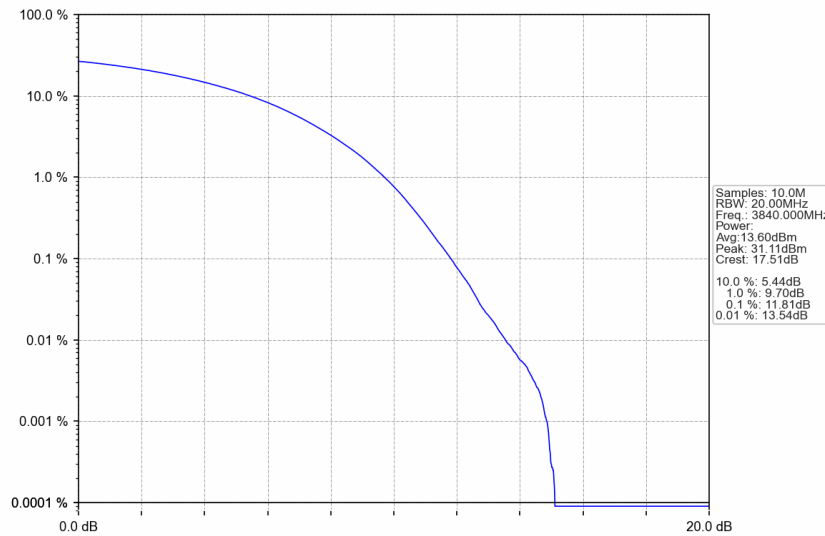
n77a_30kHz_SISO_NTNV_80MHz_CP-OFDM 64 QAM_3840MHz_Outer_Full
