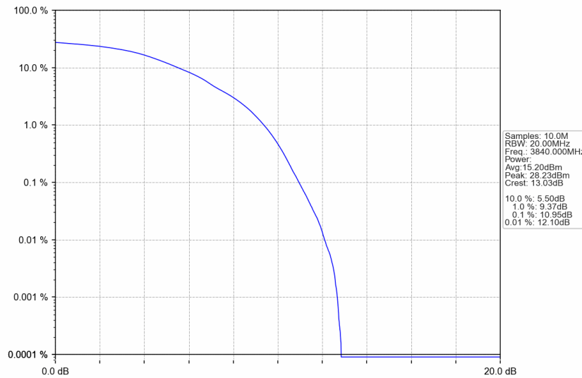
n77a_30kHz_SISO_NTNV_90MHz_DFT-s-OFDM QPSK_3840MHz_Outer_Full
