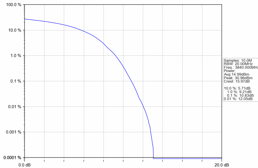
n77a_30kHz_SISO_NTNV_100MHz_DFT-s-OFDM QPSK_3840MHz_Outer_Full
