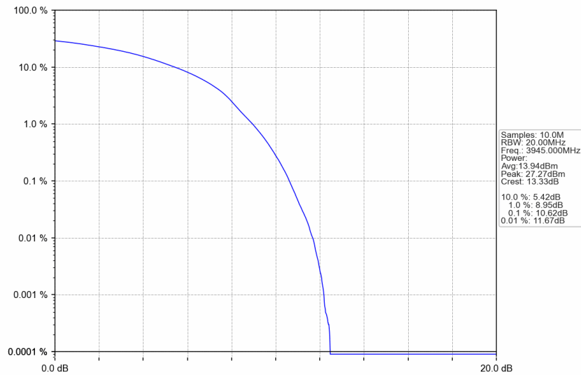
n77a_30kHz_SISO_NTNV_70MHz_DFT-s-OFDM 256 QAM_3945MHz_Outer_Full
