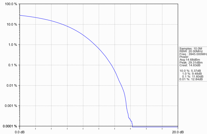
n77a_30kHz_SISO_NTNV_70MHz_CP-OFDM 64 QAM_3945MHz_Outer_Full
