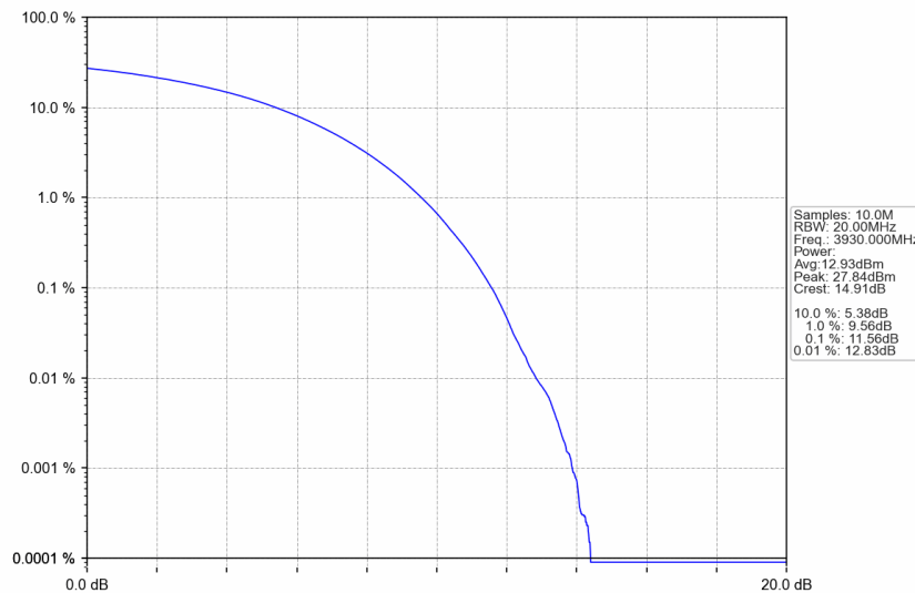
n77a_30kHz_SISO_NTNV_100MHz_CP-OFDM 64 QAM_3930MHz_Outer_Full
