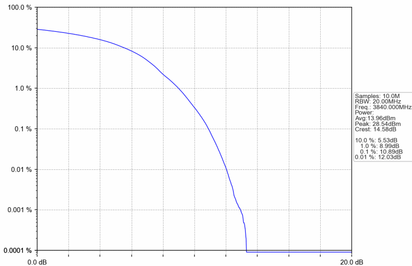
n77a_30kHz_SISO_NTNV_100MHz_DFT-s-OFDM 64 QAM_3840MHz_Outer_Full
