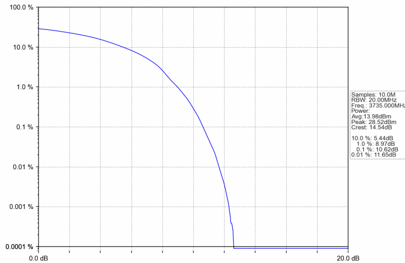
n77a_30kHz_SISO_NTNV_70MHz_DFT-s-OFDM 256 QAM_3735MHz_Outer_Full
