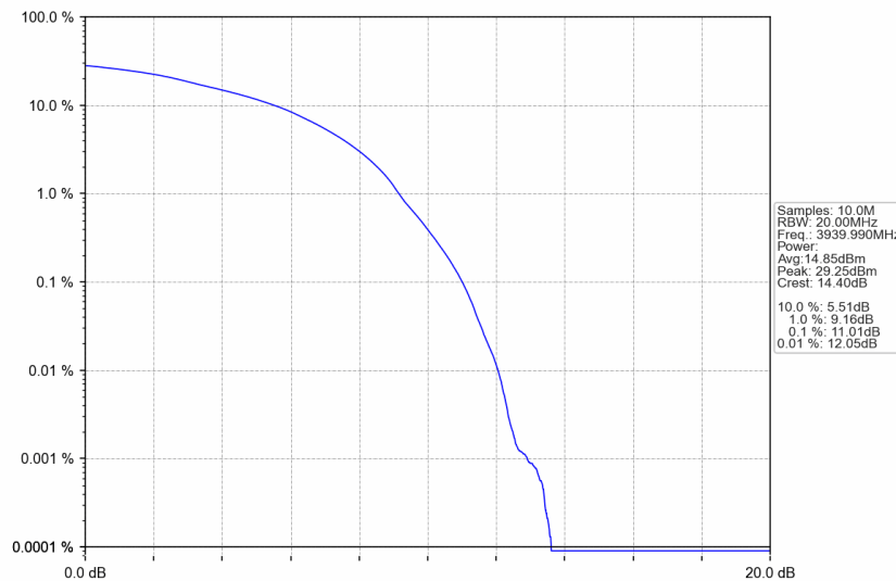
n77a_30kHz_SISO_NTNV_80MHz_DFT-s-OFDM 64 QAM_3939.99MHz_Outer_Full
