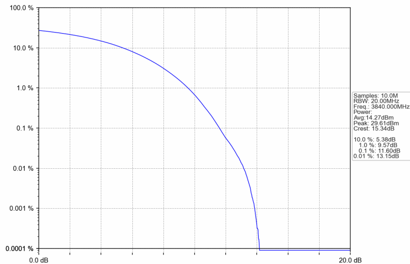
n77a_30kHz_SISO_NTNV_80MHz_CP-OFDM 16 QAM_3840MHz_Outer_Full
