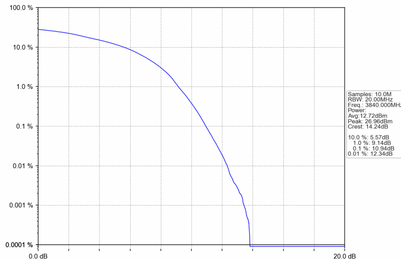
n77a_30kHz_SISO_NTNV_80MHz_DFT-s-OFDM 256 QAM_3840MHz_Outer_Full
