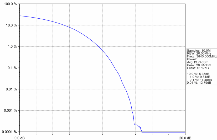
n77a_30kHz_SISO_NTNV_90MHz_CP-OFDM QPSK_3840MHz_Outer_Full
