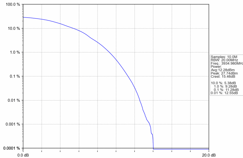
n77a_30kHz_SISO_NTNV_90MHz_DFT-s-OFDM 256 QAM_3934.98MHz_Outer_Full
