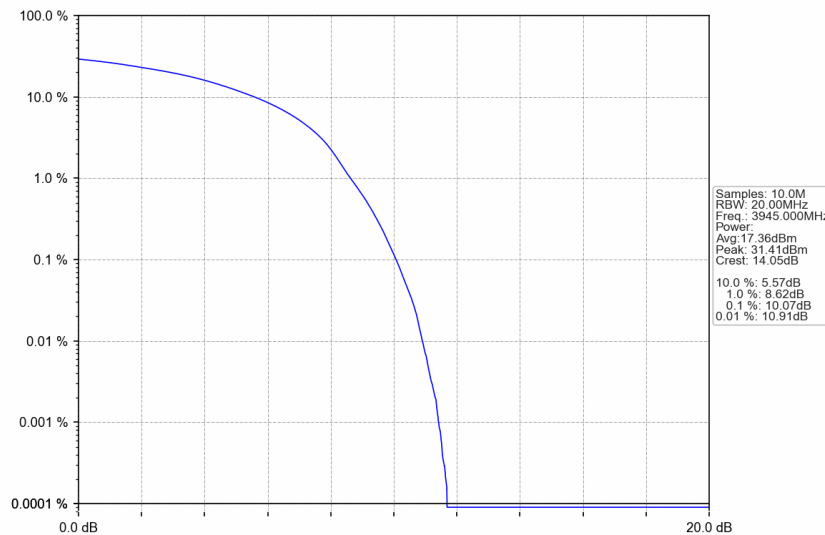
n77a_30kHz_SISO_NTNV_70MHz_DFT-s-OFDM QPSK_3945MHz_Outer_Full
