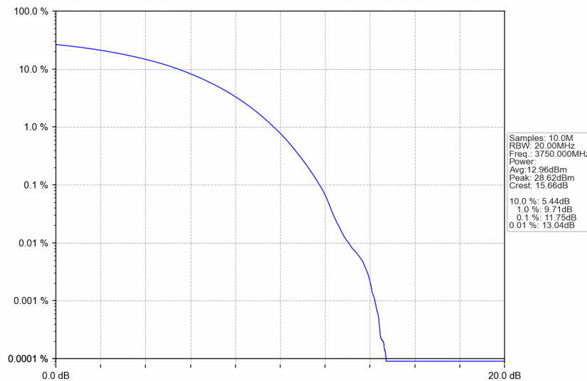
n77a_30kHz_SISO_NTNV_100MHz_CP-OFDM 64 QAM_3750MHz_Outer_Full
