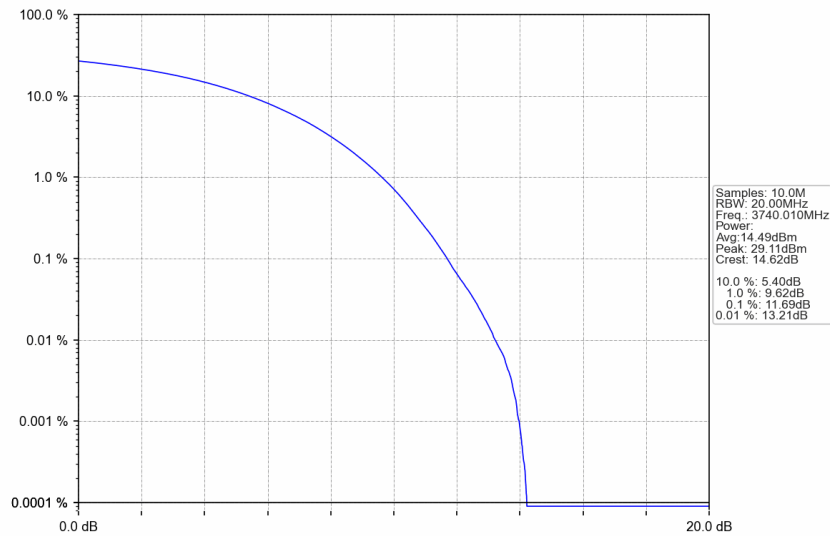
n77a_30kHz_SISO_NTNV_80MHz_CP-OFDM 16 QAM_3740.01MHz_Outer_Full
