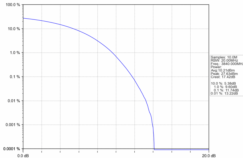
n77a_30kHz_SISO_NTNV_90MHz_CP-OFDM 256 QAM_3840MHz_Outer_Full
