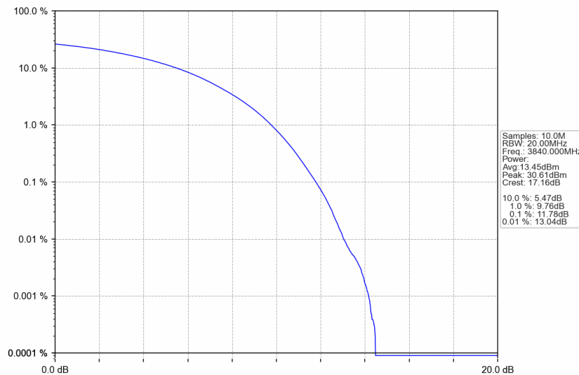
n77a_30kHz_SISO_NTNV_90MHz_CP-OFDM 16 QAM_3840MHz_Outer_Full
