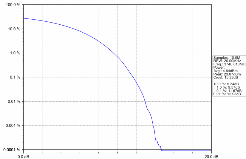
n77a_30kHz_SISO_NTNV_80MHz_CP-OFDM QPSK_3740.01MHz_Outer_Full
