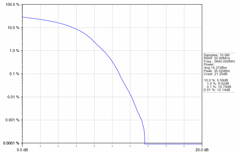
n77a_30kHz_SISO_NTNV_100MHz_DFT-s-OFDM 16 QAM_3840MHz_Outer_Full
