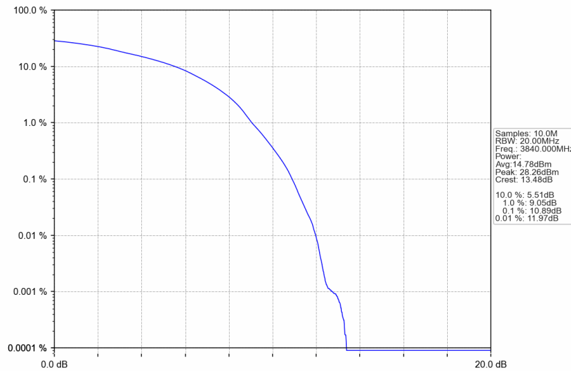
n77a_30kHz_SISO_NTNV_80MHz_DFT-s-OFDM 64 QAM_3840MHz_Outer_Full
