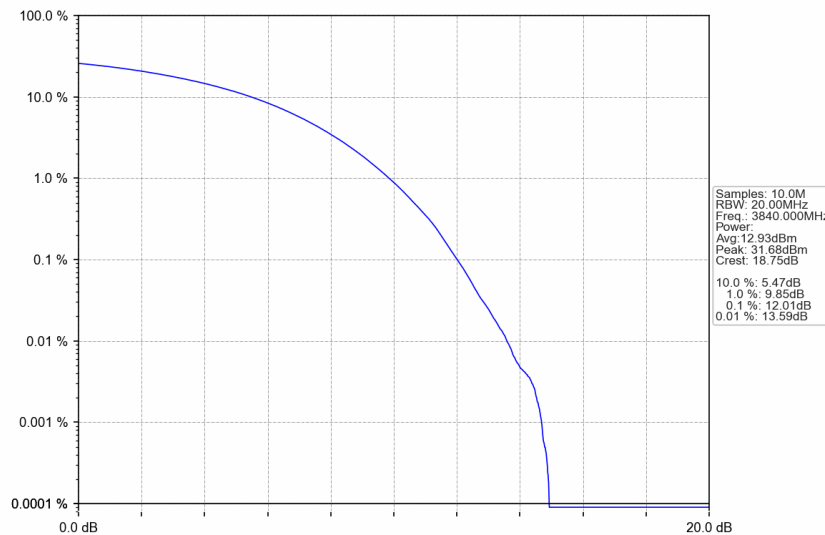
n77a_30kHz_SISO_NTNV_100MHz_CP-OFDM 16 QAM_3840MHz_Outer_Full
