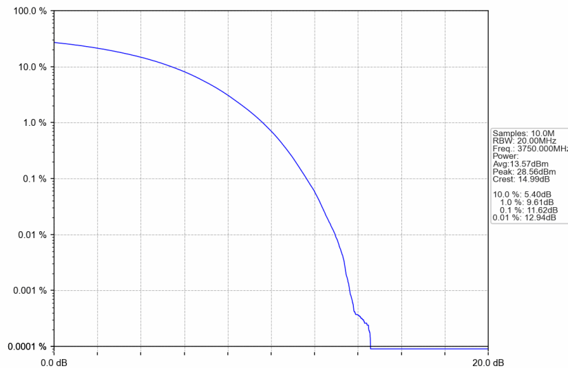
n77a_30kHz_SISO_NTNV_100MHz_CP-OFDM QPSK_3750MHz_Outer_Full
