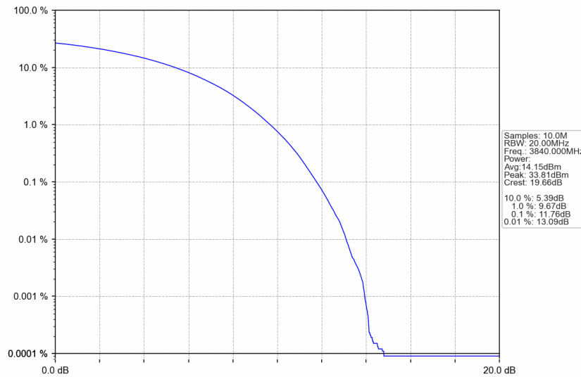
n77a_30kHz_SISO_NTNV_80MHz_CP-OFDM QPSK_3840MHz_Outer_Full
