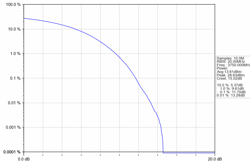
n77a_30kHz_SISO_NTNV_100MHz_CP-OFDM 16 QAM_3750MHz_Outer_Full
