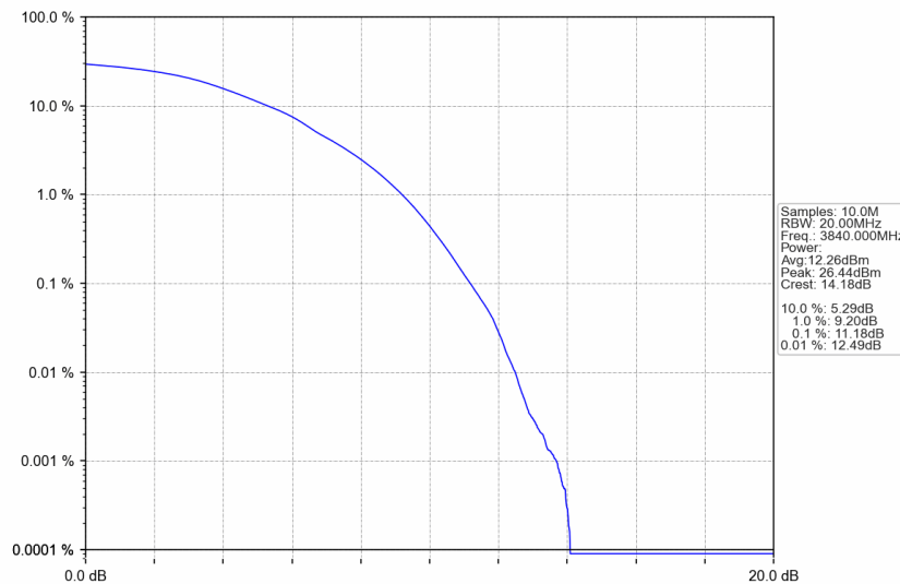
n77a_30kHz_SISO_NTNV_90MHz_DFT-s-OFDM 256 QAM_3840MHz_Outer_Full
