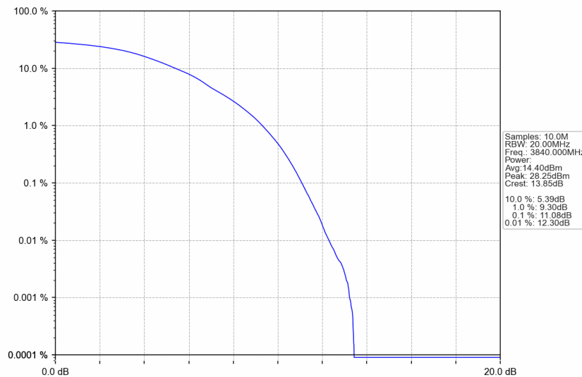
n77a_30kHz_SISO_NTNV_90MHz_DFT-s-OFDM 16 QAM_3840MHz_Outer_Full
