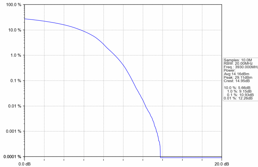
n77a_30kHz_SISO_NTNV_100MHz_DFT-s-OFDM 16 QAM_3930MHz_Outer_Full
