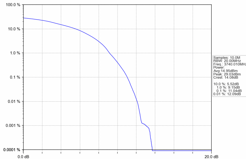
n77a_30kHz_SISO_NTNV_80MHz_DFT-s-OFDM 64 QAM_3740.01MHz_Outer_Full
