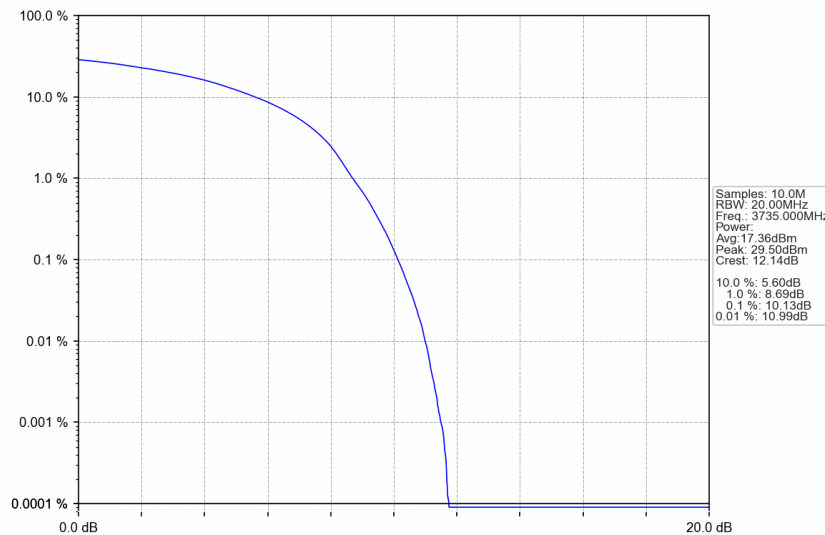
n77a_30kHz_SISO_NTNV_70MHz_DFT-s-OFDM QPSK_3735MHz_Outer_Full
