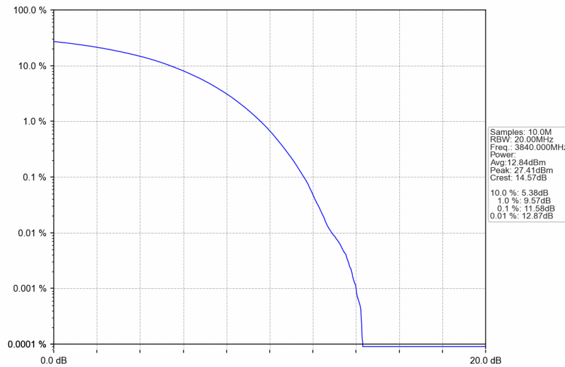
n77a_30kHz_SISO_NTNV_100MHz_CP-OFDM 64 QAM_3840MHz_Outer_Full
