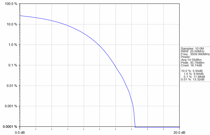
n77a_30kHz_SISO_NTNV_80MHz_CP-OFDM 16 QAM_3939.99MHz_Outer_Full
