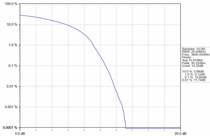
n77a_30kHz_SISO_NTNV_80MHz_DFT-s-OFDM QPSK_3840MHz_Outer_Full
