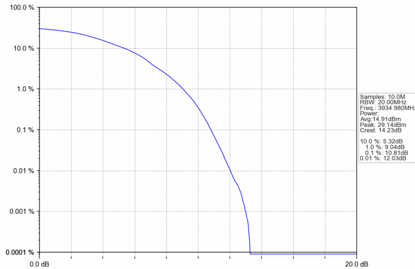
n77a_30kHz_SISO_NTNV_90MHz_DFT-s-OFDM 16 QAM_3934.98MHz_Outer_Full
