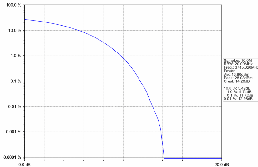
n77a_30kHz_SISO_NTNV_90MHz_CP-OFDM QPSK_3745.02MHz_Outer_Full
