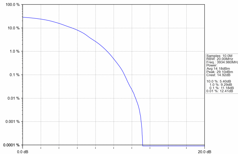
n77a_30kHz_SISO_NTNV_90MHz_DFT-s-OFDM 64 QAM_3934.98MHz_Outer_Full
