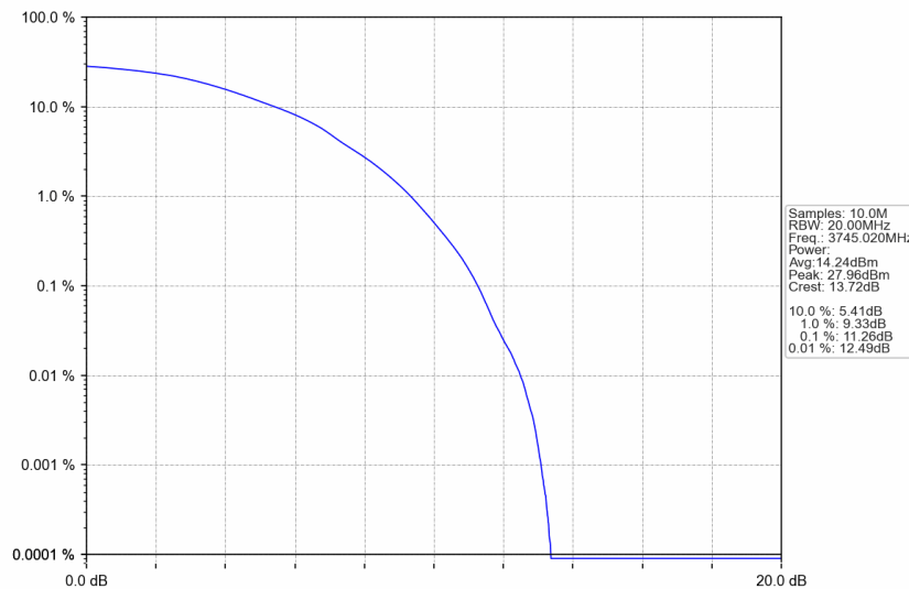
n77a_30kHz_SISO_NTNV_90MHz_DFT-s-OFDM 64 QAM_3745.02MHz_Outer_Full
