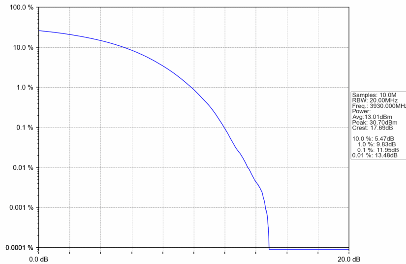
n77a_30kHz_SISO_NTNV_100MHz_CP-OFDM 16 QAM_3930MHz_Outer_Full
