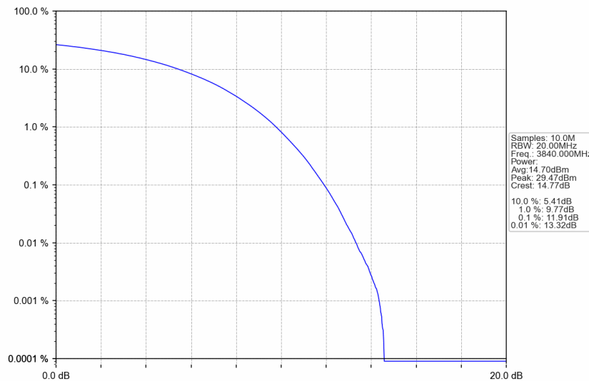
n77a_30kHz_SISO_NTNV_70MHz_CP-OFDM 16 QAM_3840MHz_Outer_Full
