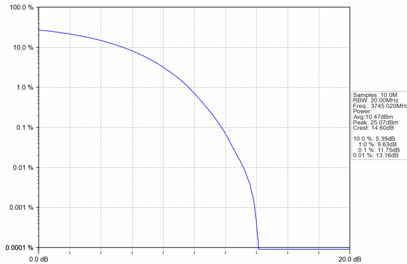
n77a_30kHz_SISO_NTNV_90MHz_CP-OFDM 256 QAM_3745.02MHz_Outer_Full
