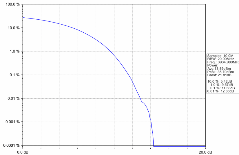
n77a_30kHz_SISO_NTNV_90MHz_CP-OFDM 16 QAM_3934.98MHz_Outer_Full
