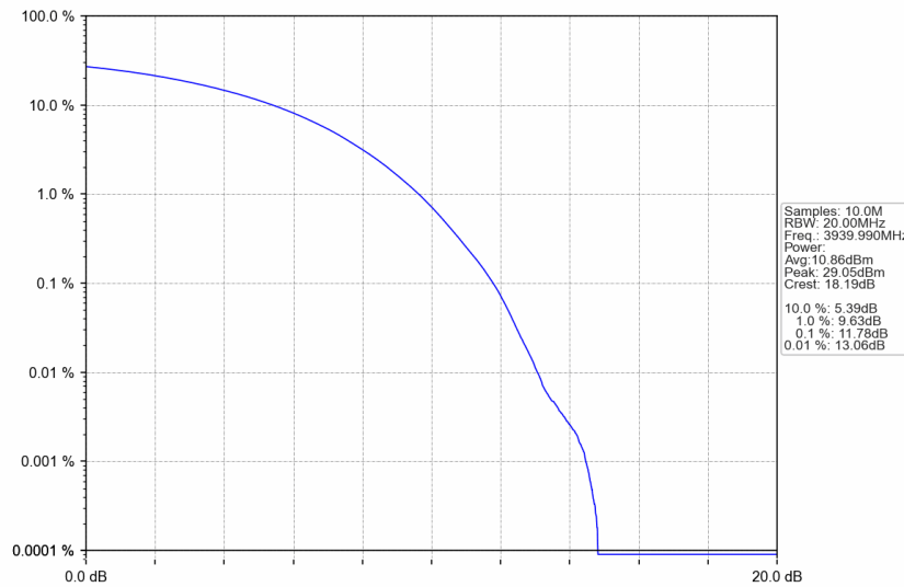
n77a_30kHz_SISO_NTNV_80MHz_CP-OFDM 256 QAM_3939.99MHz_Outer_Full
