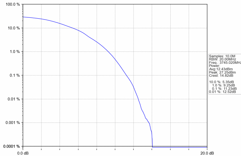
n77a_30kHz_SISO_NTNV_90MHz_DFT-s-OFDM 256 QAM_3745.02MHz_Outer_Full
