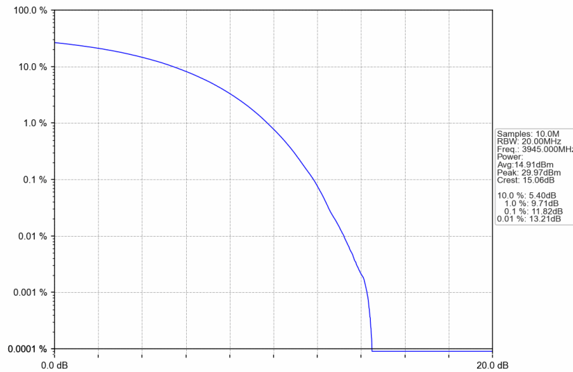
n77a_30kHz_SISO_NTNV_70MHz_CP-OFDM 16 QAM_3945MHz_Outer_Full
