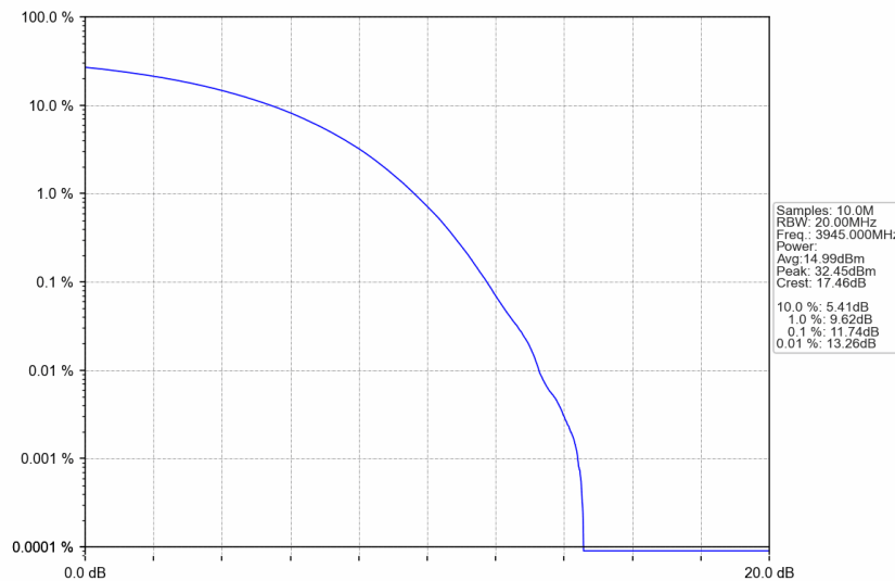
n77a_30kHz_SISO_NTNV_70MHz_CP-OFDM QPSK_3945MHz_Outer_Full
