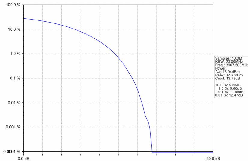
n77a_30kHz_SISO_NTNV_25MHz_CP-OFDM 64 QAM_3967.5MHz_Outer_Full
