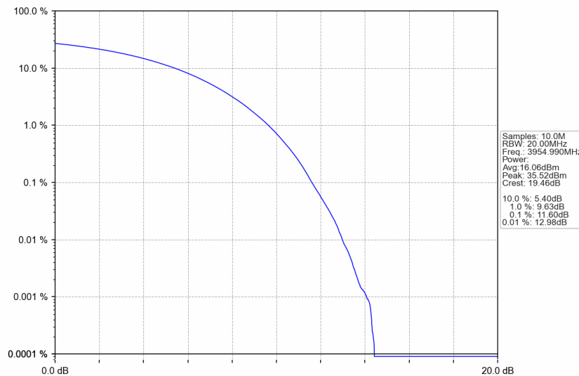
n77a_30kHz_SISO_NTNV_50MHz_CP-OFDM 64 QAM_3954.99MHz_Outer_Full
