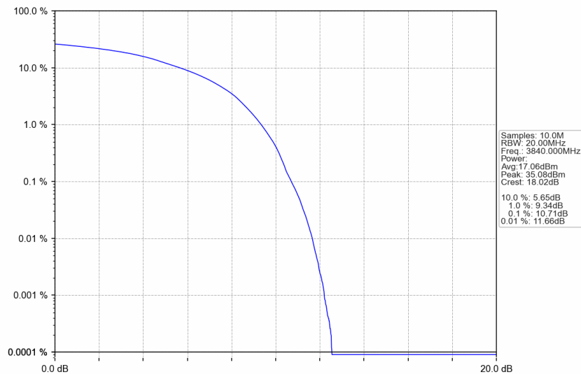
n77a_30kHz_SISO_NTNV_40MHz_DFT-s-OFDM 16 QAM_3840MHz_Outer_Full
