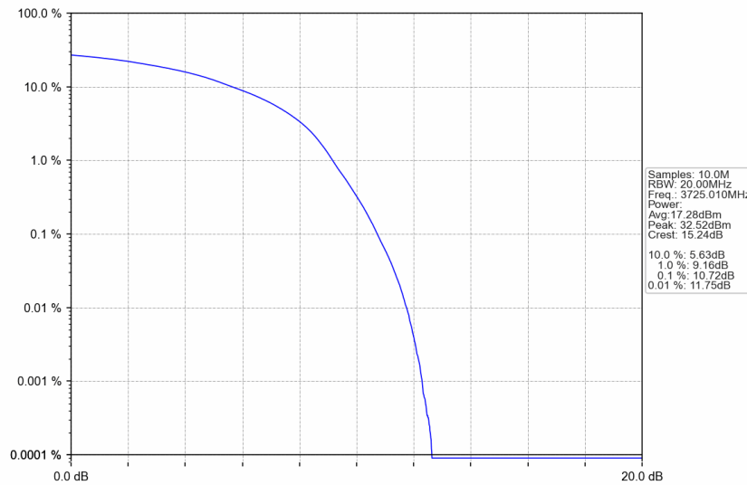
n77a_30kHz_SISO_NTNV_50MHz_DFT-s-OFDM 16 QAM_3725.01MHz_Outer_Full
