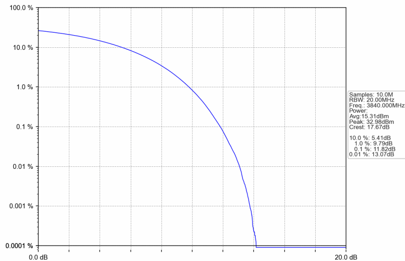
n77a_30kHz_SISO_NTNV_60MHz_CP-OFDM 16 QAM_3840MHz_Outer_Full
