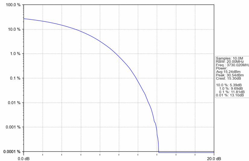
n77a_30kHz_SISO_NTNV_60MHz_CP-OFDM 64 QAM_3730.02MHz_Outer_Full
