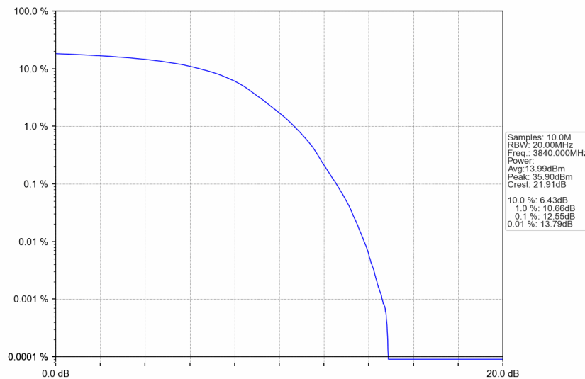
n77a_30kHz_SISO_NTNV_25MHz_DFT-s-OFDM 256 QAM_3840MHz_Outer_Full
