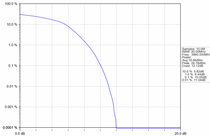
n77a_30kHz_SISO_NTNV_40MHz_DFT-s-OFDM 256 QAM_3960MHz_Outer_Full
