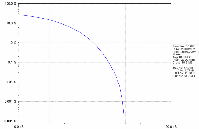
n77a_30kHz_SISO_NTNV_25MHz_CP-OFDM QPSK_3840MHz_Outer_Full
