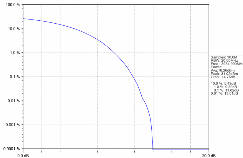
n77a_30kHz_SISO_NTNV_50MHz_CP-OFDM QPSK_3954.99MHz_Outer_Full
