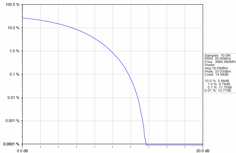
n77a_30kHz_SISO_NTNV_30MHz_CP-OFDM 64 QAM_3964.98MHz_Outer_Full
