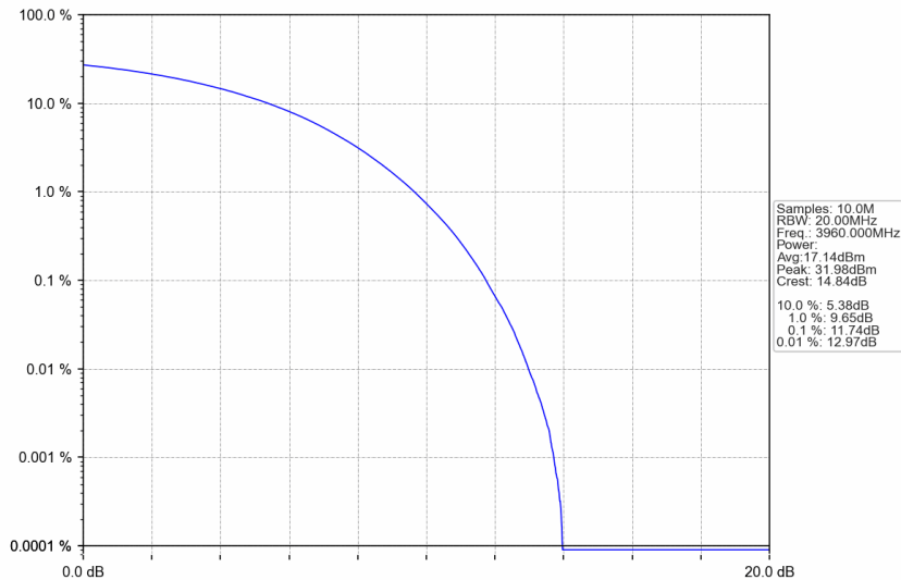
n77a_30kHz_SISO_NTNV_40MHz_CP-OFDM 64 QAM_3960MHz_Outer_Full
