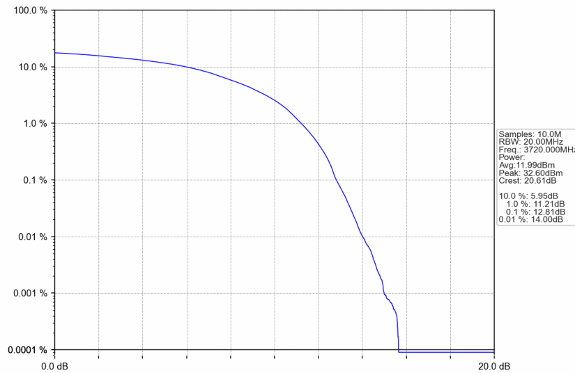
n77a_30kHz_SISO_NTNV_40MHz_DFT-s-OFDM 256 QAM_3720MHz_Outer_Full
