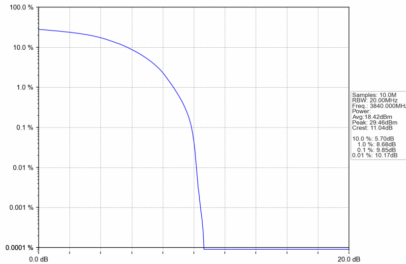
n77a_30kHz_SISO_NTNV_40MHz_DFT-s-OFDM QPSK_3840MHz_Outer_Full
