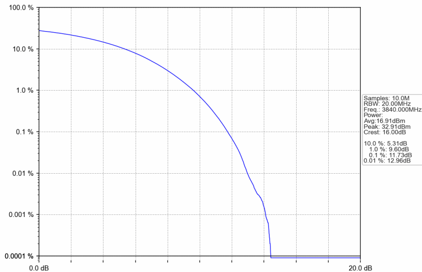
n77a_30kHz_SISO_NTNV_40MHz_CP-OFDM 64 QAM_3840MHz_Outer_Full
