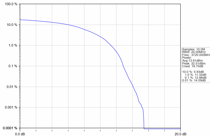
n77a_30kHz_SISO_NTNV_40MHz_DFT-s-OFDM 64 QAM_3720MHz_Outer_Full
