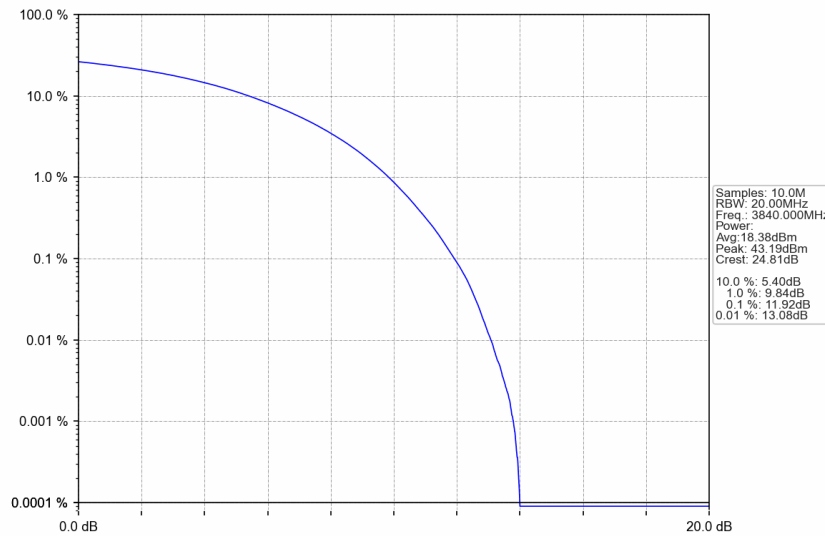
n77a_30kHz_SISO_NTNV_25MHz_CP-OFDM 64 QAM_3840MHz_Outer_Full
