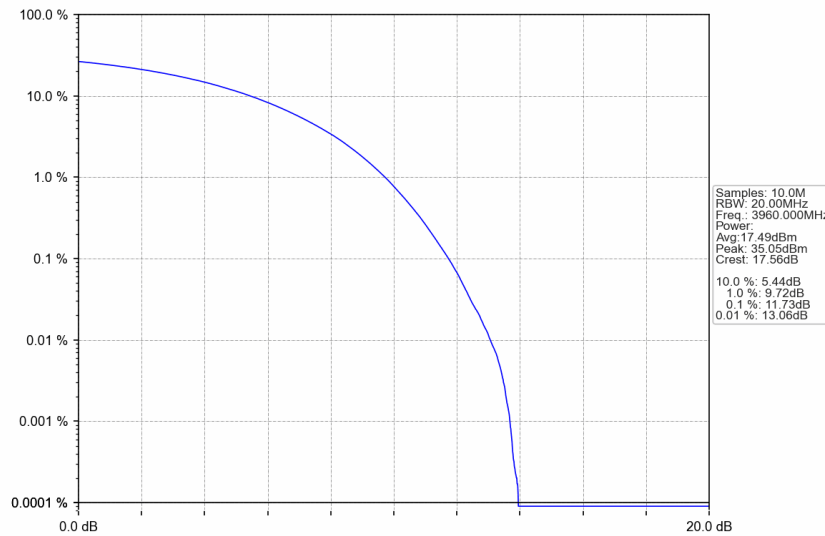
n77a_30kHz_SISO_NTNV_40MHz_CP-OFDM 16 QAM_3960MHz_Outer_Full
