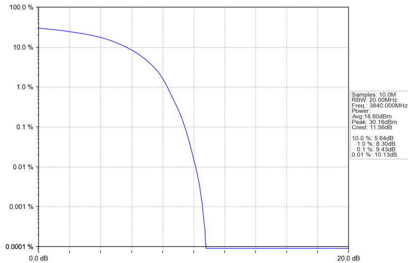
n77a_30kHz_SISO_NTNV_50MHz_DFT-s-OFDM QPSK_3840MHz_Outer_Full
