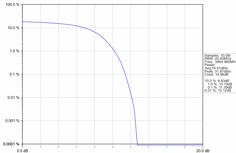
n77a_30kHz_SISO_NTNV_30MHz_DFT-s-OFDM QPSK_3964.98MHz_Outer_Full
