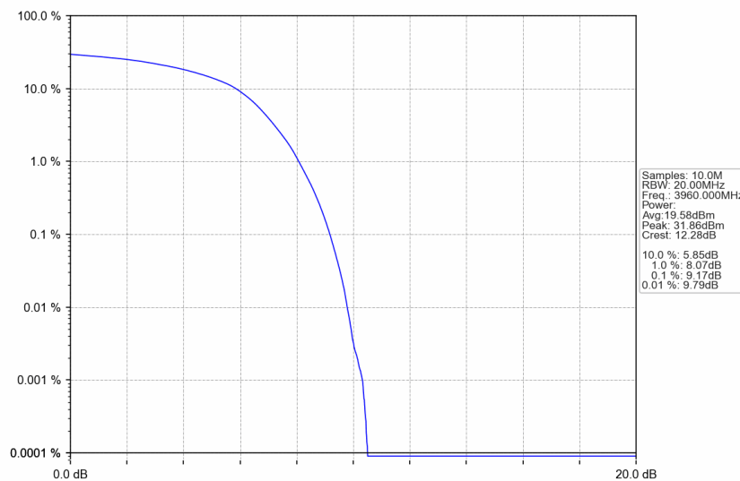
n77a_30kHz_SISO_NTNV_40MHz_DFT-s-OFDM QPSK_3960MHz_Outer_Full
