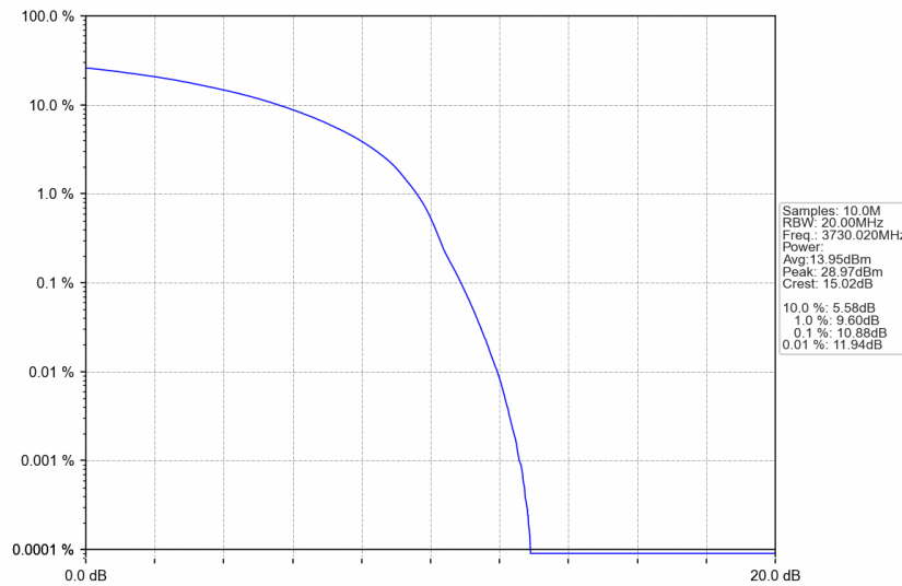
n77a_30kHz_SISO_NTNV_60MHz_DFT-s-OFDM 256 QAM_3730.02MHz_Outer_Full
