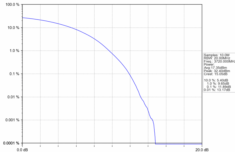
n77a_30kHz_SISO_NTNV_40MHz_CP-OFDM QPSK_3720MHz_Outer_Full
