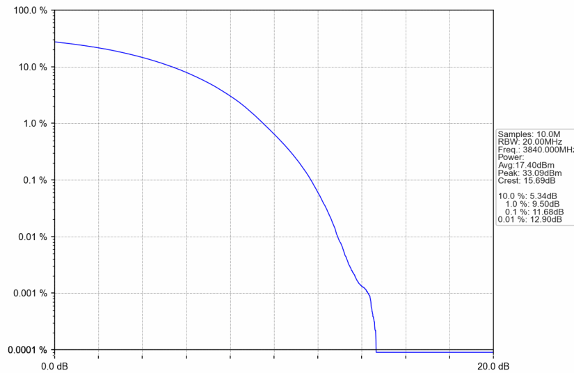
n77a_30kHz_SISO_NTNV_40MHz_CP-OFDM QPSK_3840MHz_Outer_Full
