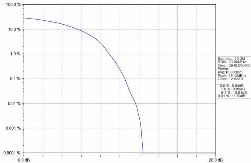
n77a_30kHz_SISO_NTNV_50MHz_DFT-s-OFDM 64 QAM_3840MHz_Outer_Full
