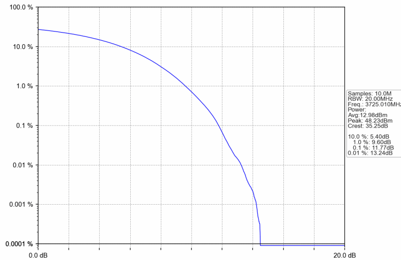
n77a_30kHz_SISO_NTNV_50MHz_CP-OFDM 256 QAM_3725.01MHz_Outer_Full
