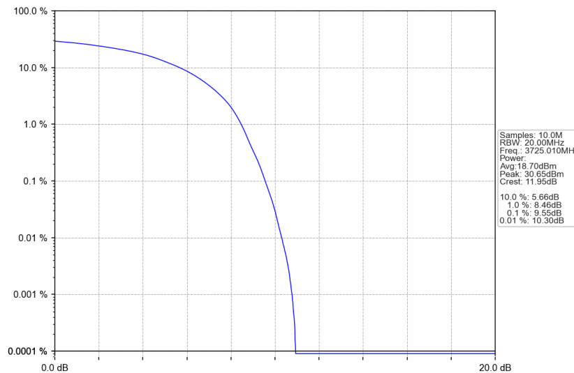
n77a_30kHz_SISO_NTNV_50MHz_DFT-s-OFDM QPSK_3725.01MHz_Outer_Full
