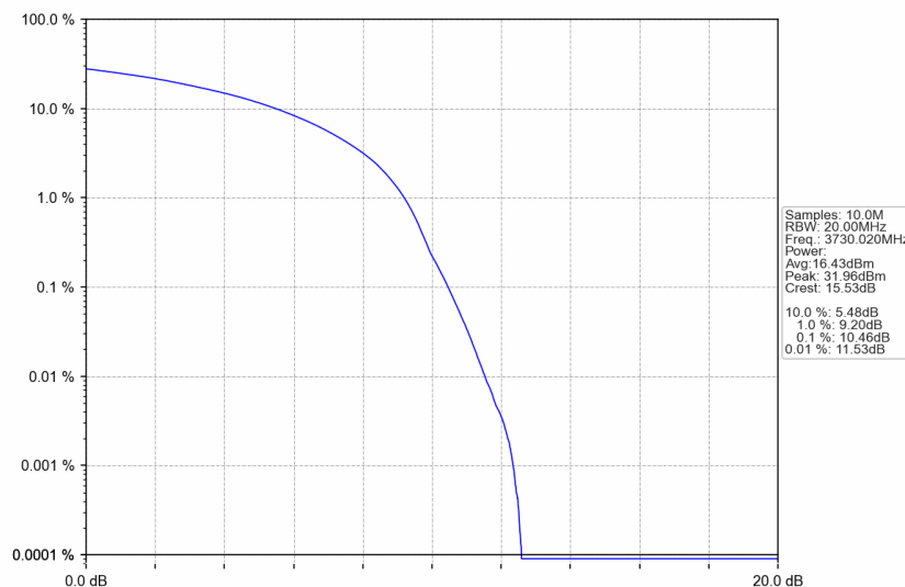
n77a_30kHz_SISO_NTNV_60MHz_DFT-s-OFDM 64 QAM_3730.02MHz_Outer_Full
