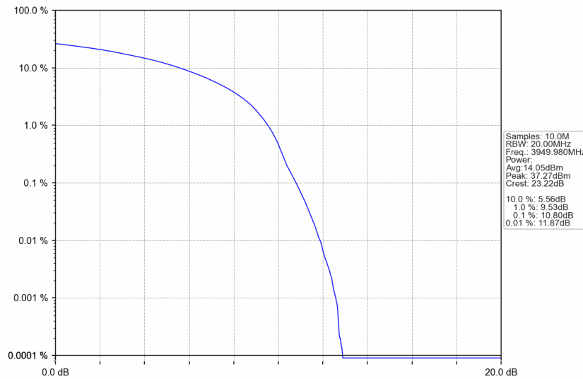
n77a_30kHz_SISO_NTNV_60MHz_DFT-s-OFDM 256 QAM_3949.98MHz_Outer_Full
