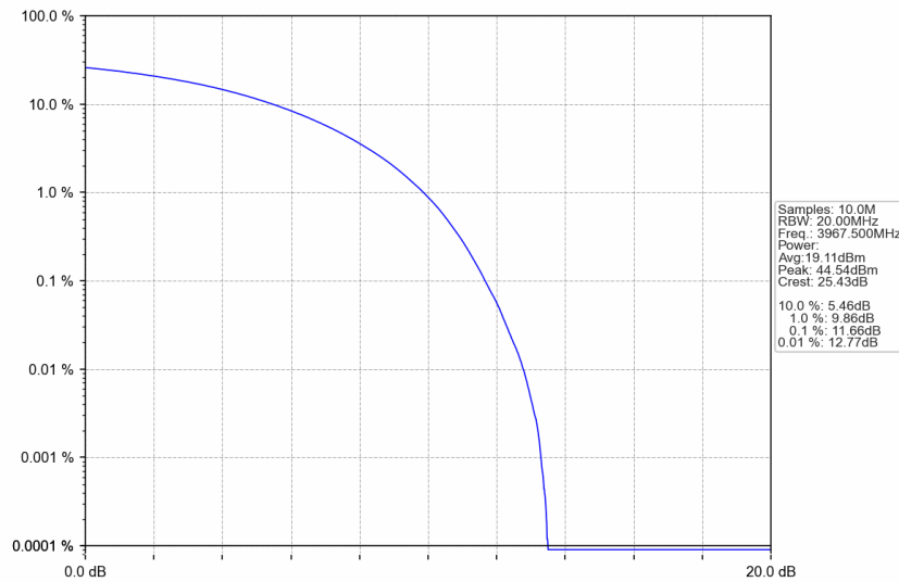
n77a_30kHz_SISO_NTNV_25MHz_CP-OFDM 16 QAM_3967.5MHz_Outer_Full
