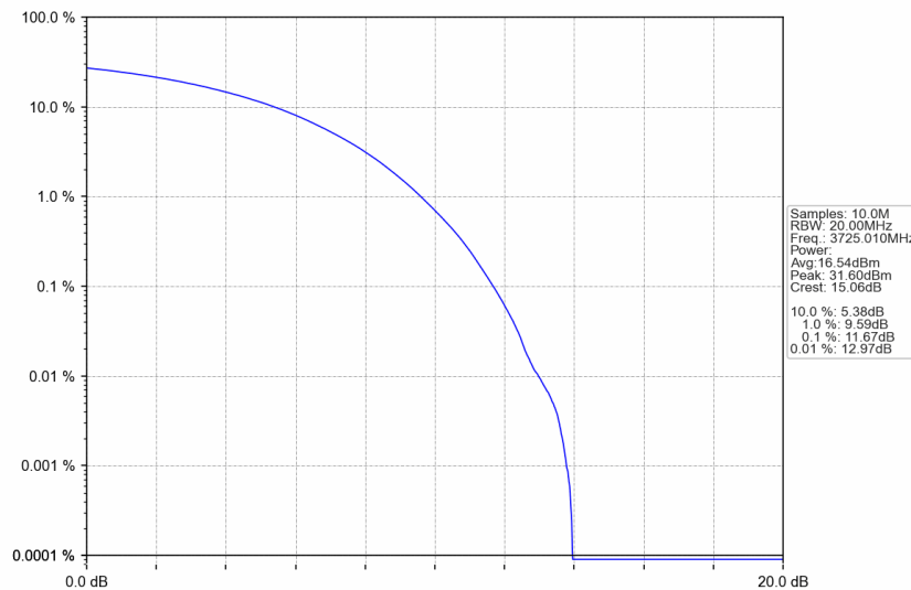
n77a_30kHz_SISO_NTNV_50MHz_CP-OFDM QPSK_3725.01MHz_Outer_Full
