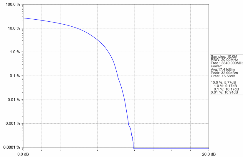
n77a_30kHz_SISO_NTNV_60MHz_DFT-s-OFDM QPSK_3840MHz_Outer_Full
