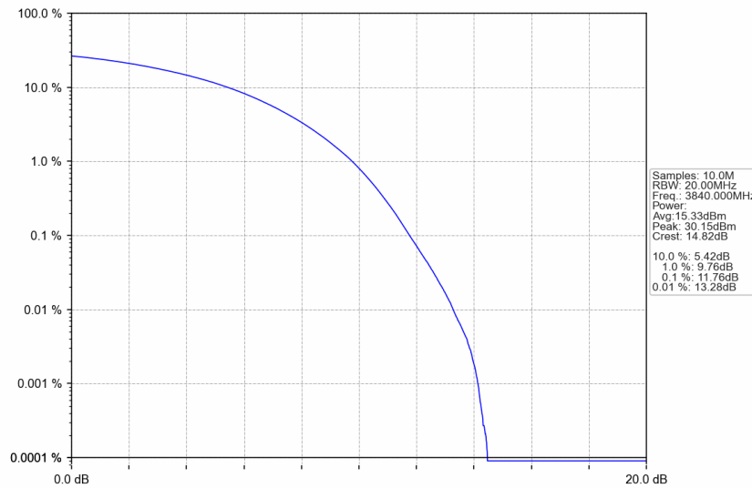
n77a_30kHz_SISO_NTNV_60MHz_CP-OFDM QPSK_3840MHz_Outer_Full
