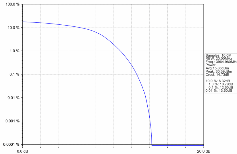
n77a_30kHz_SISO_NTNV_30MHz_DFT-s-OFDM 16 QAM_3964.98MHz_Outer_Full
