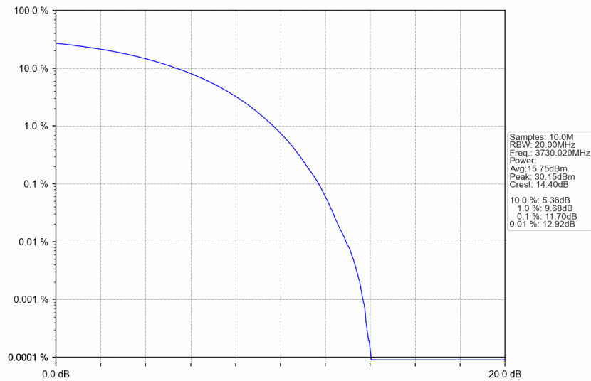
n77a_30kHz_SISO_NTNV_60MHz_CP-OFDM 16 QAM_3730.02MHz_Outer_Full
