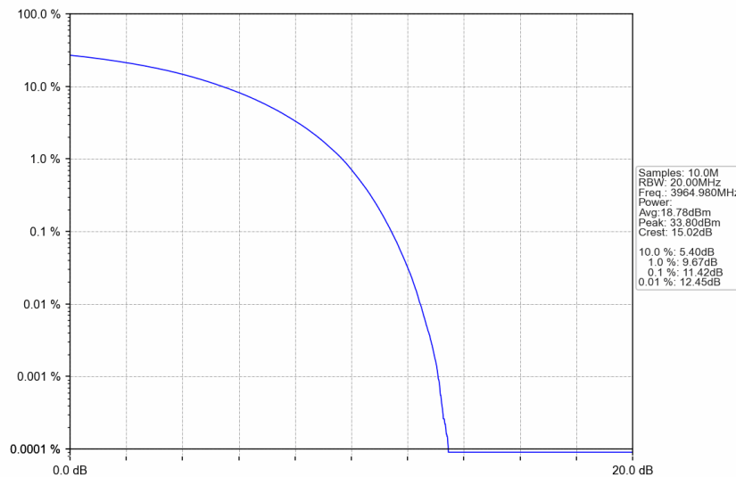
n77a_30kHz_SISO_NTNV_30MHz_CP-OFDM QPSK_3964.98MHz_Outer_Full
