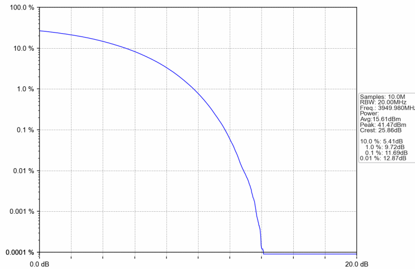
n77a_30kHz_SISO_NTNV_60MHz_CP-OFDM 16 QAM_3949.98MHz_Outer_Full
