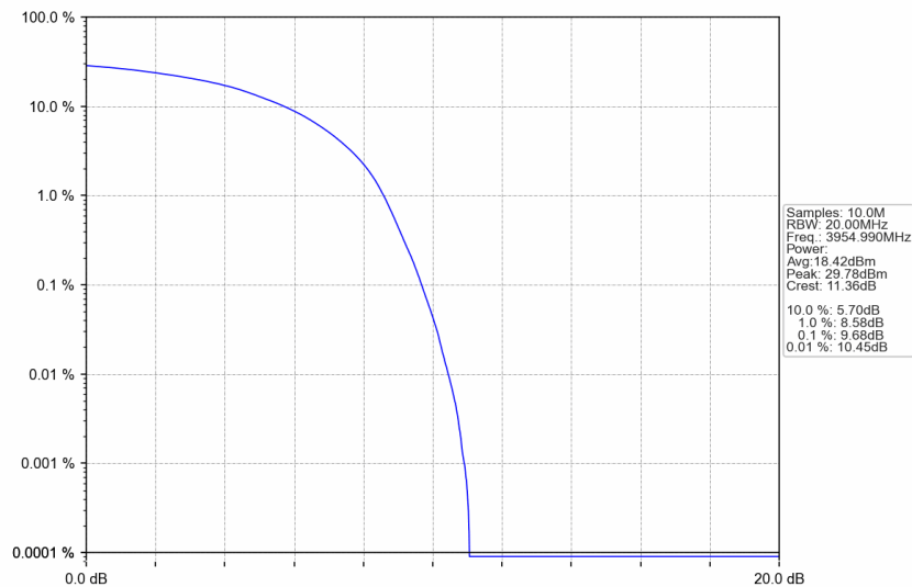
n77a_30kHz_SISO_NTNV_50MHz_DFT-s-OFDM QPSK_3954.99MHz_Outer_Full
