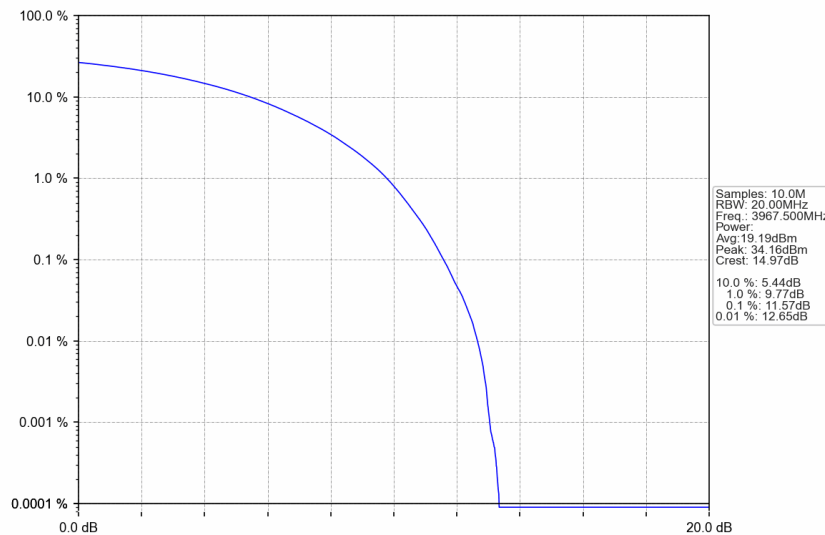
n77a_30kHz_SISO_NTNV_25MHz_CP-OFDM QPSK_3967.5MHz_Outer_Full
