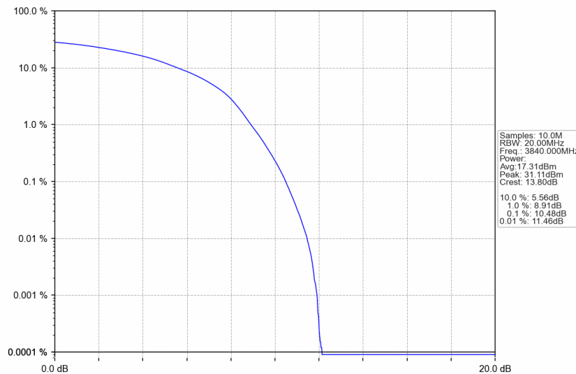
n77a_30kHz_SISO_NTNV_50MHz_DFT-s-OFDM 16 QAM_3840MHz_Outer_Full
