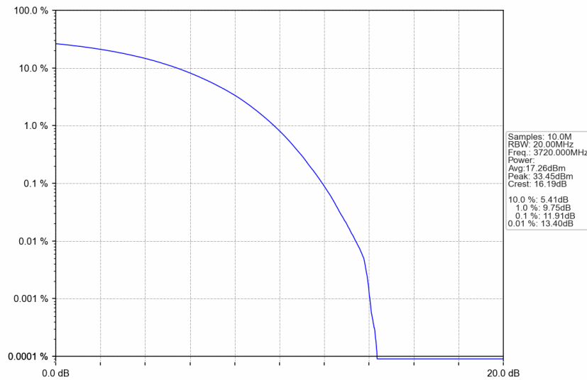
n77a_30kHz_SISO_NTNV_40MHz_CP-OFDM 16 QAM_3720MHz_Outer_Full
