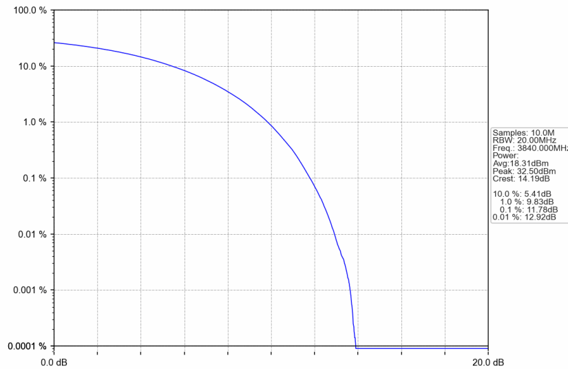
n77a_30kHz_SISO_NTNV_30MHz_CP-OFDM QPSK_3840MHz_Outer_Full
