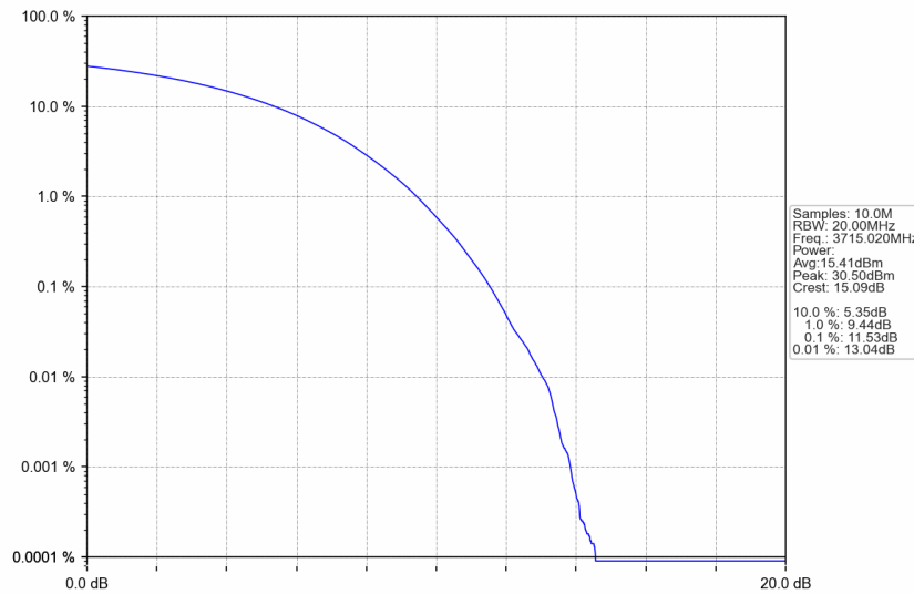
n77a_30kHz_SISO_NTNV_30MHz_CP-OFDM 256 QAM_3715.02MHz_Outer_Full
