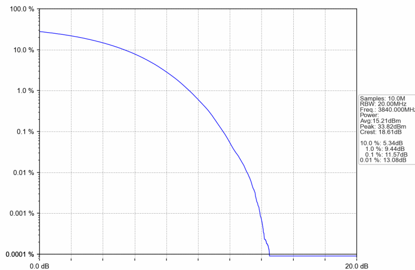
n77a_30kHz_SISO_NTNV_30MHz_CP-OFDM 256 QAM_3840MHz_Outer_Full
