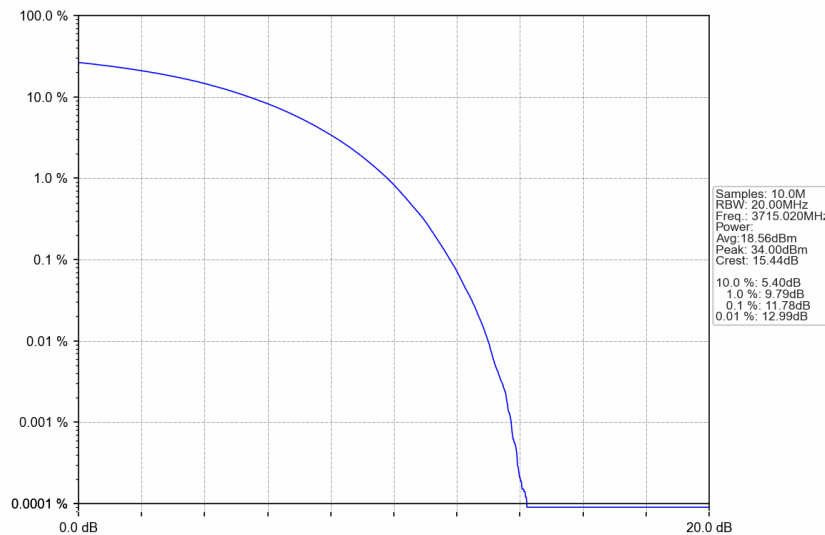
n77a_30kHz_SISO_NTNV_30MHz_CP-OFDM QPSK_3715.02MHz_Outer_Full
