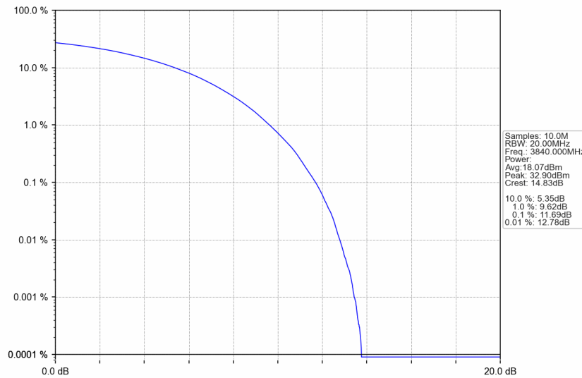
n77a_30kHz_SISO_NTNV_30MHz_CP-OFDM 64 QAM_3840MHz_Outer_Full
