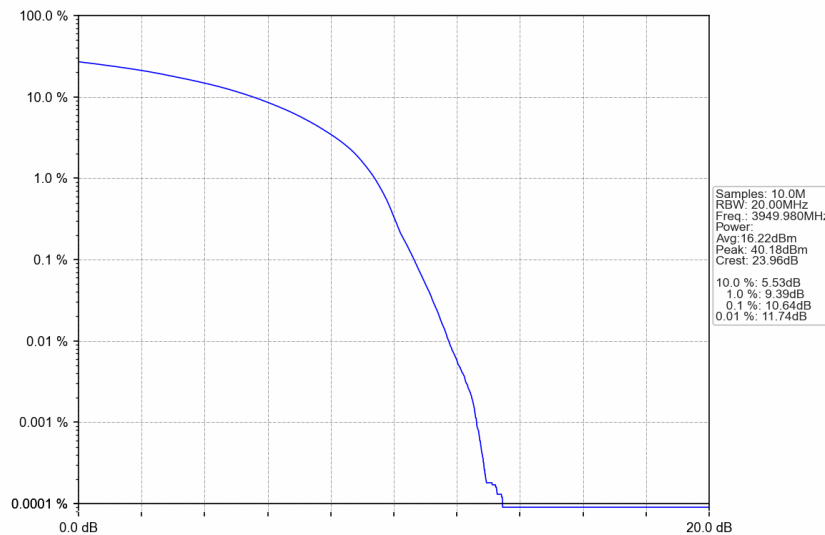
n77a_30kHz_SISO_NTNV_60MHz_DFT-s-OFDM 64 QAM_3949.98MHz_Outer_Full
