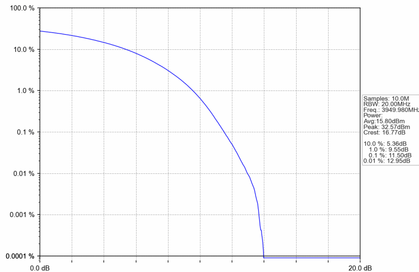
n77a_30kHz_SISO_NTNV_60MHz_CP-OFDM QPSK_3949.98MHz_Outer_Full
