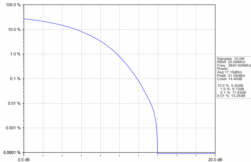
n77a_30kHz_SISO_NTNV_40MHz_CP-OFDM 16 QAM_3840MHz_Outer_Full
