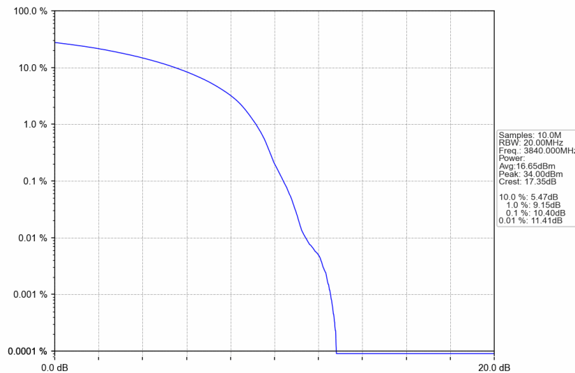
n77a_30kHz_SISO_NTNV_60MHz_DFT-s-OFDM 16 QAM_3840MHz_Outer_Full
