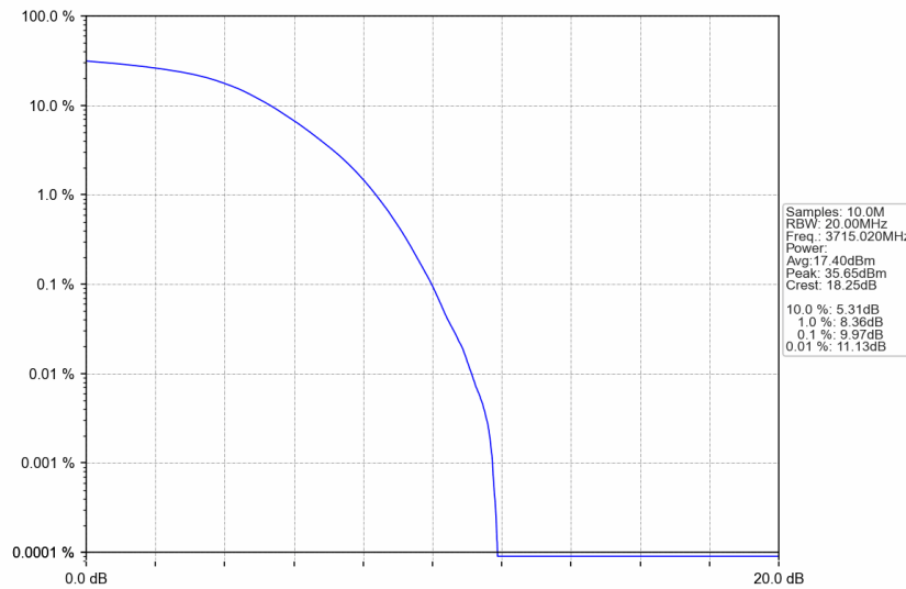
n77a_30kHz_SISO_NTNV_30MHz_DFT-s-OFDM 256 QAM_3715.02MHz_Outer_Full
