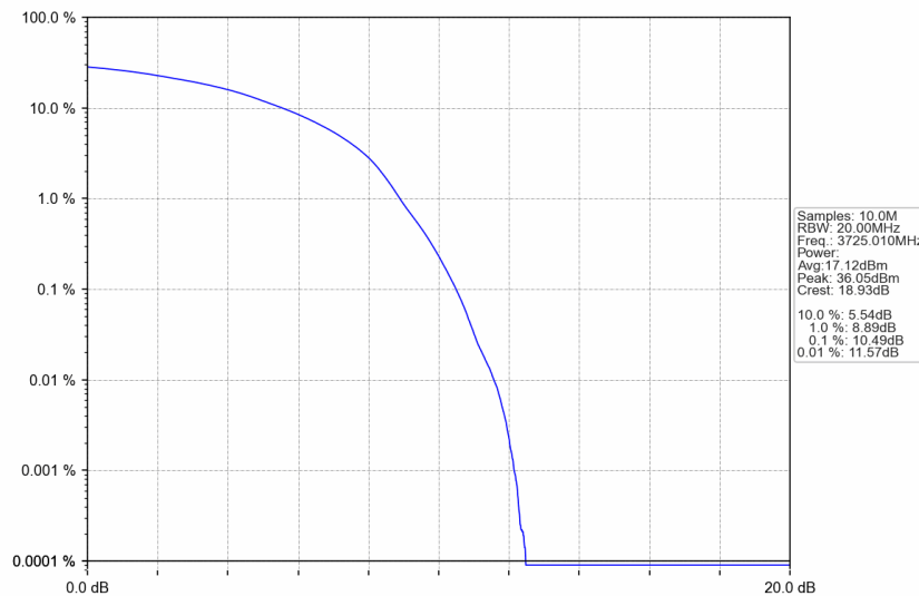
n77a_30kHz_SISO_NTNV_50MHz_DFT-s-OFDM 64 QAM_3725.01MHz_Outer_Full
