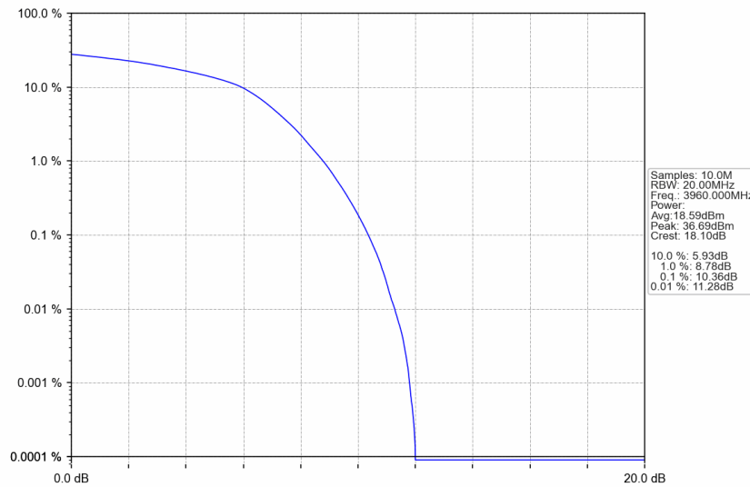
n77a_30kHz_SISO_NTNV_40MHz_DFT-s-OFDM 16 QAM_3960MHz_Outer_Full
