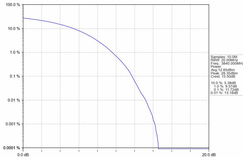
n77a_30kHz_SISO_NTNV_50MHz_CP-OFDM 256 QAM_3840MHz_Outer_Full
