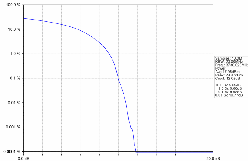
n77a_30kHz_SISO_NTNV_60MHz_DFT-s-OFDM QPSK_3730.02MHz_Outer_Full
