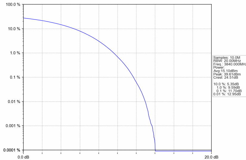
n77a_30kHz_SISO_NTNV_60MHz_CP-OFDM 64 QAM_3840MHz_Outer_Full
