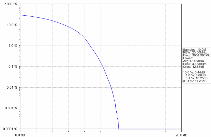
n77a_30kHz_SISO_NTNV_50MHz_DFT-s-OFDM 64 QAM_3954.99MHz_Outer_Full
