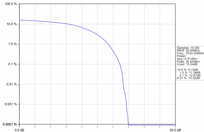
n77a_30kHz_SISO_NTNV_40MHz_DFT-s-OFDM QPSK_3720MHz_Outer_Full
