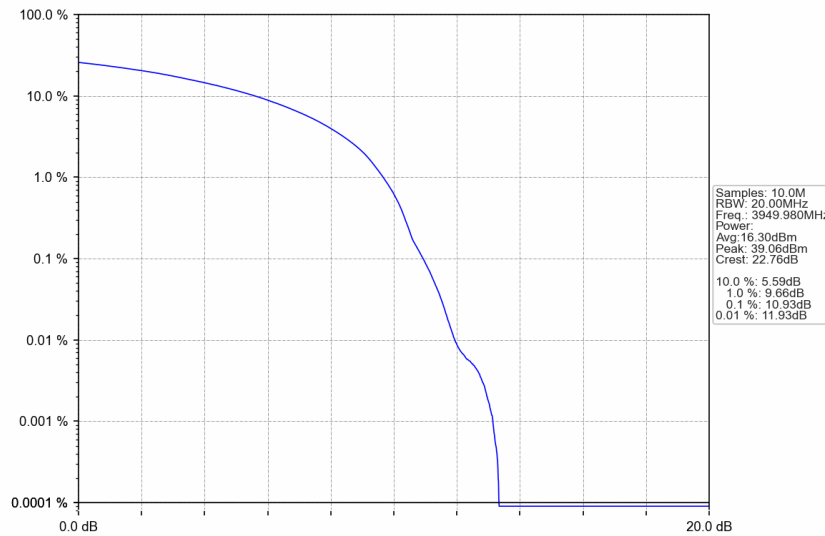
n77a_30kHz_SISO_NTNV_60MHz_DFT-s-OFDM 16 QAM_3949.98MHz_Outer_Full
