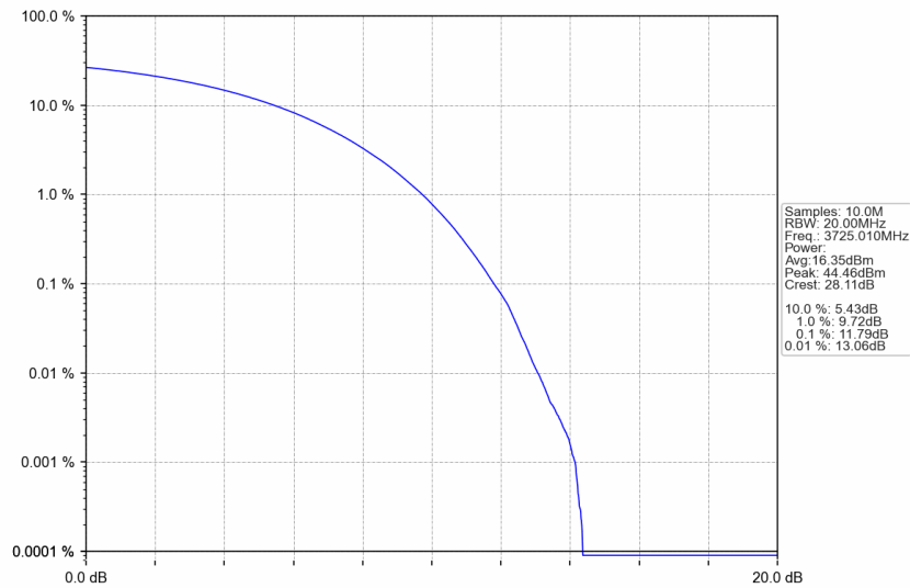
n77a_30kHz_SISO_NTNV_50MHz_CP-OFDM 16 QAM_3725.01MHz_Outer_Full
