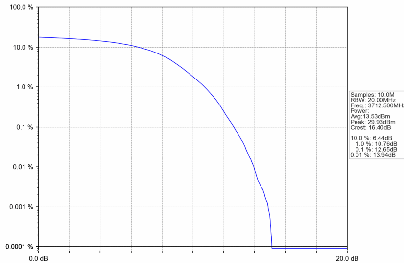
n77a_30kHz_SISO_NTNV_25MHz_DFT-s-OFDM 256 QAM_3712.5MHz_Outer_Full
