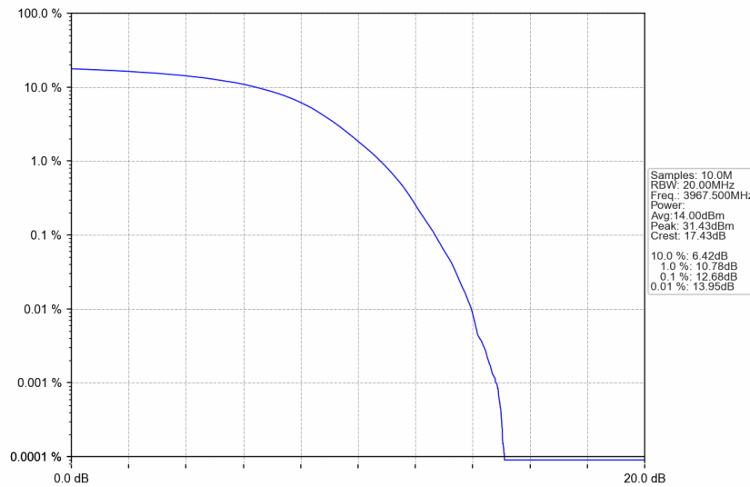
n77a_30kHz_SISO_NTNV_25MHz_DFT-s-OFDM 256 QAM_3967.5MHz_Outer_Full
