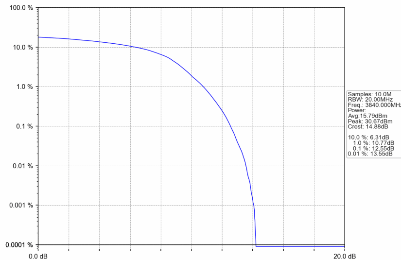
n77a_30kHz_SISO_NTNV_30MHz_DFT-s-OFDM 16 QAM_3840MHz_Outer_Full
