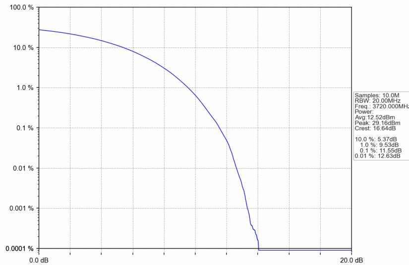
n77a_30kHz_SISO_NTNV_40MHz_CP-OFDM 256 QAM_3720MHz_Outer_Full
