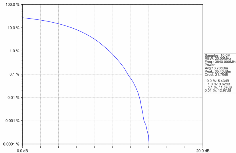
n77a_30kHz_SISO_NTNV_40MHz_CP-OFDM 256 QAM_3840MHz_Outer_Full
