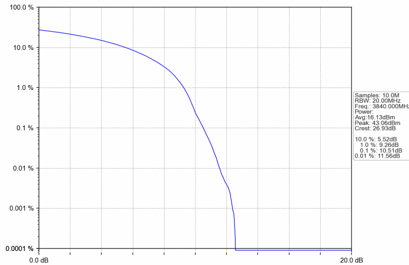
n77a_30kHz_SISO_NTNV_60MHz_DFT-s-OFDM 64 QAM_3840MHz_Outer_Full
