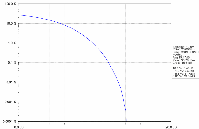
n77a_30kHz_SISO_NTNV_60MHz_CP-OFDM 64 QAM_3949.98MHz_Outer_Full
