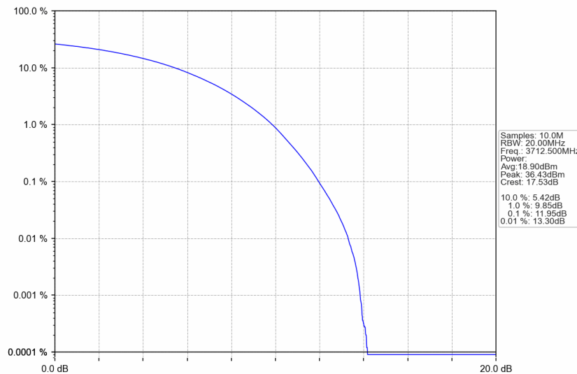
n77a_30kHz_SISO_NTNV_25MHz_CP-OFDM QPSK_3712.5MHz_Outer_Full
