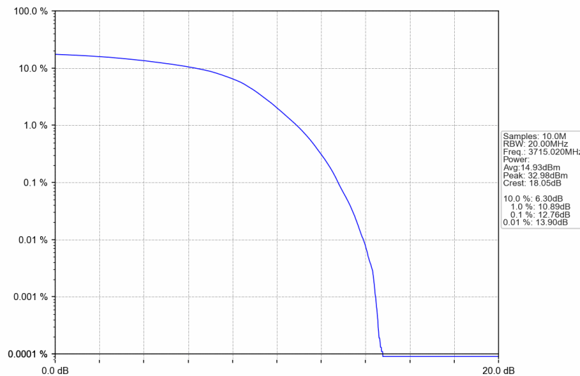
n77a_30kHz_SISO_NTNV_30MHz_DFT-s-OFDM 64 QAM_3715.02MHz_Outer_Full
