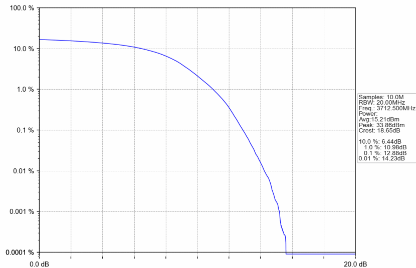
n77a_30kHz_SISO_NTNV_25MHz_DFT-s-OFDM 64 QAM_3712.5MHz_Outer_Full
