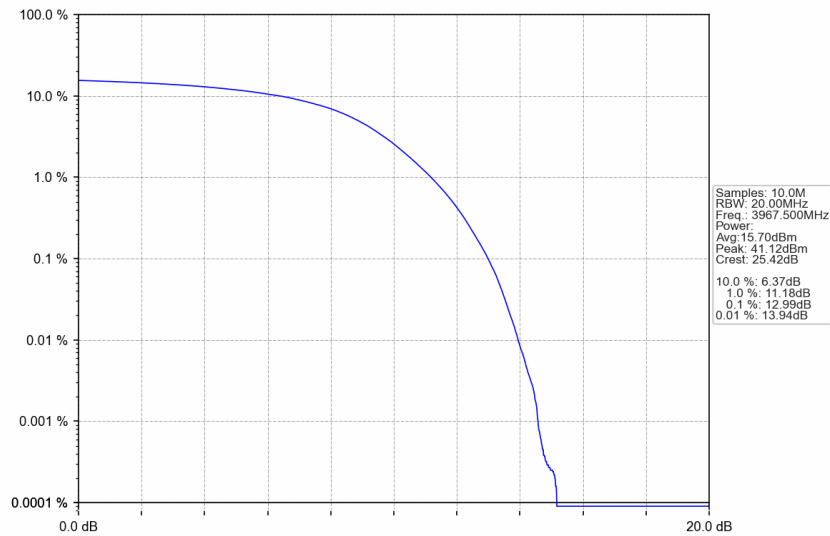
n77a_30kHz_SISO_NTNV_25MHz_DFT-s-OFDM 16 QAM_3967.5MHz_Outer_Full
