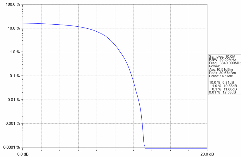
n77a_30kHz_SISO_NTNV_30MHz_DFT-s-OFDM QPSK_3840MHz_Outer_Full
