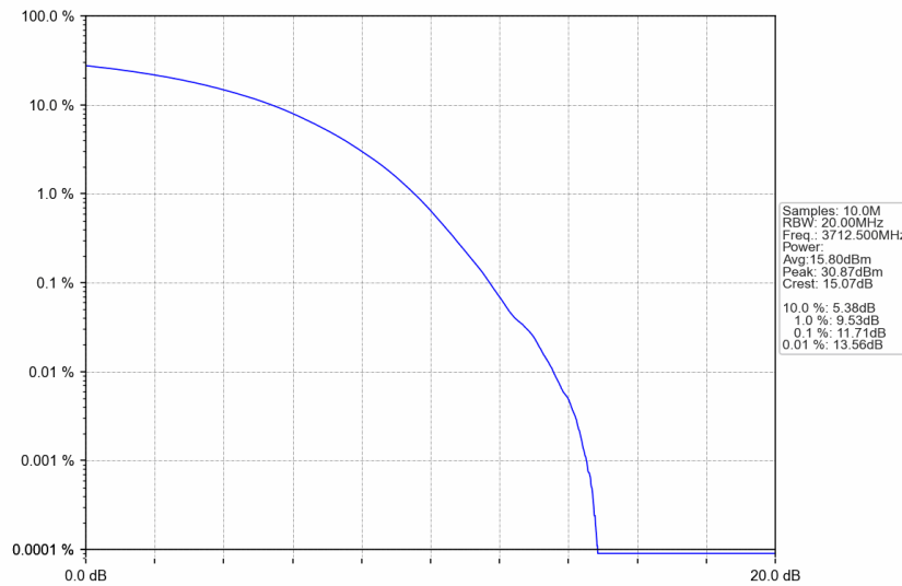
n77a_30kHz_SISO_NTNV_25MHz_CP-OFDM 256 QAM_3712.5MHz_Outer_Full
