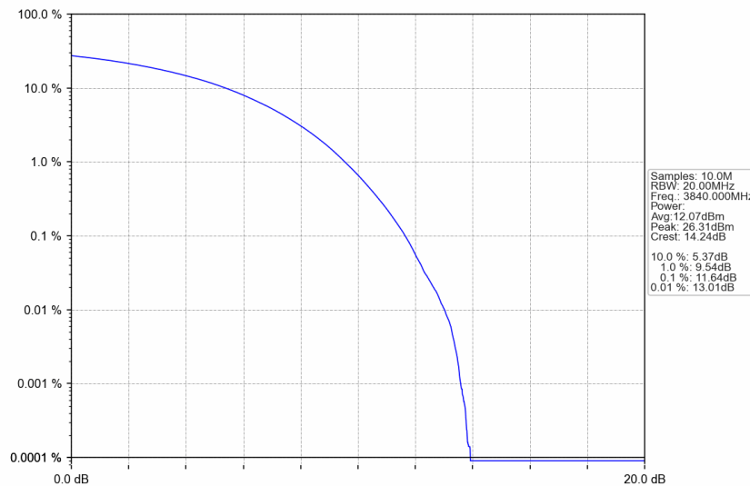
n77a_30kHz_SISO_NTNV_60MHz_CP-OFDM 256 QAM_3840MHz_Outer_Full
