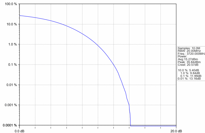
n77a_30kHz_SISO_NTNV_40MHz_CP-OFDM 64 QAM_3720MHz_Outer_Full
