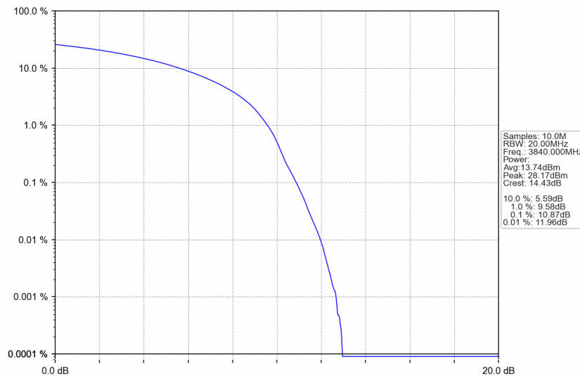
n77a_30kHz_SISO_NTNV_60MHz_DFT-s-OFDM 256 QAM_3840MHz_Outer_Full
