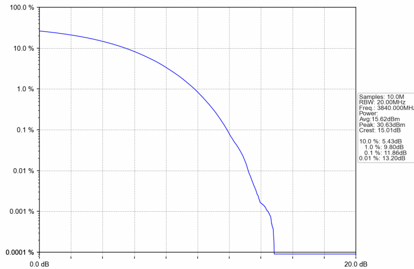
n77a_30kHz_SISO_NTNV_50MHz_CP-OFDM 64 QAM_3840MHz_Outer_Full
