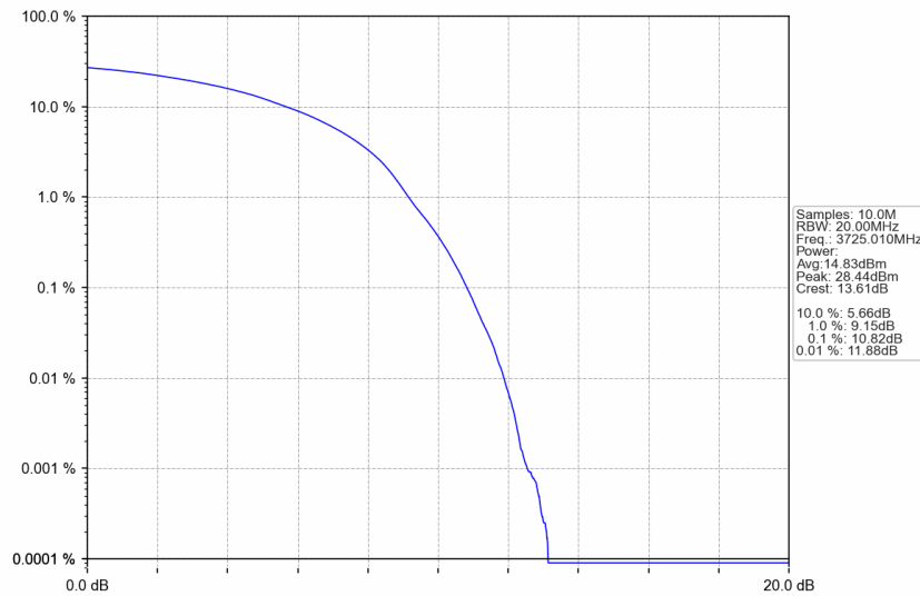
n77a_30kHz_SISO_NTNV_50MHz_DFT-s-OFDM 256 QAM_3725.01MHz_Outer_Full
