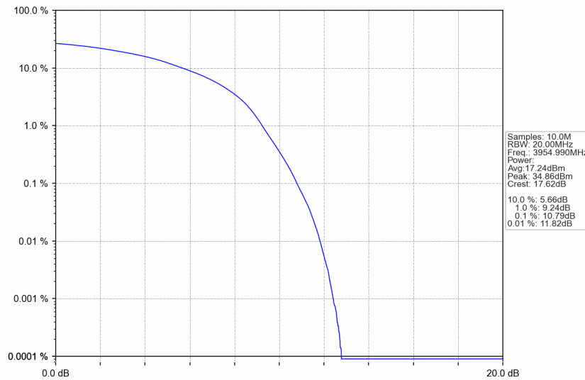
n77a_30kHz_SISO_NTNV_50MHz_DFT-s-OFDM 16 QAM_3954.99MHz_Outer_Full
