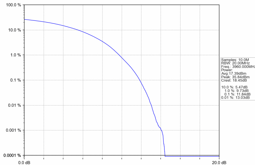
n77a_30kHz_SISO_NTNV_40MHz_CP-OFDM QPSK_3960MHz_Outer_Full
