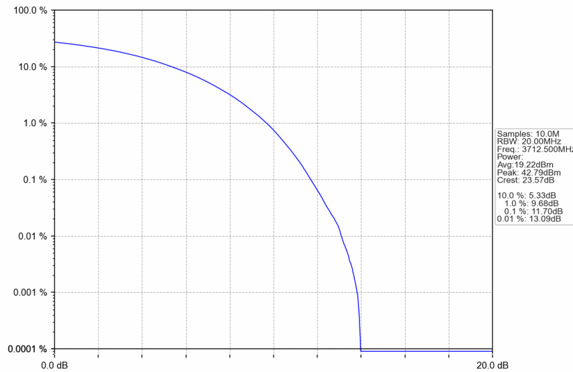
n77a_30kHz_SISO_NTNV_25MHz_CP-OFDM 16 QAM_3712.5MHz_Outer_Full
