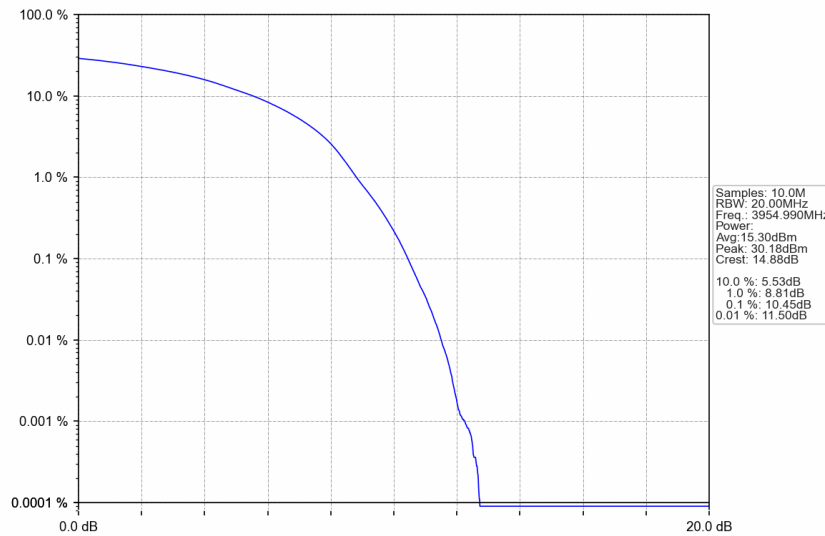
n77a_30kHz_SISO_NTNV_50MHz_DFT-s-OFDM 256 QAM_3954.99MHz_Outer_Full
