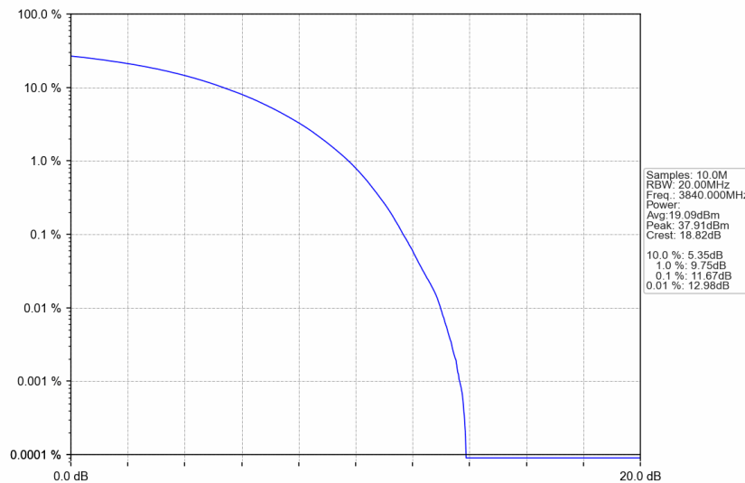
n77a_30kHz_SISO_NTNV_25MHz_CP-OFDM 16 QAM_3840MHz_Outer_Full
