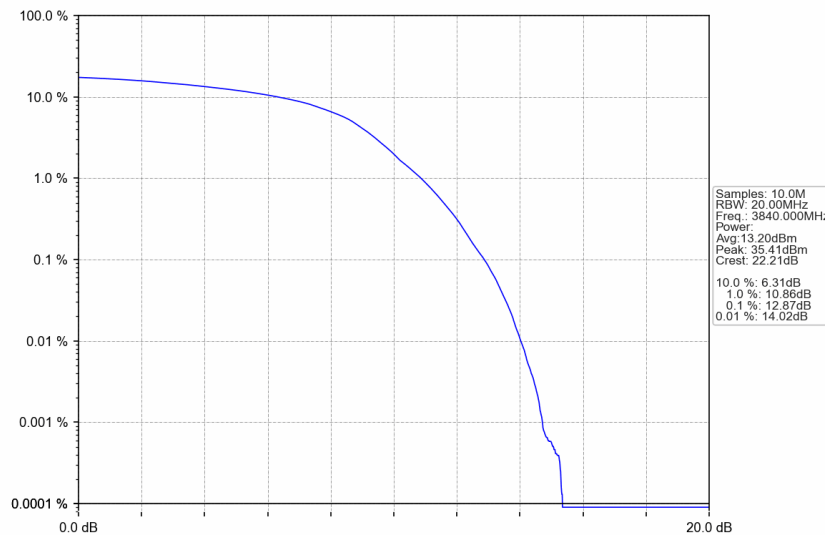
n77a_30kHz_SISO_NTNV_30MHz_DFT-s-OFDM 256 QAM_3840MHz_Outer_Full
