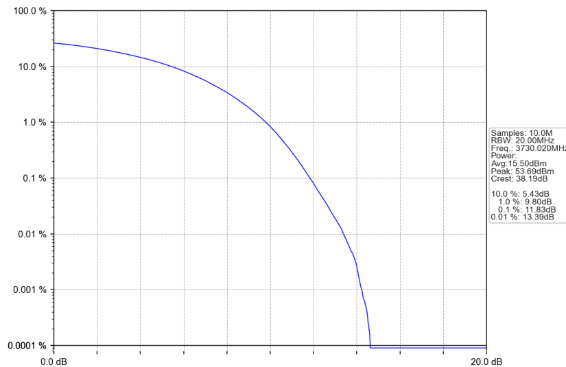
n77a_30kHz_SISO_NTNV_60MHz_CP-OFDM QPSK_3730.02MHz_Outer_Full
