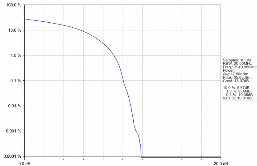
n77a_30kHz_SISO_NTNV_60MHz_DFT-s-OFDM QPSK_3949.98MHz_Outer_Full
