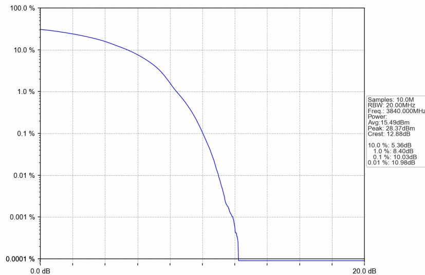
n77a_30kHz_SISO_NTNV_50MHz_DFT-s-OFDM 256 QAM_3840MHz_Outer_Full
