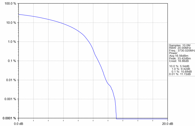
n77a_30kHz_SISO_NTNV_60MHz_DFT-s-OFDM 16 QAM_3730.02MHz_Outer_Full
