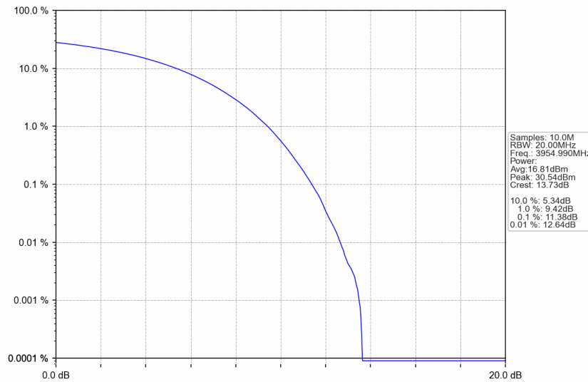
n77a_30kHz_SISO_NTNV_50MHz_CP-OFDM 16 QAM_3954.99MHz_Outer_Full
