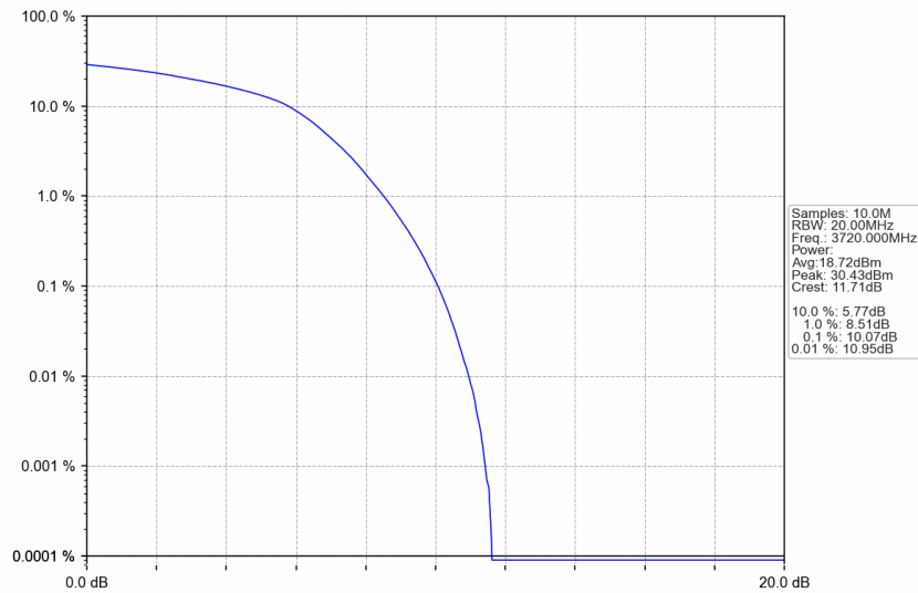
n77a_30kHz_SISO_NTNV_40MHz_DFT-s-OFDM 16 QAM_3720MHz_Outer_Full
