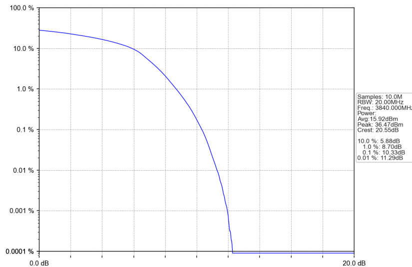
n77a_30kHz_SISO_NTNV_40MHz_DFT-s-OFDM 256 QAM_3840MHz_Outer_Full
