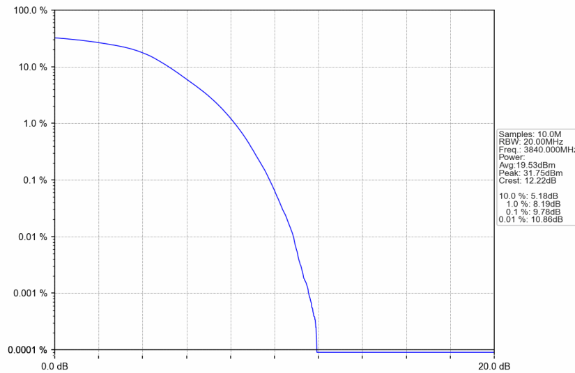
n77a_30kHz_SISO_NTNV_30MHz_DFT-s-OFDM 64 QAM_3840MHz_Outer_Full
