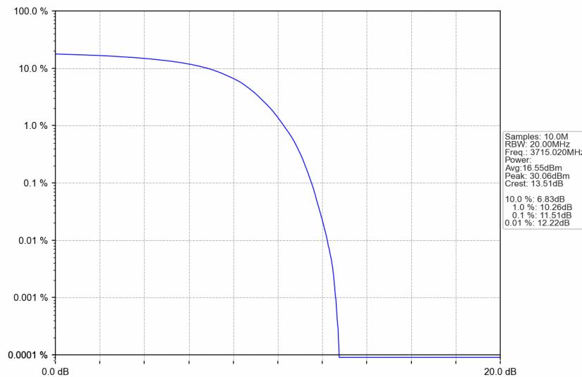
n77a_30kHz_SISO_NTNV_30MHz_DFT-s-OFDM QPSK_3715.02MHz_Outer_Full
