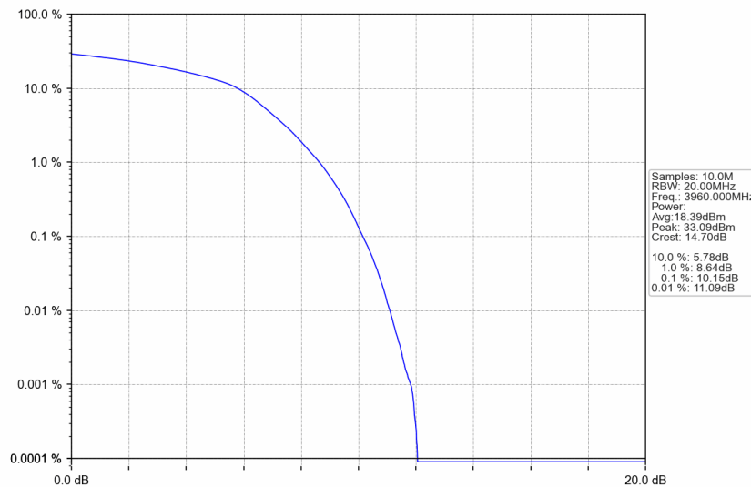
n77a_30kHz_SISO_NTNV_40MHz_DFT-s-OFDM 64 QAM_3960MHz_Outer_Full
