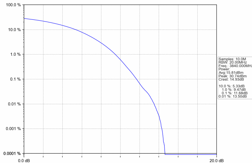
n77a_30kHz_SISO_NTNV_25MHz_CP-OFDM 256 QAM_3840MHz_Outer_Full
