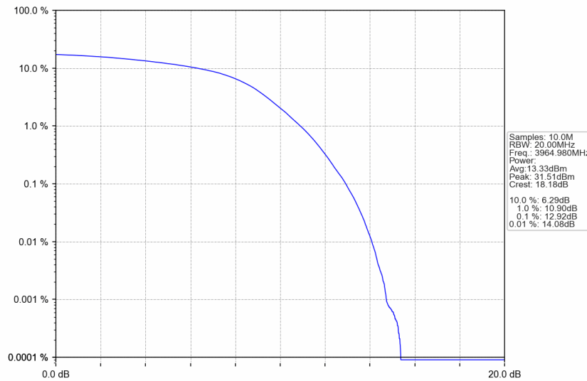
n77a_30kHz_SISO_NTNV_30MHz_DFT-s-OFDM 256 QAM_3964.98MHz_Outer_Full
