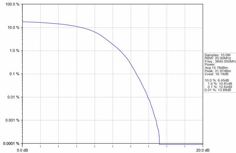
n77a_30kHz_SISO_NTNV_25MHz_DFT-s-OFDM 64 QAM_3840MHz_Outer_Full
