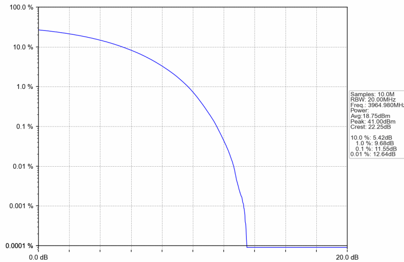
n77a_30kHz_SISO_NTNV_30MHz_CP-OFDM 16 QAM_3964.98MHz_Outer_Full
