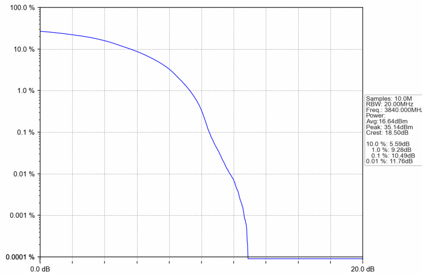
n77a_30kHz_SISO_NTNV_40MHz_DFT-s-OFDM 64 QAM_3840MHz_Outer_Full
