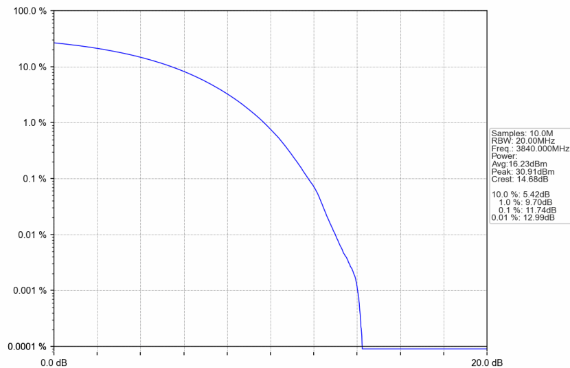
n77a_30kHz_SISO_NTNV_50MHz_CP-OFDM 16 QAM_3840MHz_Outer_Full
