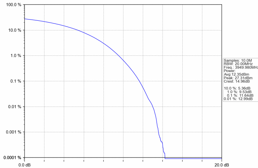
n77a_30kHz_SISO_NTNV_60MHz_CP-OFDM 256 QAM_3949.98MHz_Outer_Full
