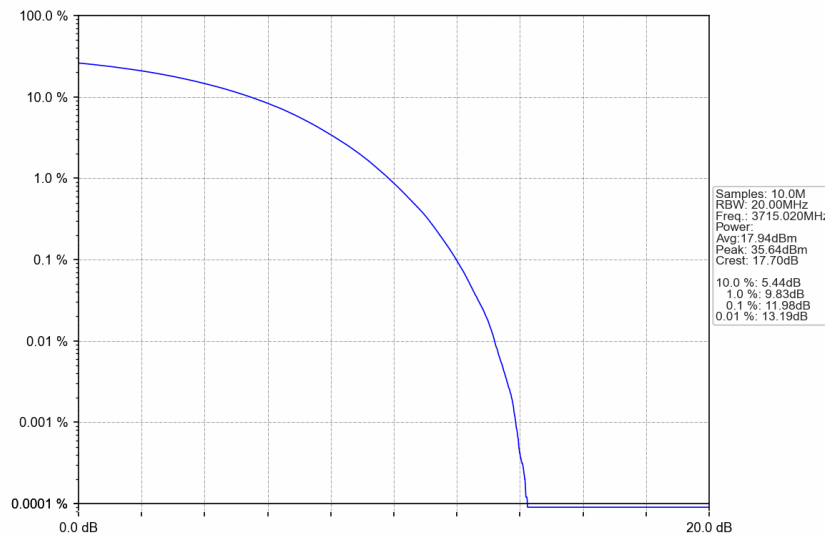
n77a_30kHz_SISO_NTNV_30MHz_CP-OFDM 64 QAM_3715.02MHz_Outer_Full
