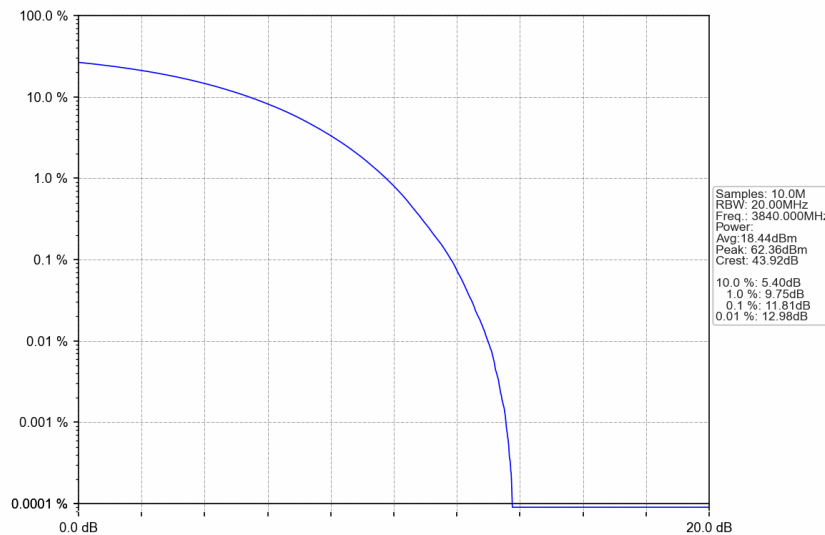
n77a_30kHz_SISO_NTNV_30MHz_CP-OFDM 16 QAM_3840MHz_Outer_Full
