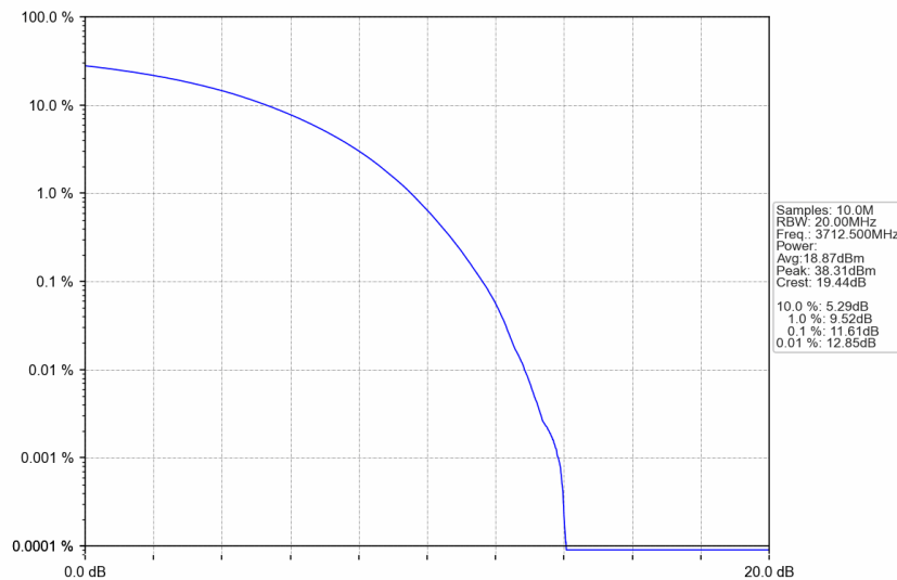
n77a_30kHz_SISO_NTNV_25MHz_CP-OFDM 64 QAM_3712.5MHz_Outer_Full
