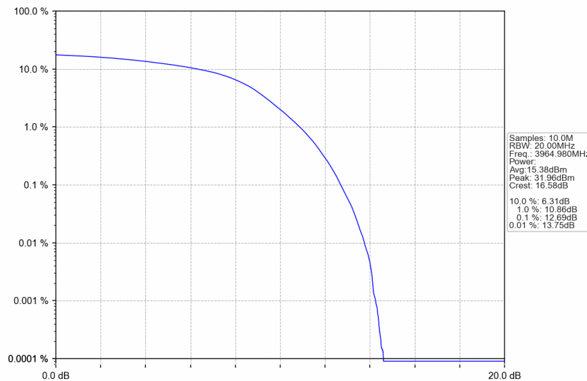
n77a_30kHz_SISO_NTNV_30MHz_DFT-s-OFDM 64 QAM_3964.98MHz_Outer_Full
