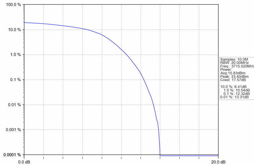
n77a_30kHz_SISO_NTNV_30MHz_DFT-s-OFDM 16 QAM_3715.02MHz_Outer_Full
