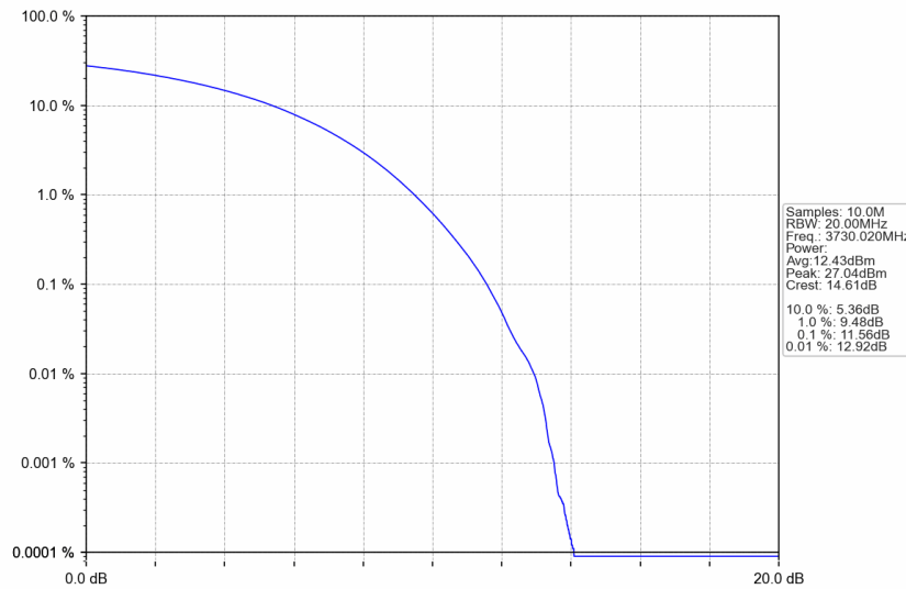
n77a_30kHz_SISO_NTNV_60MHz_CP-OFDM 256 QAM_3730.02MHz_Outer_Full
