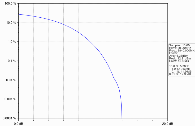
n77a_30kHz_SISO_NTNV_50MHz_CP-OFDM QPSK_3840MHz_Outer_Full
