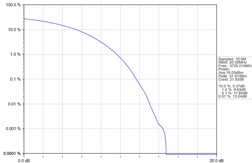
n77a_30kHz_SISO_NTNV_50MHz_CP-OFDM 64 QAM_3725.01MHz_Outer_Full
