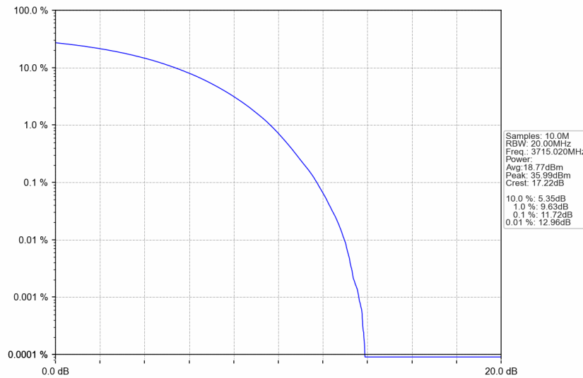
n77a_30kHz_SISO_NTNV_30MHz_CP-OFDM 16 QAM_3715.02MHz_Outer_Full
