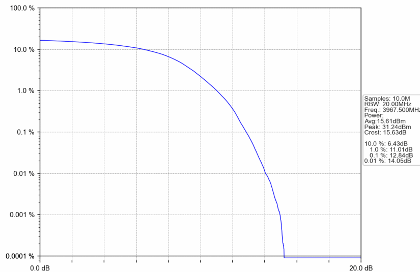
n77a_30kHz_SISO_NTNV_25MHz_DFT-s-OFDM 64 QAM_3967.5MHz_Outer_Full
