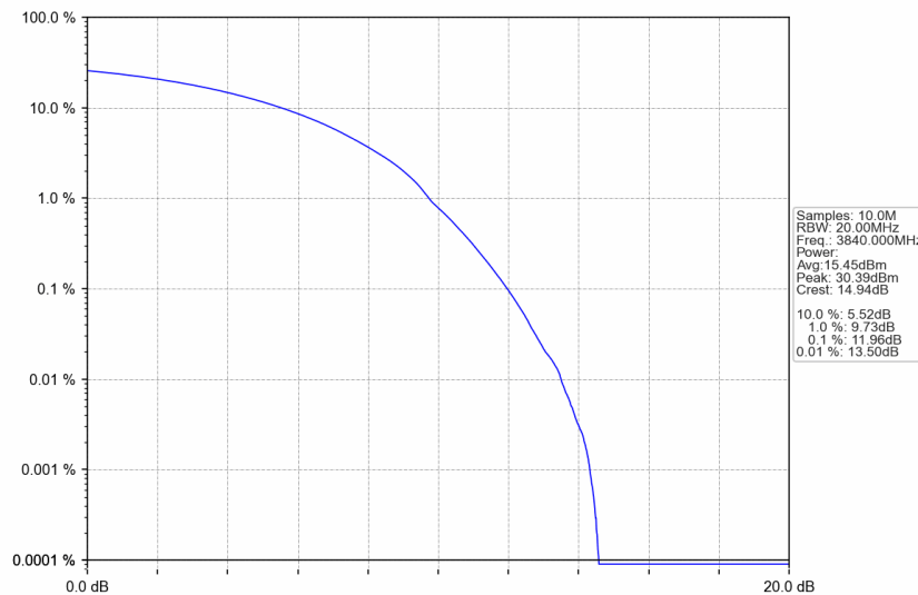
n77a_15kHz_SISO_NTNV_20MHz_CP-OFDM 256 QAM_3840MHz_Outer_Full
