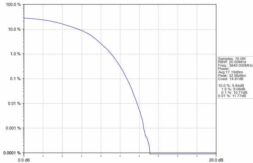
n77a_15kHz_SISO_NTNV_40MHz_DFT-s-OFDM 64 QAM_3840MHz_Outer_Full
