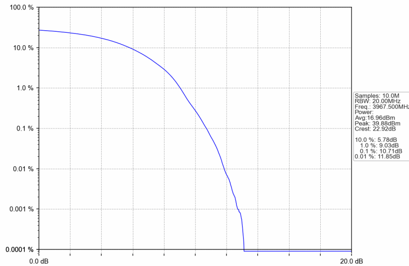
n77a_15kHz_SISO_NTNV_25MHz_DFT-s-OFDM 256 QAM_3967.5MHz_Outer_Full
