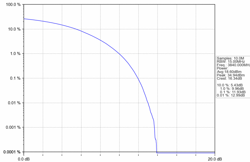
n77a_15kHz_SISO_NTNV_15MHz_CP-OFDM 64 QAM_3840MHz_Outer_Full
