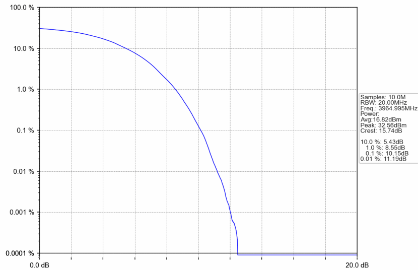
n77a_15kHz_SISO_NTNV_30MHz_DFT-s-OFDM 256 QAM_3964.995MHz_Outer_Full
