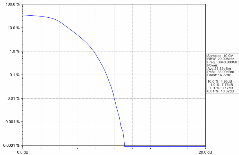
n77a_15kHz_SISO_NTNV_20MHz_DFT-s-OFDM QPSK_3840MHz_Outer_Full
