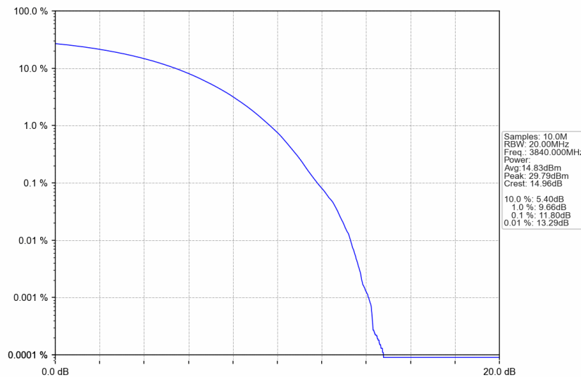
n77a_15kHz_SISO_NTNV_30MHz_CP-OFDM 256 QAM_3840MHz_Outer_Full
