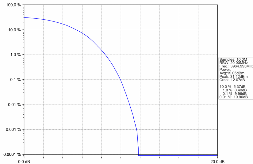
n77a_15kHz_SISO_NTNV_30MHz_DFT-s-OFDM 64 QAM_3964.995MHz_Outer_Full
