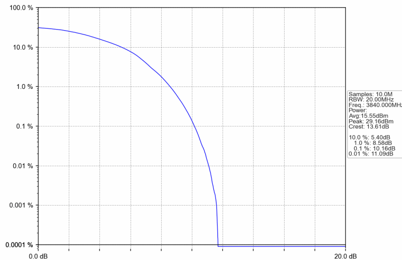
n77a_15kHz_SISO_NTNV_40MHz_DFT-s-OFDM 256 QAM_3840MHz_Outer_Full
