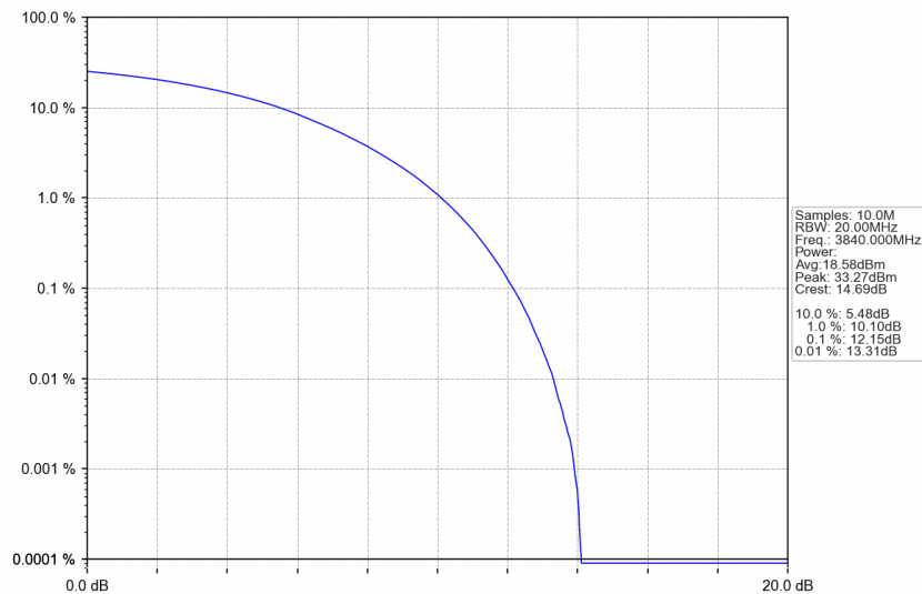
n77a_15kHz_SISO_NTNV_20MHz_CP-OFDM 16 QAM_3840MHz_Outer_Full
