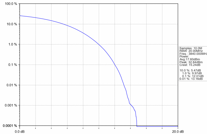
n77a_15kHz_SISO_NTNV_30MHz_CP-OFDM 64 QAM_3840MHz_Outer_Full
