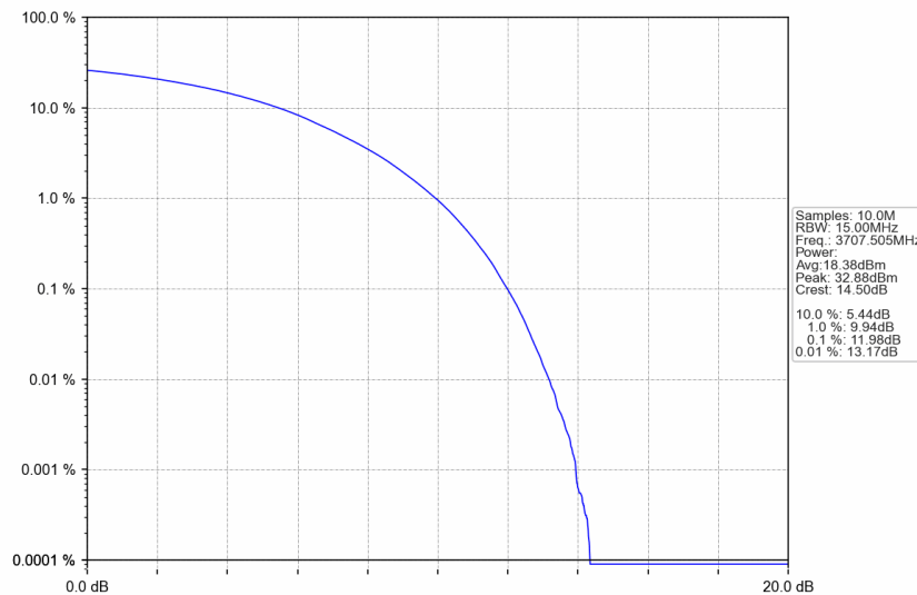
n77a_15kHz_SISO_NTNV_15MHz_CP-OFDM 64 QAM_3707.505MHz_Outer_Full
