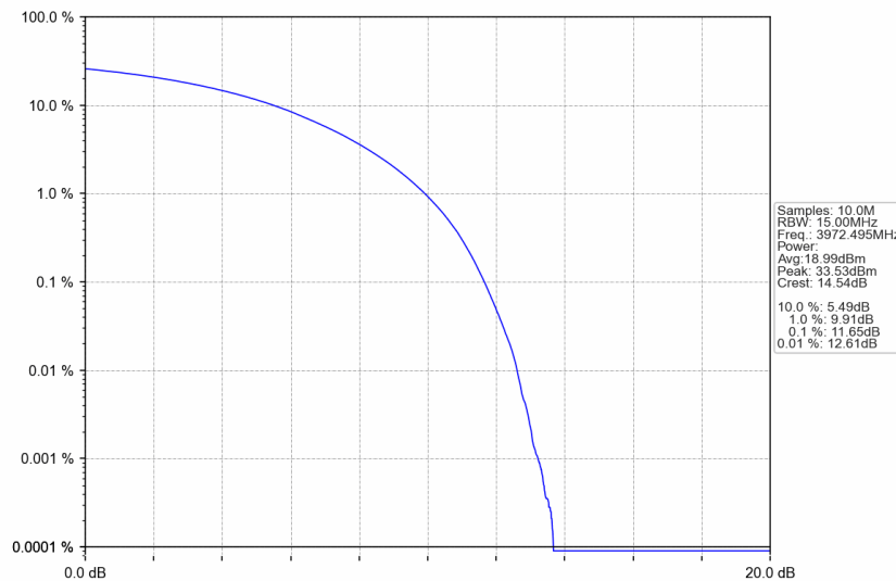
n77a_15kHz_SISO_NTNV_15MHz_CP-OFDM QPSK_3972.495MHz_Outer_Full
