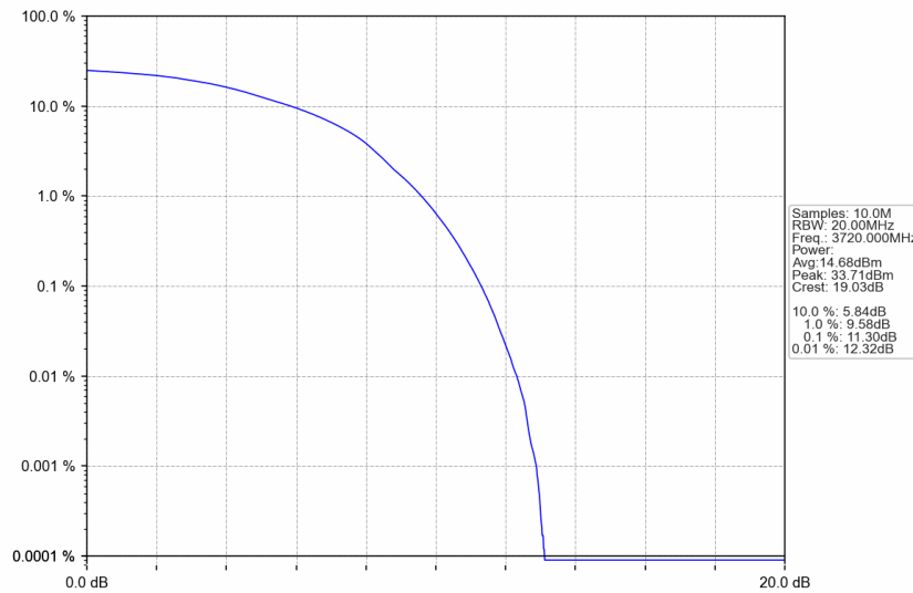
n77a_15kHz_SISO_NTNV_40MHz_DFT-s-OFDM 256 QAM_3720MHz_Outer_Full
