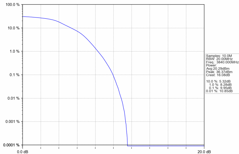
n77a_15kHz_SISO_NTNV_20MHz_DFT-s-OFDM 16 QAM_3840MHz_Outer_Full
