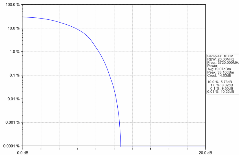
n77a_15kHz_SISO_NTNV_40MHz_DFT-s-OFDM QPSK_3720MHz_Outer_Full
