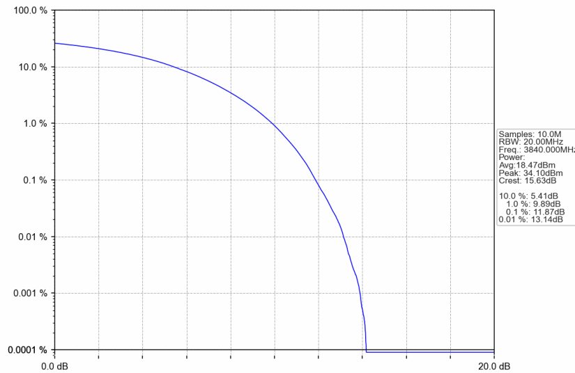
n77a_15kHz_SISO_NTNV_25MHz_CP-OFDM 64 QAM_3840MHz_Outer_Full
