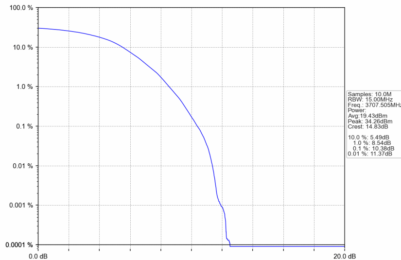
n77a_15kHz_SISO_NTNV_15MHz_DFT-s-OFDM 64 QAM_3707.505MHz_Outer_Full
