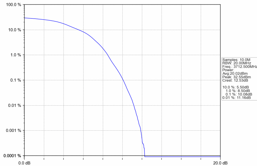
n77a_15kHz_SISO_NTNV_25MHz_DFT-s-OFDM 16 QAM_3712.5MHz_Outer_Full
