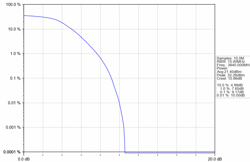
n77a_15kHz_SISO_NTNV_15MHz_DFT-s-OFDM QPSK_3840MHz_Outer_Full
