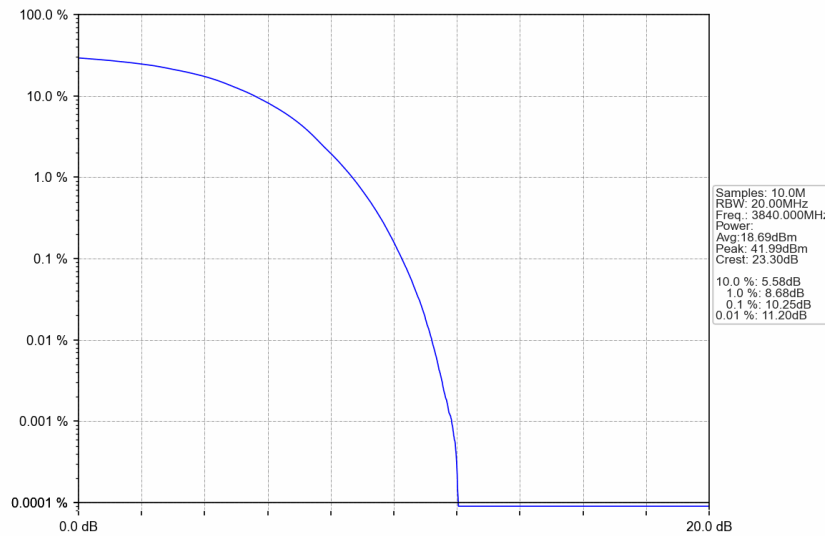
n77a_15kHz_SISO_NTNV_30MHz_DFT-s-OFDM 64 QAM_3840MHz_Outer_Full
