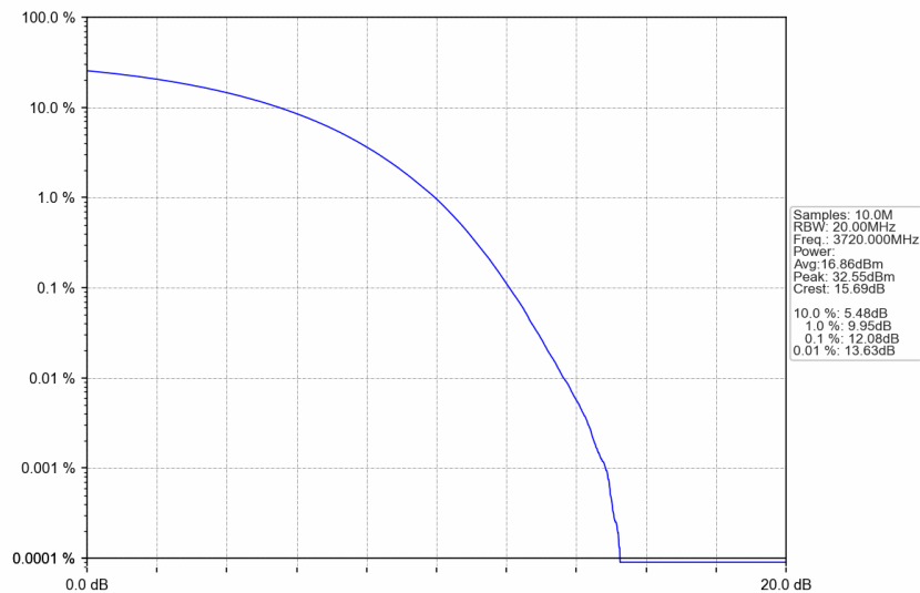
n77a_15kHz_SISO_NTNV_40MHz_CP-OFDM QPSK_3720MHz_Outer_Full
