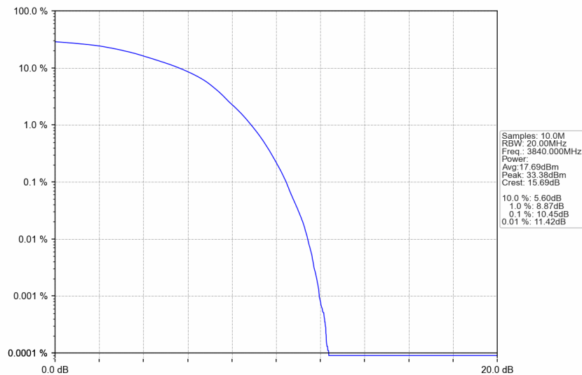
n77a_15kHz_SISO_NTNV_40MHz_DFT-s-OFDM 16 QAM_3840MHz_Outer_Full
