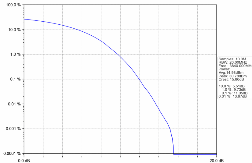
n77a_15kHz_SISO_NTNV_25MHz_CP-OFDM 256 QAM_3840MHz_Outer_Full
