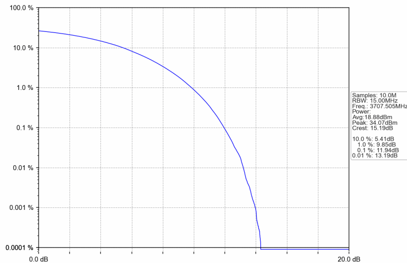
n77a_15kHz_SISO_NTNV_15MHz_CP-OFDM QPSK_3707.505MHz_Outer_Full
