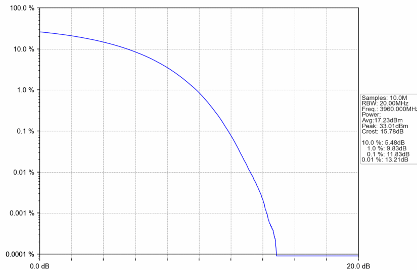
n77a_15kHz_SISO_NTNV_40MHz_CP-OFDM QPSK_3960MHz_Outer_Full
