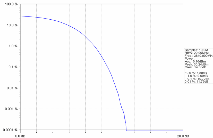
n77a_15kHz_SISO_NTNV_30MHz_DFT-s-OFDM 256 QAM_3840MHz_Outer_Full
