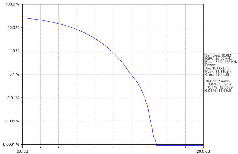
n77a_15kHz_SISO_NTNV_30MHz_CP-OFDM 256 QAM_3964.995MHz_Outer_Full
