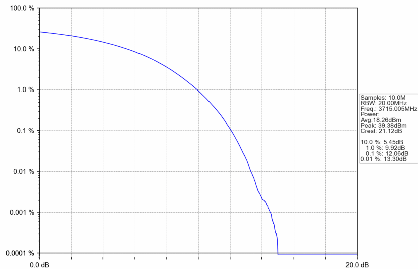
n77a_15kHz_SISO_NTNV_30MHz_CP-OFDM QPSK_3715.005MHz_Outer_Full
