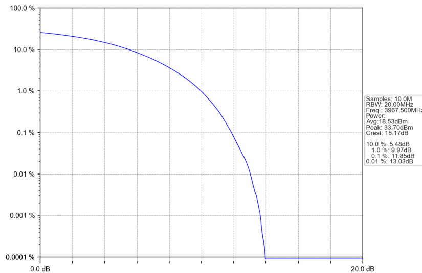
n77a_15kHz_SISO_NTNV_25MHz_CP-OFDM 64 QAM_3967.5MHz_Outer_Full
