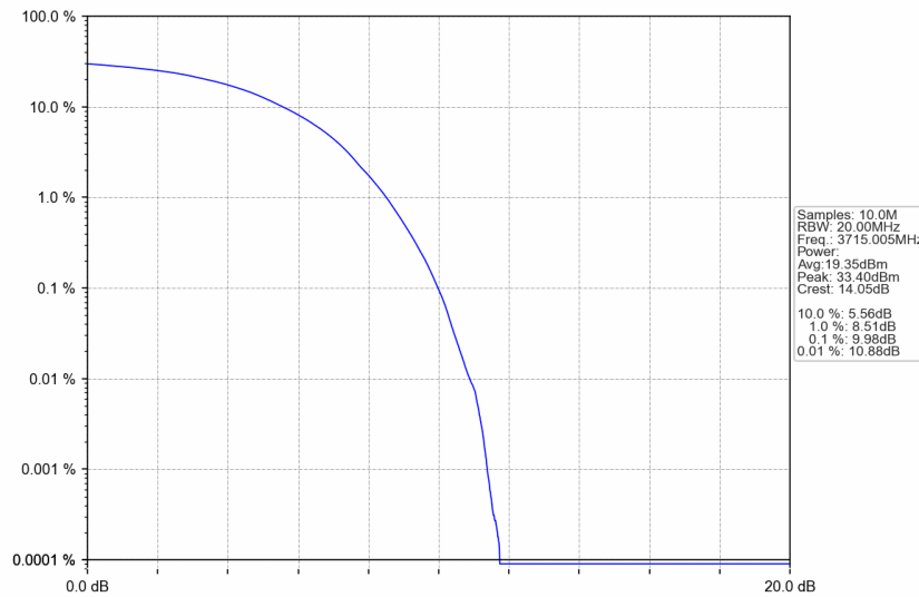
n77a_15kHz_SISO_NTNV_30MHz_DFT-s-OFDM 16 QAM_3715.005MHz_Outer_Full
