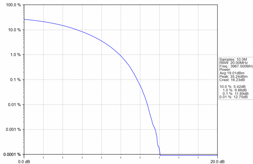
n77a_15kHz_SISO_NTNV_25MHz_CP-OFDM QPSK_3967.5MHz_Outer_Full
