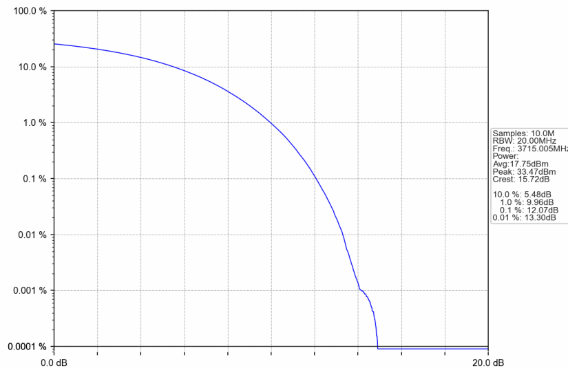
n77a_15kHz_SISO_NTNV_30MHz_CP-OFDM 64 QAM_3715.005MHz_Outer_Full
