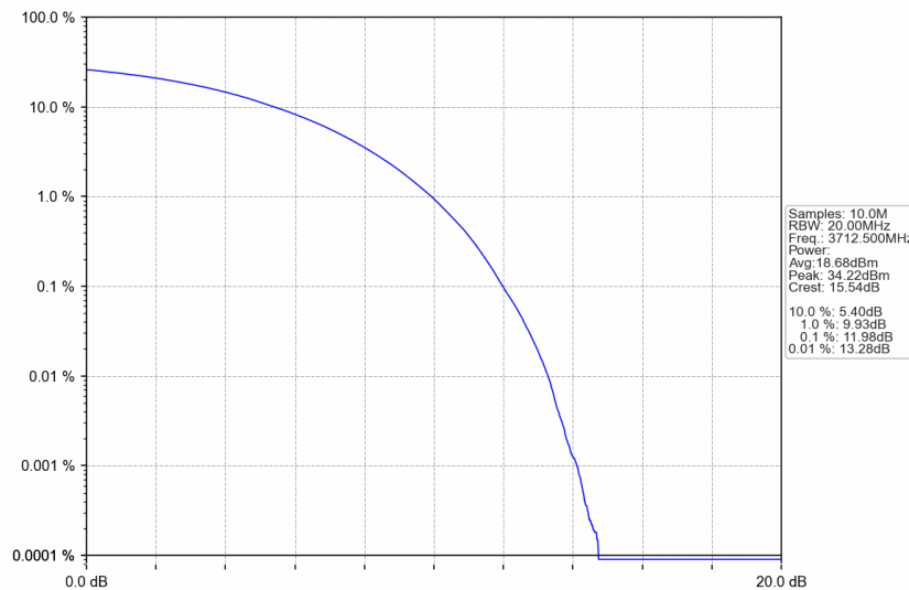
n77a_15kHz_SISO_NTNV_25MHz_CP-OFDM QPSK_3712.5MHz_Outer_Full
