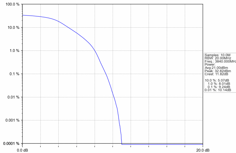
n77a_15kHz_SISO_NTNV_25MHz_DFT-s-OFDM QPSK_3840MHz_Outer_Full
