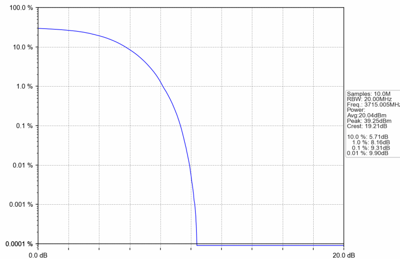
n77a_15kHz_SISO_NTNV_30MHz_DFT-s-OFDM QPSK_3715.005MHz_Outer_Full
