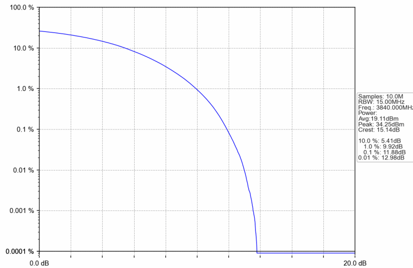
n77a_15kHz_SISO_NTNV_15MHz_CP-OFDM QPSK_3840MHz_Outer_Full
