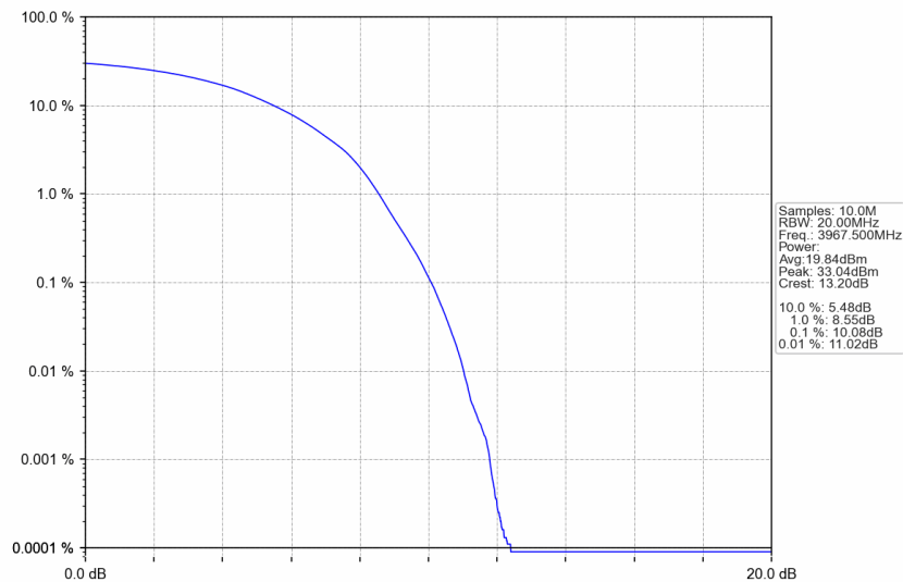
n77a_15kHz_SISO_NTNV_25MHz_DFT-s-OFDM 64 QAM_3967.5MHz_Outer_Full
