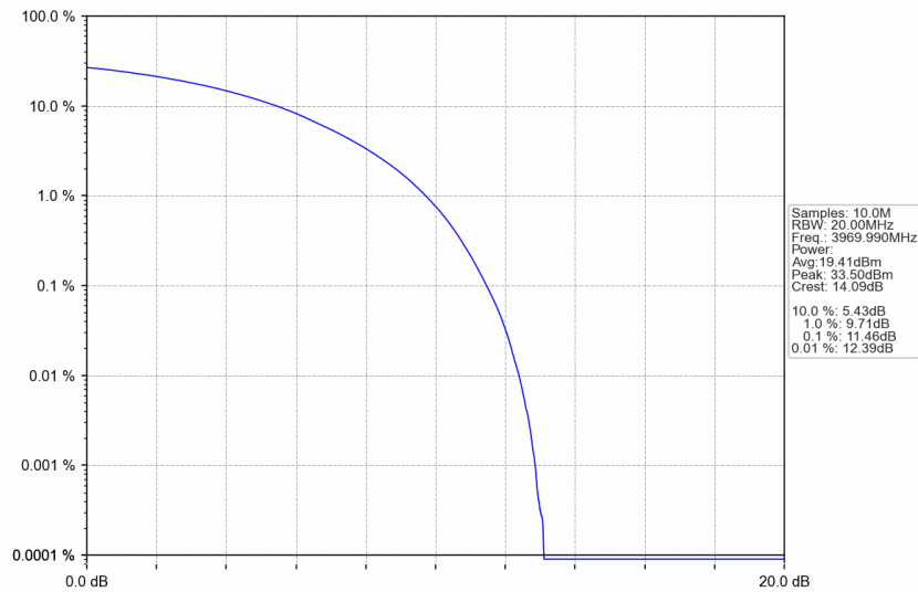
n77a_15kHz_SISO_NTNV_20MHz_CP-OFDM 16 QAM_3969.99MHz_Outer_Full
