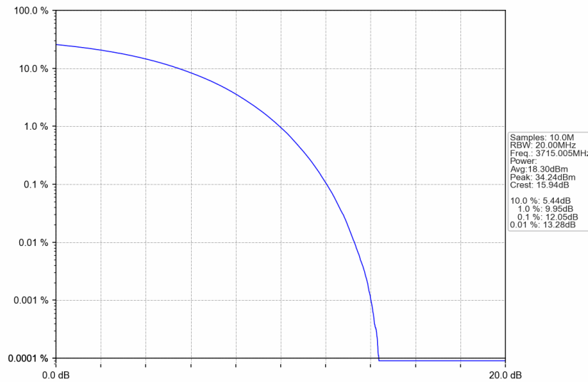
n77a_15kHz_SISO_NTNV_30MHz_CP-OFDM 16 QAM_3715.005MHz_Outer_Full
