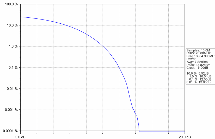
n77a_15kHz_SISO_NTNV_30MHz_CP-OFDM 64 QAM_3964.995MHz_Outer_Full
