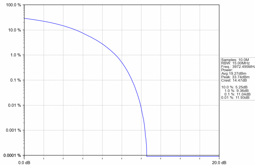
n77a_15kHz_SISO_NTNV_15MHz_CP-OFDM 64 QAM_3972.495MHz_Outer_Full
