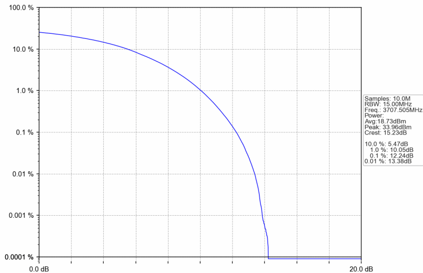
n77a_15kHz_SISO_NTNV_15MHz_CP-OFDM 16 QAM_3707.505MHz_Outer_Full
