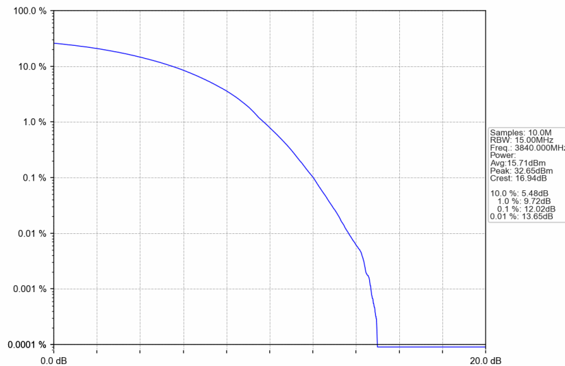
n77a_15kHz_SISO_NTNV_15MHz_CP-OFDM 256 QAM_3840MHz_Outer_Full
