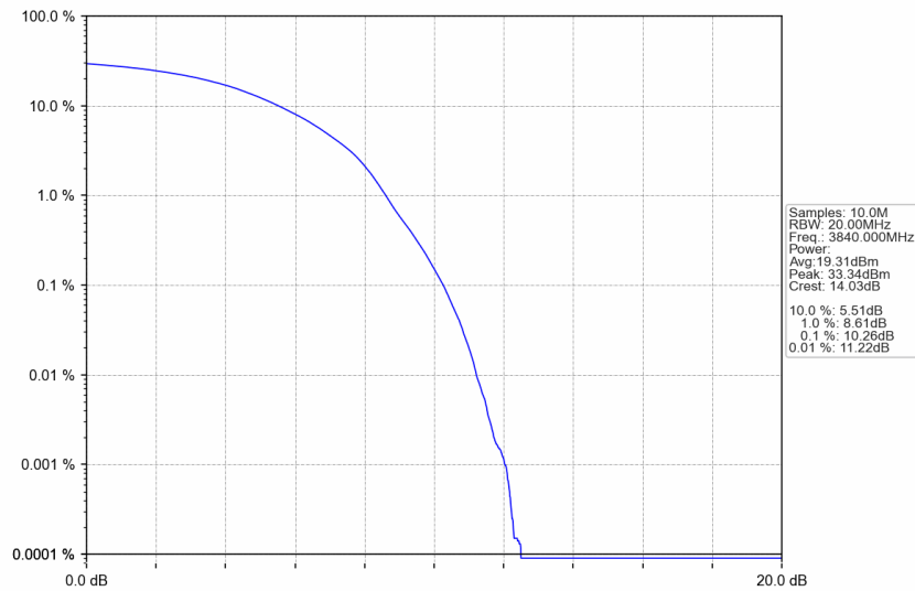
n77a_15kHz_SISO_NTNV_25MHz_DFT-s-OFDM 64 QAM_3840MHz_Outer_Full
