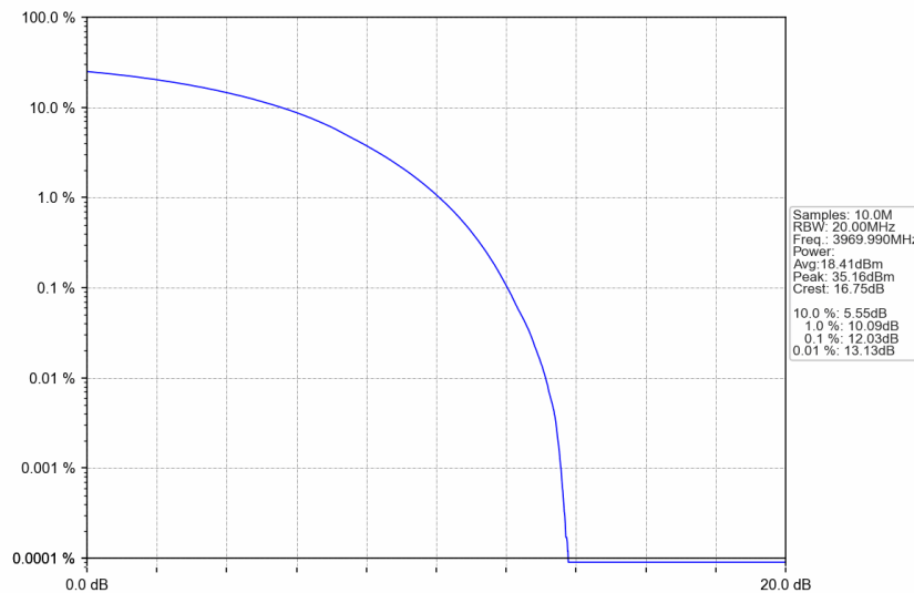
n77a_15kHz_SISO_NTNV_20MHz_CP-OFDM 64 QAM_3969.99MHz_Outer_Full
