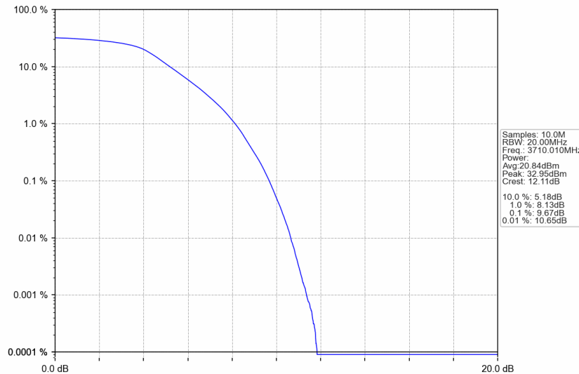
n77a_15kHz_SISO_NTNV_20MHz_DFT-s-OFDM QPSK_3710.01MHz_Outer_Full
