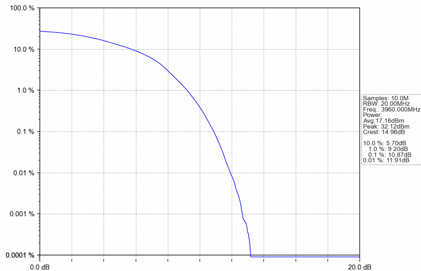
n77a_15kHz_SISO_NTNV_40MHz_DFT-s-OFDM 64 QAM_3960MHz_Outer_Full
