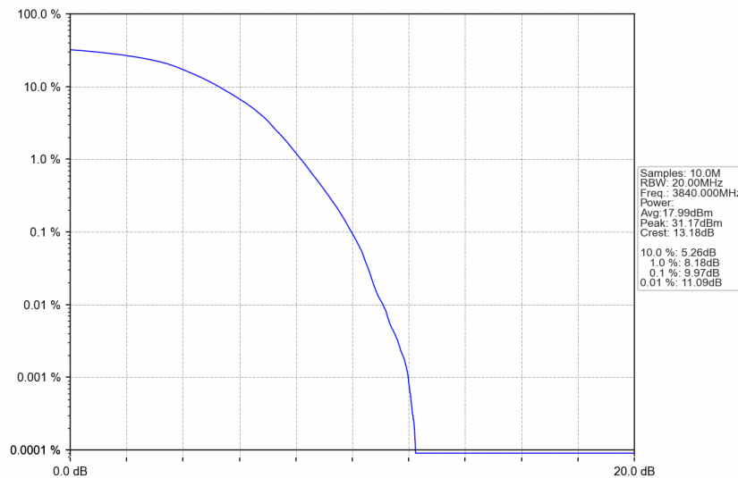
n77a_15kHz_SISO_NTNV_20MHz_DFT-s-OFDM 256 QAM_3840MHz_Outer_Full
