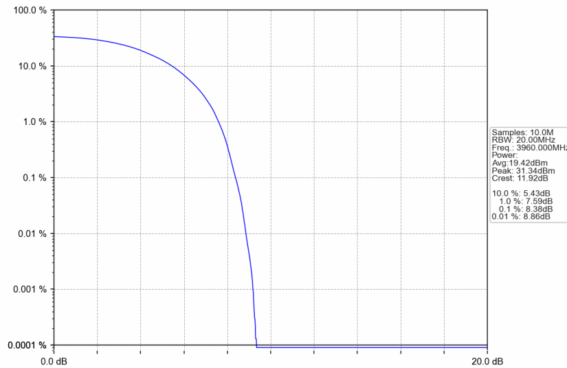
n77a_15kHz_SISO_NTNV_40MHz_DFT-s-OFDM PI/2 BPSK_3960MHz_Outer_Full
