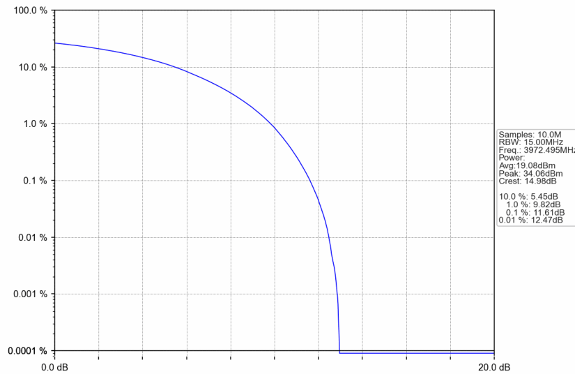
n77a_15kHz_SISO_NTNV_15MHz_CP-OFDM 16 QAM_3972.495MHz_Outer_Full
