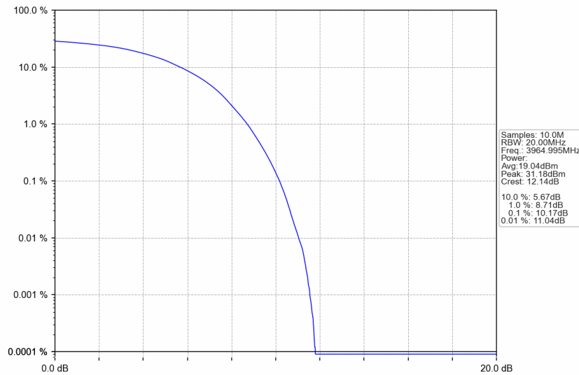
n77a_15kHz_SISO_NTNV_30MHz_DFT-s-OFDM 16 QAM_3964.995MHz_Outer_Full
