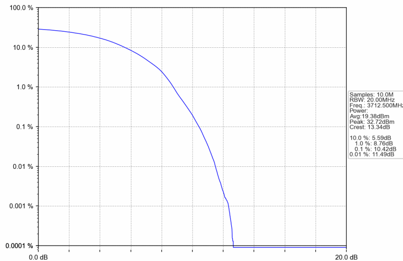
n77a_15kHz_SISO_NTNV_25MHz_DFT-s-OFDM 64 QAM_3712.5MHz_Outer_Full
