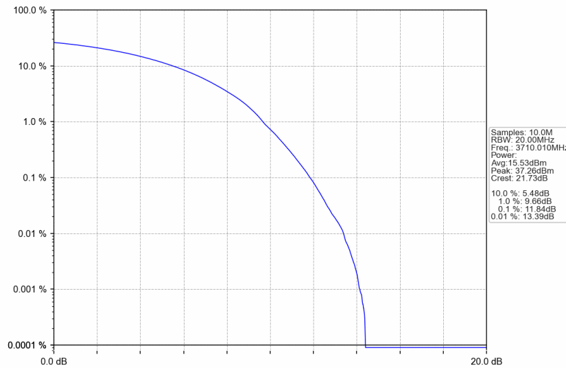
n77a_15kHz_SISO_NTNV_20MHz_CP-OFDM 256 QAM_3710.01MHz_Outer_Full
