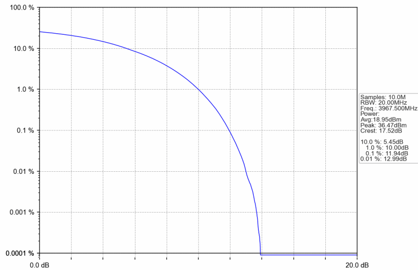
n77a_15kHz_SISO_NTNV_25MHz_CP-OFDM 16 QAM_3967.5MHz_Outer_Full
