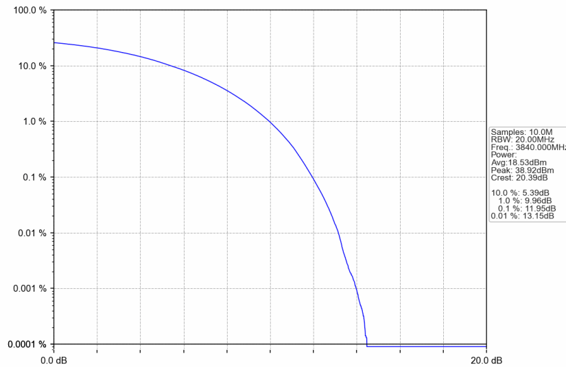
n77a_15kHz_SISO_NTNV_25MHz_CP-OFDM QPSK_3840MHz_Outer_Full
