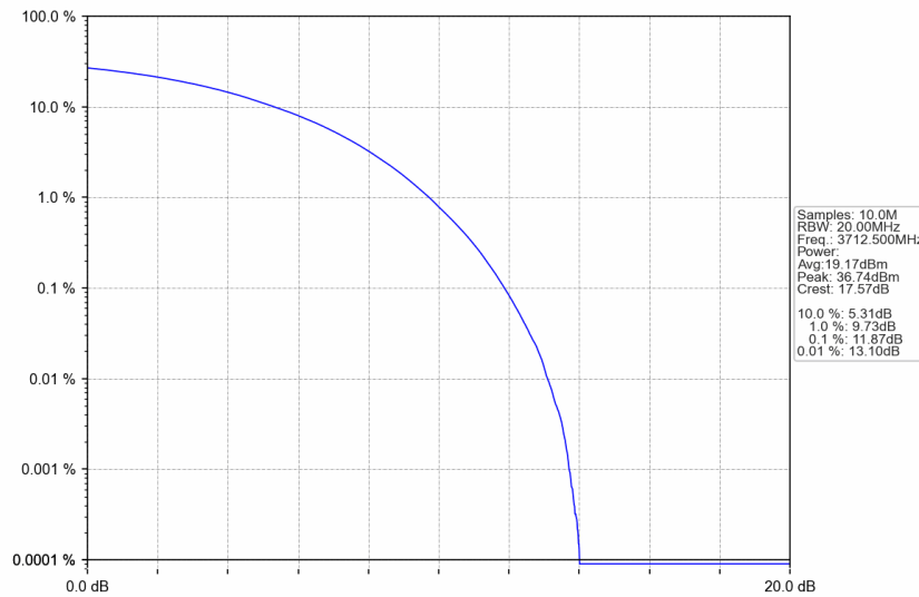
n77a_15kHz_SISO_NTNV_25MHz_CP-OFDM 16 QAM_3712.5MHz_Outer_Full
