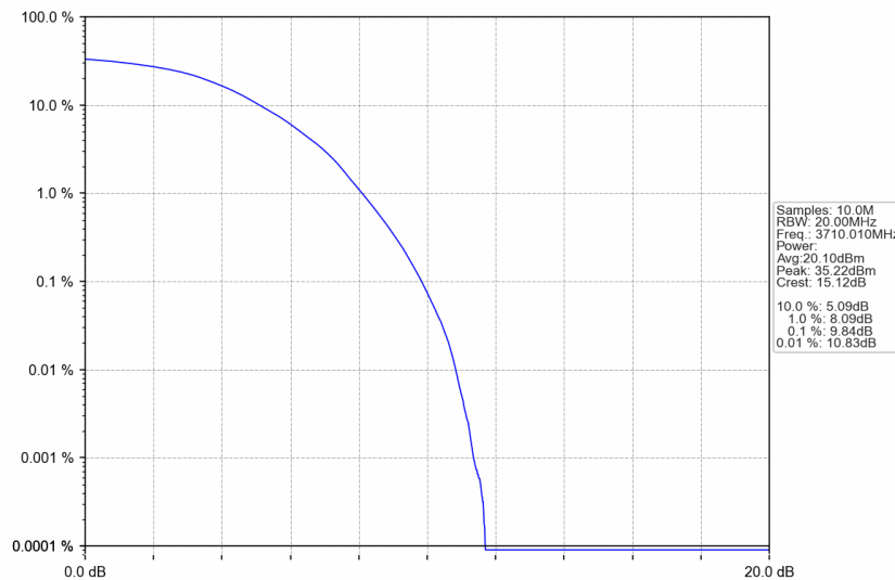
n77a_15kHz_SISO_NTNV_20MHz_DFT-s-OFDM 64 QAM_3710.01MHz_Outer_Full
