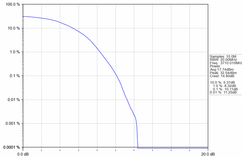
n77a_15kHz_SISO_NTNV_20MHz_DFT-s-OFDM 256 QAM_3710.01MHz_Outer_Full
