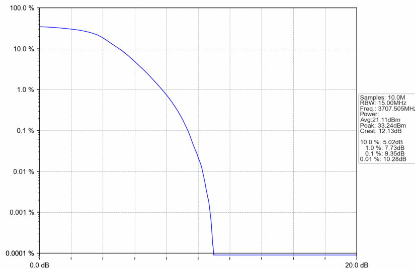
n77a_15kHz_SISO_NTNV_15MHz_DFT-s-OFDM QPSK_3707.505MHz_Outer_Full
