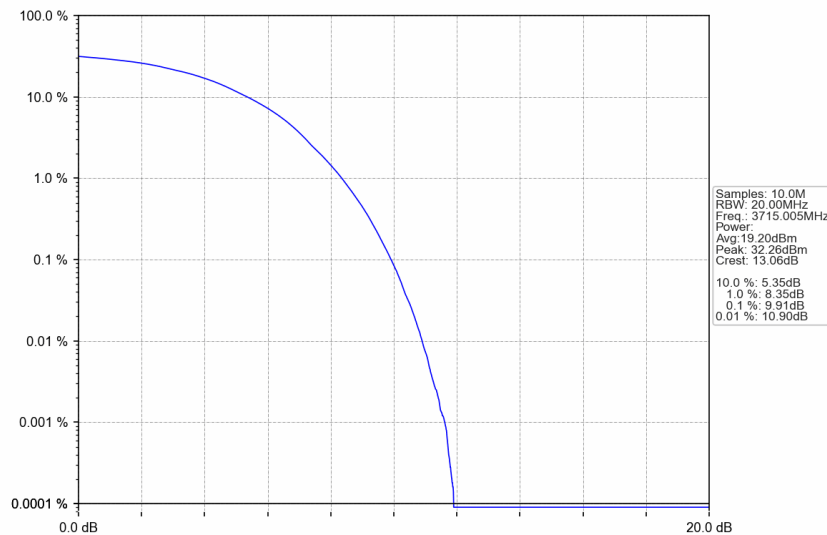
n77a_15kHz_SISO_NTNV_30MHz_DFT-s-OFDM 64 QAM_3715.005MHz_Outer_Full
