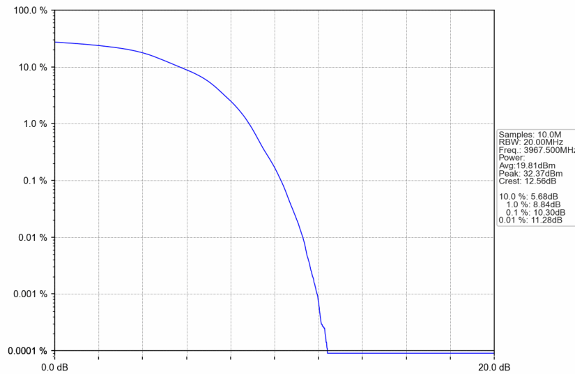
n77a_15kHz_SISO_NTNV_25MHz_DFT-s-OFDM 16 QAM_3967.5MHz_Outer_Full
