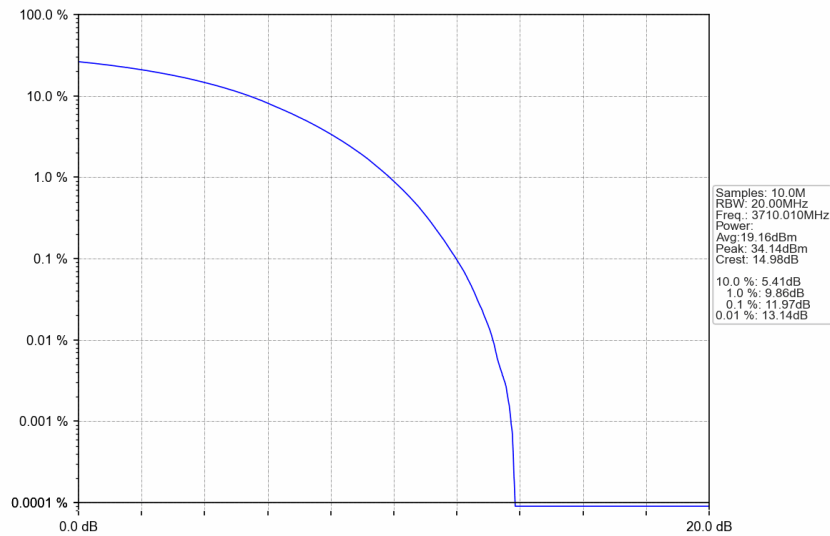
n77a_15kHz_SISO_NTNV_20MHz_CP-OFDM 16 QAM_3710.01MHz_Outer_Full
