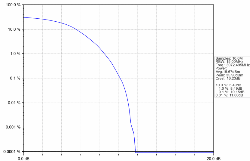
n77a_15kHz_SISO_NTNV_15MHz_DFT-s-OFDM 64 QAM_3972.495MHz_Outer_Full
