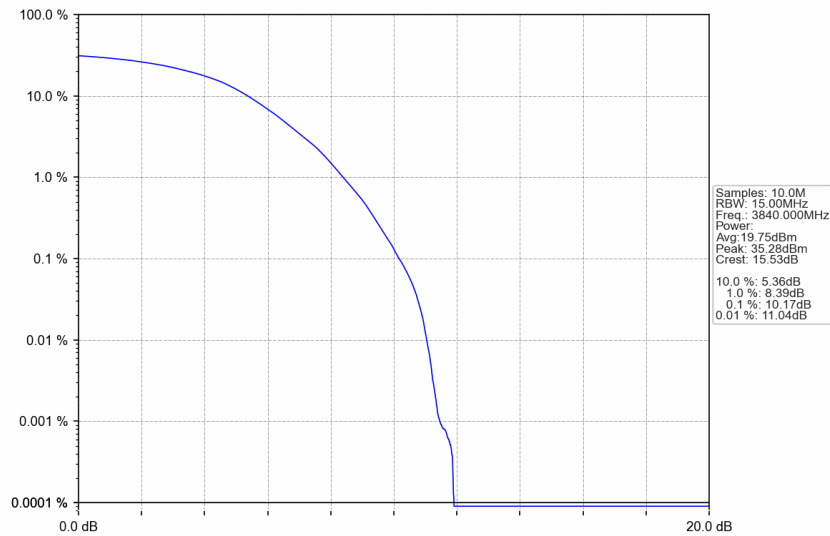
n77a_15kHz_SISO_NTNV_15MHz_DFT-s-OFDM 64 QAM_3840MHz_Outer_Full
