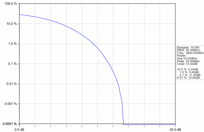
n77a_15kHz_SISO_NTNV_20MHz_CP-OFDM 64 QAM_3840MHz_Outer_Full
