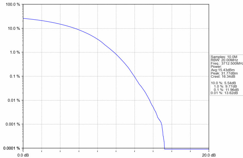
n77a_15kHz_SISO_NTNV_25MHz_CP-OFDM 256 QAM_3712.5MHz_Outer_Full
