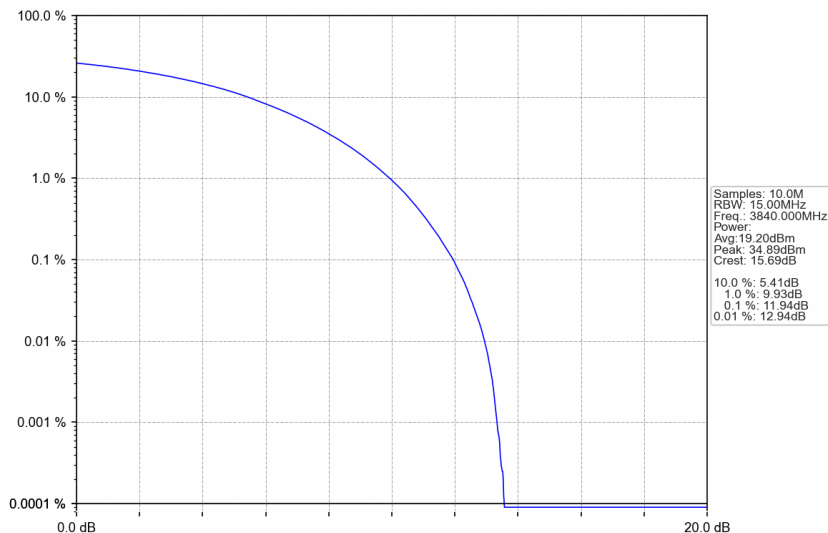
n77a_15kHz_SISO_NTNV_15MHz_CP-OFDM 16 QAM_3840MHz_Outer_Full
