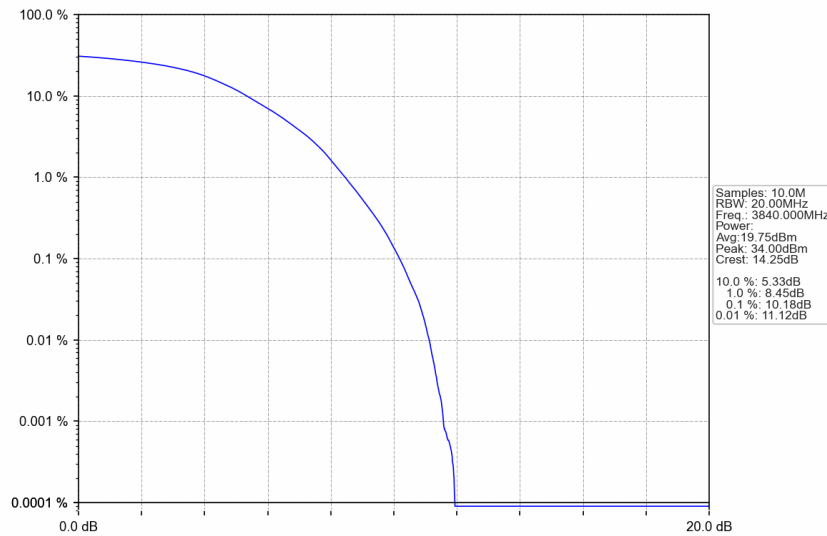
n77a_15kHz_SISO_NTNV_20MHz_DFT-s-OFDM 64 QAM_3840MHz_Outer_Full
