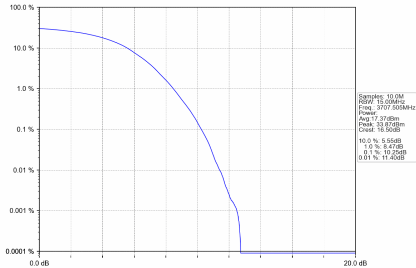
n77a_15kHz_SISO_NTNV_15MHz_DFT-s-OFDM 256 QAM_3707.505MHz_Outer_Full
