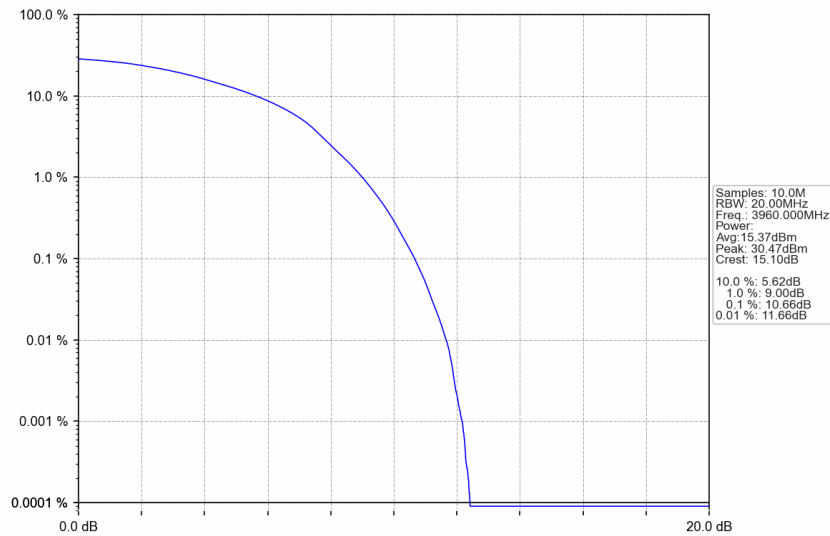
n77a_15kHz_SISO_NTNV_40MHz_DFT-s-OFDM 256 QAM_3960MHz_Outer_Full
