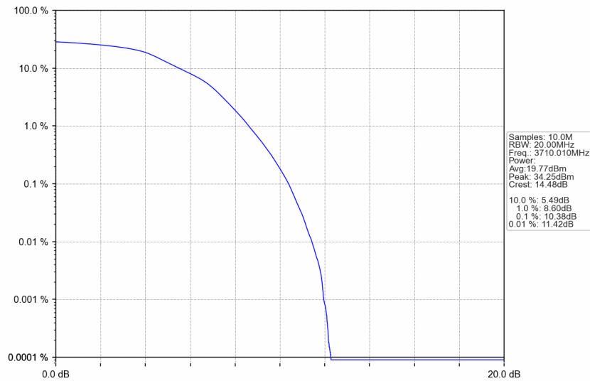
n77a_15kHz_SISO_NTNV_20MHz_DFT-s-OFDM 16 QAM_3710.01MHz_Outer_Full
