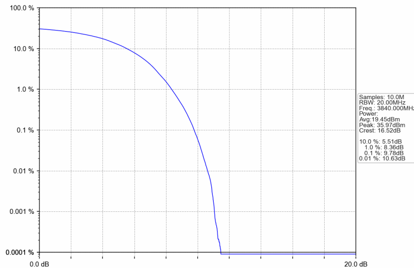
n77a_15kHz_SISO_NTNV_30MHz_DFT-s-OFDM 16 QAM_3840MHz_Outer_Full
