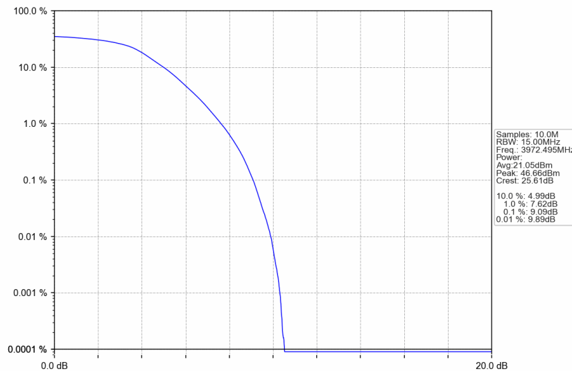
n77a_15kHz_SISO_NTNV_15MHz_DFT-s-OFDM QPSK_3972.495MHz_Outer_Full
