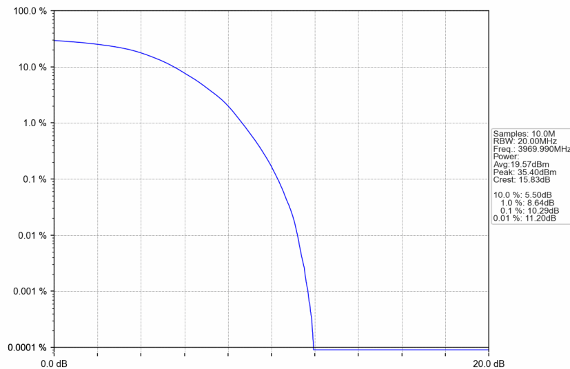
n77a_15kHz_SISO_NTNV_20MHz_DFT-s-OFDM 64 QAM_3969.99MHz_Outer_Full
