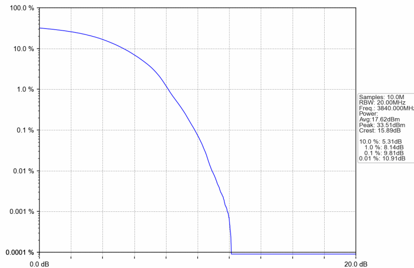
n77a_15kHz_SISO_NTNV_25MHz_DFT-s-OFDM 256 QAM_3840MHz_Outer_Full
