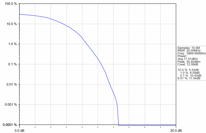
n77a_15kHz_SISO_NTNV_20MHz_DFT-s-OFDM 256 QAM_3969.99MHz_Outer_Full
