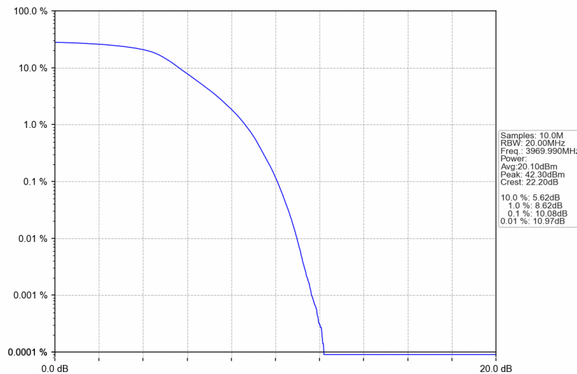
n77a_15kHz_SISO_NTNV_20MHz_DFT-s-OFDM QPSK_3969.99MHz_Outer_Full
