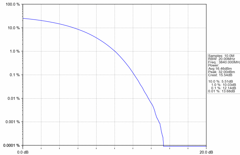
n77a_15kHz_SISO_NTNV_40MHz_CP-OFDM QPSK_3840MHz_Outer_Full
