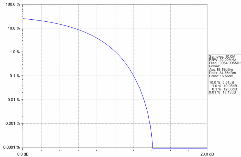
n77a_15kHz_SISO_NTNV_30MHz_CP-OFDM 16 QAM_3964.995MHz_Outer_Full
