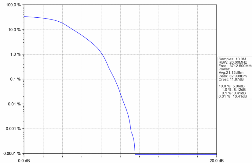
n77a_15kHz_SISO_NTNV_25MHz_DFT-s-OFDM QPSK_3712.5MHz_Outer_Full
