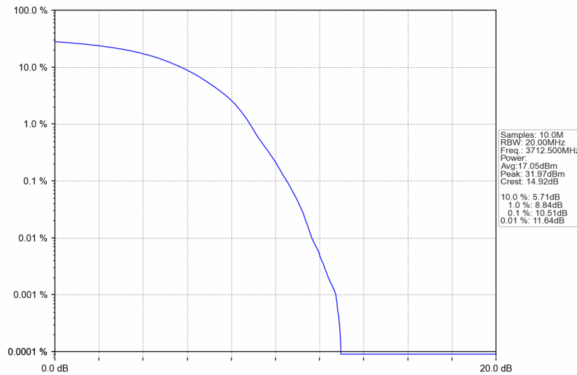
n77a_15kHz_SISO_NTNV_25MHz_DFT-s-OFDM 256 QAM_3712.5MHz_Outer_Full
