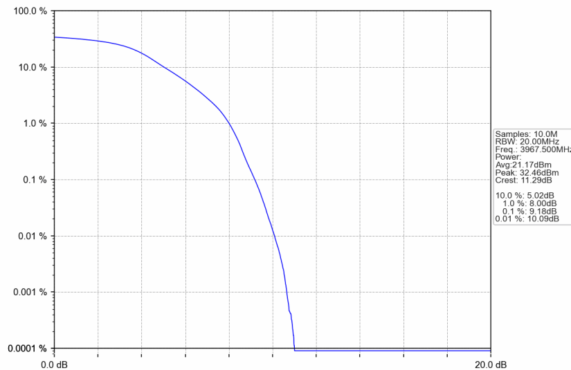
n77a_15kHz_SISO_NTNV_25MHz_DFT-s-OFDM QPSK_3967.5MHz_Outer_Full
