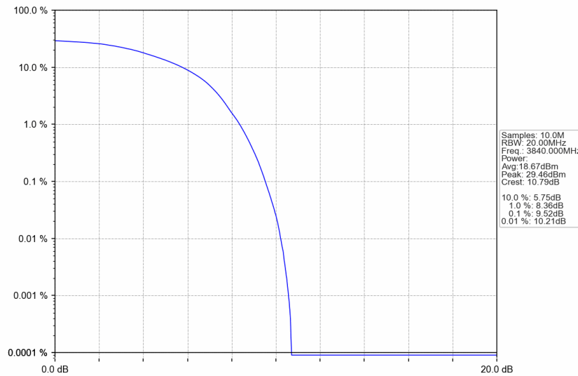
n77a_15kHz_SISO_NTNV_40MHz_DFT-s-OFDM QPSK_3840MHz_Outer_Full
