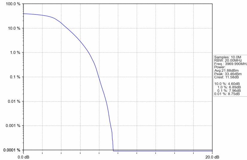
n77a_15kHz_SISO_NTNV_20MHz_DFT-s-OFDM PI/2 BPSK_3969.99MHz_Outer_Full
