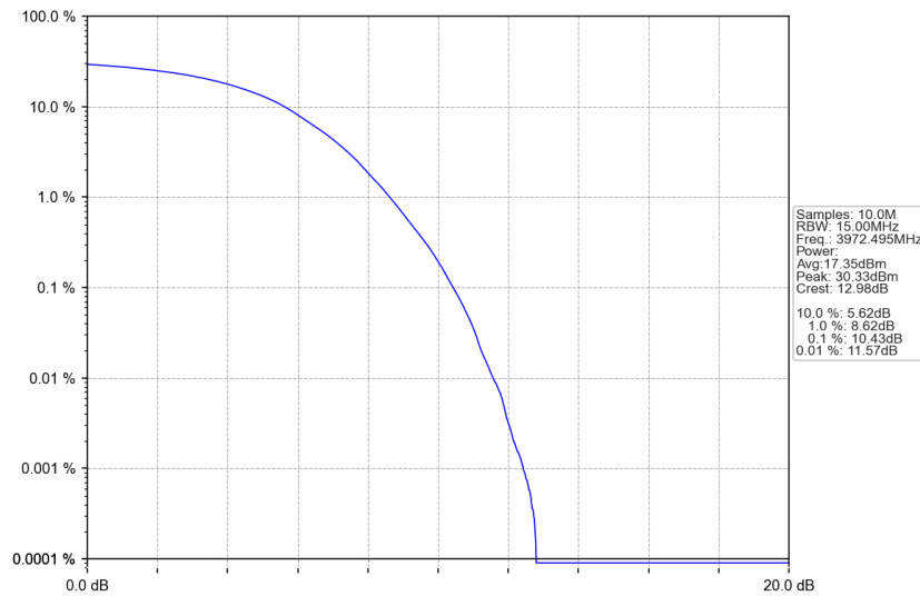
n77a_15kHz_SISO_NTNV_15MHz_DFT-s-OFDM 256 QAM_3972.495MHz_Outer_Full
