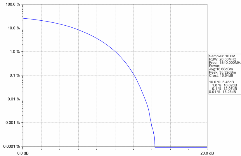
n77a_15kHz_SISO_NTNV_20MHz_CP-OFDM QPSK_3840MHz_Outer_Full
