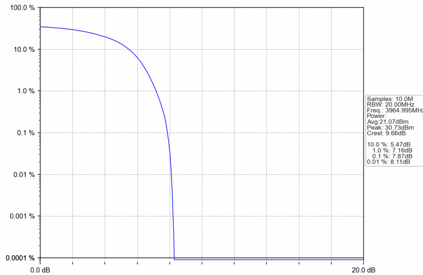
n77a_15kHz_SISO_NTNV_30MHz_DFT-s-OFDM PI/2 BPSK_3964.995MHz_Outer_Full
