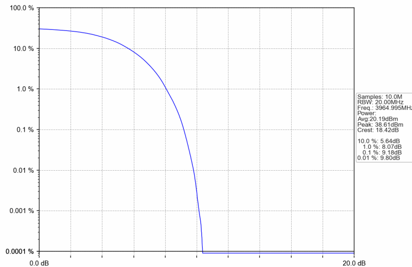
n77a_15kHz_SISO_NTNV_30MHz_DFT-s-OFDM QPSK_3964.995MHz_Outer_Full
