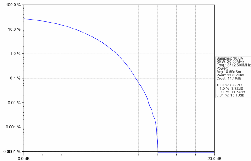
n77a_15kHz_SISO_NTNV_25MHz_CP-OFDM 64 QAM_3712.5MHz_Outer_Full
