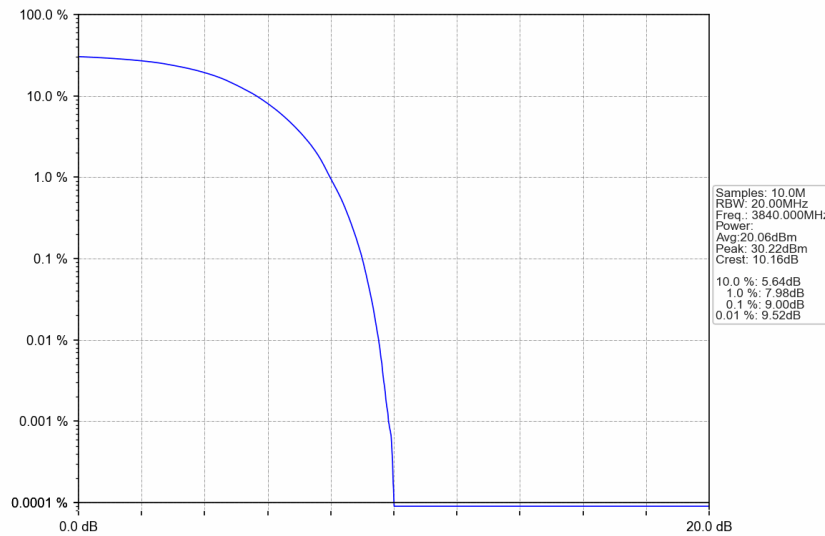
n77a_15kHz_SISO_NTNV_30MHz_DFT-s-OFDM QPSK_3840MHz_Outer_Full
