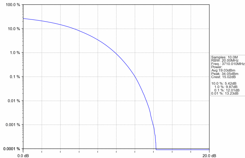
n77a_15kHz_SISO_NTNV_20MHz_CP-OFDM QPSK_3710.01MHz_Outer_Full
