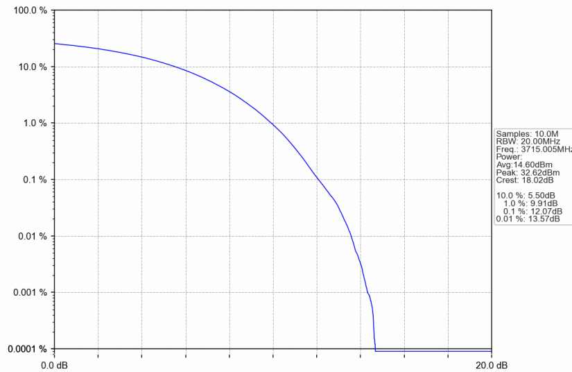
n77a_15kHz_SISO_NTNV_30MHz_CP-OFDM 256 QAM_3715.005MHz_Outer_Full
