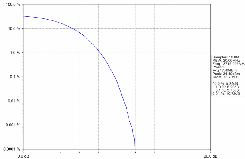
n77a_15kHz_SISO_NTNV_30MHz_DFT-s-OFDM 256 QAM_3715.005MHz_Outer_Full
