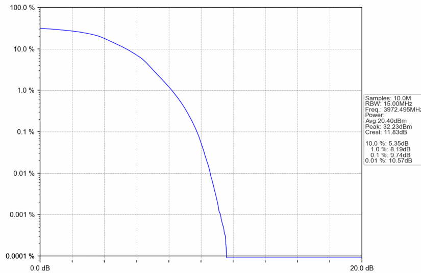
n77a_15kHz_SISO_NTNV_15MHz_DFT-s-OFDM 16 QAM_3972.495MHz_Outer_Full
