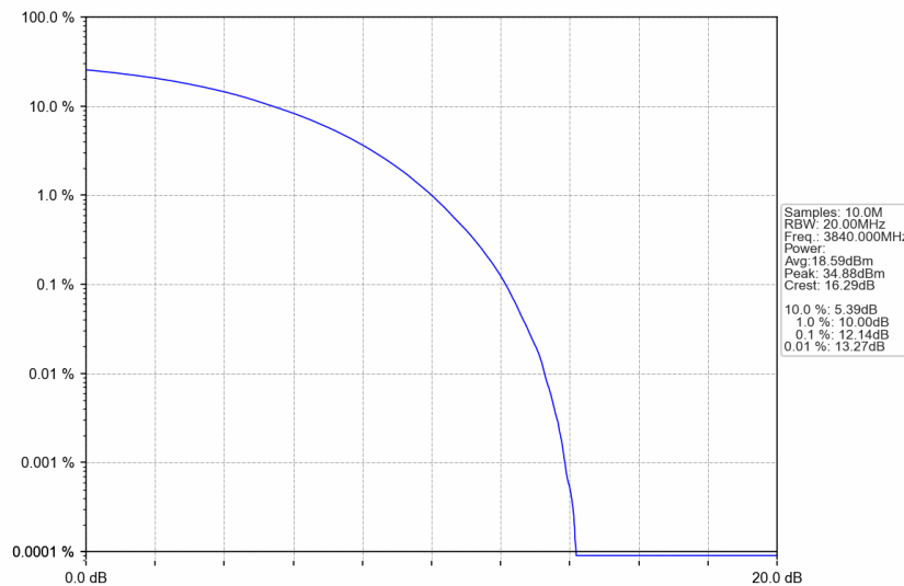
n77a_15kHz_SISO_NTNV_25MHz_CP-OFDM 16 QAM_3840MHz_Outer_Full
