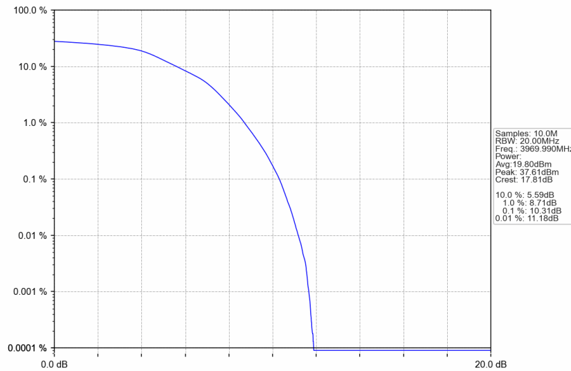
n77a_15kHz_SISO_NTNV_20MHz_DFT-s-OFDM 16 QAM_3969.99MHz_Outer_Full
