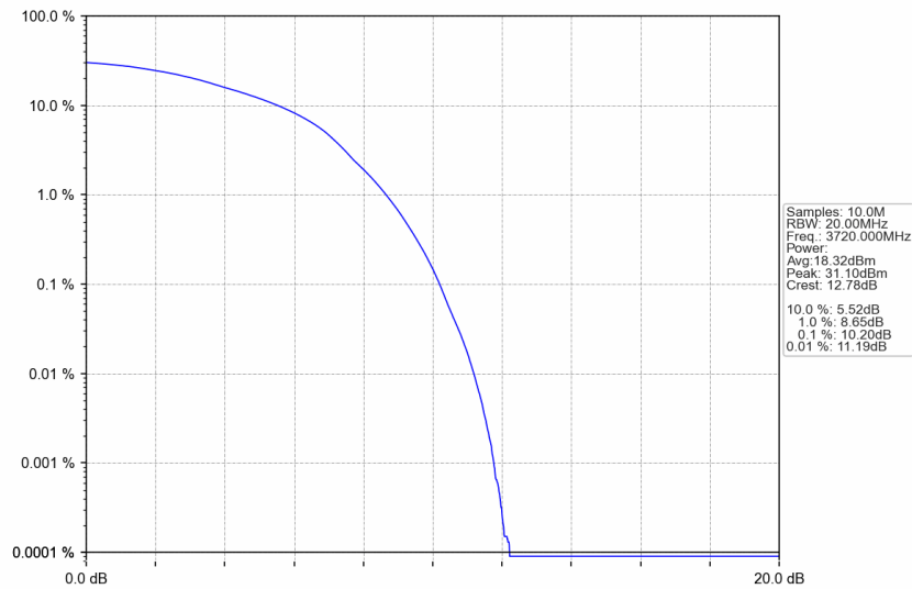
n77a_15kHz_SISO_NTNV_40MHz_DFT-s-OFDM 16 QAM_3720MHz_Outer_Full
