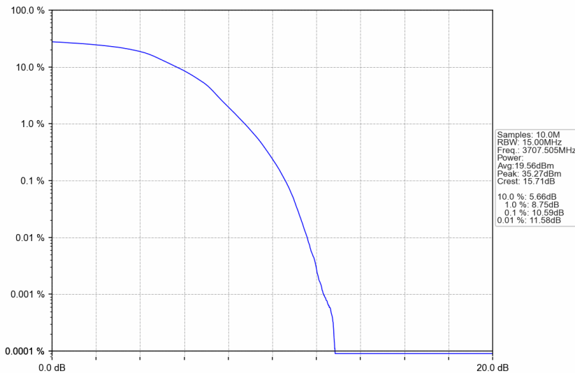
n77a_15kHz_SISO_NTNV_15MHz_DFT-s-OFDM 16 QAM_3707.505MHz_Outer_Full
