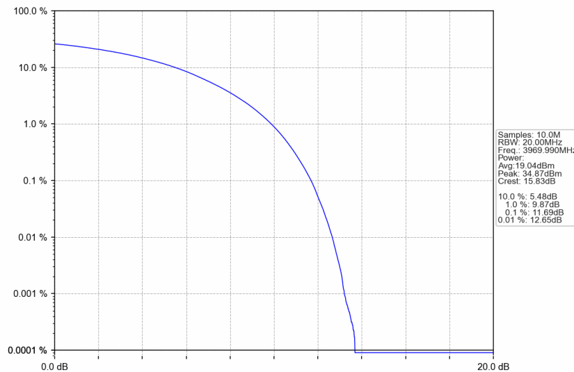
n77a_15kHz_SISO_NTNV_20MHz_CP-OFDM QPSK_3969.99MHz_Outer_Full
