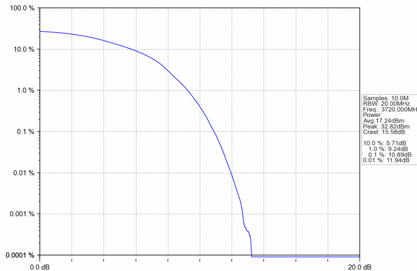
n77a_15kHz_SISO_NTNV_40MHz_DFT-s-OFDM 64 QAM_3720MHz_Outer_Full
