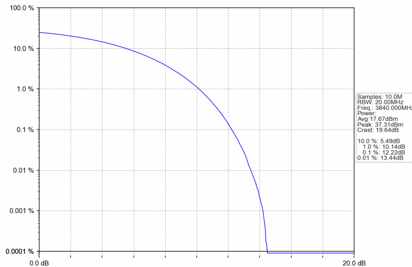
n77a_15kHz_SISO_NTNV_30MHz_CP-OFDM 16 QAM_3840MHz_Outer_Full
