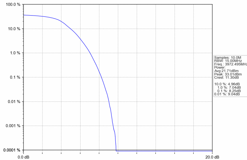
n77a_15kHz_SISO_NTNV_15MHz_DFT-s-OFDM PI/2 BPSK_3972.495MHz_Outer_Full
