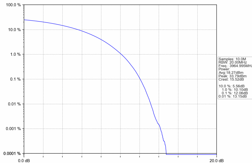
n77a_15kHz_SISO_NTNV_30MHz_CP-OFDM QPSK_3964.995MHz_Outer_Full
