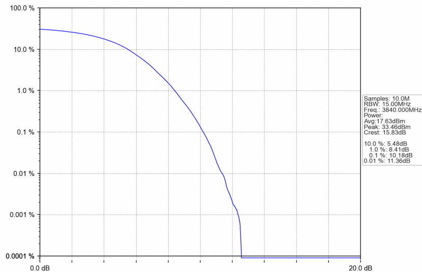
n77a_15kHz_SISO_NTNV_15MHz_DFT-s-OFDM 256 QAM_3840MHz_Outer_Full
