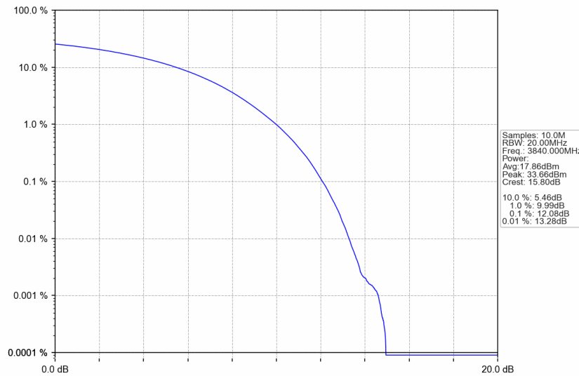
n77a_15kHz_SISO_NTNV_30MHz_CP-OFDM QPSK_3840MHz_Outer_Full
