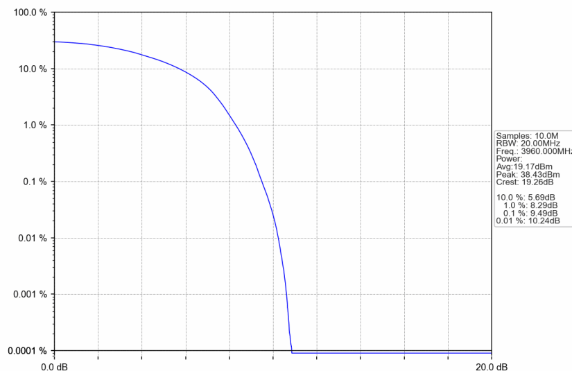
n77a_15kHz_SISO_NTNV_40MHz_DFT-s-OFDM QPSK_3960MHz_Outer_Full
