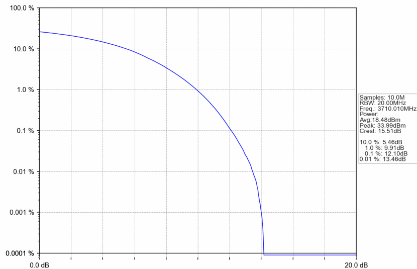
n77a_15kHz_SISO_NTNV_20MHz_CP-OFDM 64 QAM_3710.01MHz_Outer_Full
