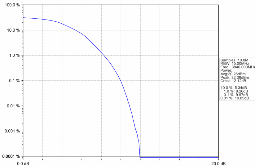
n77a_15kHz_SISO_NTNV_15MHz_DFT-s-OFDM 16 QAM_3840MHz_Outer_Full
