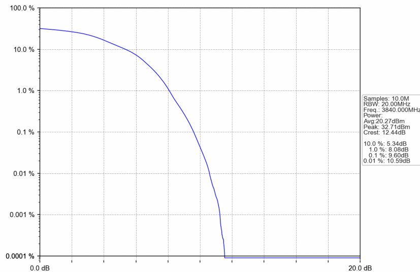
n77a_15kHz_SISO_NTNV_25MHz_DFT-s-OFDM 16 QAM_3840MHz_Outer_Full
