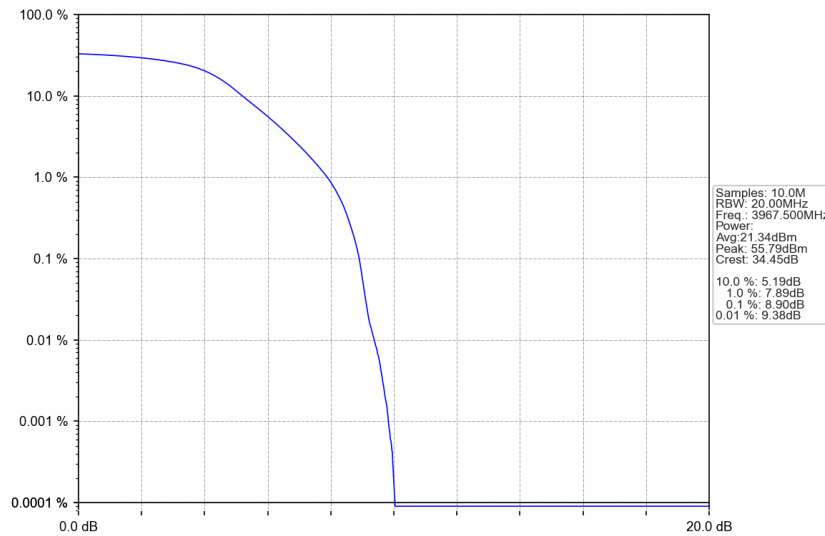
n77a_15kHz_SISO_NTNV_25MHz_DFT-s-OFDM PI/2 BPSK_3967.5MHz_Outer_Full
