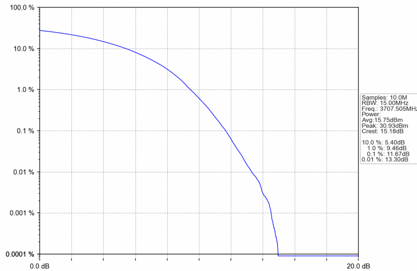
n77a_15kHz_SISO_NTNV_15MHz_CP-OFDM 256 QAM_3707.505MHz_Outer_Full
