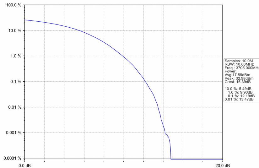
n77a_15kHz_SISO_NTNV_10MHz_CP-OFDM 64 QAM_3705MHz_Outer_Full
