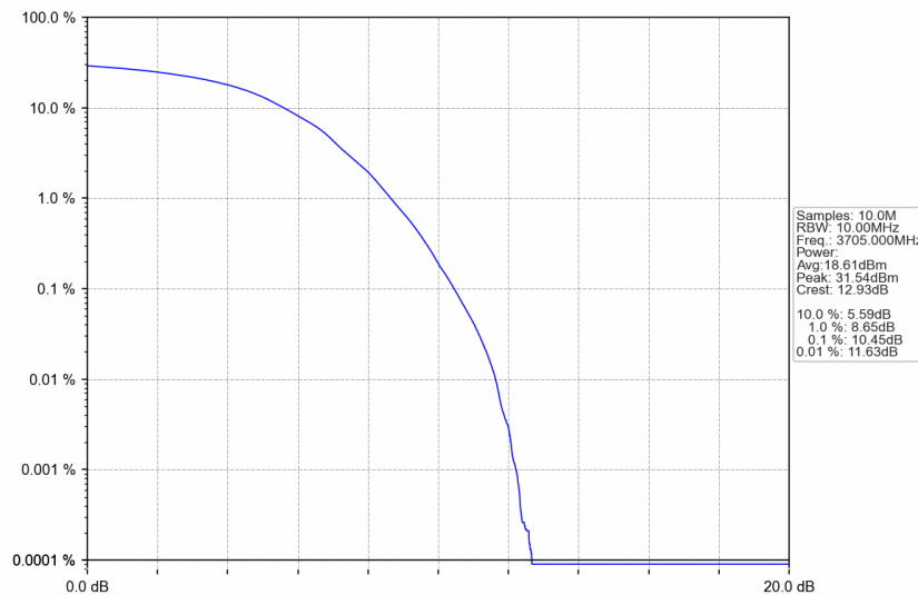
n77a_15kHz_SISO_NTNV_10MHz_DFT-s-OFDM 64 QAM_3705MHz_Outer_Full
