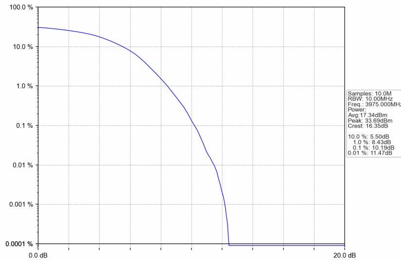
n77a_15kHz_SISO_NTNV_10MHz_DFT-s-OFDM 256 QAM_3975MHz_Outer_Full
