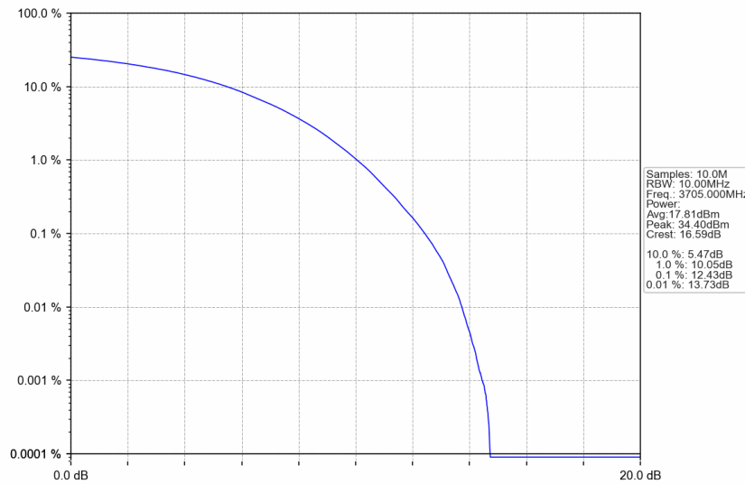
n77a_15kHz_SISO_NTNV_10MHz_CP-OFDM 16 QAM_3705MHz_Outer_Full
