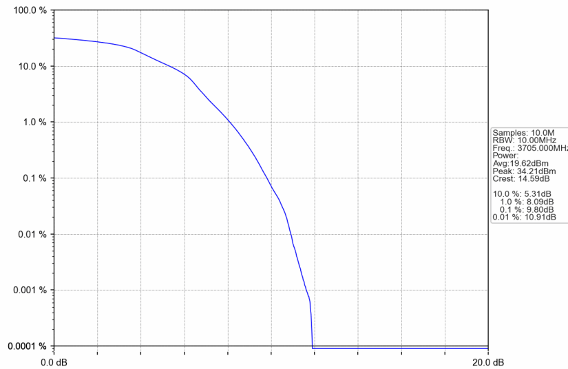
n77a_15kHz_SISO_NTNV_10MHz_DFT-s-OFDM 16 QAM_3705MHz_Outer_Full
