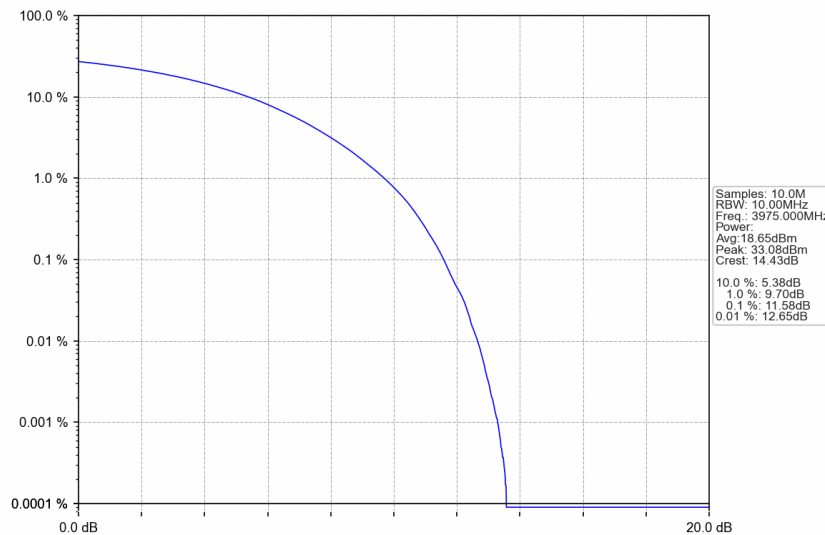
n77a_15kHz_SISO_NTNV_10MHz_CP-OFDM 64 QAM_3975MHz_Outer_Full
