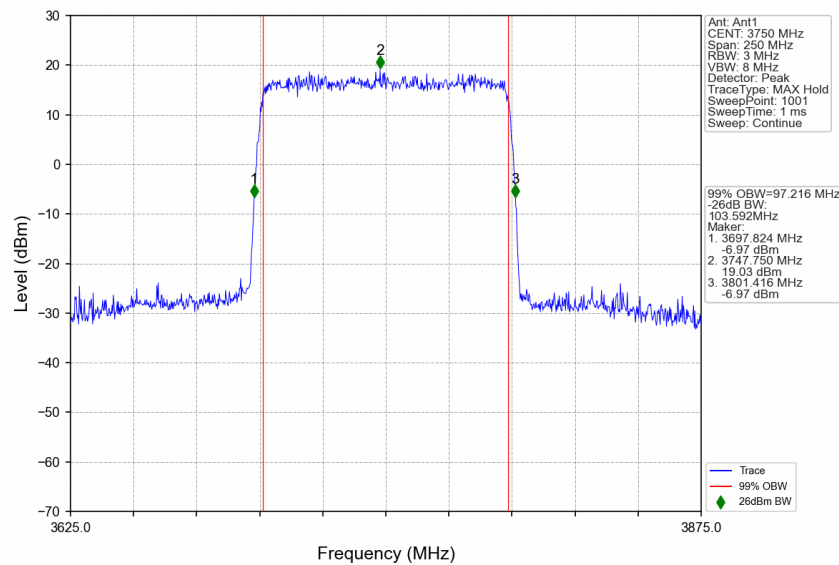
n77a_30kHz_SISO_NTNV_100MHz_DFT-s-OFDM 64 QAM_3750MHz_Outer_Full
