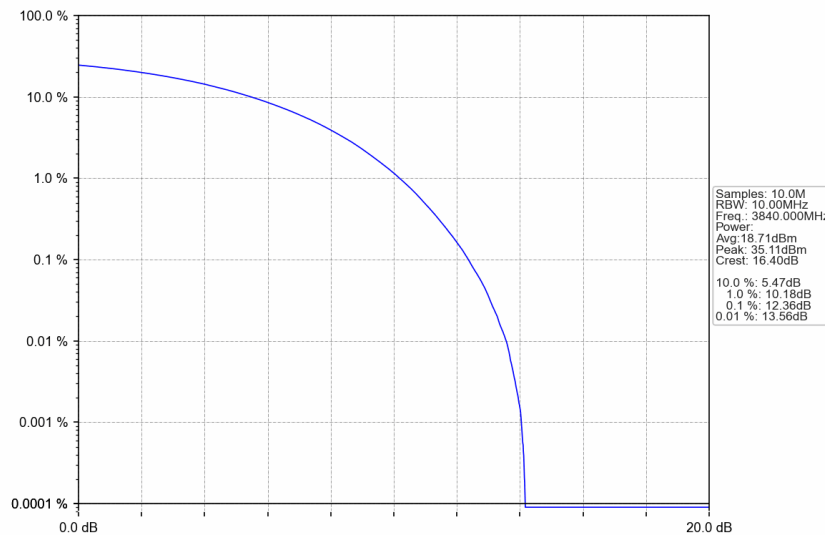
n77a_15kHz_SISO_NTNV_10MHz_CP-OFDM 16 QAM_3840MHz_Outer_Full
