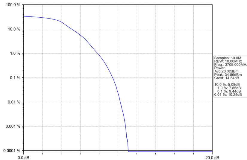
n77a_15kHz_SISO_NTNV_10MHz_DFT-s-OFDM QPSK_3705MHz_Outer_Full
