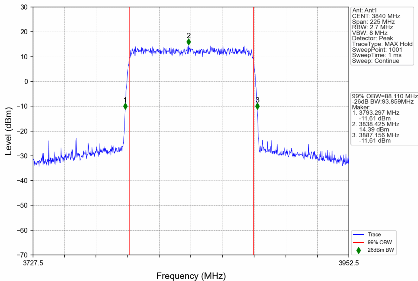
n77a_30kHz_SISO_NTNV_90MHz_CP-OFDM 256 QAM_3840MHz_Outer_Full
