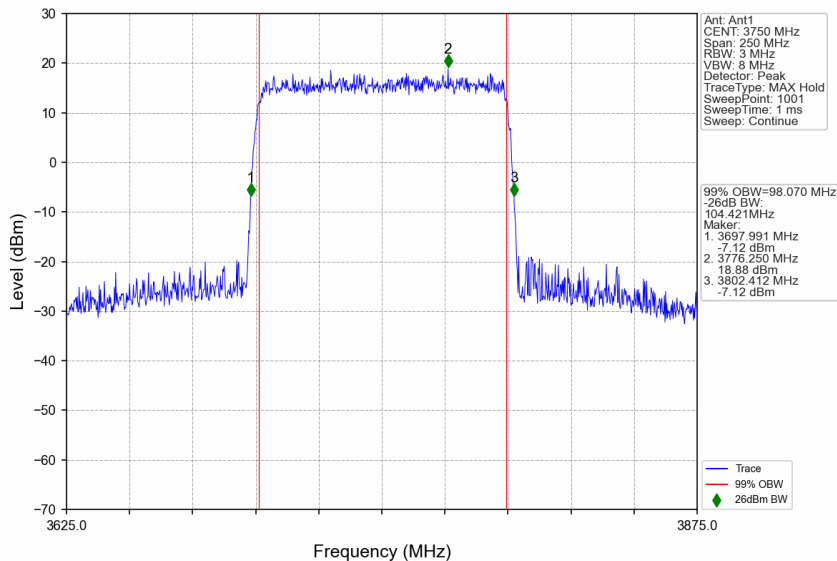
n77a_30kHz_SISO_NTNV_100MHz_CP-OFDM 64 QAM_3750MHz_Outer_Full
