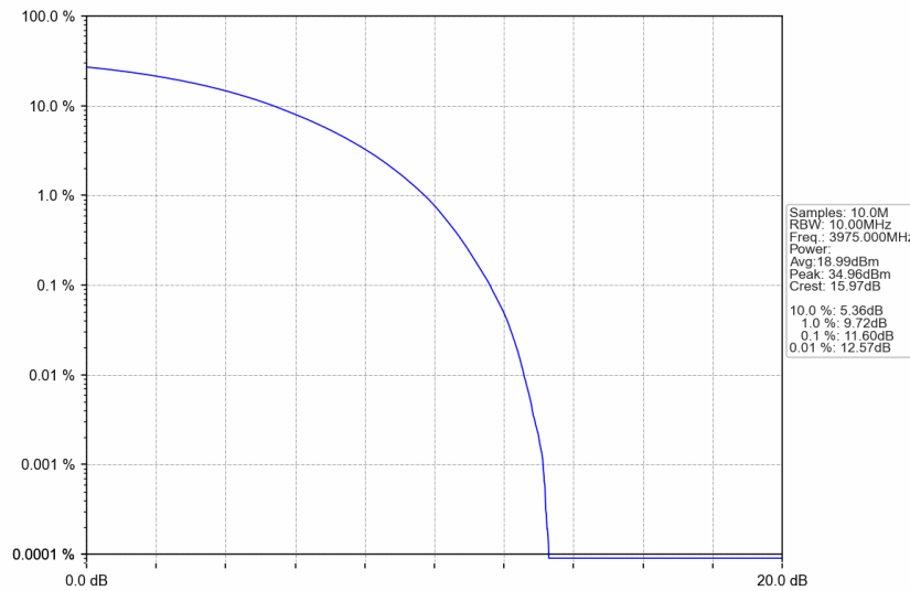
n77a_15kHz_SISO_NTNV_10MHz_CP-OFDM 16 QAM_3975MHz_Outer_Full
