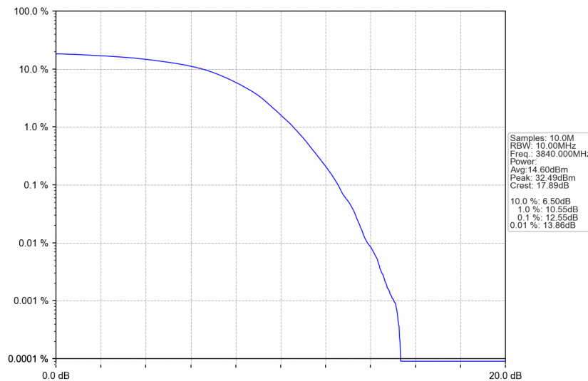
n77a_15kHz_SISO_NTNV_10MHz_DFT-s-OFDM 256 QAM_3840MHz_Outer_Full
