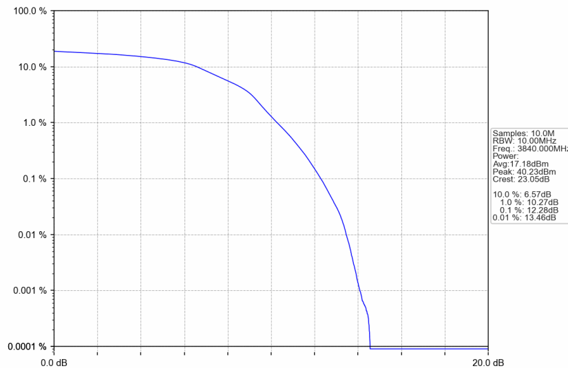
n77a_15kHz_SISO_NTNV_10MHz_DFT-s-OFDM 16 QAM_3840MHz_Outer_Full
