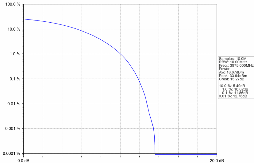
n77a_15kHz_SISO_NTNV_10MHz_CP-OFDM QPSK_3975MHz_Outer_Full
