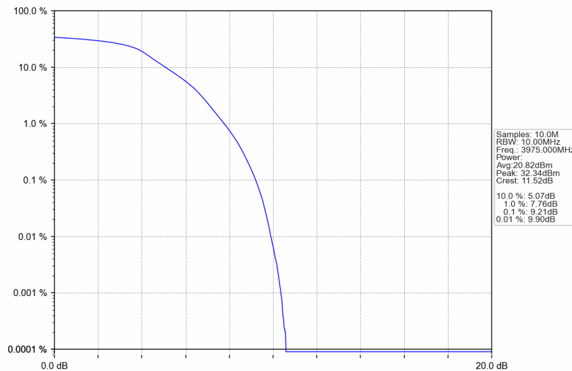
n77a_15kHz_SISO_NTNV_10MHz_DFT-s-OFDM QPSK_3975MHz_Outer_Full
