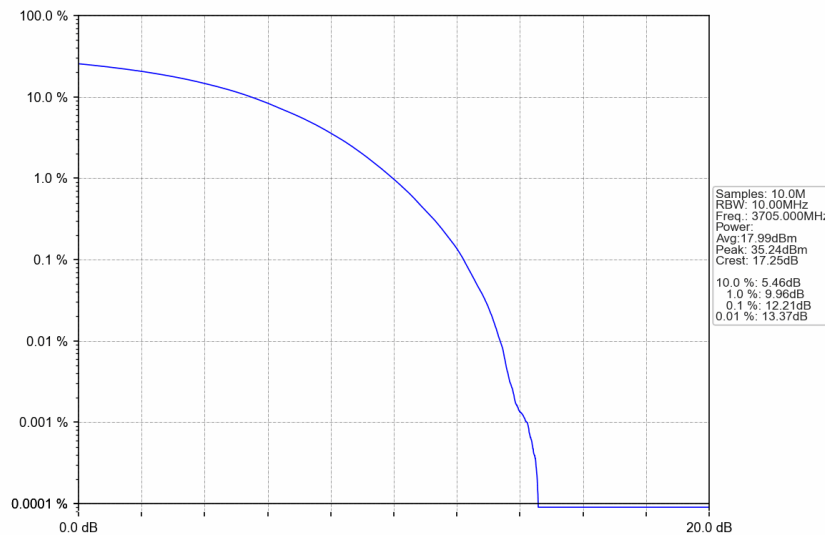
n77a_15kHz_SISO_NTNV_10MHz_CP-OFDM QPSK_3705MHz_Outer_Full
