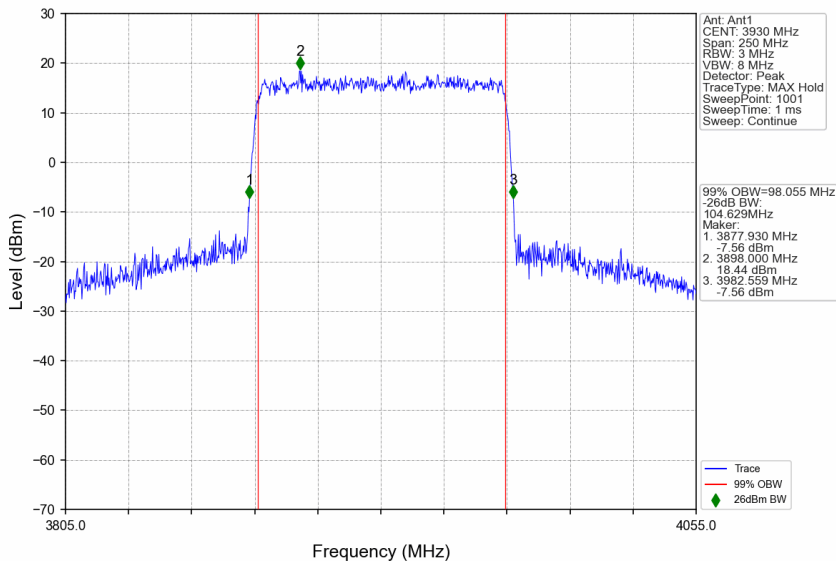
n77a_30kHz_SISO_NTNV_100MHz_CP-OFDM 64 QAM_3930MHz_Outer_Full
