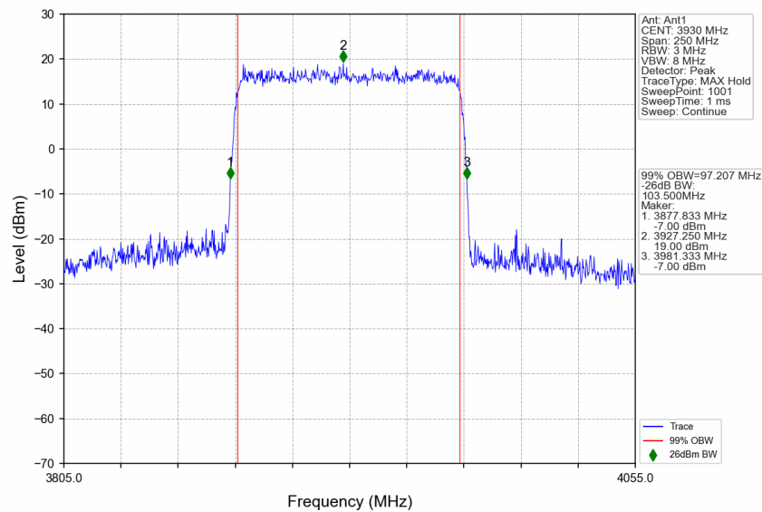
n77a_30kHz_SISO_NTNV_100MHz_DFT-s-OFDM 64 QAM_3930MHz_Outer_Full
