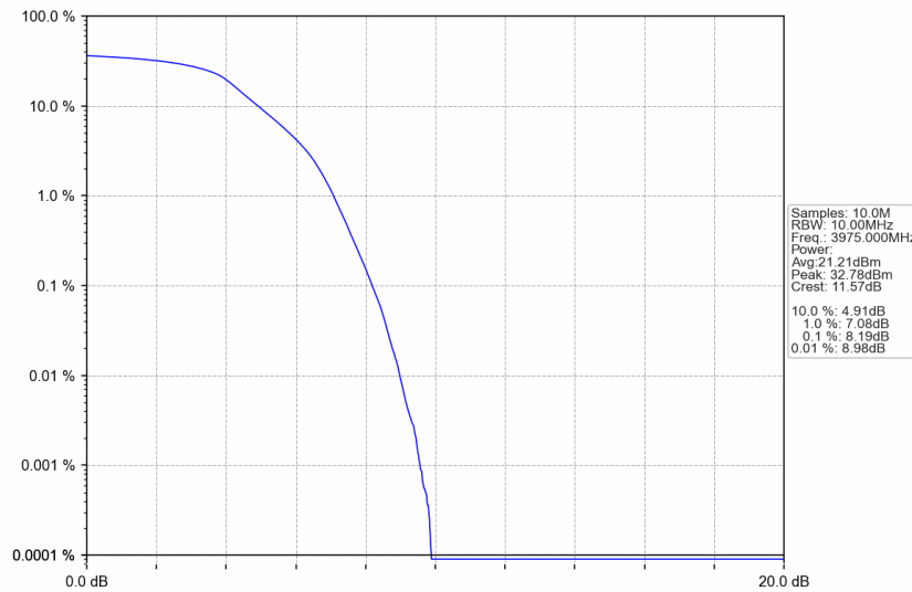
n77a_15kHz_SISO_NTNV_10MHz_DFT-s-OFDM PI/2 BPSK_3975MHz_Outer_Full
