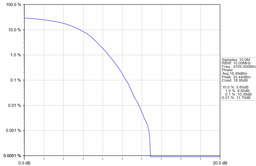
n77a_15kHz_SISO_NTNV_10MHz_DFT-s-OFDM 256 QAM_3705MHz_Outer_Full
