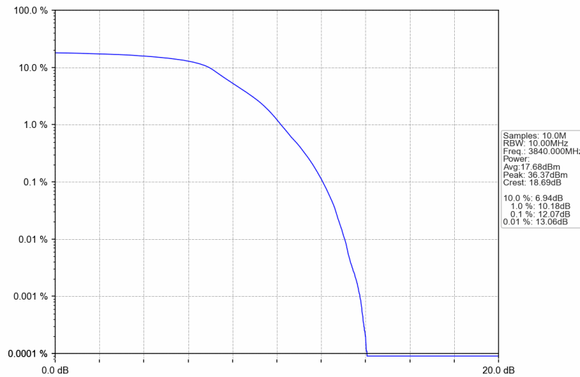
n77a_15kHz_SISO_NTNV_10MHz_DFT-s-OFDM QPSK_3840MHz_Outer_Full
