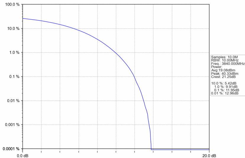
n77a_15kHz_SISO_NTNV_10MHz_CP-OFDM QPSK_3840MHz_Outer_Full
