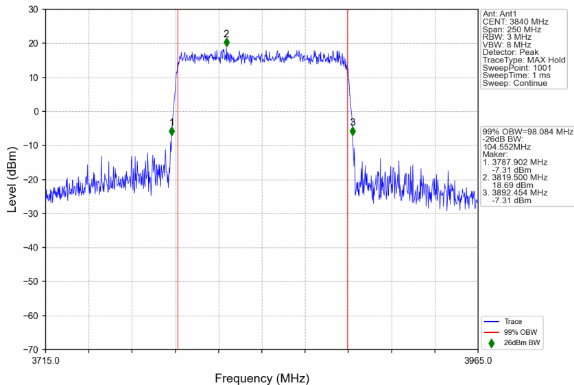
n77a_30kHz_SISO_NTNV_100MHz_CP-OFDM 16 QAM_3840MHz_Outer_Full
