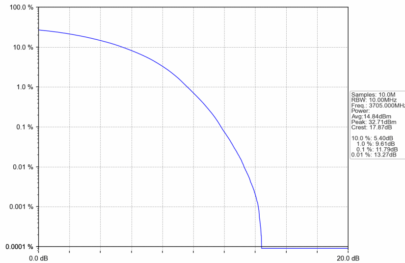
n77a_15kHz_SISO_NTNV_10MHz_CP-OFDM 256 QAM_3705MHz_Outer_Full
