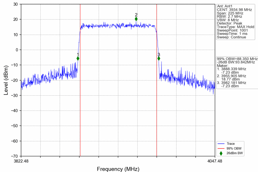
n77a_30kHz_SISO_NTNV_90MHz_CP-OFDM QPSK_3934.98MHz_Outer_Full
