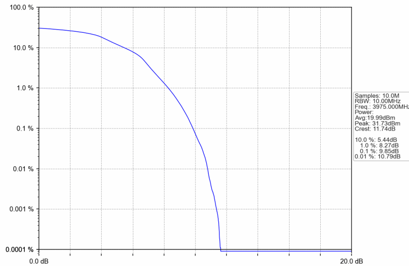
n77a_15kHz_SISO_NTNV_10MHz_DFT-s-OFDM 16 QAM_3975MHz_Outer_Full
