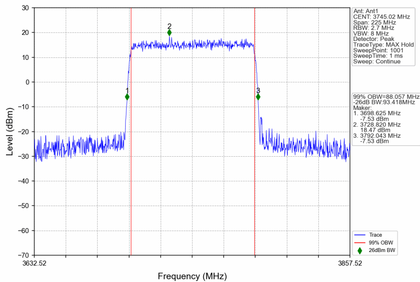
n77a_30kHz_SISO_NTNV_90MHz_CP-OFDM 64 QAM_3745.02MHz_Outer_Full
