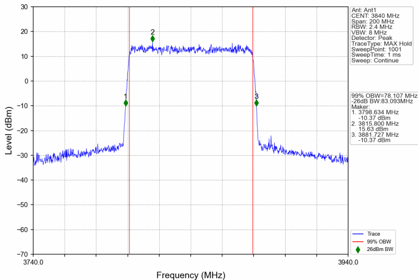
n77a_30kHz_SISO_NTNV_80MHz_CP-OFDM 256 QAM_3840MHz_Outer_Full
