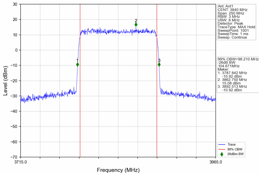
n77a_30kHz_SISO_NTNV_100MHz_CP-OFDM 256 QAM_3840MHz_Outer_Full
