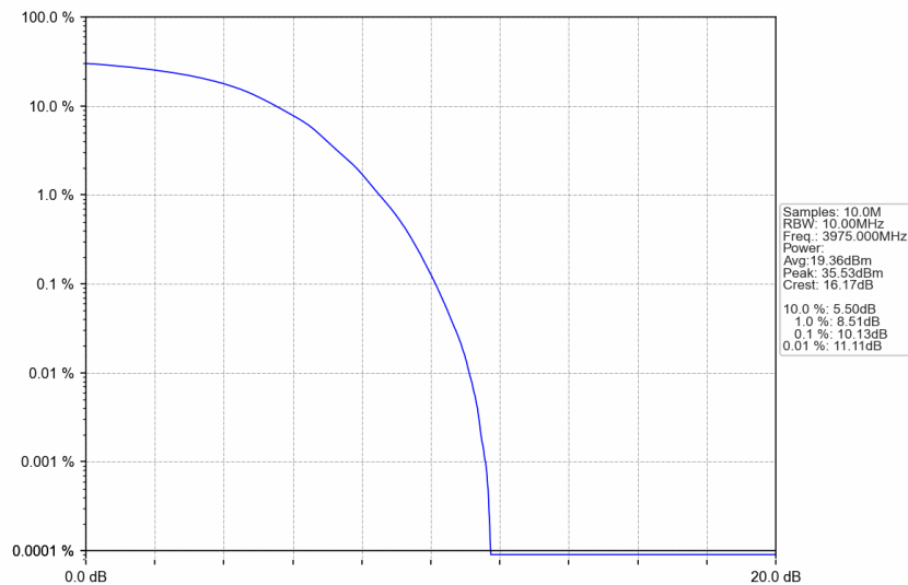
n77a_15kHz_SISO_NTNV_10MHz_DFT-s-OFDM 64 QAM_3975MHz_Outer_Full
