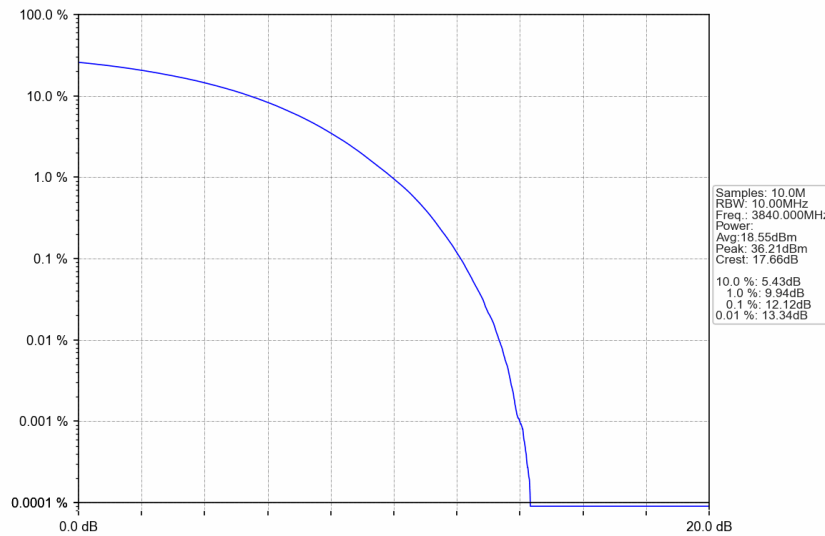
n77a_15kHz_SISO_NTNV_10MHz_CP-OFDM 64 QAM_3840MHz_Outer_Full
