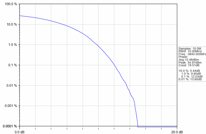
n77a_15kHz_SISO_NTNV_10MHz_CP-OFDM 256 QAM_3840MHz_Outer_Full
