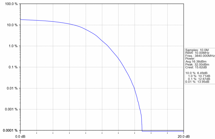
n77a_15kHz_SISO_NTNV_10MHz_DFT-s-OFDM 64 QAM_3840MHz_Outer_Full
