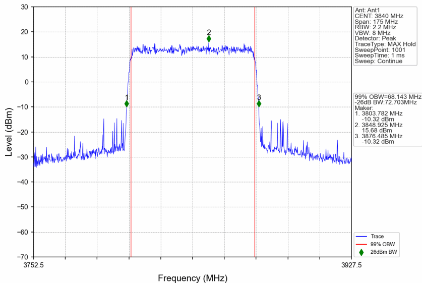
n77a_30kHz_SISO_NTNV_70MHz_CP-OFDM 256 QAM_3840MHz_Outer_Full
