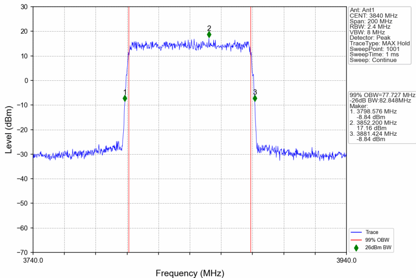
n77a_30kHz_SISO_NTNV_80MHz_DFT-s-OFDM 256 QAM_3840MHz_Outer_Full
