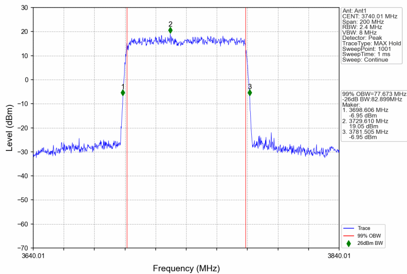
n77a_30kHz_SISO_NTNV_80MHz_DFT-s-OFDM 64 QAM_3740.01MHz_Outer_Full
