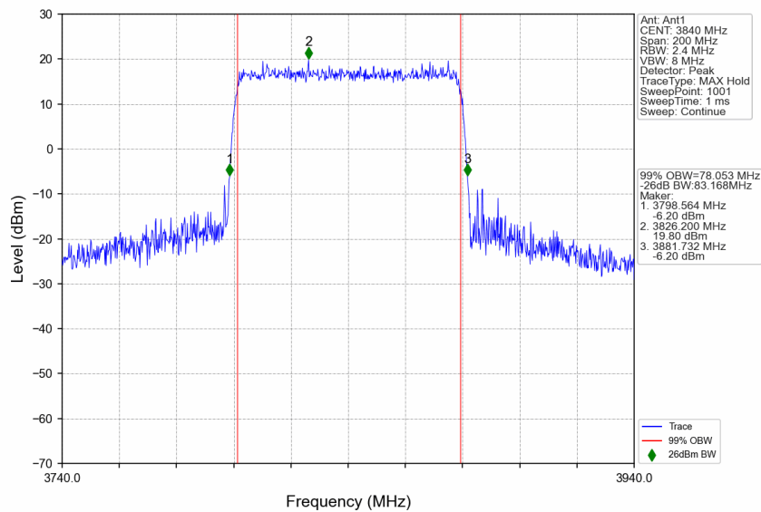
n77a_30kHz_SISO_NTNV_80MHz_CP-OFDM 16 QAM_3840MHz_Outer_Full
