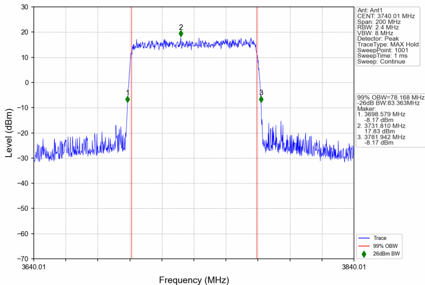
n77a_30kHz_SISO_NTNV_80MHz_CP-OFDM 64 QAM_3740.01MHz_Outer_Full
