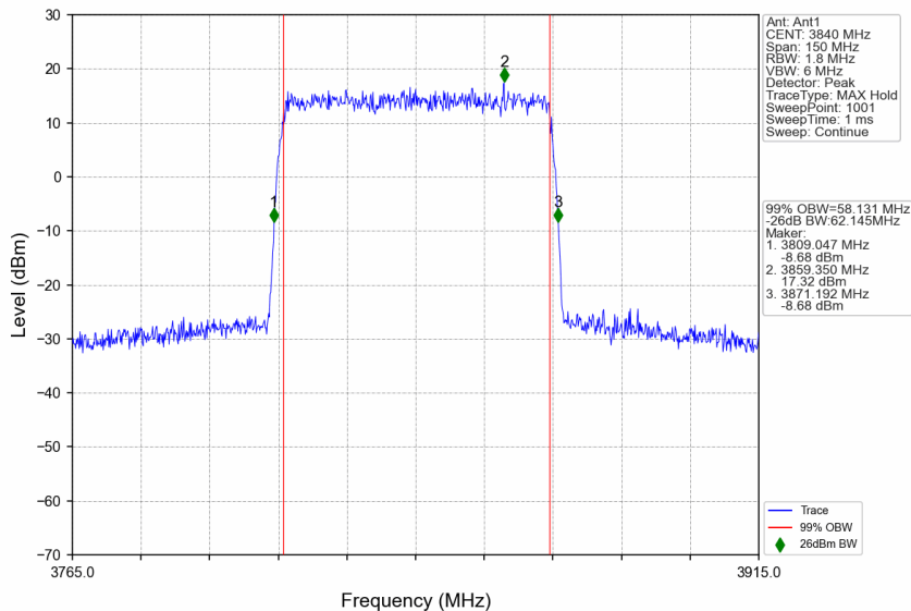
n77a_30kHz_SISO_NTNV_60MHz_DFT-s-OFDM 256 QAM_3840MHz_Outer_Full
