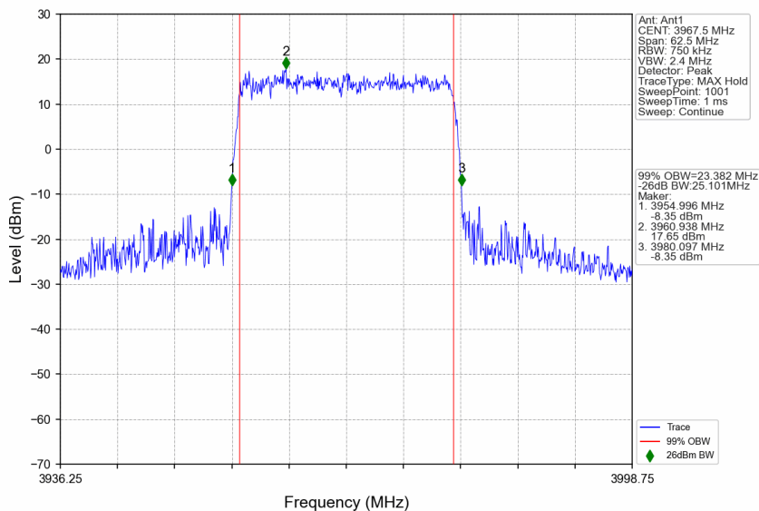
n77a_30kHz_SISO_NTNV_25MHz_CP-OFDM 64 QAM_3967.5MHz_Outer_Full
