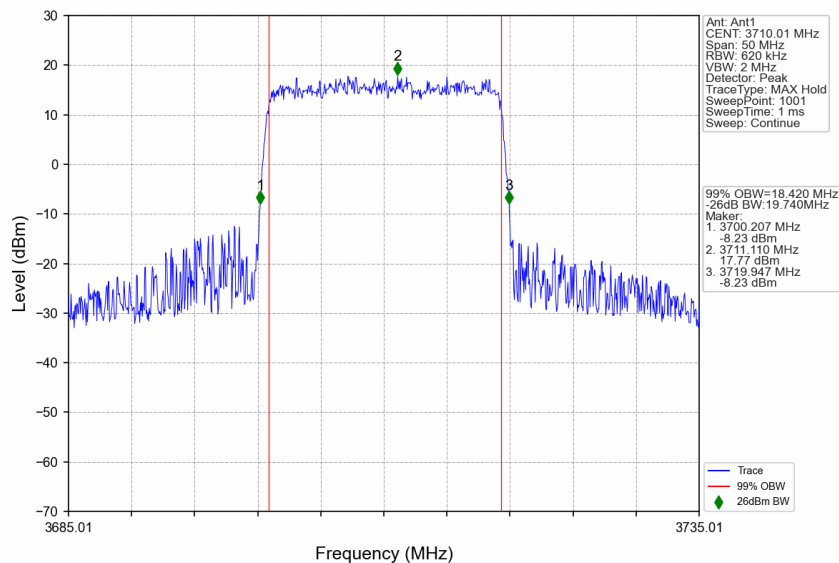
n77a_30kHz_SISO_NTNV_20MHz_CP-OFDM QPSK_3710.01MHz_Outer_Full
