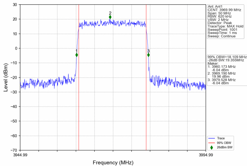
n77a_30kHz_SISO_NTNV_20MHz_DFT-s-OFDM QPSK_3969.99MHz_Outer_Full
