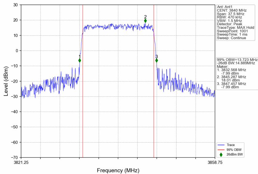
n77a_30kHz_SISO_NTNV_15MHz_CP-OFDM 16 QAM_3840MHz_Outer_Full
