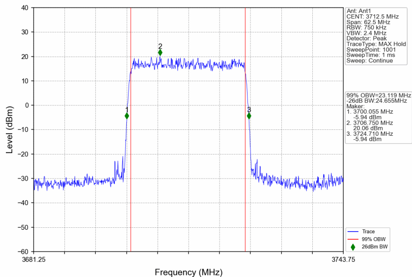
n77a_30kHz_SISO_NTNV_25MHz_DFT-s-OFDM QPSK_3712.5MHz_Outer_Full
