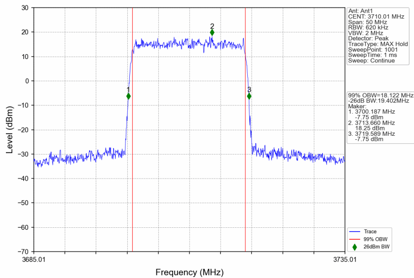
n77a_30kHz_SISO_NTNV_20MHz_DFT-s-OFDM 64 QAM_3710.01MHz_Outer_Full
