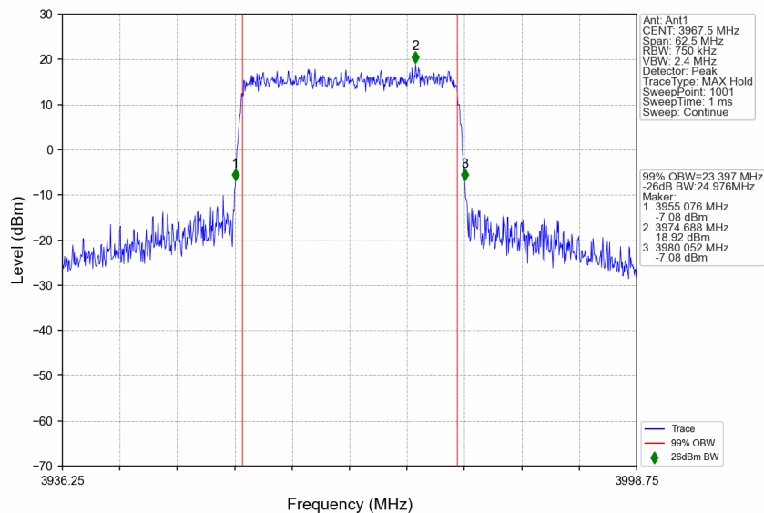
n77a_30kHz_SISO_NTNV_25MHz_CP-OFDM QPSK_3967.5MHz_Outer_Full
