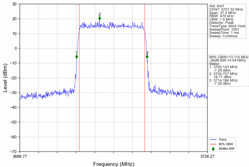
n77a_30kHz_SISO_NTNV_15MHz_DFT-s-OFDM 64 QAM_3707.52MHz_Outer_Full
