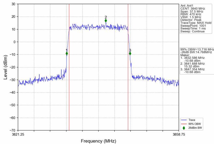
n77a_30kHz_SISO_NTNV_15MHz_CP-OFDM 256 QAM_3840MHz_Outer_Full
