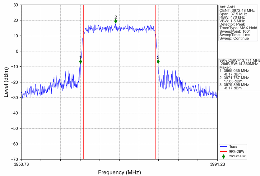
n77a_30kHz_SISO_NTNV_15MHz_CP-OFDM 64 QAM_3972.48MHz_Outer_Full
