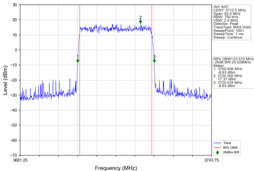
n77a_30kHz_SISO_NTNV_25MHz_CP-OFDM 64 QAM_3712.5MHz_Outer_Full
