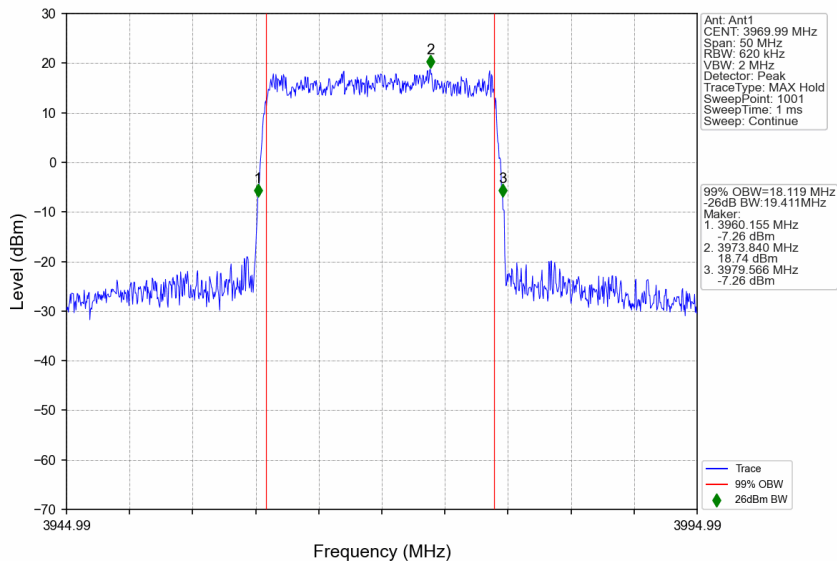
n77a_30kHz_SISO_NTNV_20MHz_DFT-s-OFDM_64_QAM_3969.99MHz_Outer_Full
