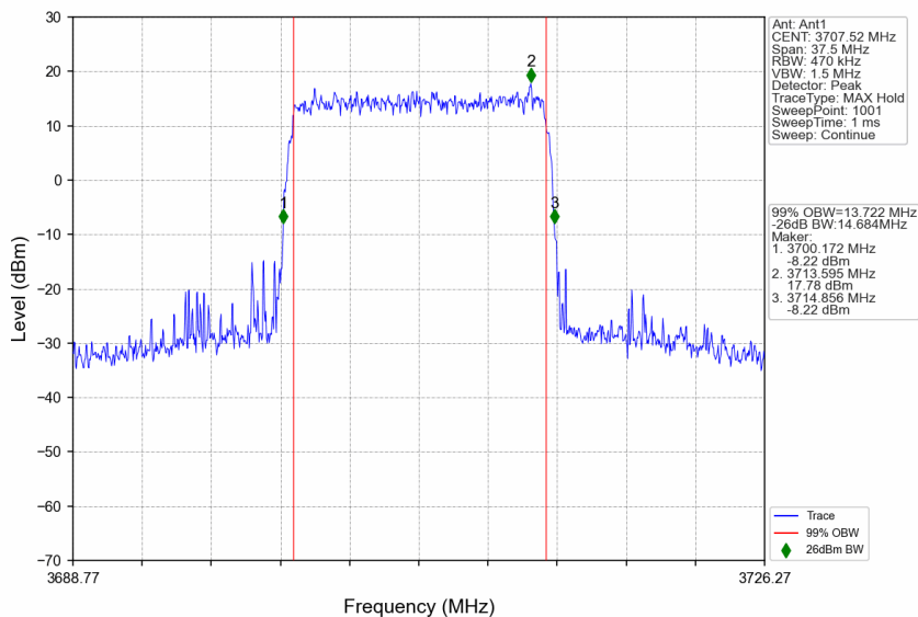
n77a_30kHz_SISO_NTNV_15MHz_CP-OFDM 64 QAM_3707.52MHz_Outer_Full
