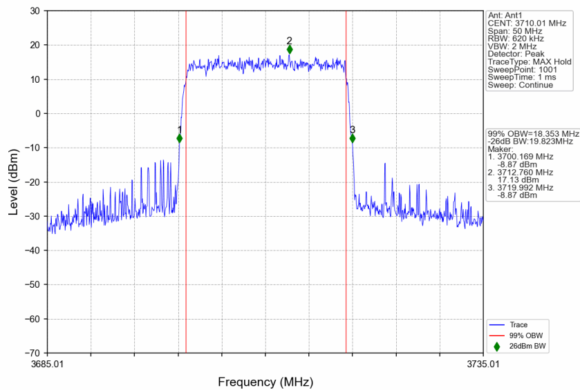
n77a_30kHz_SISO_NTNV_20MHz_CP-OFDM 64 QAM_3710.01MHz_Outer_Full
