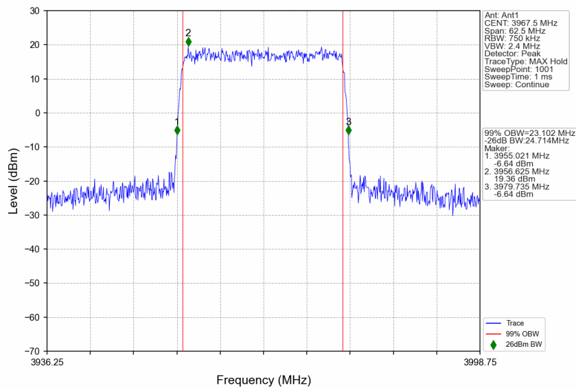
n77a_30kHz_SISO_NTNV_25MHz_DFT-s-OFDM QPSK_3967.5MHz_Outer_Full
