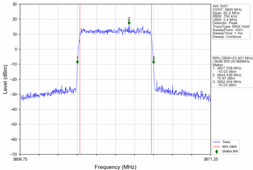
n77a_30kHz_SISO_NTNV_25MHz_CP-OFDM 256 QAM_3840MHz_Outer_Full
