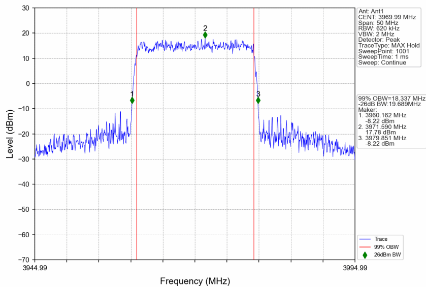
n77a_30kHz_SISO_NTNV_20MHz_CP-OFDM 64 QAM_3969.99MHz_Outer_Full
