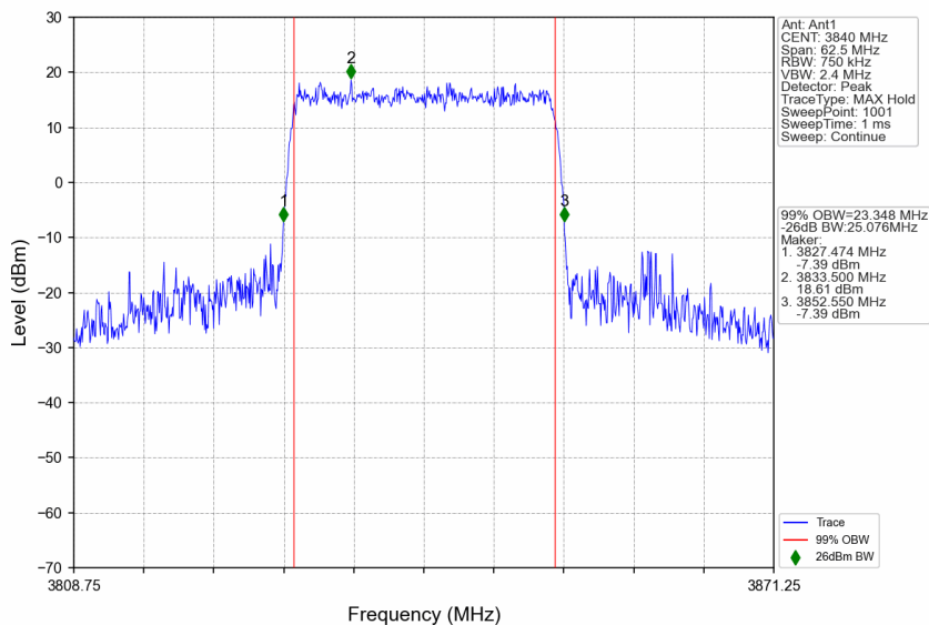
n77a_30kHz_SISO_NTNV_25MHz_CP-OFDM 16 QAM_3840MHz_Outer_Full
