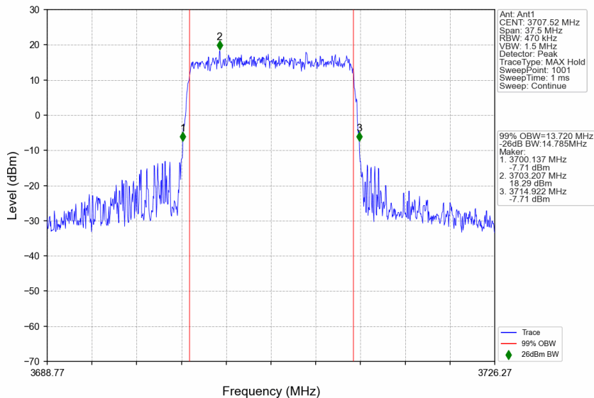
n77a_30kHz_SISO_NTNV_15MHz_CP-OFDM QPSK_3707.52MHz_Outer_Full
