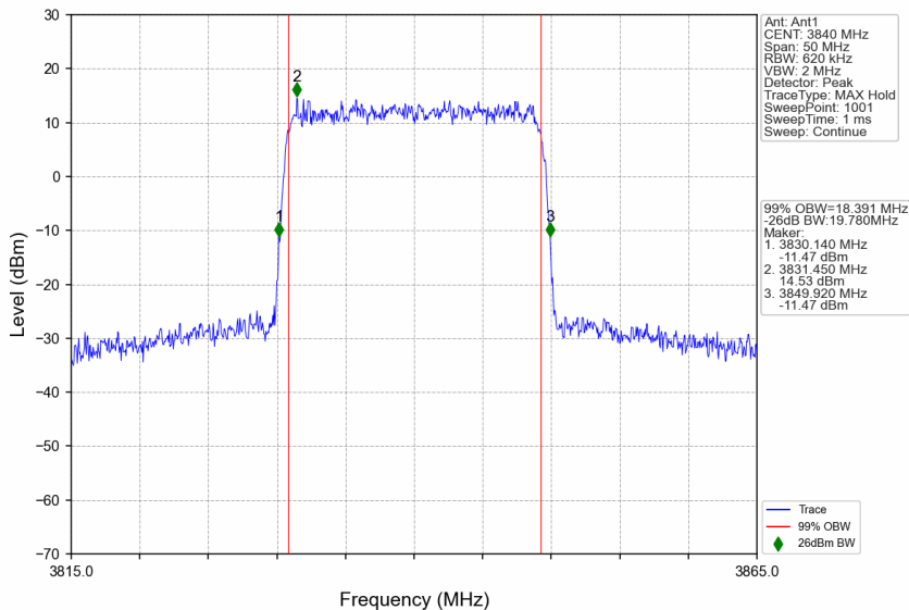
n77a_30kHz_SISO_NTNV_20MHz_CP-OFDM 256 QAM_3840MHz_Outer_Full
