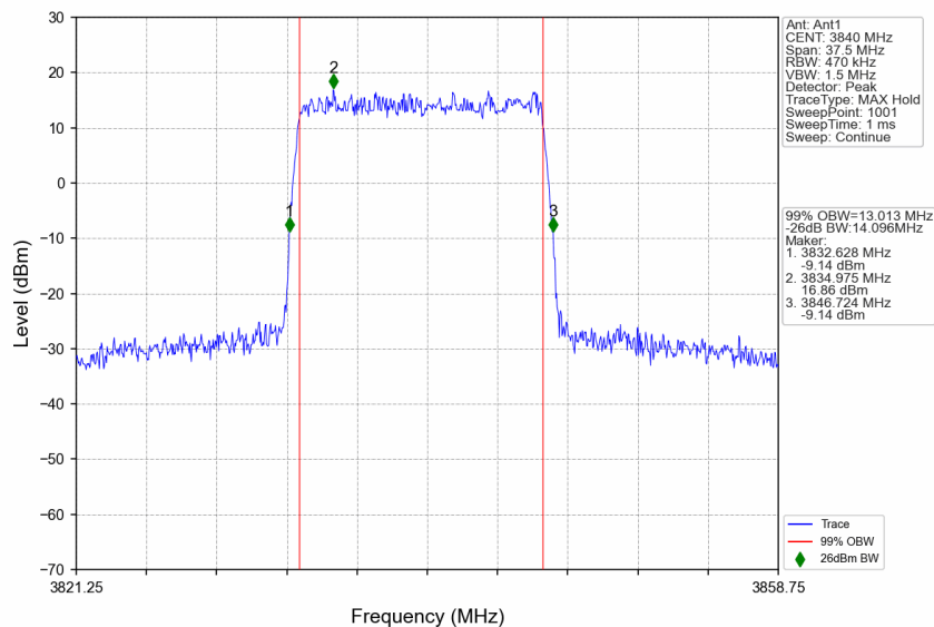
n77a_30kHz_SISO_NTNV_15MHz_DFT-s-OFDM 256 QAM_3840MHz_Outer_Full
