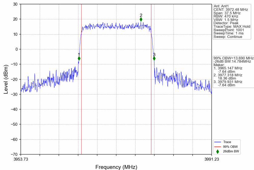
n77a_30kHz_SISO_NTNV_15MHz_CP-OFDM QPSK_3972.48MHz_Outer_Full
