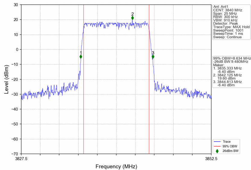
n77a_30kHz_SISO_NTNV_10MHz_DFT-s-OFDM 16 QAM_3840MHz_Outer_Full
