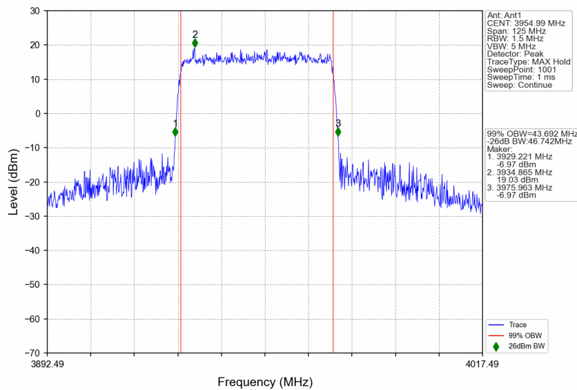
n77a_15kHz_SISO_NTNV_50MHz_CP-OFDM 64 QAM_3954.99MHz_Outer_Full
