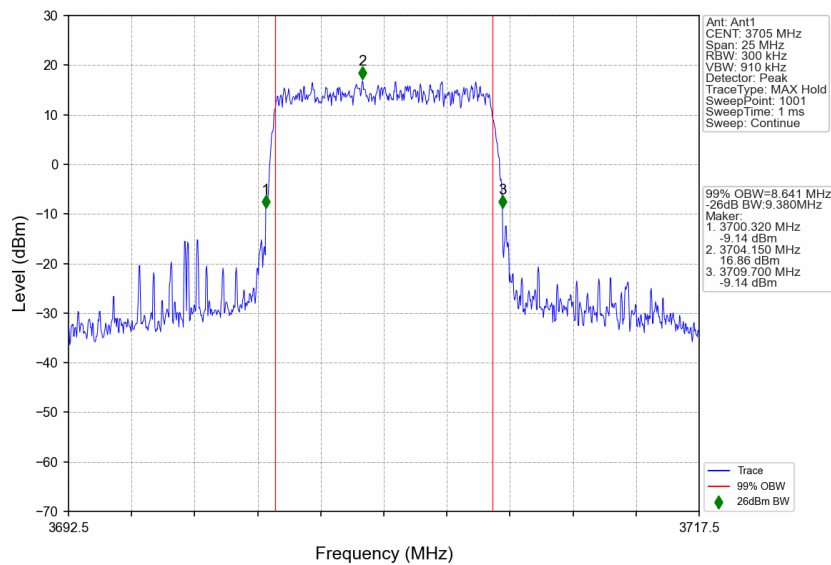
n77a_30kHz_SISO_NTNV_10MHz_CP-OFDM 64 QAM_3705MHz_Outer_Full
