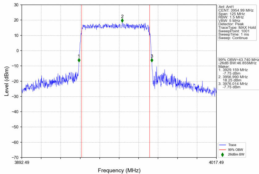
n77a_15kHz_SISO_NTNV_50MHz_CP-OFDM QPSK_3954.99MHz_Outer_Full
