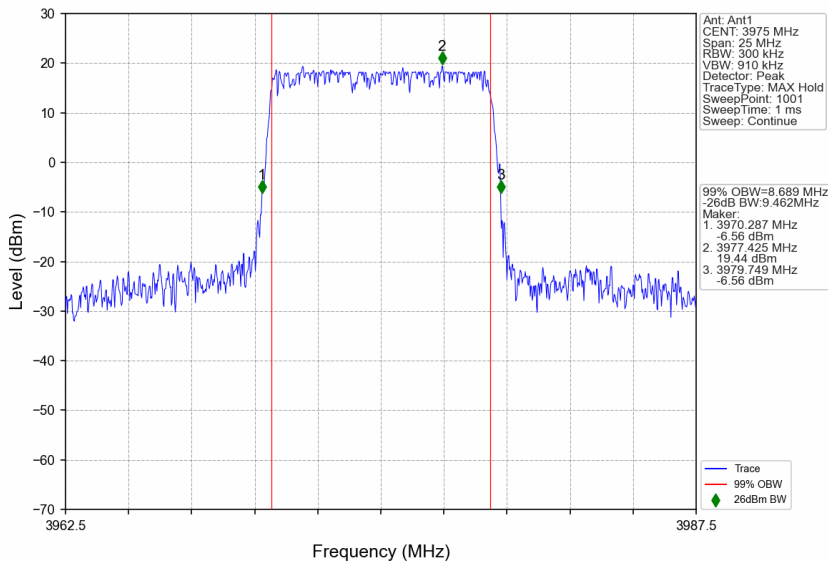
n77a_30kHz_SISO_NTNV_10MHz_DFT-s-OFDM QPSK_3975MHz_Outer_Full
