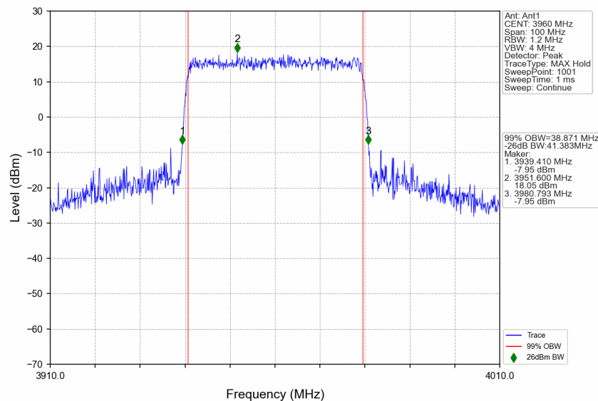
n77a_15kHz_SISO_NTNV_40MHz_CP-OFDM QPSK_3960MHz_Outer_Full
