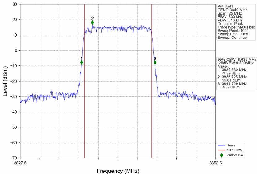
n77a_30kHz_SISO_NTNV_10MHz_DFT-s-OFDM 256 QAM_3840MHz_Outer_Full
