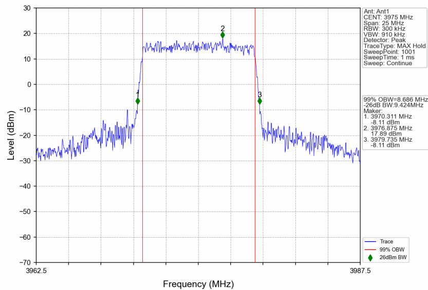
n77a_30kHz_SISO_NTNV_10MHz_CP-OFDM QPSK_3975MHz_Outer_Full
