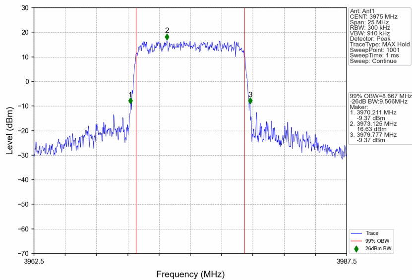
n77a_30kHz_SISO_NTNV_10MHz_CP-OFDM 64 QAM_3975MHz_Outer_Full
