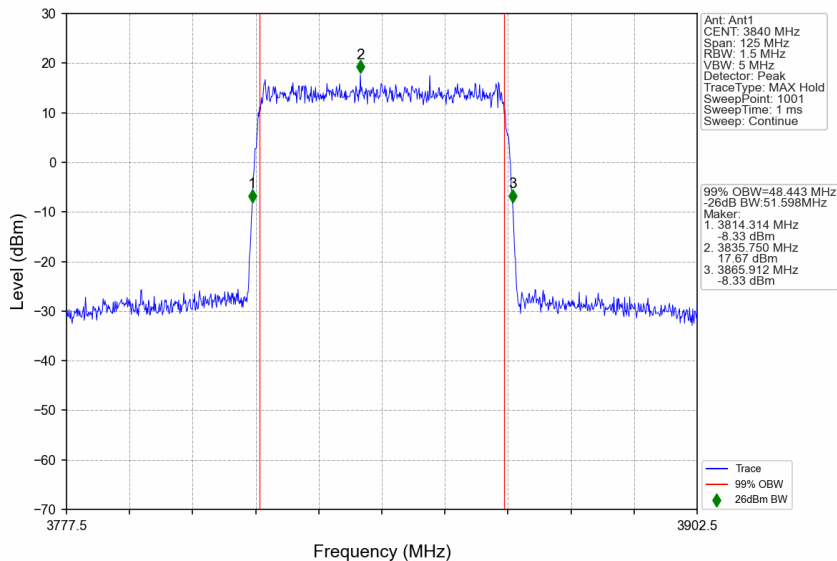
n77a_15kHz_SISO_NTNV_50MHz_DFT-s-OFDM 256 QAM_3840MHz_Outer_Full
