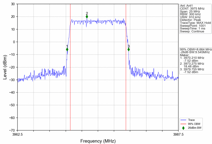
n77a_30kHz_SISO_NTNV_10MHz_DFT-s-OFDM 64 QAM_3975MHz_Outer_Full
