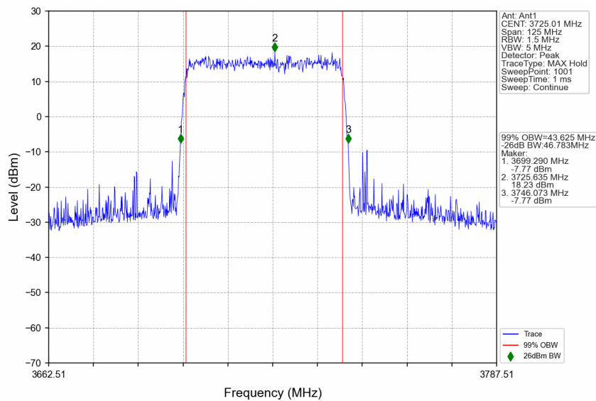
n77a_15kHz_SISO_NTNV_50MHz_CP-OFDM 64 QAM_3725.01MHz_Outer_Full
