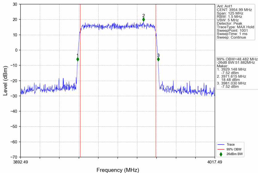
n77a_15kHz_SISO_NTNV_50MHz_DFT-s-OFDM 64 QAM_3954.99MHz_Outer_Full
