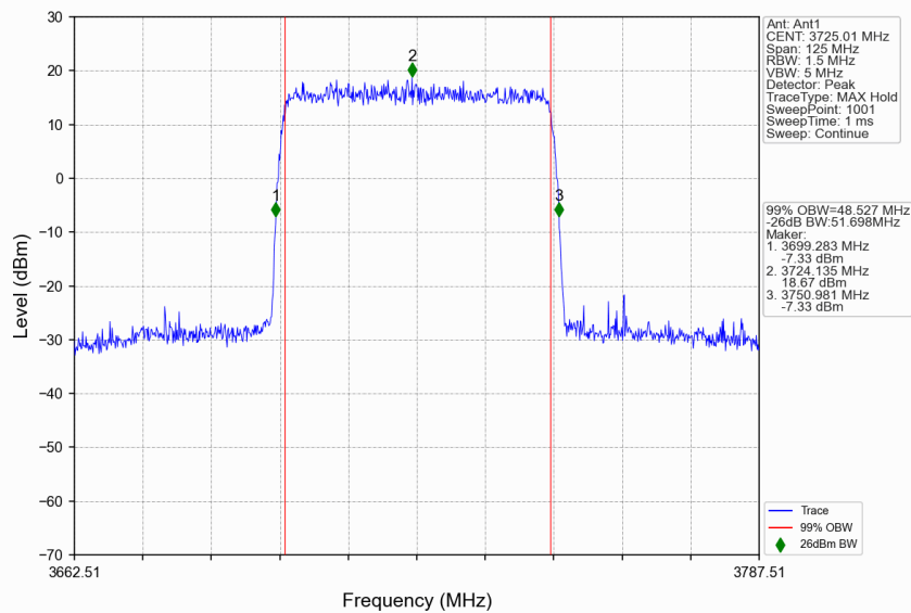
n77a_15kHz_SISO_NTNV_50MHz_DFT-s-OFDM 64 QAM_3725.01MHz_Outer_Full
