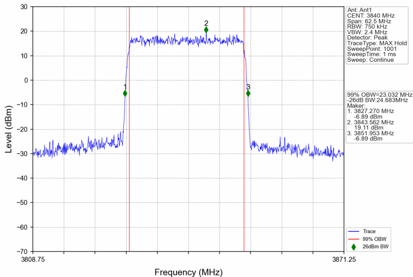
n77a_15kHz_SISO_NTNV_25MHz_DFT-s-OFDM 16 QAM_3840MHz_Outer_Full
