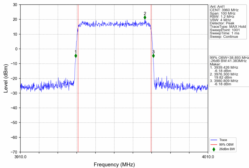
n77a_15kHz_SISO_NTNV_40MHz_DFT-s-OFDM QPSK_3960MHz_Outer_Full
