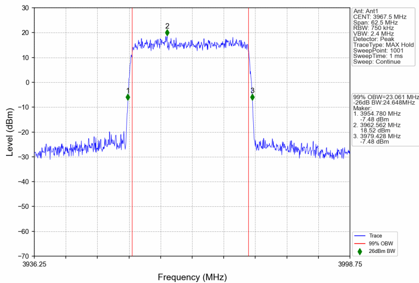
n77a_15kHz_SISO_NTNV_25MHz_DFT-s-OFDM 64 QAM_3967.5MHz_Outer_Full
