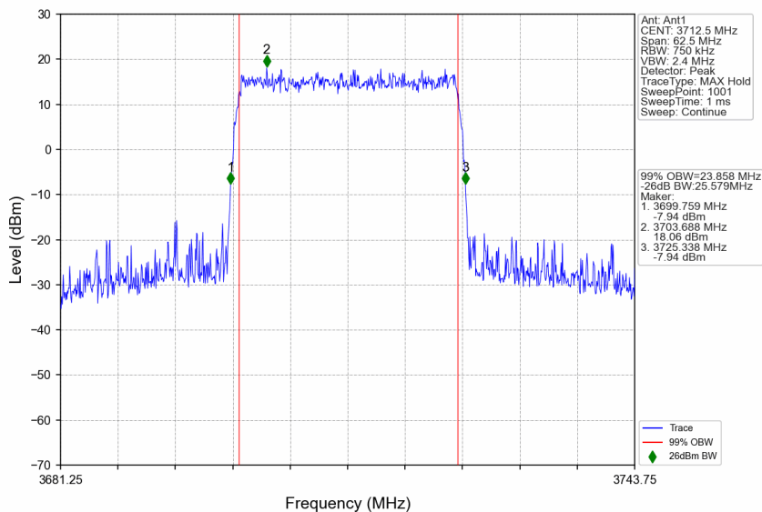
n77a_15kHz_SISO_NTNV_25MHz_CP-OFDM QPSK_3712.5MHz_Outer_Full
