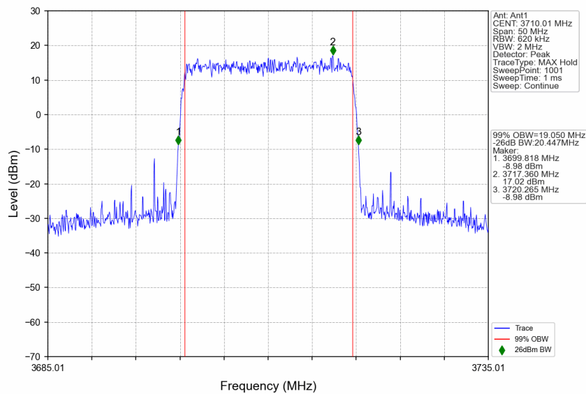
n77a_15kHz_SISO_NTNV_20MHz_CP-OFDM 64 QAM_3710.01MHz_Outer_Full
