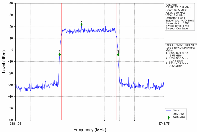
n77a_15kHz_SISO_NTNV_25MHz_DFT-s-OFDM QPSK_3712.5MHz_Outer_Full
