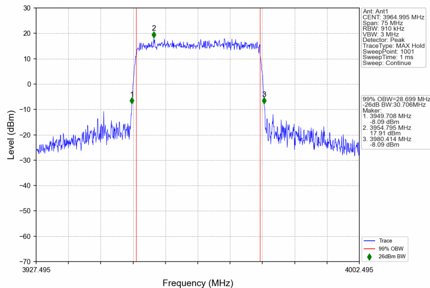
n77a_15kHz_SISO_NTNV_30MHz_CP-OFDM QPSK_3964.995MHz_Outer_Full
