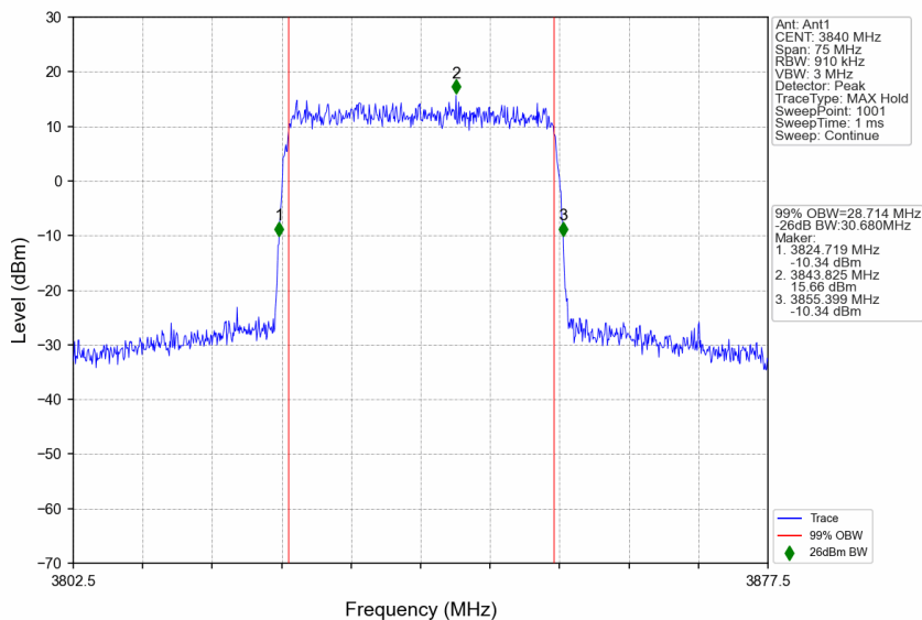
n77a_15kHz_SISO_NTNV_30MHz_CP-OFDM 256 QAM_3840MHz_Outer_Full
