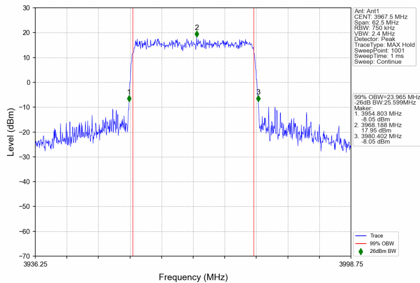
n77a_15kHz_SISO_NTNV_25MHz_CP-OFDM QPSK_3967.5MHz_Outer_Full
