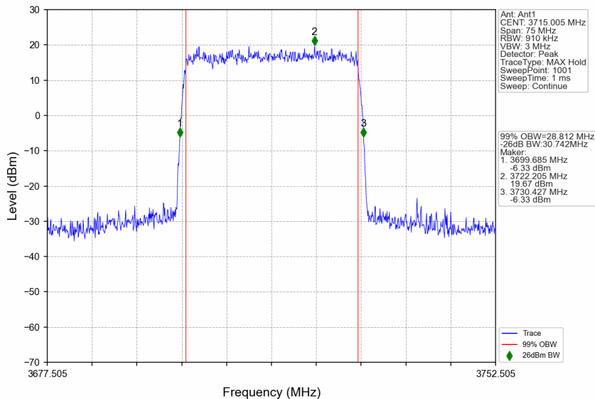
n77a_15kHz_SISO_NTNV_30MHz_DFT-s-OFDM QPSK_3715.005MHz_Outer_Full
