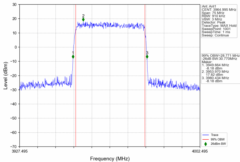
n77a_15kHz_SISO_NTNV_30MHz_DFT-s-OFDM 64 QAM_3964.995MHz_Outer_Full
