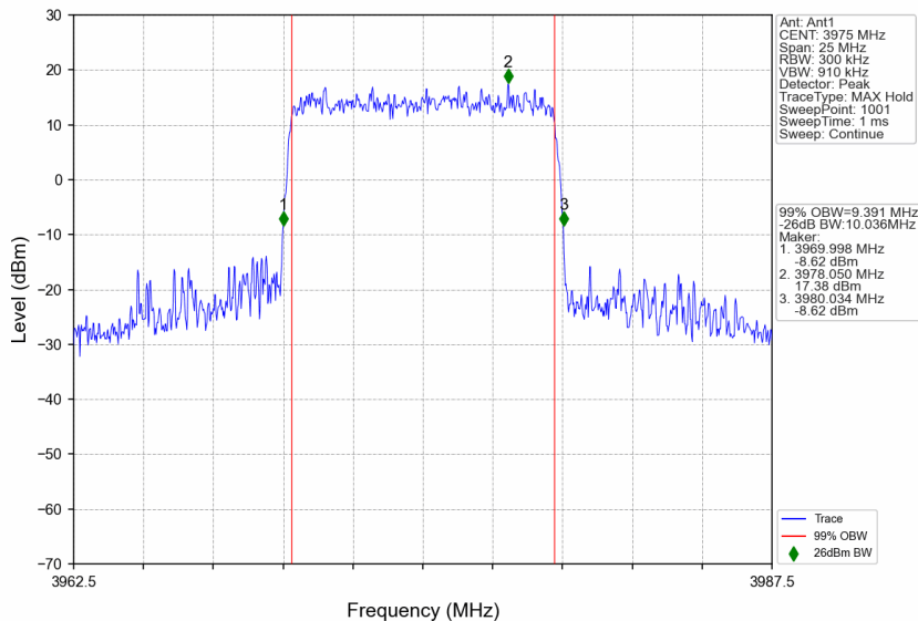
n77a_15kHz_SISO_NTNV_10MHz_CP-OFDM 64 QAM_3975MHz_Outer_Full
