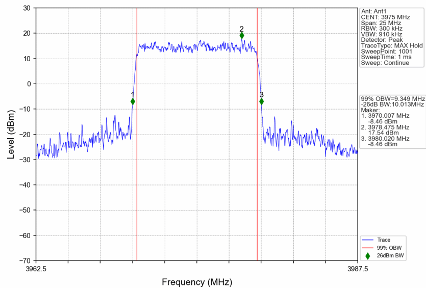
n77a_15kHz_SISO_NTNV_10MHz_CP-OFDM QPSK_3975MHz_Outer_Full
