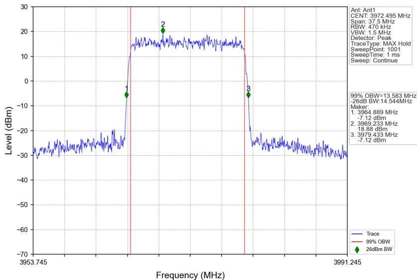
n77a_15kHz_SISO_NTNV_15MHz_DFT-s-OFDM 64 QAM_3972.495MHz_Outer_Full
