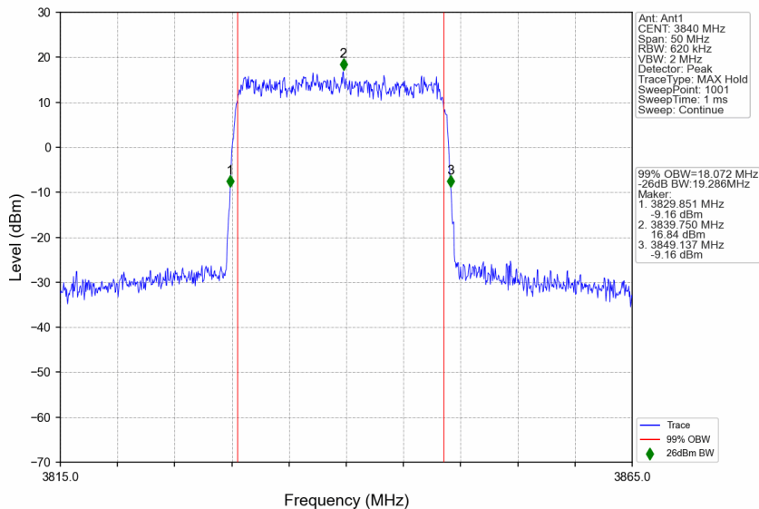
n77a_15kHz_SISO_NTNV_20MHz_DFT-s-OFDM 256 QAM_3840MHz_Outer_Full
