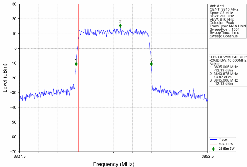
n77a_15kHz_SISO_NTNV_10MHz_CP-OFDM 256 QAM_3840MHz_Outer_Full
