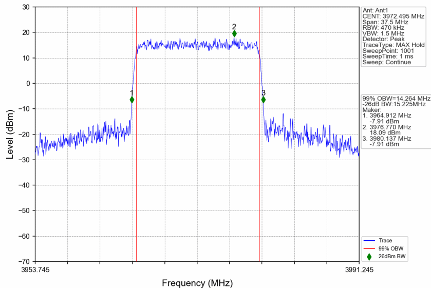
n77a_15kHz_SISO_NTNV_15MHz_CP-OFDM QPSK_3972.495MHz_Outer_Full
