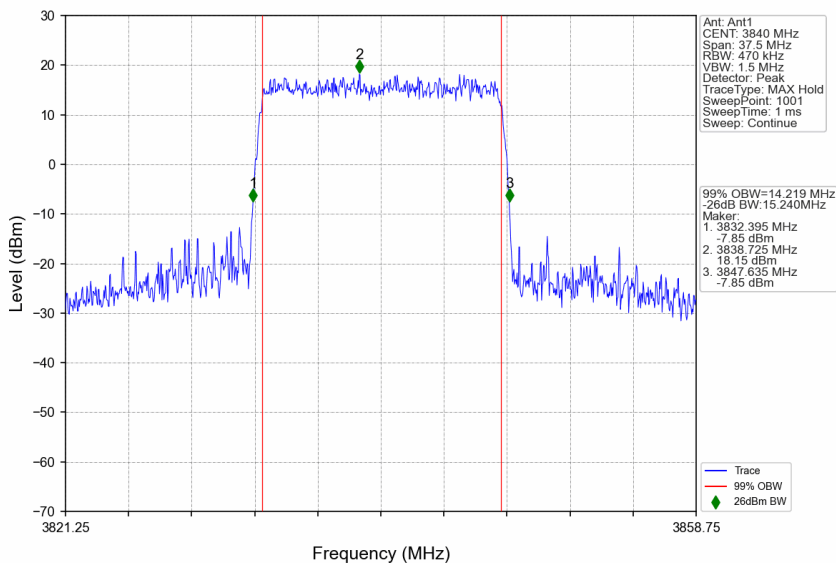
n77a_15kHz_SISO_NTNV_15MHz_CP-OFDM 16 QAM_3840MHz_Outer_Full
