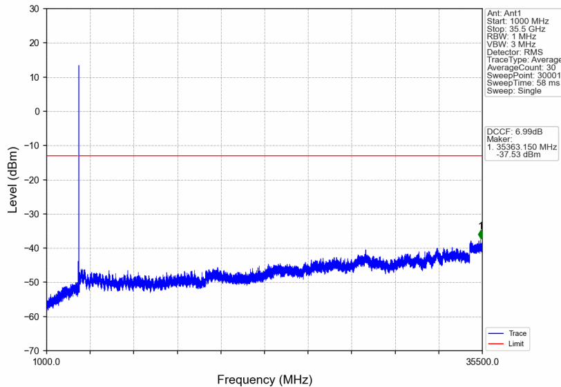
n77d_30kHz_SISO_NTNV_100MHz_CP-OFDM QPSK_3499.98MHz_Edge_1RB_Right
