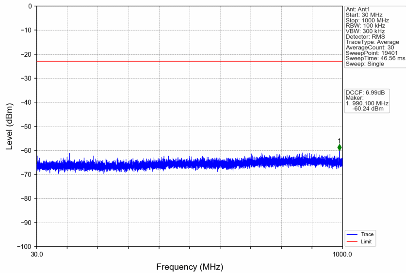
n77d_30kHz_SISO_NTNV_100MHz_CP-OFDM QPSK_3499.98MHz_Edge_1RB_Right
