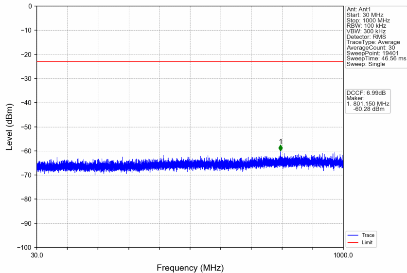
n77d_30kHz_SISO_NTNV_100MHz_CP-OFDM QPSK_3500.01MHz_Edge_1RB_Left
