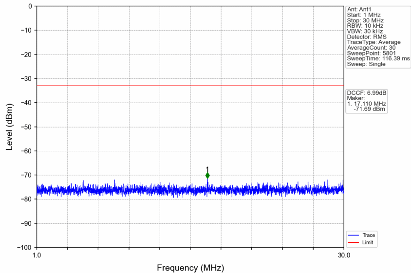
n77d_30kHz_SISO_NTNV_100MHz_CP-OFDM QPSK_3499.98MHz_Edge_1RB_Right
