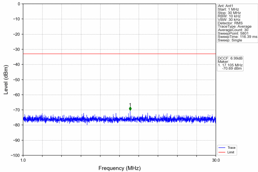
n77d_30kHz_SISO_NTNV_90MHz_DFT-s-OFDM_QPSK_3500.01MHz_Edge_1RB_Left
