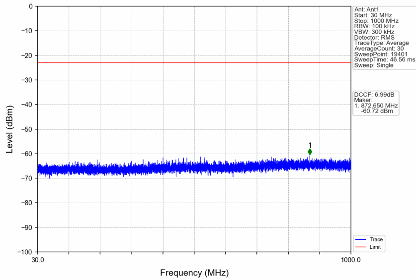
n77d_30kHz_SISO_NTNV_100MHz_DFT-s-OFDM QPSK_3499.98MHz_Edge_1RB_Right
