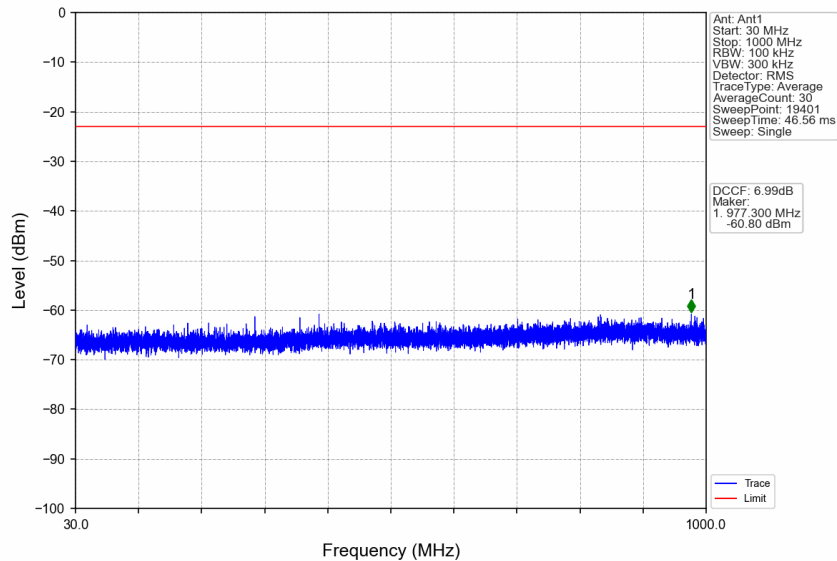
n77d_30kHz_SISO_NTNV_90MHz_DFT-s-OFDM_QPSK_3500.01MHz_Edge_1RB_Left
