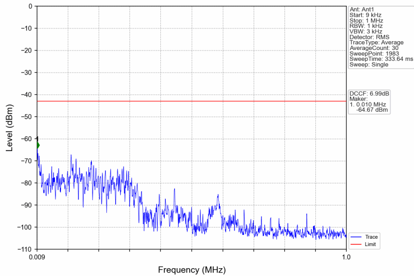
n77d_30kHz_SISO_NTNV_90MHz_DFT-s-OFDM QPSK_3504.99MHz_Edge_1RB_Right
