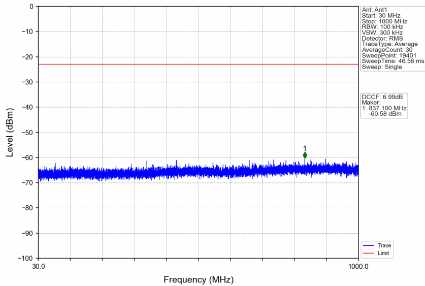
n77d_30kHz_SISO_NTNV_90MHz_CP-OFDM QPSK_3504.99MHz_Edge_1RB_Right
