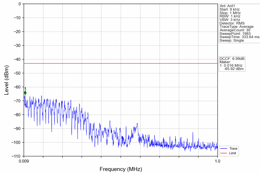
n77d_30kHz_SISO_NTNV_90MHz_CP-OFDM QPSK_3504.99MHz_Edge_1RB_Right
