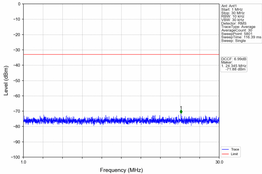
n77d_30kHz_SISO_NTNV_100MHz_DFT-s-OFDM_QPSK_3500.01MHz_Edge_1RB_Left
