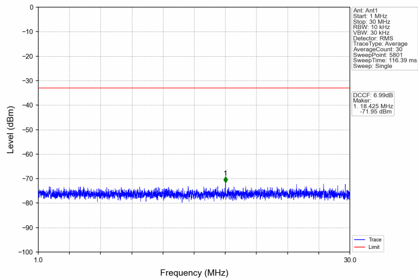
n77d_30kHz_SISO_NTNV_90MHz_CP-OFDM QPSK_3500.01MHz_Edge_1RB_Left
