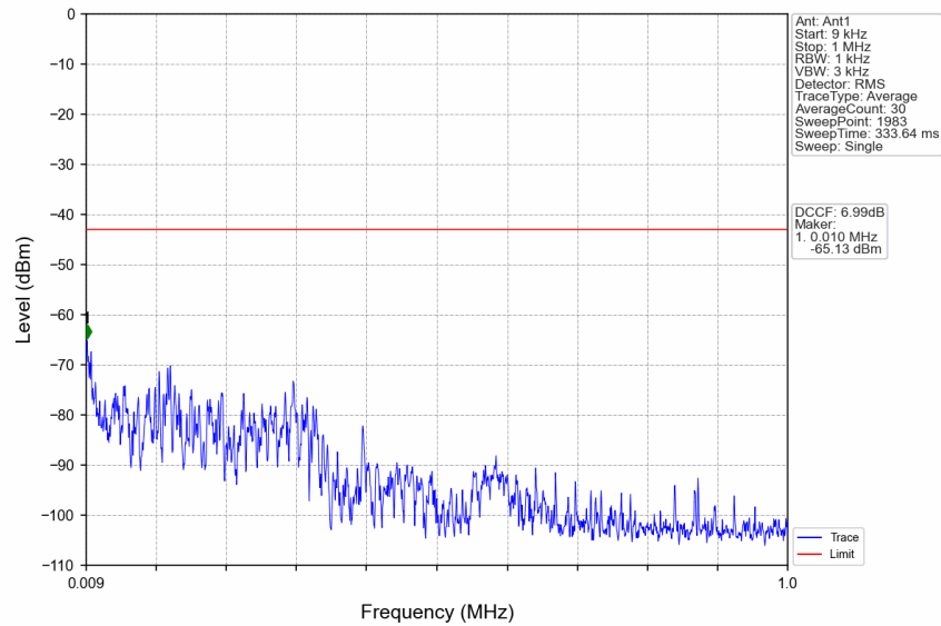
n77d_30kHz_SISO_NTNV_100MHz_DFT-s-OFDM PI/2 BPSK_3499.98MHz_Edge_1RB_Right
