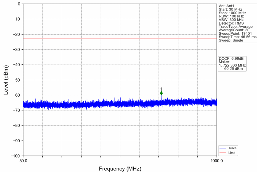
n77d_30kHz_SISO_NTNV_90MHz_CP-OFDM QPSK_3495MHz_Edge_1RB_Left
