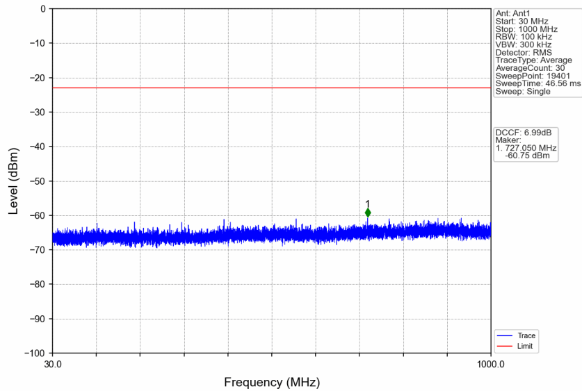
n77d_30kHz_SISO_NTNV_90MHz_DFT-s-OFDM QPSK_3504.99MHz_Edge_1RB_Right
