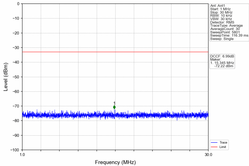
n77d_30kHz_SISO_NTNV_100MHz_DFT-s-OFDM PI/2 BPSK_3500.01MHz_Edge_1RB_Left
