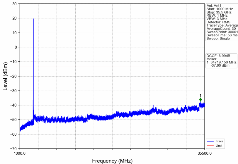
n77d_30kHz_SISO_NTNV_100MHz_DFT-s-OFDM PI/2 BPSK_3499.98MHz_Edge_1RB_Right
