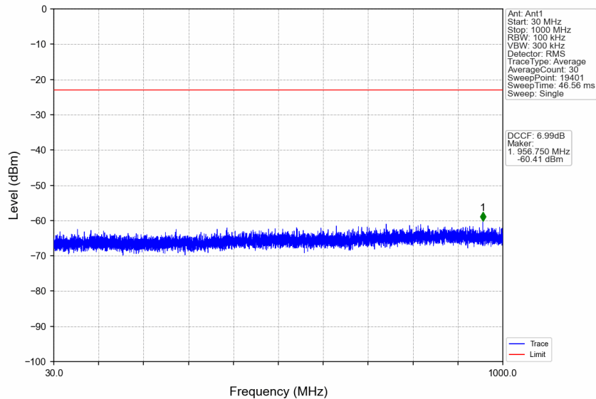
n77d_30kHz_SISO_NTNV_90MHz_DFT-s-OFDM_QPSK_3495MHz_Edge_1RB_Left
