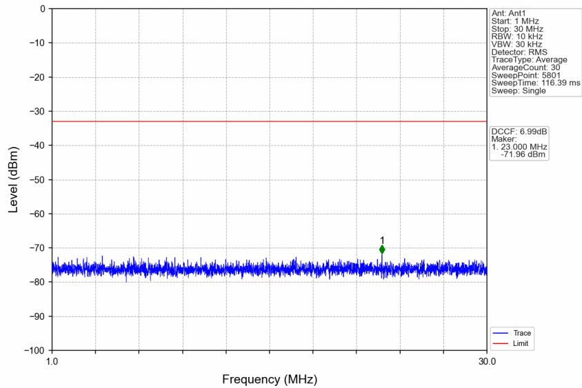
n77d_30kHz_SISO_NTNV_90MHz_CP-OFDM QPSK_3495MHz_Edge_1RB_Left
