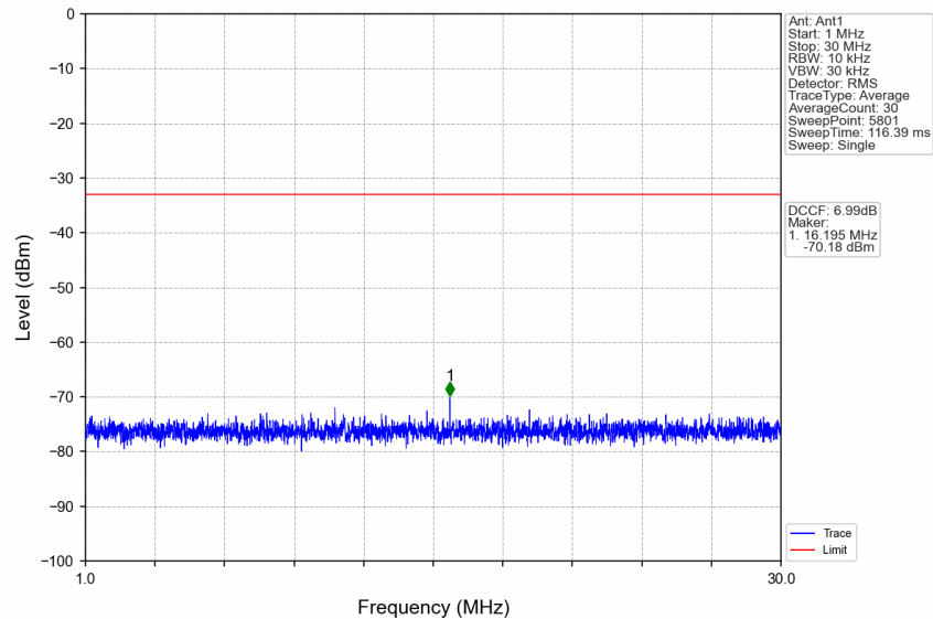
n77d_30kHz_SISO_NTNV_90MHz_CP-OFDM QPSK_3504.99MHz_Edge_1RB_Right
