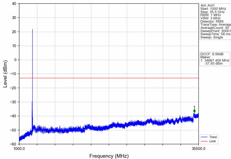
n77d_30kHz_SISO_NTNV_100MHz_DFT-s-OFDM QPSK_3499.98MHz_Edge_1RB_Right
