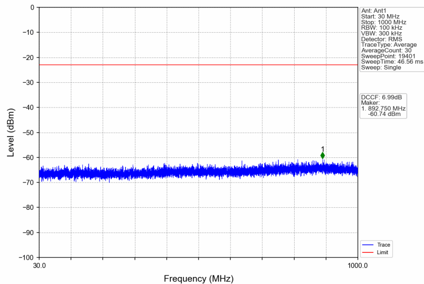
n77d_30kHz_SISO_NTNV_90MHz_CP-OFDM QPSK_3500.01MHz_Edge_1RB_Left
