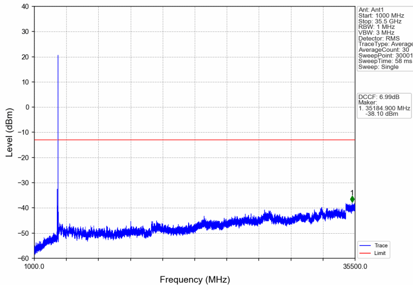
n77d_30kHz_SISO_NTNV_90MHz_DFT-s-OFDM QPSK_3504.99MHz_Edge_1RB_Right
