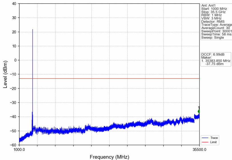
n77d_30kHz_SISO_NTNV_90MHz_CP-OFDM QPSK_3504.99MHz_Edge_1RB_Right
