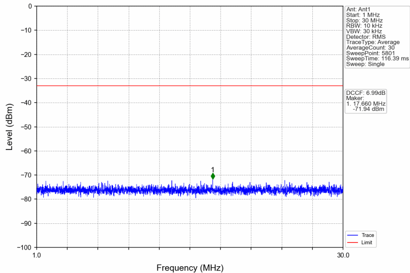
n77d_30kHz_SISO_NTNV_90MHz_DFT-s-OFDM QPSK_3504.99MHz_Edge_1RB_Right
