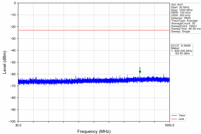
n77d_30kHz_SISO_NTNV_100MHz_DFT-s-OFDM_QPSK_3500.01MHz_Edge_1RB_Left
