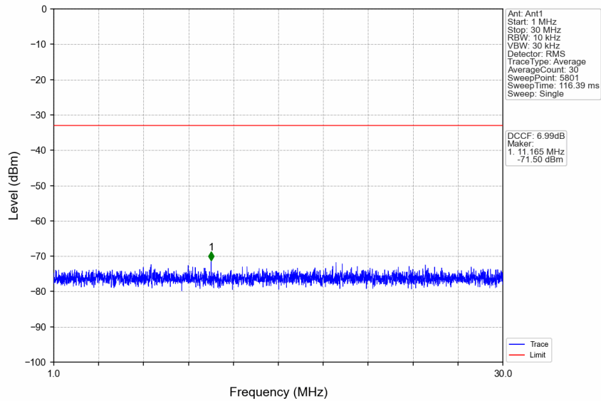
n77d_30kHz_SISO_NTNV_90MHz_DFT-s-OFDM_QPSK_3495MHz_Edge_1RB_Left
