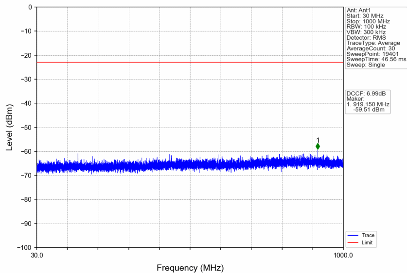
n77d_30kHz_SISO_NTNV_80MHz_DFT-s-OFDM_QPSK_3500.01MHz_Edge_1RB_Left
