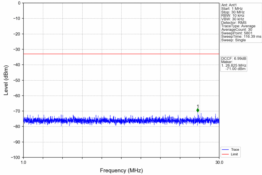
n77d_30kHz_SISO_NTNV_80MHz_CP-OFDM QPSK_3490.02MHz_Edge_1RB_Left
