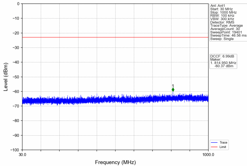
n77d_30kHz_SISO_NTNV_80MHz_DFT-s-OFDM QPSK_3510MHz_Edge_1RB_Right
