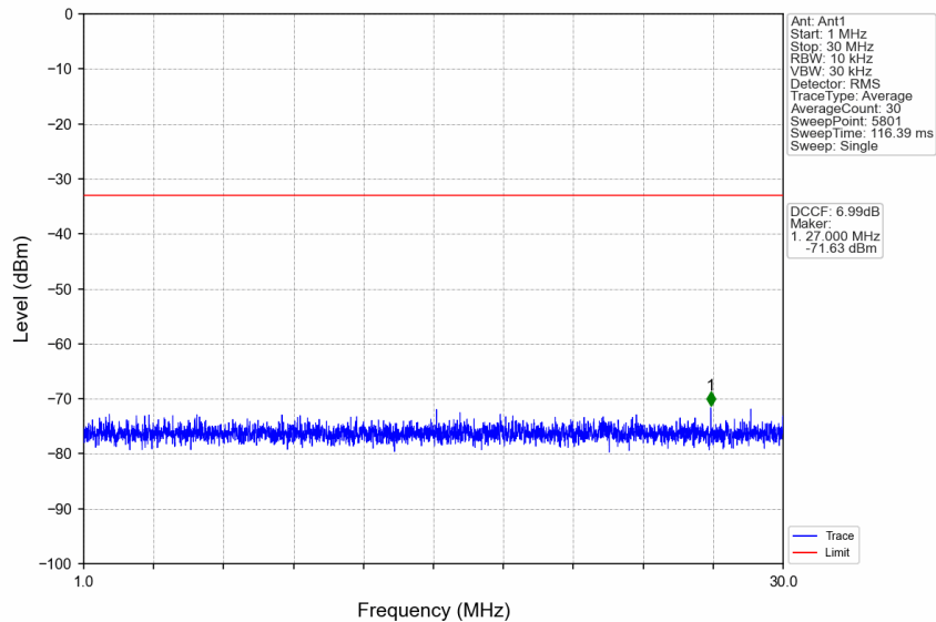
n77d_30kHz_SISO_NTNV_80MHz_DFT-s-OFDM_QPSK_3510MHz_Edge_1RB_Right
