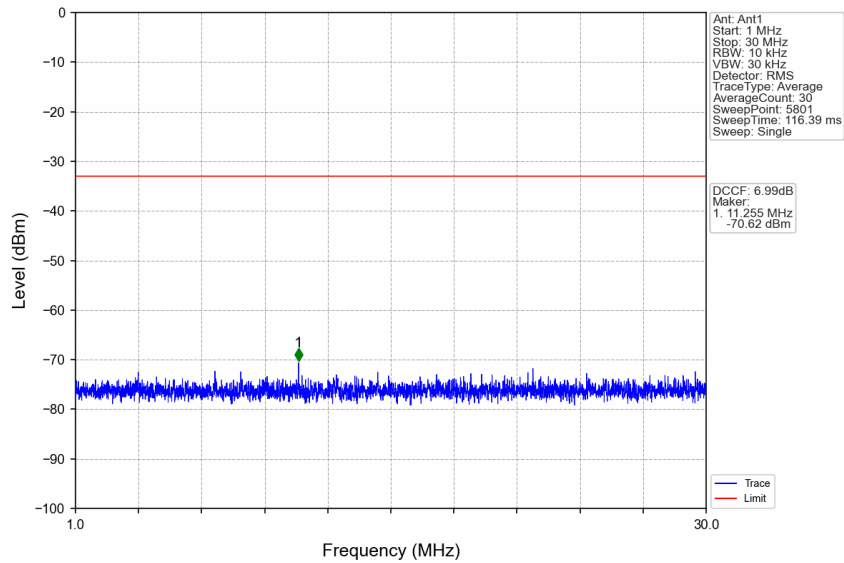
n77d_30kHz_SISO_NTNV_80MHz_DFT-s-OFDM_QPSK_3500.01MHz_Edge_1RB_Left
