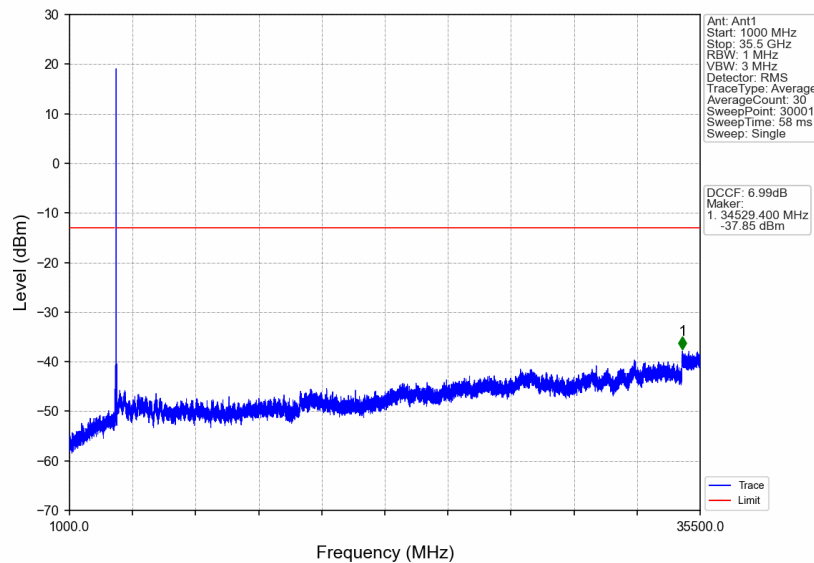
n77d_30kHz_SISO_NTNV_70MHz_CP-OFDM_QPSK_3514.98MHz_Edge_1RB_Right
