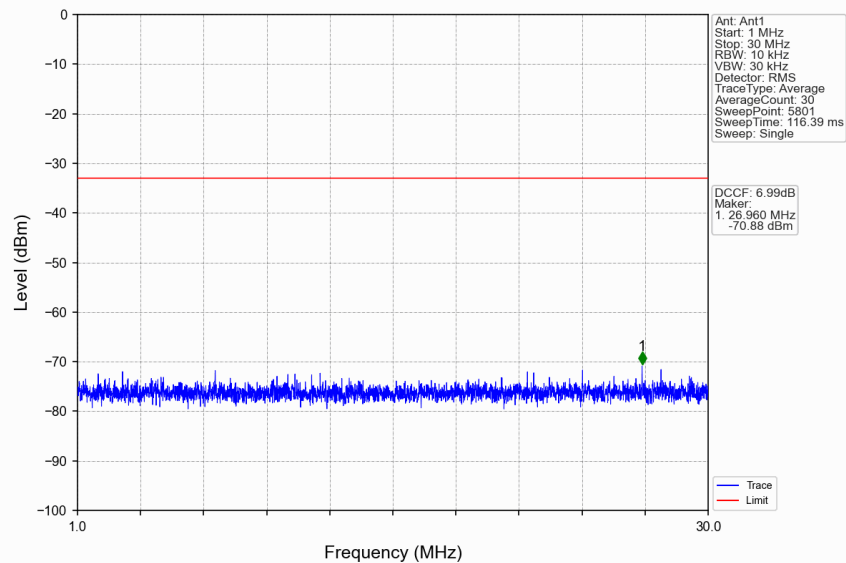
n77d_30kHz_SISO_NTNV_70MHz_CP-OFDM QPSK_3514.98MHz_Edge_1RB_Right
