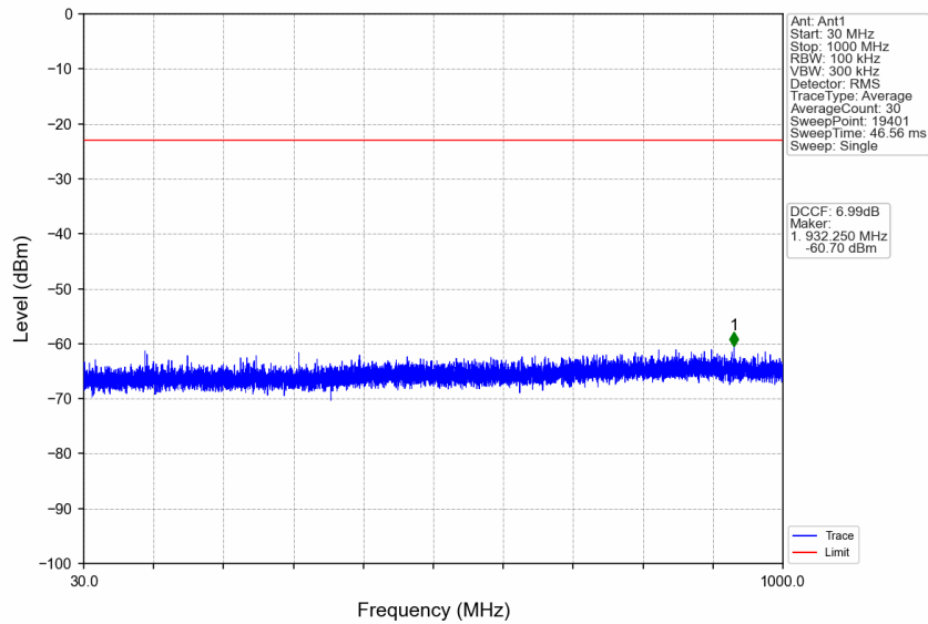
n77d_30kHz_SISO_NTNV_80MHz_CP-OFDM QPSK_3490.02MHz_Edge_1RB_Left
