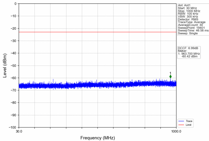
n77d_30kHz_SISO_NTNV_70MHz_CP-OFDM_QPSK_3514.98MHz_Edge_1RB_Right
