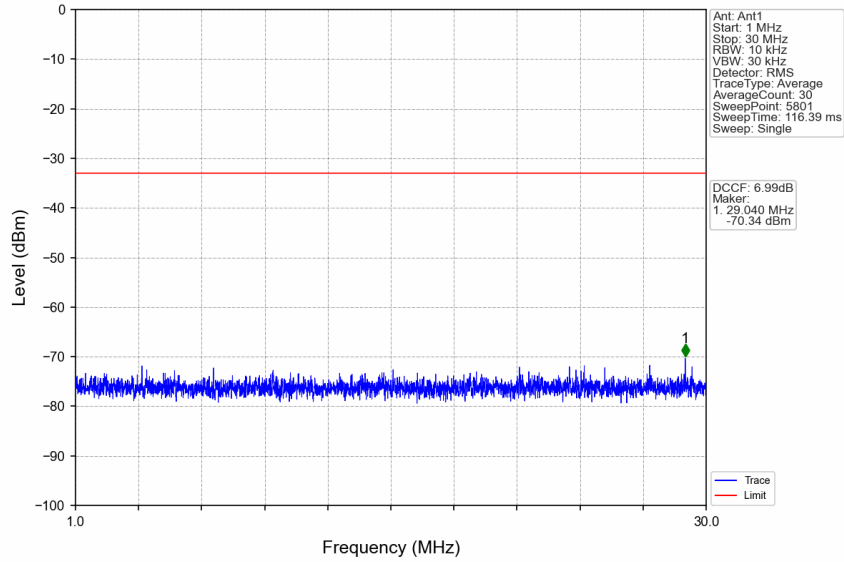
n77d_30kHz_SISO_NTNV_70MHz_CP-OFDM QPSK_3500.01MHz_Edge_1RB_Left
