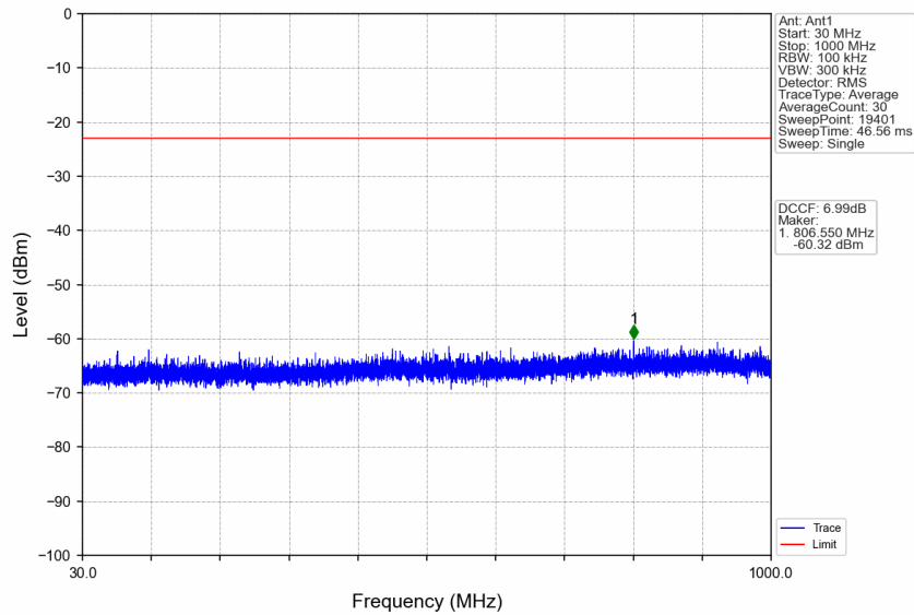
n77d_30kHz_SISO_NTNV_70MHz_CP-OFDM QPSK_3500.01MHz_Edge_1RB_Left
