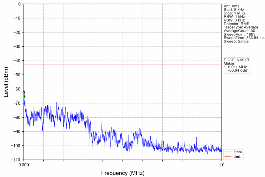
n77d_30kHz_SISO_NTNV_80MHz_DFT-s-OFDM_QPSK_3510MHz_Edge_1RB_Right
