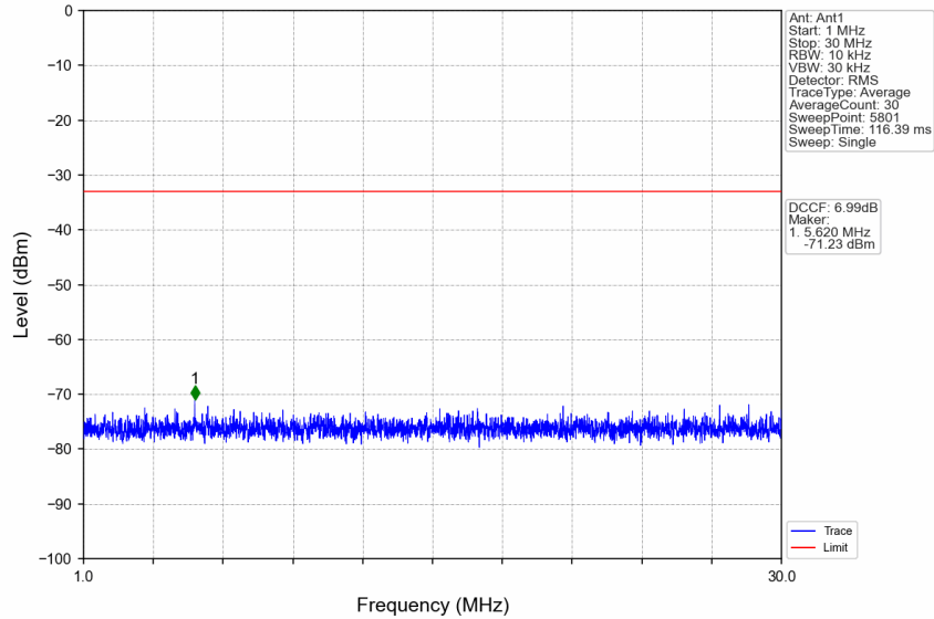
n77d_30kHz_SISO_NTNV_70MHz_CP-OFDM QPSK_3485.01MHz_Edge_1RB_Left
