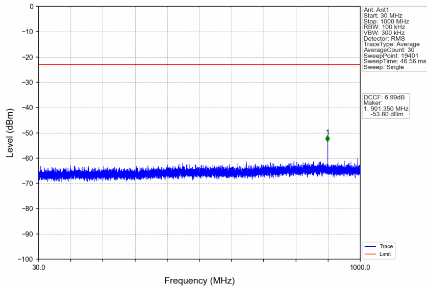
n77d_30kHz_SISO_NTNV_70MHz_CP-OFDM QPSK_3485.01MHz_Edge_1RB_Left
