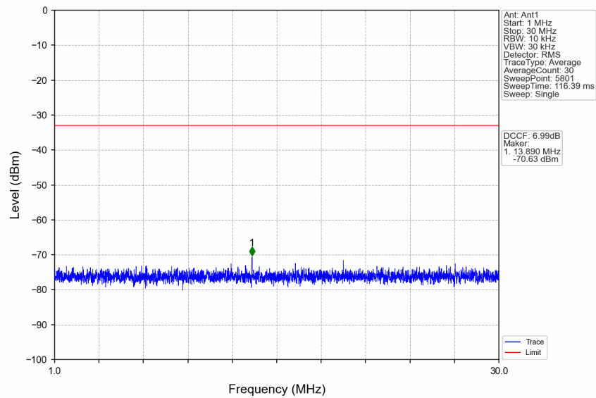
n77d_30kHz_SISO_NTNV_80MHz_CP-OFDM QPSK_3500.01MHz_Edge_1RB_Left
