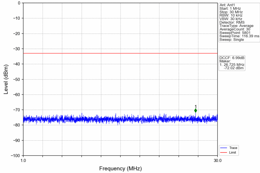
n77d_30kHz_SISO_NTNV_80MHz_DFT-s-OFDM_QPSK_3490.02MHz_Edge_1RB_Left
