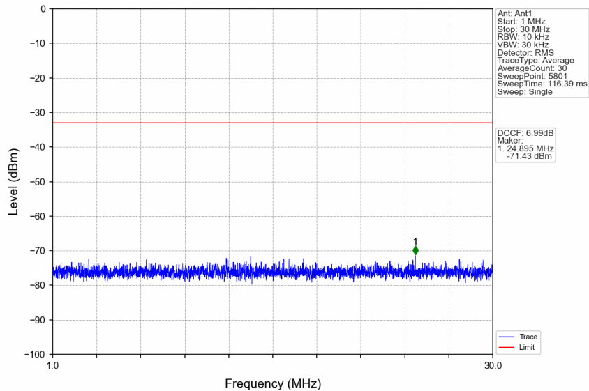
n77d_30kHz_SISO_NTNV_80MHz_DFT-s-OFDM PI/2 BPSK_3510MHz_Edge_1RB_Right
