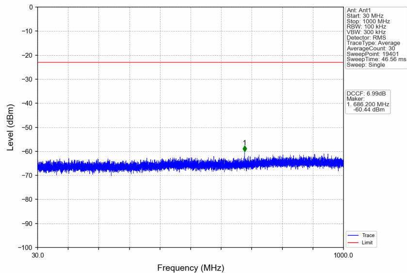
n77d_30kHz_SISO_NTNV_80MHz_DFT-s-OFDM PI/2 BPSK_3490.02MHz_Edge_1RB_Left
