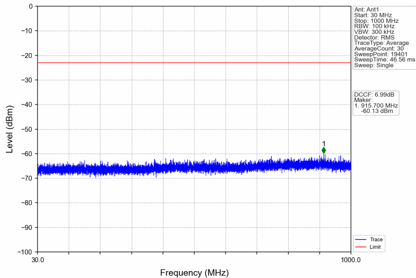
n77d_30kHz_SISO_NTNV_70MHz_DFT-s-OFDM_QPSK_3485.01MHz_Edge_1RB_Left
