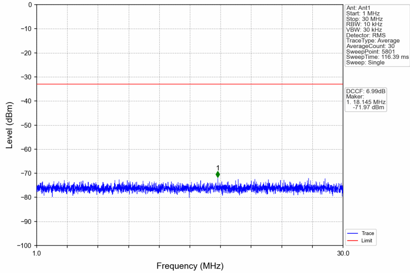
n77d_30kHz_SISO_NTNV_60MHz_DFT-s-OFDM_QPSK_3480MHz_Edge_1RB_Left
