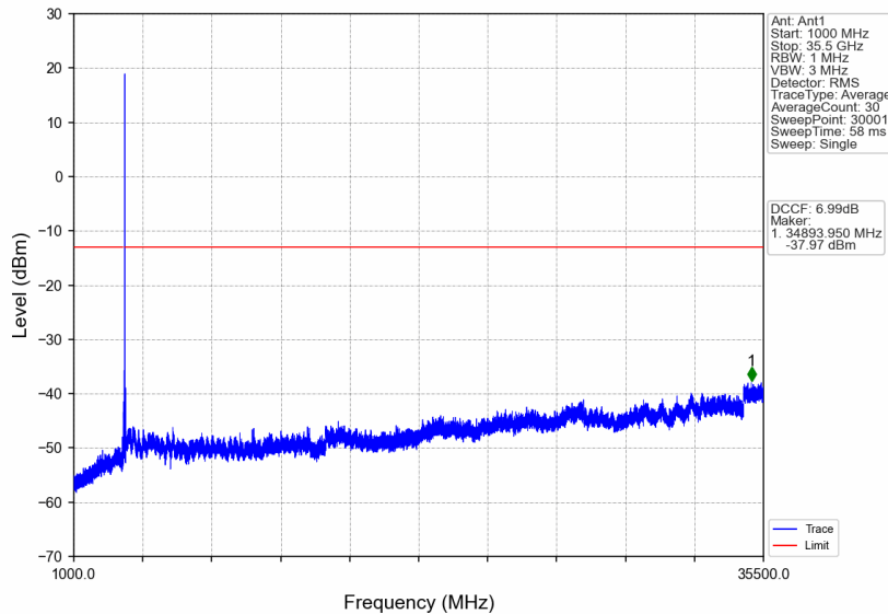
n77d_30kHz_SISO_NTNV_60MHz_CP-OFDM QPSK_3519.99MHz_Edge_1RB_Right
