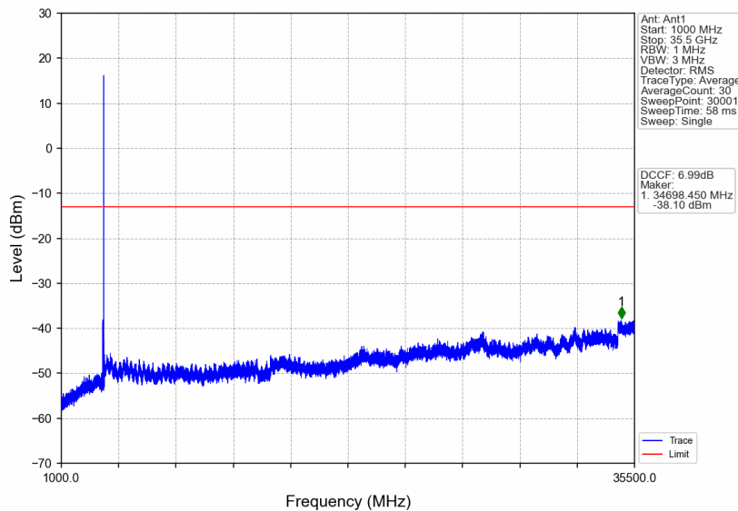
n77d_30kHz_SISO_NTNV_70MHz_DFT-s-OFDM QPSK_3514.98MHz_Edge_1RB_Right
