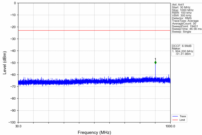
n77d_30kHz_SISO_NTNV_60MHz_CP-OFDM_QPSK_3500.01MHz_Edge_1RB_Left
