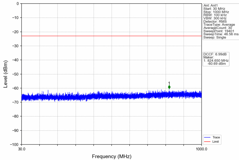
n77d_30kHz_SISO_NTNV_70MHz_DFT-s-OFDM QPSK_3514.98MHz_Edge_1RB_Right
