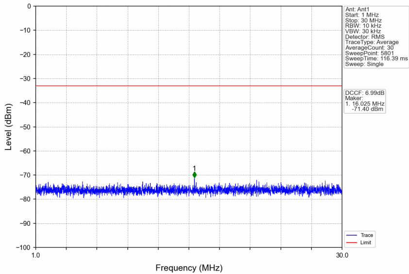
n77d_30kHz_SISO_NTNV_70MHz_DFT-s-OFDM_QPSK_3500.01MHz_Edge_1RB_Left
