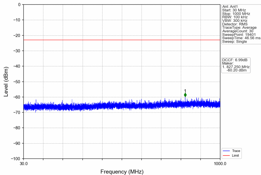
n77d_30kHz_SISO_NTNV_60MHz_CP-OFDM QPSK_3480MHz_Edge_1RB_Left
