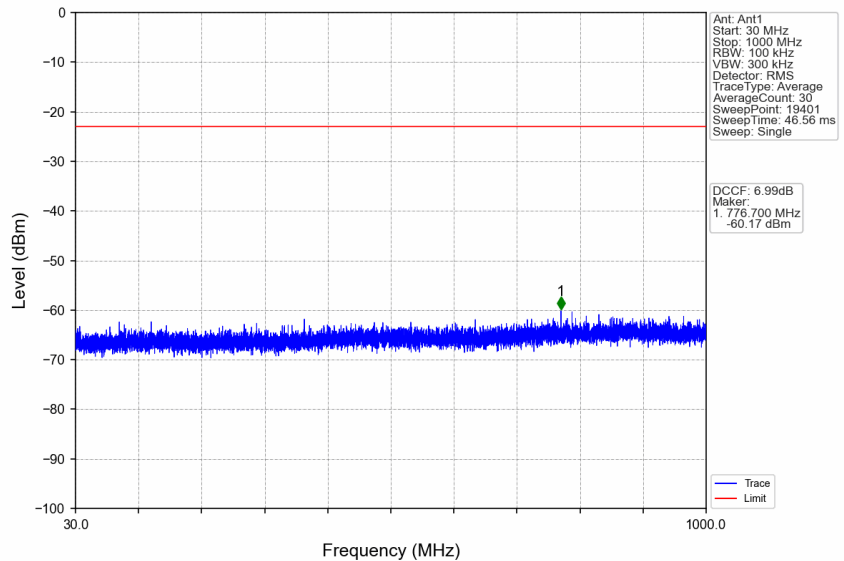
n77d_30kHz_SISO_NTNV_60MHz_DFT-s-OFDM_QPSK_3500.01MHz_Edge_1RB_Left
