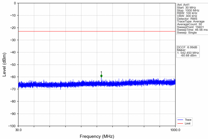
n77d_30kHz_SISO_NTNV_70MHz_DFT-s-OFDM_QPSK_3500.01MHz_Edge_1RB_Left
