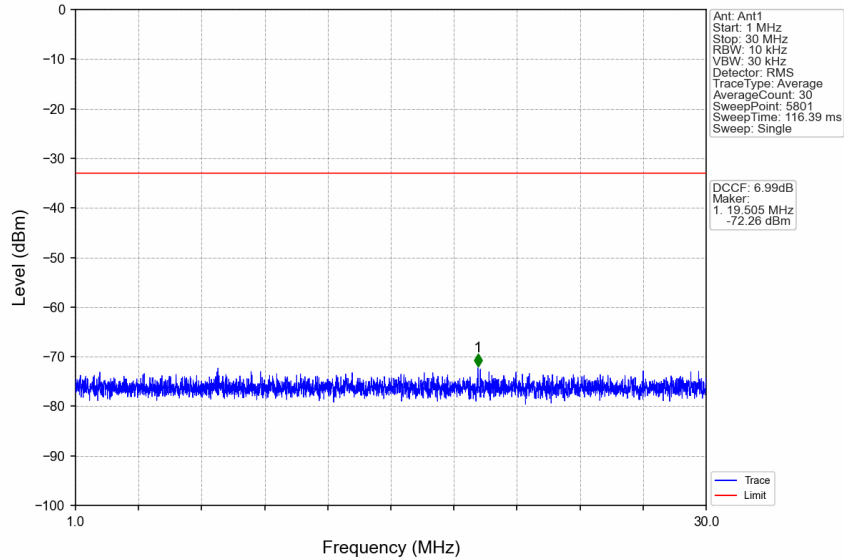
n77d_30kHz_SISO_NTNV_70MHz_DFT-s-OFDM_QPSK_3485.01MHz_Edge_1RB_Left
