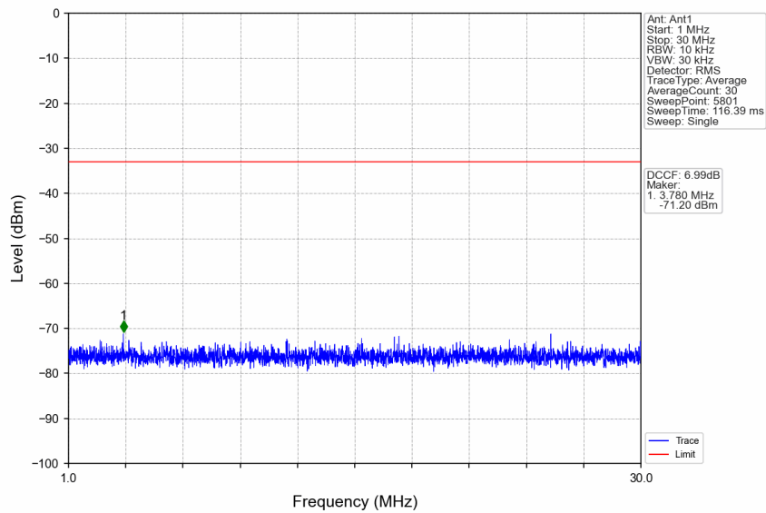
n77d_30kHz_SISO_NTNV_60MHz_CP-OFDM QPSK_3480MHz_Edge_1RB_Left
