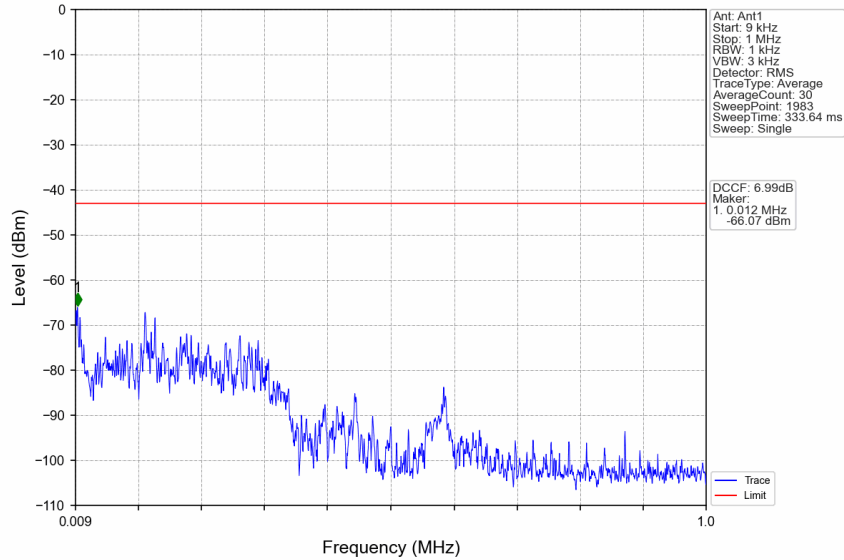
n77d_30kHz_SISO_NTNV_60MHz_DFT-s-OFDM QPSK_3519.99MHz_Edge_1RB_Right
