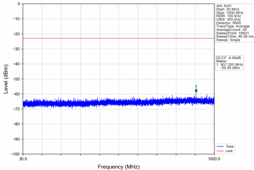
n77d_30kHz_SISO_NTNV_60MHz_DFT-s-OFDM_QPSK_3480MHz_Edge_1RB_Left
