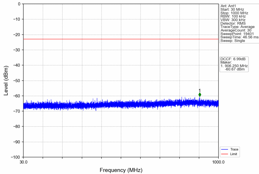
n77d_30kHz_SISO_NTNV_60MHz_CP-OFDM QPSK_3519.99MHz_Edge_1RB_Right
