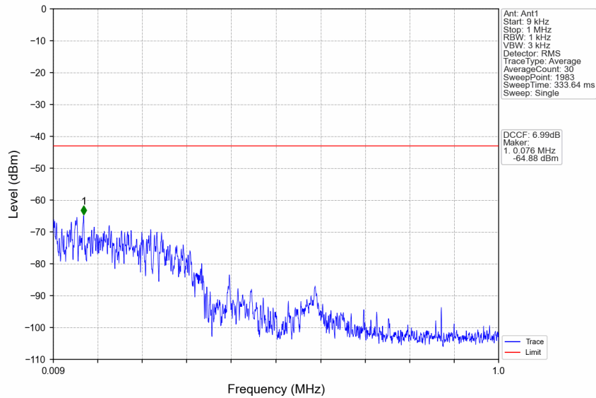
n77d_30kHz_SISO_NTNV_60MHz_CP-OFDM QPSK_3519.99MHz_Edge_1RB_Right
