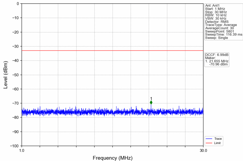
n77d_30kHz_SISO_NTNV_60MHz_CP-OFDM QPSK_3519.99MHz_Edge_1RB_Right
