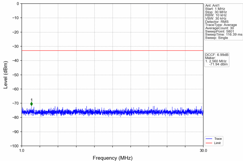
n77d_30kHz_SISO_NTNV_70MHz_DFT-s-OFDM QPSK_3514.98MHz_Edge_1RB_Right
