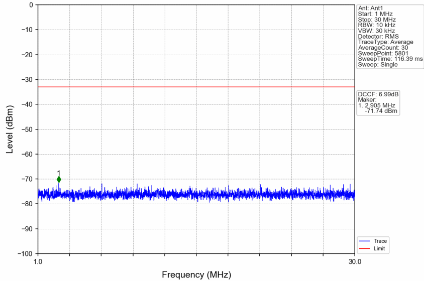
n77d_30kHz_SISO_NTNV_60MHz_CP-OFDM_QPSK_3500.01MHz_Edge_1RB_Left
