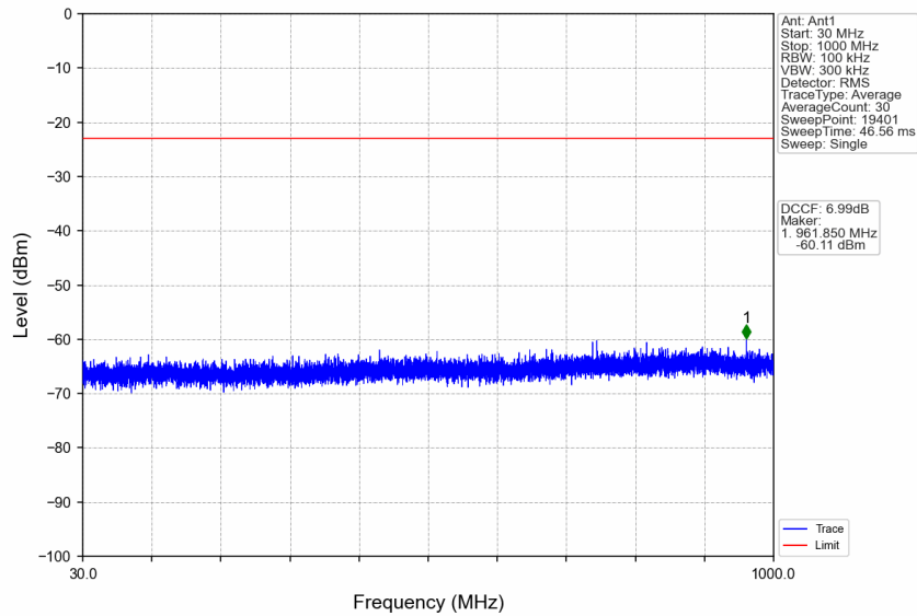
n77d_30kHz_SISO_NTNV_50MHz_CP-OFDM QPSK_3525MHz_Edge_1RB_Right
