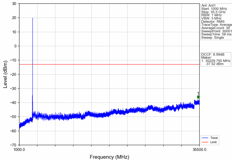
n77d_30kHz_SISO_NTNV_50MHz_CP-OFDM QPSK_3525MHz_Edge_1RB_Right
