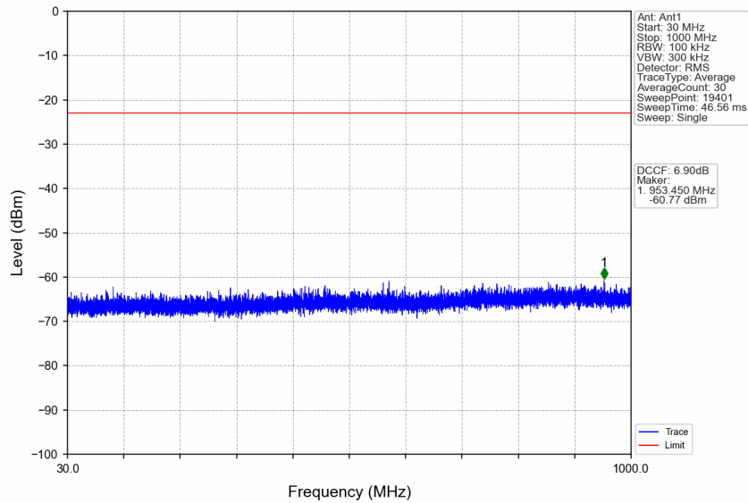
n77d_30kHz_SISO_NTNV_50MHz_DFT-s-OFDM_QPSK_3475.02MHz_Edge_1RB_Left
