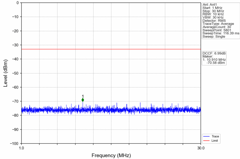
n77d_30kHz_SISO_NTNV_50MHz_CP-OFDM QPSK_3475.02MHz_Edge_1RB_Left
