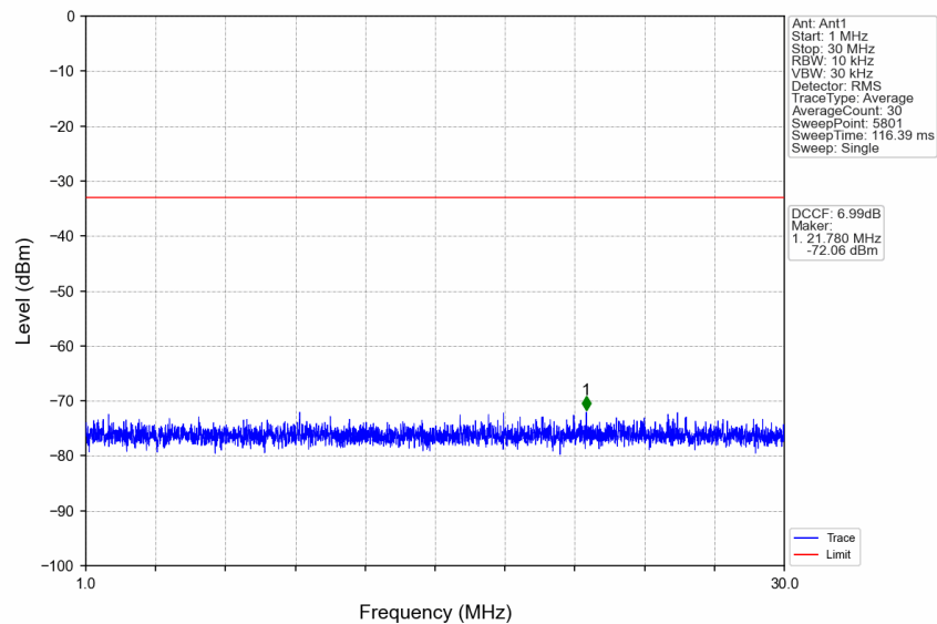
n77d_30kHz_SISO_NTNV_50MHz_DFT-s-OFDM QPSK_3525MHz_Edge_1RB_Right
