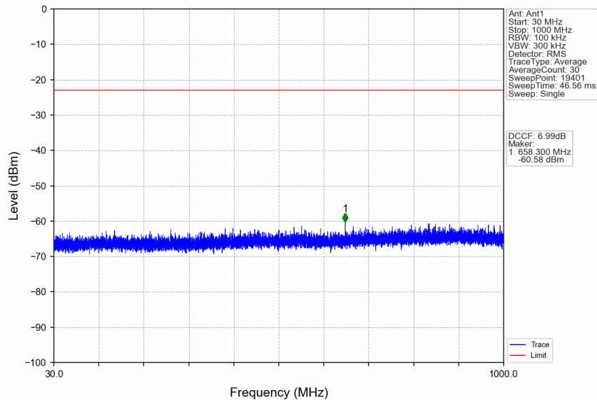
n77d_30kHz_SISO_NTNV_50MHz_CP-OFDM QPSK_3500.01MHz_Edge_1RB_Left
