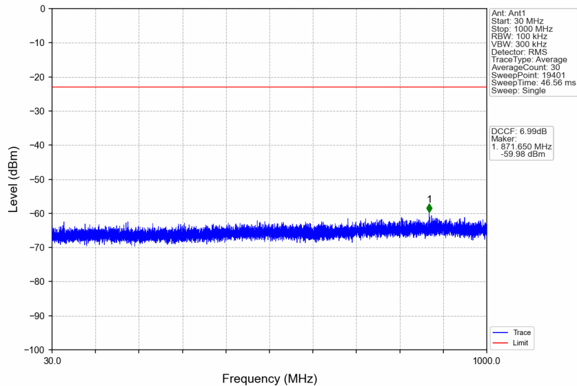
n77d_30kHz_SISO_NTNV_50MHz_CP-OFDM QPSK_3475.02MHz_Edge_1RB_Left
