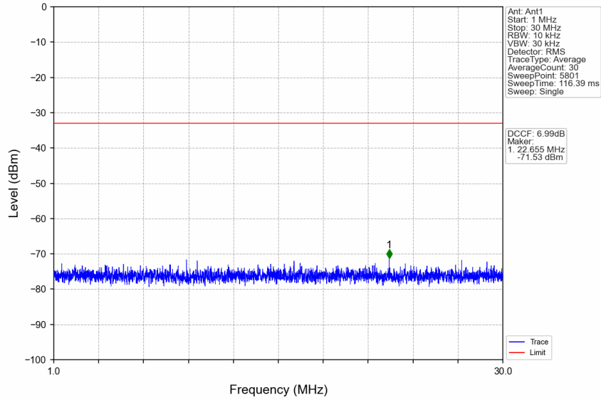
n77d_30kHz_SISO_NTNV_50MHz_DFT-s-OFDM_QPSK_3500.01MHz_Edge_1RB_Left
