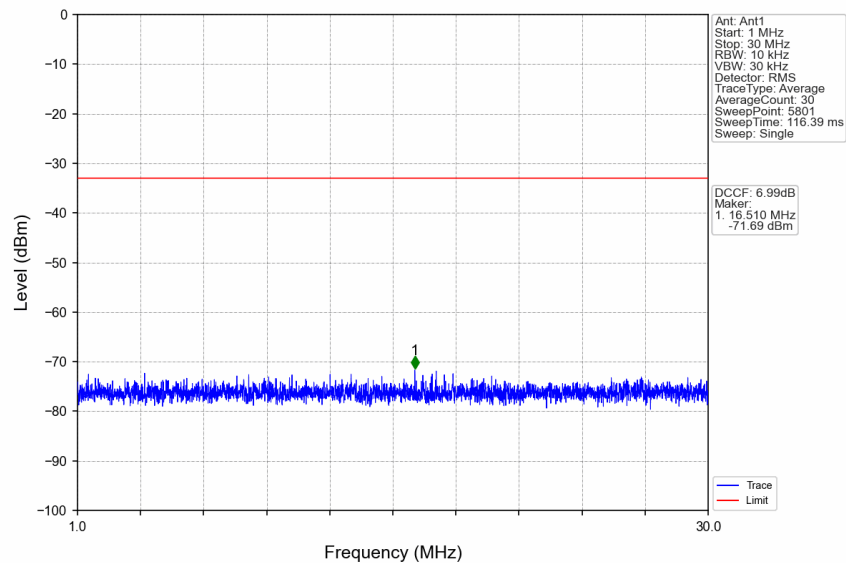
n77d_30kHz_SISO_NTNV_40MHz_CP-OFDM QPSK_3529.98MHz_Edge_1RB_Right
