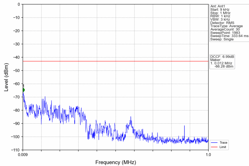
n77d_30kHz_SISO_NTNV_50MHz_DFT-s-OFDM PI/2 BPSK_3525MHz_Edge_1RB_Right
