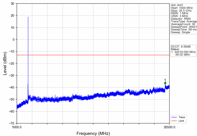
n77d_30kHz_SISO_NTNV_50MHz_DFT-s-OFDM_QPSK_3525MHz_Edge_1RB_Right
