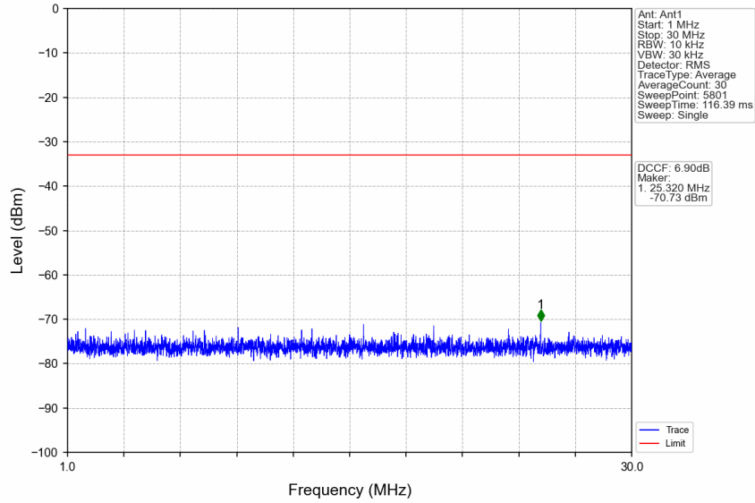
n77d_30kHz_SISO_NTNV_50MHz_DFT-s-OFDM_QPSK_3475.02MHz_Edge_1RB_Left
