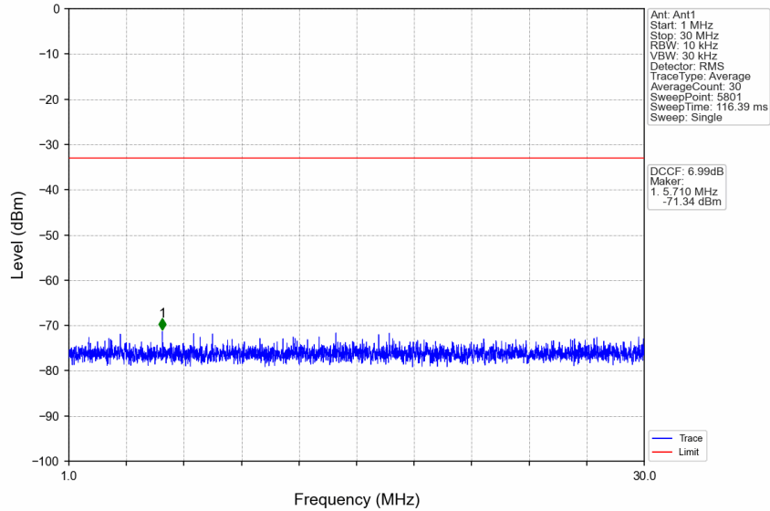
n77d_30kHz_SISO_NTNV_40MHz_CP-OFDM QPSK_3500.01MHz_Edge_1RB_Left
