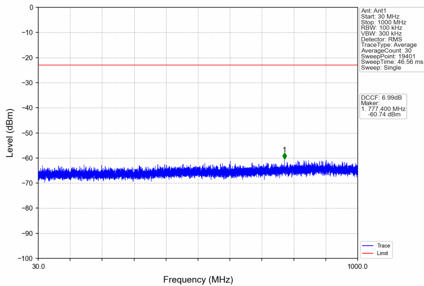
n77d_30kHz_SISO_NTNV_50MHz_DFT-s-OFDM_QPSK_3525MHz_Edge_1RB_Right
