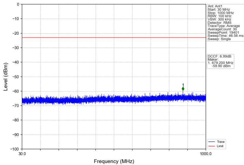
n77d_30kHz_SISO_NTNV_40MHz_CP-OFDM QPSK_3529.98MHz_Edge_1RB_Right
