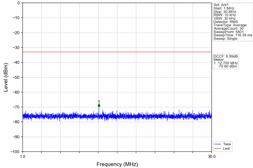
n77d_30kHz_SISO_NTNV_50MHz_CP-OFDM QPSK_3500.01MHz_Edge_1RB_Left
