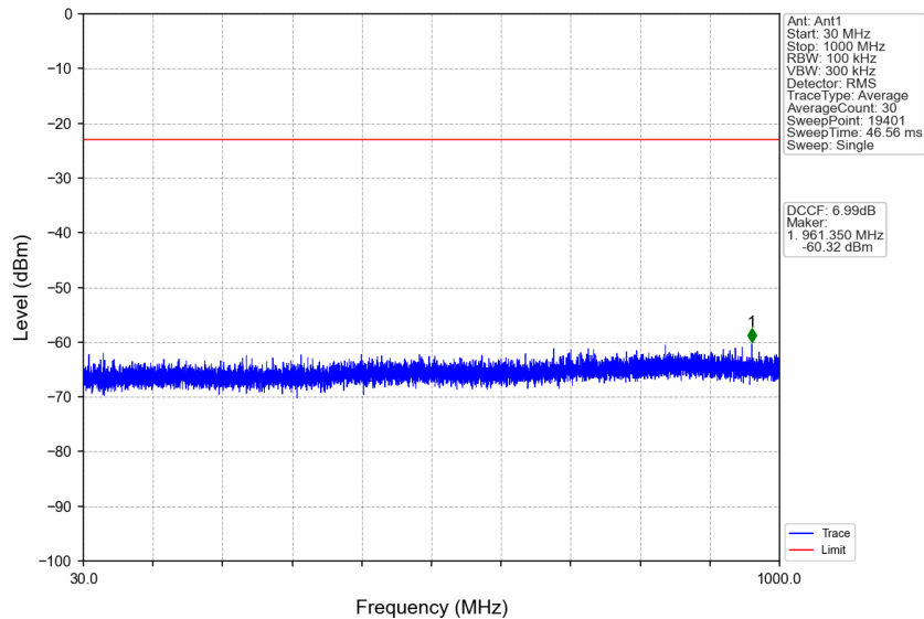
n77d_30kHz_SISO_NTNV_40MHz_CP-OFDM QPSK_3470.01MHz_Edge_1RB_Left
