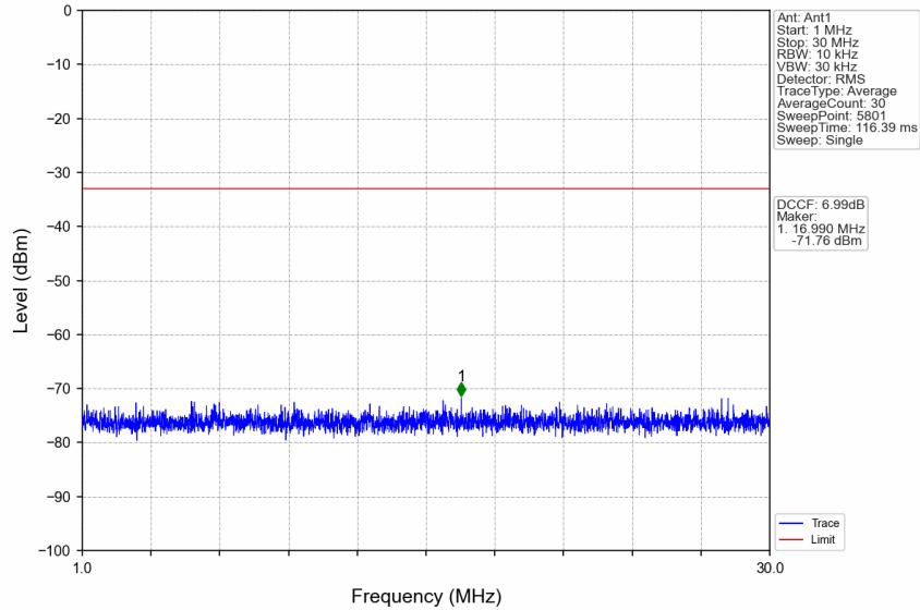
n77d_30kHz_SISO_NTNV_40MHz_CP-OFDM QPSK_3470.01MHz_Edge_1RB_Left
