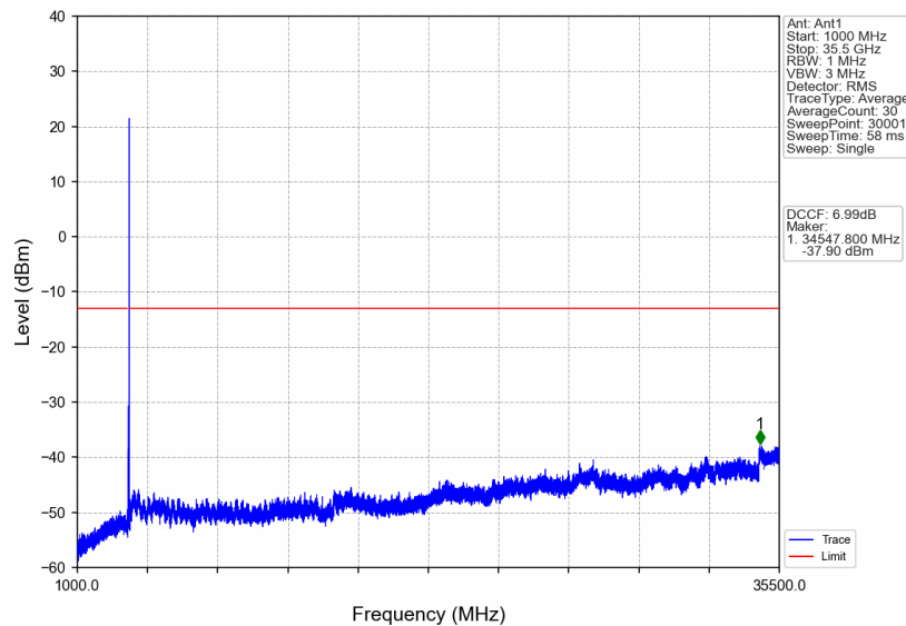
n77d_30kHz_SISO_NTNV_40MHz_CP-OFDM QPSK_3529.98MHz_Edge_1RB_Right
