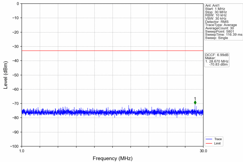
n77d_30kHz_SISO_NTNV_40MHz_DFT-s-OFDM_QPSK_3470.01MHz_Edge_1RB_Left
