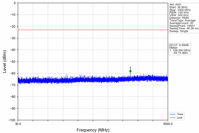
n77d_30kHz_SISO_NTNV_30MHz_CP-OFDM QPSK_3534.99MHz_Edge_1RB_Right
