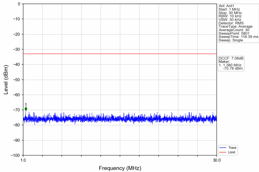
n77d_30kHz_SISO_NTNV_30MHz_CP-OFDM QPSK_3465MHz_Edge_1RB_Left
