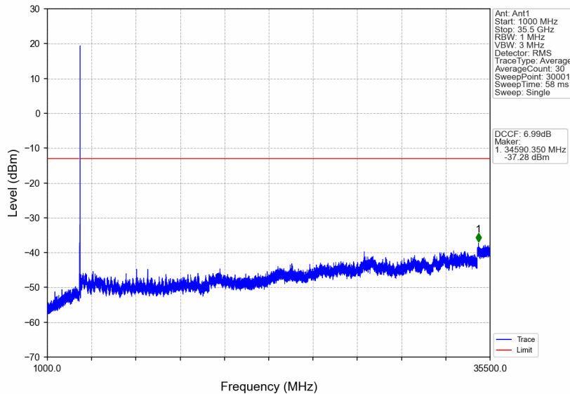
n77d_30kHz_SISO_NTNV_30MHz_DFT-s-OFDM QPSK_3534.99MHz_Edge_1RB_Right
