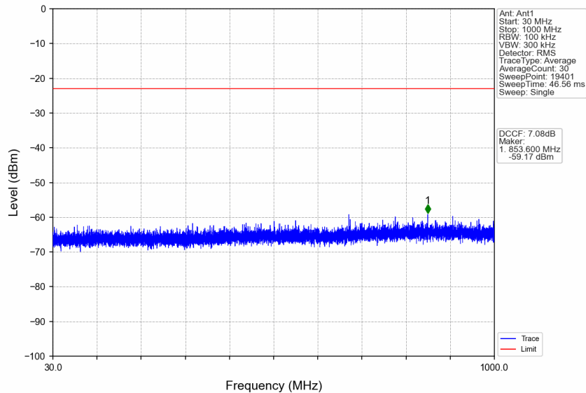
n77d_30kHz_SISO_NTNV_30MHz_DFT-s-OFDM_QPSK_3500.01MHz_Edge_1RB_Left
