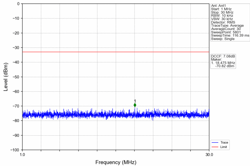
n77d_30kHz_SISO_NTNV_30MHz_DFT-s-OFDM QPSK_3465MHz_Edge_1RB_Left
