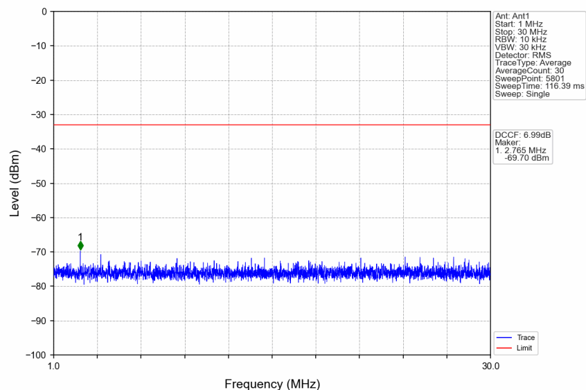
n77d_30kHz_SISO_NTNV_30MHz_CP-OFDM QPSK_3534.99MHz_Edge_1RB_Right
