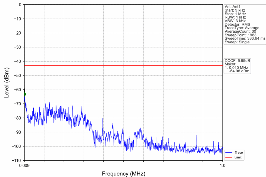
n77d_30kHz_SISO_NTNV_30MHz_DFT-s-OFDM QPSK_3534.99MHz_Edge_1RB_Right
