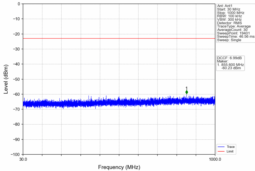
n77d_30kHz_SISO_NTNV_30MHz_DFT-s-OFDM QPSK_3534.99MHz_Edge_1RB_Right
