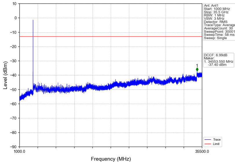
n77d_30kHz_SISO_NTNV_30MHz_CP-OFDM QPSK_3534.99MHz_Edge_1RB_Right
