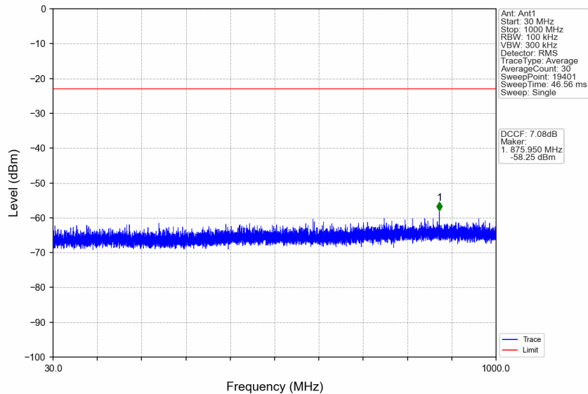
n77d_30kHz_SISO_NTNV_30MHz_DFT-s-OFDM QPSK_3465MHz_Edge_1RB_Left
