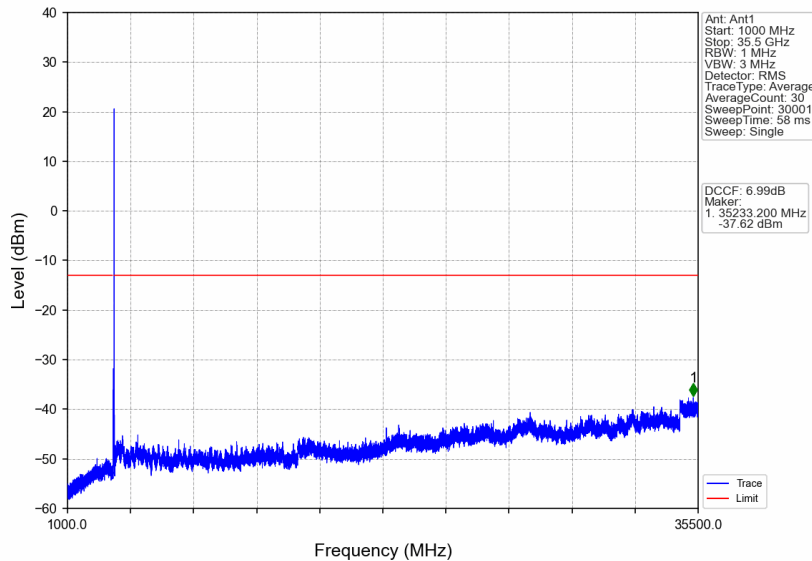
n77d_30kHz_SISO_NTNV_40MHz_DFT-s-OFDM QPSK_3529.98MHz_Edge_1RB_Right
