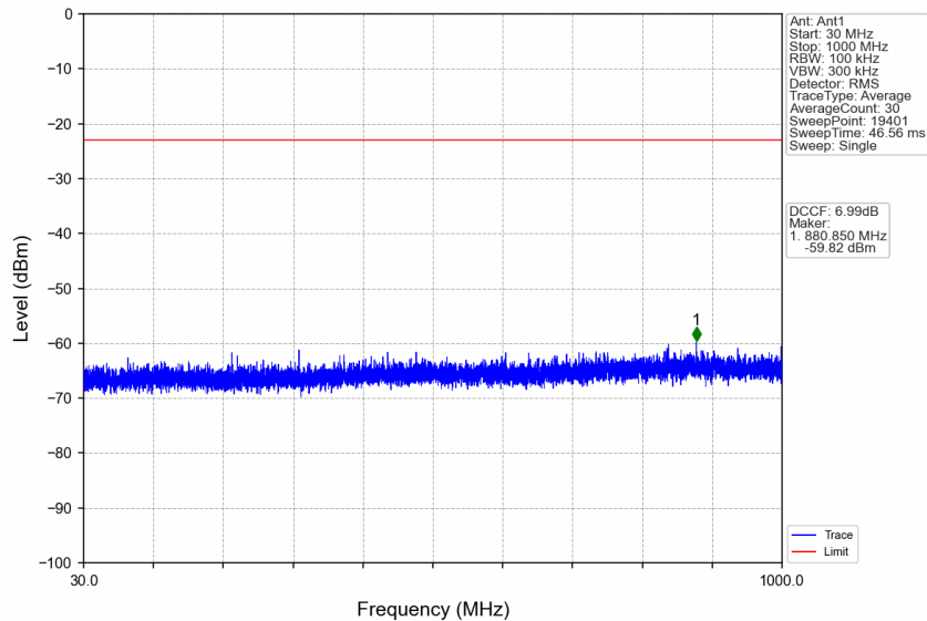
n77d_30kHz_SISO_NTNV_40MHz_DFT-s-OFDM_QPSK_3470.01MHz_Edge_1RB_Left
