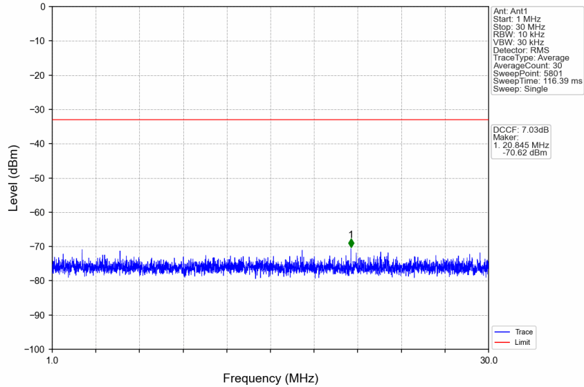
n77d_30kHz_SISO_NTNV_30MHz_CP-OFDM QPSK_3500.01MHz_Edge_1RB_Left
