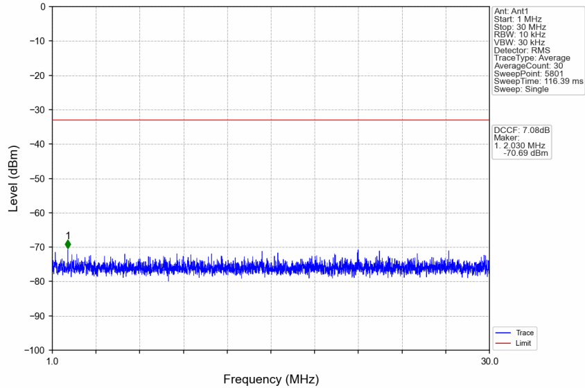
n77d_30kHz_SISO_NTNV_30MHz_DFT-s-OFDM_QPSK_3500.01MHz_Edge_1RB_Left
