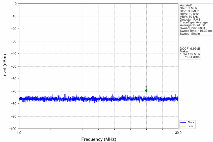
n77d_30kHz_SISO_NTNV_40MHz_DFT-s-OFDM QPSK_3529.98MHz_Edge_1RB_Right
