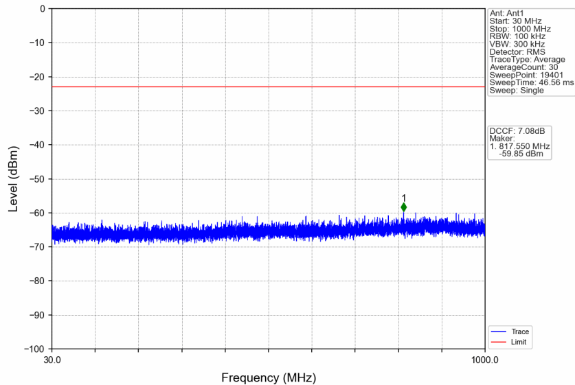
n77d_30kHz_SISO_NTNV_30MHz_CP-OFDM QPSK_3465MHz_Edge_1RB_Left
