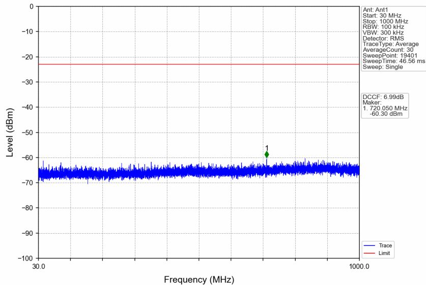
n77d_30kHz_SISO_NTNV_40MHz_DFT-s-OFDM_QPSK_3500.01MHz_Edge_1RB_Left
