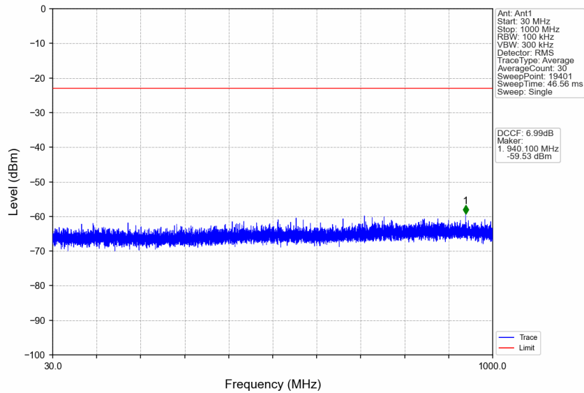
n77d_30kHz_SISO_NTNV_25MHz_DFT-s-OFDM QPSK_3537.48MHz_Edge_1RB_Right
