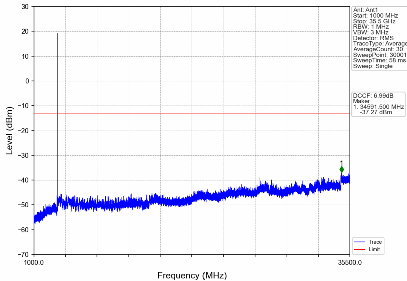
n77d_30kHz_SISO_NTNV_25MHz_DFT-s-OFDM QPSK_3537.48MHz_Edge_1RB_Right
