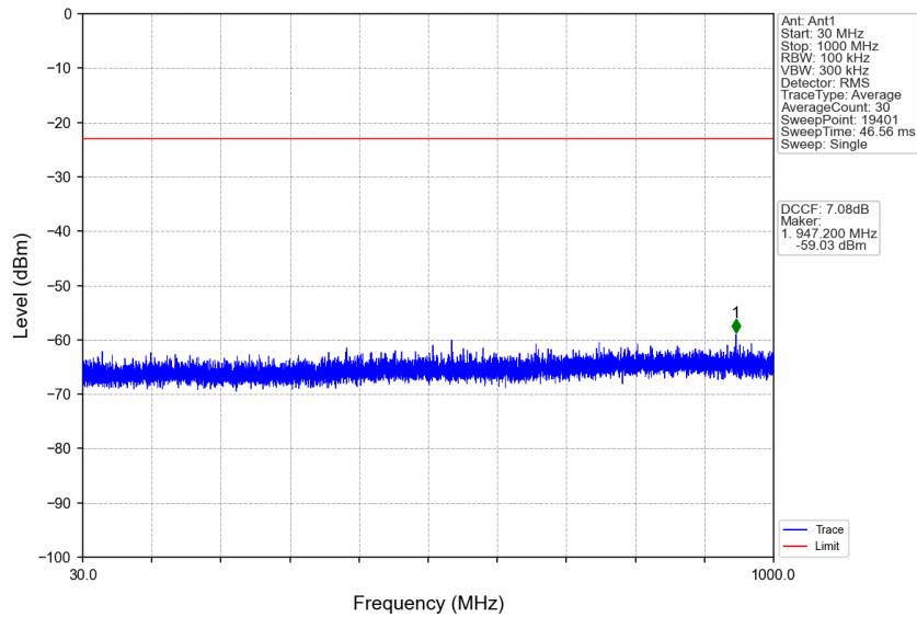
n77d_30kHz_SISO_NTNV_20MHz_CP-OFDM QPSK_3460.02MHz_Edge_1RB_Left
