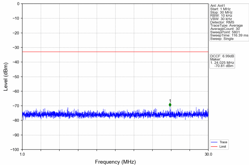
n77d_30kHz_SISO_NTNV_25MHz_CP-OFDM QPSK_3537.48MHz_Edge_1RB_Right
