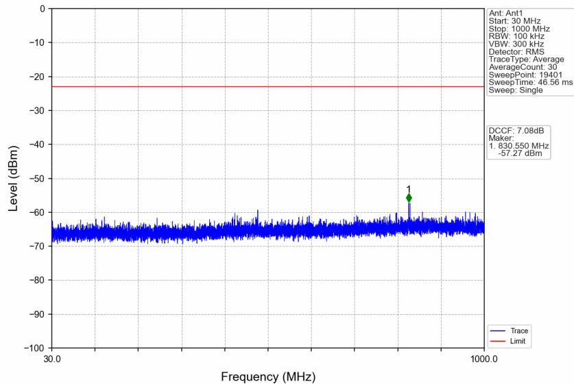
n77d_30kHz_SISO_NTNV_25MHz_DFT-s-OFDM_QPSK_3462.51MHz_Edge_1RB_Left
