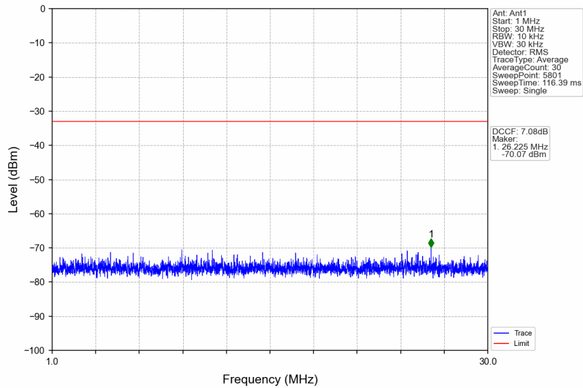
n77d_30kHz_SISO_NTNV_25MHz_DFT-s-OFDM_QPSK_3462.51MHz_Edge_1RB_Left
