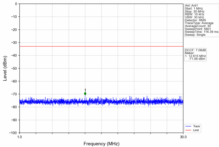
n77d_30kHz_SISO_NTNV_25MHz_DFT-s-OFDM_QPSK_3500.01MHz_Edge_1RB_Left
