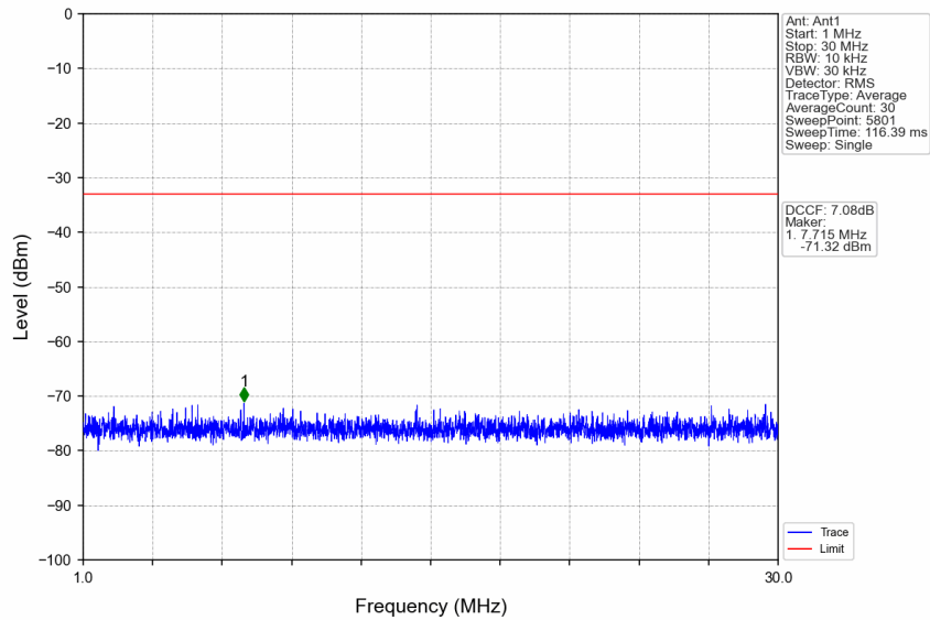
n77d_30kHz_SISO_NTNV_20MHz_CP-OFDM QPSK_3500.01MHz_Edge_1RB_Left
