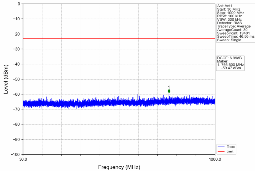
n77d_30kHz_SISO_NTNV_20MHz_CP-OFDM QPSK_3540MHz_Edge_1RB_Right
