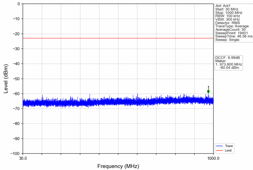
n77d_30kHz_SISO_NTNV_25MHz_CP-OFDM QPSK_3537.48MHz_Edge_1RB_Right
