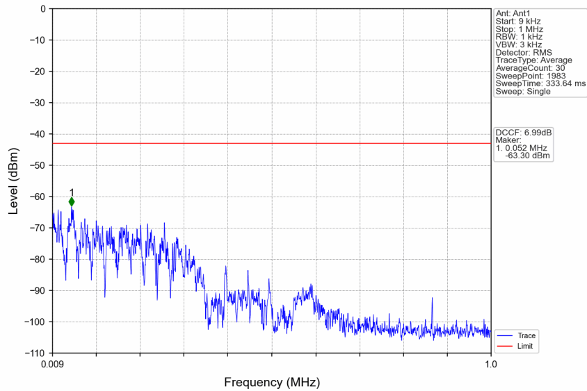
n77d_30kHz_SISO_NTNV_25MHz_CP-OFDM QPSK_3537.48MHz_Edge_1RB_Right
