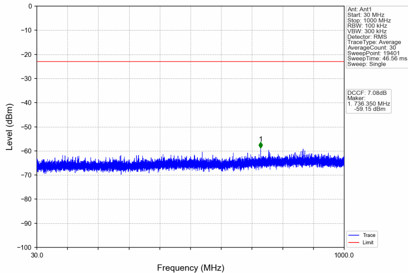
n77d_30kHz_SISO_NTNV_20MHz_CP-OFDM QPSK_3500.01MHz_Edge_1RB_Left
