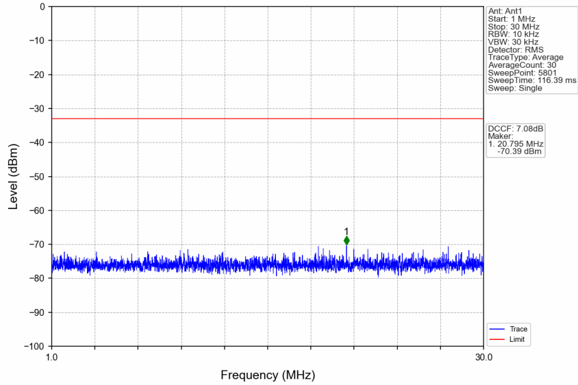
n77d_30kHz_SISO_NTNV_20MHz_CP-OFDM QPSK_3460.02MHz_Edge_1RB_Left
