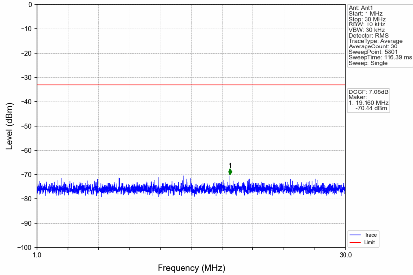
n77d_30kHz_SISO_NTNV_25MHz_CP-OFDM QPSK_3500.01MHz_Edge_1RB_Left
