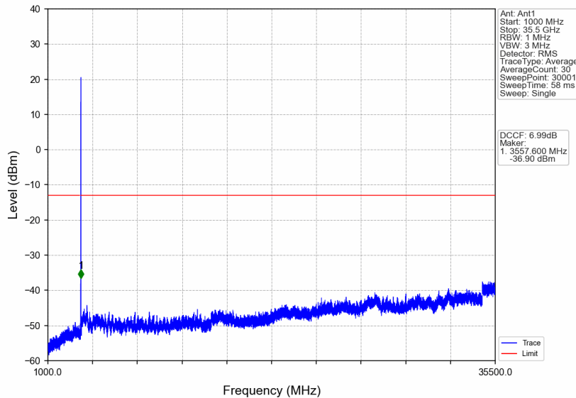
n77d_30kHz_SISO_NTNV_20MHz_CP-OFDM QPSK_3540MHz_Edge_1RB_Right
