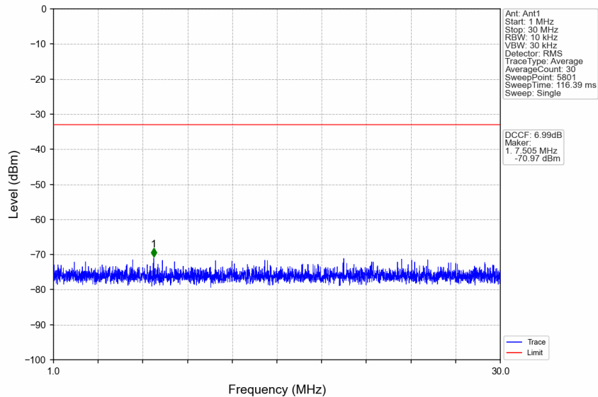
n77d_30kHz_SISO_NTNV_25MHz_DFT-s-OFDM QPSK_3537.48MHz_Edge_1RB_Right
