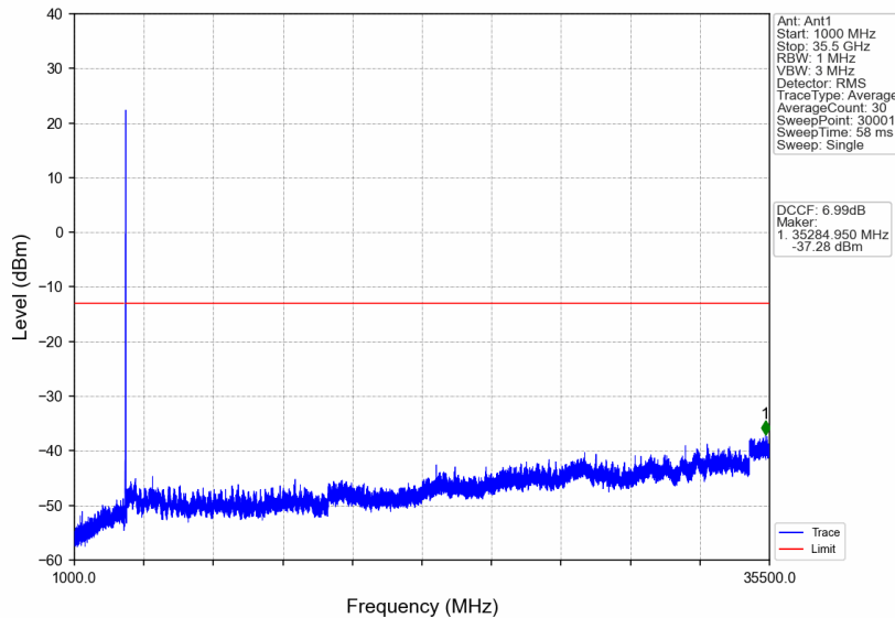
n77d_30kHz_SISO_NTNV_25MHz_CP-OFDM QPSK_3537.48MHz_Edge_1RB_Right
