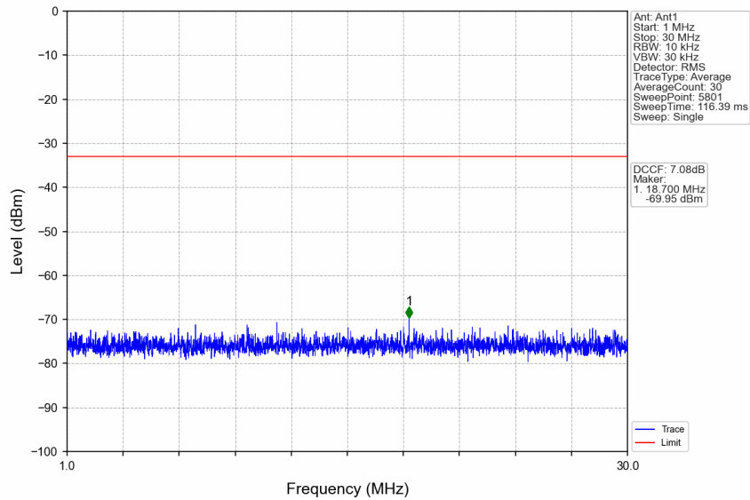
n77d_30kHz_SISO_NTNV_25MHz_CP-OFDM QPSK_3462.51MHz_Edge_1RB_Left
