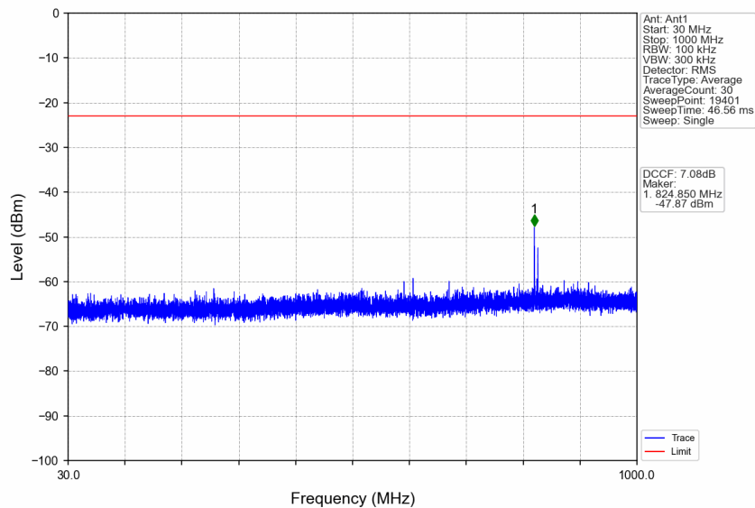
n77d_30kHz_SISO_NTNV_25MHz_DFT-s-OFDM_QPSK_3500.01MHz_Edge_1RB_Left
