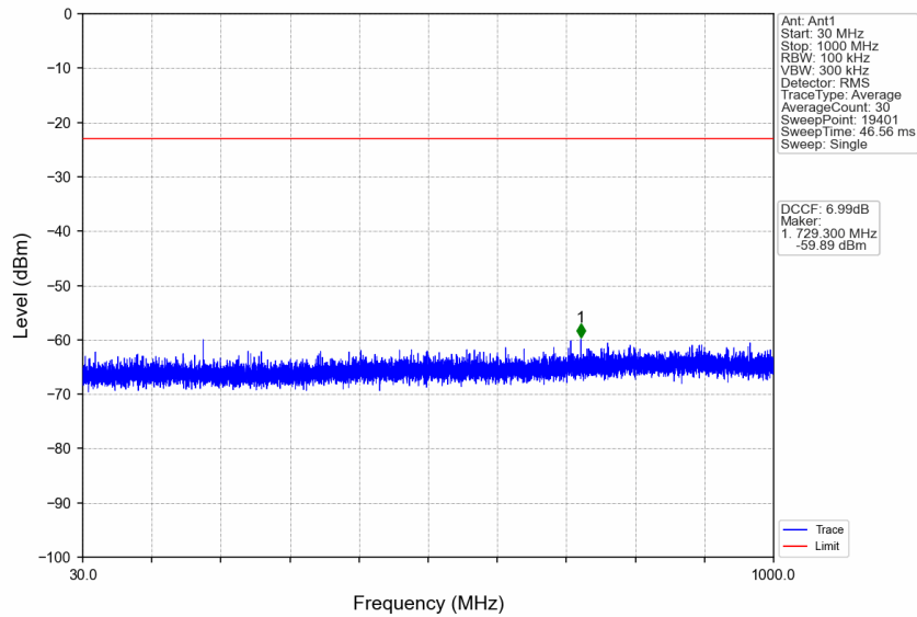
n77d_30kHz_SISO_NTNV_15MHz_DFT-s-OFDM PI/2 BPSK_3542.49MHz_Edge_1RB_Right
