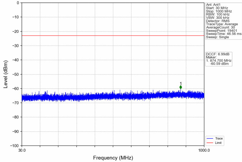
n77d_30kHz_SISO_NTNV_20MHz_DFT-s-OFDM QPSK_3540MHz_Edge_1RB_Right
