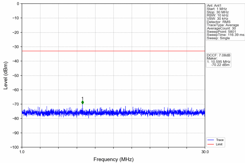
n77d_30kHz_SISO_NTNV_20MHz_DFT-s-OFDM_QPSK_3500.01MHz_Edge_1RB_Left
