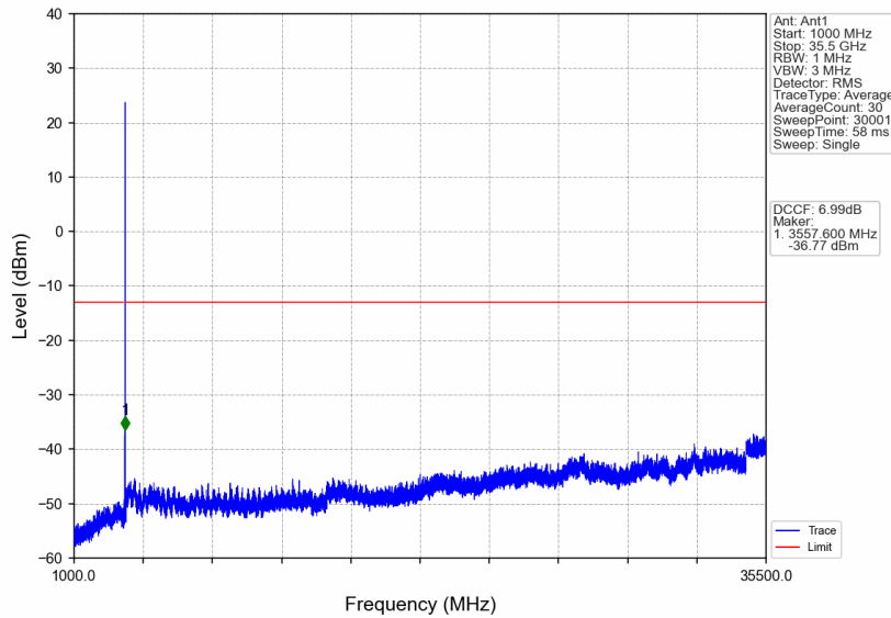
n77d_30kHz_SISO_NTNV_20MHz_DFT-s-OFDM QPSK_3540MHz_Edge_1RB_Right
