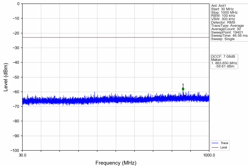
n77d_30kHz_SISO_NTNV_15MHz_CP-OFDM QPSK_3457.5MHz_Edge_1RB_Left
