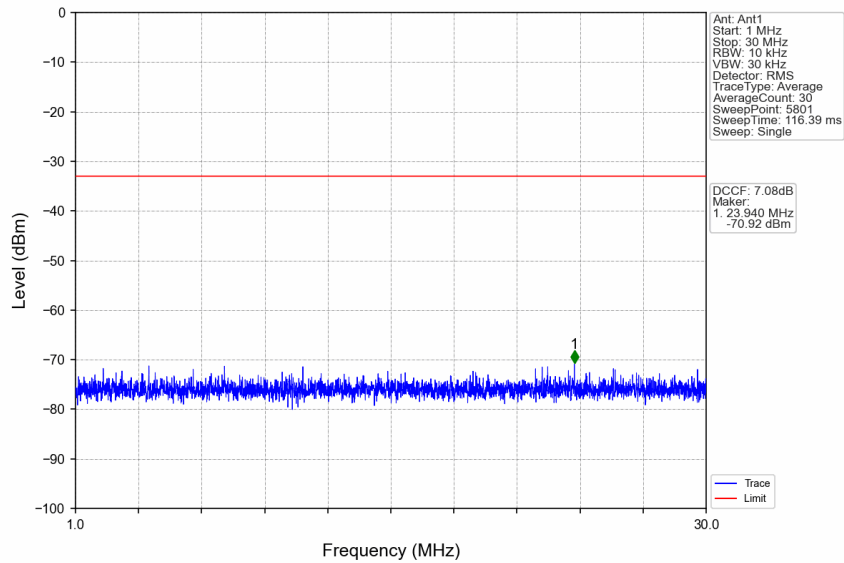
n77d_30kHz_SISO_NTNV_15MHz_CP-OFDM QPSK_3457.5MHz_Edge_1RB_Left
