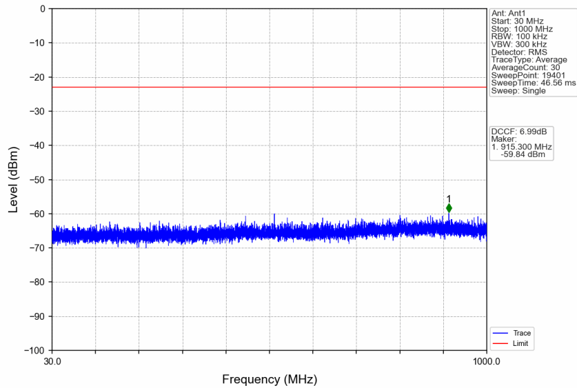
n77d_30kHz_SISO_NTNV_15MHz_CP-OFDM QPSK_3542.49MHz_Edge_1RB_Right
