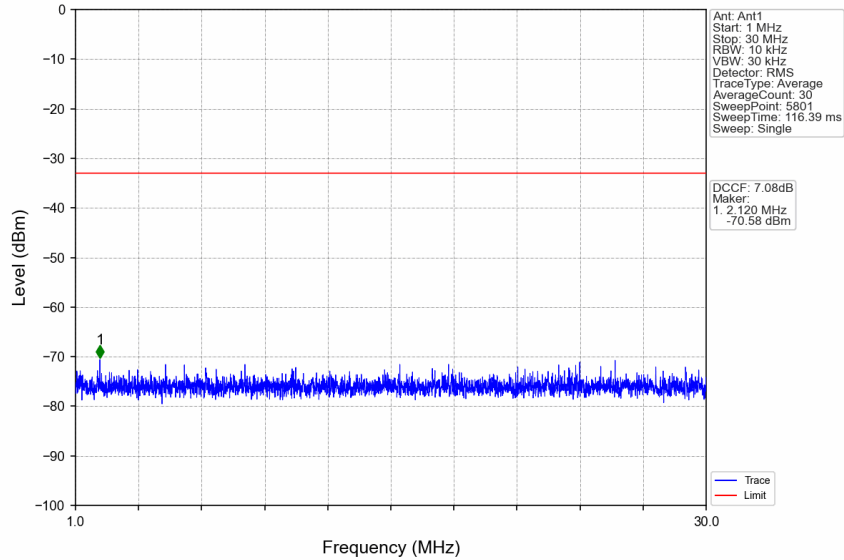
n77d_30kHz_SISO_NTNV_15MHz_CP-OFDM QPSK_3500.01MHz_Edge_1RB_Left
