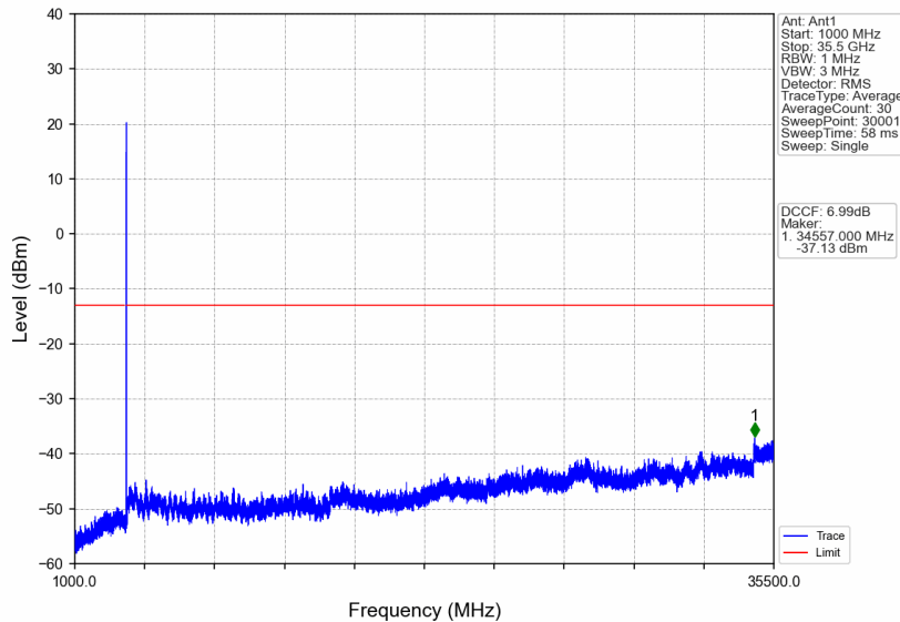
n77d_30kHz_SISO_NTNV_15MHz_DFT-s-OFDM PI/2 BPSK_3542.49MHz_Edge_1RB_Right
