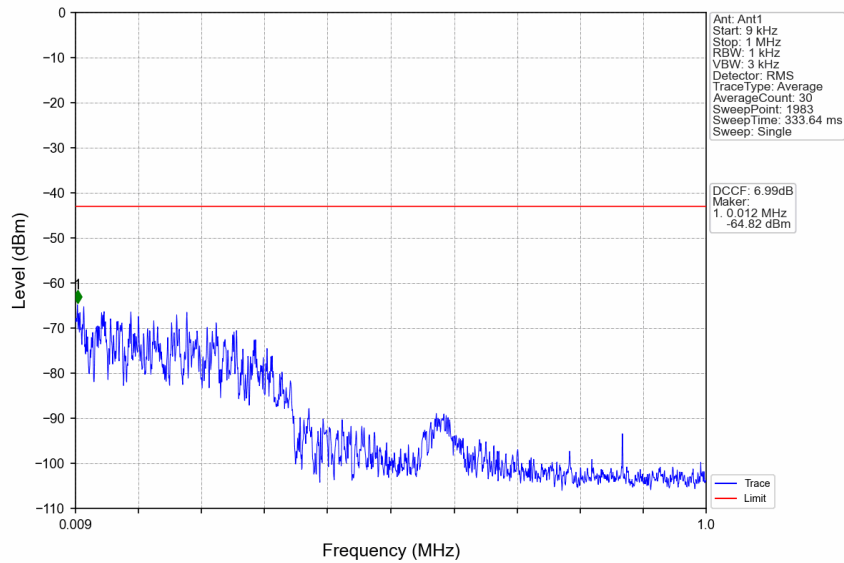
n77d_30kHz_SISO_NTNV_15MHz_CP-OFDM QPSK_3542.49MHz_Edge_1RB_Right
