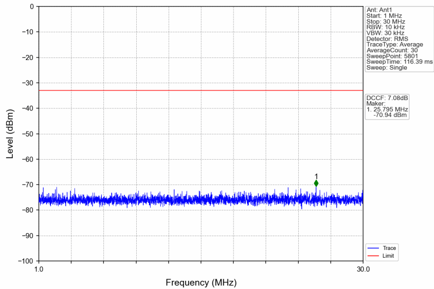
n77d_30kHz_SISO_NTNV_15MHz_DFT-s-OFDM PI/2 BPSK_3500.01MHz_Edge_1RB_Left
