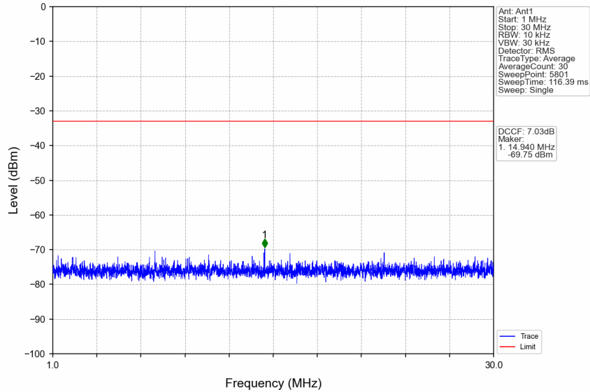
n77d_30kHz_SISO_NTNV_20MHz_DFT-s-OFDM PI/2 BPSK_3460.02MHz_Edge_1RB_Left
