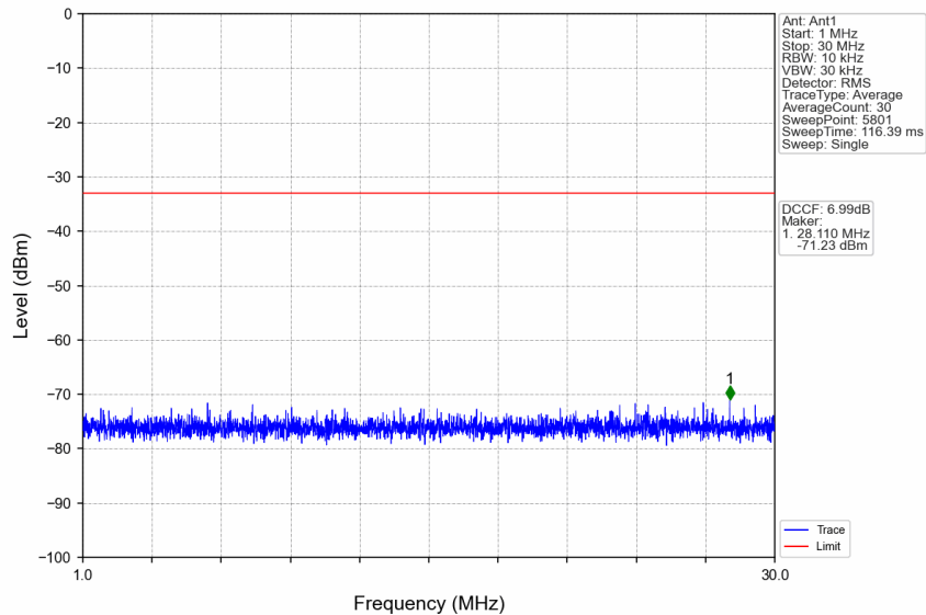
n77d_30kHz_SISO_NTNV_15MHz_CP-OFDM QPSK_3542.49MHz_Edge_1RB_Right
