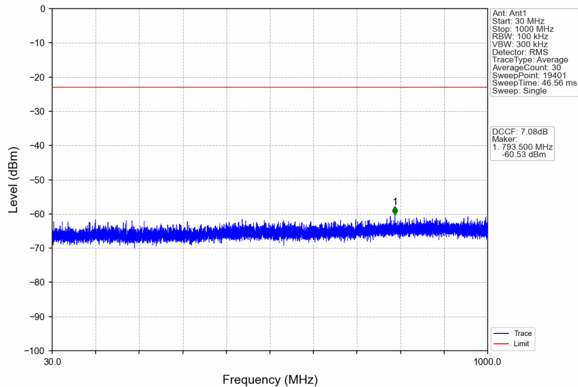
n77d_30kHz_SISO_NTNV_15MHz_CP-OFDM QPSK_3500.01MHz_Edge_1RB_Left
