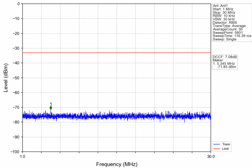
n77d_30kHz_SISO_NTNV_20MHz_DFT-s-OFDM_QPSK_3460.02MHz_Edge_1RB_Left
