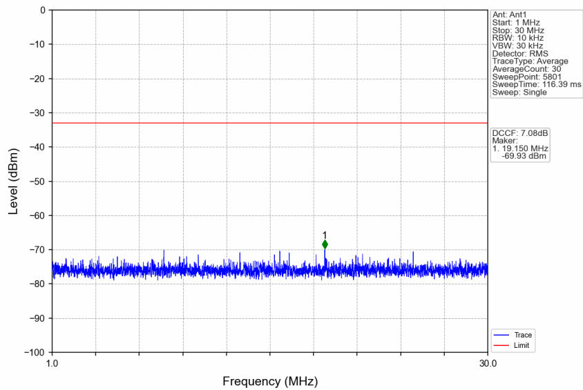
n77d_30kHz_SISO_NTNV_15MHz_DFT-s-OFDM_QPSK_3500.01MHz_Edge_1RB_Left
