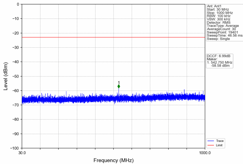
n77d_30kHz_SISO_NTNV_15MHz_DFT-s-OFDM_QPSK_3542.49MHz_Edge_1RB_Right
