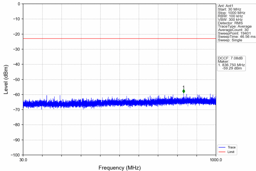
n77d_30kHz_SISO_NTNV_20MHz_DFT-s-OFDM PI/2 BPSK_3500.01MHz_Edge_1RB_Left
