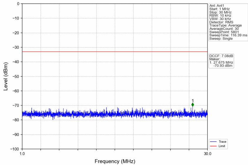
n77d_30kHz_SISO_NTNV_15MHz_DFT-s-OFDM_QPSK_3457.5MHz_Edge_1RB_Left
