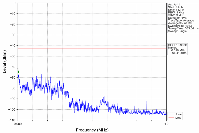
n77d_30kHz_SISO_NTNV_20MHz_DFT-s-OFDM QPSK_3540MHz_Edge_1RB_Right
