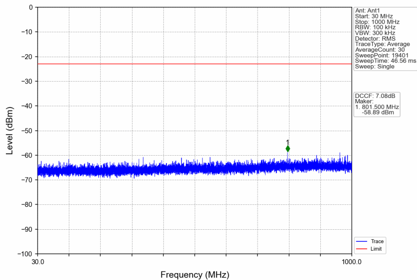
n77d_30kHz_SISO_NTNV_15MHz_DFT-s-OFDM_QPSK_3500.01MHz_Edge_1RB_Left
