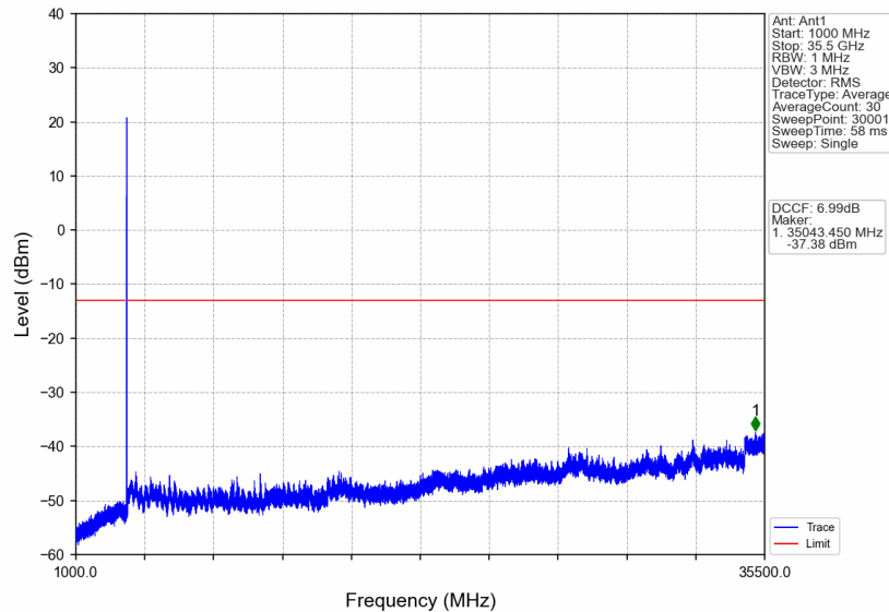
n77d_30kHz_SISO_NTNV_15MHz_CP-OFDM QPSK_3542.49MHz_Edge_1RB_Right
