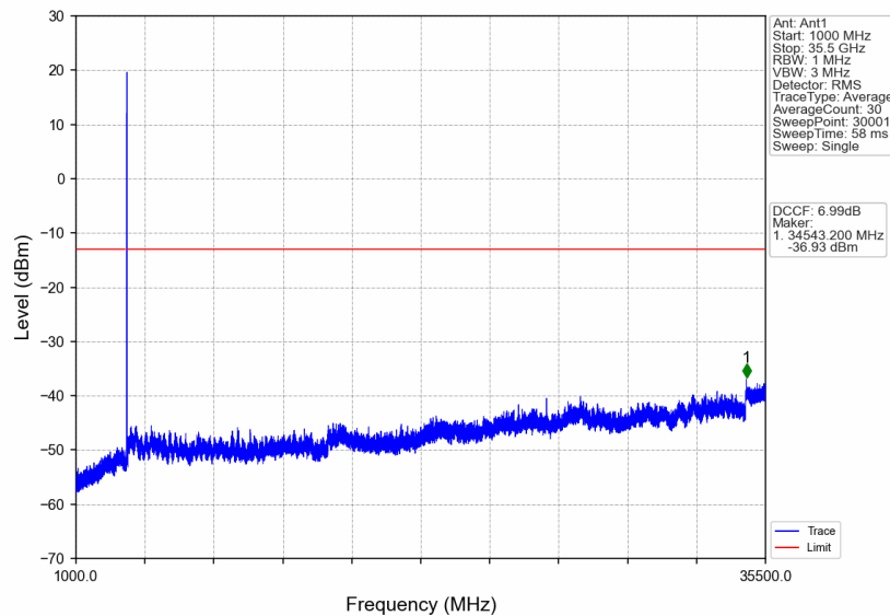
n77d_30kHz_SISO_NTNV_15MHz_DFT-s-OFDM_QPSK_3542.49MHz_Edge_1RB_Right
