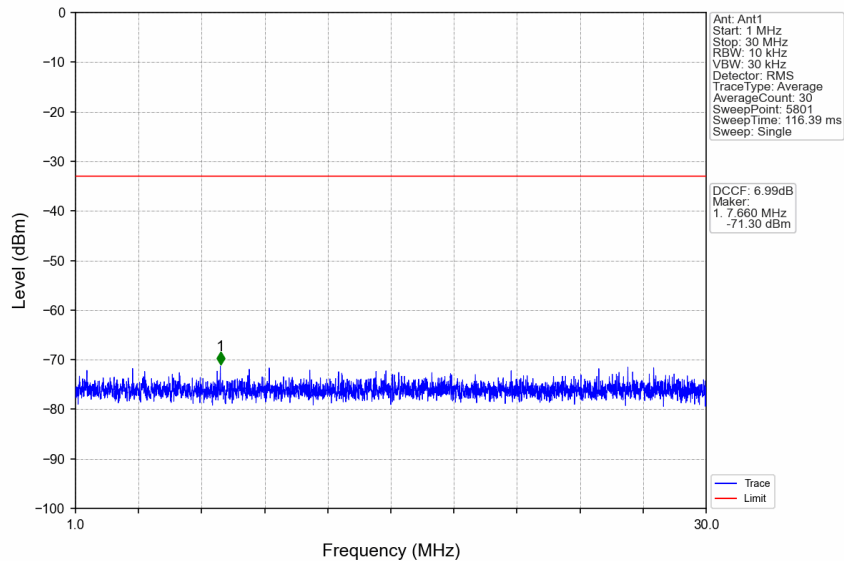
n77d_30kHz_SISO_NTNV_20MHz_DFT-s-OFDM QPSK_3540MHz_Edge_1RB_Right
