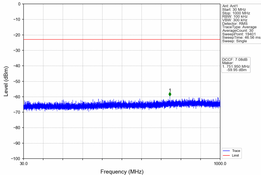
n77d_30kHz_SISO_NTNV_20MHz_DFT-s-OFDM_QPSK_3460.02MHz_Edge_1RB_Left
