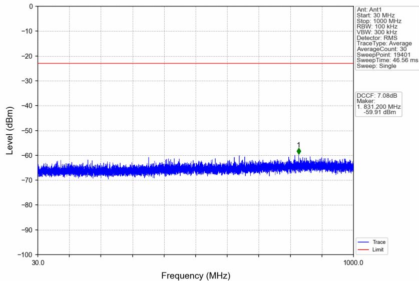
n77d_30kHz_SISO_NTNV_20MHz_DFT-s-OFDM_QPSK_3500.01MHz_Edge_1RB_Left
