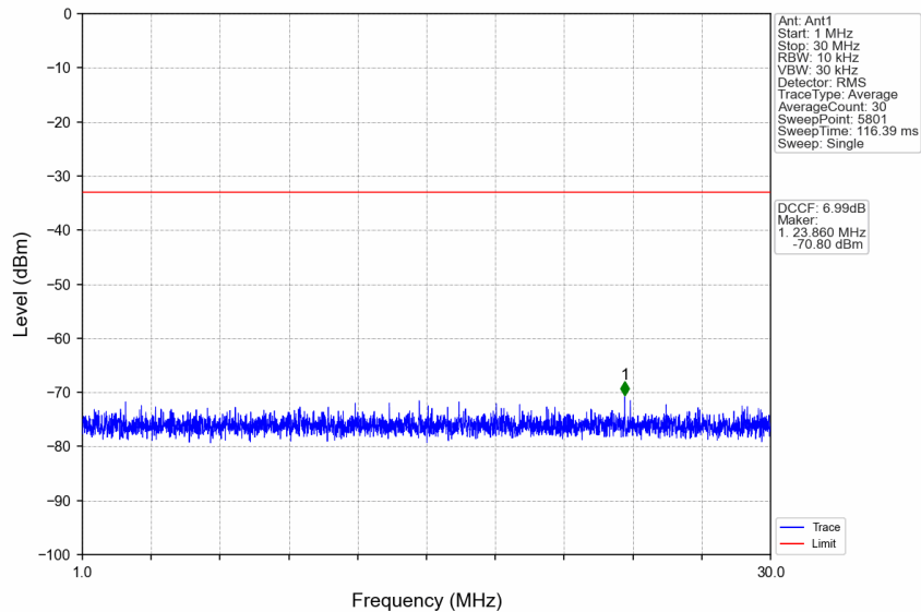
n77d_30kHz_SISO_NTNV_15MHz_DFT-s-OFDM QPSK_3542.49MHz_Edge_1RB_Right
