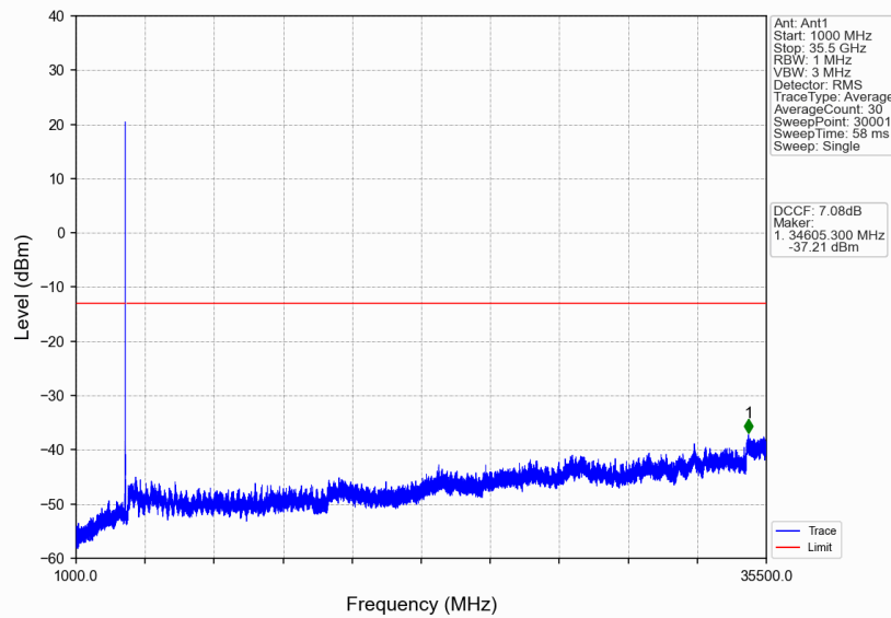
n77d_30kHz_SISO_NTNV_15MHz_CP-OFDM QPSK_3457.5MHz_Outer_Full
