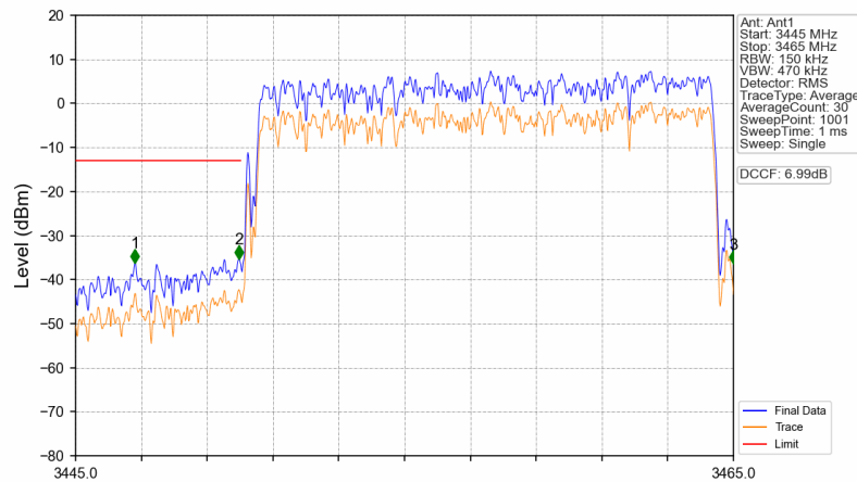
n77d_30kHz_SISO_NTNV_15MHz_CP-OFDM QPSK_3457.5MHz_Outer_Full
