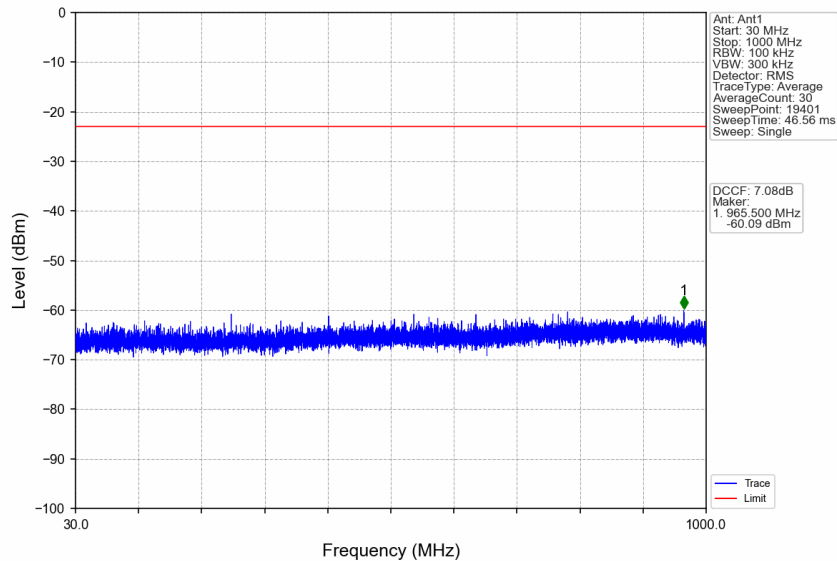
n77d_30kHz_SISO_NTNV_15MHz_DFT-s-OFDM_QPSK_3457.5MHz_Edge_1RB_Left
