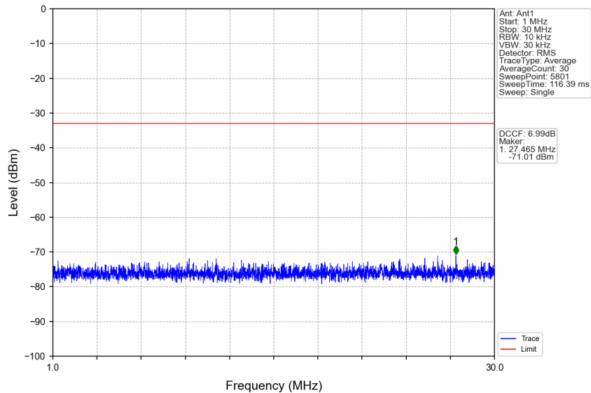
n77d_30kHz_SISO_NTNV_10MHz_DFT-s-OFDM QPSK_3544.98MHz_Edge_1RB_Right
