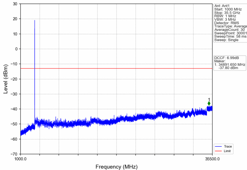
n77d_30kHz_SISO_NTNV_10MHz_CP-OFDM QPSK_3544.98MHz_Edge_1RB_Right
