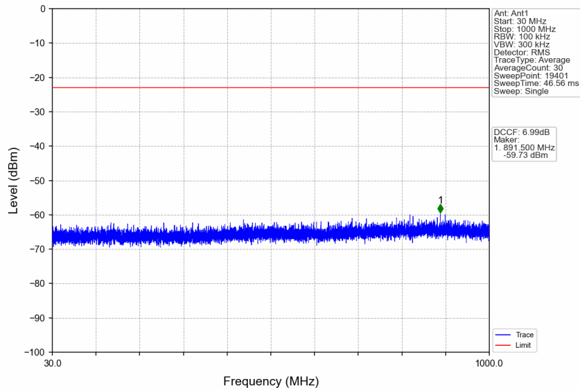
n77d_30kHz_SISO_NTNV_10MHz_CP-OFDM QPSK_3544.98MHz_Edge_1RB_Right
