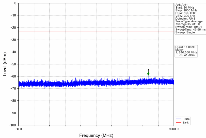
n77d_30kHz_SISO_NTNV_10MHz_DFT-s-OFDM_QPSK_3500.01MHz_Edge_1RB_Left
