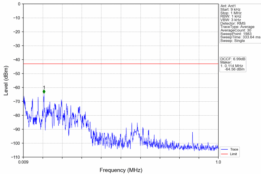
n77d_30kHz_SISO_NTNV_10MHz_DFT-s-OFDM QPSK_3544.98MHz_Edge_1RB_Right
