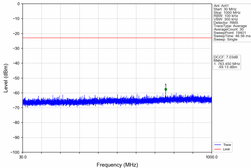
n77d_30kHz_SISO_NTNV_10MHz_CP-OFDM QPSK_3500.01MHz_Edge_1RB_Left
