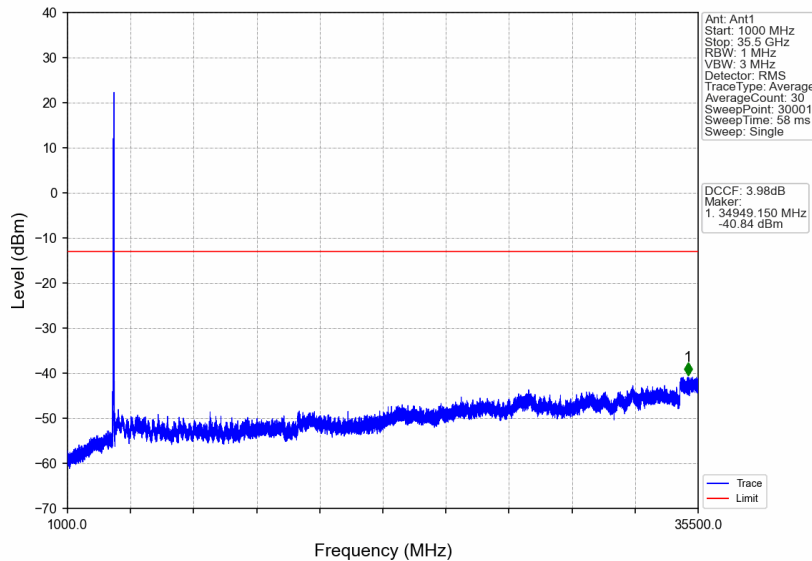
n77d_15kHz_SISO_NTNV_50MHz_CP-OFDM QPSK_3525MHz_Edge_1RB_Right
