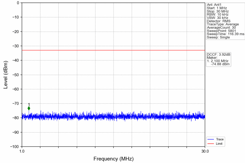
n77d_15kHz_SISO_NTNV_50MHz_CP-OFDM QPSK_3499.995MHz_Edge_1RB_Left
