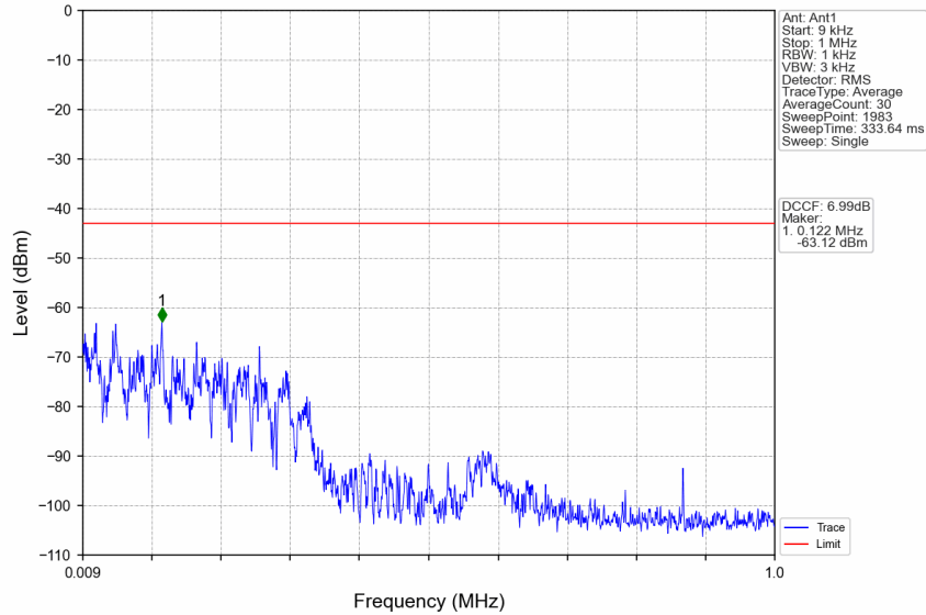
n77d_30kHz_SISO_NTNV_10MHz_CP-OFDM QPSK_3544.98MHz_Edge_1RB_Right
