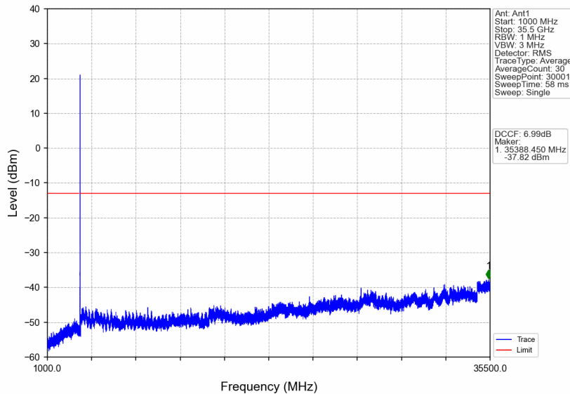
n77d_30kHz_SISO_NTNV_10MHz_DFT-s-OFDM QPSK_3544.98MHz_Edge_1RB_Right
