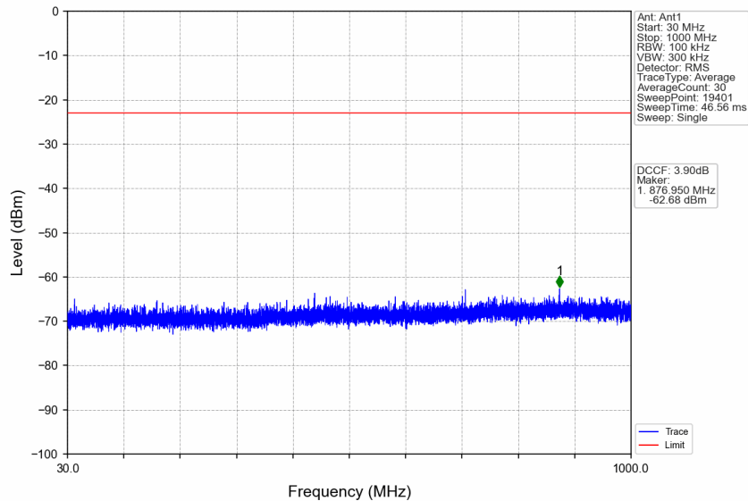
n77d_15kHz_SISO_NTNV_50MHz_CP-OFDM QPSK_3475.005MHz_Edge_1RB_Left
