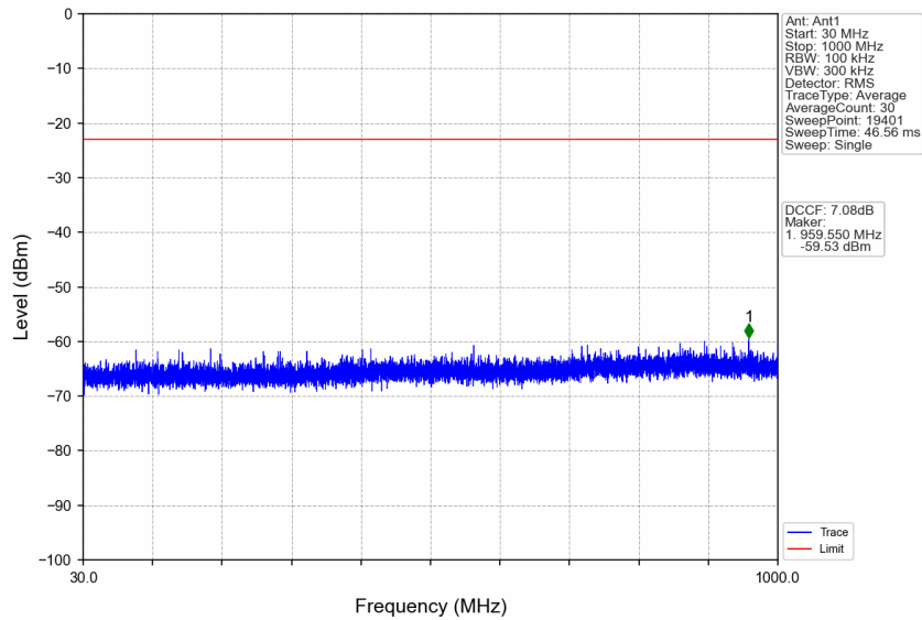
n77d_30kHz_SISO_NTNV_10MHz_CP-OFDM QPSK_3455.01MHz_Edge_1RB_Left
