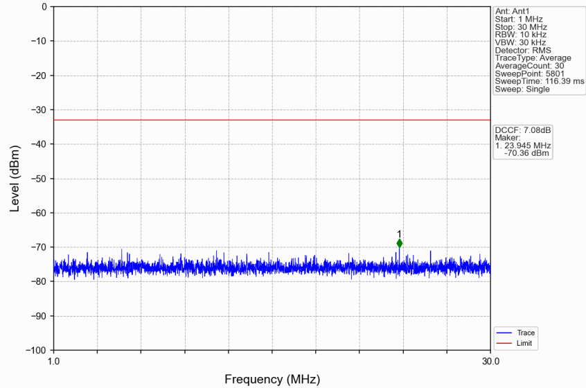
n77d_30kHz_SISO_NTNV_10MHz_DFT-s-OFDM_QPSK_3455.01MHz_Edge_1RB_Left
