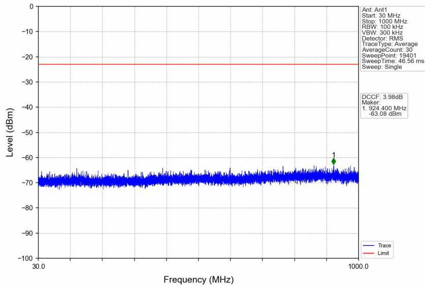
n77d_15kHz_SISO_NTNV_50MHz_CP-OFDM QPSK_3525MHz_Edge_1RB_Right
