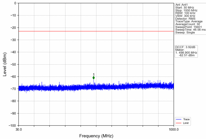
n77d_15kHz_SISO_NTNV_50MHz_CP-OFDM QPSK_3499.995MHz_Edge_1RB_Left
