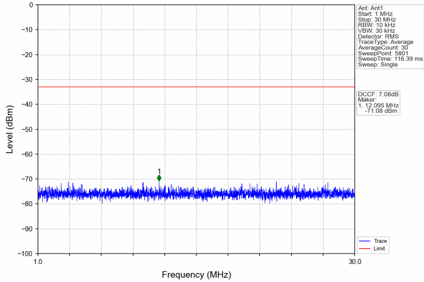
n77d_30kHz_SISO_NTNV_10MHz_CP-OFDM QPSK_3455.01MHz_Edge_1RB_Left
