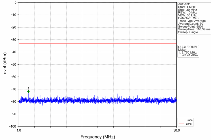
n77d_15kHz_SISO_NTNV_50MHz_CP-OFDM QPSK_3475.005MHz_Edge_1RB_Left
