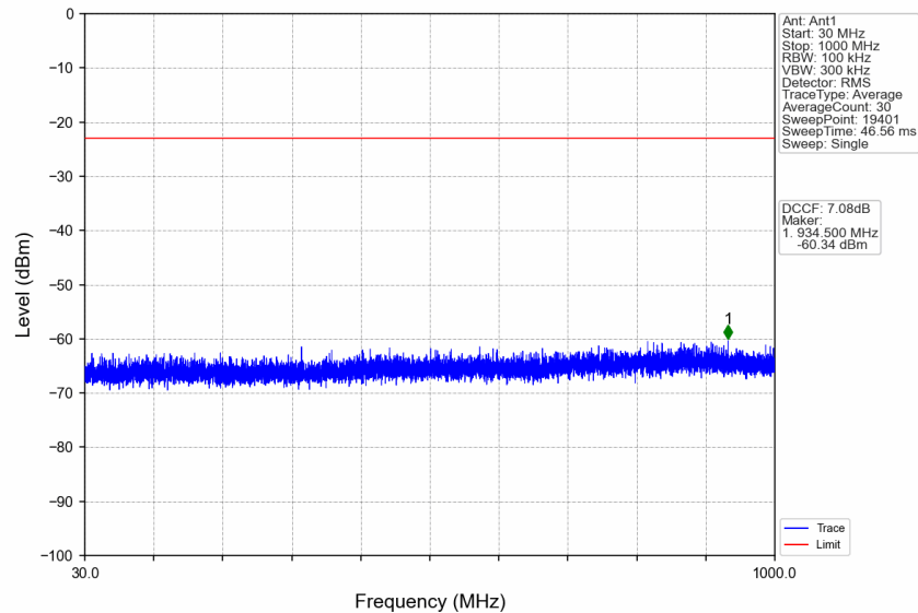
n77d_30kHz_SISO_NTNV_10MHz_DFT-s-OFDM_QPSK_3455.01MHz_Edge_1RB_Left
