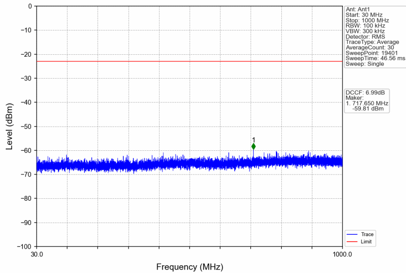
n77d_30kHz_SISO_NTNV_10MHz_DFT-s-OFDM QPSK_3544.98MHz_Edge_1RB_Right
