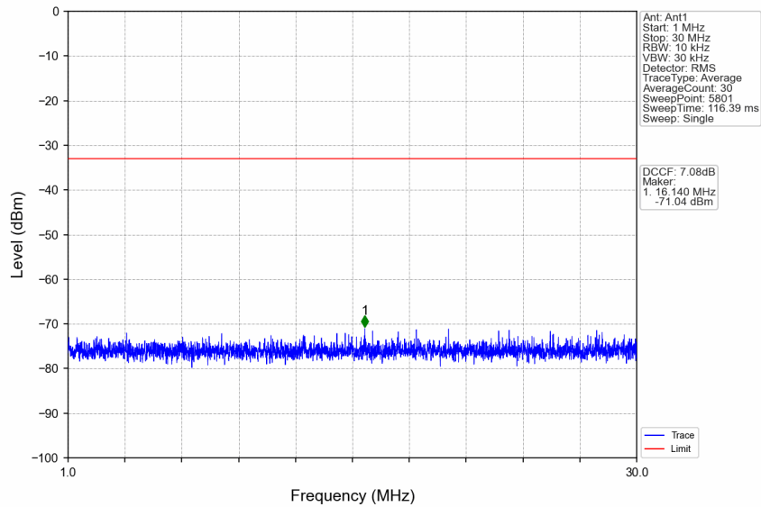
n77d_30kHz_SISO_NTNV_10MHz_DFT-s-OFDM_QPSK_3500.01MHz_Edge_1RB_Left
