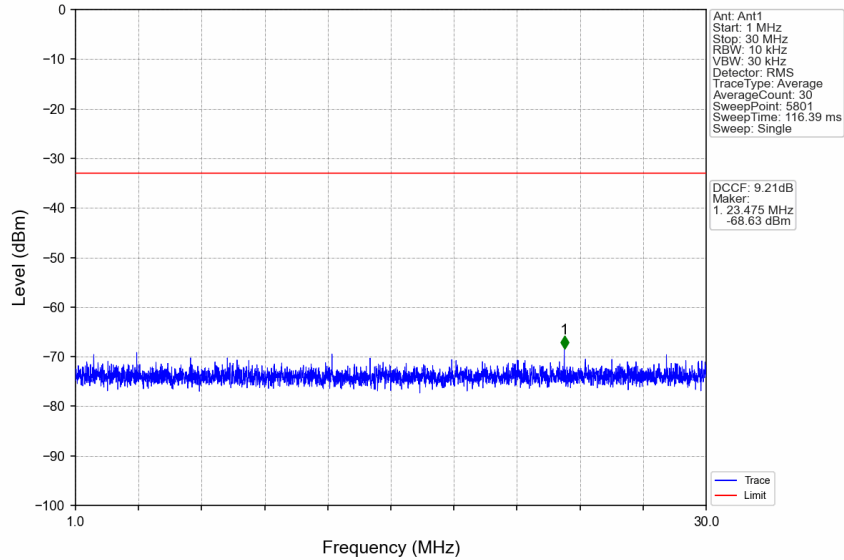
n77d_15kHz_SISO_NTNV_25MHz_CP-OFDM QPSK_3499.995MHz_Edge_1RB_Left
