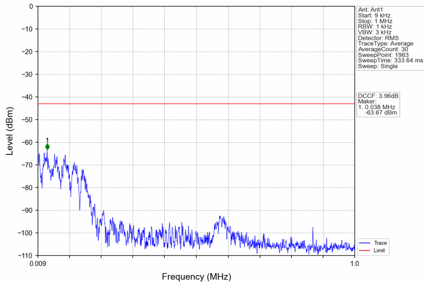
n77d_15kHz_SISO_NTNV_30MHz_CP-OFDM QPSK_3534.99MHz_Edge_1RB_Right
