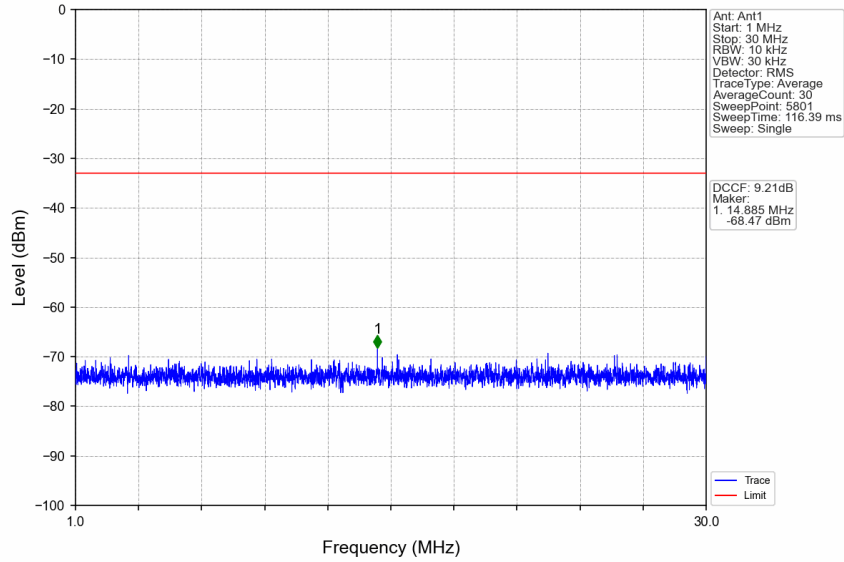
n77d_15kHz_SISO_NTNV_30MHz_DFT-s-OFDM_QPSK_3465MHz_Edge_1RB_Left
