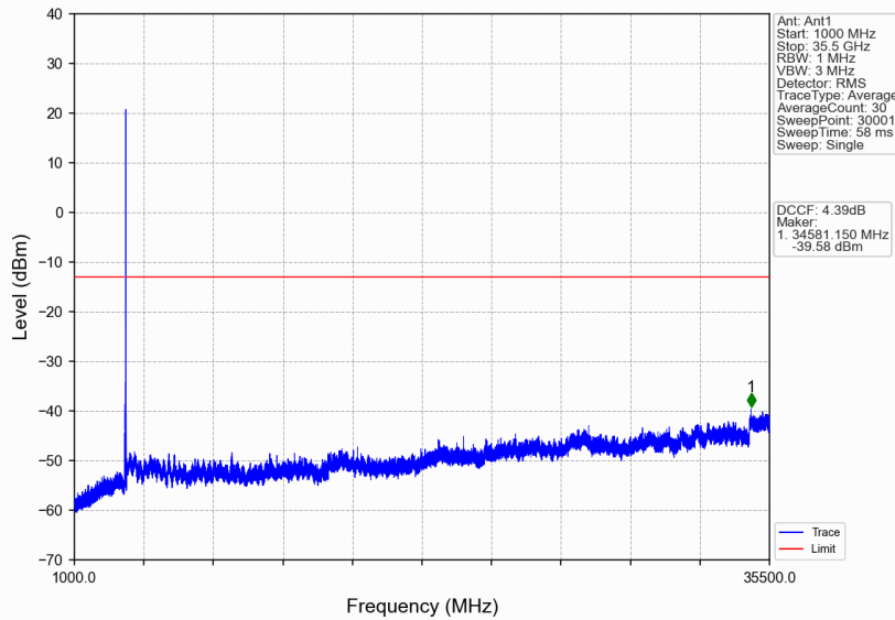
n77d_15kHz_SISO_NTNV_30MHz_DFT-s-OFDM QPSK_3534.99MHz_Edge_1RB_Right
