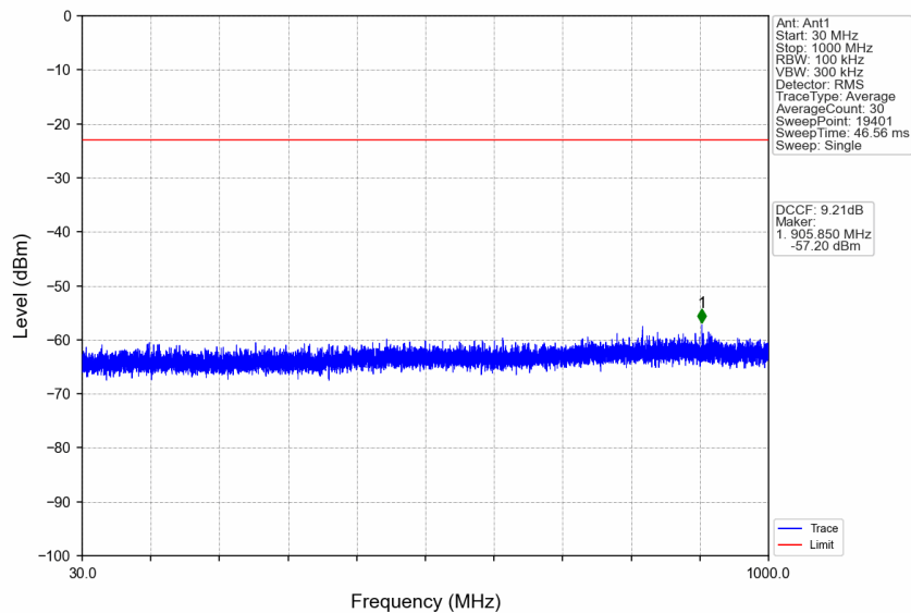
n77d_15kHz_SISO_NTNV_30MHz_DFT-s-OFDM QPSK_3499.995MHz_Edge_1RB_Left
