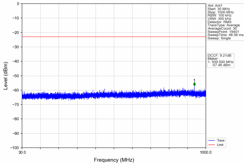
n77d_15kHz_SISO_NTNV_25MHz_CP-OFDM QPSK_3499.995MHz_Edge_1RB_Left
