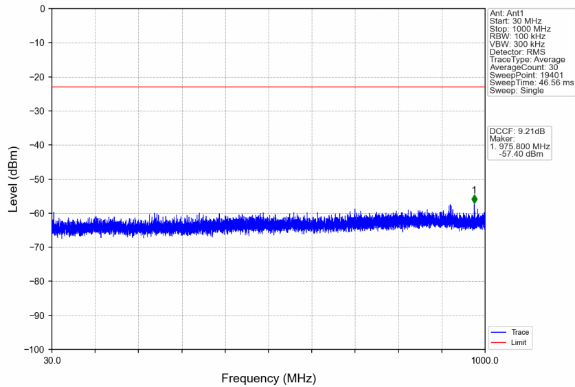
n77d_15kHz_SISO_NTNV_30MHz_CP-OFDM QPSK_3499.995MHz_Edge_1RB_Left
