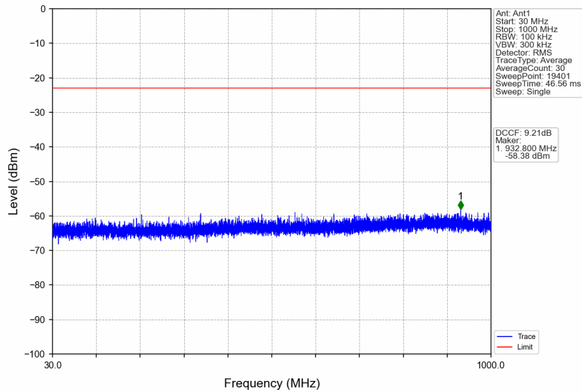
n77d_15kHz_SISO_NTNV_30MHz_DFT-s-OFDM_QPSK_3465MHz_Edge_1RB_Left
