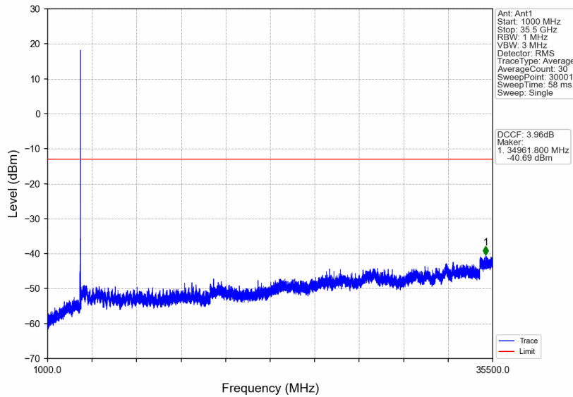
n77d_15kHz_SISO_NTNV_30MHz_CP-OFDM QPSK_3534.99MHz_Edge_1RB_Right
