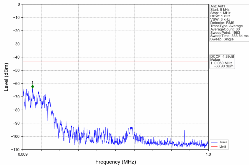
n77d_15kHz_SISO_NTNV_25MHz_CP-OFDM QPSK_3537.495MHz_Edge_1RB_Right
