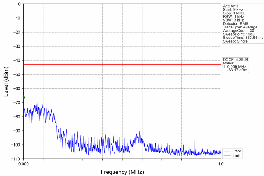
n77d_15kHz_SISO_NTNV_30MHz_DFT-s-OFDM QPSK_3534.99MHz_Edge_1RB_Right
