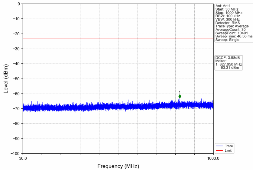
n77d_15kHz_SISO_NTNV_30MHz_DFT-s-OFDM PI/2 BPSK_3534.99MHz_Edge_1RB_Right
