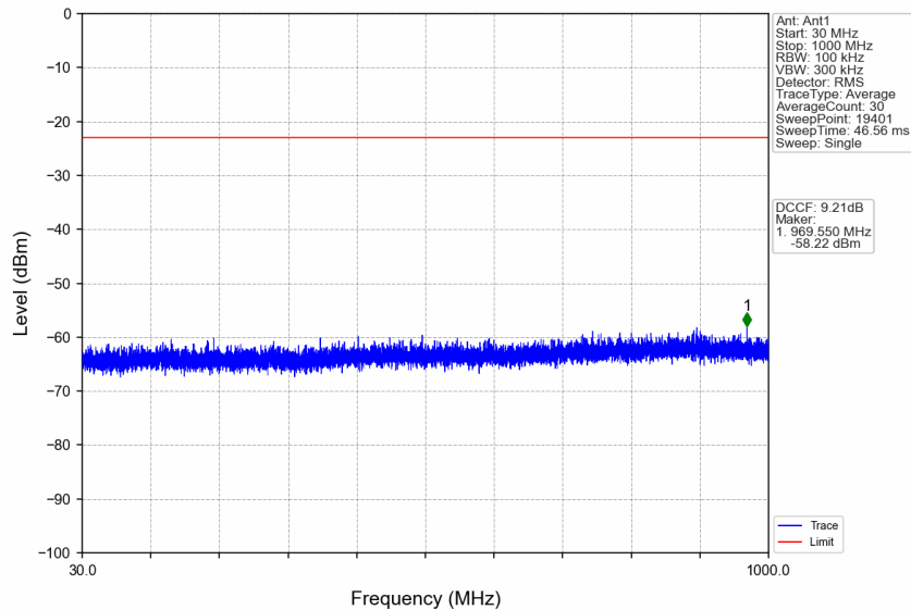
n77d_15kHz_SISO_NTNV_30MHz_DFT-s-OFDM PI/2 BPSK_3465MHz_Edge_1RB_Left
