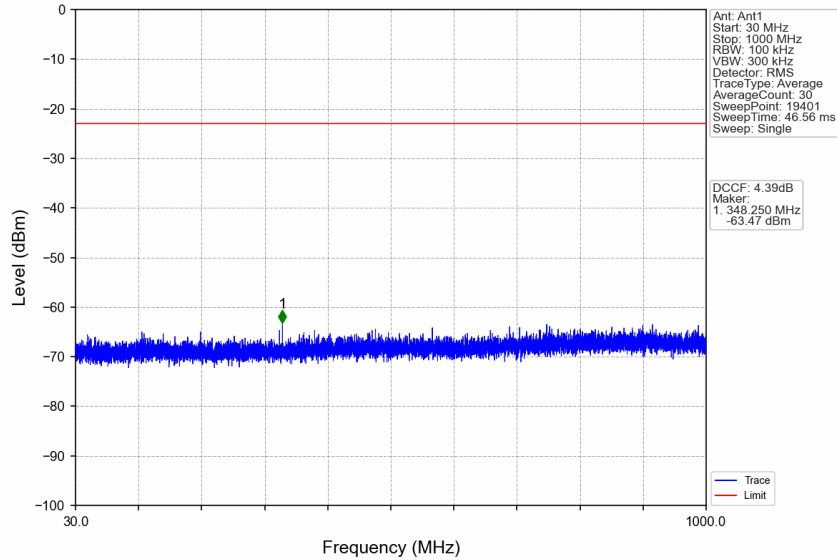
n77d_15kHz_SISO_NTNV_25MHz_CP-OFDM QPSK_3537.495MHz_Edge_1RB_Right
