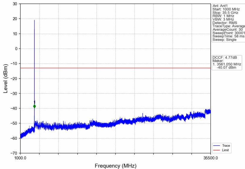
n77d_15kHz_SISO_NTNV_25MHz_DFT-s-OFDM_QPSK_3537.495MHz_Edge_1RB_Right
