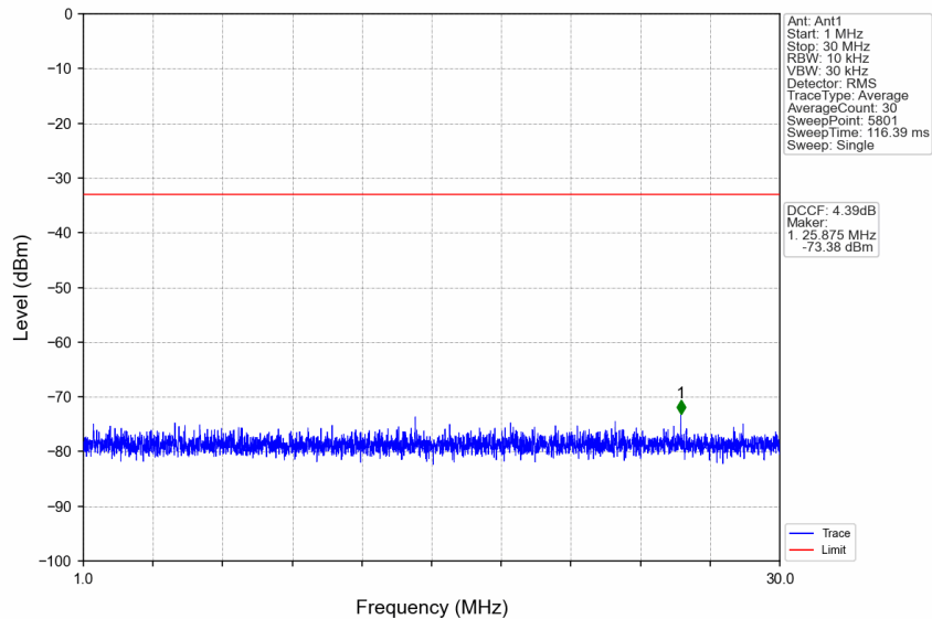
n77d_15kHz_SISO_NTNV_30MHz_DFT-s-OFDM QPSK_3534.99MHz_Edge_1RB_Right
