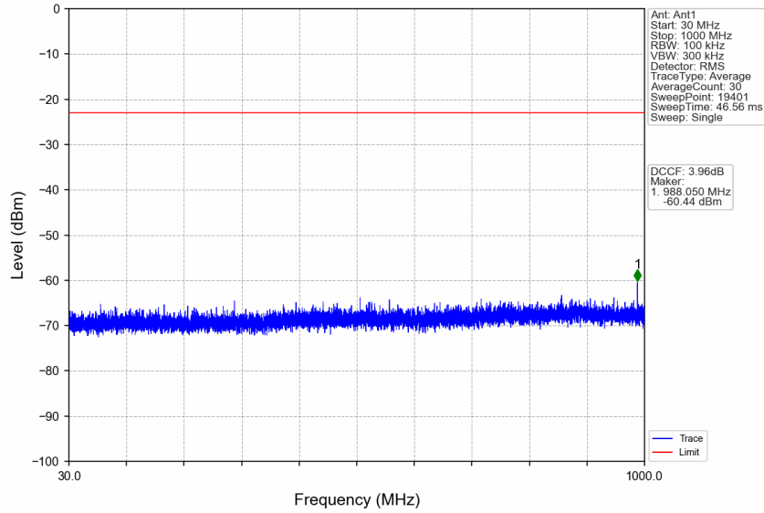
n77d_15kHz_SISO_NTNV_30MHz_CP-OFDM QPSK_3534.99MHz_Edge_1RB_Right
