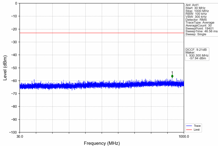
n77d_15kHz_SISO_NTNV_30MHz_CP-OFDM QPSK_3465MHz_Edge_1RB_Left
