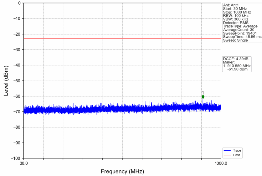
n77d_15kHz_SISO_NTNV_30MHz_DFT-s-OFDM QPSK_3534.99MHz_Edge_1RB_Right
