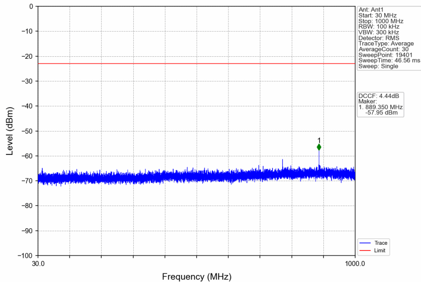
n77d_15kHz_SISO_NTNV_25MHz_CP-OFDM QPSK_3462.51MHz_Edge_1RB_Left
