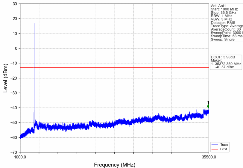
n77d_15kHz_SISO_NTNV_30MHz_DFT-s-OFDM PI/2 BPSK_3534.99MHz_Edge_1RB_Right
