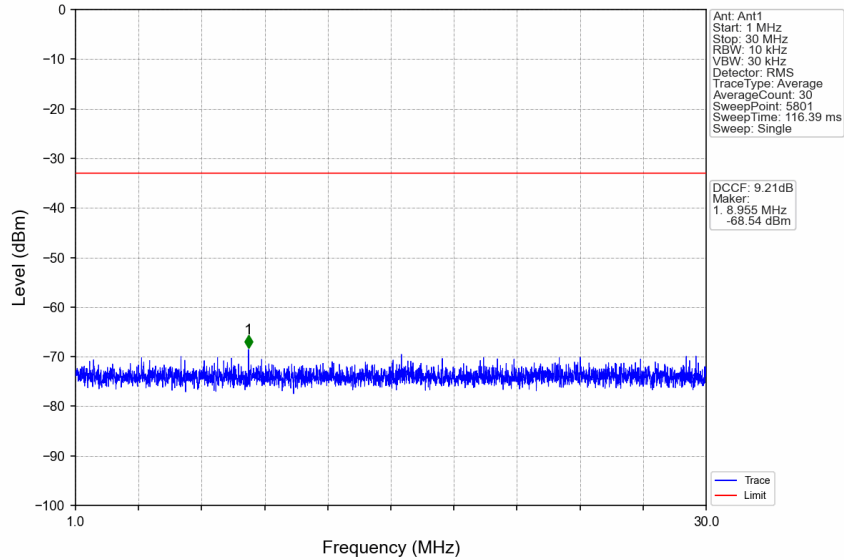
n77d_15kHz_SISO_NTNV_30MHz_CP-OFDM QPSK_3465MHz_Edge_1RB_Left
