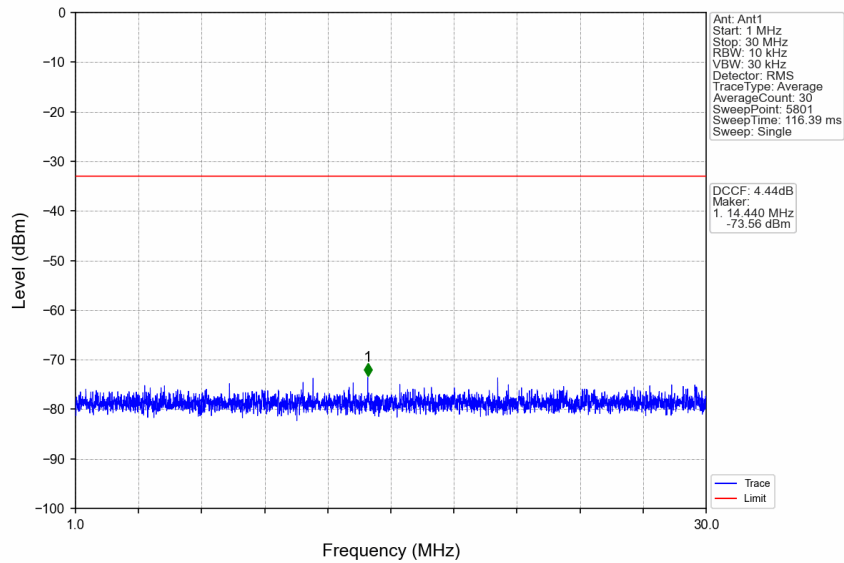
n77d_15kHz_SISO_NTNV_25MHz_CP-OFDM QPSK_3462.51MHz_Edge_1RB_Left
