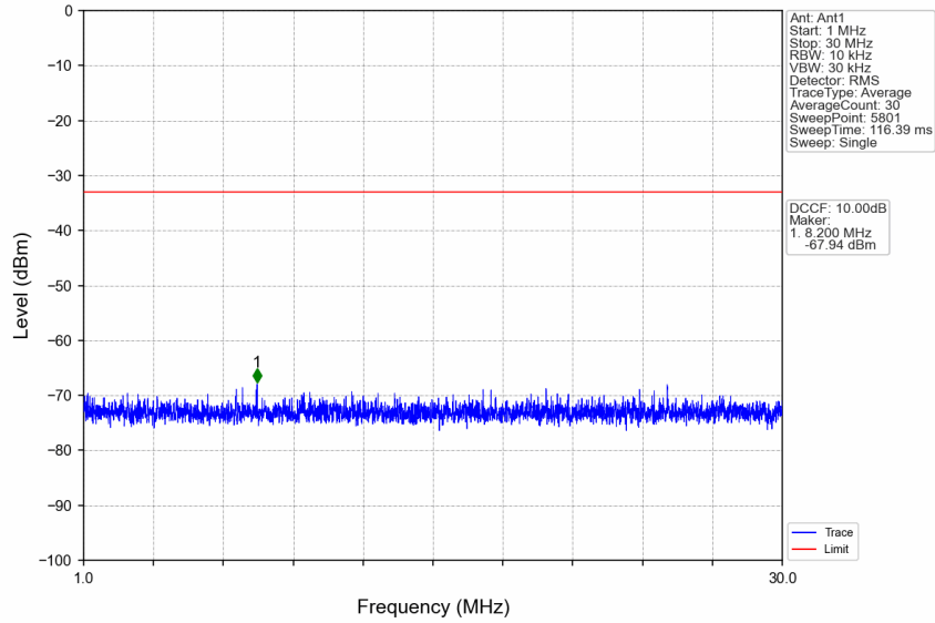
n77d_15kHz_SISO_NTNV_40MHz_DFT-s-OFDM PI/2 BPSK_3470.01MHz_Edge_1RB_Left
