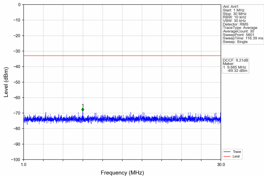
n77d_15kHz_SISO_NTNV_30MHz_DFT-s-OFDM QPSK_3499.995MHz_Edge_1RB_Left
