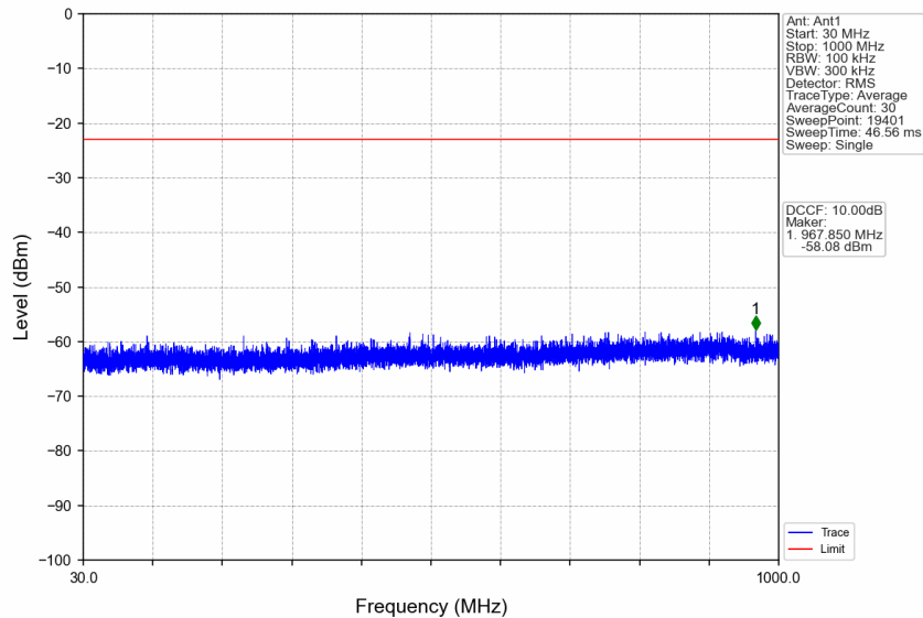
n77d_15kHz_SISO_NTNV_30MHz_DFT-s-OFDM PI/2 BPSK_3499.995MHz_Edge_1RB_Left
