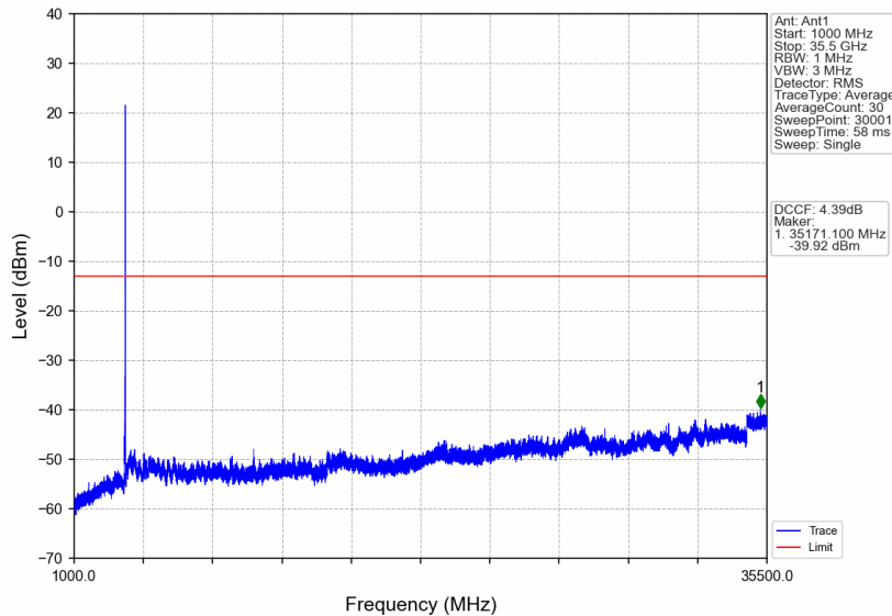
n77d_15kHz_SISO_NTNV_25MHz_CP-OFDM QPSK_3537.495MHz_Edge_1RB_Right
