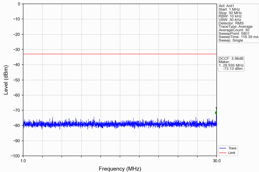
n77d_15kHz_SISO_NTNV_30MHz_CP-OFDM QPSK_3534.99MHz_Edge_1RB_Right
