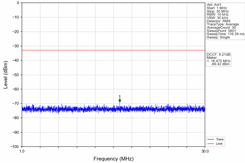
n77d_15kHz_SISO_NTNV_30MHz_CP-OFDM QPSK_3499.995MHz_Edge_1RB_Left
