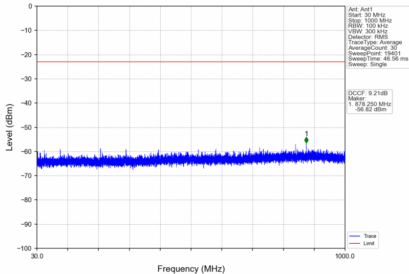
n77d_15kHz_SISO_NTNV_20MHz_DFT-s-OFDM QPSK_3499.995MHz_Edge_1RB_Left
