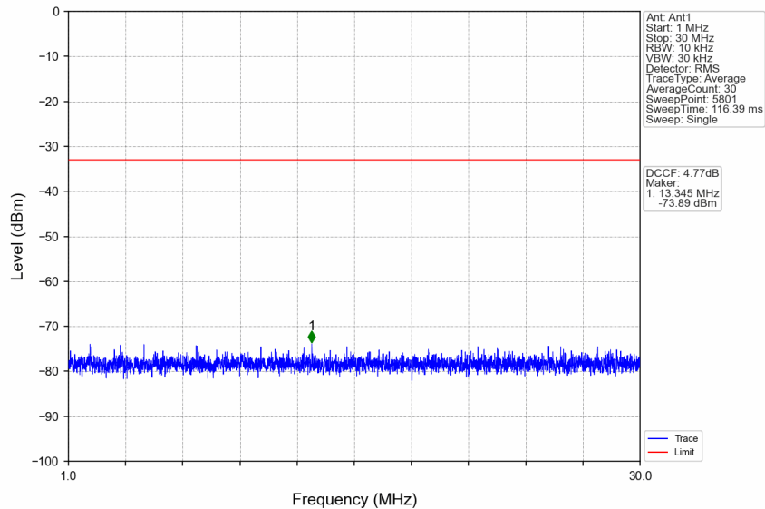
n77d_15kHz_SISO_NTNV_25MHz_DFT-s-OFDM QPSK_3537.495MHz_Edge_1RB_Right
