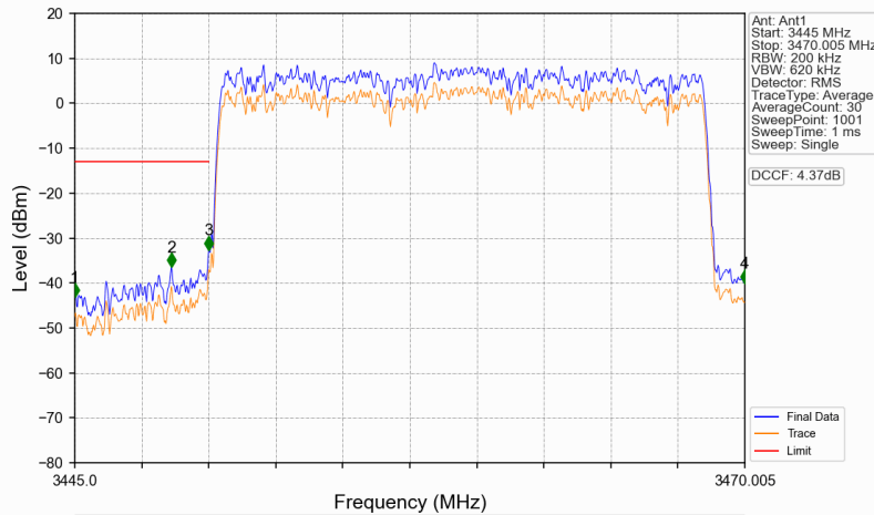
n77d_15kHz_SISO_NTNV_20MHz_DFT-s-OFDM QPSK_3460.005MHz_Outer_Full
