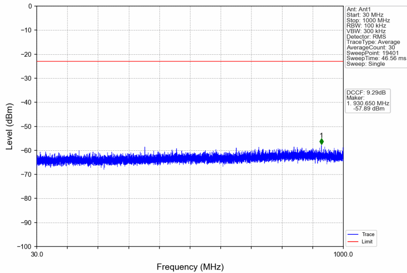
n77d_15kHz_SISO_NTNV_20MHz_CP-OFDM QPSK_3460.005MHz_Edge_1RB_Left
