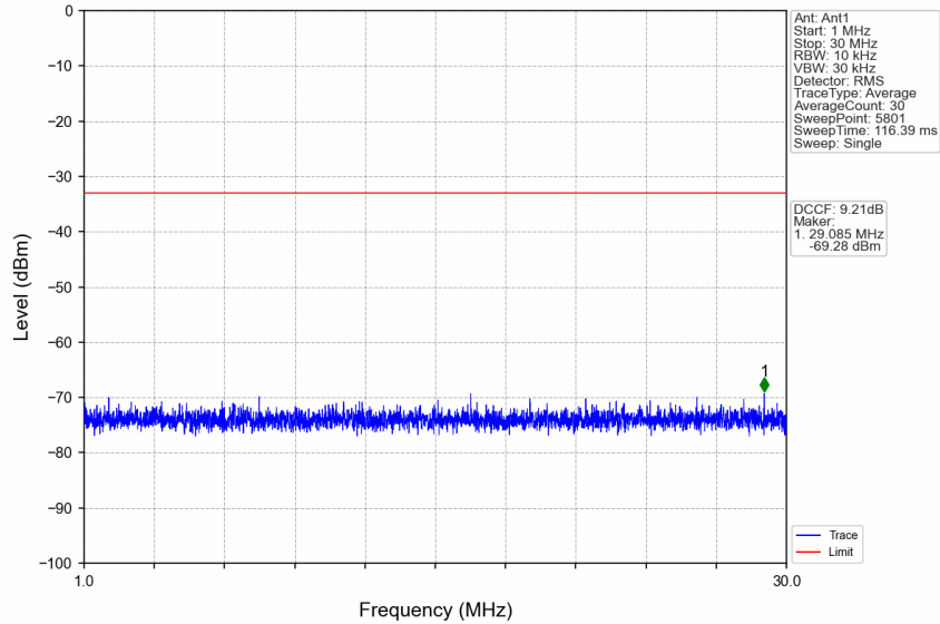
n77d_15kHz_SISO_NTNV_25MHz_DFT-s-OFDM_QPSK_3462.51MHz_Edge_1RB_Left
