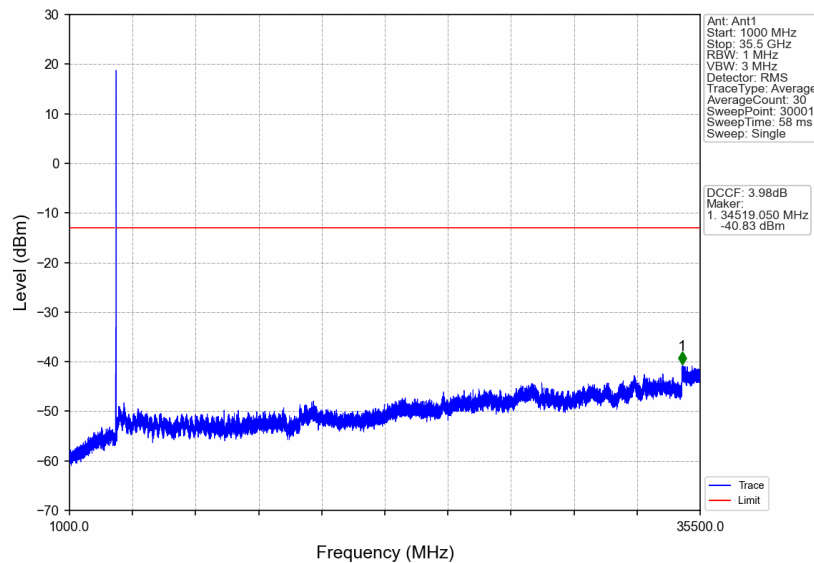
n77d_15kHz_SISO_NTNV_20MHz_DFT-s-OFDM QPSK_3540MHz_Edge_1RB_Right
