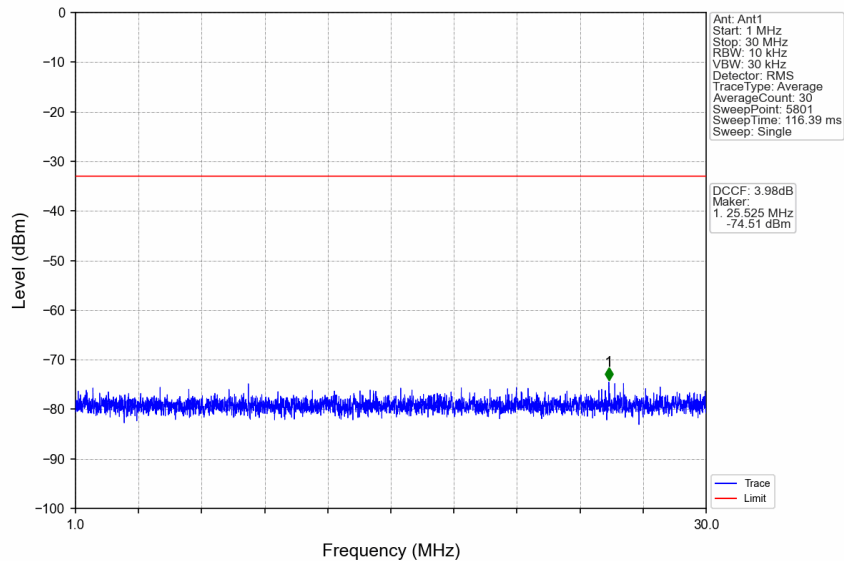
n77d_15kHz_SISO_NTNV_20MHz_DFT-s-OFDM QPSK_3540MHz_Edge_1RB_Right
