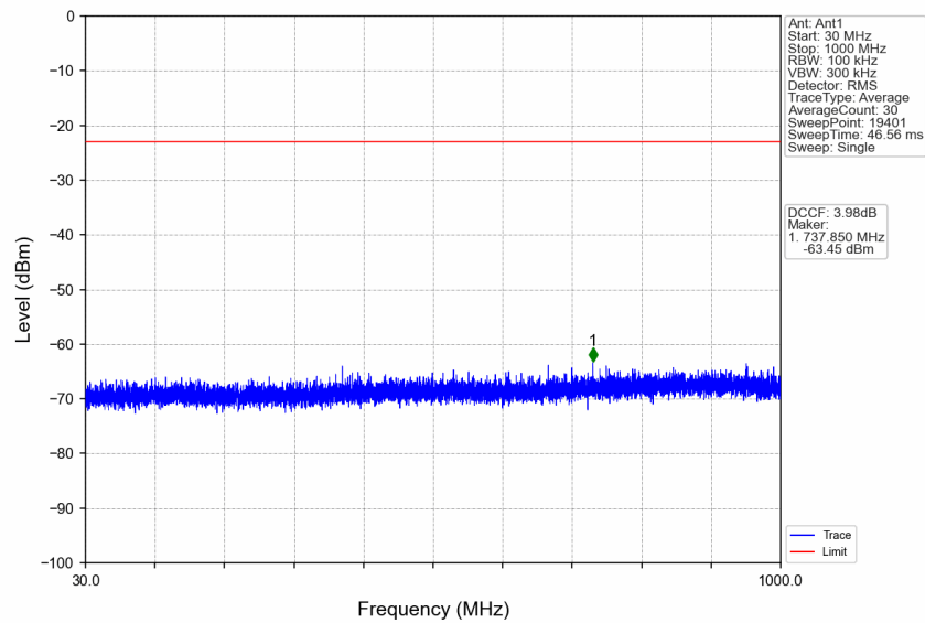
n77d_15kHz_SISO_NTNV_20MHz_DFT-s-OFDM QPSK_3540MHz_Edge_1RB_Right
