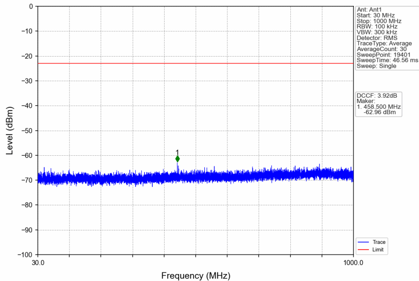
n77d_15kHz_SISO_NTNV_25MHz_DFT-s-OFDM QPSK_3499.995MHz_Edge_1RB_Left
