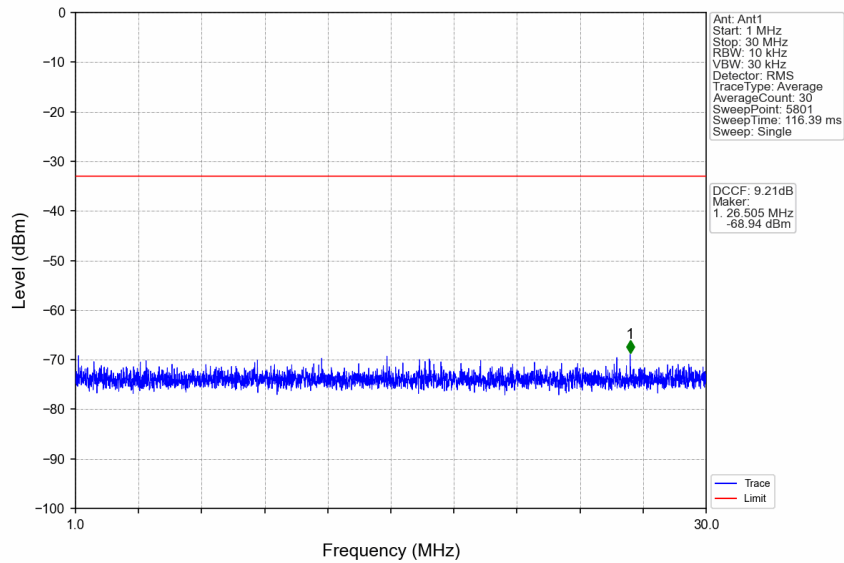
n77d_15kHz_SISO_NTNV_20MHz_DFT-s-OFDM QPSK_3460.005MHz_Edge_1RB_Left
