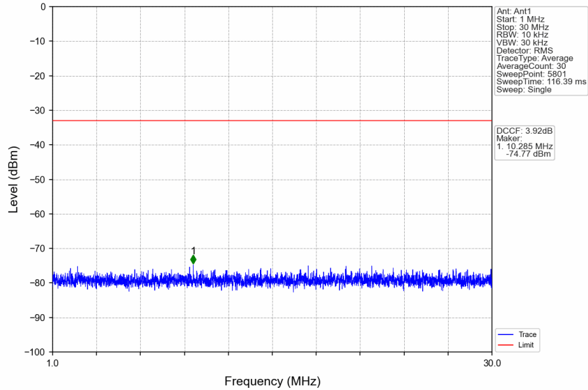
n77d_15kHz_SISO_NTNV_25MHz_DFT-s-OFDM QPSK_3499.995MHz_Edge_1RB_Left
