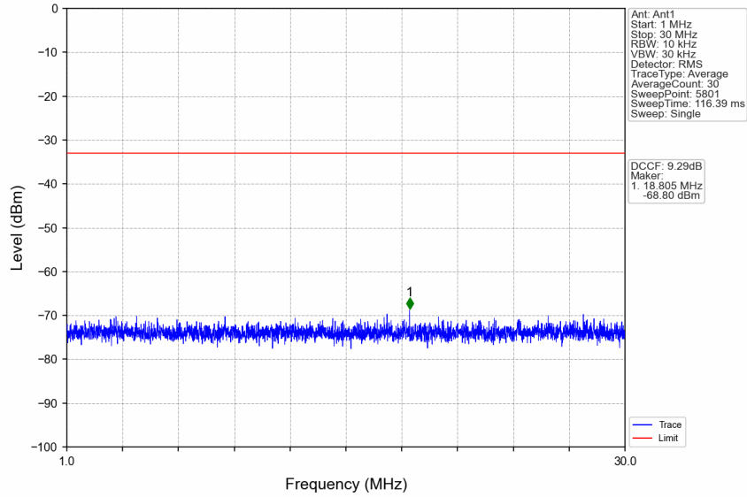
n77d_15kHz_SISO_NTNV_20MHz_CP-OFDM QPSK_3460.005MHz_Edge_1RB_Left
