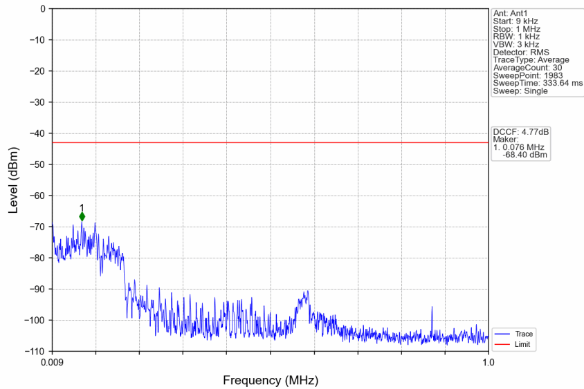
n77d_15kHz_SISO_NTNV_25MHz_DFT-s-OFDM QPSK_3537.495MHz_Edge_1RB_Right
