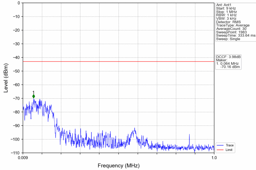
n77d_15kHz_SISO_NTNV_20MHz_DFT-s-OFDM QPSK_3540MHz_Edge_1RB_Right
