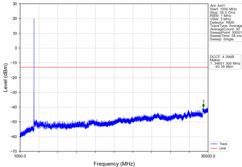
n77d_15kHz_SISO_NTNV_20MHz_CP-OFDM QPSK_3540MHz_Edge_1RB_Right
