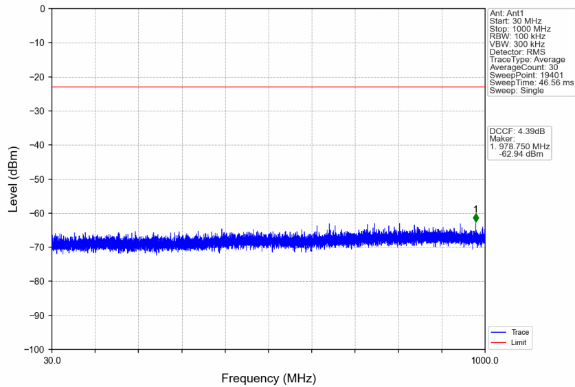
n77d_15kHz_SISO_NTNV_20MHz_CP-OFDM QPSK_3540MHz_Edge_1RB_Right
