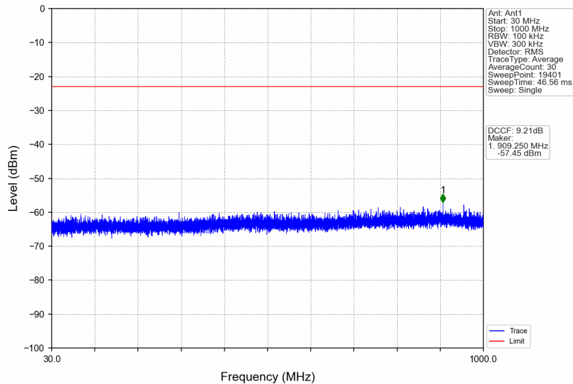
n77d_15kHz_SISO_NTNV_25MHz_DFT-s-OFDM_QPSK_3462.51MHz_Edge_1RB_Left
