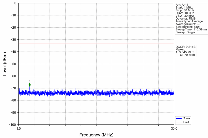
n77d_15kHz_SISO_NTNV_20MHz_DFT-s-OFDM QPSK_3499.995MHz_Edge_1RB_Left
