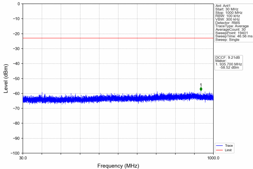
n77d_15kHz_SISO_NTNV_20MHz_DFT-s-OFDM QPSK_3460.005MHz_Edge_1RB_Left
