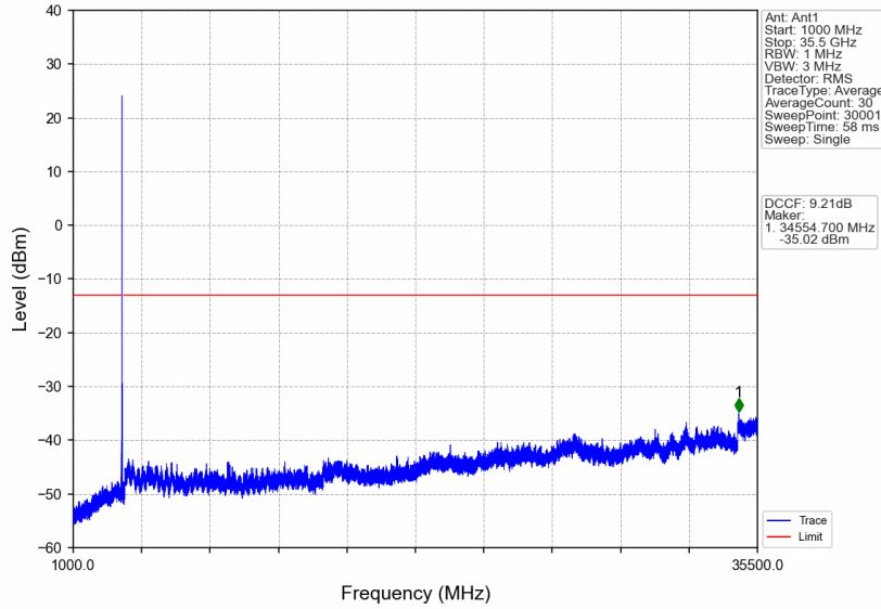
n77d_15kHz_SISO_NTNV_20MHz_DFT-s-OFDM QPSK_3460.005MHz_Outer_Full
