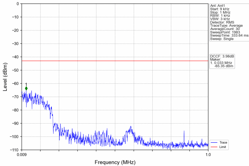
n77d_15kHz_SISO_NTNV_10MHz_CP-OFDM QPSK_3544.995MHz_Edge_1RB_Right
