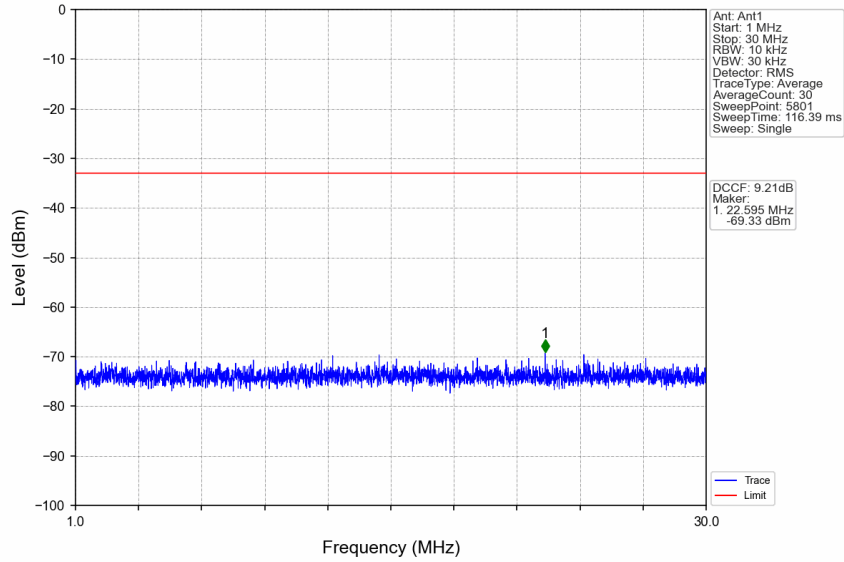
n77d_15kHz_SISO_NTNV_15MHz_CP-OFDM QPSK_3499.995MHz_Edge_1RB_Left
