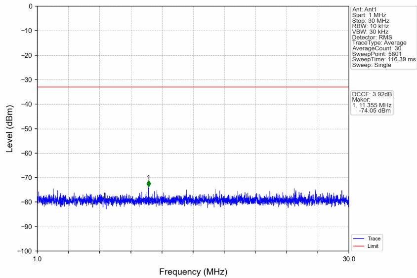
n77d_15kHz_SISO_NTNV_15MHz_DFT-s-OFDM QPSK_3457.5MHz_Edge_1RB_Left
