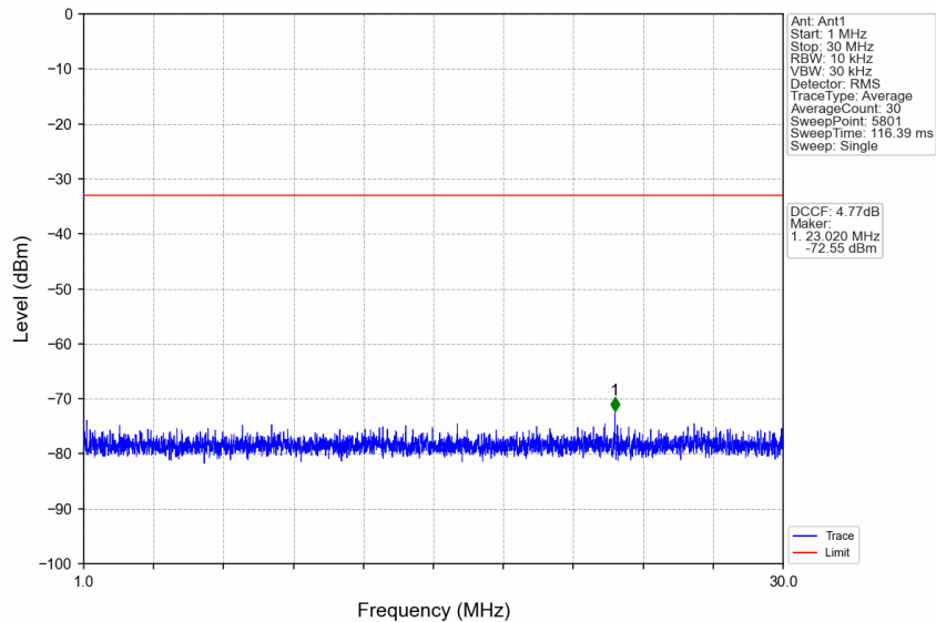
n77d_15kHz_SISO_NTNV_15MHz_CP-OFDM QPSK_3542.49MHz_Edge_1RB_Right
