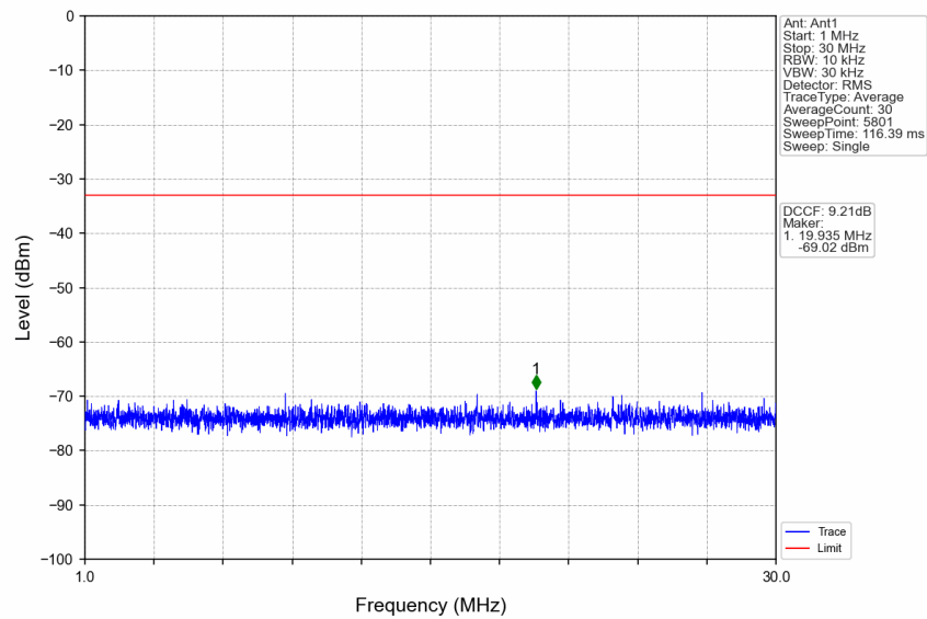
n77d_15kHz_SISO_NTNV_10MHz_CP-OFDM QPSK_3455.01MHz_Edge_1RB_Left
