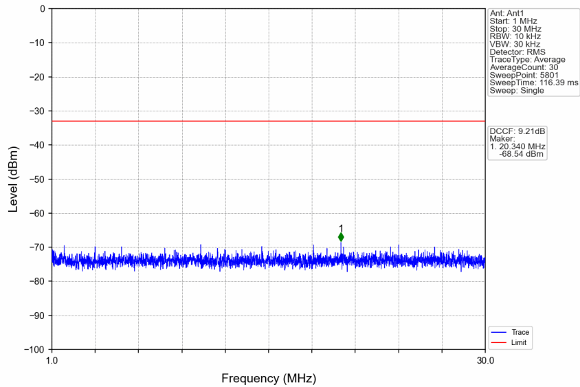
n77d_15kHz_SISO_NTNV_15MHz_DFT-s-OFDM QPSK_3499.995MHz_Edge_1RB_Left
