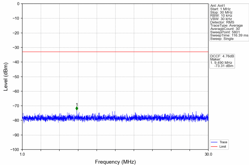
n77d_15kHz_SISO_NTNV_15MHz_DFT-s-OFDM PI/2 BPSK_3542.49MHz_Edge_1RB_Right
