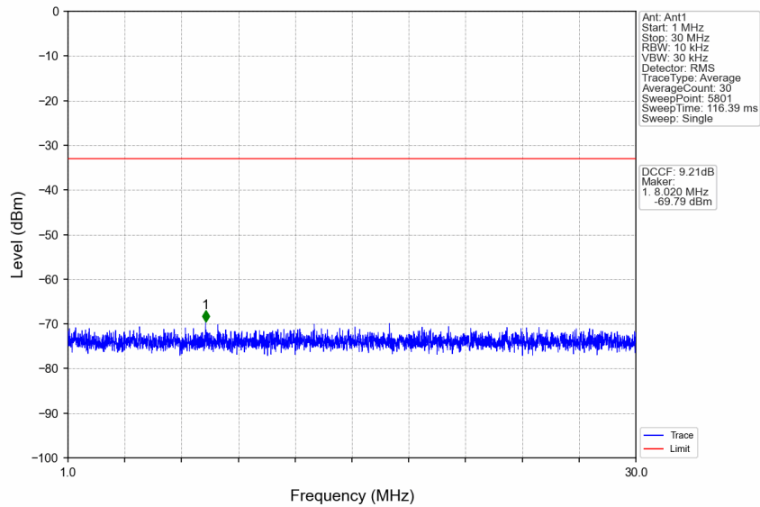
n77d_15kHz_SISO_NTNV_10MHz_DFT-s-OFDM QPSK_3499.995MHz_Edge_1RB_Left
