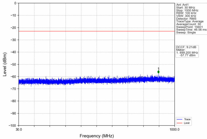
n77d_15kHz_SISO_NTNV_15MHz_CP-OFDM QPSK_3499.995MHz_Edge_1RB_Left
