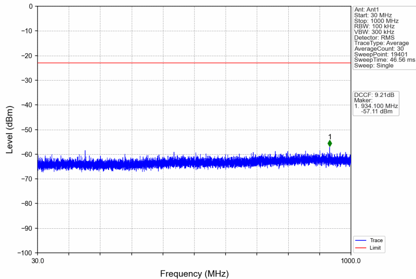
n77d_15kHz_SISO_NTNV_10MHz_CP-OFDM QPSK_3499.995MHz_Edge_1RB_Left
