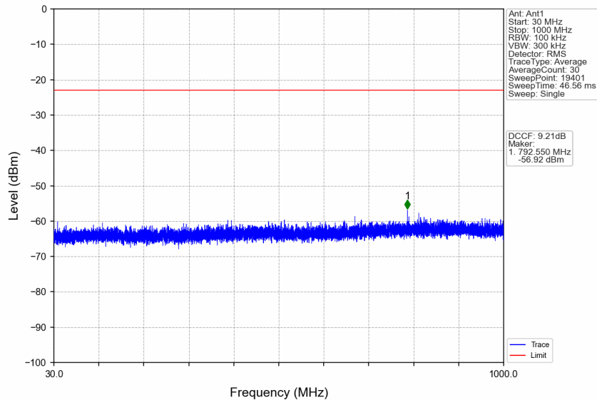
n77d_15kHz_SISO_NTNV_15MHz_DFT-s-OFDM QPSK_3499.995MHz_Edge_1RB_Left
