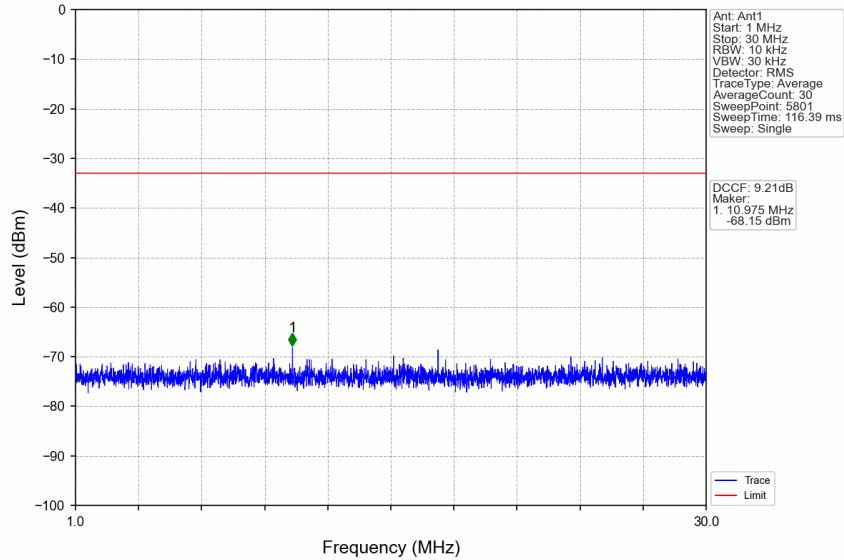
n77d_15kHz_SISO_NTNV_10MHz_CP-OFDM QPSK_3499.995MHz_Edge_1RB_Left
