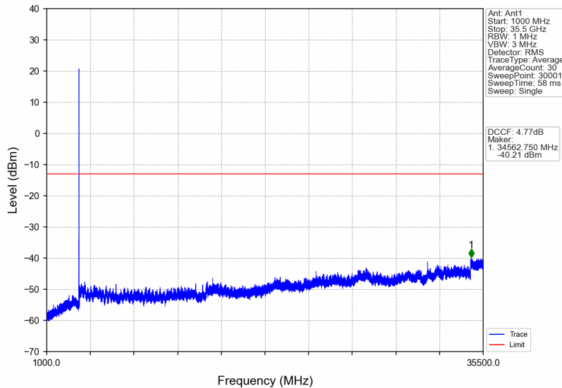
n77d_15kHz_SISO_NTNV_10MHz_DFT-s-OFDM_QPSK_3544.995MHz_Edge_1RB_Right
