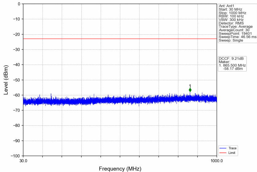
n77d_15kHz_SISO_NTNV_10MHz_DFT-s-OFDM QPSK_3499.995MHz_Edge_1RB_Left
