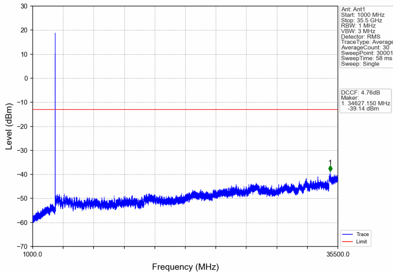
n77d_15kHz_SISO_NTNV_15MHz_DFT-s-OFDM PI/2 BPSK_3542.49MHz_Edge_1RB_Right
