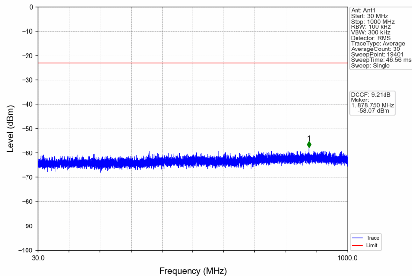
n77d_15kHz_SISO_NTNV_10MHz_CP-OFDM QPSK_3455.01MHz_Edge_1RB_Left
