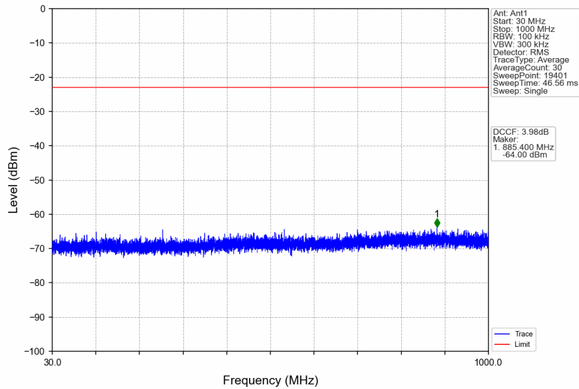
n77d_15kHz_SISO_NTNV_10MHz_CP-OFDM QPSK_3544.995MHz_Edge_1RB_Right
