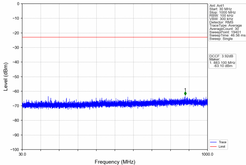
n77d_15kHz_SISO_NTNV_15MHz_DFT-s-OFDM QPSK_3457.5MHz_Edge_1RB_Left
