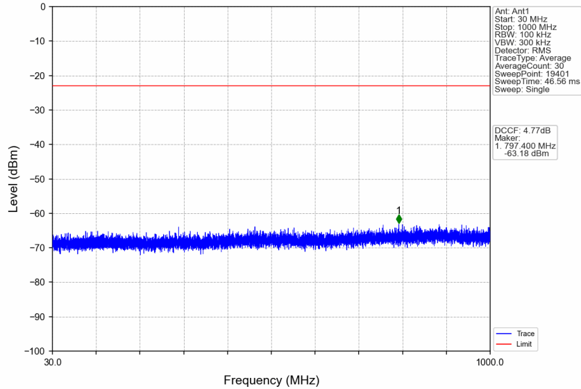
n77d_15kHz_SISO_NTNV_10MHz_DFT-s-OFDM_QPSK_3544.995MHz_Edge_1RB_Right
