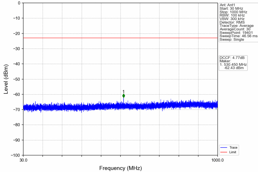
n77d_15kHz_SISO_NTNV_15MHz_DFT-s-OFDM QPSK_3542.49MHz_Edge_1RB_Right
