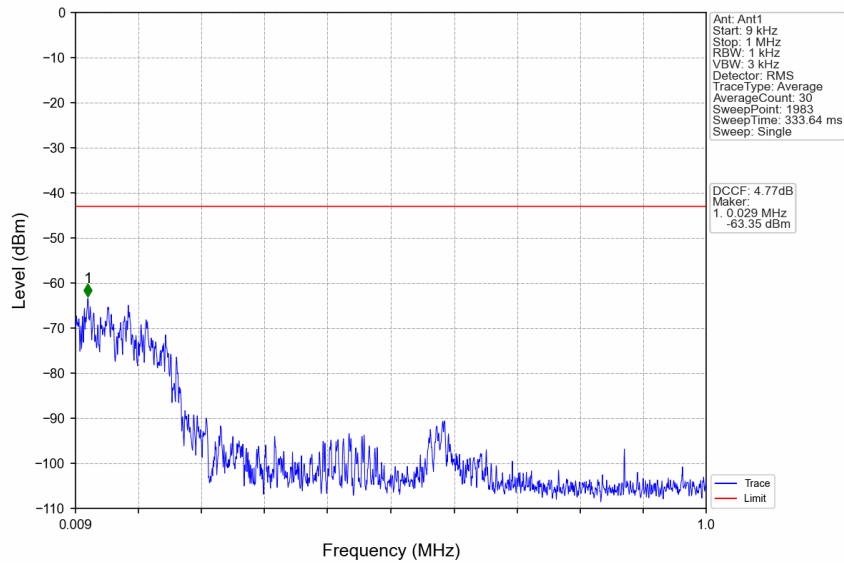
n77d_15kHz_SISO_NTNV_15MHz_CP-OFDM QPSK_3542.49MHz_Edge_1RB_Right
