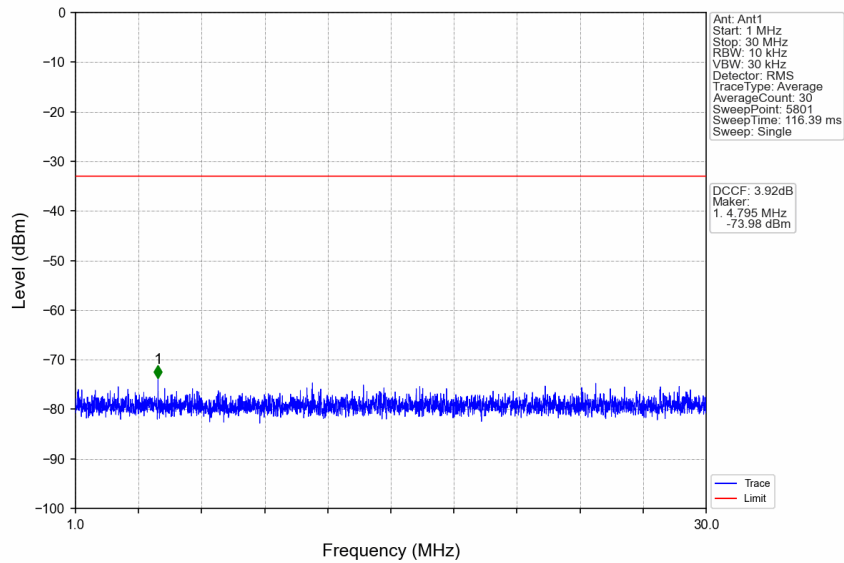
n77d_15kHz_SISO_NTNV_15MHz_CP-OFDM QPSK_3457.5MHz_Edge_1RB_Left
