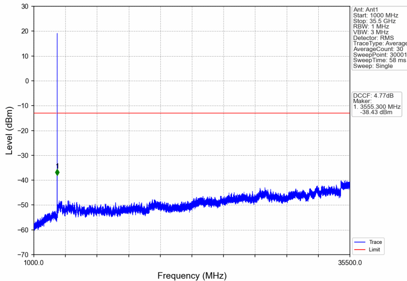
n77d_15kHz_SISO_NTNV_15MHz_DFT-s-OFDM QPSK_3542.49MHz_Edge_1RB_Right
