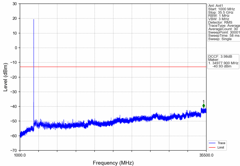
n77d_15kHz_SISO_NTNV_10MHz_CP-OFDM QPSK_3544.995MHz_Edge_1RB_Right
