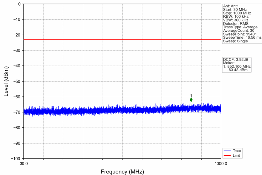
n77d_15kHz_SISO_NTNV_15MHz_CP-OFDM QPSK_3457.5MHz_Edge_1RB_Left
