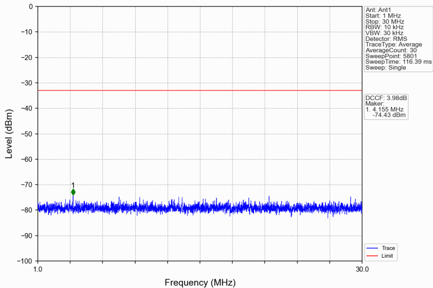
n77d_15kHz_SISO_NTNV_10MHz_CP-OFDM QPSK_3544.995MHz_Edge_1RB_Right
