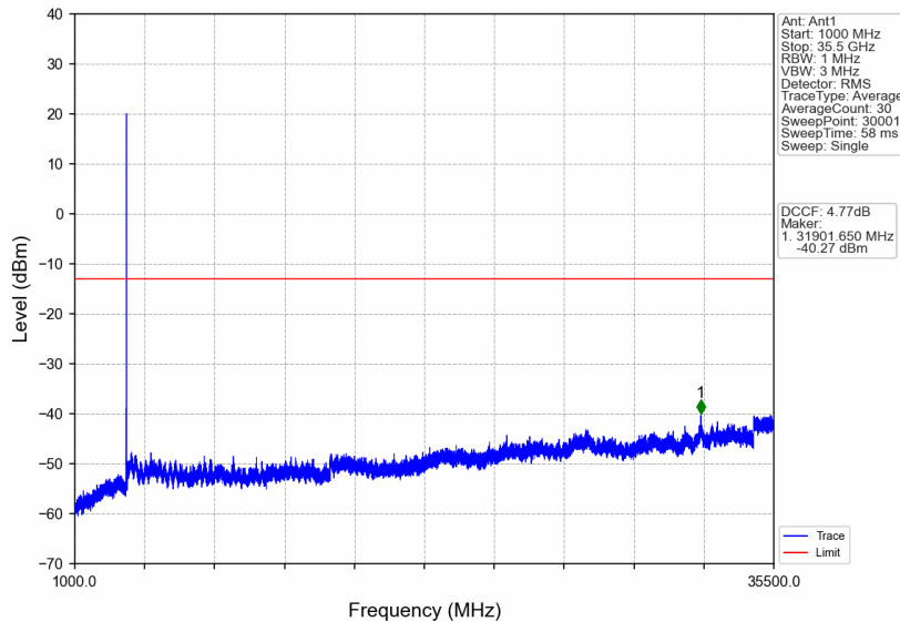
n77d_15kHz_SISO_NTNV_15MHz_CP-OFDM QPSK_3542.49MHz_Edge_1RB_Right
