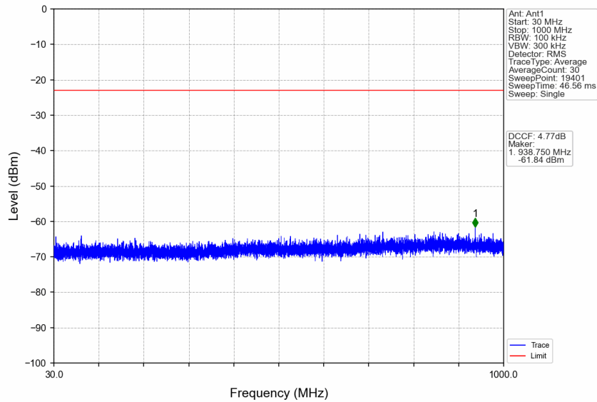
n77d_15kHz_SISO_NTNV_15MHz_CP-OFDM QPSK_3542.49MHz_Edge_1RB_Right
