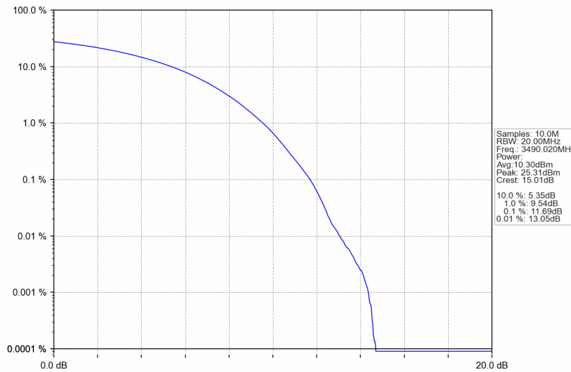
n77d_30kHz_SISO_NTNV_80MHz_CP-OFDM 256 QAM_3490.02MHz_Outer_Full
