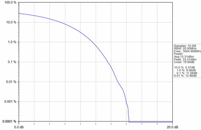
n77d_30kHz_SISO_NTNV_90MHz_CP-OFDM 16 QAM_3504.99MHz_Outer_Full
