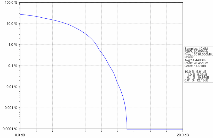
n77d_30kHz_SISO_NTNV_80MHz_DFT-s-OFDM 16 QAM_3510MHz_Outer_Full
