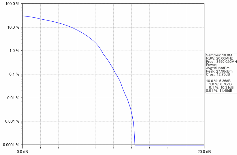
n77d_30kHz_SISO_NTNV_80MHz_DFT-s-OFDM 16 QAM_3490.02MHz_Outer_Full
