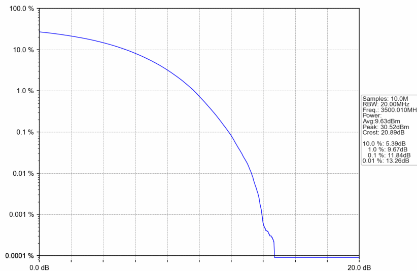
n77d_30kHz_SISO_NTNV_90MHz_CP-OFDM 256 QAM_3500.01MHz_Outer_Full
