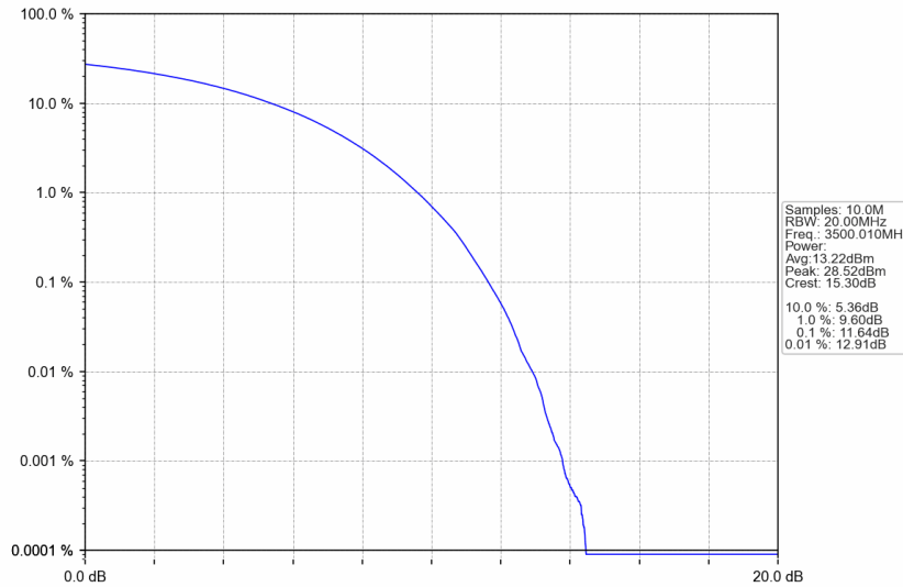
n77d_30kHz_SISO_NTNV_90MHz_CP-OFDM QPSK_3500.01MHz_Outer_Full
