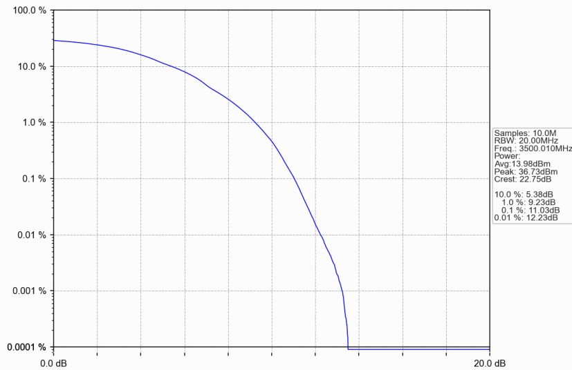
n77d_30kHz_SISO_NTNV_90MHz_DFT-s-OFDM 16 QAM_3500.01MHz_Outer_Full
