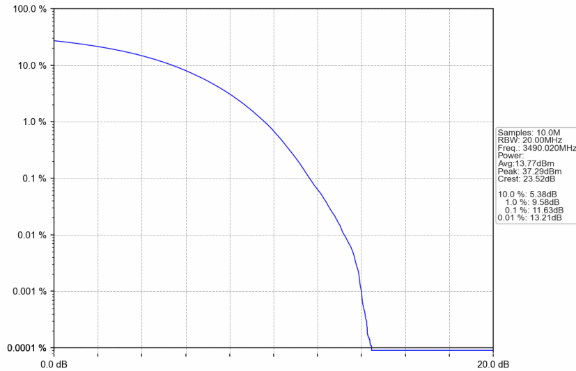
n77d_30kHz_SISO_NTNV_80MHz_CP-OFDM 16 QAM_3490.02MHz_Outer_Full
