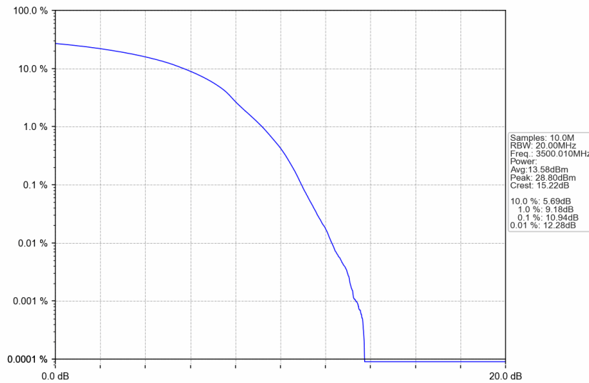
n77d_30kHz_SISO_NTNV_100MHz_DFT-s-OFDM 16 QAM_3500.01MHz_Outer_Full
