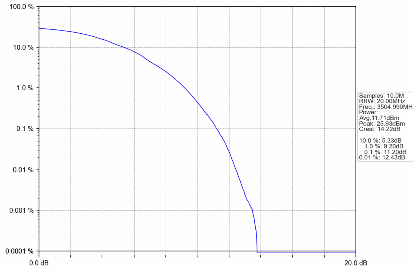
n77d_30kHz_SISO_NTNV_90MHz_DFT-s-OFDM 256 QAM_3504.99MHz_Outer_Full
