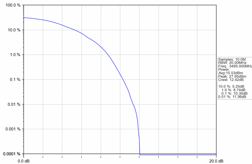
n77d_30kHz_SISO_NTNV_90MHz_DFT-s-OFDM QPSK_3495MHz_Outer_Full
