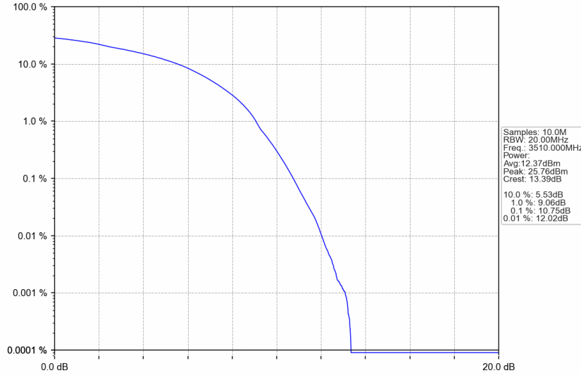
n77d_30kHz_SISO_NTNV_80MHz_DFT-s-OFDM 256 QAM_3510MHz_Outer_Full
