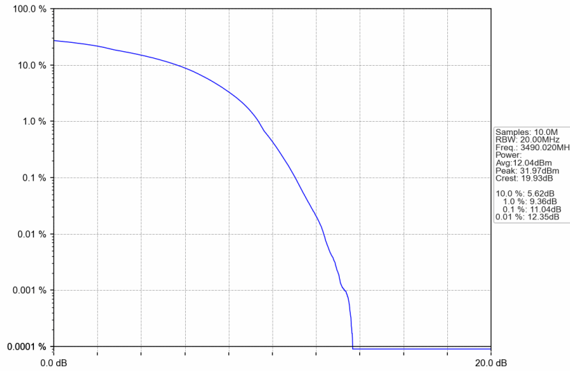
n77d_30kHz_SISO_NTNV_80MHz_DFT-s-OFDM 256 QAM_3490.02MHz_Outer_Full
