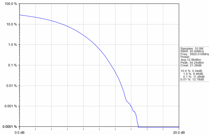
n77d_30kHz_SISO_NTNV_100MHz_CP-OFDM QPSK_3500.01MHz_Outer_Full
