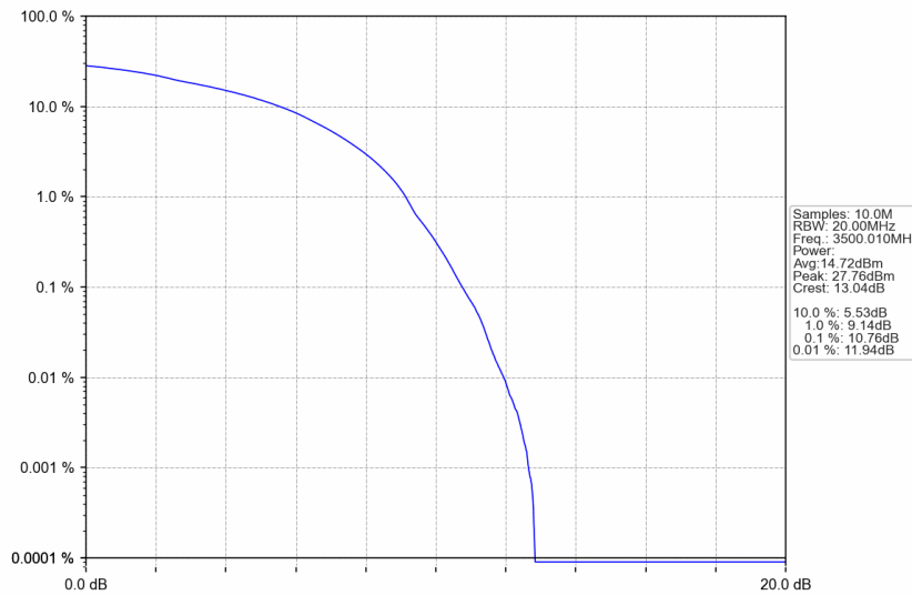
n77d_30kHz_SISO_NTNV_80MHz_DFT-s-OFDM 16 QAM_3500.01MHz_Outer_Full
