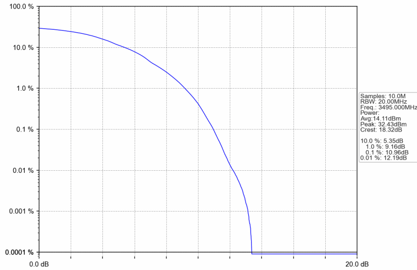
n77d_30kHz_SISO_NTNV_90MHz_DFT-s-OFDM 16 QAM_3495MHz_Outer_Full
