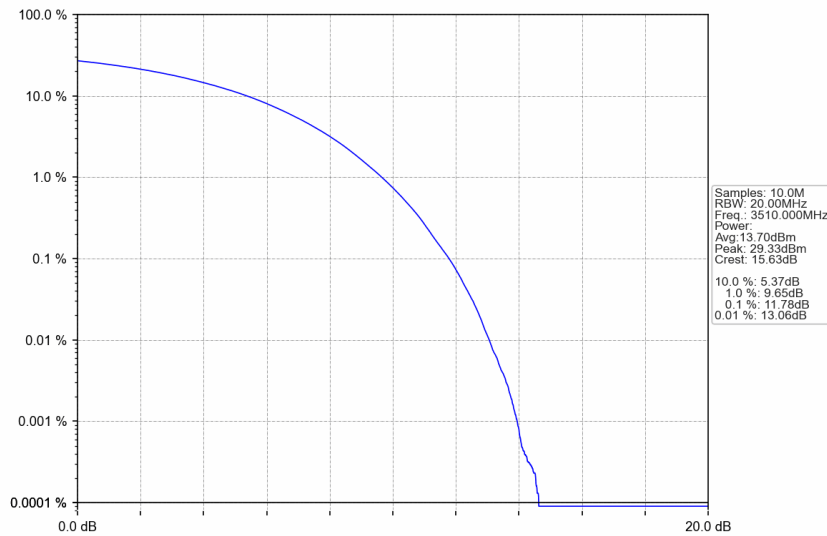
n77d_30kHz_SISO_NTNV_80MHz_CP-OFDM QPSK_3510MHz_Outer_Full
