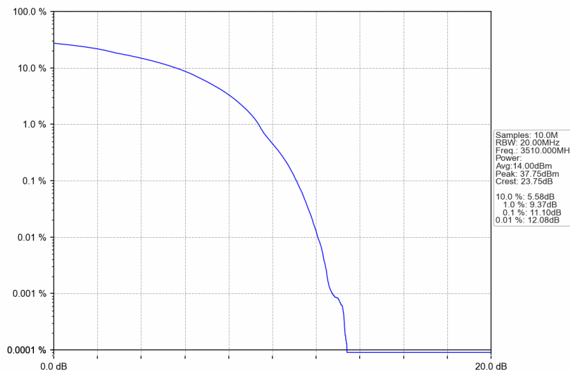
n77d_30kHz_SISO_NTNV_80MHz_DFT-s-OFDM 64 QAM_3510MHz_Outer_Full
