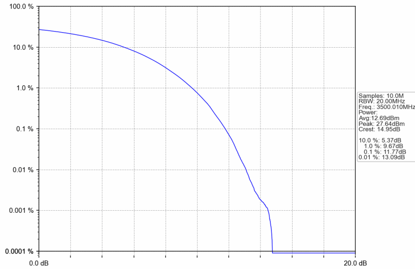
n77d_30kHz_SISO_NTNV_90MHz_CP-OFDM 64 QAM_3500.01MHz_Outer_Full
