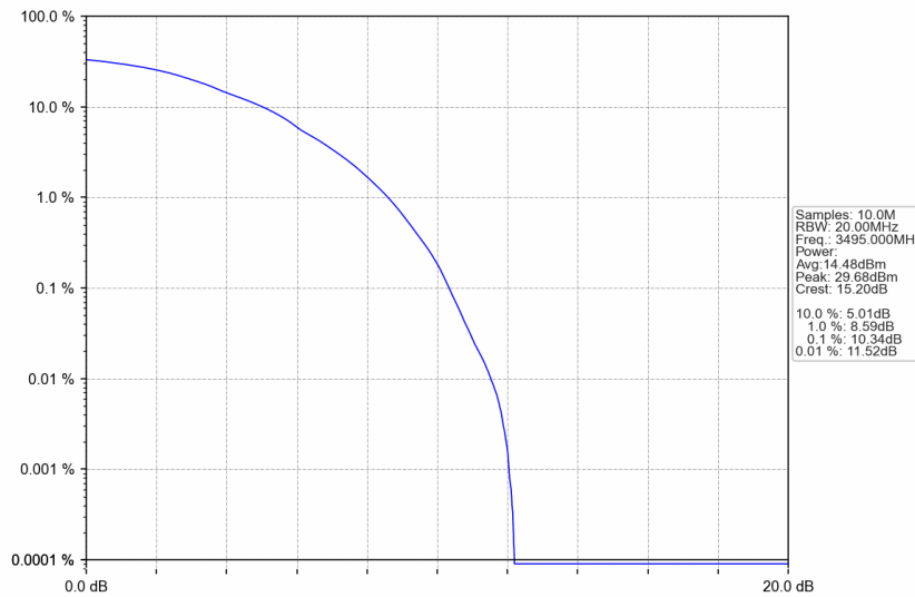
n77d_30kHz_SISO_NTNV_90MHz_DFT-s-OFDM 64 QAM_3495MHz_Outer_Full
