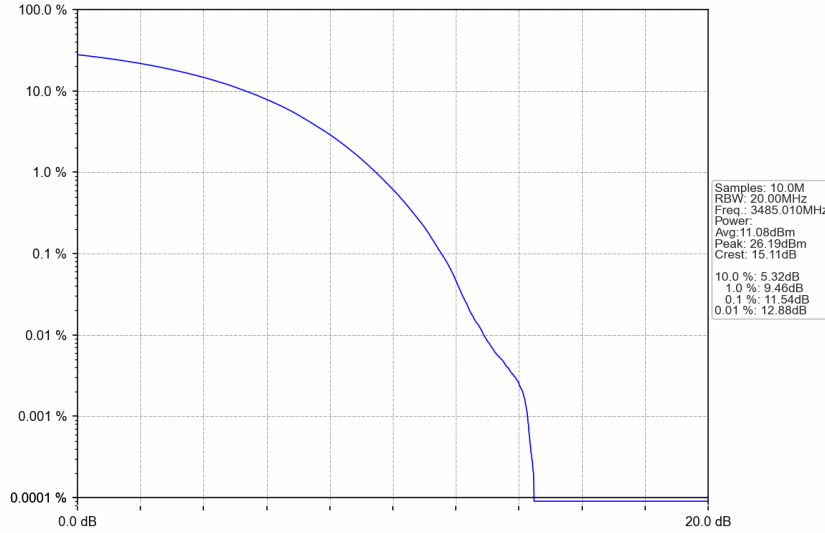
n77d_30kHz_SISO_NTNV_70MHz_CP-OFDM 256 QAM_3485.01MHz_Outer_Full
