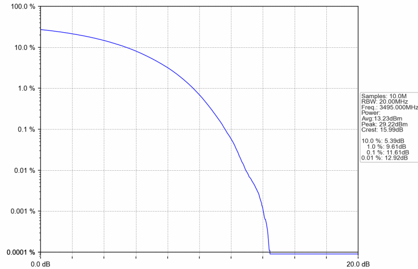
n77d_30kHz_SISO_NTNV_90MHz_CP-OFDM 16 QAM_3495.00MHz_Outer_Full
