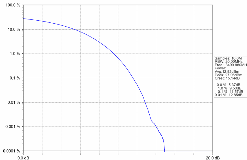
n77d_30kHz_SISO_NTNV_100MHz_CP-OFDM QPSK_3499.98MHz_Outer_Full
