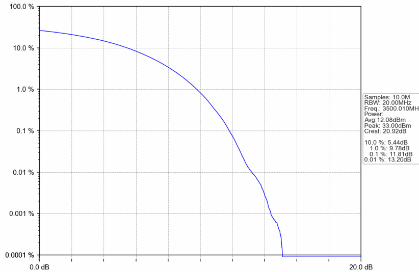
n77d_30kHz_SISO_NTNV_100MHz_CP-OFDM 64 QAM_3500.01MHz_Outer_Full
