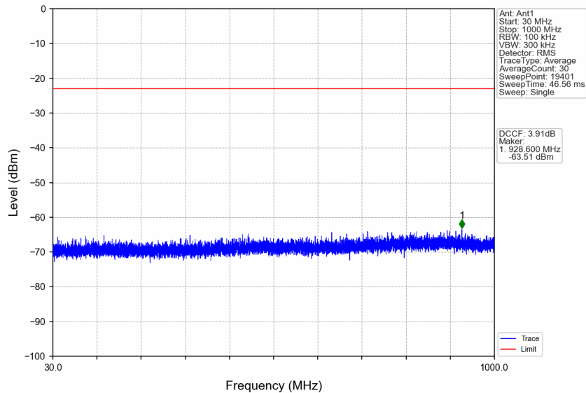
n77d_15kHz_SISO_NTNV_10MHz_DFT-s-OFDM_QPSK_3455.01MHz_Edge_1RB_Left
