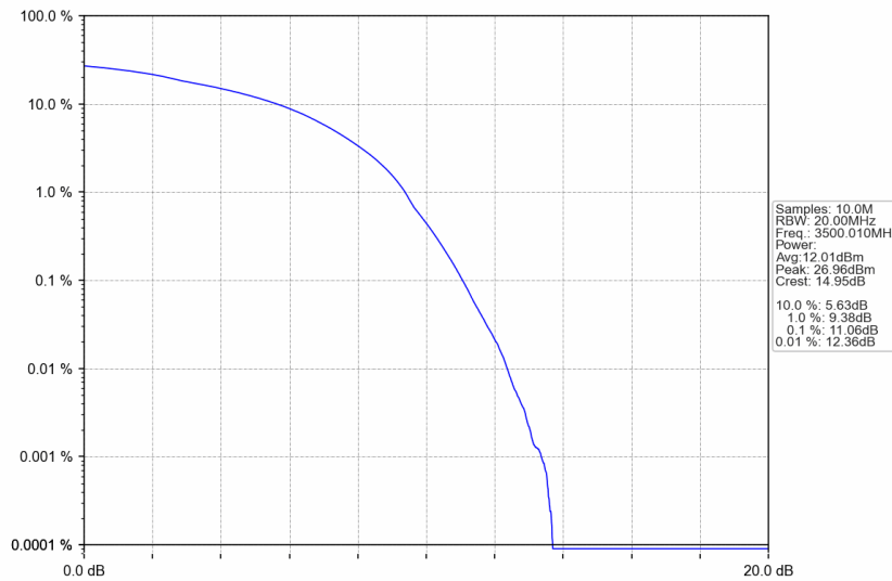
n77d_30kHz_SISO_NTNV_80MHz_DFT-s-OFDM 256 QAM_3500.01MHz_Outer_Full
