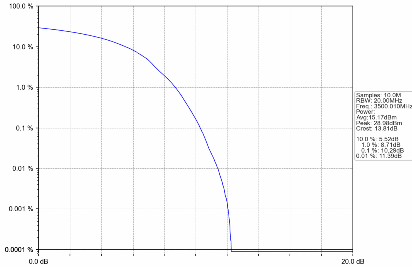
n77d_30kHz_SISO_NTNV_100MHz_DFT-s-OFDM QPSK_3500.01MHz_Outer_Full
