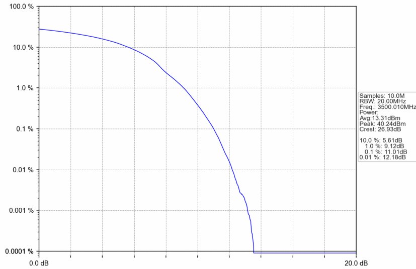
n77d_30kHz_SISO_NTNV_100MHz_DFT-s-OFDM 64 QAM_3500.01MHz_Outer_Full
