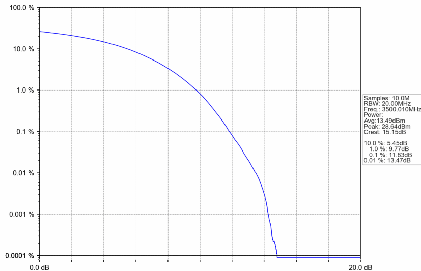
n77d_30kHz_SISO_NTNV_80MHz_CP-OFDM 16 QAM_3500.01MHz_Outer_Full
