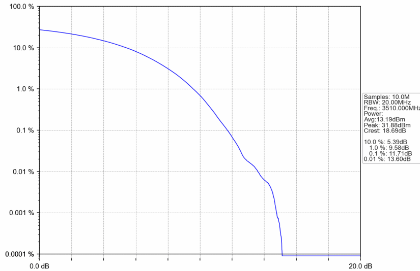
n77d_30kHz_SISO_NTNV_80MHz_CP-OFDM 64 QAM_3510MHz_Outer_Full
