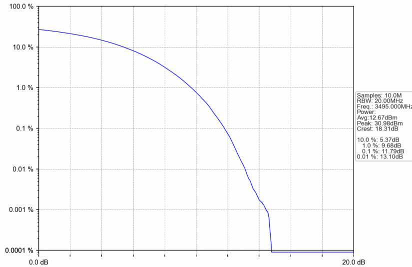
n77d_30kHz_SISO_NTNV_90MHz_CP-OFDM 64 QAM_3495MHz_Outer_Full
