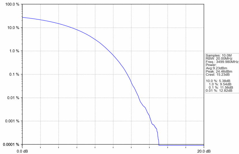
n77d_30kHz_SISO_NTNV_100MHz_CP-OFDM 256 QAM_3499.98MHz_Outer_Full
