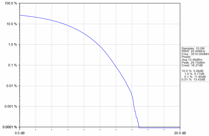
n77d_30kHz_SISO_NTNV_80MHz_CP-OFDM 16 QAM_3510MHz_Outer_Full
