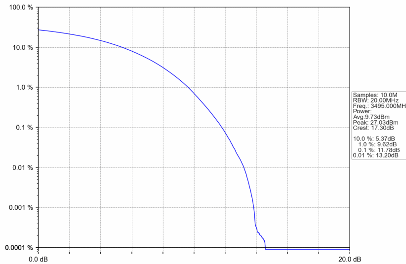
n77d_30kHz_SISO_NTNV_90MHz_CP-OFDM 256 QAM_3495MHz_Outer_Full
