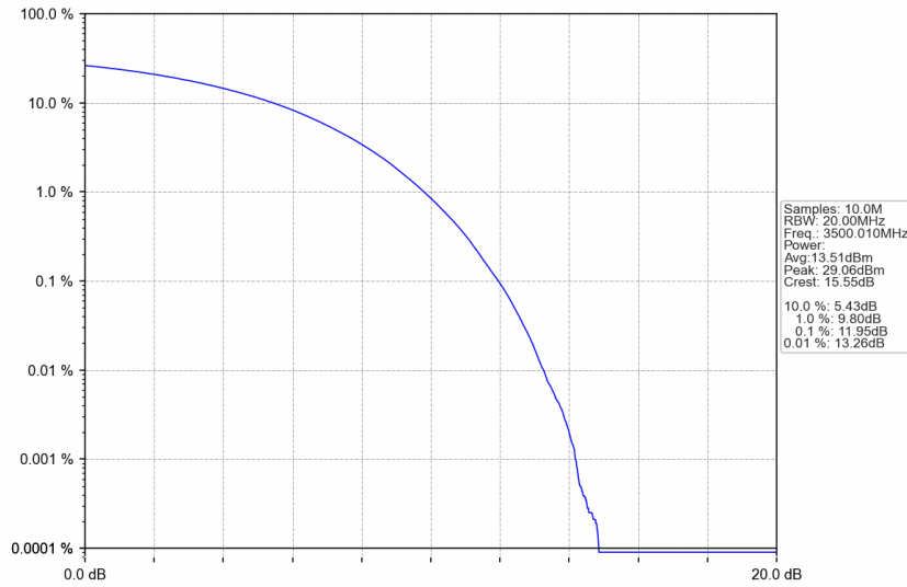
n77d_30kHz_SISO_NTNV_80MHz_CP-OFDM QPSK_3500.01MHz_Outer_Full
