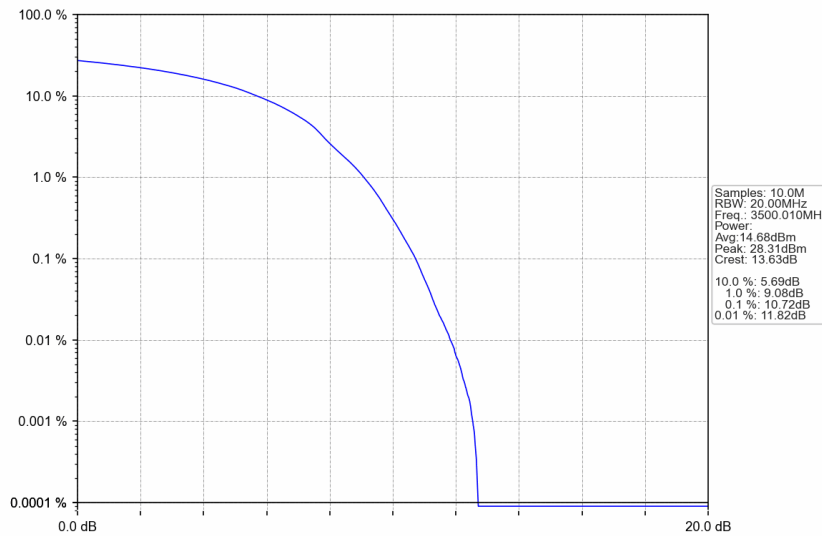
n77d_30kHz_SISO_NTNV_100MHz_DFT-s-OFDM QPSK_3500.01MHz_Outer_Full
