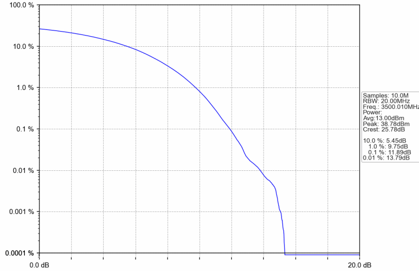
n77d_30kHz_SISO_NTNV_80MHz_CP-OFDM 64 QAM_3500.01MHz_Outer_Full
