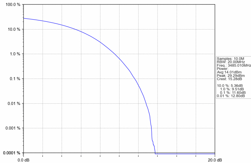
n77d_30kHz_SISO_NTNV_70MHz_CP-OFDM 64 QAM_3485.01MHz_Outer_Full
