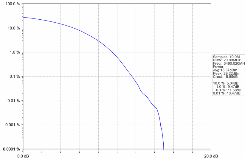
n77d_30kHz_SISO_NTNV_80MHz_CP-OFDM 64 QAM_3490.02MHz_Outer_Full
