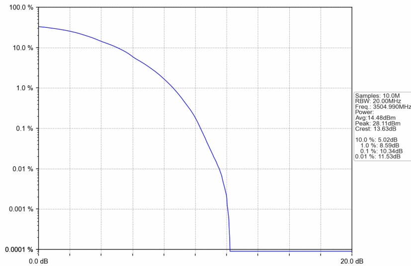
n77d_30kHz_SISO_NTNV_90MHz_DFT-s-OFDM 64 QAM_3504.99MHz_Outer_Full
