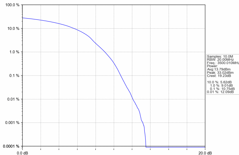
n77d_30kHz_SISO_NTNV_100MHz_DFT-s-OFDM 16 QAM_3500.01MHz_Outer_c_Full
