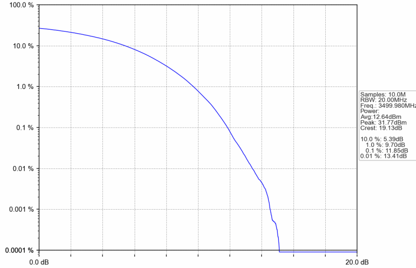
n77d_30kHz_SISO_NTNV_100MHz_CP-OFDM 16 QAM_3499.98MHz_Outer_Full
