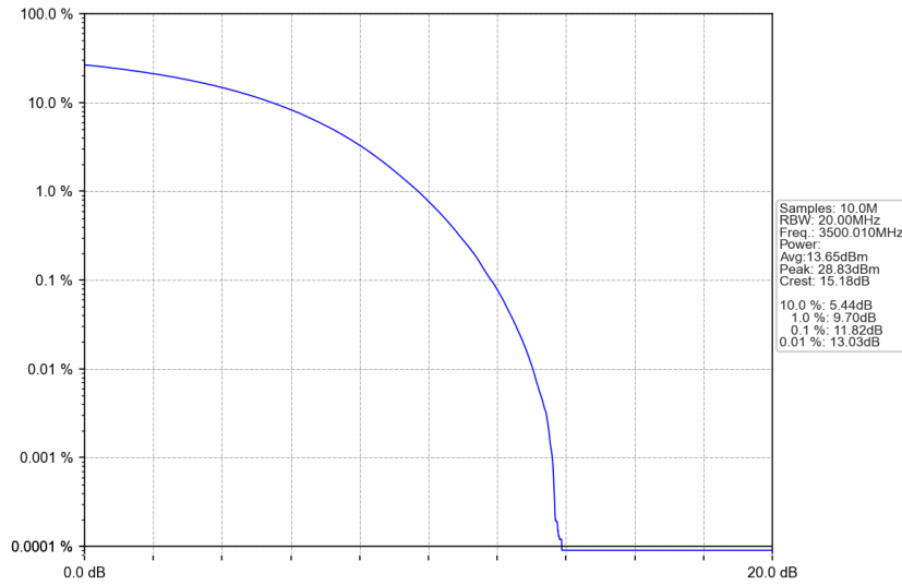
n77d_30kHz_SISO_NTNV_70MHz_CP-OFDM 64 QAM_3500.01MHz_Outer_Full
