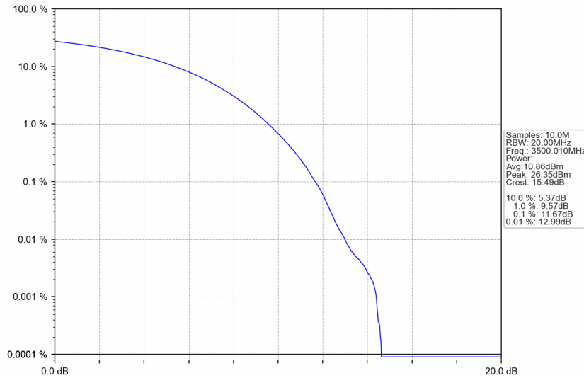
n77d_30kHz_SISO_NTNV_70MHz_CP-OFDM 256 QAM_3500.01MHz_Outer_Full
