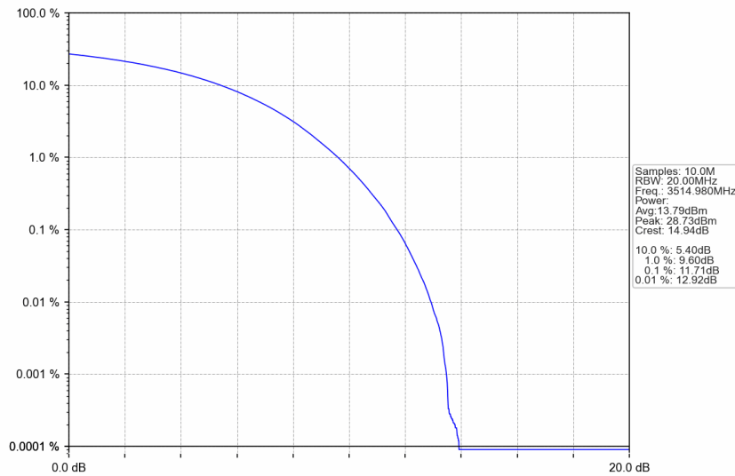
n77d_30kHz_SISO_NTNV_70MHz_CP-OFDM 64 QAM_3514.98MHz_Outer_Full
