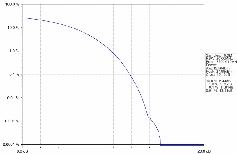
n77d_30kHz_SISO_NTNV_100MHz_CP-OFDM QPSK_3500.01MHz_Outer_Full
