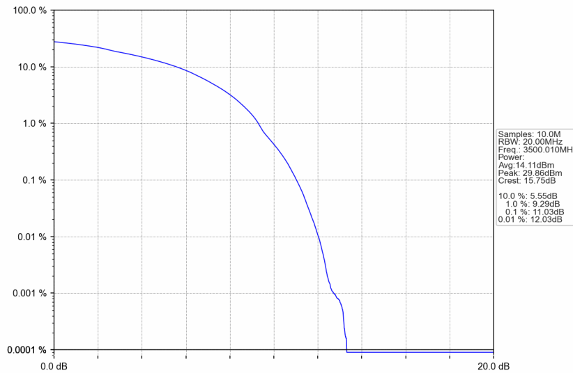
n77d_30kHz_SISO_NTNV_80MHz_DFT-s-OFDM 64 QAM_3500.01MHz_Outer_Full
