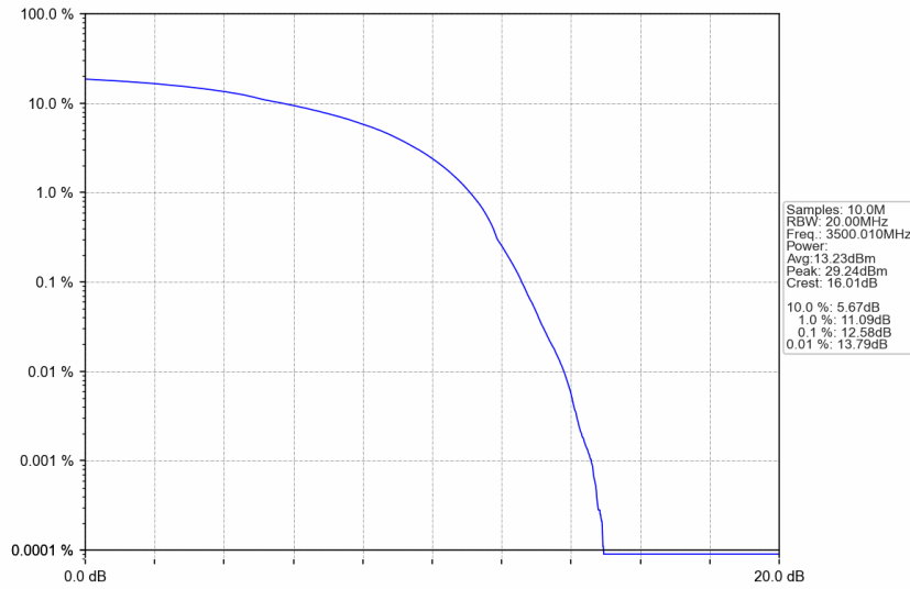
n77d_30kHz_SISO_NTNV_80MHz_DFT-s-OFDM QPSK_3500.01MHz_Outer_Full
