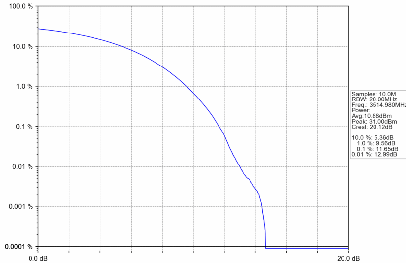
n77d_30kHz_SISO_NTNV_70MHz_CP-OFDM 256 QAM_3514.98MHz_Outer_Full
