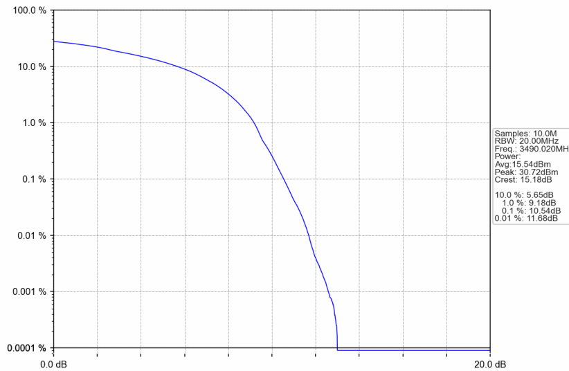
n77d_30kHz_SISO_NTNV_80MHz_DFT-s-OFDM QPSK_3490.02MHz_Outer_Full
