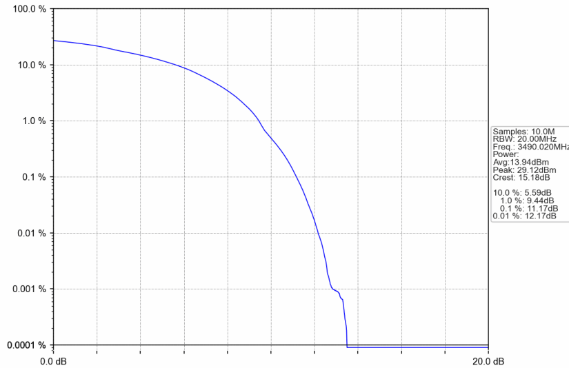
n77d_30kHz_SISO_NTNV_80MHz_DFT-s-OFDM 64 QAM_3490.02MHz_Outer_Full
