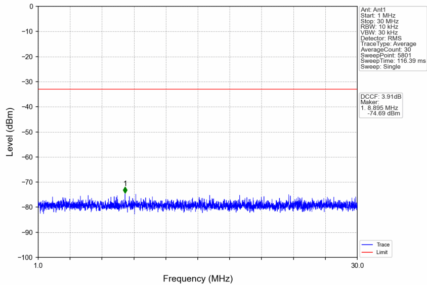
n77d_15kHz_SISO_NTNV_10MHz_DFT-s-OFDM_QPSK_3455.01MHz_Edge_1RB_Left
