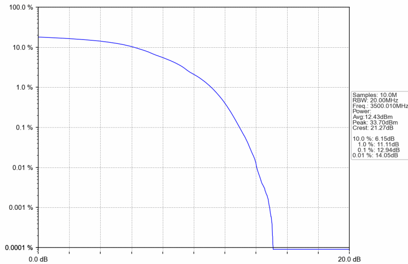
n77d_30kHz_SISO_NTNV_90MHz_DFT-s-OFDM QPSK_3500.01MHz_Outer_Full
