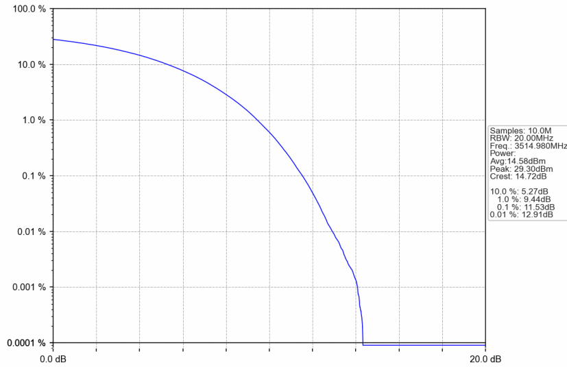
n77d_30kHz_SISO_NTNV_70MHz_CP-OFDM 16 QAM_3514.98MHz_Outer_Full
