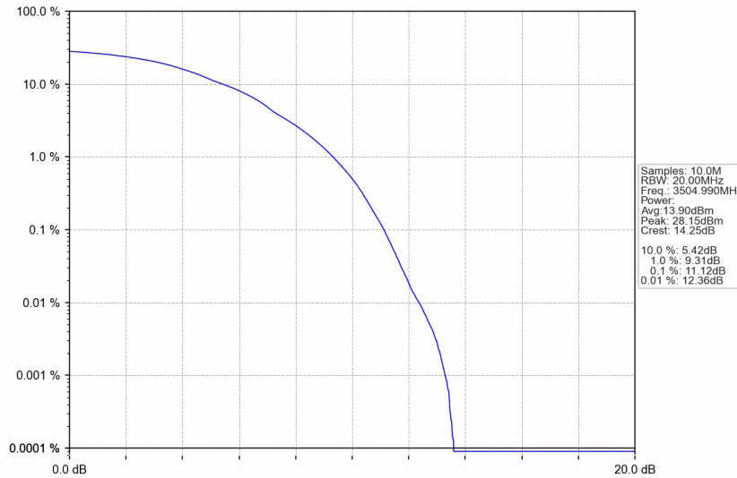
n77d_30kHz_SISO_NTNV_90MHz_DFT-s-OFDM 16 QAM_3504.99MHz_Outer_Full
