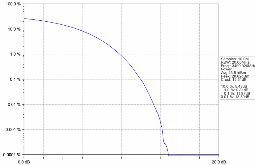
n77d_30kHz_SISO_NTNV_80MHz_CP-OFDM QPSK_3490.02MHz_Outer_Full
