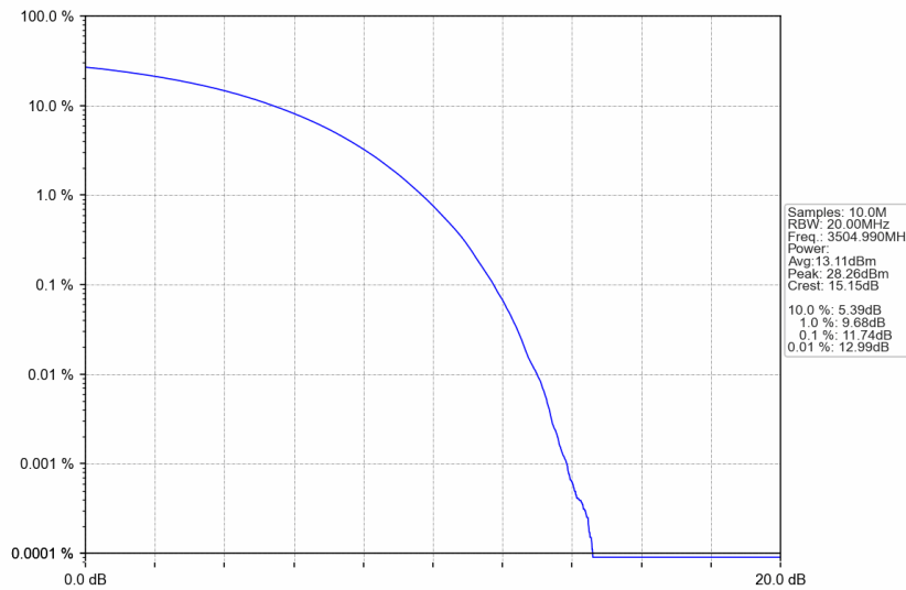
n77d_30kHz_SISO_NTNV_90MHz_CP-OFDM QPSK_3504.99MHz_Outer_Full
