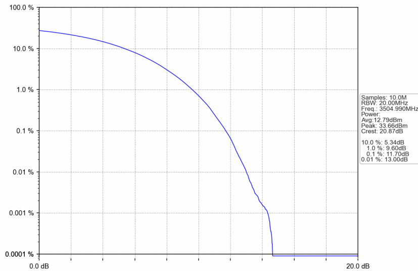
n77d_30kHz_SISO_NTNV_90MHz_CP-OFDM 64 QAM_3504.99MHz_Outer_Full
