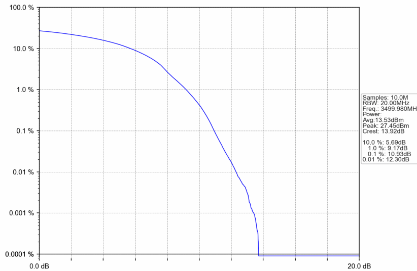
n77d_30kHz_SISO_NTNV_100MHz_DFT-s-OFDM 16 QAM_3499.98MHz_Outer_Full
