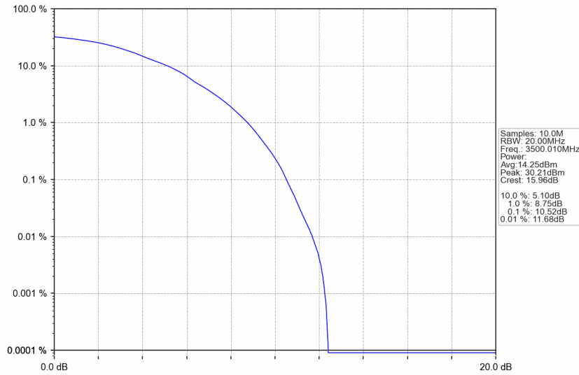
n77d_30kHz_SISO_NTNV_90MHz_DFT-s-OFDM 64 QAM_3500.01MHz_Outer_Full
