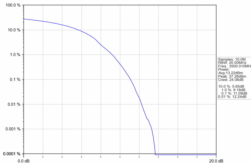
n77d_30kHz_SISO_NTNV_100MHz_DFT-s-OFDM 64 QAM_3500.01MHz_Outer_Full
