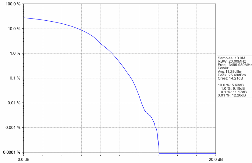
n77d_30kHz_SISO_NTNV_100MHz_DFT-s-OFDM 256 QAM_3499.98MHz_Outer_Full
