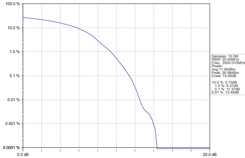
n77d_30kHz_SISO_NTNV_100MHz_DFT-s-OFDM 256 QAM_3500.01MHz_Outer_Full
