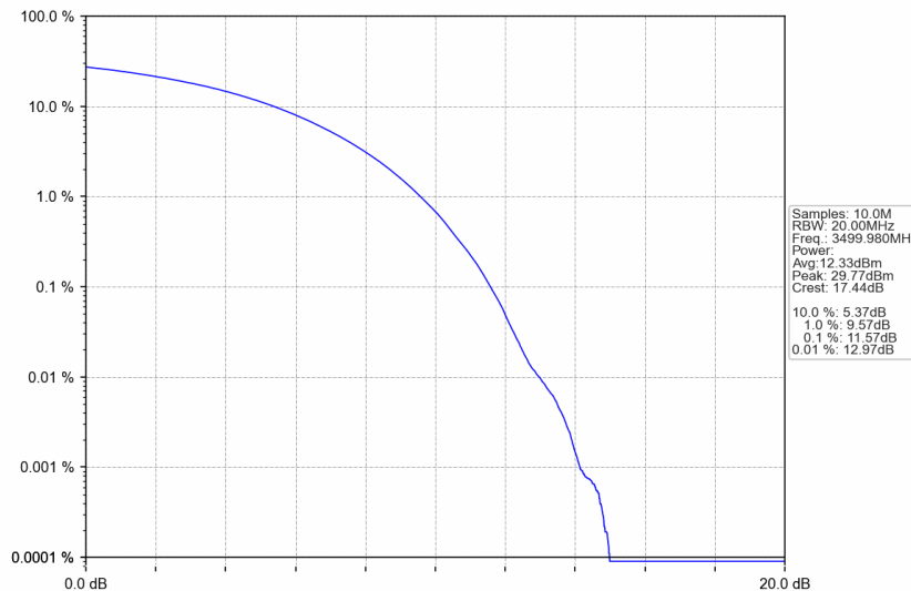
n77d_30kHz_SISO_NTNV_100MHz_CP-OFDM 64 QAM_3499.98MHz_Outer_Full
