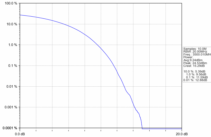
n77d_30kHz_SISO_NTNV_100MHz_CP-OFDM 256 QAM_3500.01MHz_Outer_Full
