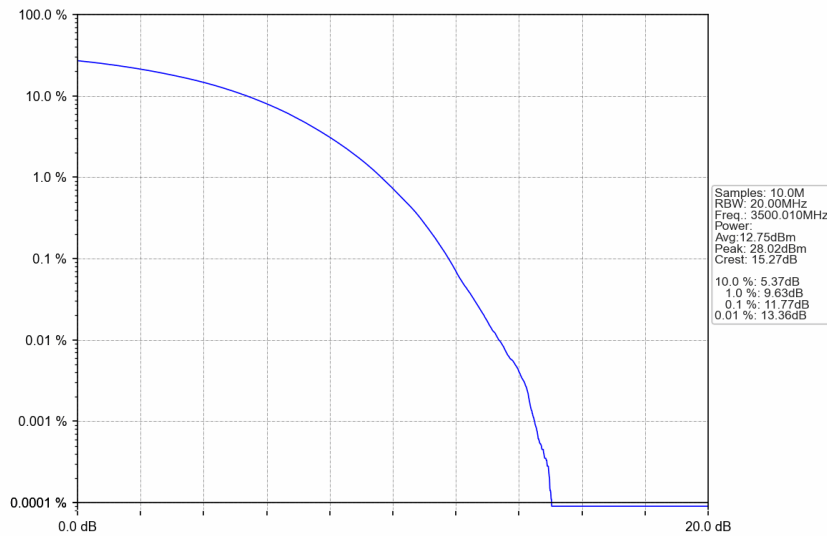
n77d_30kHz_SISO_NTNV_100MHz_CP-OFDM 16 QAM_3500.01MHz_Outer_Full
