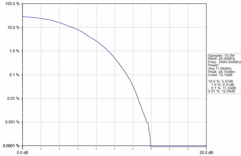
n77d_30kHz_SISO_NTNV_90MHz_DFT-s-OFDM 256 QAM_3495MHz_Outer_Full
