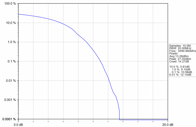
n77d_30kHz_SISO_NTNV_100MHz_DFT-s-OFDM 64 QAM_3499.98MHz_Outer_Full
