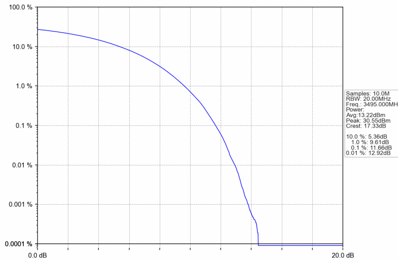
n77d_30kHz_SISO_NTNV_90MHz_CP-OFDM QPSK_3495MHz_Outer_Full
