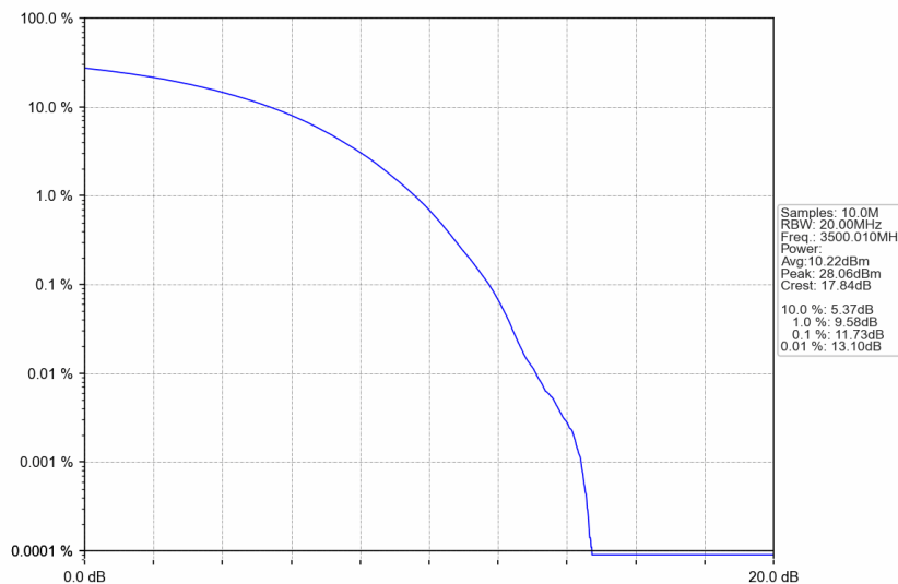
n77d_30kHz_SISO_NTNV_80MHz_CP-OFDM 256 QAM_3500.01MHz_Outer_Full
