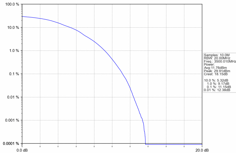
n77d_30kHz_SISO_NTNV_90MHz_DFT-s-OFDM 256 QAM_3500.01MHz_Outer_Full
