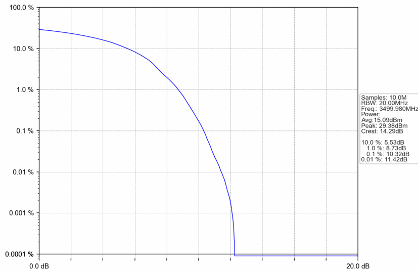
n77d_30kHz_SISO_NTNV_100MHz_DFT-s-OFDM QPSK_3499.98MHz_Outer_Full
