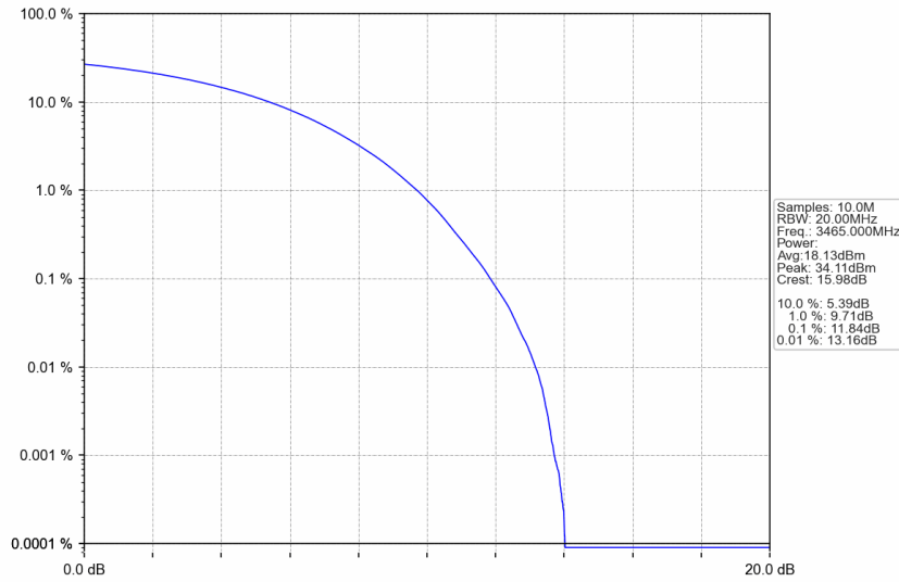
n77d_30kHz_SISO_NTNV_30MHz_CP-OFDM 16 QAM_3465MHz_Outer_Full
