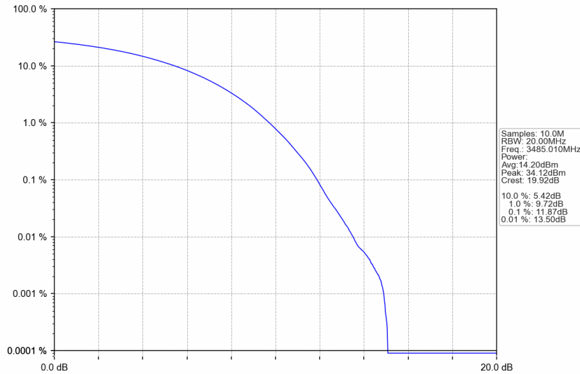
n77d_30kHz_SISO_NTNV_70MHz_CP-OFDM QPSK_3485.01MHz_Outer_Full
