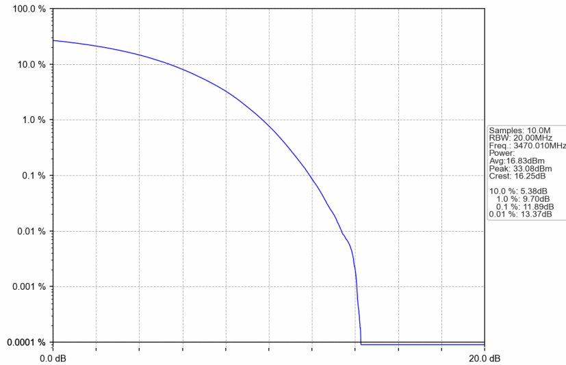
n77d_30kHz_SISO_NTNV_40MHz_CP-OFDM 16 QAM_3470.01MHz_Outer_Full
