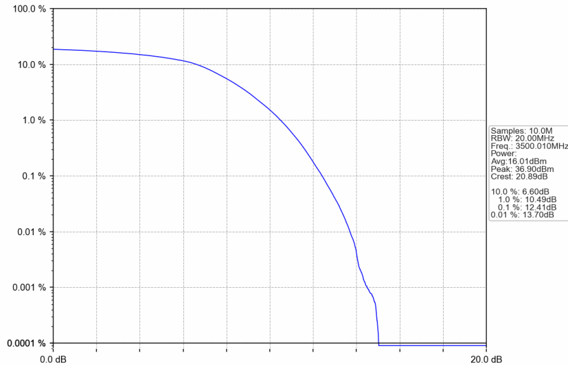
n77d_30kHz_SISO_NTNV_30MHz_DFT-s-OFDM 64 QAM_3500.01MHz_Outer_Full
