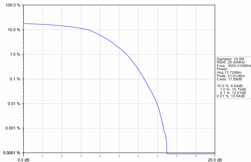
n77d_30kHz_SISO_NTNV_30MHz_DFT-s-OFDM 256 QAM_3500.01MHz_Outer_c Full
