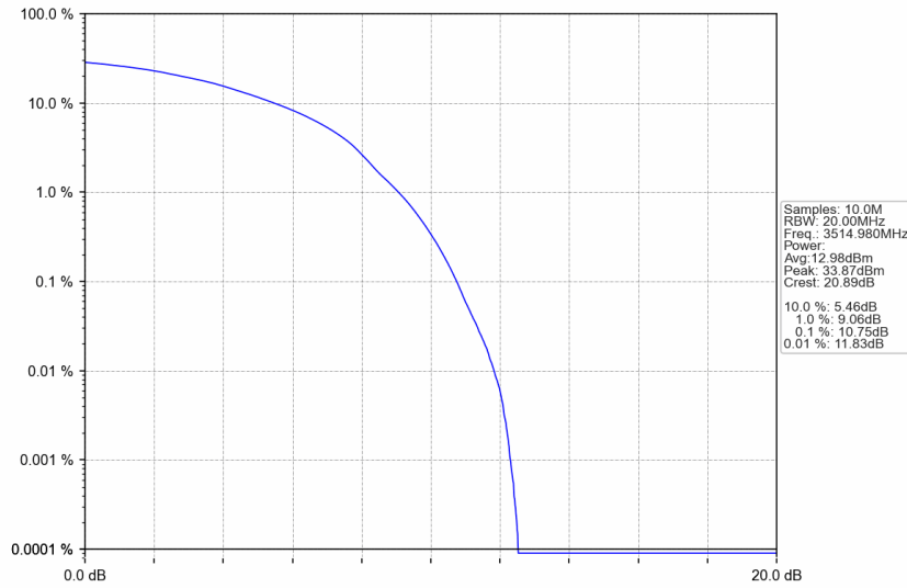
n77d_30kHz_SISO_NTNV_70MHz_DFT-s-OFDM 256 QAM_3514.98MHz_Outer_Full
