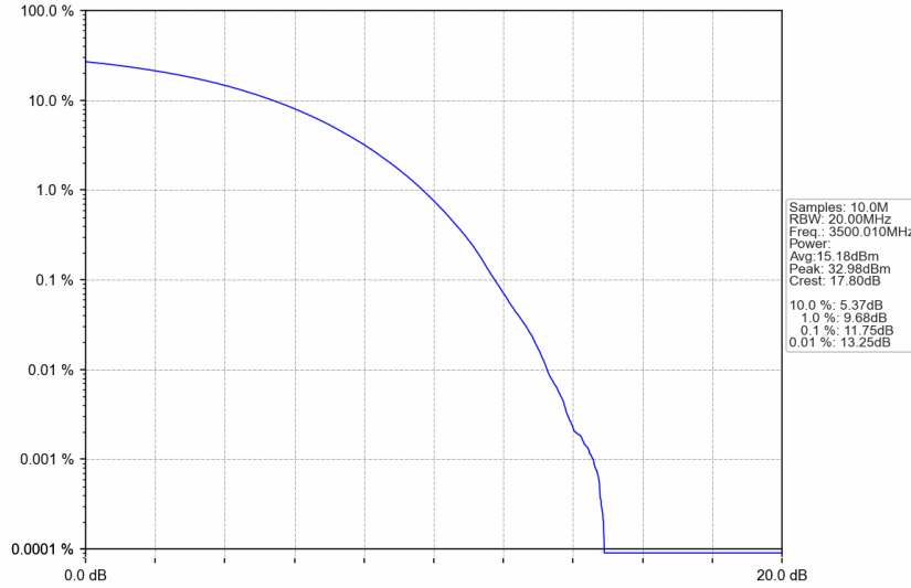
n77d_30kHz_SISO_NTNV_50MHz_CP-OFDM 64 QAM_3500.01MHz_Outer_Full
