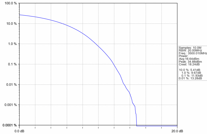
n77d_30kHz_SISO_NTNV_40MHz_CP-OFDM QPSK_3500.01MHz_Outer_Full
