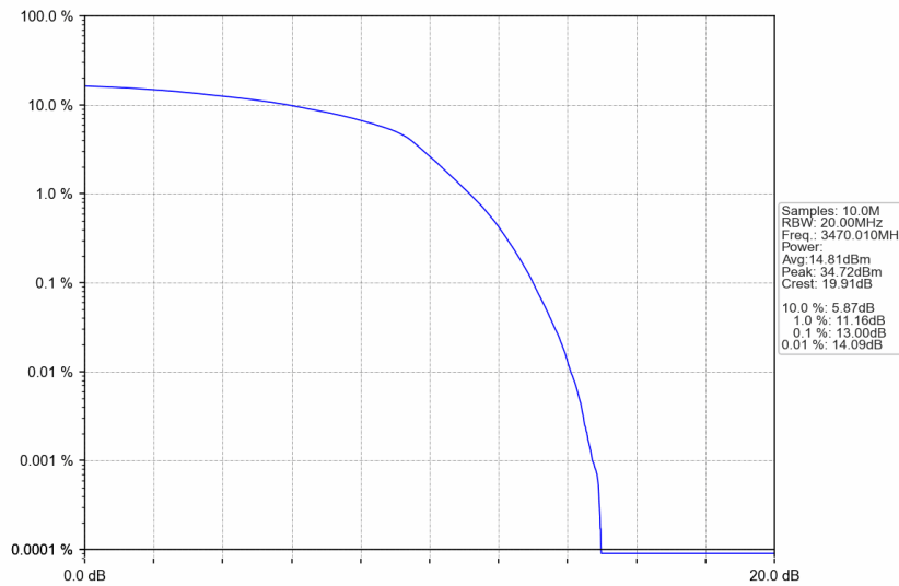
n77d_30kHz_SISO_NTNV_40MHz_DFT-s-OFDM 16 QAM_3470.01MHz_Outer_Full
