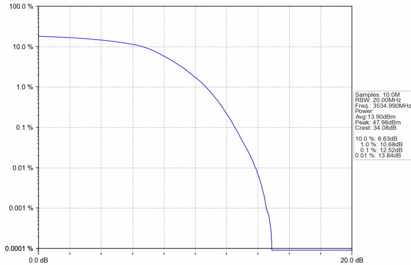
n77d_30kHz_SISO_NTNV_30MHz_DFT-s-OFDM 256 QAM_3534.99MHz_Outer_Full
