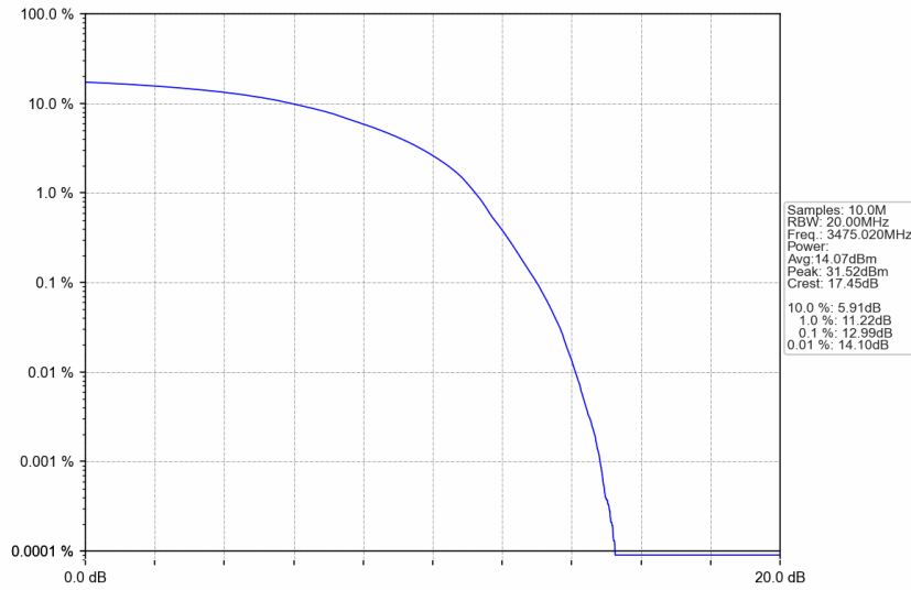
n77d_30kHz_SISO_NTNV_50MHz_DFT-s-OFDM 16 QAM_3475.02MHz_Outer_Full
