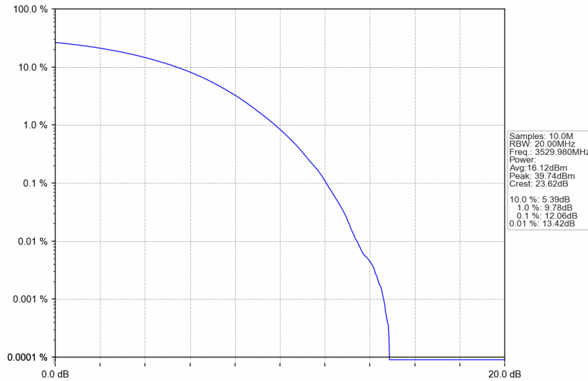
n77d_30kHz_SISO_NTNV_40MHz_CP-OFDM 64 QAM_3529.98MHz_Outer_Full
