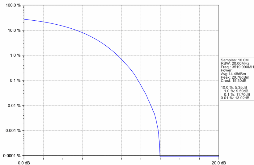
n77d_30kHz_SISO_NTNV_60MHz_CP-OFDM 64 QAM_3519.99MHz_Outer_Full
