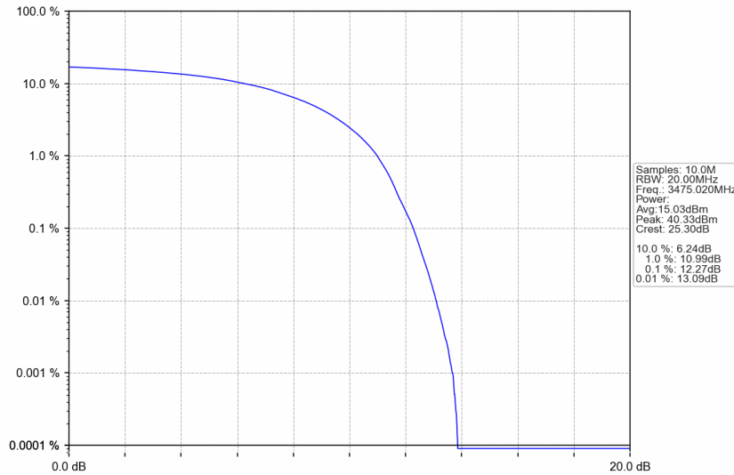
n77d_30kHz_SISO_NTNV_50MHz_DFT-s-OFDM QPSK_3475.02MHz_Outer_Full
