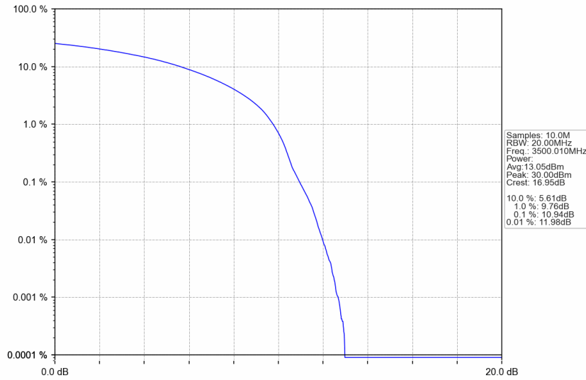
n77d_30kHz_SISO_NTNV_60MHz_DFT-s-OFDM 256 QAM_3500.01MHz_Outer_c Full
