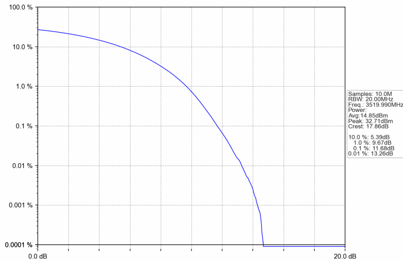
n77d_30kHz_SISO_NTNV_60MHz_CP-OFDM QPSK_3519.99MHz_Outer_Full
