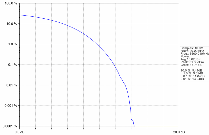
n77d_30kHz_SISO_NTNV_50MHz_CP-OFDM QPSK_3500.01MHz_Outer_Full
