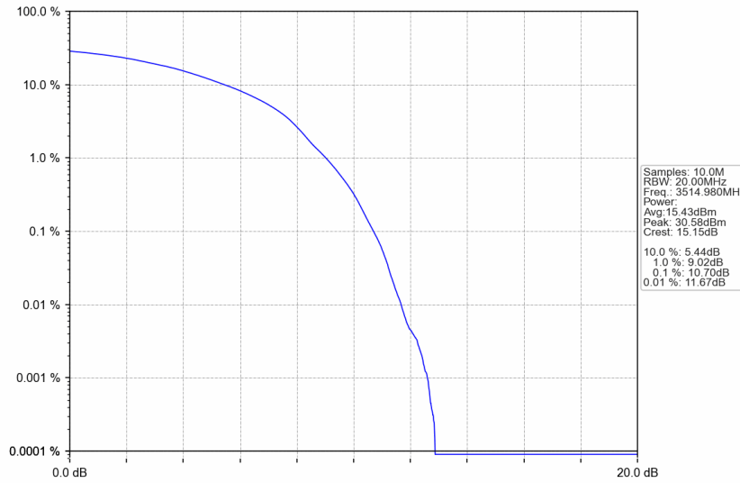
n77d_30kHz_SISO_NTNV_70MHz_DFT-s-OFDM 16 QAM_3514.98MHz_Outer_Full
