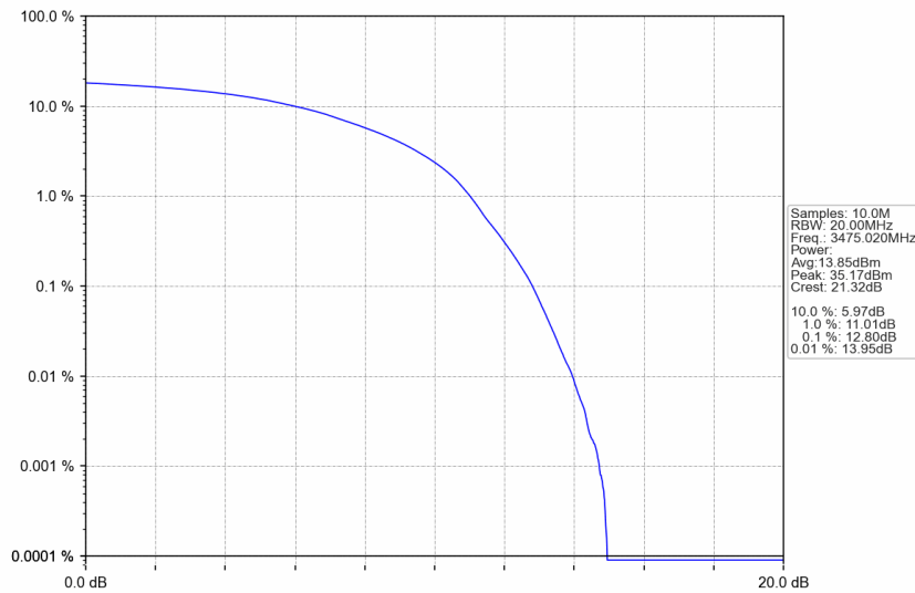
n77d_30kHz_SISO_NTNV_50MHz_DFT-s-OFDM 64 QAM_3475.02MHz_Outer_Full
