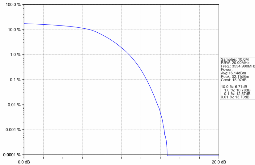
n77d_30kHz_SISO_NTNV_30MHz_DFT-s-OFDM 16 QAM_3534.99MHz_Outer_Full
