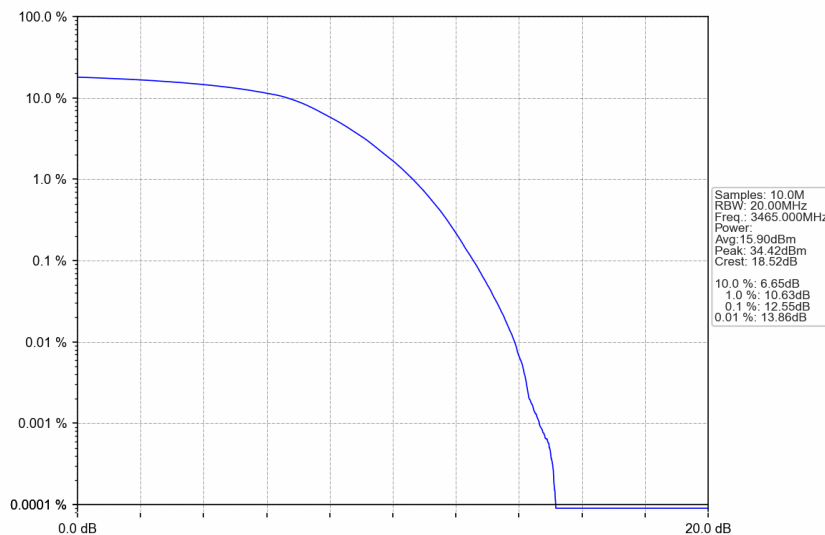
n77d_30kHz_SISO_NTNV_30MHz_DFT-s-OFDM 64 QAM_3465MHz_Outer_Full
