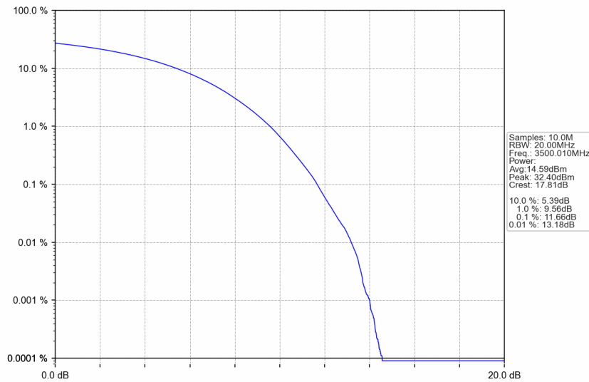
n77d_30kHz_SISO_NTNV_30MHz_CP-OFDM 256 QAM_3500.01MHz_Outer_Full
