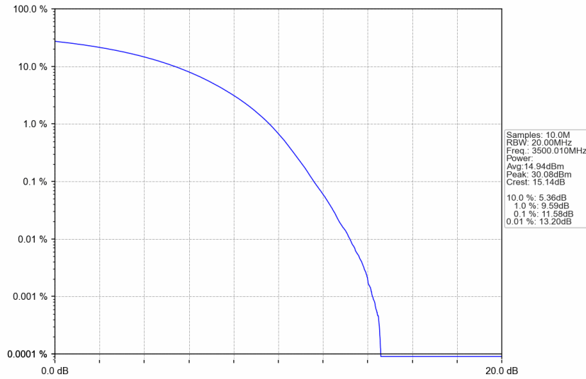
n77d_30kHz_SISO_NTNV_60MHz_CP-OFDM QPSK_3500.01MHz_Outer_Full
