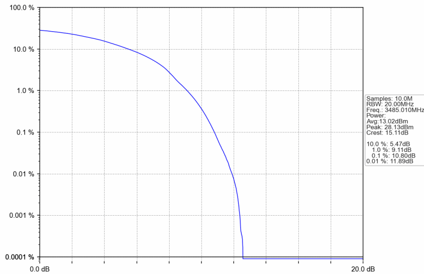
n77d_30kHz_SISO_NTNV_70MHz_DFT-s-OFDM 256 QAM_3485.01MHz_Outer_Full
