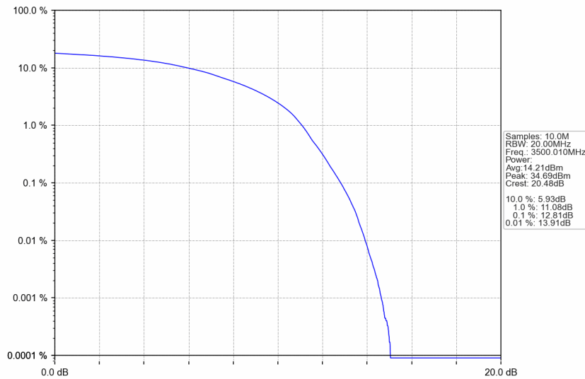
n77d_30kHz_SISO_NTNV_50MHz_DFT-s-OFDM 16 QAM_3500.01MHz_Outer_Full
