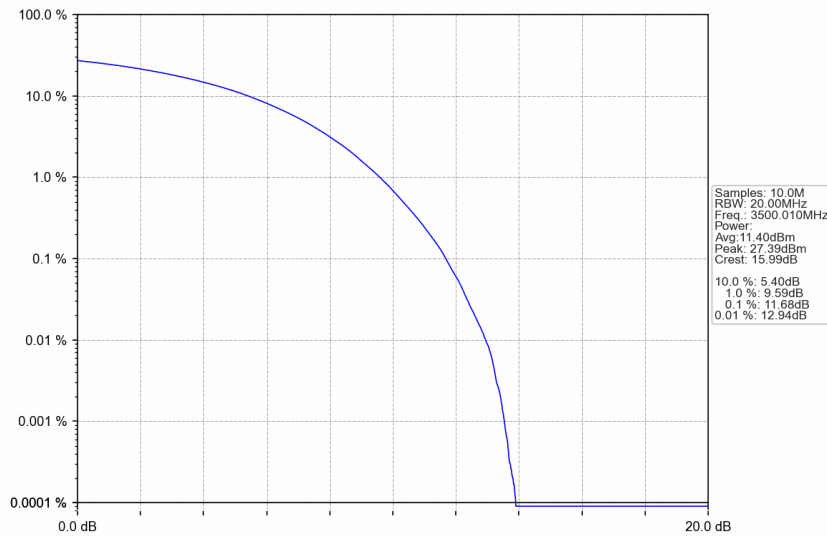
n77d_30kHz_SISO_NTNV_60MHz_CP-OFDM 256 QAM_3500.01MHz_Outer_Full
