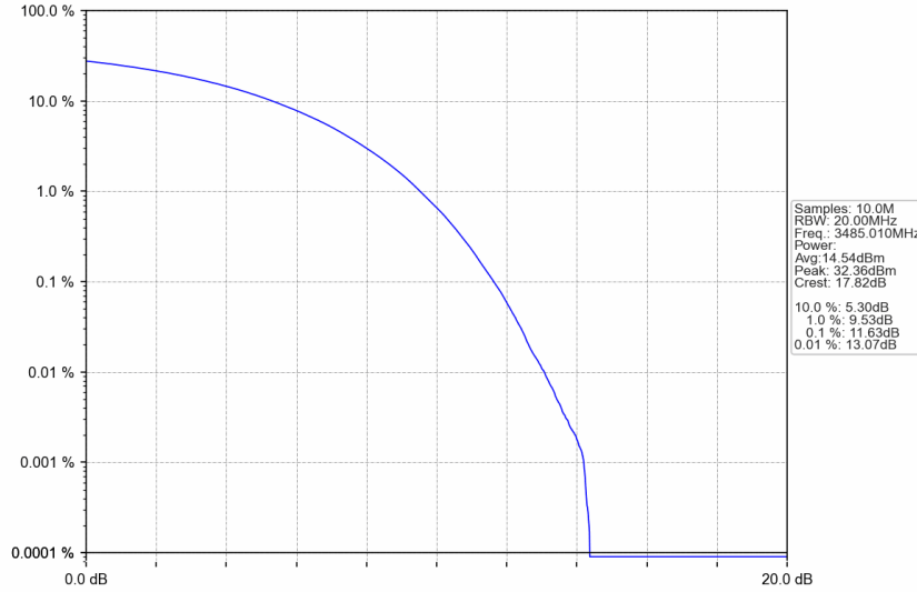
n77d_30kHz_SISO_NTNV_70MHz_CP-OFDM 16 QAM_3485.01MHz_Outer_Full
