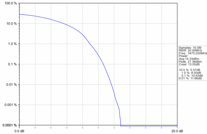
n77d_30kHz_SISO_NTNV_50MHz_DFT-s-OFDM 256 QAM_3475.02MHz_Outer_Full
