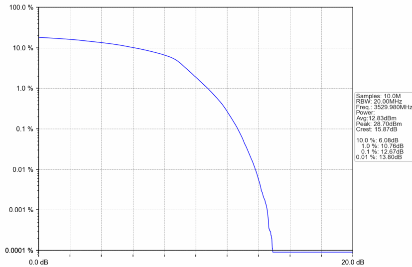
n77d_30kHz_SISO_NTNV_40MHz_DFT-s-OFDM 256 QAM_3529.98MHz_Outer_Full
