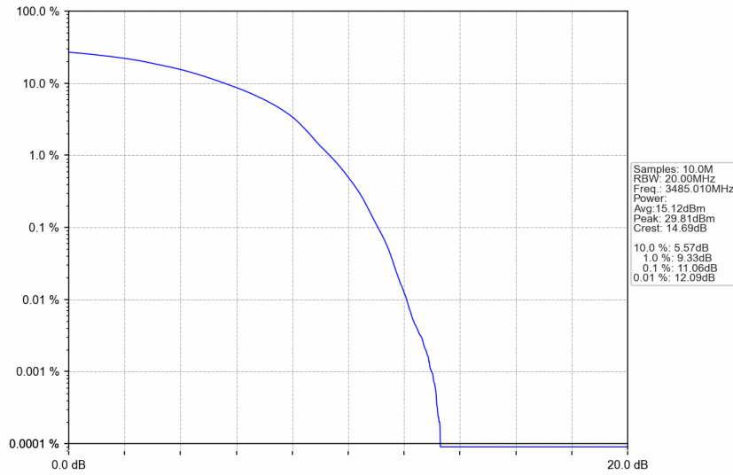
n77d_30kHz_SISO_NTNV_70MHz_DFT-s-OFDM 16 QAM_3485.01MHz_Outer_Full
