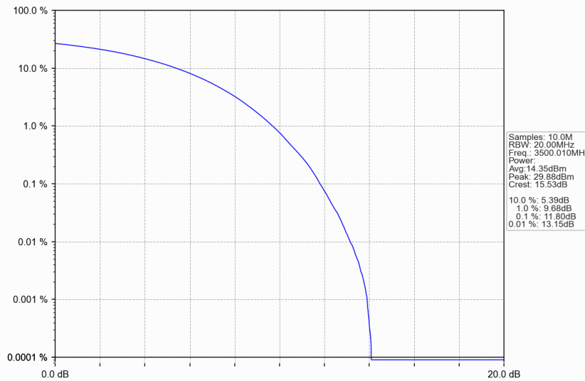
n77d_30kHz_SISO_NTNV_60MHz_CP-OFDM 64 QAM_3500.01MHz_Outer_Full
