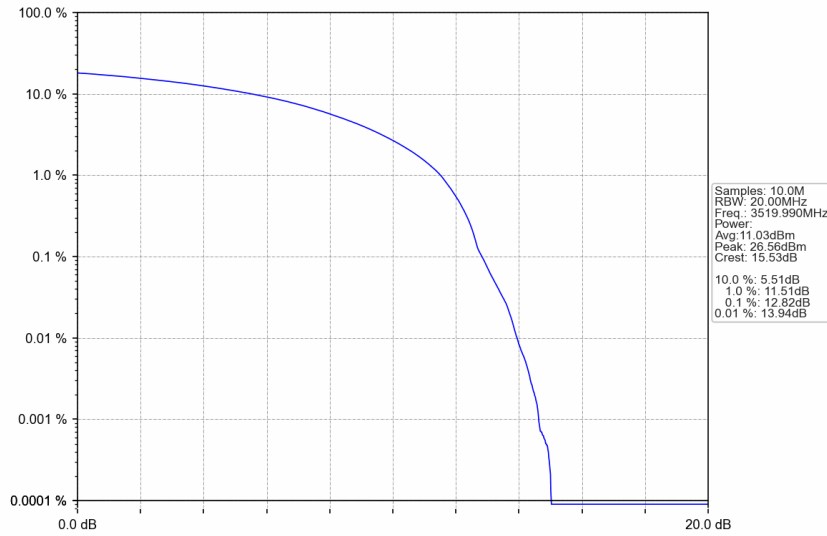
n77d_30kHz_SISO_NTNV_60MHz_DFT-s-OFDM 256 QAM_3519.99MHz_Outer_Full
