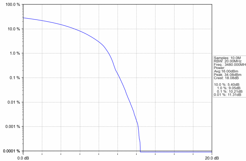
n77d_30kHz_SISO_NTNV_60MHz_DFT-s-OFDM 64 QAM_3480MHz_Outer_Full
