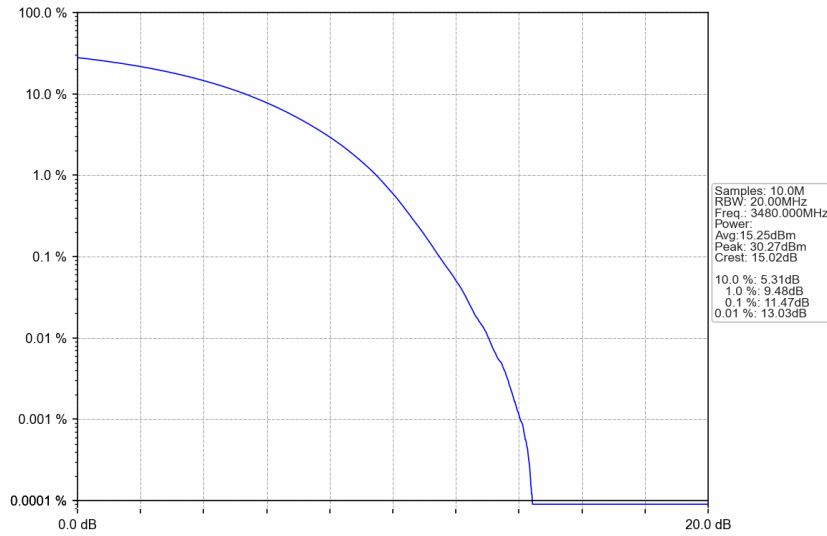
n77d_30kHz_SISO_NTNV_60MHz_CP-OFDM QPSK_3480MHz_Outer_Full
