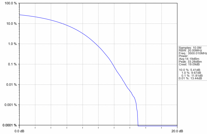
n77d_30kHz_SISO_NTNV_70MHz_CP-OFDM QPSK_3500.01MHz_Outer_Full
