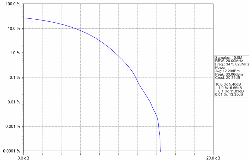
n77d_30kHz_SISO_NTNV_50MHz_CP-OFDM 256 QAM_3475.02MHz_Outer_Full
