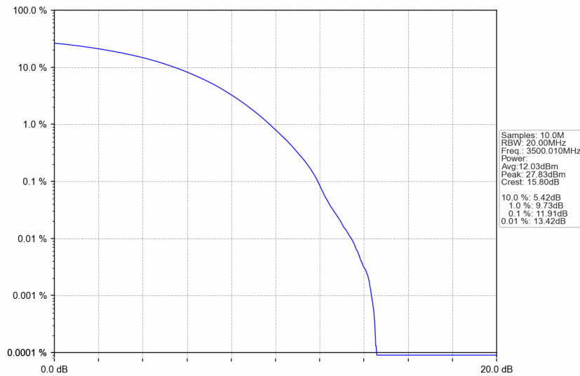
n77d_30kHz_SISO_NTNV_50MHz_CP-OFDM 256 QAM_3500.01MHz_Outer_Full
