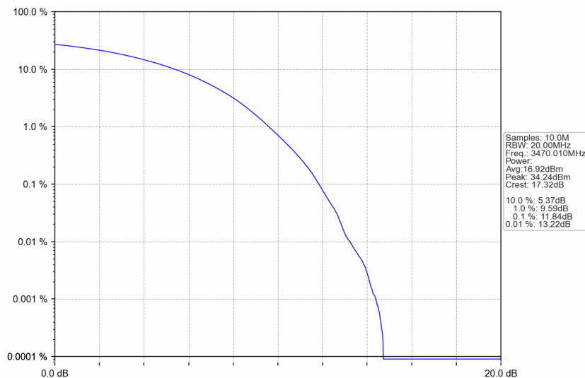
n77d_30kHz_SISO_NTNV_40MHz_CP-OFDM QPSK_3470.01MHz_Outer_Full
