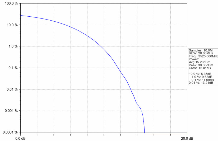
n77d_30kHz_SISO_NTNV_50MHz_CP-OFDM 64 QAM_3525MHz_Outer_Full
