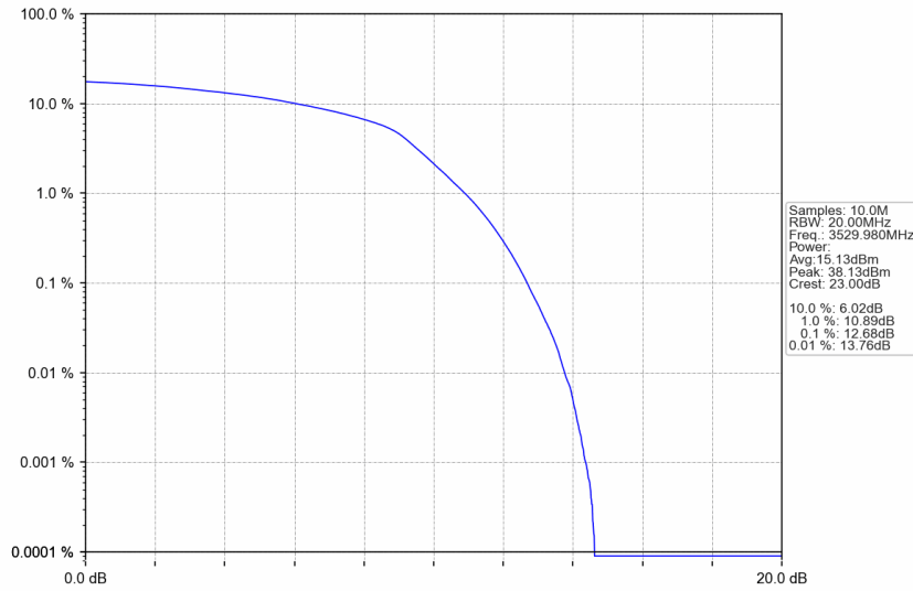
n77d_30kHz_SISO_NTNV_40MHz_DFT-s-OFDM 16 QAM_3529.98MHz_Outer_Full
