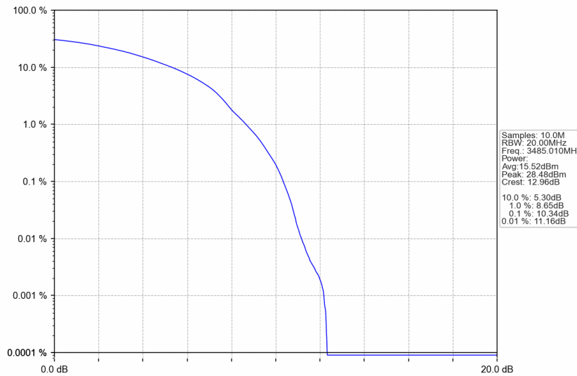
n77d_30kHz_SISO_NTNV_70MHz_DFT-s-OFDM 64 QAM_3485.01MHz_Outer_Full
