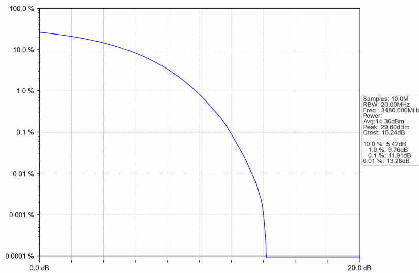
n77d_30kHz_SISO_NTNV_60MHz_CP-OFDM 64 QAM_3480MHz_Outer_Full
