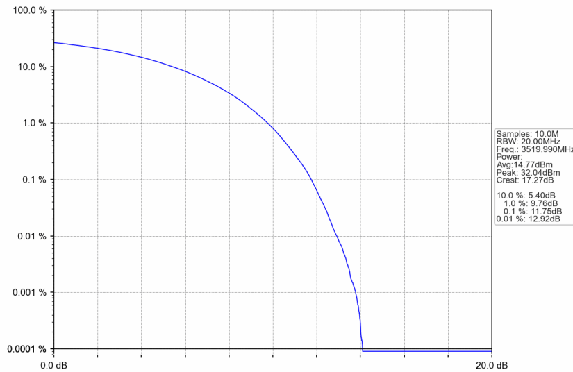
n77d_30kHz_SISO_NTNV_60MHz_CP-OFDM 16 QAM_3519.99MHz_Outer_Full
