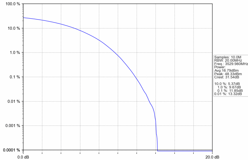
n77d_30kHz_SISO_NTNV_40MHz_CP-OFDM 16 QAM_3529.98MHz_Outer_Full
