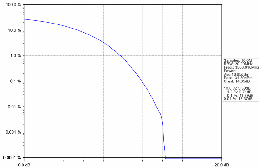
n77d_30kHz_SISO_NTNV_40MHz_CP-OFDM 16 QAM_3500.01MHz_Outer_Full
