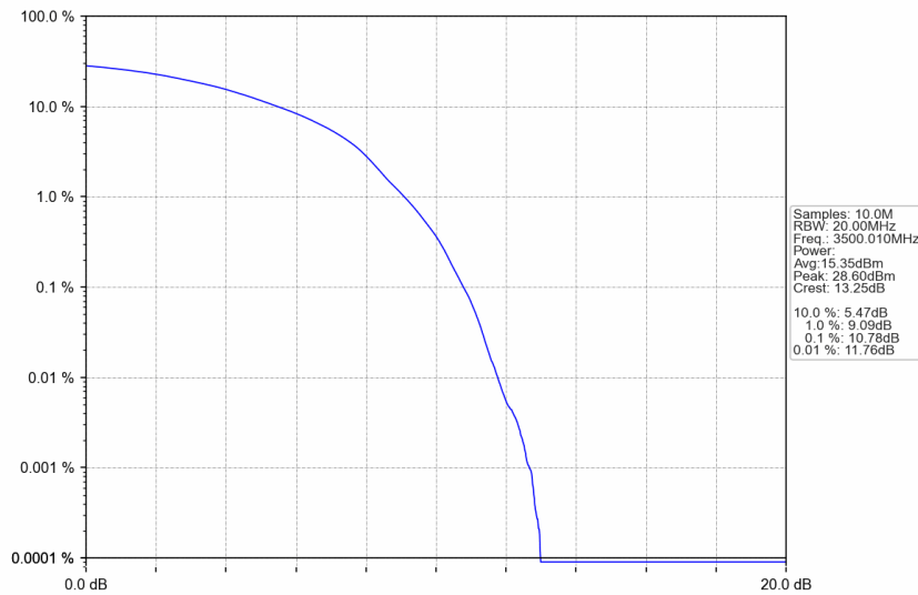
n77d_30kHz_SISO_NTNV_70MHz_DFT-s-OFDM 16 QAM_3500.01MHz_Outer_Full
