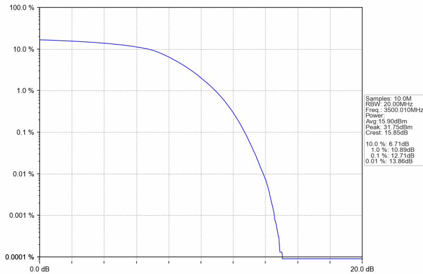
n77d_30kHz_SISO_NTNV_30MHz_DFT-s-OFDM 16 QAM_3500.01MHz_Outer_Full
