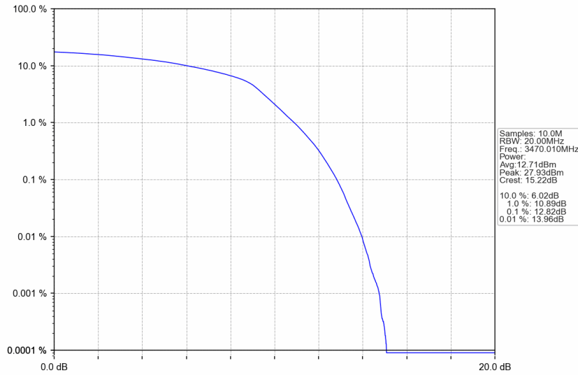
n77d_30kHz_SISO_NTNV_40MHz_DFT-s-OFDM 256 QAM_3470.01MHz_Outer_Full
