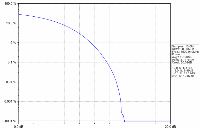
n77d_30kHz_SISO_NTNV_30MHz_CP-OFDM 64 QAM_3500.01MHz_Outer_Full
