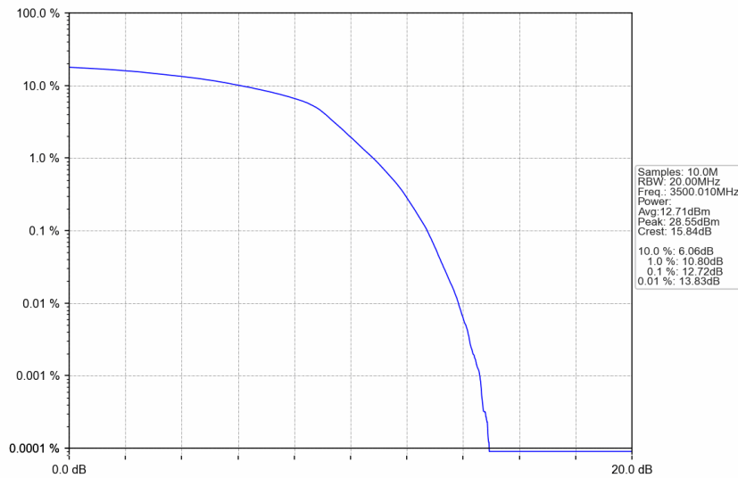
n77d_30kHz_SISO_NTNV_40MHz_DFT-s-OFDM 256 QAM_3500.01MHz_Outer_c_Full
