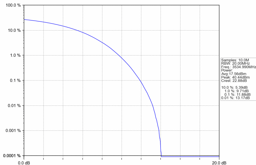
n77d_30kHz_SISO_NTNV_30MHz_CP-OFDM 64 QAM_3534.99MHz_Outer_Full
