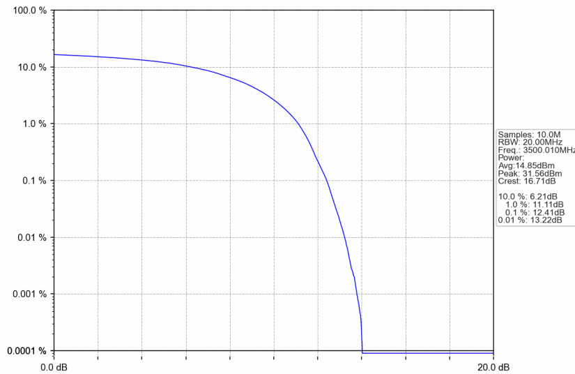
n77d_30kHz_SISO_NTNV_50MHz_DFT-s-OFDM QPSK_3500.01MHz_Outer_Full
