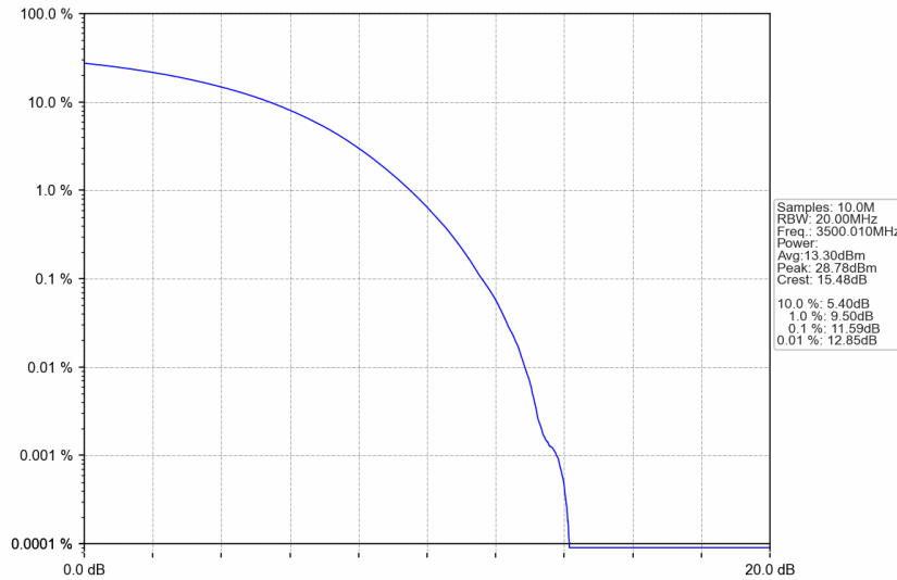
n77d_30kHz_SISO_NTNV_40MHz_CP-OFDM 256 QAM_3500.01MHz_Outer_Full
