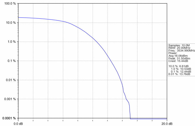
n77d_30kHz_SISO_NTNV_30MHz_DFT-s-OFDM 64 QAM_3534.99MHz_Outer_Full
