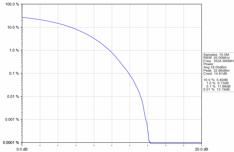
n77d_30kHz_SISO_NTNV_30MHz_CP-OFDM 16 QAM_3534.99MHz_Outer_Full
