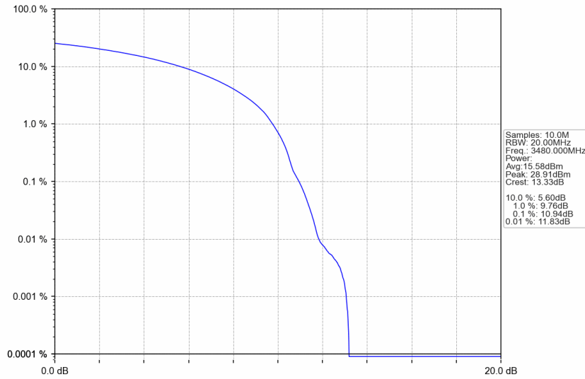
n77d_30kHz_SISO_NTNV_60MHz_DFT-s-OFDM 16 QAM_3480MHz_Outer_Full
