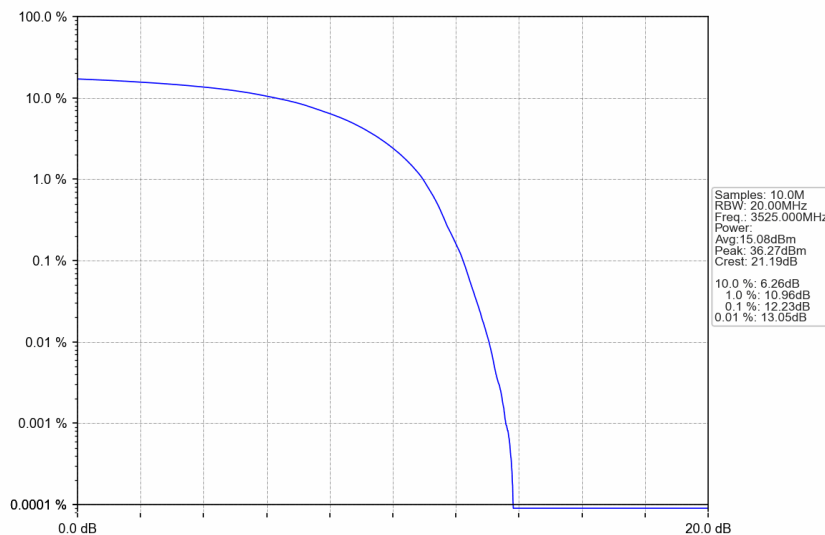
n77d_30kHz_SISO_NTNV_50MHz_DFT-s-OFDM QPSK_3525MHz_Outer_Full
