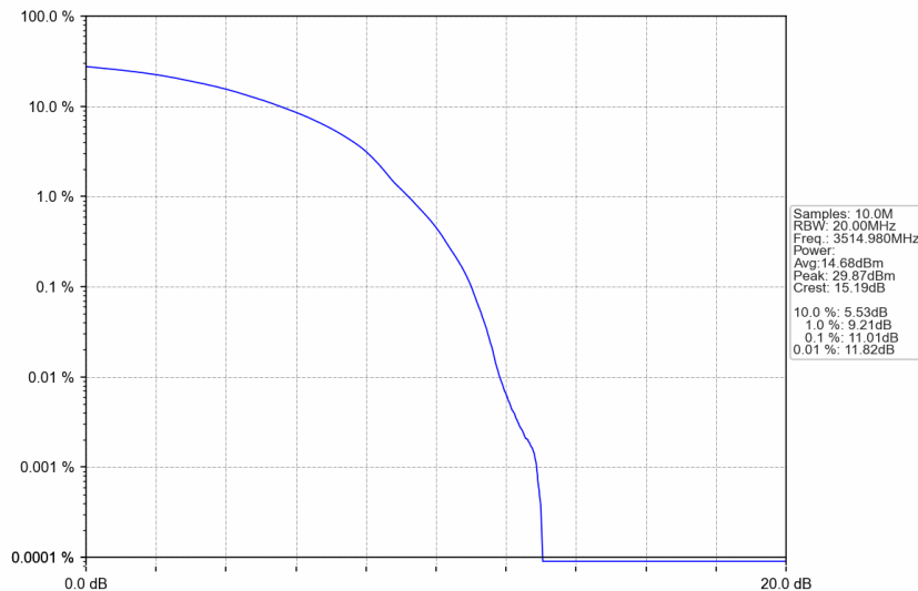
n77d_30kHz_SISO_NTNV_70MHz_DFT-s-OFDM 64 QAM_3514.98MHz_Outer_Full
