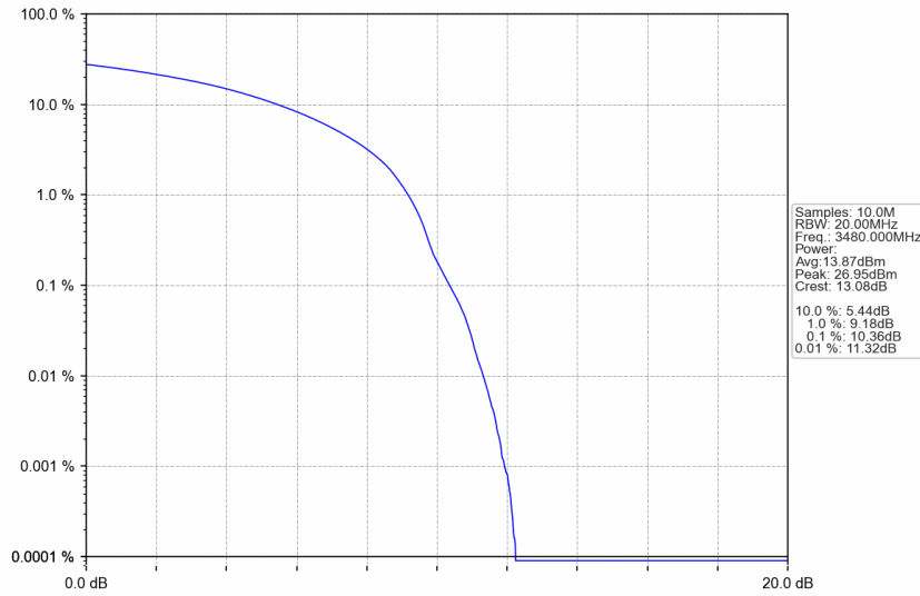
n77d_30kHz_SISO_NTNV_60MHz_DFT-s-OFDM 256 QAM_3480MHz_Outer_Full
