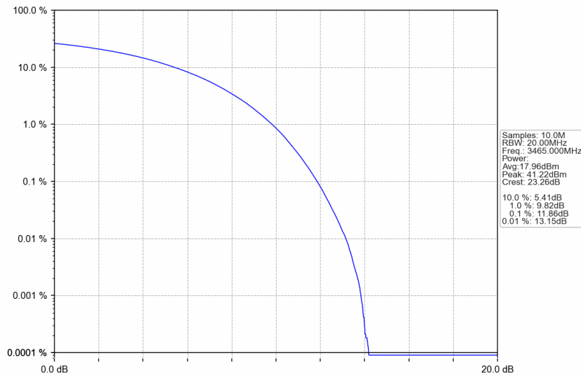
n77d_30kHz_SISO_NTNV_30MHz_CP-OFDM QPSK_3465MHz_Outer_Full
