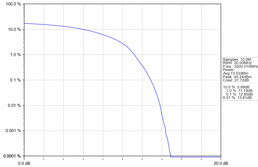
n77d_30kHz_SISO_NTNV_70MHz_DFT-s-OFDM QPSK_3500.01MHz_Outer_Full
