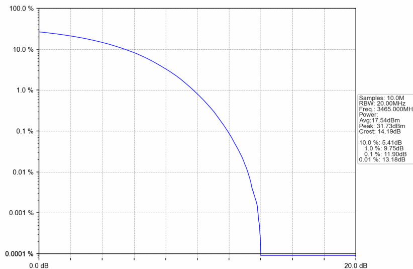
n77d_30kHz_SISO_NTNV_30MHz_CP-OFDM 64 QAM_3465MHz_Outer_Full
