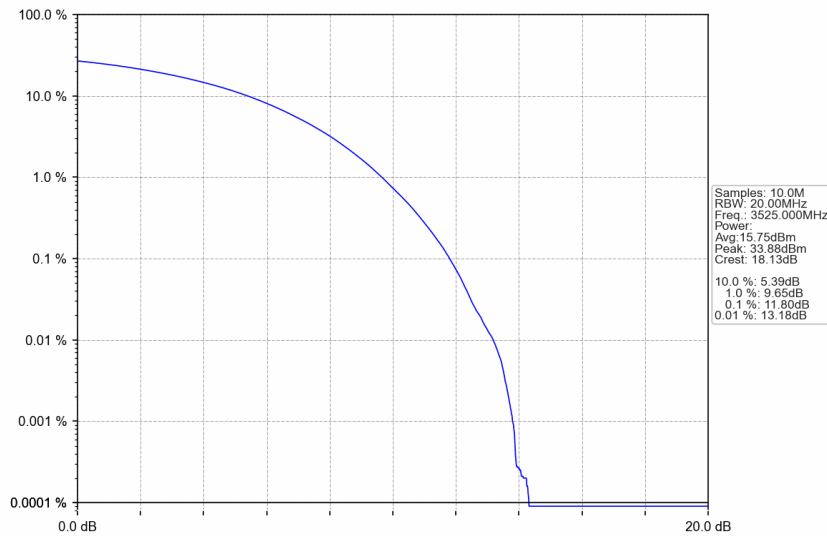
n77d_30kHz_SISO_NTNV_50MHz_CP-OFDM QPSK_3525MHz_Outer_Full
