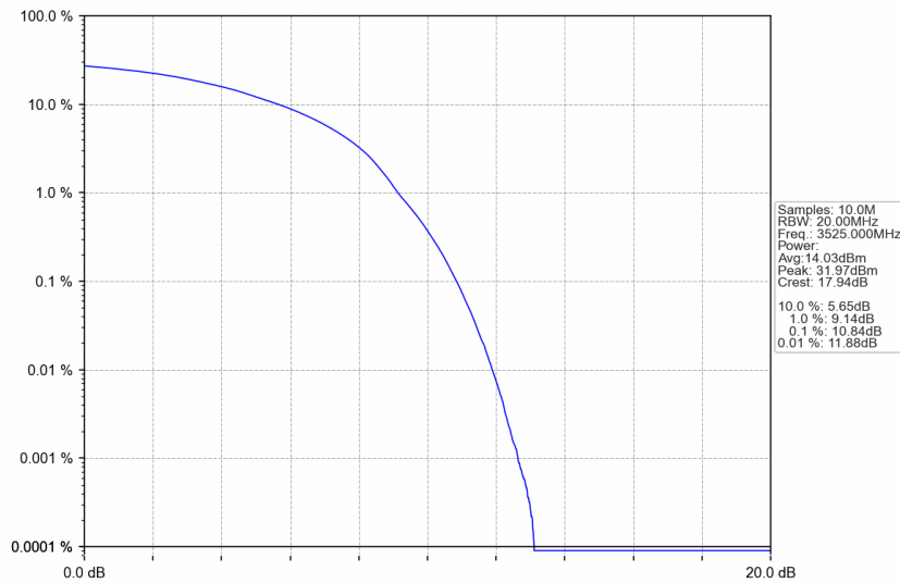
n77d_30kHz_SISO_NTNV_50MHz_DFT-s-OFDM 256 QAM_3525MHz_Outer_Full
