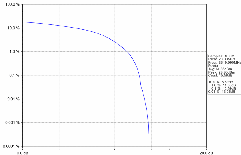
n77d_30kHz_SISO_NTNV_60MHz_DFT-s-OFDM QPSK_3519.99MHz_Outer_Full
