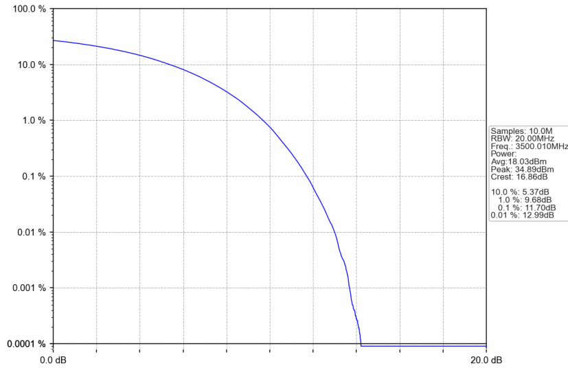
n77d_30kHz_SISO_NTNV_30MHz_CP-OFDM QPSK_3500.01MHz_Outer_Full
