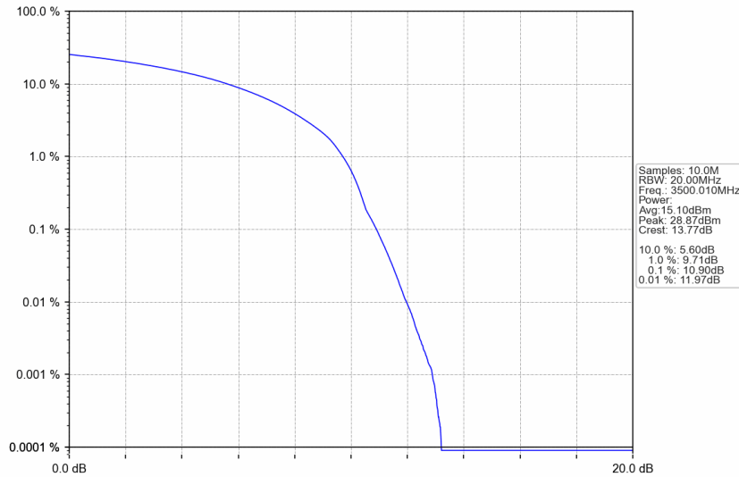
n77d_30kHz_SISO_NTNV_60MHz_DFT-s-OFDM 64 QAM_3500.01MHz_Outer_Full
