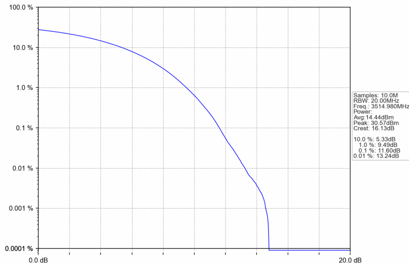
n77d_30kHz_SISO_NTNV_70MHz_CP-OFDM QPSK_3514.98MHz_Outer_Full
