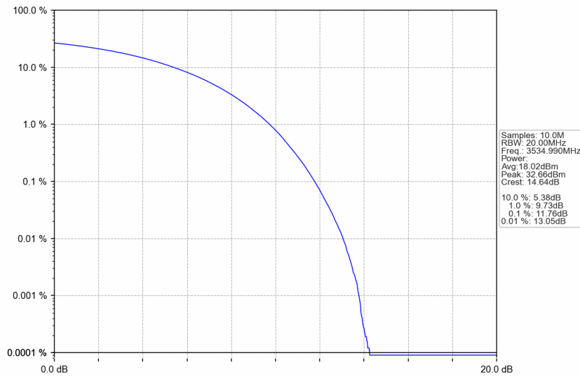
n77d_30kHz_SISO_NTNV_30MHz_CP-OFDM QPSK_3534.99MHz_Outer_Full
