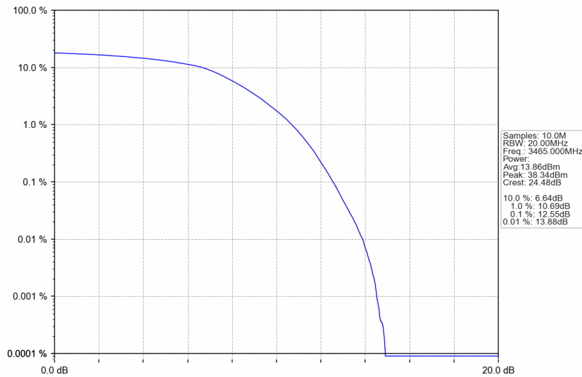
n77d_30kHz_SISO_NTNV_30MHz_DFT-s-OFDM 256 QAM_3465MHz_Outer_Full
