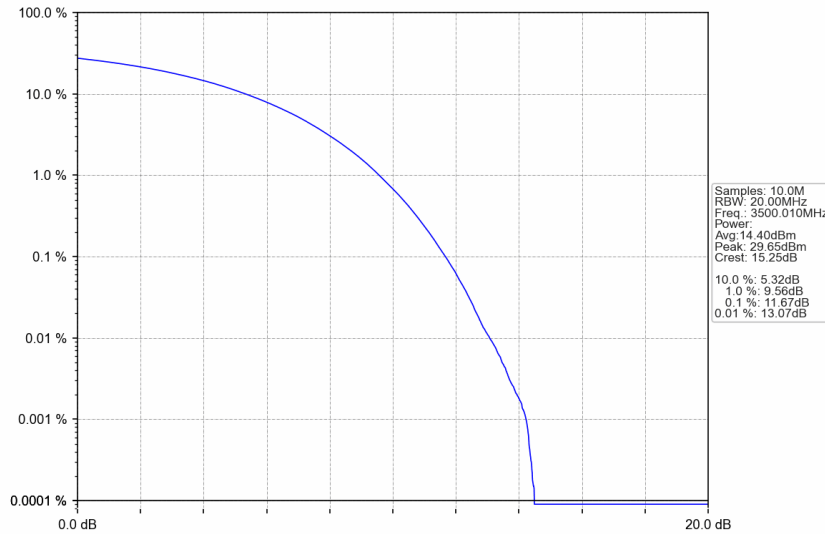
n77d_30kHz_SISO_NTNV_70MHz_CP-OFDM 16 QAM_3500.01MHz_Outer_Full
