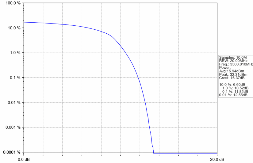
n77d_30kHz_SISO_NTNV_40MHz_DFT-s-OFDM QPSK_3500.01MHz_Outer_Full
