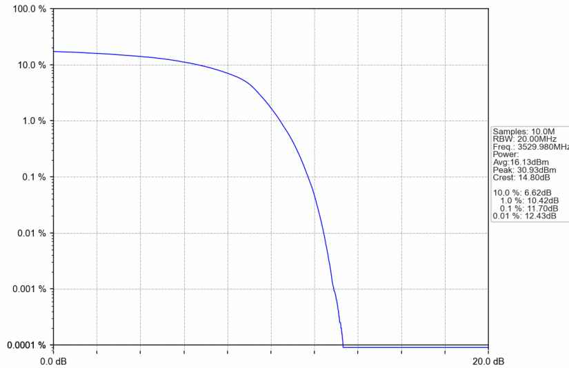
n77d_30kHz_SISO_NTNV_40MHz_DFT-s-OFDM QPSK_3529.98MHz_Outer_Full
