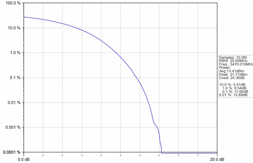
n77d_30kHz_SISO_NTNV_40MHz_CP-OFDM 256 QAM_3470.01MHz_Outer_Full
