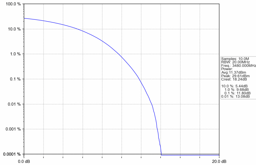
n77d_30kHz_SISO_NTNV_60MHz_CP-OFDM 256 QAM_3480MHz_Outer_Full
