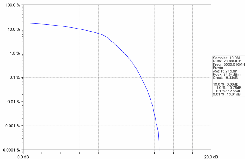
n77d_30kHz_SISO_NTNV_40MHz_DFT-s-OFDM 16 QAM_3500.01MHz_Outer_Full
