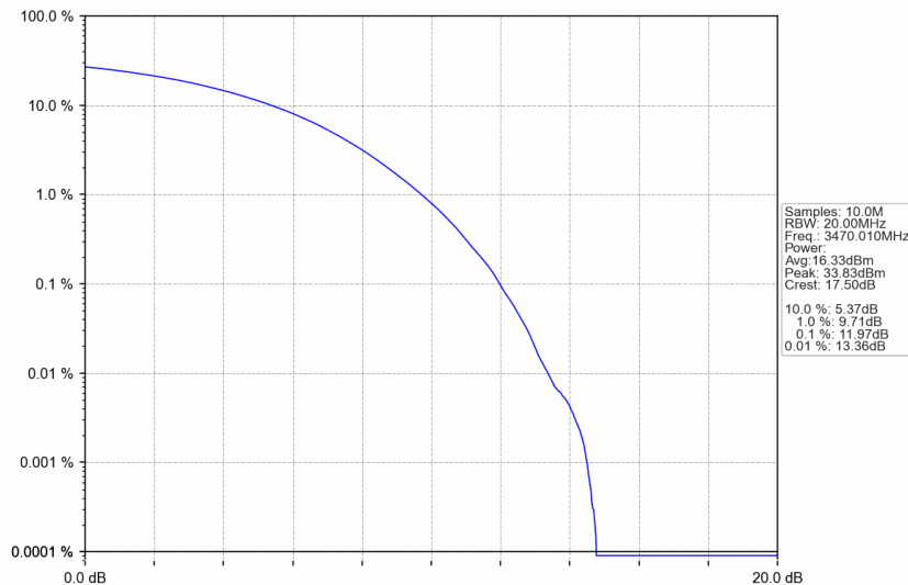
n77d_30kHz_SISO_NTNV_40MHz_CP-OFDM 64 QAM_3470.01MHz_Outer_Full
