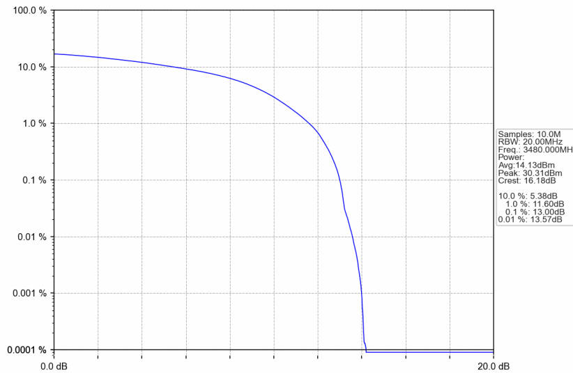
n77d_30kHz_SISO_NTNV_60MHz_DFT-s-OFDM QPSK_3480MHz_Outer_Full
