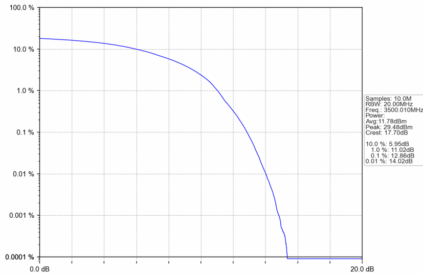
n77d_30kHz_SISO_NTNV_50MHz_DFT-s-OFDM 256 QAM_3500.01MHz_Outer_c_Full
