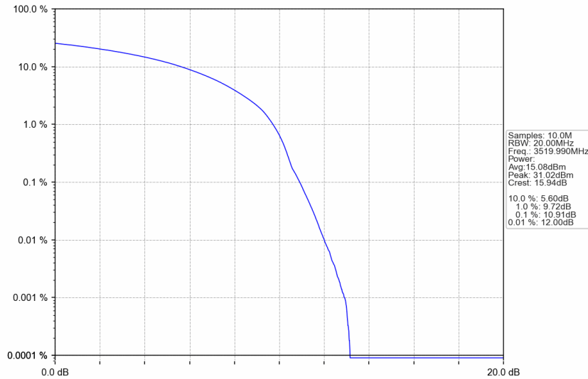
n77d_30kHz_SISO_NTNV_60MHz_DFT-s-OFDM 64 QAM_3519.99MHz_Outer_Full
