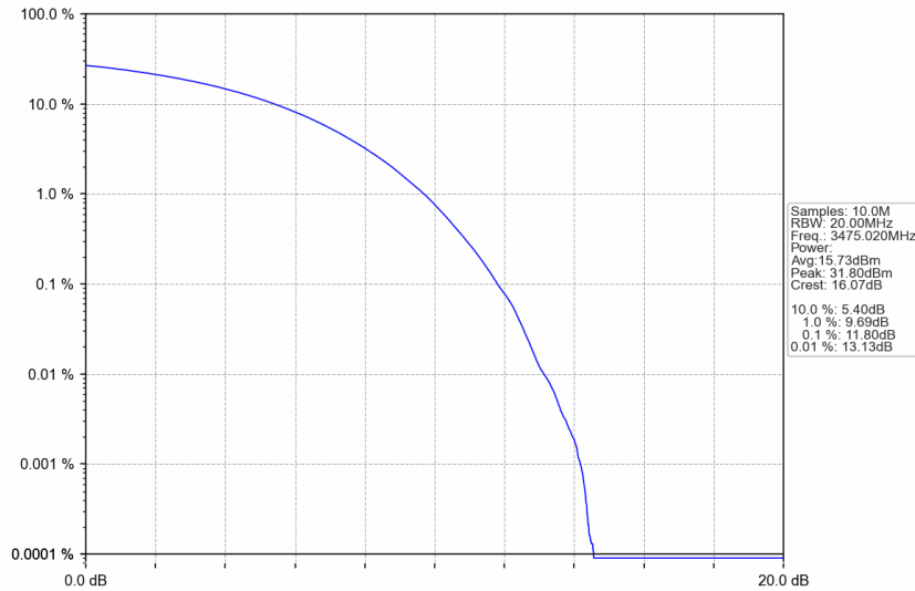
n77d_30kHz_SISO_NTNV_50MHz_CP-OFDM 16 QAM_3475.02MHz_Outer_Full
