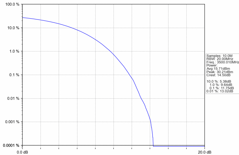
n77d_30kHz_SISO_NTNV_50MHz_CP-OFDM 16 QAM_3500.01MHz_Outer_Full
