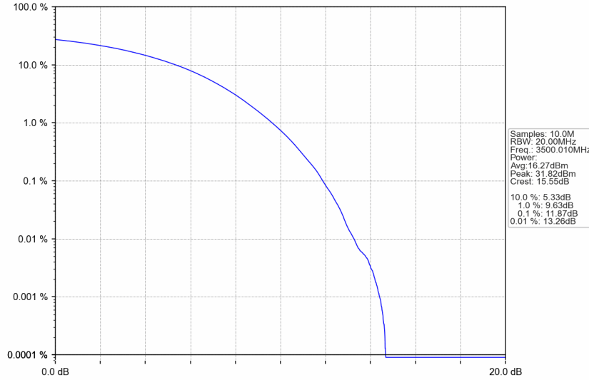
n77d_30kHz_SISO_NTNV_40MHz_CP-OFDM 64 QAM_3500.01MHz_Outer_Full
