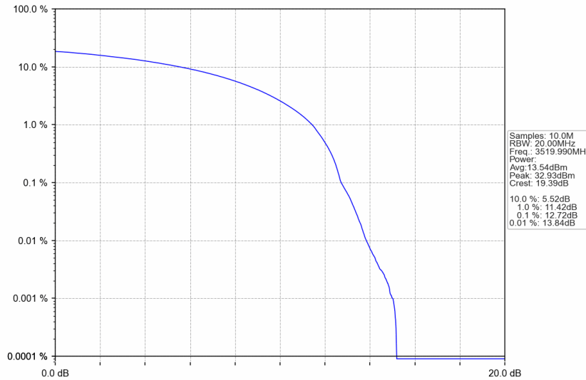
n77d_30kHz_SISO_NTNV_60MHz_DFT-s-OFDM 16 QAM_3519.99MHz_Outer_Full
