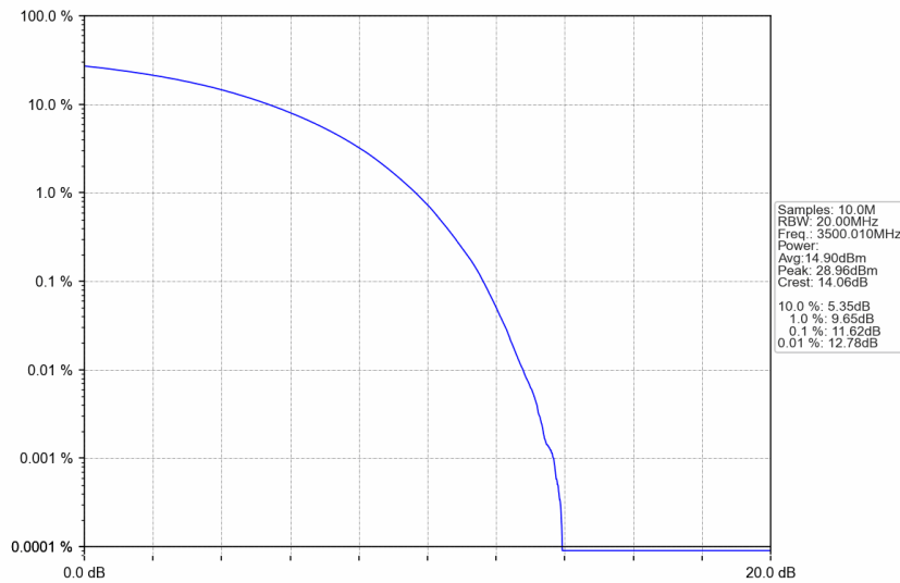
n77d_30kHz_SISO_NTNV_60MHz_CP-OFDM 16 QAM_3500.01MHz_Outer_Full
