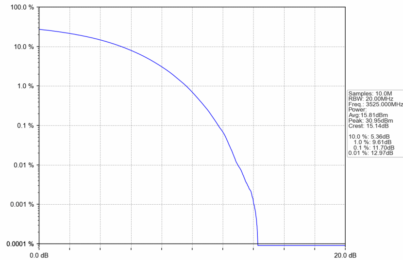
n77d_30kHz_SISO_NTNV_50MHz_CP-OFDM 16 QAM_3525MHz_Outer_Full
