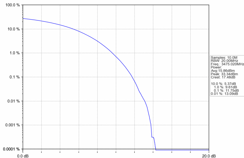
n77d_30kHz_SISO_NTNV_50MHz_CP-OFDM QPSK_3475.02MHz_Outer_Full
