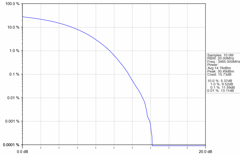
n77d_30kHz_SISO_NTNV_30MHz_CP-OFDM 256 QAM_3465MHz_Outer_Full
