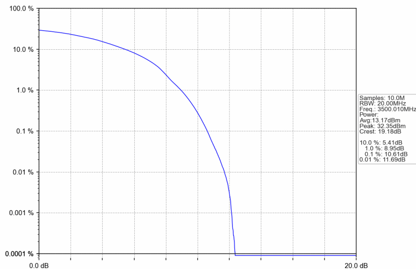
n77d_30kHz_SISO_NTNV_70MHz_DFT-s-OFDM 256 QAM_3500.01MHz_Outer_Full
