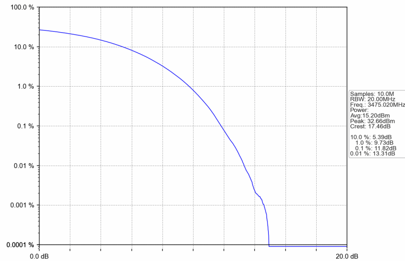
n77d_30kHz_SISO_NTNV_50MHz_CP-OFDM 64 QAM_3475.02MHz_Outer_Full
