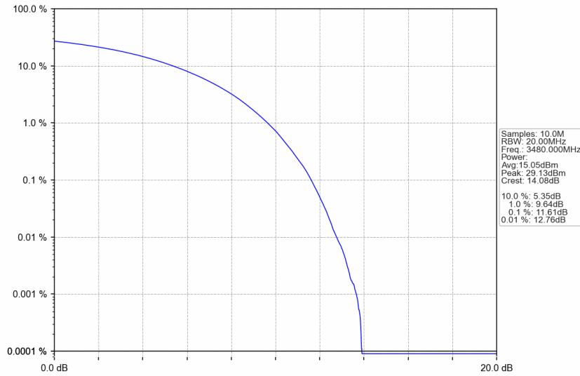
n77d_30kHz_SISO_NTNV_60MHz_CP-OFDM 16 QAM_3480MHz_Outer_Full
