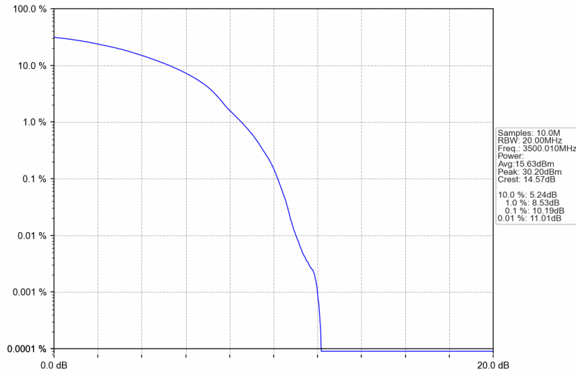
n77d_30kHz_SISO_NTNV_70MHz_DFT-s-OFDM 64 QAM_3500.01MHz_Outer_Full
