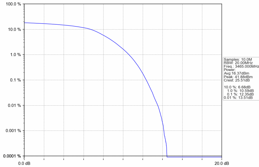
n77d_30kHz_SISO_NTNV_30MHz_DFT-s-OFDM 16 QAM_3465MHz_Outer_Full
