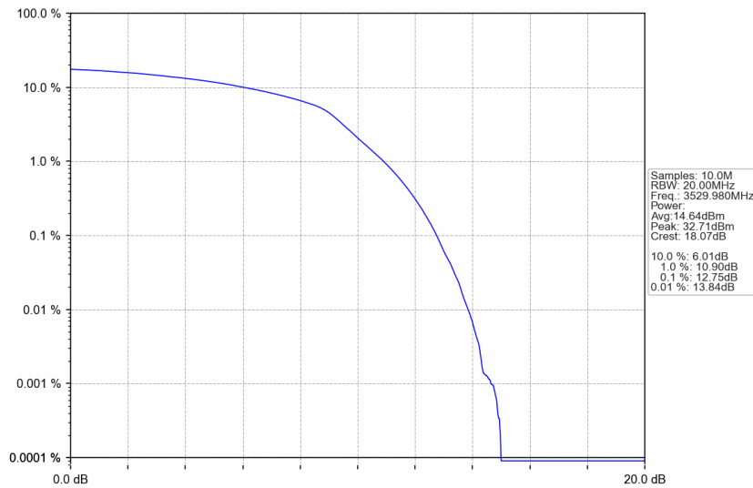
n77d_30kHz_SISO_NTNV_40MHz_DFT-s-OFDM 64 QAM_3529.98MHz_Outer_Full
