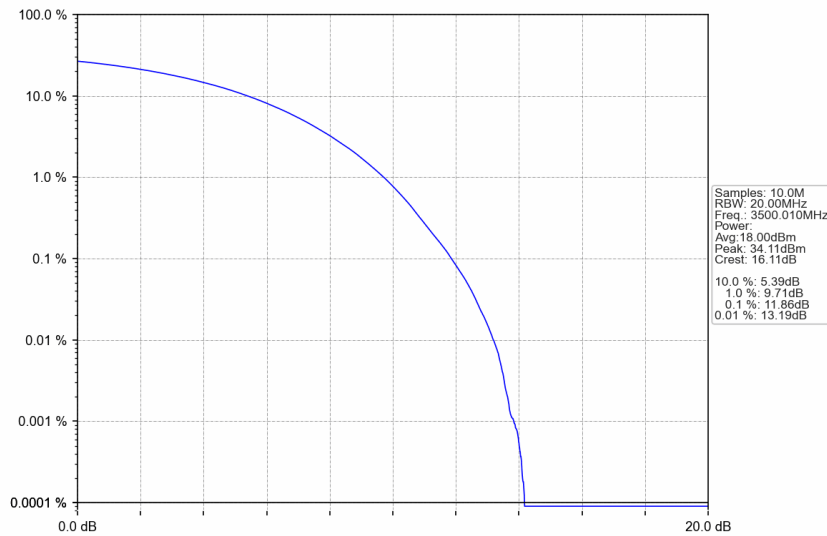
n77d_30kHz_SISO_NTNV_30MHz_CP-OFDM 16 QAM_3500.01MHz_Outer_Full
