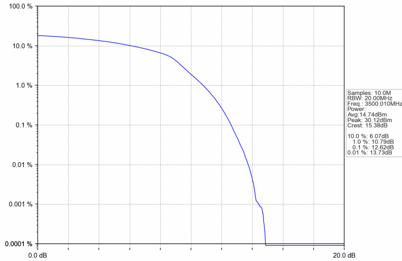
n77d_30kHz_SISO_NTNV_40MHz_DFT-s-OFDM 64 QAM_3500.01MHz_Outer_Full
