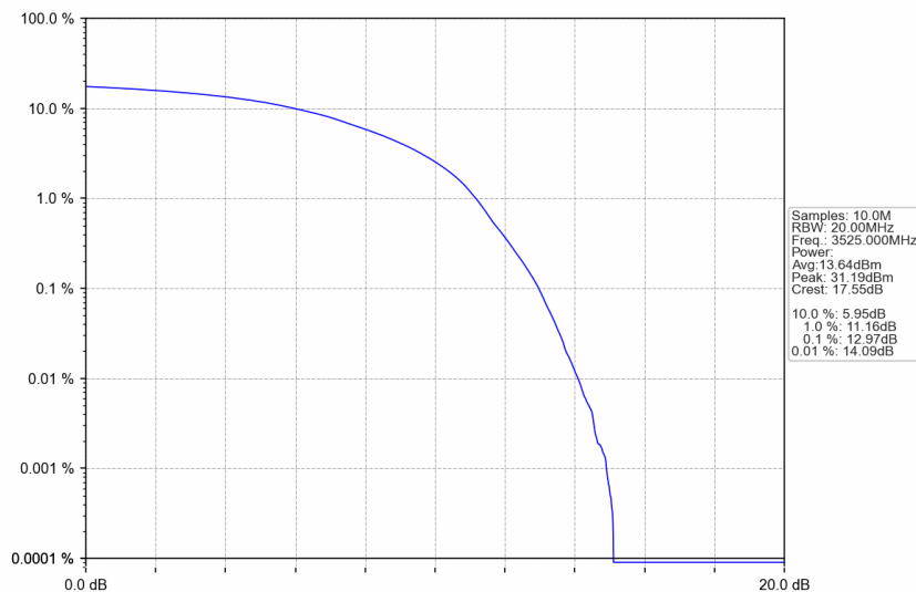
n77d_30kHz_SISO_NTNV_50MHz_DFT-s-OFDM 64 QAM_3525MHz_Outer_Full
