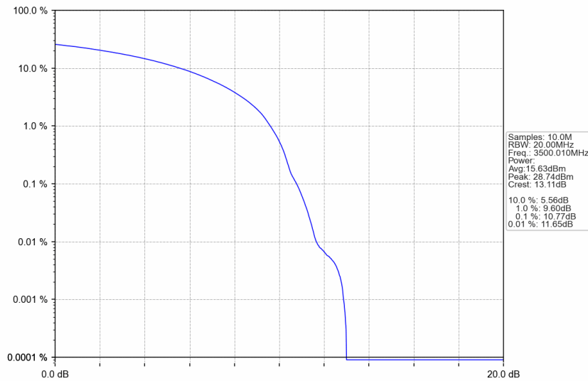
n77d_30kHz_SISO_NTNV_60MHz_DFT-s-OFDM 16 QAM_3500.01MHz_Outer_Full
