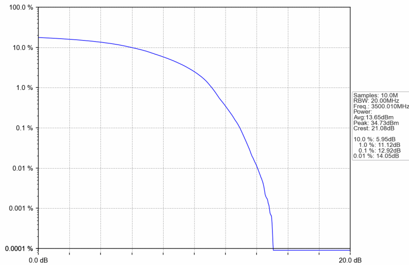
n77d_30kHz_SISO_NTNV_50MHz_DFT-s-OFDM 64 QAM_3500.01MHz_Outer_Full
