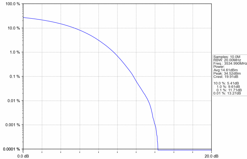
n77d_30kHz_SISO_NTNV_30MHz_CP-OFDM 256 QAM_3534.99MHz_Outer_Full
