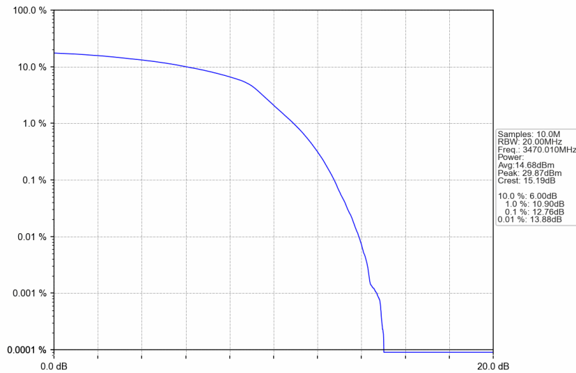
n77d_30kHz_SISO_NTNV_40MHz_DFT-s-OFDM 64 QAM_3470.01MHz_Outer_Full
