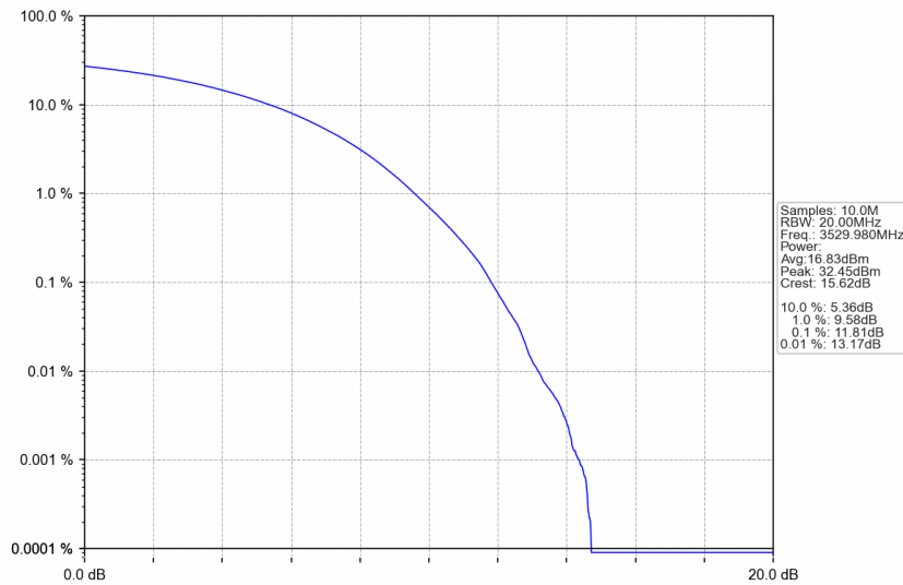
n77d_30kHz_SISO_NTNV_40MHz_CP-OFDM QPSK_3529.98MHz_Outer_Full
