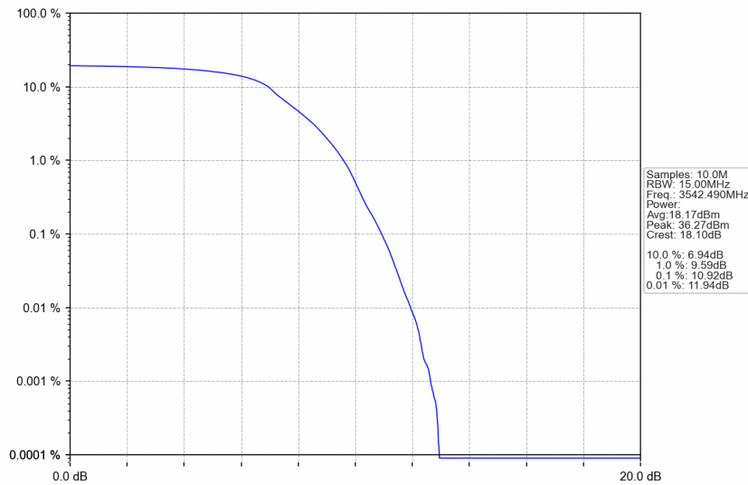
n77d_30kHz_SISO_NTNV_15MHz_DFT-s-OFDM PI/2 BPSK_3542.49MHz_Outer_Full
