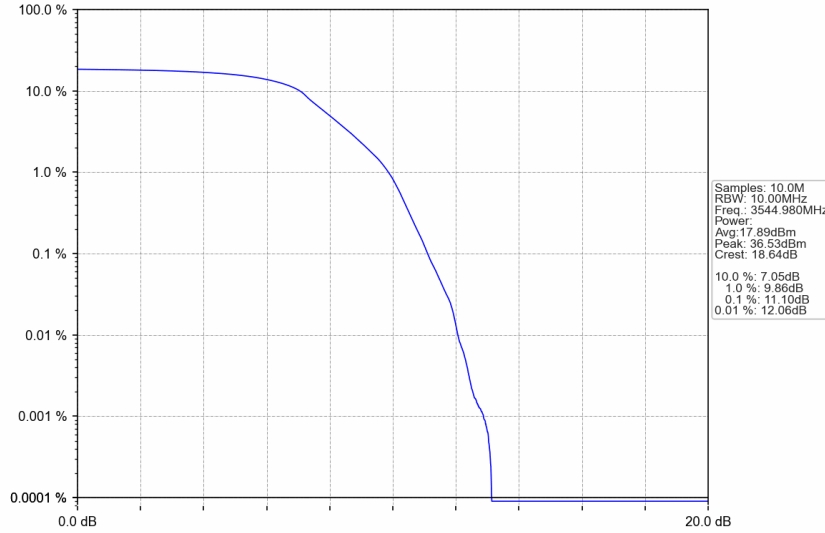
n77d_30kHz_SISO_NTNV_10MHz_DFT-s-OFDM PI/2 BPSK_3544.98MHz_Outer_Full
