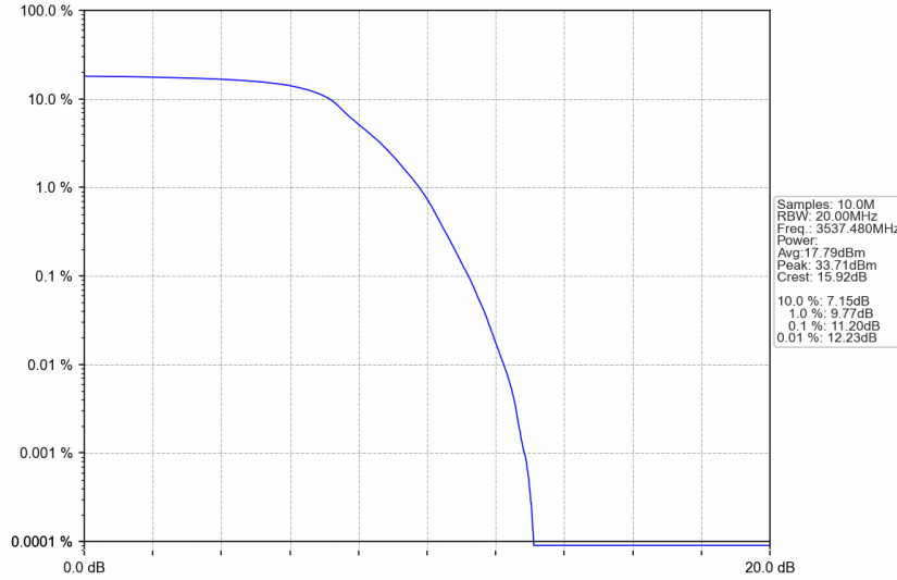
n77d_30kHz_SISO_NTNV_25MHz_DFT-s-OFDM PI/2 BPSK_3537.48MHz_Outer_Full
