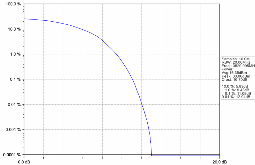
n77d_15kHz_SISO_NTNV_40MHz_DFT-s-OFDM 16 QAM_3529.995MHz_Outer_Full
