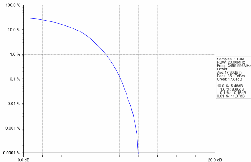
n77d_15kHz_SISO_NTNV_40MHz_DFT-s-OFDM 16 QAM_3499.995MHz_Outer_Full
