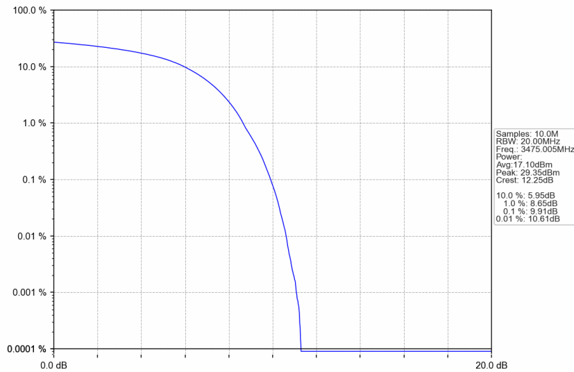
n77d_15kHz_SISO_NTNV_50MHz_DFT-s-OFDM QPSK_3475.005MHz_Outer_Full
