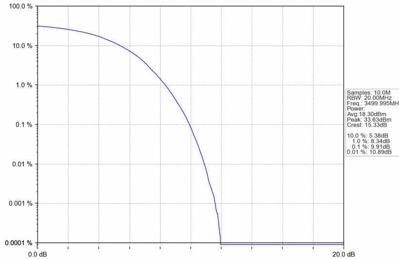
n77d_15kHz_SISO_NTNV_30MHz_DFT-s-OFDM 64 QAM_3499.995MHz_Outer_Full
