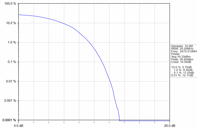
n77d_15kHz_SISO_NTNV_40MHz_DFT-s-OFDM 64 QAM_3470.01MHz_Outer_Full
