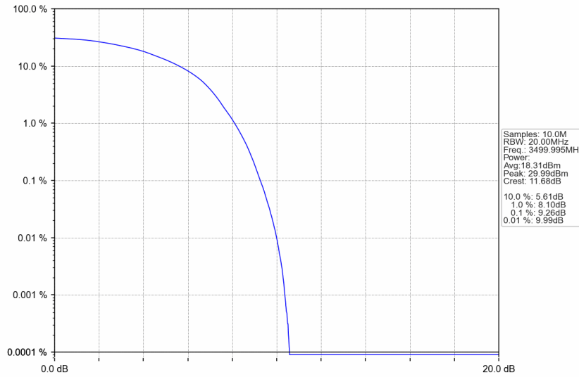
n77d_15kHz_SISO_NTNV_40MHz_DFT-s-OFDM QPSK_3499.995MHz_Outer_Full
