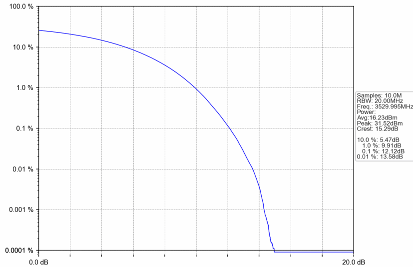
n77d_15kHz_SISO_NTNV_40MHz_CP-OFDM 16 QAM_3529.995MHz_Outer_Full
