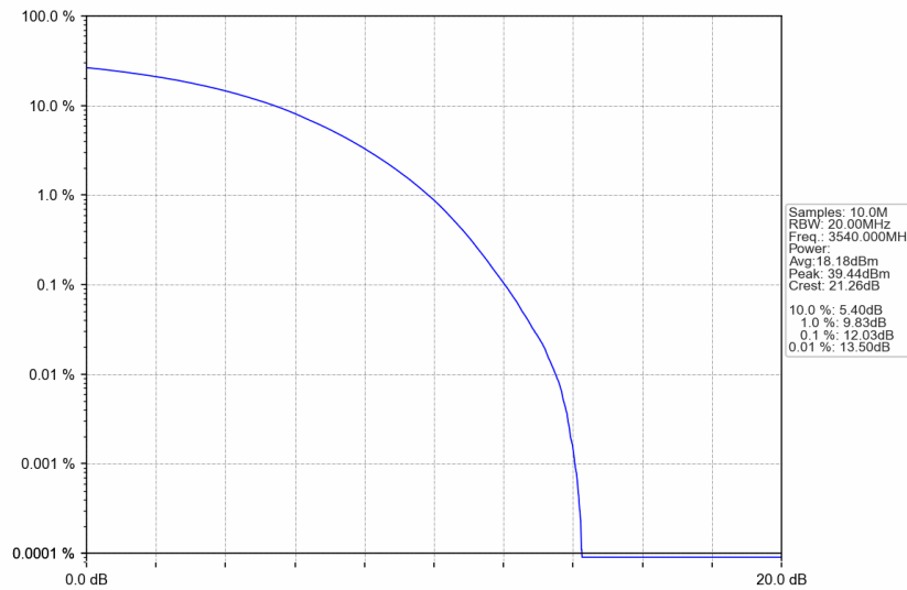
n77d_15kHz_SISO_NTNV_20MHz_CP-OFDM 64 QAM_3540MHz_Outer_Full
