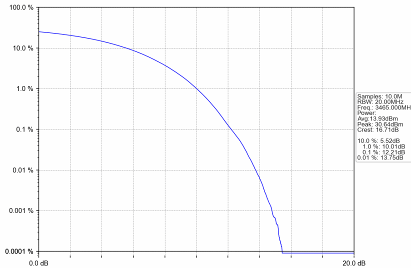
n77d_15kHz_SISO_NTNV_30MHz_CP-OFDM 256 QAM_3465MHz_Outer_Full
