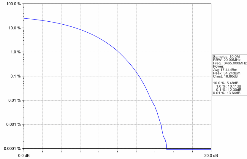
n77d_15kHz_SISO_NTNV_30MHz_CP-OFDM 16 QAM_3465MHz_Outer_Full
