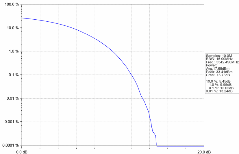
n77d_15kHz_SISO_NTNV_15MHz_CP-OFDM 64 QAM_3542.49MHz_Outer_Full
