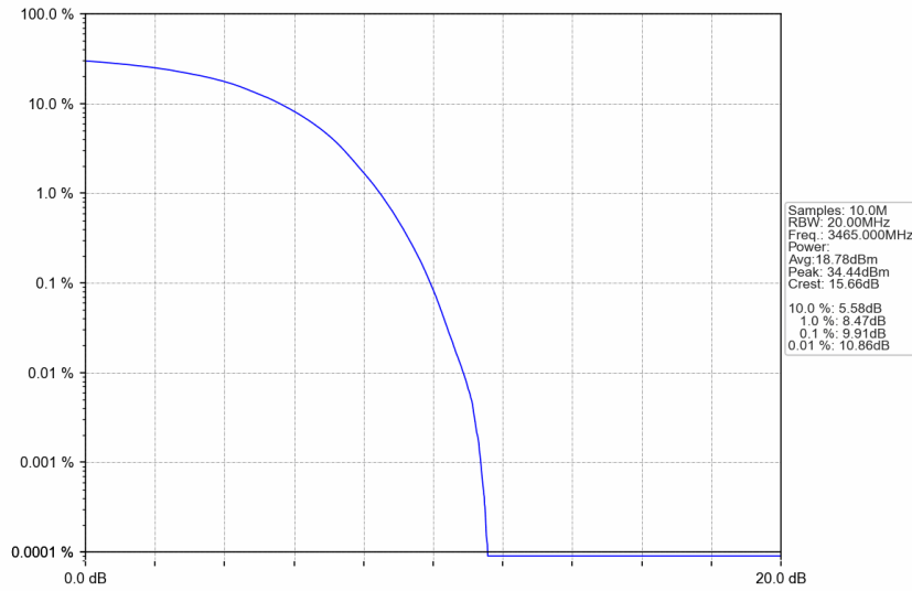
n77d_15kHz_SISO_NTNV_30MHz_DFT-s-OFDM_16_QAM_3465MHz_Outer_Full
