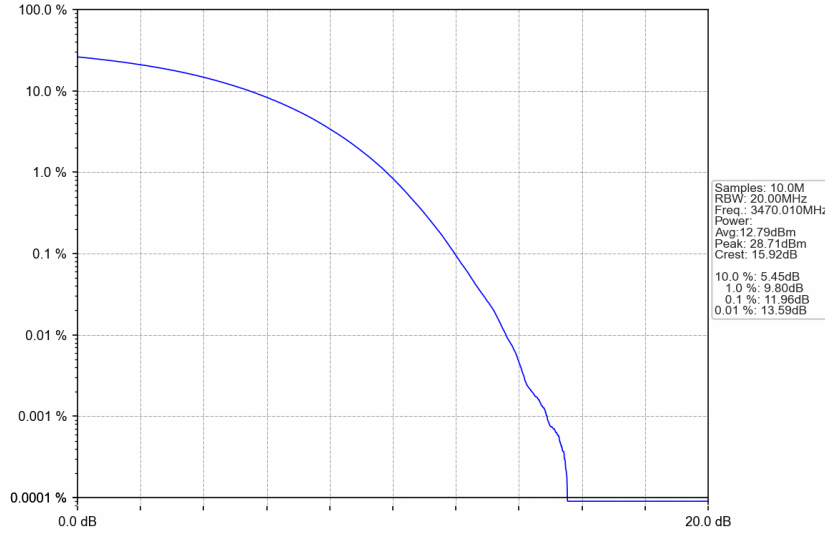
n77d_15kHz_SISO_NTNV_40MHz_CP-OFDM 256 QAM_3470.01MHz_Outer_Full
