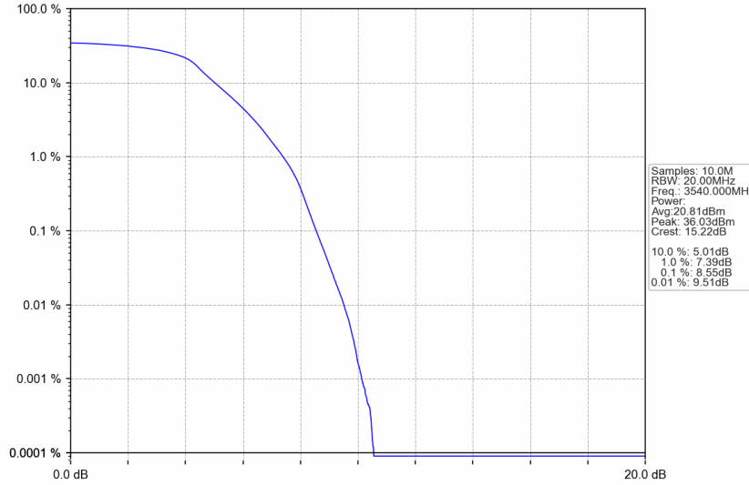
n77d_15kHz_SISO_NTNV_20MHz_DFT-s-OFDM PI/2 BPSK_3540MHz_Outer_Full
