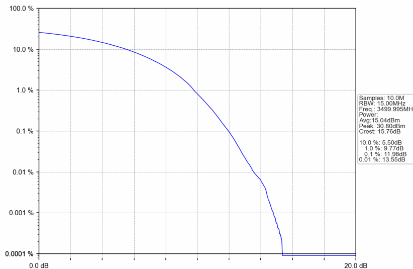
n77d_15kHz_SISO_NTNV_15MHz_CP-OFDM 256 QAM_3499.995MHz_Outer_Full
