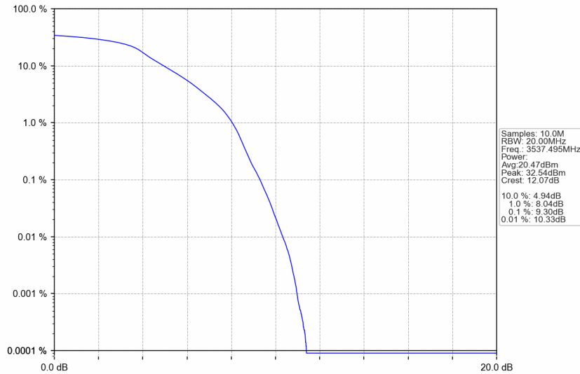
n77d_15kHz_SISO_NTNV_25MHz_DFT-s-OFDM QPSK_3537.495MHz_Outer_Full
