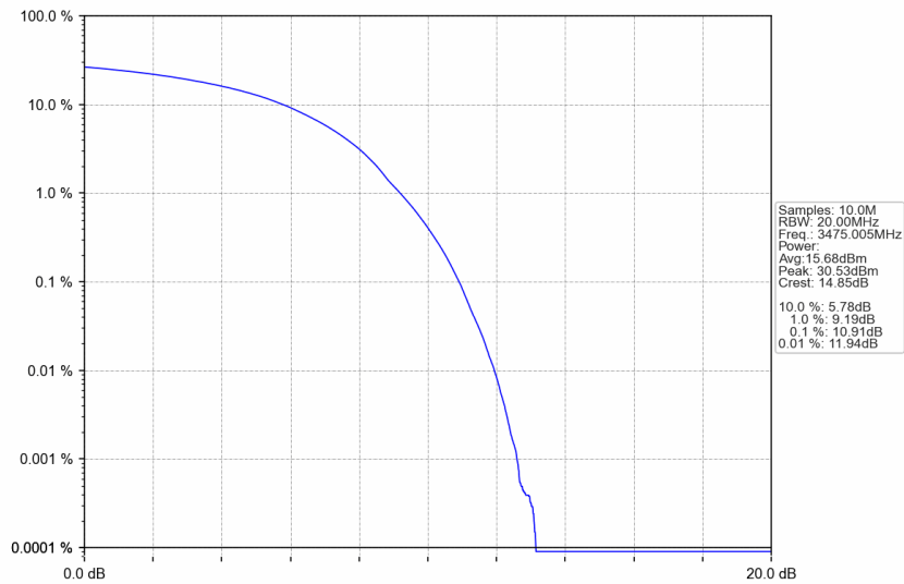
n77d_15kHz_SISO_NTNV_50MHz_DFT-s-OFDM 64 QAM_3475.005MHz_Outer_Full
