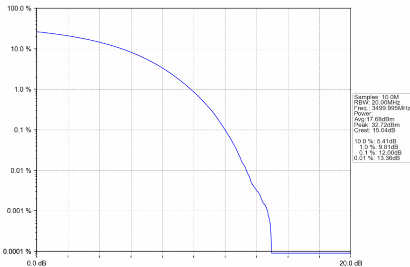
n77d_15kHz_SISO_NTNV_30MHz_CP-OFDM QPSK_3499.995MHz_Outer_Full
