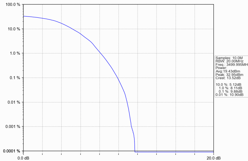
n77d_15kHz_SISO_NTNV_20MHz_DFT-s-OFDM 64 QAM_3499.995MHz_Outer_Full
