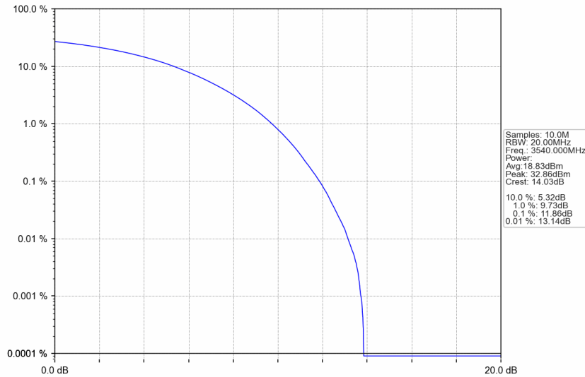
n77d_15kHz_SISO_NTNV_20MHz_CP-OFDM 16 QAM_3540MHz_Outer_Full
