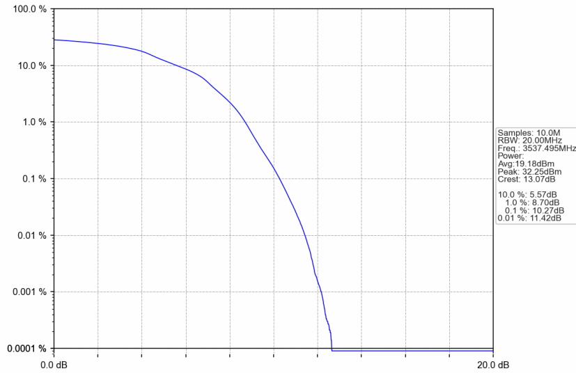
n77d_15kHz_SISO_NTNV_25MHz_DFT-s-OFDM 16 QAM_3537.495MHz_Outer_Full
