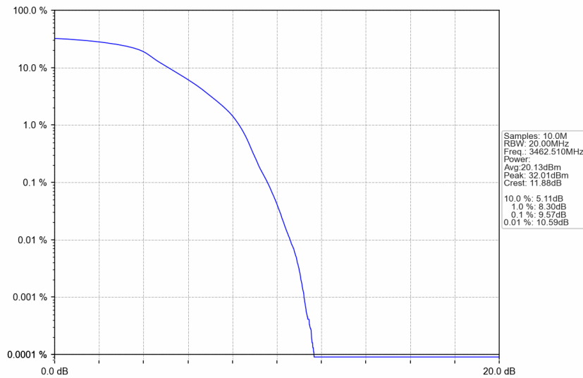
n77d_15kHz_SISO_NTNV_25MHz_DFT-s-OFDM QPSK_3462.51MHz_Outer_Full
