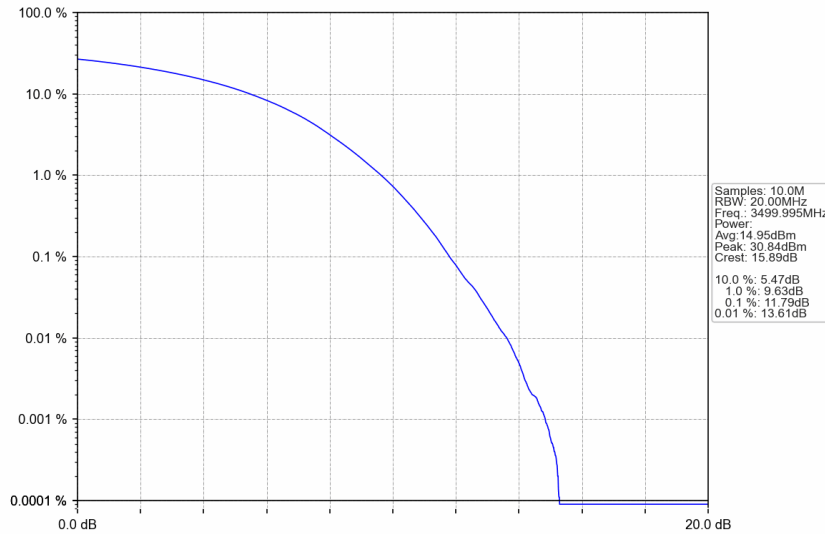
n77d_15kHz_SISO_NTNV_25MHz_CP-OFDM 256 QAM_3499.995MHz_Outer_Full
