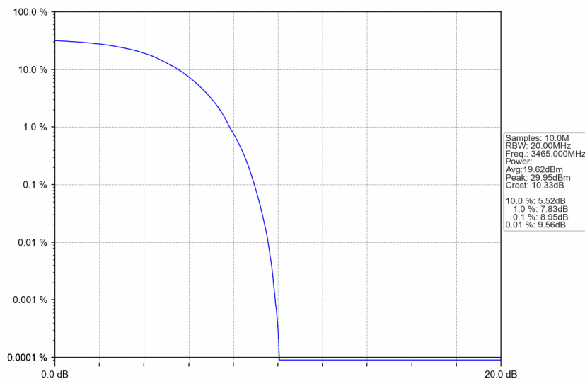
n77d_15kHz_SISO_NTNV_30MHz_DFT-s-OFDM QPSK_3465MHz_Outer_Full
