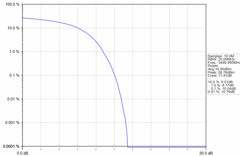
n77d_15kHz_SISO_NTNV_50MHz_DFT-s-OFDM QPSK_3499.995MHz_Outer_Full
