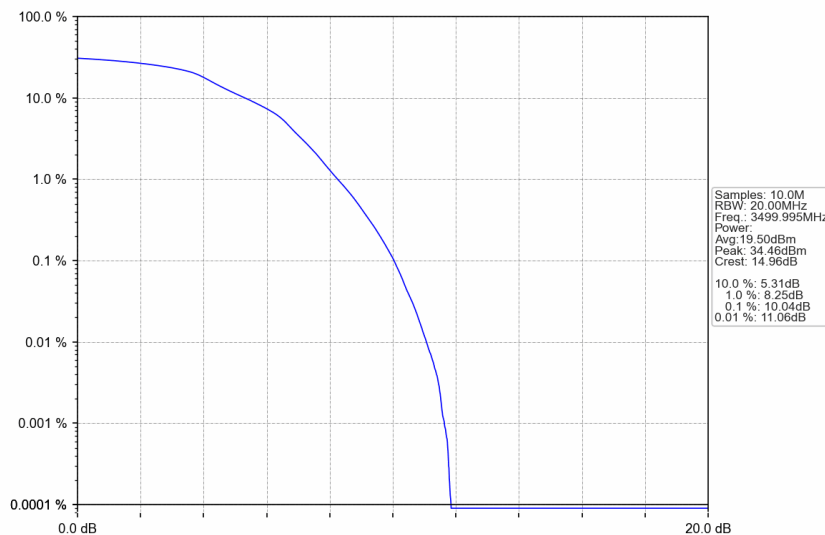
n77d_15kHz_SISO_NTNV_20MHz_DFT-s-OFDM 16 QAM_3499.995MHz_Outer_Full
