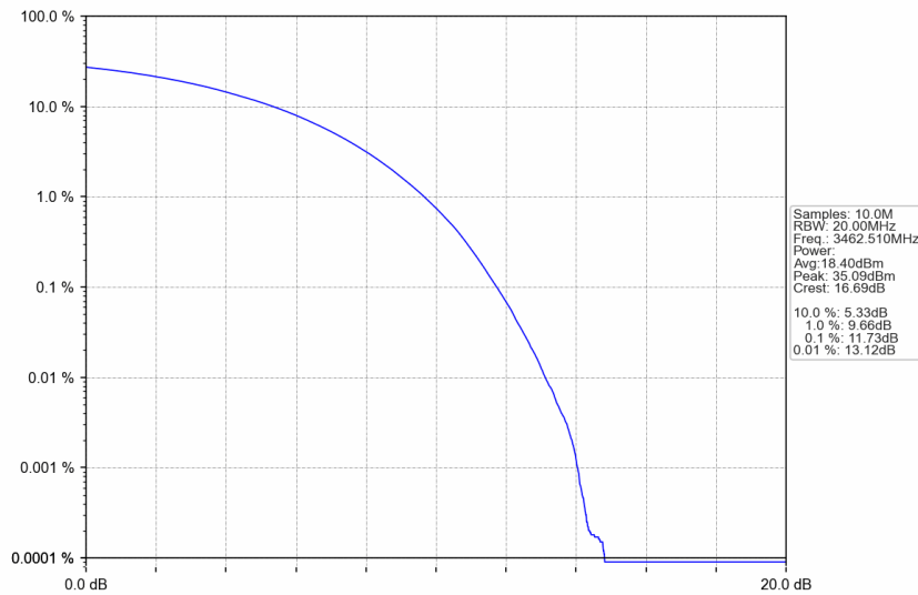
n77d_15kHz_SISO_NTNV_25MHz_CP-OFDM QPSK_3462.51MHz_Outer_Full
