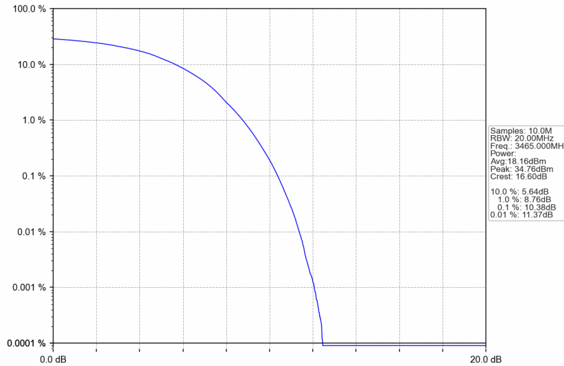
n77d_15kHz_SISO_NTNV_30MHz_DFT-s-OFDM 64 QAM_3465MHz_Outer_Full
