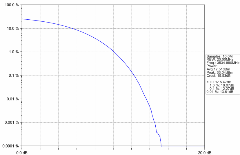
n77d_15kHz_SISO_NTNV_30MHz_CP-OFDM 16 QAM_3534.99MHz_Outer_Full
