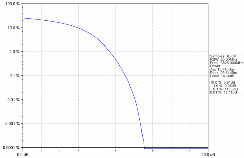
n77d_15kHz_SISO_NTNV_50MHz_DFT-s-OFDM 16 QAM_3525MHz_Outer_Full
