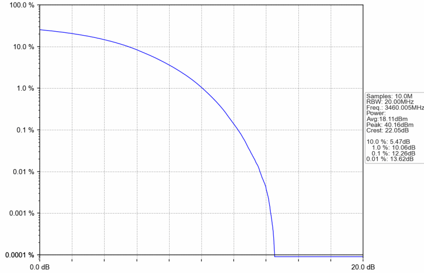
n77d_15kHz_SISO_NTNV_20MHz_CP-OFDM 16 QAM_3460.005MHz_Outer_Full
