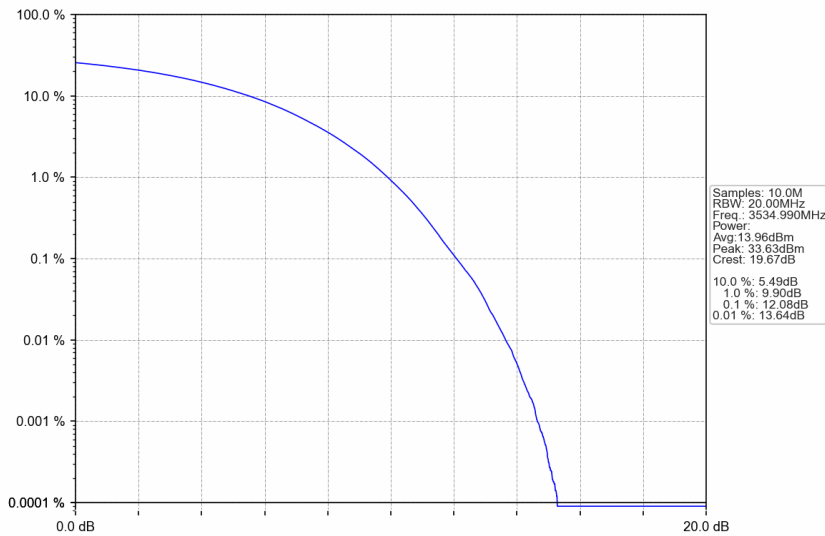
n77d_15kHz_SISO_NTNV_30MHz_CP-OFDM 256 QAM_3534.99MHz_Outer_Full
