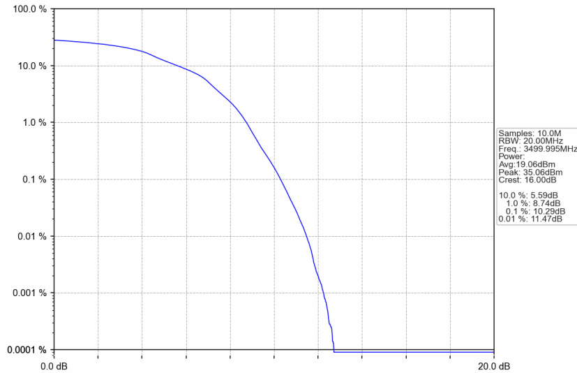
n77d_15kHz_SISO_NTNV_25MHz_DFT-s-OFDM 16 QAM_3499.995MHz_Outer_Full
