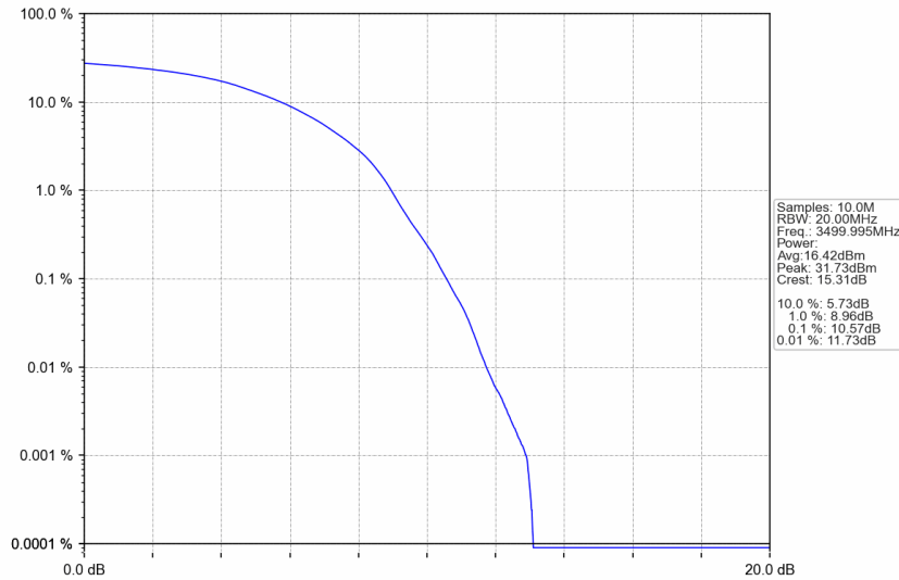
n77d_15kHz_SISO_NTNV_25MHz_DFT-s-OFDM 256 QAM_3499.995MHz_Outer_Full
