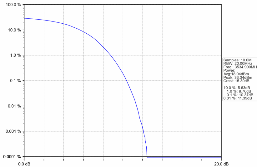
n77d_15kHz_SISO_NTNV_30MHz_DFT-s-OFDM 64 QAM_3534.99MHz_Outer_Full
