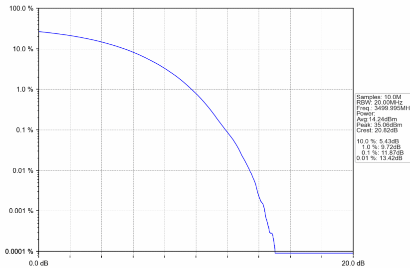
n77d_15kHz_SISO_NTNV_30MHz_CP-OFDM 256 QAM_3499.995MHz_Outer_Full
