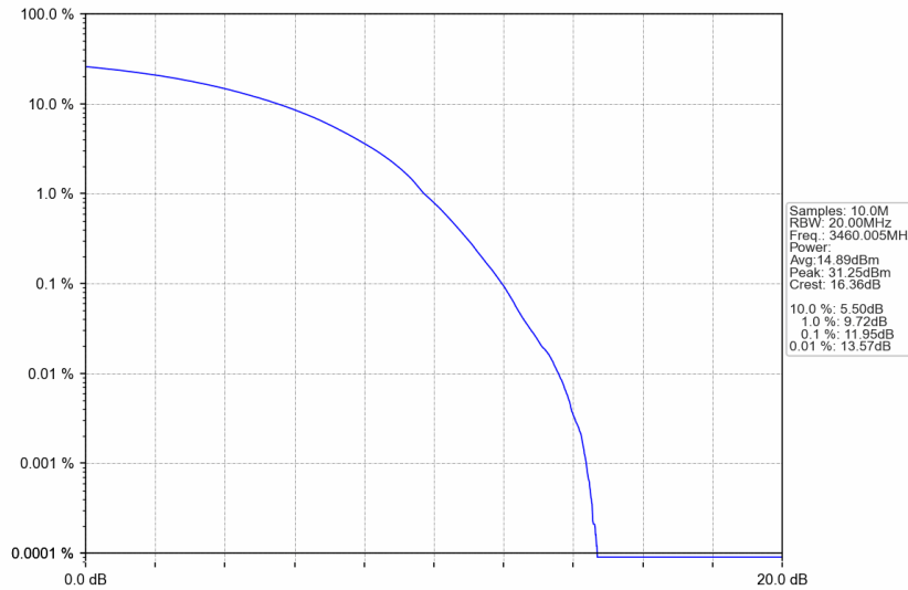
n77d_15kHz_SISO_NTNV_20MHz_CP-OFDM 256 QAM_3460.005MHz_Outer_Full
