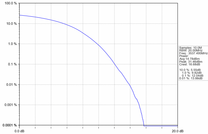
n77d_15kHz_SISO_NTNV_25MHz_CP-OFDM 256 QAM_3537.495MHz_Outer_Full
