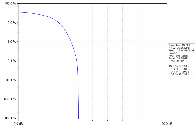
n77d_15kHz_SISO_NTNV_30MHz_DFT-s-OFDM PI/2 BPSK_3534.99MHz_Outer_Full
