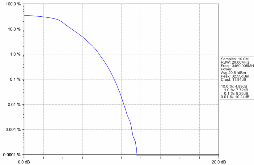
n77d_15kHz_SISO_NTNV_20MHz_DFT-s-OFDM QPSK_3460.005MHz_Outer_Full
