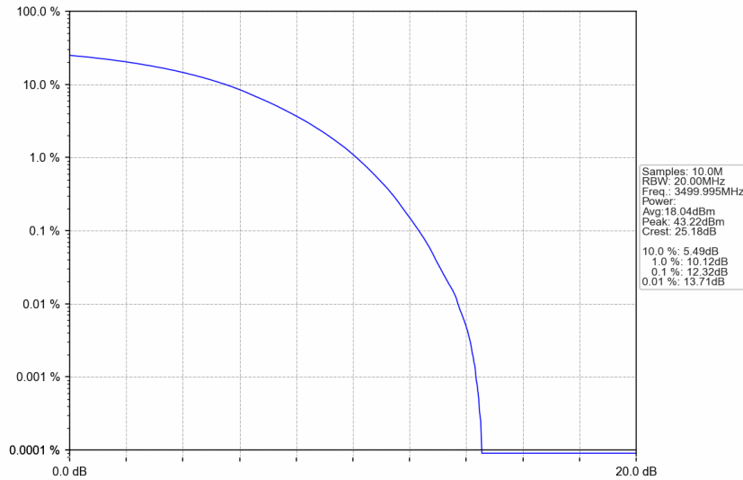
n77d_15kHz_SISO_NTNV_20MHz_CP-OFDM 16 QAM_3499.995MHz_Outer_Full
