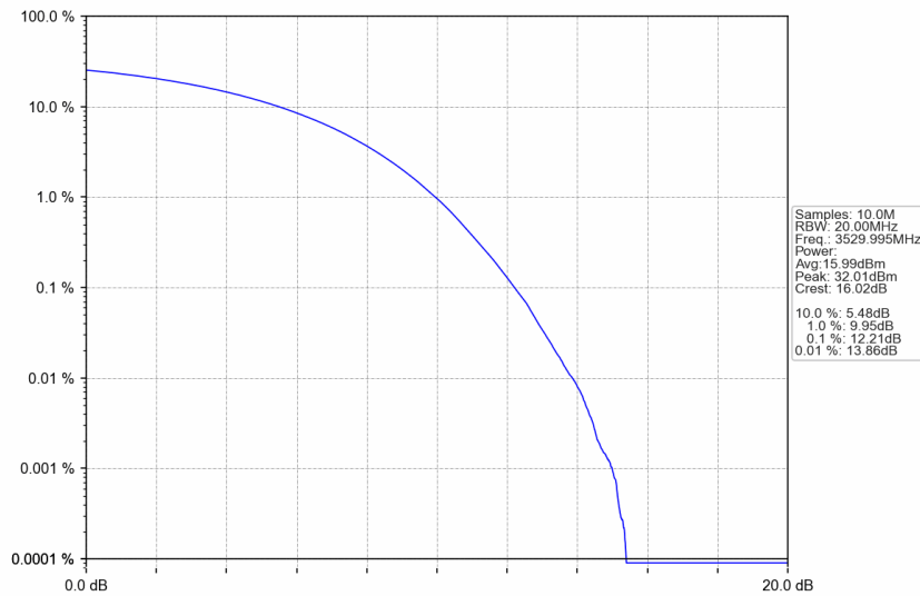
n77d_15kHz_SISO_NTNV_40MHz_CP-OFDM QPSK_3529.995MHz_Outer_Full
