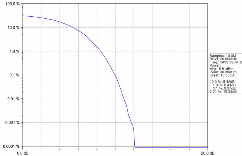
n77d_15kHz_SISO_NTNV_30MHz_DFT-s-OFDM 256 QAM_3499.995MHz_Outer_Full
