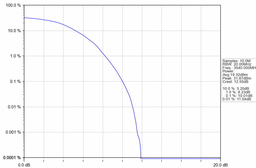
n77d_15kHz_SISO_NTNV_20MHz_DFT-s-OFDM 64 QAM_3540MHz_Outer_Full
