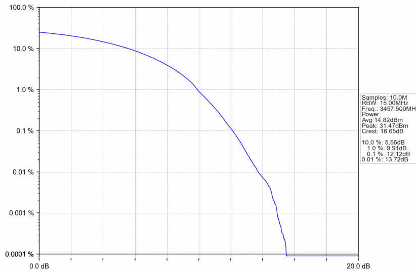
n77d_15kHz_SISO_NTNV_15MHz_CP-OFDM 256 QAM_3457.5MHz_Outer_Full
