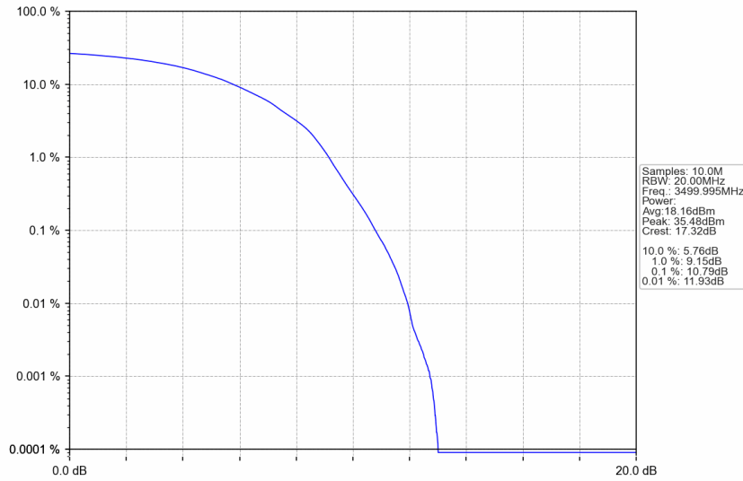
n77d_15kHz_SISO_NTNV_25MHz_DFT-s-OFDM 64 QAM_3499.995MHz_Outer_Full
