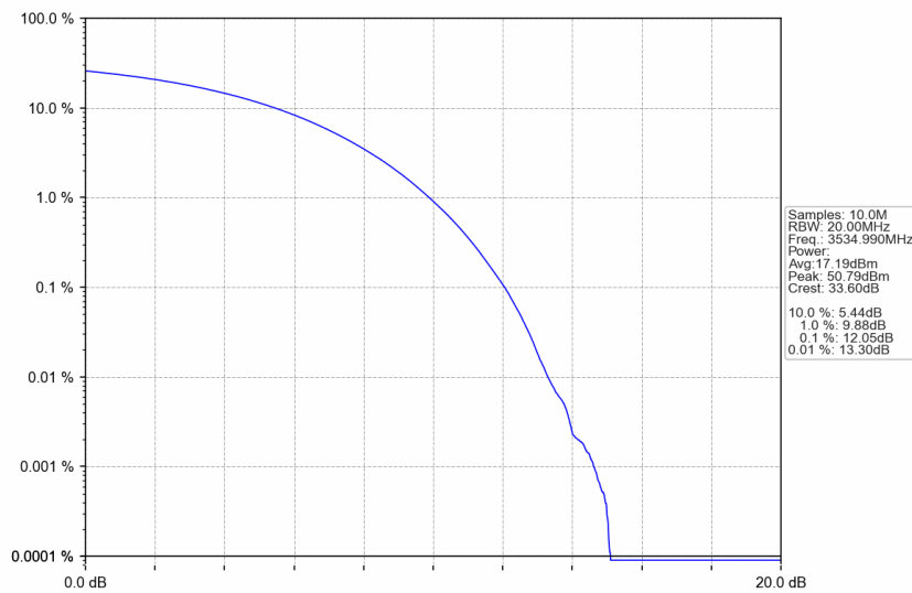
n77d_15kHz_SISO_NTNV_30MHz_CP-OFDM 64 QAM_3534.99MHz_Outer_Full
