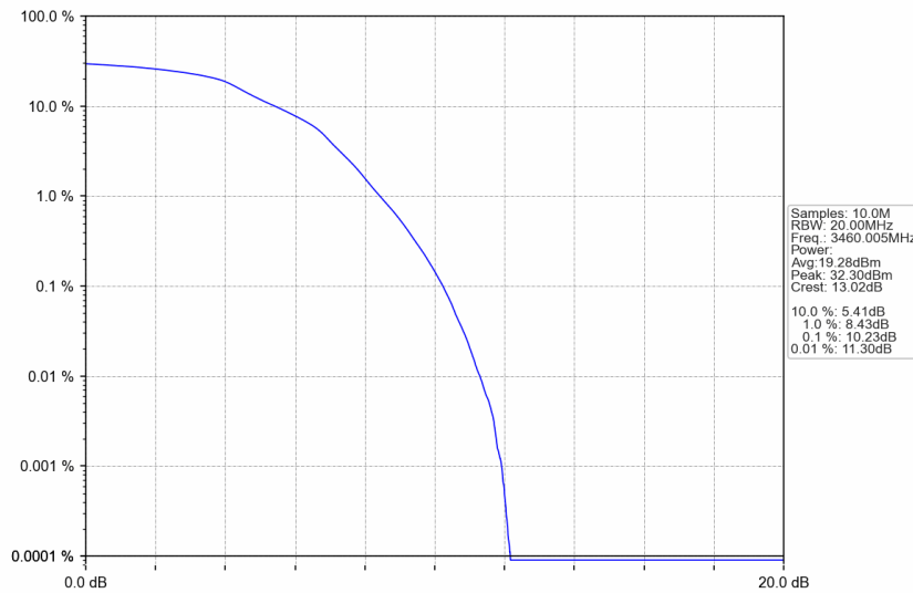
n77d_15kHz_SISO_NTNV_20MHz_DFT-s-OFDM 16 QAM_3460.005MHz_Outer_Full
