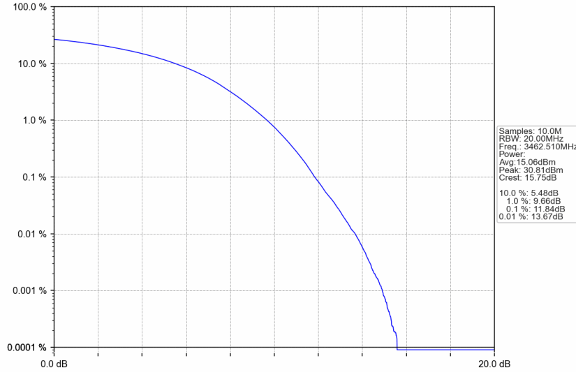
n77d_15kHz_SISO_NTNV_25MHz_CP-OFDM 256 QAM_3462.51MHz_Outer_Full
