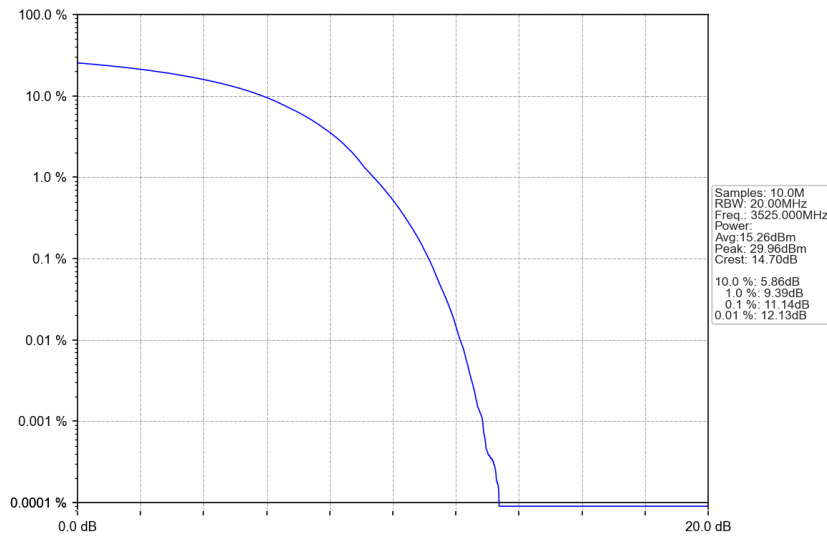
n77d_15kHz_SISO_NTNV_50MHz_DFT-s-OFDM 64 QAM_3525MHz_Outer_Full
