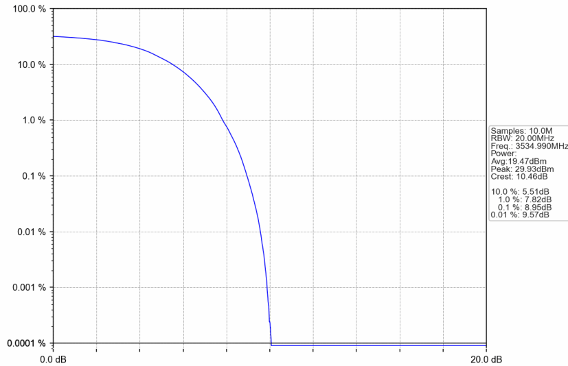
n77d_15kHz_SISO_NTNV_30MHz_DFT-s-OFDM QPSK_3534.99MHz_Outer_Full
