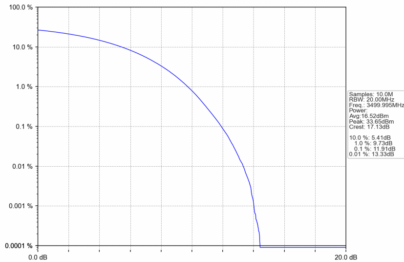
n77d_15kHz_SISO_NTNV_40MHz_CP-OFDM 16 QAM_3499.995MHz_Outer_Full
