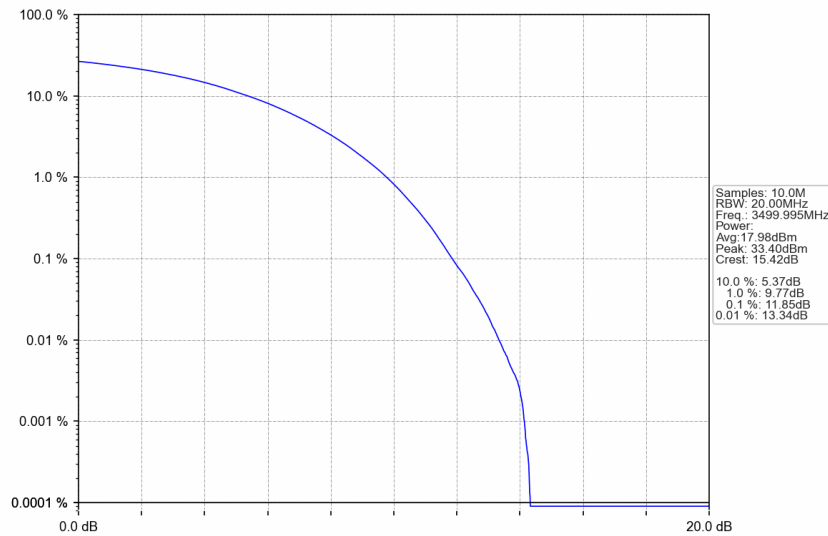
n77d_15kHz_SISO_NTNV_25MHz_CP-OFDM 64 QAM_3499.995MHz_Outer_Full
