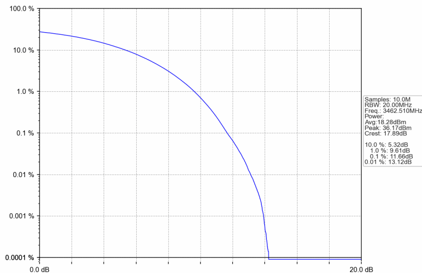
n77d_15kHz_SISO_NTNV_25MHz_CP-OFDM 64 QAM_3462.51MHz_Outer_Full
