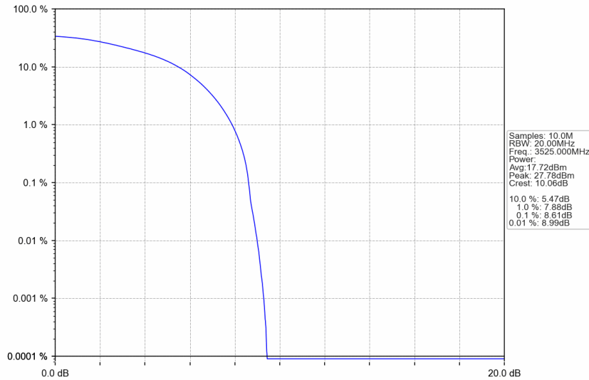
n77d_15kHz_SISO_NTNV_50MHz_DFT-s-OFDM PI/2 BPSK_3525MHz_Outer_Full
