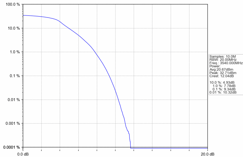
n77d_15kHz_SISO_NTNV_20MHz_DFT-s-OFDM QPSK_3540MHz_Outer_Full
