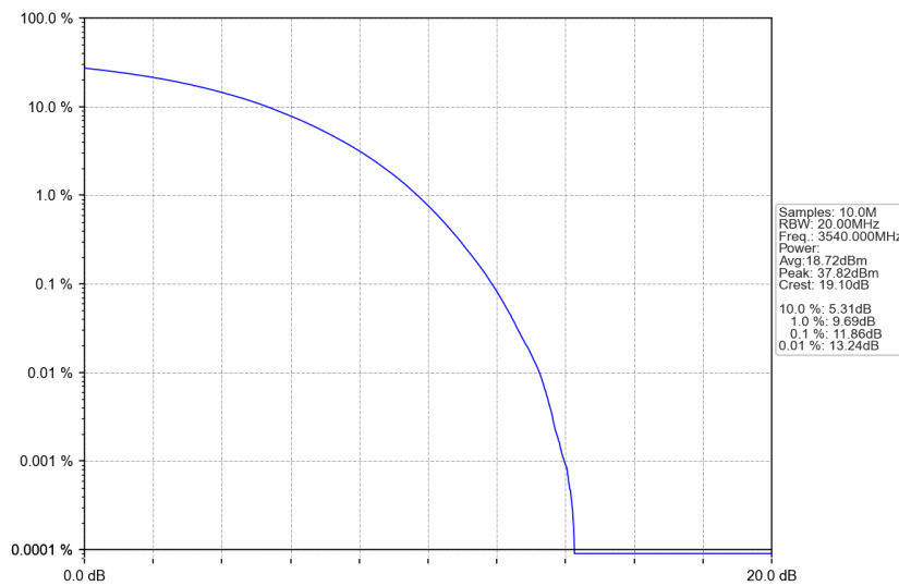
n77d_15kHz_SISO_NTNV_20MHz_CP-OFDM QPSK_3540MHz_Outer_Full
