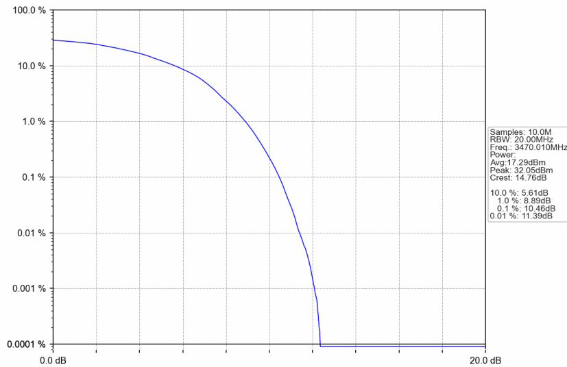
n77d_15kHz_SISO_NTNV_40MHz_DFT-s-OFDM 16 QAM_3470.01MHz_Outer_Full
