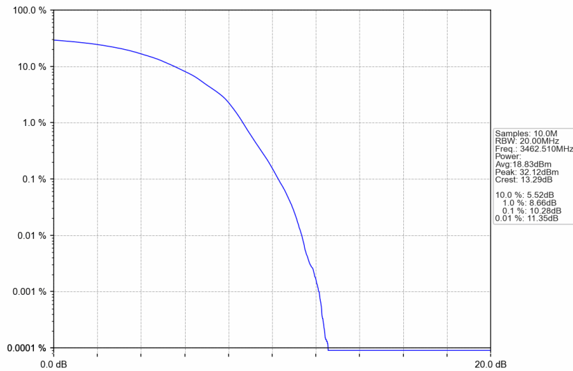
n77d_15kHz_SISO_NTNV_25MHz_DFT-s-OFDM 64 QAM_3462.51MHz_Outer_Full
