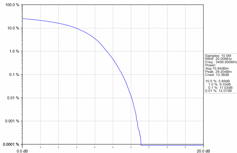
n77d_15kHz_SISO_NTNV_50MHz_DFT-s-OFDM 16 QAM_3499.995MHz_Outer_Full
