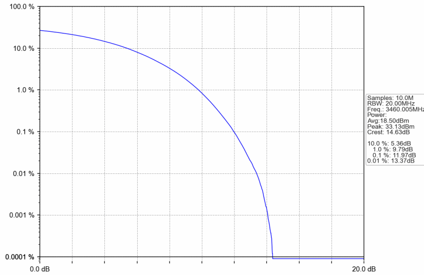
n77d_15kHz_SISO_NTNV_20MHz_CP-OFDM QPSK_3460.005MHz_Outer_Full
