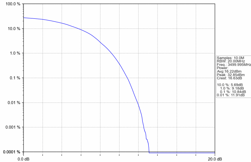
n77d_15kHz_SISO_NTNV_40MHz_DFT-s-OFDM 64 QAM_3499.995MHz_Outer_Full
