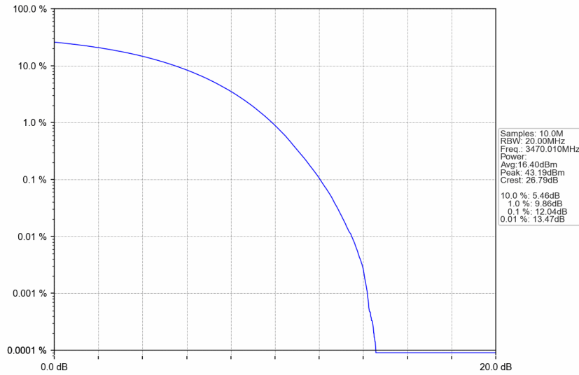
n77d_15kHz_SISO_NTNV_40MHz_CP-OFDM 16 QAM_3470.01MHz_Outer_Full
