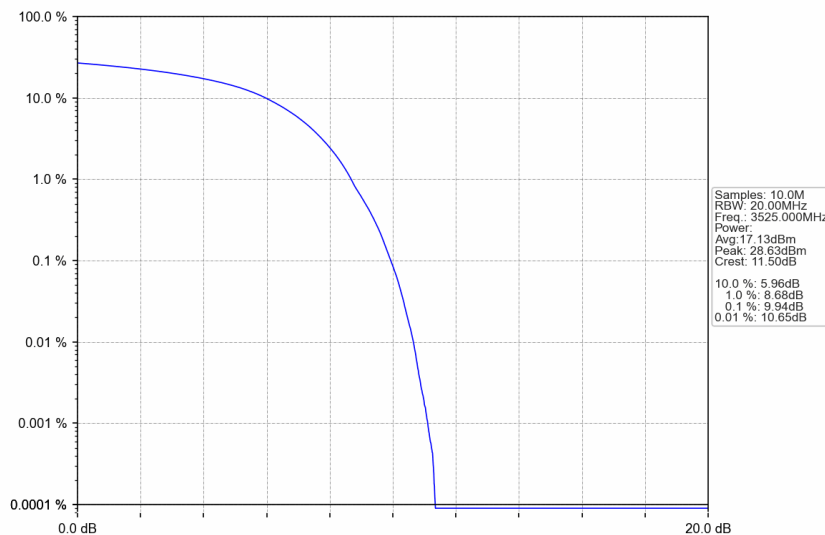
n77d_15kHz_SISO_NTNV_50MHz_DFT-s-OFDM QPSK_3525MHz_Outer_Full
