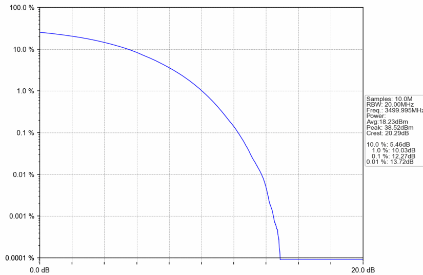
n77d_15kHz_SISO_NTNV_20MHz_CP-OFDM QPSK_3499.995MHz_Outer_Full
