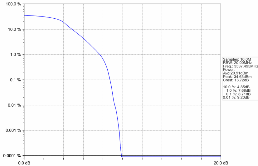
n77d_15kHz_SISO_NTNV_25MHz_DFT-s-OFDM PI/2 BPSK_3537.495MHz_Outer_Full
