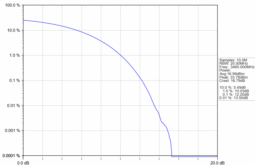
n77d_15kHz_SISO_NTNV_30MHz_CP-OFDM 64 QAM_3465MHz_Outer_Full
