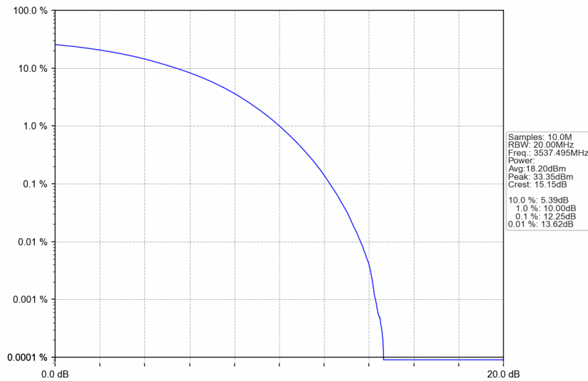
n77d_15kHz_SISO_NTNV_25MHz_CP-OFDM 16 QAM_3537.495MHz_Outer_Full
