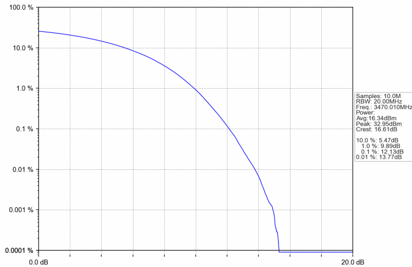
n77d_15kHz_SISO_NTNV_40MHz_CP-OFDM QPSK_3470.01MHz_Outer_Full
