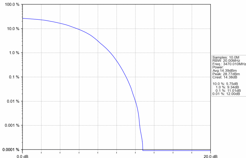
n77d_15kHz_SISO_NTNV_40MHz_DFT-s-OFDM 256 QAM_3470.01MHz_Outer_Full
