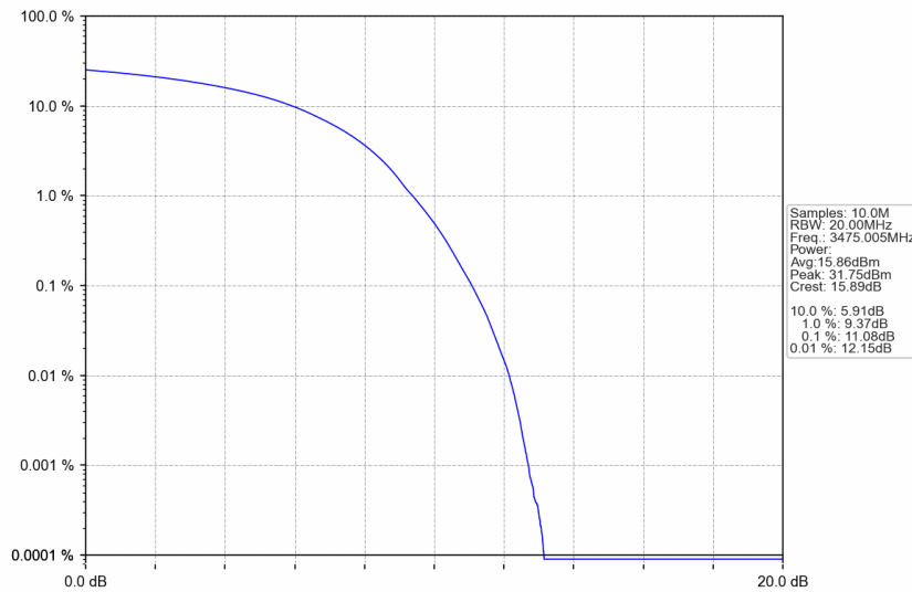
n77d_15kHz_SISO_NTNV_50MHz_DFT-s-OFDM 16 QAM_3475.005MHz_Outer_Full
