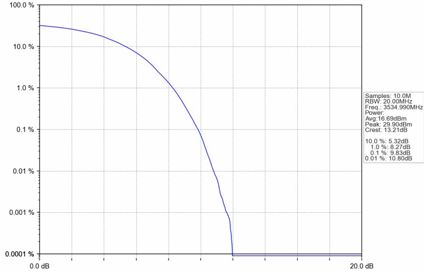
n77d_15kHz_SISO_NTNV_30MHz_DFT-s-OFDM 256 QAM_3534.99MHz_Outer_Full
