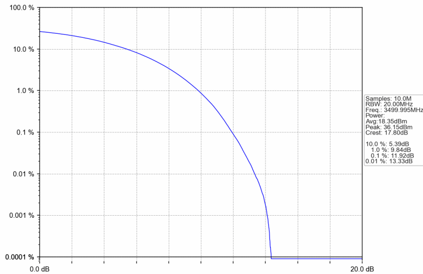
n77d_15kHz_SISO_NTNV_25MHz_CP-OFDM QPSK_3499.995MHz_Outer_Full
