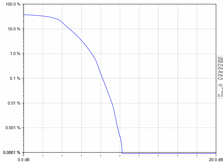
n77d_15kHz_SISO_NTNV_20MHz_DFT-s-OFDM PI/2 BPSK_3499.995MHz_Outer_Full
