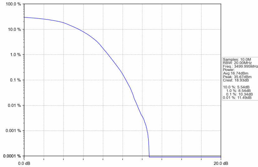
n77d_15kHz_SISO_NTNV_20MHz_DFT-s-OFDM 256 QAM_3499.995MHz_Outer_Full
