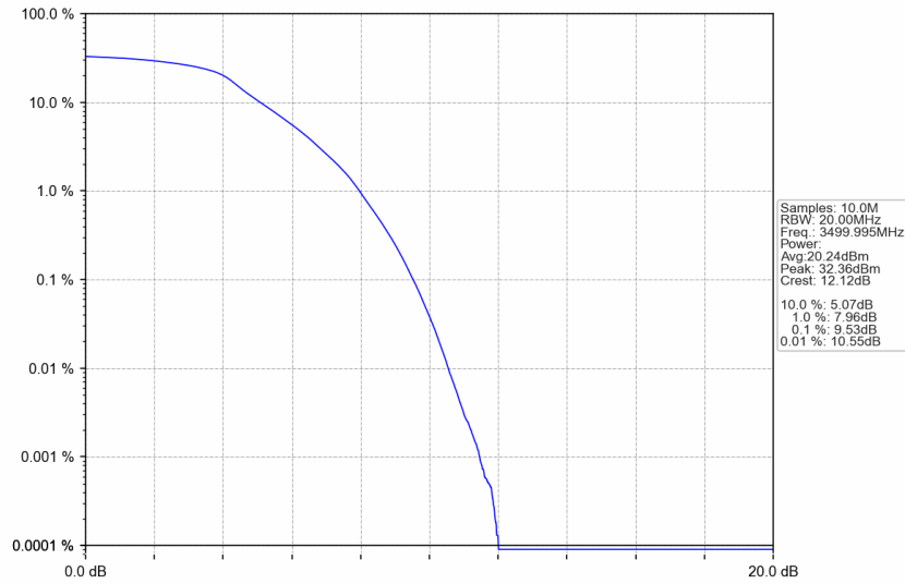
n77d_15kHz_SISO_NTNV_20MHz_DFT-s-OFDM QPSK_3499.995MHz_Outer_Full
