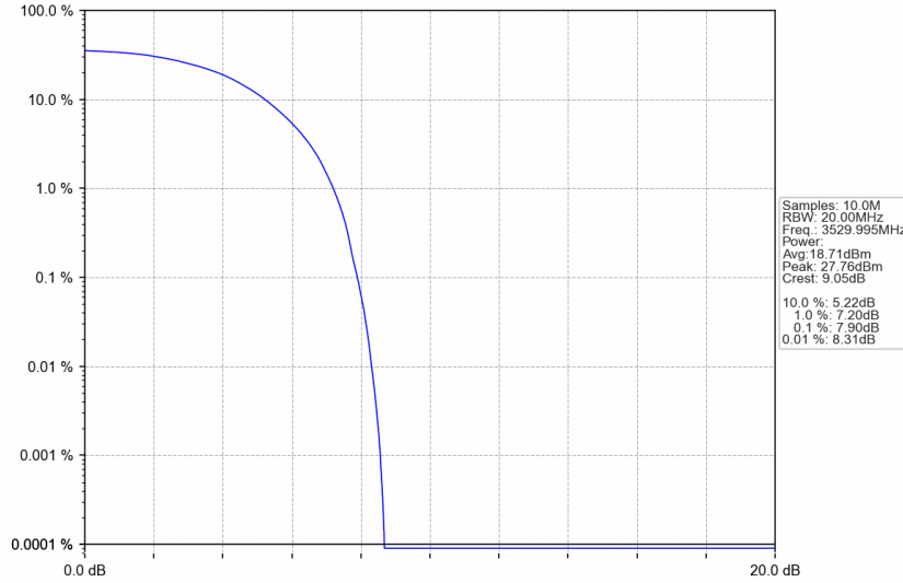
n77d_15kHz_SISO_NTNV_40MHz_DFT-s-OFDM PI/2 BPSK_3529.995MHz_Outer_Full
