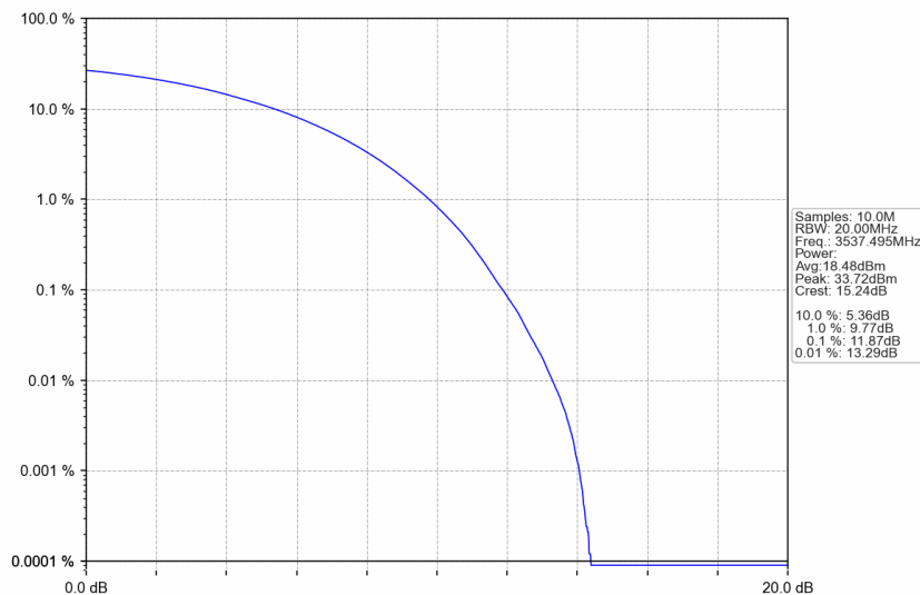
n77d_15kHz_SISO_NTNV_25MHz_CP-OFDM QPSK_3537.495MHz_Outer_Full
