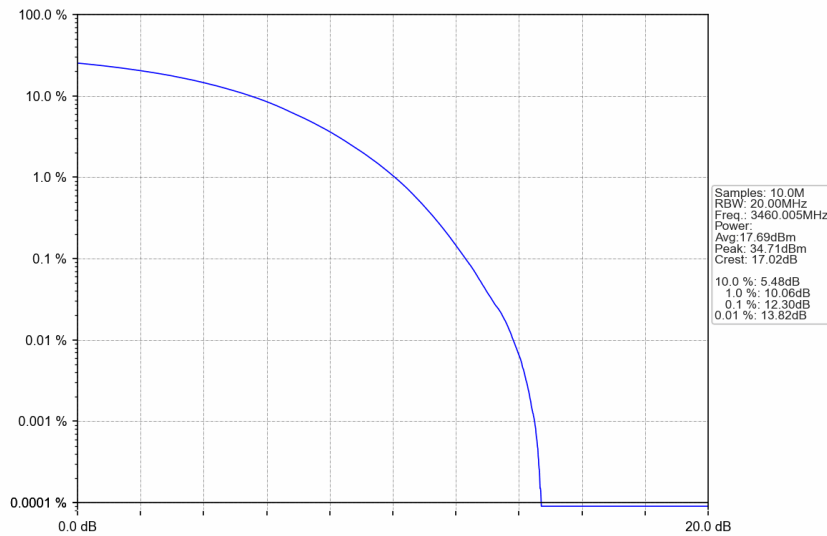
n77d_15kHz_SISO_NTNV_20MHz_CP-OFDM 64 QAM_3460.005MHz_Outer_Full
