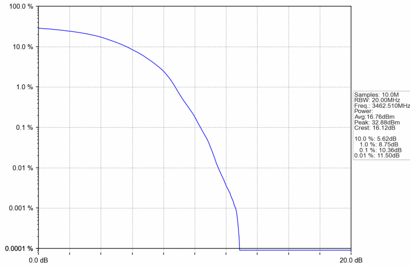
n77d_15kHz_SISO_NTNV_25MHz_DFT-s-OFDM 256 QAM_3462.51MHz_Outer_Full
