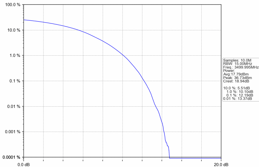
n77d_15kHz_SISO_NTNV_15MHz_CP-OFDM 64 QAM_3499.995MHz_Outer_Full
