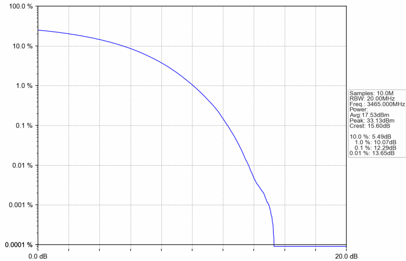
n77d_15kHz_SISO_NTNV_30MHz_CP-OFDM QPSK_3465MHz_Outer_Full
