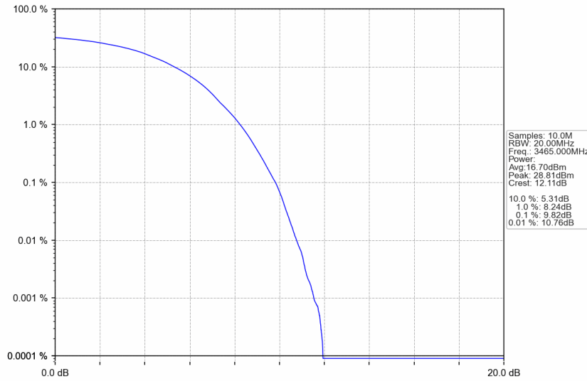
n77d_15kHz_SISO_NTNV_30MHz_DFT-s-OFDM 256 QAM_3465MHz_Outer_Full
