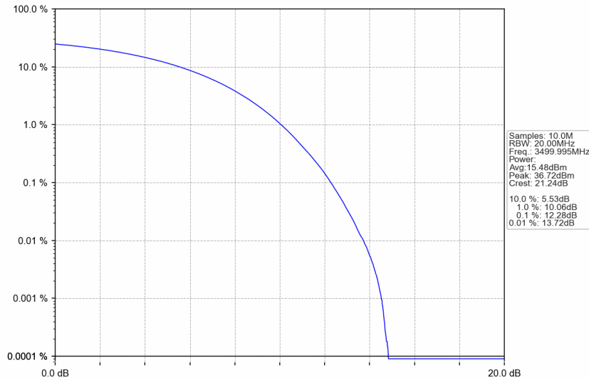
n77d_15kHz_SISO_NTNV_40MHz_CP-OFDM 64 QAM_3499.995MHz_Outer_Full
