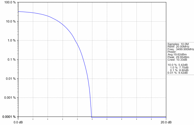
n77d_15kHz_SISO_NTNV_30MHz_DFT-s-OFDM QPSK_3499.995MHz_Outer_Full
