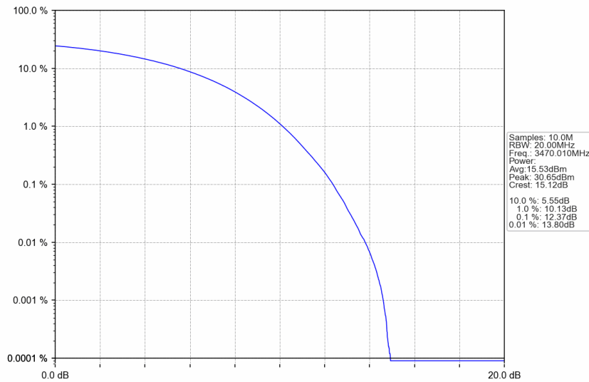
n77d_15kHz_SISO_NTNV_40MHz_CP-OFDM 64 QAM_3470.01MHz_Outer_Full
