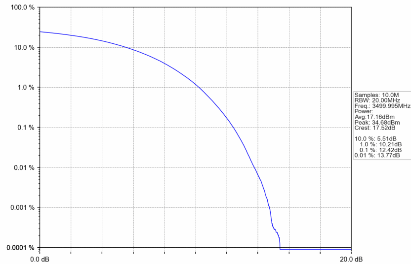
n77d_15kHz_SISO_NTNV_30MHz_CP-OFDM 16 QAM_3499.995MHz_Outer_Full
