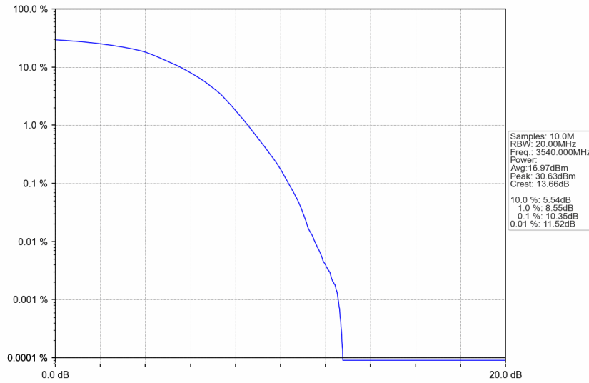
n77d_15kHz_SISO_NTNV_20MHz_DFT-s-OFDM 256 QAM_3540MHz_Outer_Full
