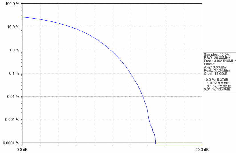
n77d_15kHz_SISO_NTNV_25MHz_CP-OFDM 16 QAM_3462.51MHz_Outer_Full
