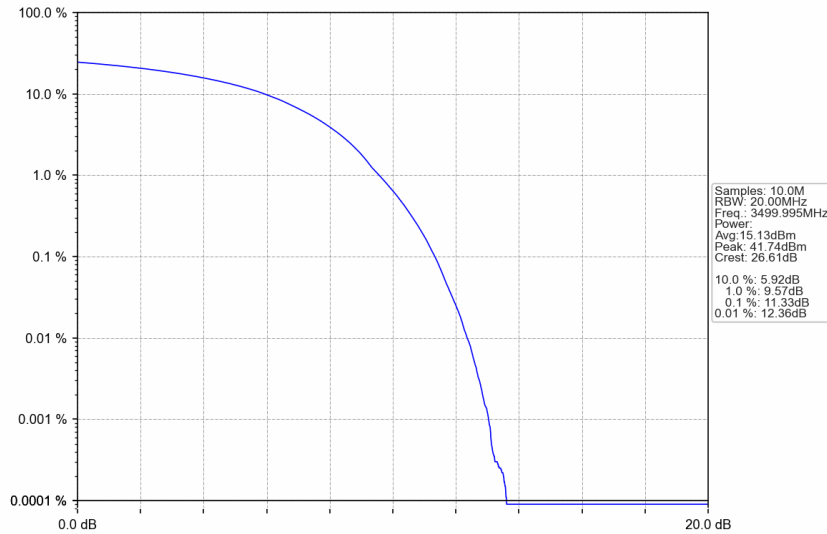
n77d_15kHz_SISO_NTNV_50MHz_DFT-s-OFDM 64 QAM_3499.995MHz_Outer_Full
