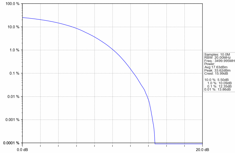
n77d_15kHz_SISO_NTNV_20MHz_CP-OFDM 64 QAM_3499.995MHz_Outer_Full
