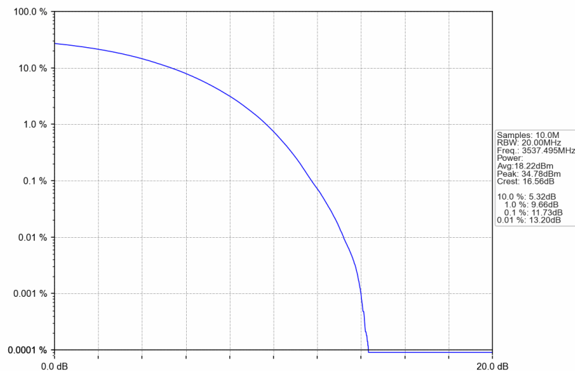
n77d_15kHz_SISO_NTNV_25MHz_CP-OFDM 64 QAM_3537.495MHz_Outer_Full
