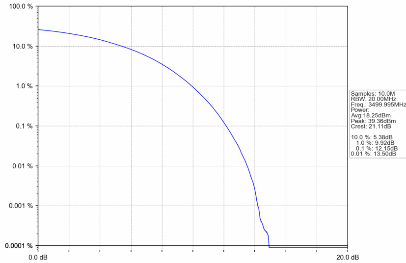
n77d_15kHz_SISO_NTNV_25MHz_CP-OFDM 16 QAM_3499.995MHz_Outer_Full
