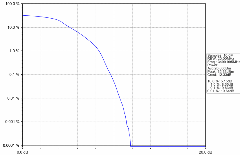
n77d_15kHz_SISO_NTNV_25MHz_DFT-s-OFDM QPSK_3499.995MHz_Outer_Full
