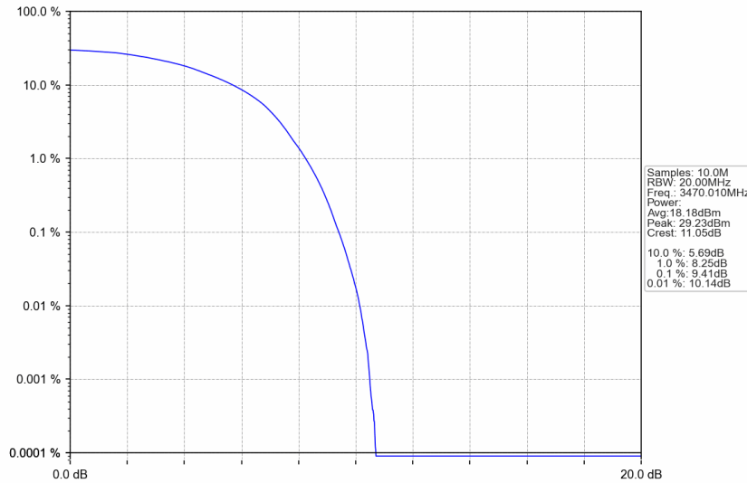
n77d_15kHz_SISO_NTNV_40MHz_DFT-s-OFDM QPSK_3470.01MHz_Outer_Full
