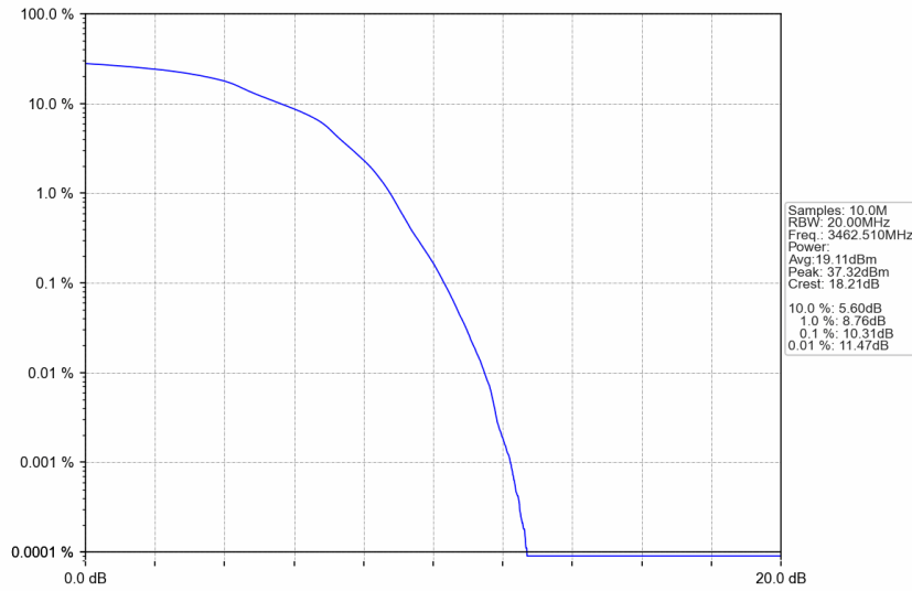
n77d_15kHz_SISO_NTNV_25MHz_DFT-s-OFDM 16 QAM_3462.51MHz_Outer_Full
