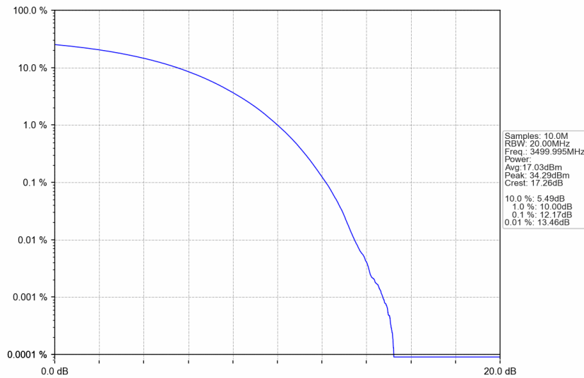
n77d_15kHz_SISO_NTNV_30MHz_CP-OFDM 64 QAM_3499.995MHz_Outer_Full
