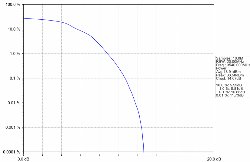
n77d_15kHz_SISO_NTNV_20MHz_DFT-s-OFDM 16 QAM_3540MHz_Outer_Full
