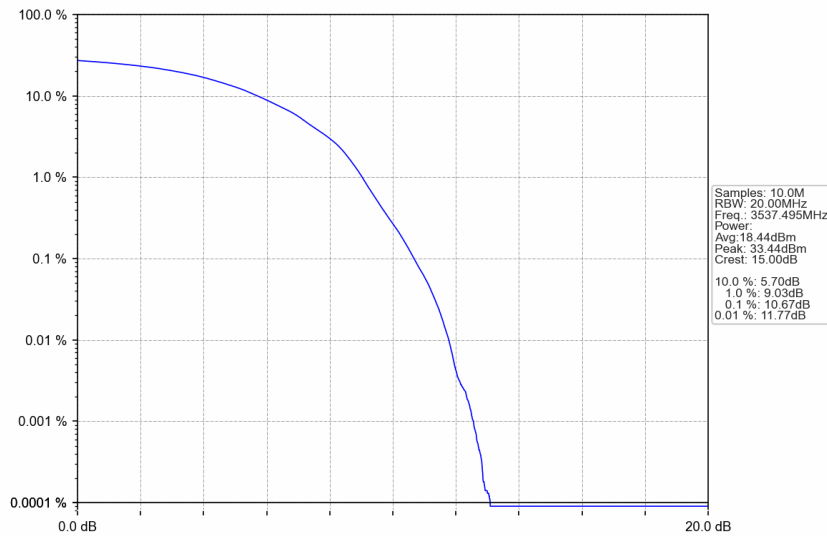
n77d_15kHz_SISO_NTNV_25MHz_DFT-s-OFDM 64 QAM_3537.495MHz_Outer_c_Full
