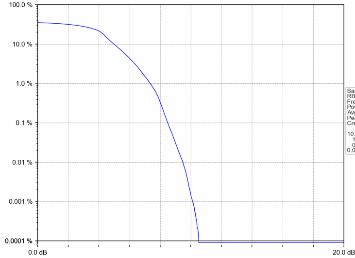
n77d_15kHz_SISO_NTNV_20MHz_DFT-s-OFDM PI/2 BPSK_3460.005MHz_Outer_Full
