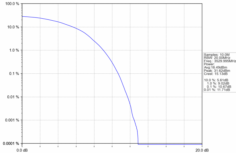
n77d_15kHz_SISO_NTNV_40MHz_DFT-s-OFDM 64 QAM_3529.995MHz_Outer_Full
