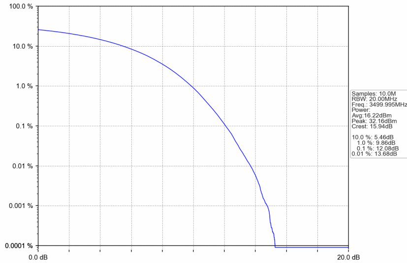
n77d_15kHz_SISO_NTNV_40MHz_CP-OFDM QPSK_3499.995MHz_Outer_Full
