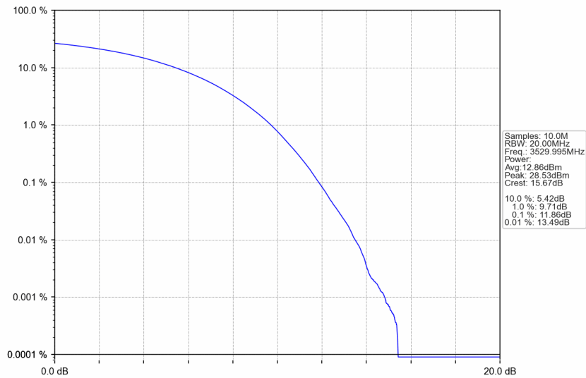
n77d_15kHz_SISO_NTNV_40MHz_CP-OFDM 256 QAM_3529.995MHz_Outer_Full
