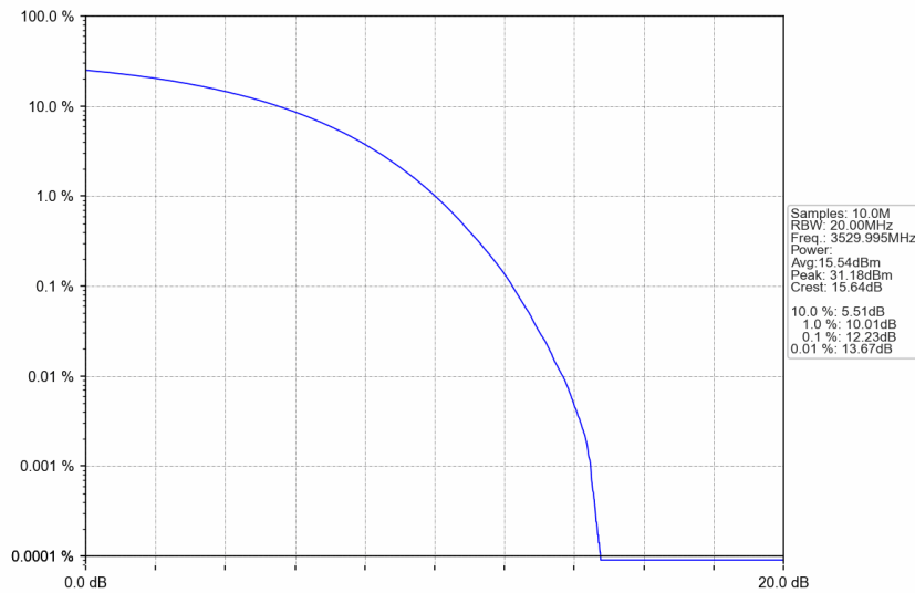
n77d_15kHz_SISO_NTNV_40MHz_CP-OFDM 64 QAM_3529.995MHz_Outer_Full
