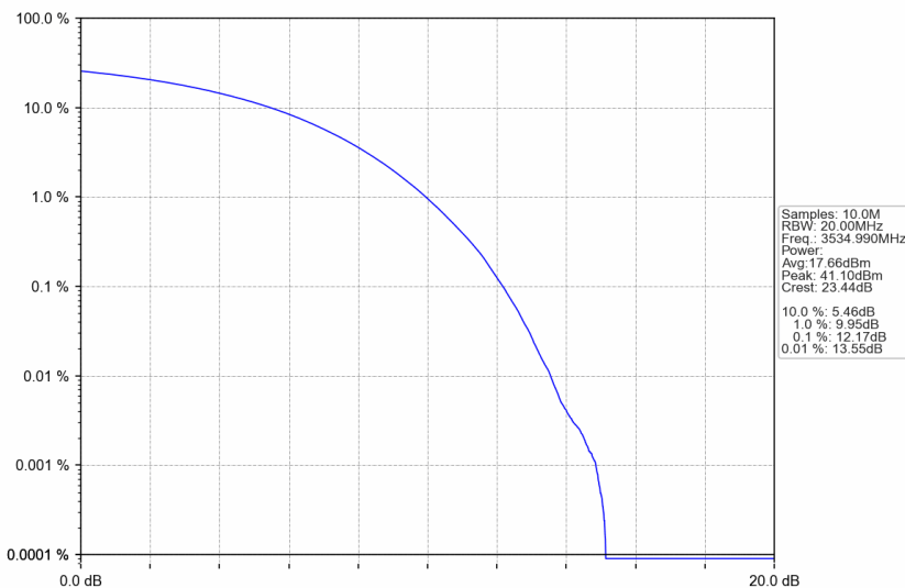
n77d_15kHz_SISO_NTNV_30MHz_CP-OFDM QPSK_3534.99MHz_Outer_Full
