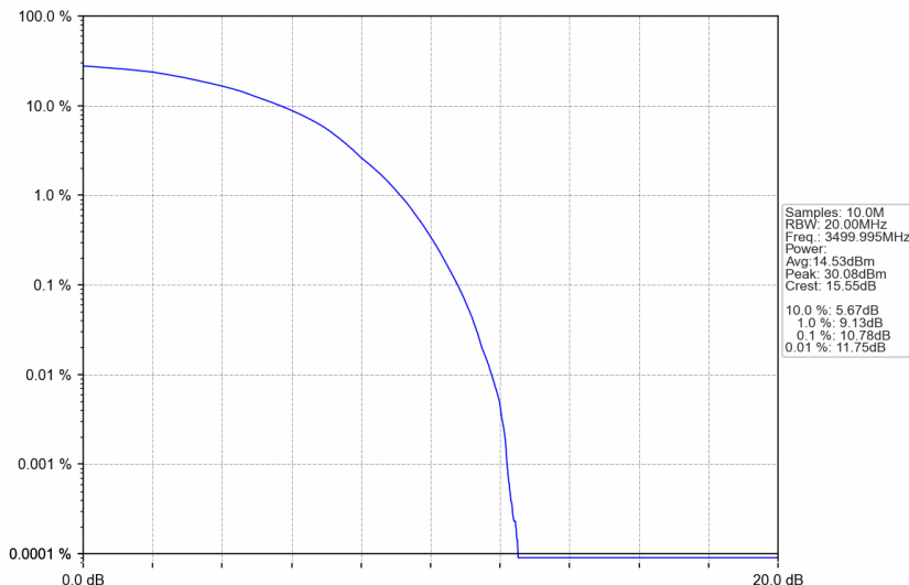
n77d_15kHz_SISO_NTNV_40MHz_DFT-s-OFDM 256 QAM_3499.995MHz_Outer_Full
