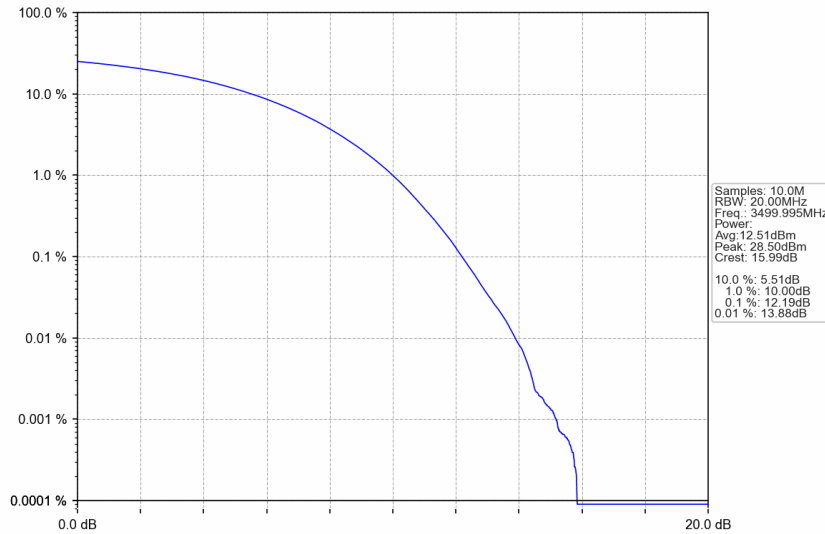
n77d_15kHz_SISO_NTNV_40MHz_CP-OFDM 256 QAM_3499.995MHz_Outer_Full
