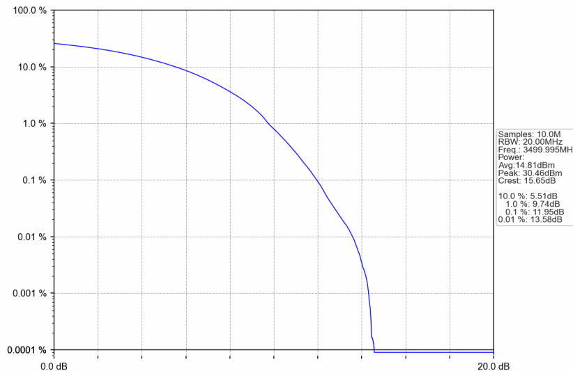
n77d_15kHz_SISO_NTNV_20MHz_CP-OFDM 256 QAM_3499.995MHz_Outer_Full
