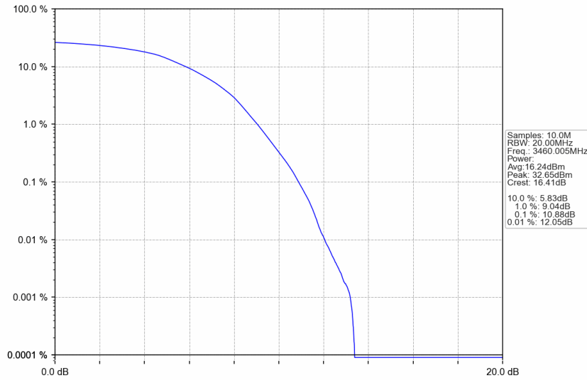
n77d_15kHz_SISO_NTNV_20MHz_DFT-s-OFDM 256 QAM_3460.005MHz_Outer_Full
