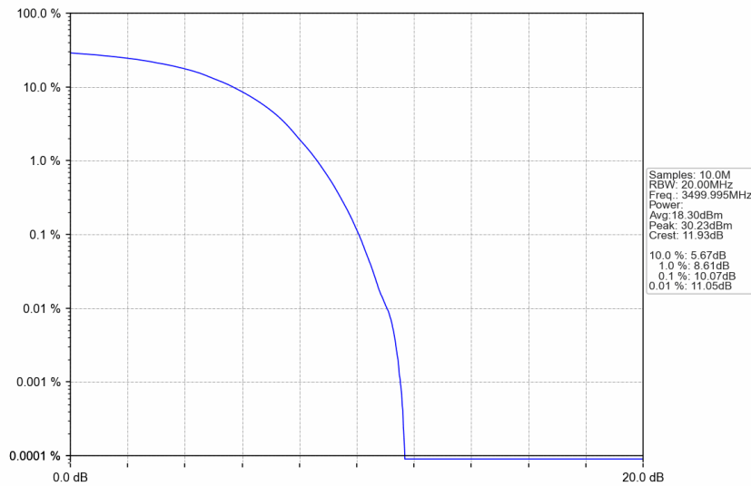
n77d_15kHz_SISO_NTNV_30MHz_DFT-s-OFDM_16_QAM_3499.995MHz_Outer_Full
