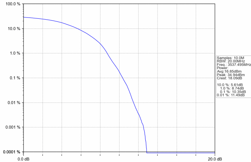
n77d_15kHz_SISO_NTNV_25MHz_DFT-s-OFDM 256 QAM_3537.495MHz_Outer_Full
