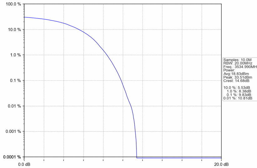
n77d_15kHz_SISO_NTNV_30MHz_DFT-s-OFDM 16 QAM_3534.99MHz_Outer_Full
