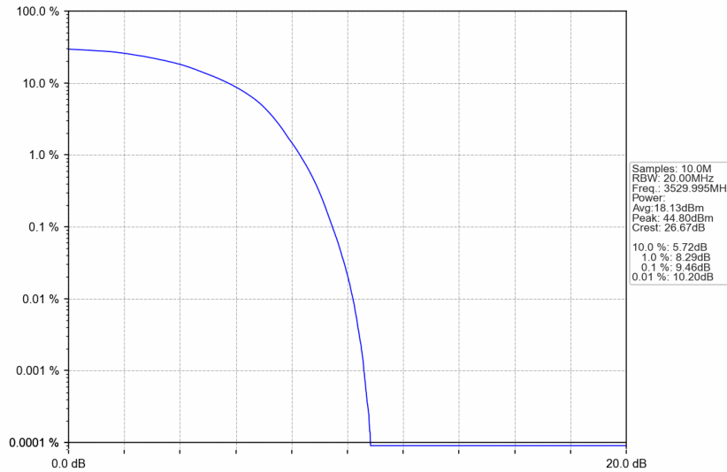
n77d_15kHz_SISO_NTNV_40MHz_DFT-s-OFDM QPSK_3529.995MHz_Outer_Full
