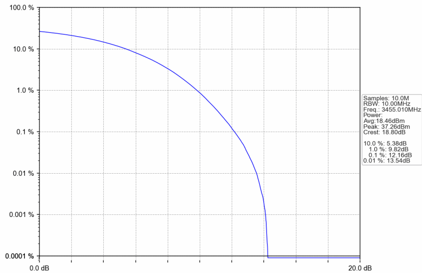
n77d_15kHz_SISO_NTNV_10MHz_CP-OFDM 16 QAM_3455.01MHz_Outer_Full
