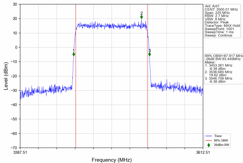
n77d_30kHz_SISO_NTNV_90MHz_CP-OFDM 16 QAM_3500.01MHz_Outer_Full
