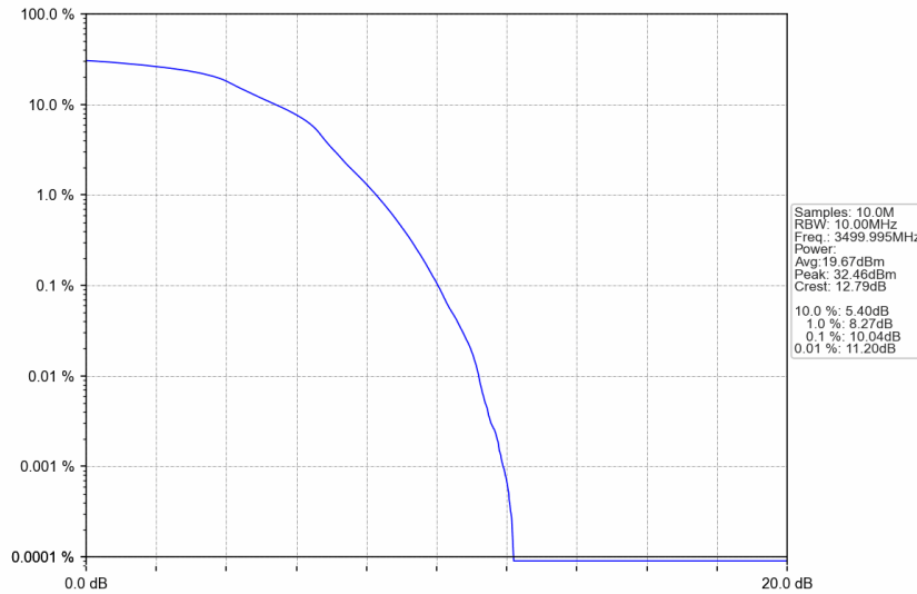
n77d_15kHz_SISO_NTNV_10MHz_DFT-s-OFDM 16 QAM_3499.995MHz_Outer_Full
