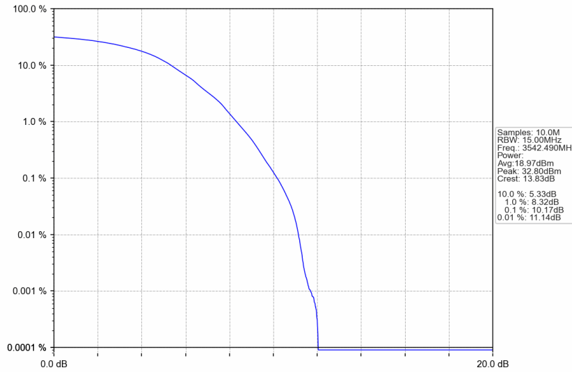
n77d_15kHz_SISO_NTNV_15MHz_DFT-s-OFDM 64 QAM_3542.49MHz_Outer_Full
