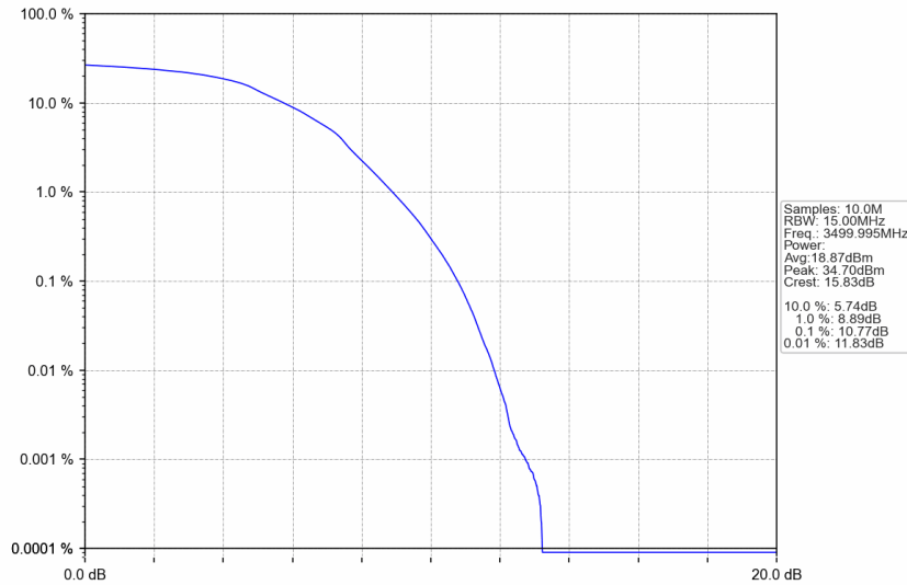
n77d_15kHz_SISO_NTNV_15MHz_DFT-s-OFDM 16 QAM_3499.995MHz_Outer_Full
