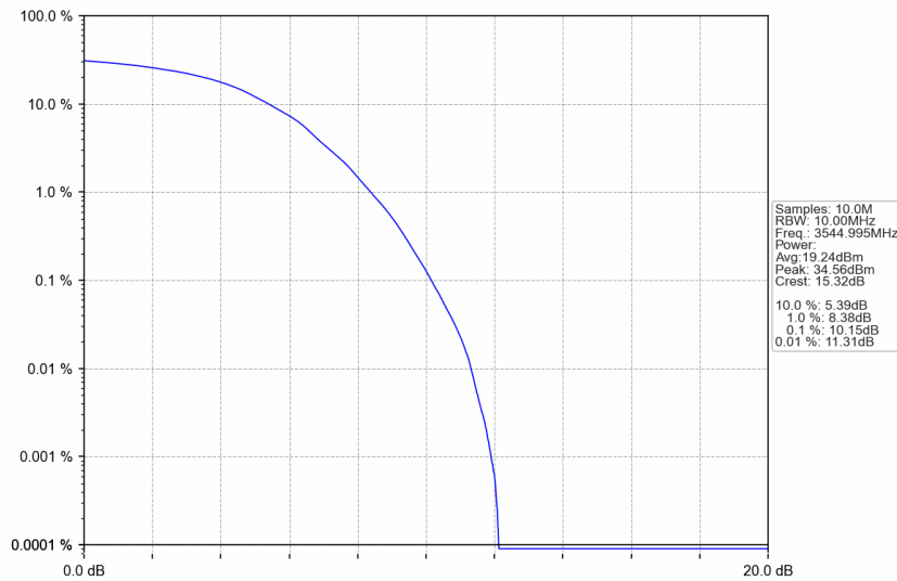
n77d_15kHz_SISO_NTNV_10MHz_DFT-s-OFDM 64 QAM_3544.995MHz_Outer_Full
