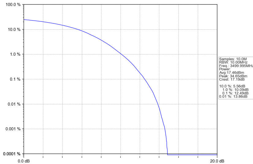
n77d_15kHz_SISO_NTNV_10MHz_CP-OFDM 64 QAM_3499.995MHz_Outer_Full
