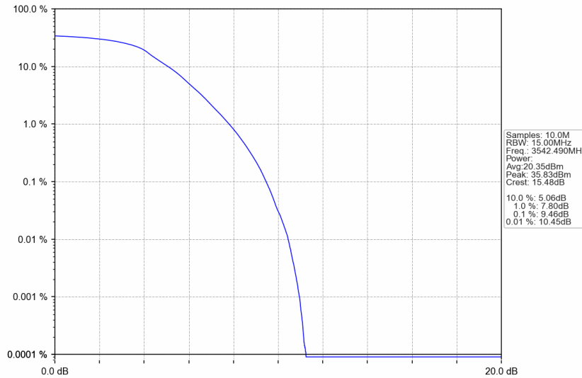
n77d_15kHz_SISO_NTNV_15MHz_DFT-s-OFDM QPSK_3542.49MHz_Outer_Full
