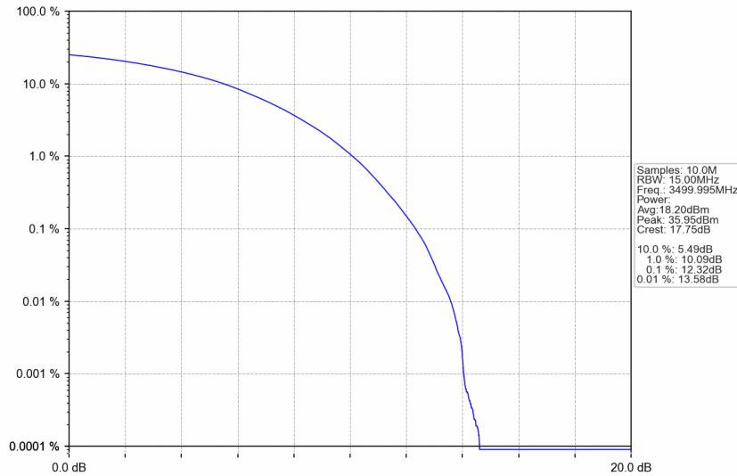
n77d_15kHz_SISO_NTNV_15MHz_CP-OFDM 16 QAM_3499.995MHz_Outer_Full
