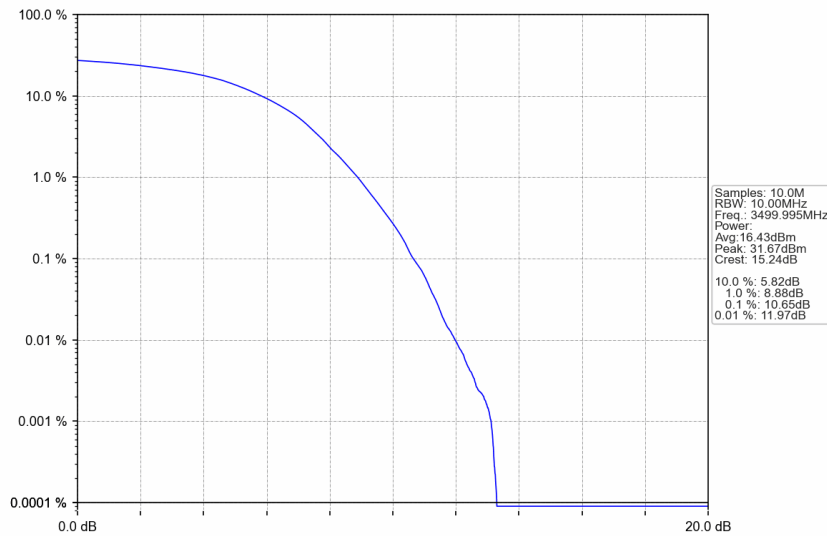
n77d_15kHz_SISO_NTNV_10MHz_DFT-s-OFDM 256 QAM_3499.995MHz_Outer_Full
