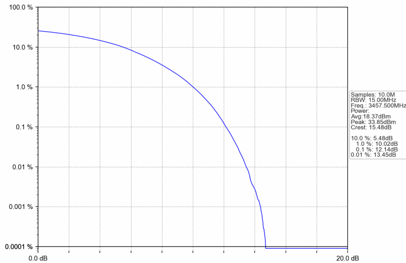
n77d_15kHz_SISO_NTNV_15MHz_CP-OFDM QPSK_3457.5MHz_Outer_Full
