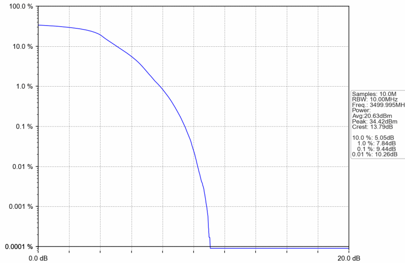
n77d_15kHz_SISO_NTNV_10MHz_DFT-s-OFDM QPSK_3499.995MHz_Outer_Full
