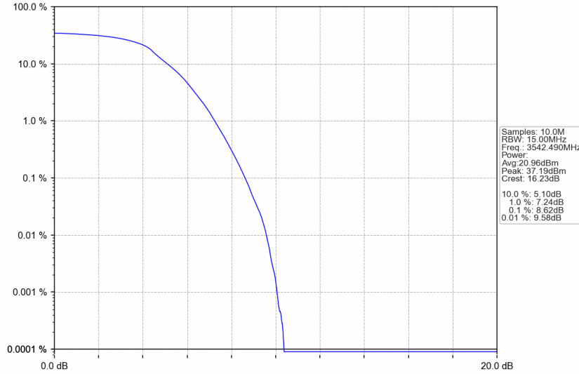
n77d_15kHz_SISO_NTNV_15MHz_DFT-s-OFDM PI/2 BPSK_3542.49MHz_Outer_Full
