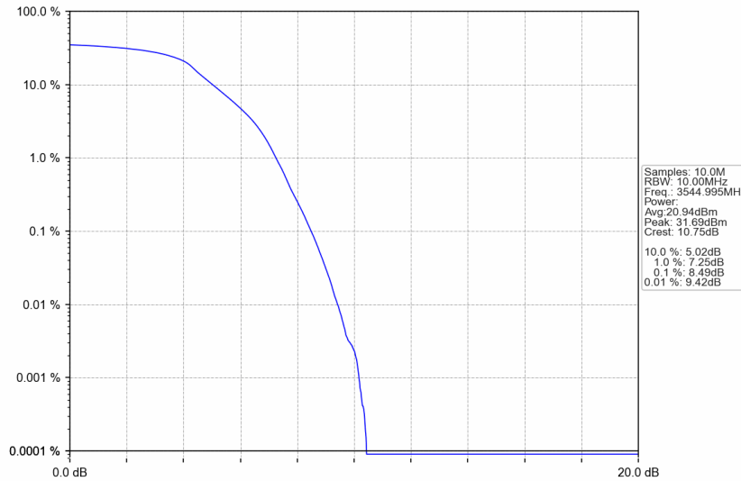
n77d_15kHz_SISO_NTNV_10MHz_DFT-s-OFDM PI/2 BPSK_3544.995MHz_Outer_Full
