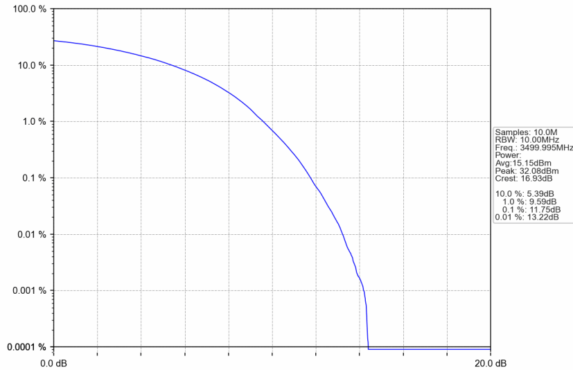
n77d_15kHz_SISO_NTNV_10MHz_CP-OFDM 256 QAM_3499.995MHz_Outer_Full
