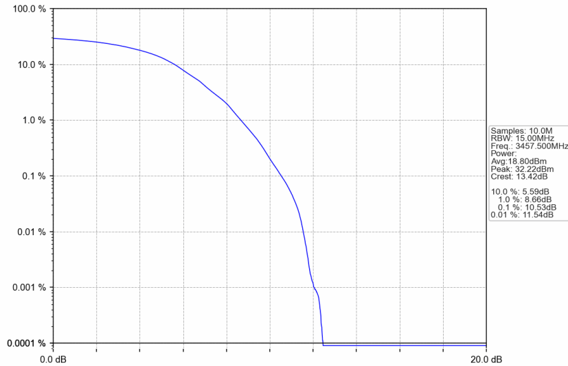
n77d_15kHz_SISO_NTNV_15MHz_DFT-s-OFDM 64 QAM_3457.5MHz_Outer_Full
