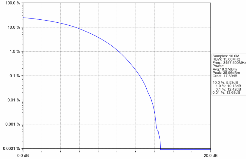
n77d_15kHz_SISO_NTNV_15MHz_CP-OFDM 16 QAM_3457.5MHz_Outer_Full
