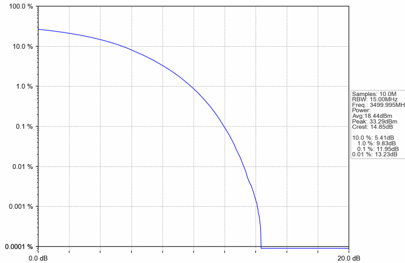
n77d_15kHz_SISO_NTNV_15MHz_CP-OFDM QPSK_3499.995MHz_Outer_Full
