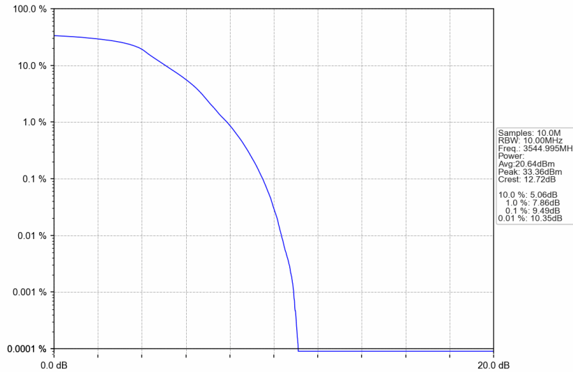
n77d_15kHz_SISO_NTNV_10MHz_DFT-s-OFDM QPSK_3544.995MHz_Outer_Full
