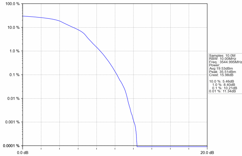
n77d_15kHz_SISO_NTNV_10MHz_DFT-s-OFDM 16 QAM_3544.995MHz_Outer_Full
