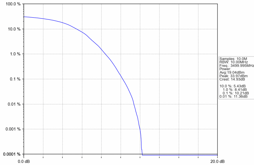
n77d_15kHz_SISO_NTNV_10MHz_DFT-s-OFDM 64 QAM_3499.995MHz_Outer_Full
