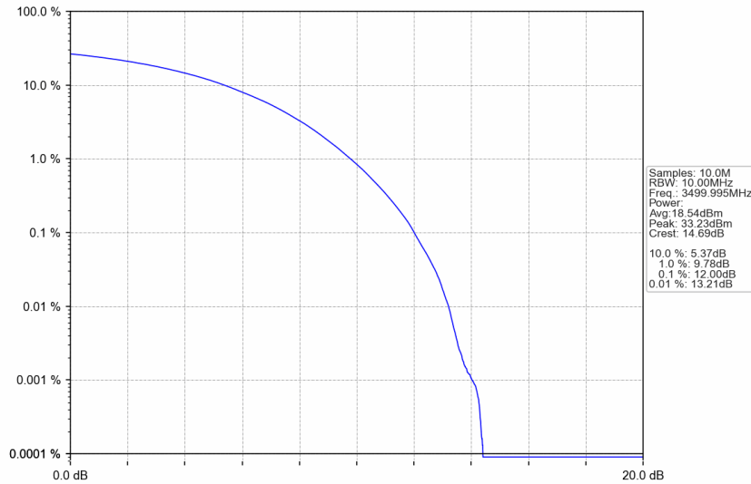
n77d_15kHz_SISO_NTNV_10MHz_CP-OFDM QPSK_3499.995MHz_Outer_Full
