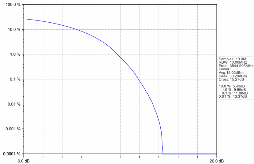
n77d_15kHz_SISO_NTNV_10MHz_CP-OFDM 256 QAM_3544.995MHz_Outer_Full
