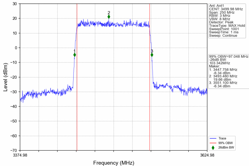
n77d_30kHz_SISO_NTNV_100MHz_DFT-s-OFDM QPSK_3499.98MHz_Outer_Full
