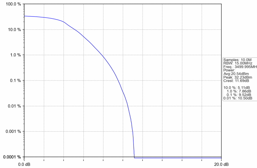
n77d_15kHz_SISO_NTNV_15MHz_DFT-s-OFDM QPSK_3499.995MHz_Outer_Full
