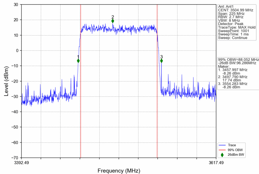
n77d_30kHz_SISO_NTNV_90MHz_CP-OFDM QPSK_3504.99MHz_Outer_Full
