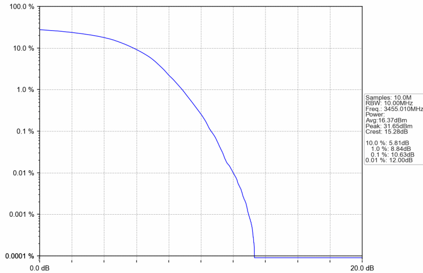
n77d_15kHz_SISO_NTNV_10MHz_DFT-s-OFDM 256 QAM_3455.01MHz_Outer_Full
