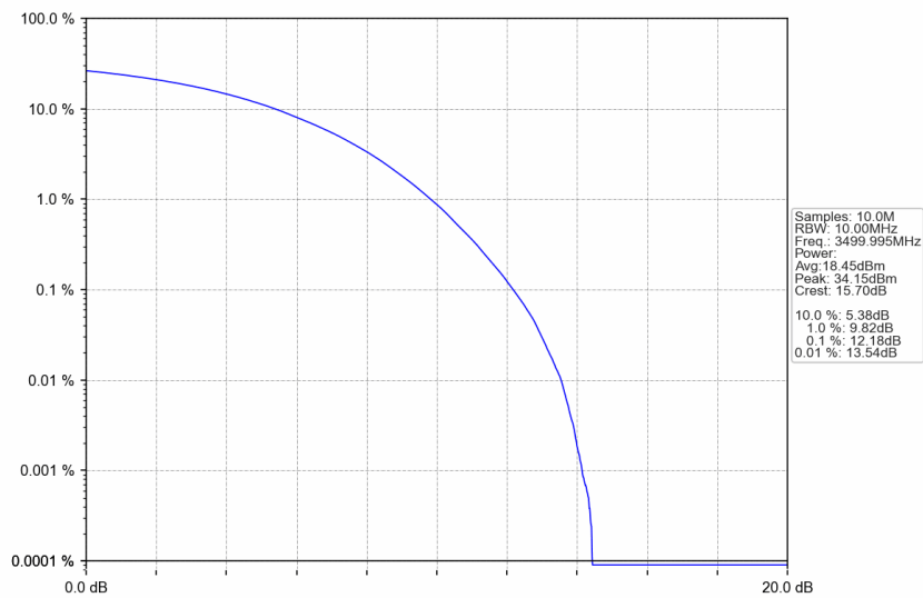
n77d_15kHz_SISO_NTNV_10MHz_CP-OFDM 16 QAM_3499.995MHz_Outer_Full
