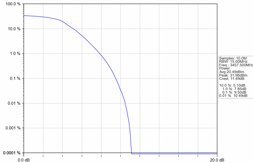
n77d_15kHz_SISO_NTNV_15MHz_DFT-s-OFDM QPSK_3457.5MHz_Outer_Full
