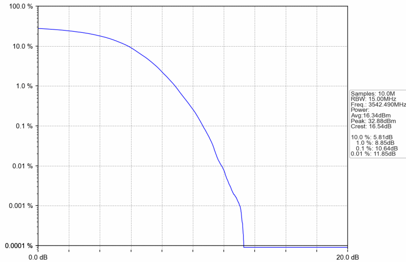
n77d_15kHz_SISO_NTNV_15MHz_DFT-s-OFDM 256 QAM_3542.49MHz_Outer_Full
