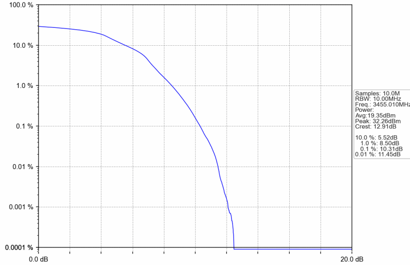
n77d_15kHz_SISO_NTNV_10MHz_DFT-s-OFDM 16 QAM_3455.01MHz_Outer_Full
