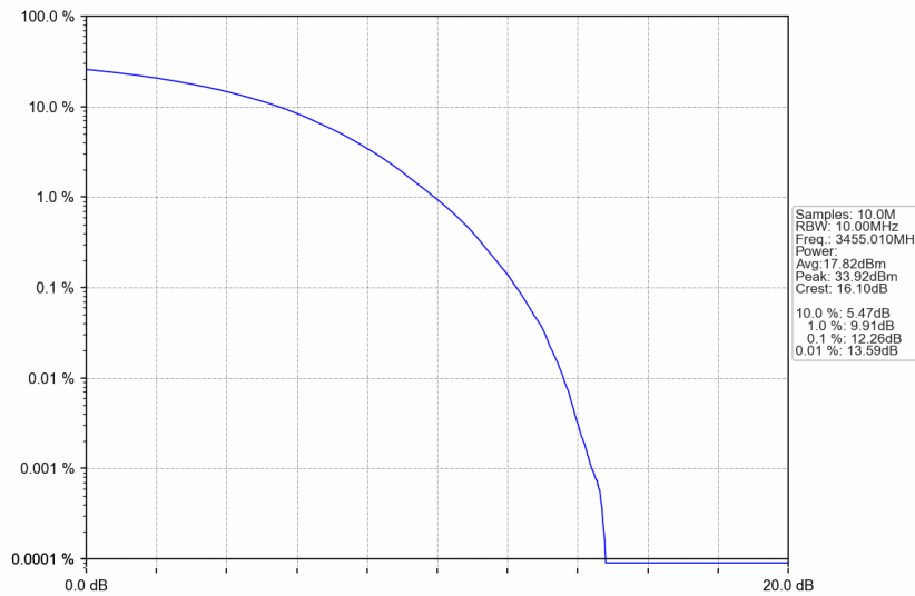
n77d_15kHz_SISO_NTNV_10MHz_CP-OFDM 64 QAM_3455.01MHz_Outer_Full
