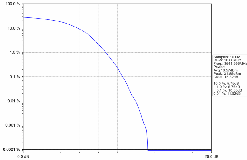
n77d_15kHz_SISO_NTNV_10MHz_DFT-s-OFDM 256 QAM_3544.995MHz_Outer_Full
