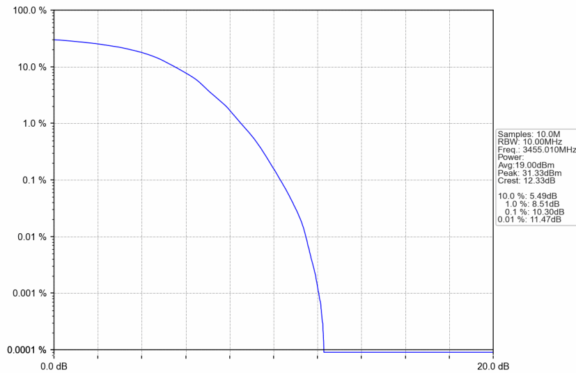
n77d_15kHz_SISO_NTNV_10MHz_DFT-s-OFDM 64 QAM_3455.01MHz_Outer_Full
