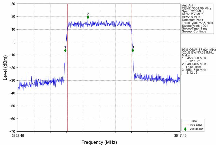
n77d_30kHz_SISO_NTNV_90MHz_CP-OFDM 64 QAM_3504.99MHz_Outer_Full
