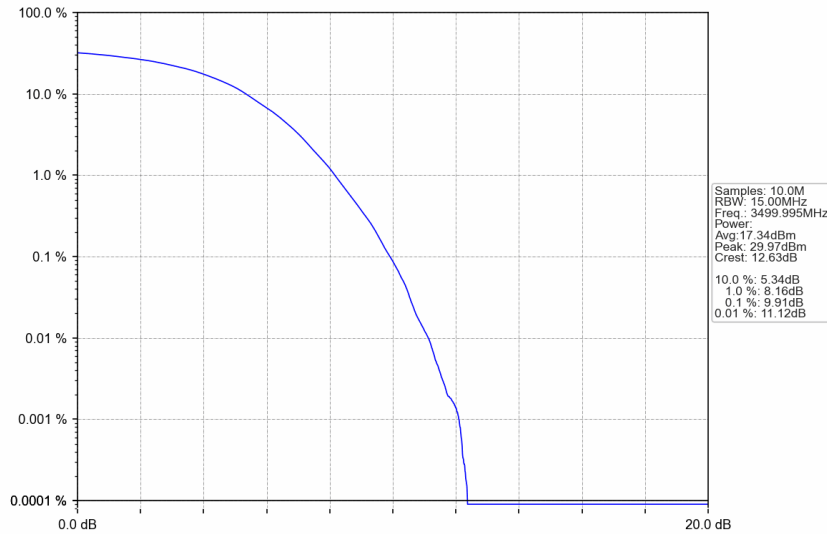
n77d_15kHz_SISO_NTNV_15MHz_DFT-s-OFDM 256 QAM_3499.995MHz_Outer_Full
