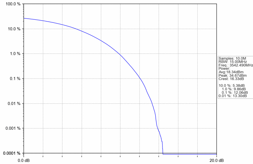
n77d_15kHz_SISO_NTV_15MHz_CP-OFDM 16 QAM_3542.49MHz_Outer_Full
