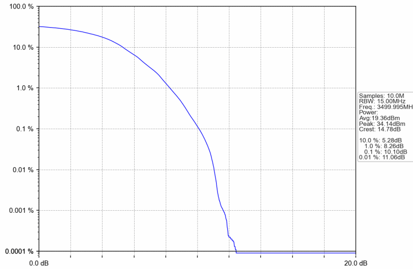
n77d_15kHz_SISO_NTNV_15MHz_DFT-s-OFDM 64 QAM_3499.995MHz_Outer_Full
