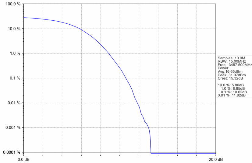
n77d_15kHz_SISO_NTNV_15MHz_DFT-s-OFDM 256 QAM_3457.5MHz_Outer_Full
