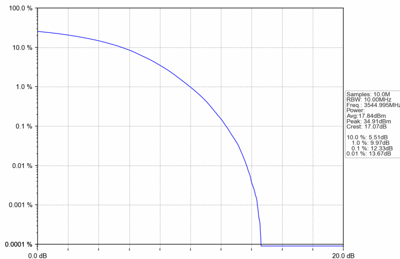
n77d_15kHz_SISO_NTNV_10MHz_CP-OFDM 64 QAM_3544.995MHz_Outer_Full
