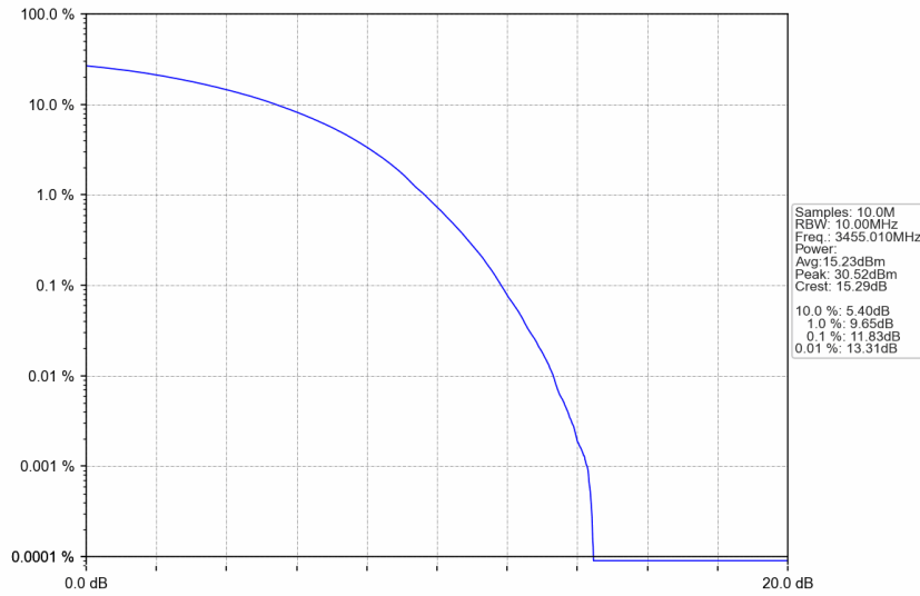
n77d_15kHz_SISO_NTNV_10MHz_CP-OFDM 256 QAM_3455.01MHz_Outer_Full
