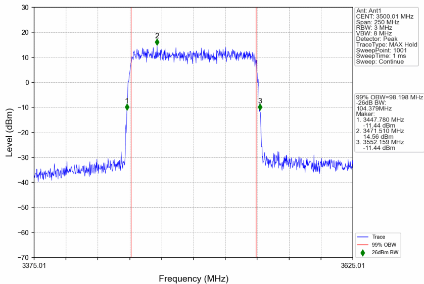
n77d_30kHz_SISO_NTNV_100MHz_CP-OFDM 256 QAM_3500.01MHz_Outer_Full
