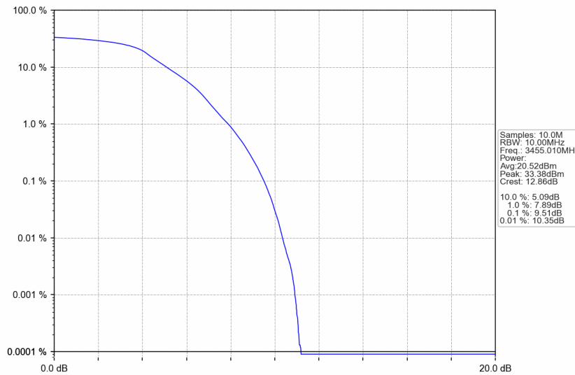
n77d_15kHz_SISO_NTNV_10MHz_DFT-s-OFDM QPSK_3455.01MHz_Outer_Full
