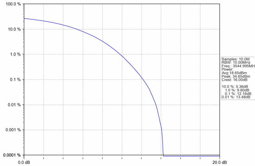
n77d_15kHz_SISO_NTNV_10MHz_CP-OFDM 16 QAM_3544.995MHz_Outer_Full
