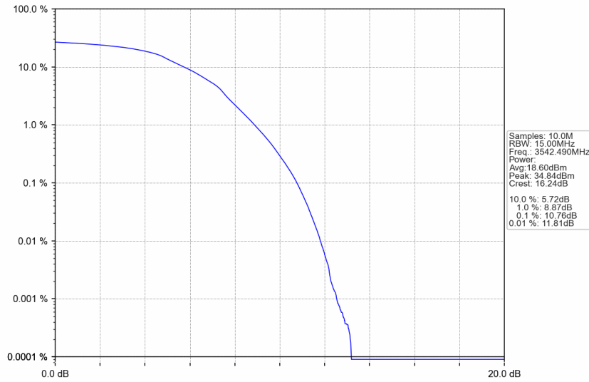
n77d_15kHz_SISO_NTNV_15MHz_DFT-s-OFDM 16 QAM_3542.49MHz_Outer_Full
