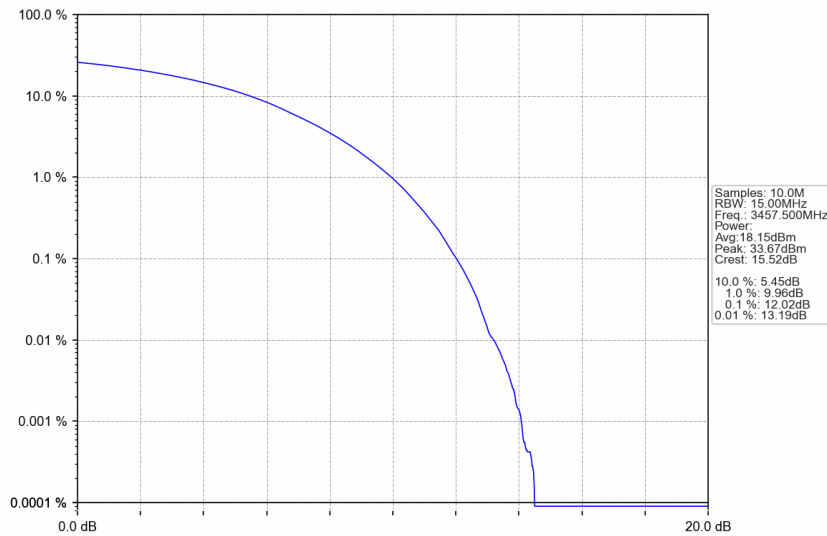
n77d_15kHz_SISO_NTV_15MHz_CP-OFDM 64 QAM_3457.5MHz_Outer_Full
