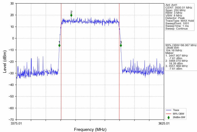
n77d_30kHz_SISO_NTNV_100MHz_CP-OFDM 16 QAM_3500.01MHz_Outer_Full
