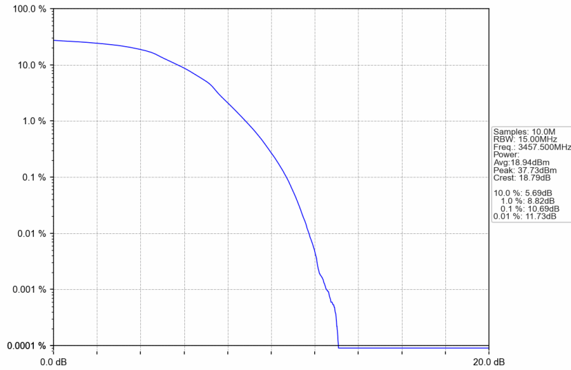
n77d_15kHz_SISO_NTNV_15MHz_DFT-s-OFDM 16 QAM_3457.5MHz_Outer_Full
