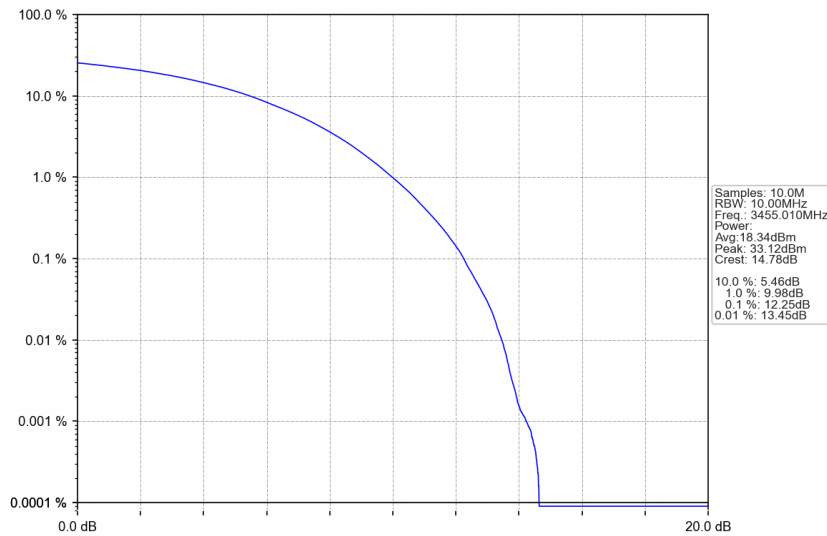
n77d_15kHz_SISO_NTNV_10MHz_CP-OFDM QPSK_3455.01MHz_Outer_Full
