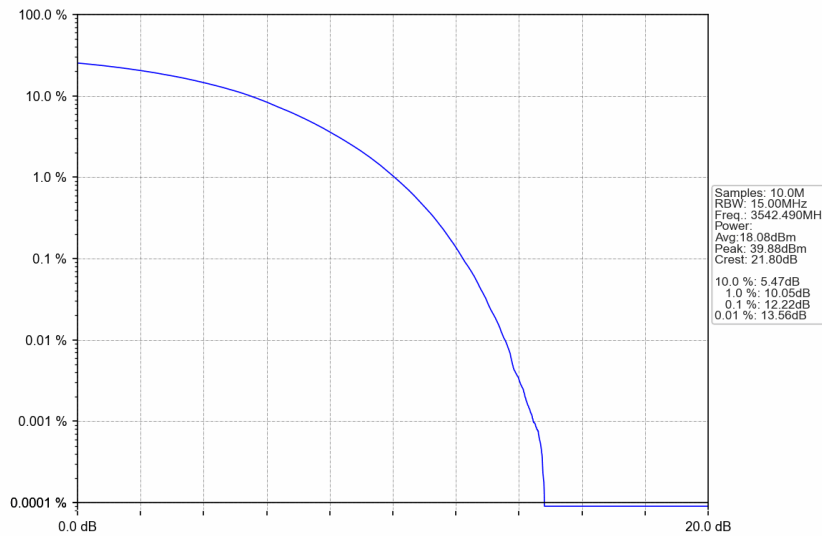
n77d_15kHz_SISO_NTNV_15MHz_CP-OFDM QPSK_3542.49MHz_Outer_Full
