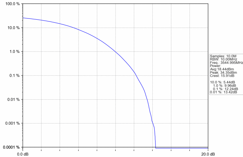
n77d_15kHz_SISO_NTNV_10MHz_CP-OFDM QPSK_3544.995MHz_Outer_Full
