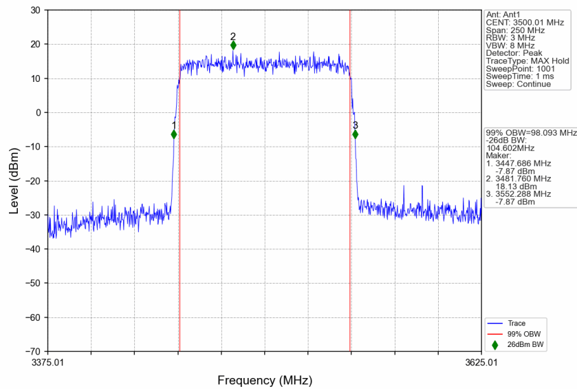
n77d_30kHz_SISO_NTNV_100MHz_CP-OFDM 64 QAM_3499.98MHz_Outer_Full
