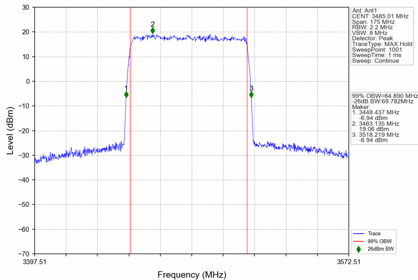
n77d_30kHz_SISO_NTNV_70MHz_DFT-s-OFDM 64 QAM_3485.01MHz_Outer_Full
