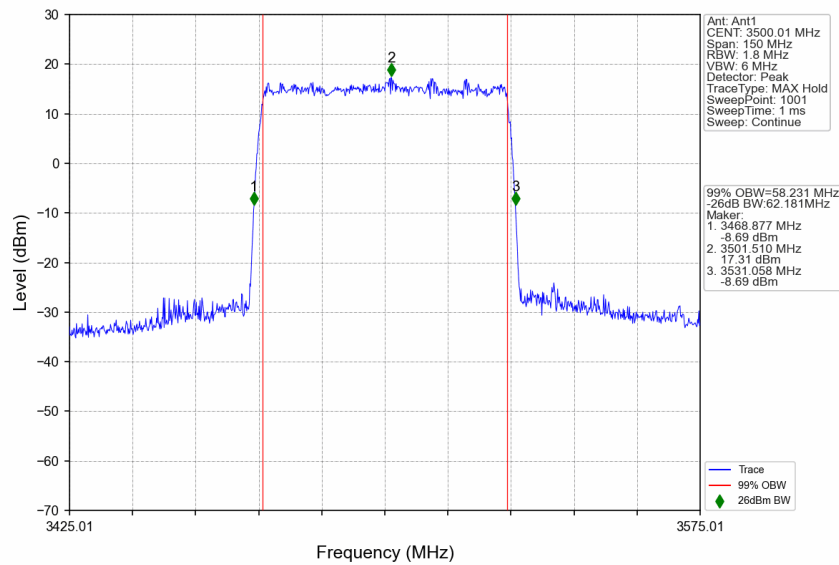
n77d_30kHz_SISO_NTNV_60MHz_DFT-s-OFDM 256 QAM_3500.01MHz_Outer_Full
