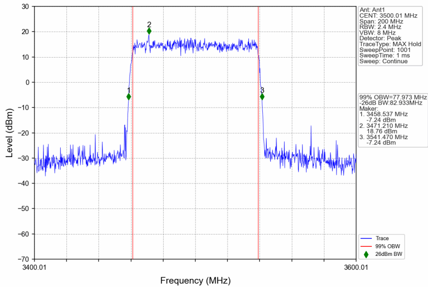
n77d_30kHz_SISO_NTNV_80MHz_CP-OFDM 16 QAM_3500.01MHz_Outer_Full
