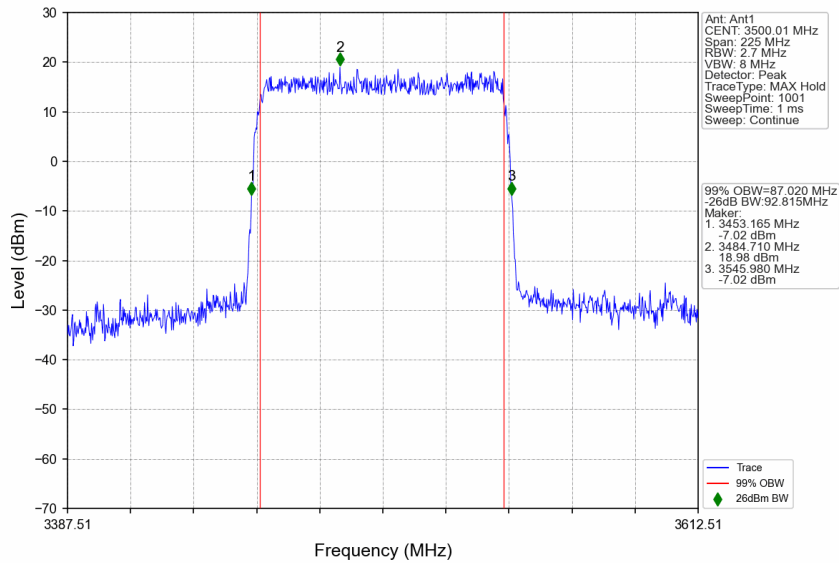
n77d_30kHz_SISO_NTNV_90MHz_DFT-s-OFDM 16 QAM_3500.01MHz_Outer_Full
