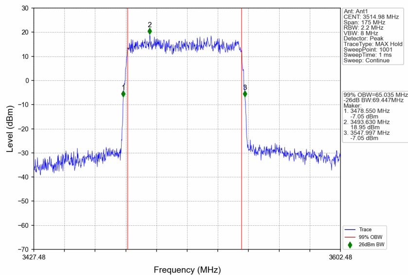
n77d_30kHz_SISO_NTNV_70MHz_DFT-s-OFDM 64 QAM_3514.98MHz_Outer_Full
