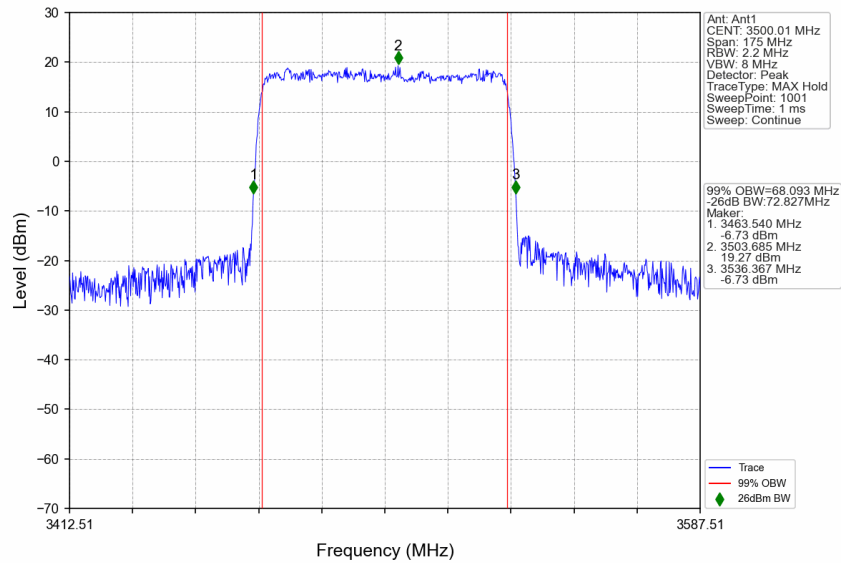
n77d_30kHz_SISO_NTNV_70MHz_CP-OFDM 16 QAM_3500.01MHz_Outer_Full
