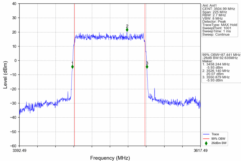
n77d_30kHz_SISO_NTNV_90MHz_DFT-s-OFDM QPSK_3504.99MHz_Outer_Full
