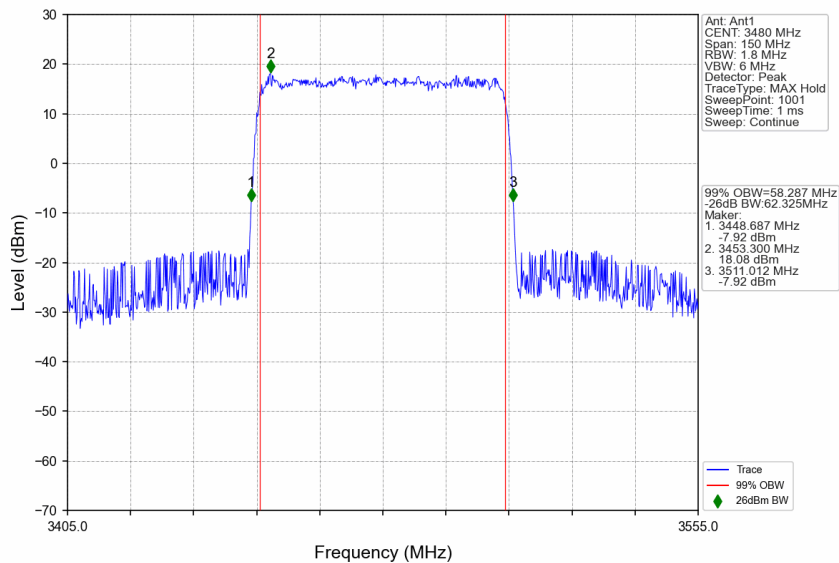
n77d_30kHz_SISO_NTNV_60MHz_CP-OFDM 64 QAM_3480MHz_Outer_Full
