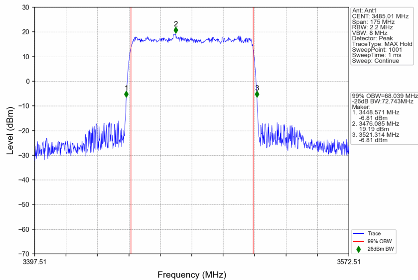
n77d_30kHz_SISO_NTNV_70MHz_CP-OFDM 64 QAM_3485.01MHz_Outer_Full
