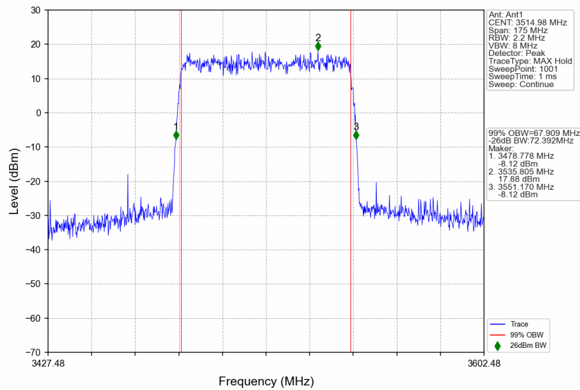
n77d_30kHz_SISO_NTNV_70MHz_CP-OFDM 64 QAM_3514.98MHz_Outer_Full
