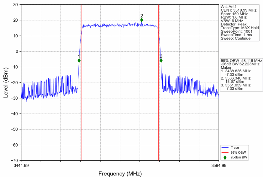
n77d_30kHz_SISO_NTNV_60MHz_CP-OFDM QPSK_3519.99MHz_Outer_Full
