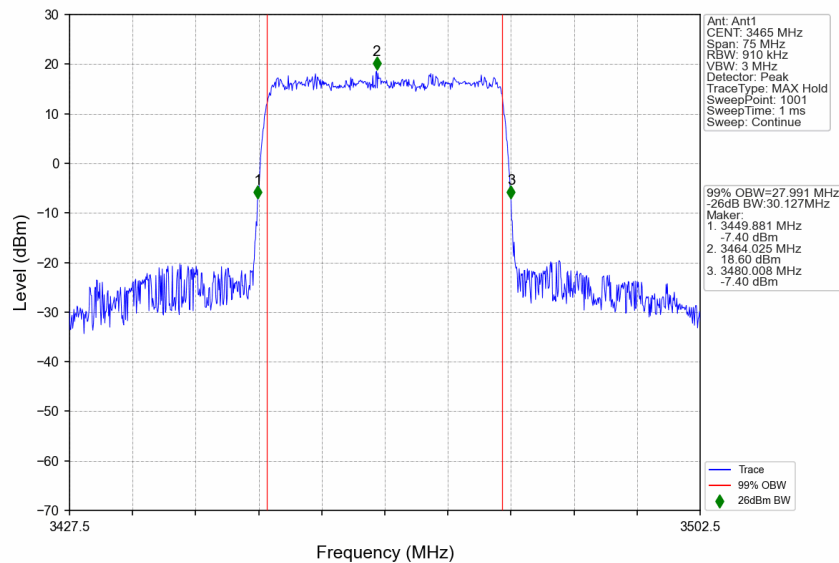
n77d_30kHz_SISO_NTNV_30MHz_CP-OFDM 64 QAM_3465MHz_Outer_Full
