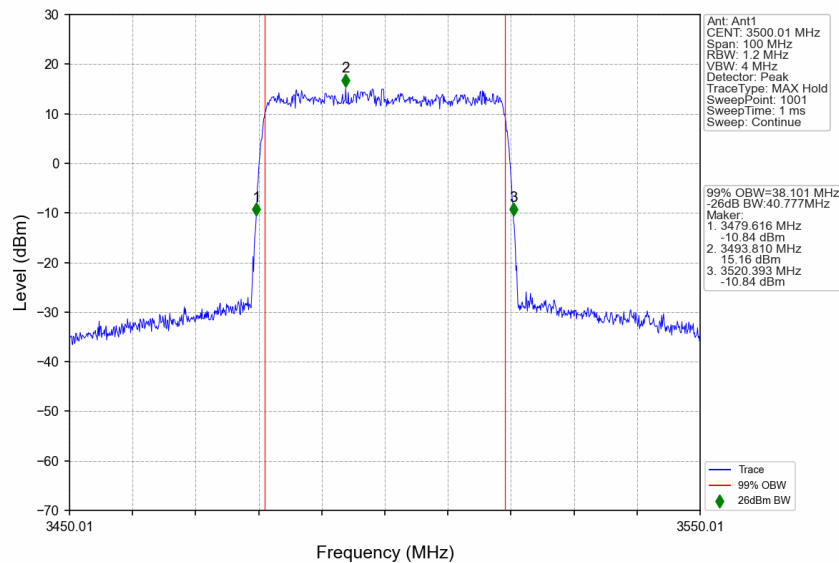
n77d_30kHz_SISO_NTNV_40MHz_CP-OFDM 256 QAM_3500.01MHz_Outer_Full
