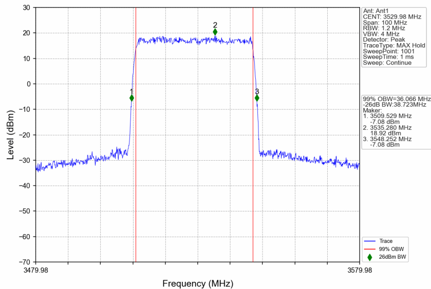
n77d_30kHz_SISO_NTNV_40MHz_DFT-s-OFDM 64 QAM_3529.98MHz_Outer_Full
