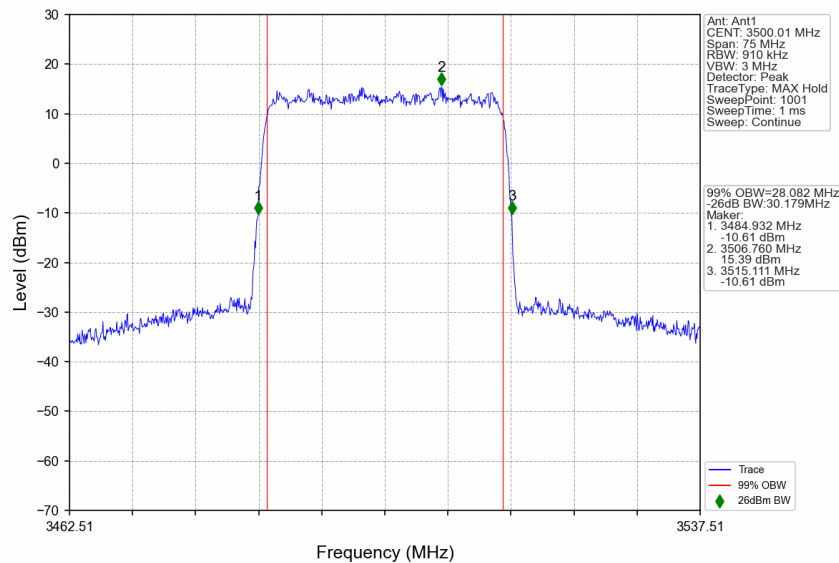
n77d_30kHz_SISO_NTNV_30MHz_CP-OFDM 256 QAM_3500.01MHz_Outer_Full
