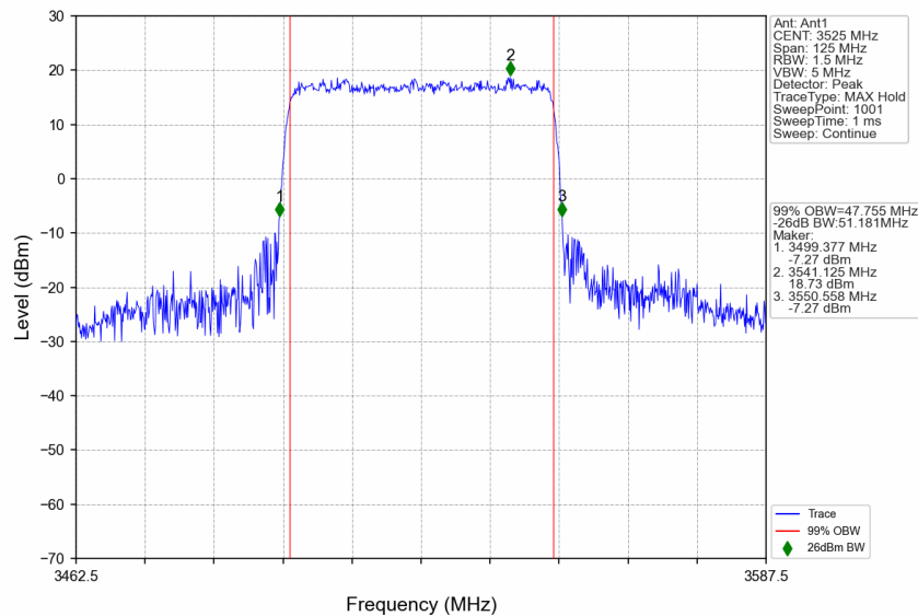
n77d_30kHz_SISO_NTNV_50MHz_CP-OFDM QPSK_3525MHz_Outer_Full
