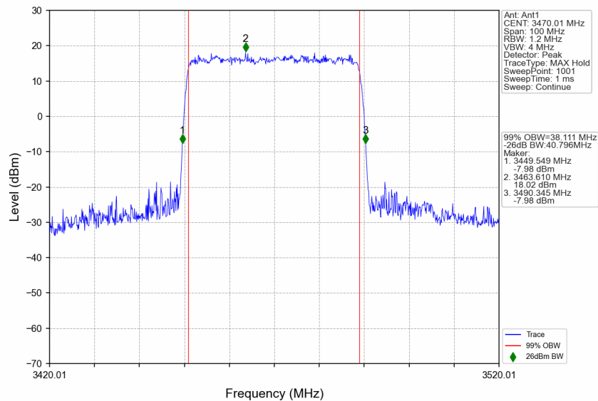
n77d_30kHz_SISO_NTNV_40MHz_CP-OFDM 64 QAM_3470.01MHz_Outer_Full
