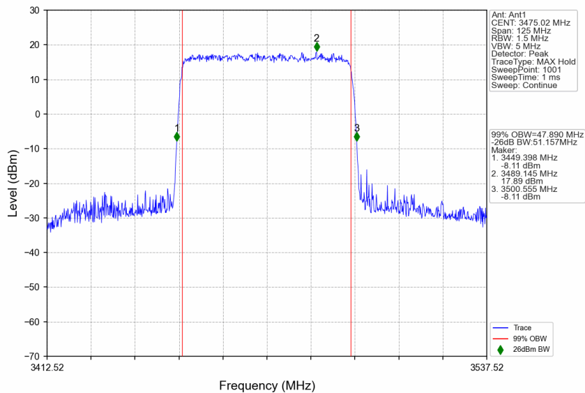
n77d_30kHz_SISO_NTNV_50MHz_CP-OFDM 64 QAM_3475.02MHz_Outer_Full
