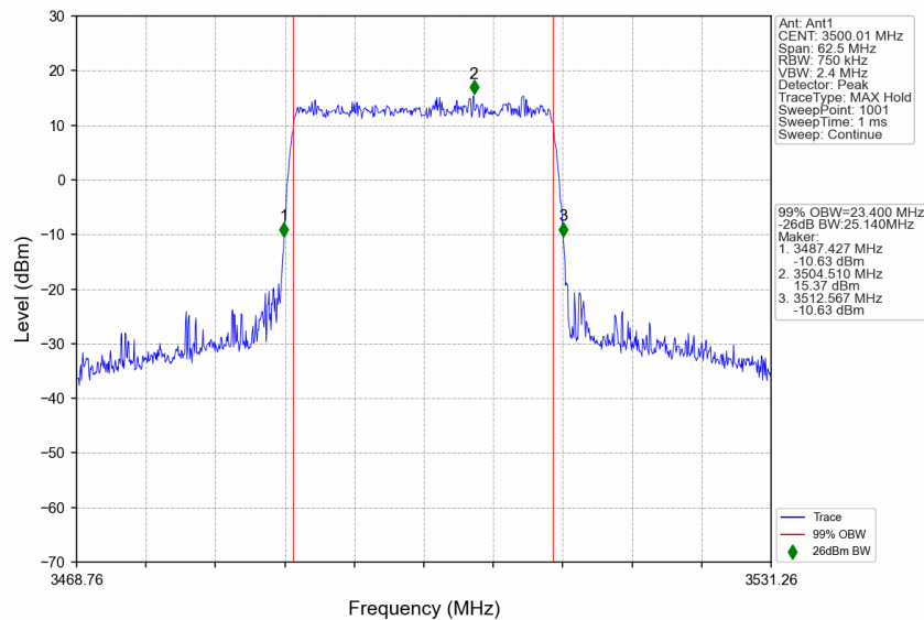
n77d_30kHz_SISO_NTNV_25MHz_CP-OFDM 256 QAM_3500.01MHz_Outer_Full
