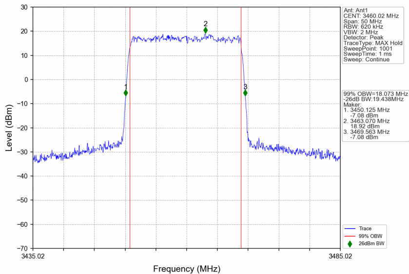
n77d_30kHz_SISO_NTNV_20MHz_DFT-s-OFDM 64 QAM_3460.02MHz_Outer_Full
