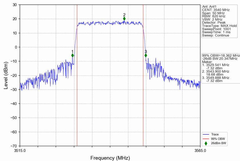
n77d_30kHz_SISO_NTNV_20MHz_CP-OFDM QPSK_3540MHz_Outer_Full
