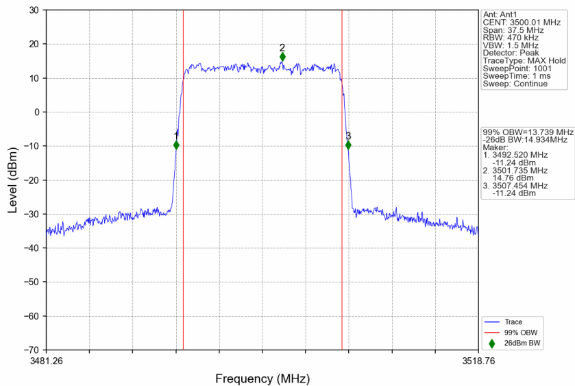
n77d_30kHz_SISO_NTNV_15MHz_CP-OFDM 256 QAM_3500.01MHz_Outer_Full
