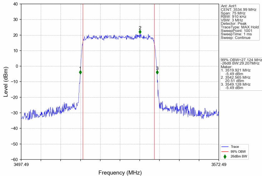
n77d_30kHz_SISO_NTNV_30MHz_DFT-s-OFDM QPSK_3534.99MHz_Outer_Full
