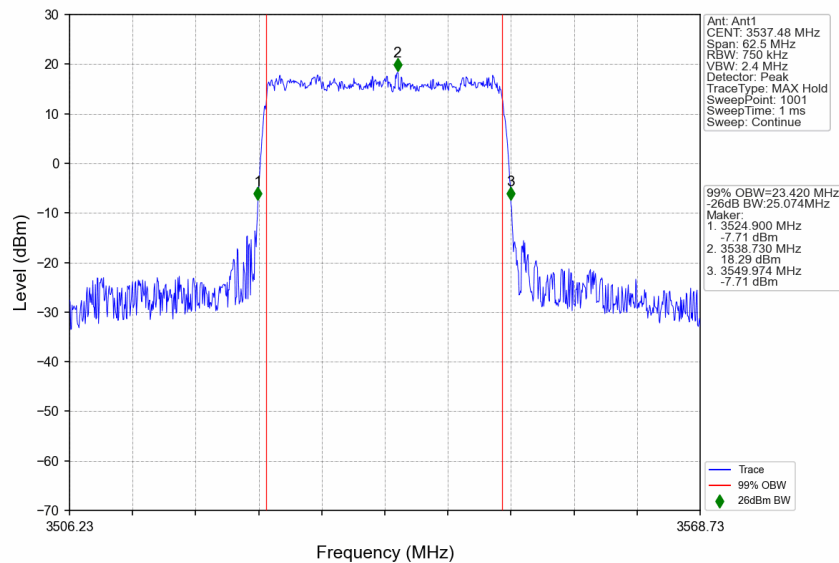
n77d_30kHz_SISO_NTNV_25MHz_CP-OFDM 64 QAM_3537.48MHz_Outer_Full
