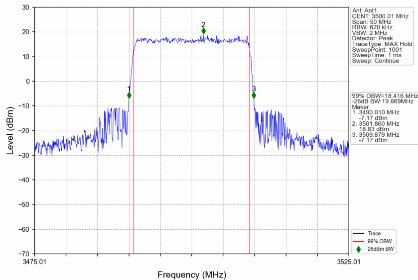
n77d_30kHz_SISO_NTNV_20MHz_CP-OFDM 16 QAM_3500.01MHz_Outer_Full
