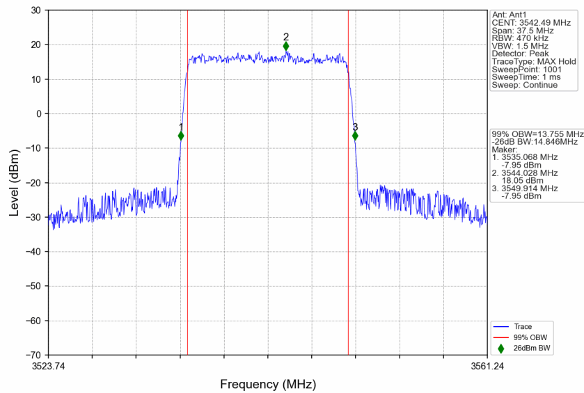
n77d_30kHz_SISO_NTNV_15MHz_CP-OFDM 64 QAM_3542.49MHz_Outer_Full
