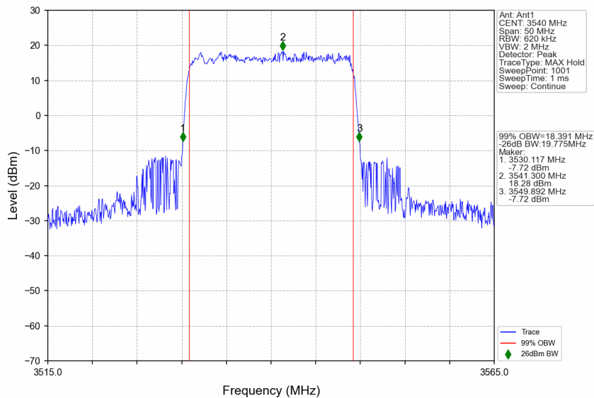
n77d_30kHz_SISO_NTNV_20MHz_CP-OFDM 64 QAM_3540MHz_Outer_Full
