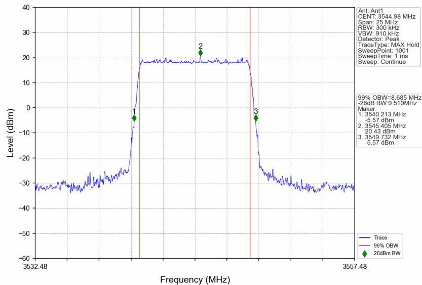
n77d_30kHz_SISO_NTNV_10MHz_DFT-s-OFDM QPSK_3544.98MHz_Outer_Full
