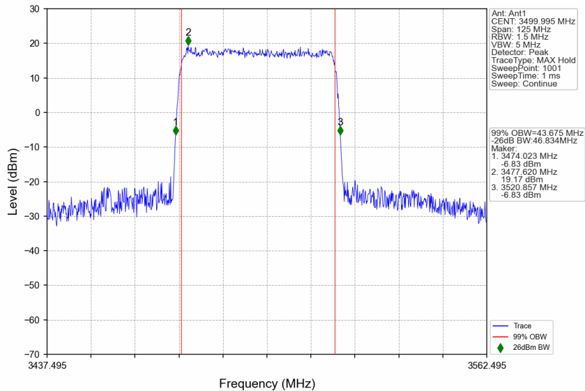
n77d_15kHz_SISO_NTNV_50MHz_CP-OFDM 16 QAM_3499.995MHz_Outer_Full
