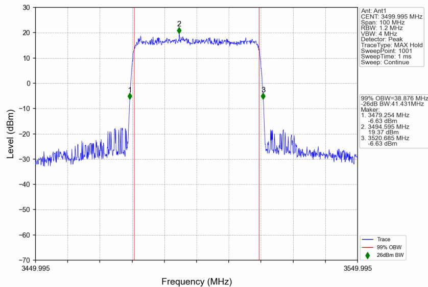
n77d_15kHz_SISO_NTNV_40MHz_CP-OFDM 16 QAM_3499.995MHz_Outer_Full
