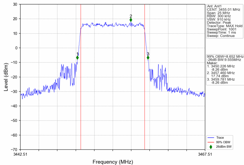
n77d_30kHz_SISO_NTNV_10MHz_CP-OFDM 64 QAM_3455.01MHz_Outer_Full
