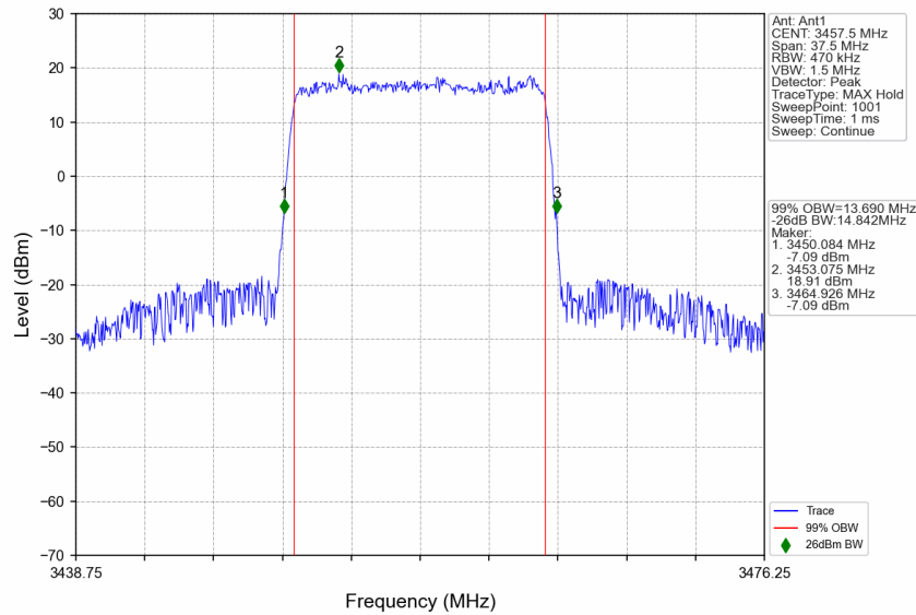
n77d_30kHz_SISO_NTNV_15MHz_CP-OFDM QPSK_3457.5MHz_Outer_Full
