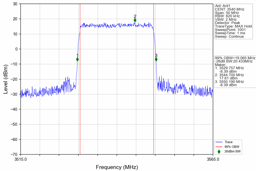
n77d_15kHz_SISO_NTNV_20MHz_CP-OFDM 64 QAM_3540MHz_Outer_Full
