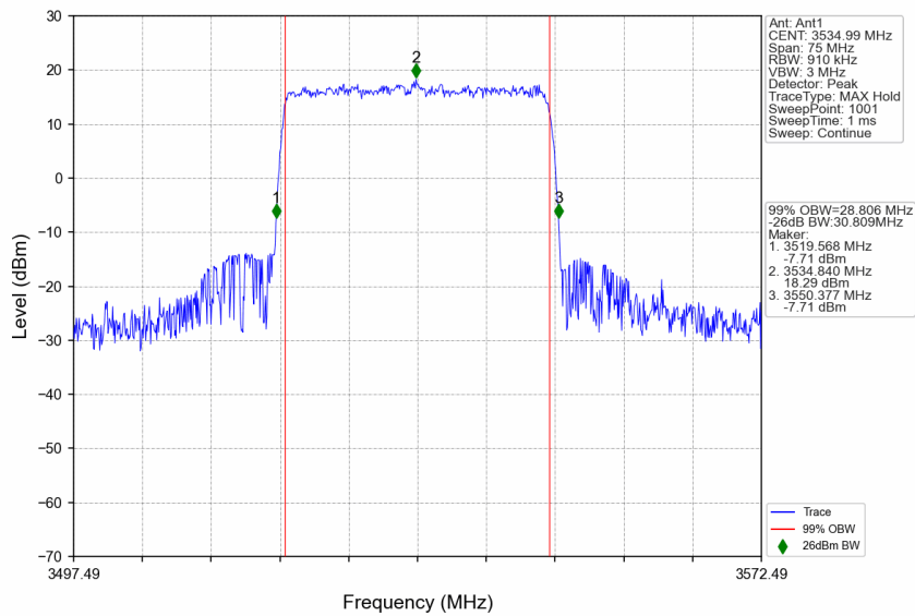
n77d_15kHz_SISO_NTNV_30MHz_CP-OFDM 64 QAM_3534.99MHz_Outer_Full
