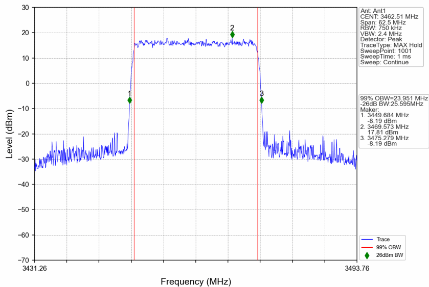
n77d_15kHz_SISO_NTNV_25MHz_CP-OFDM 64 QAM_3462.51MHz_Outer_Full
