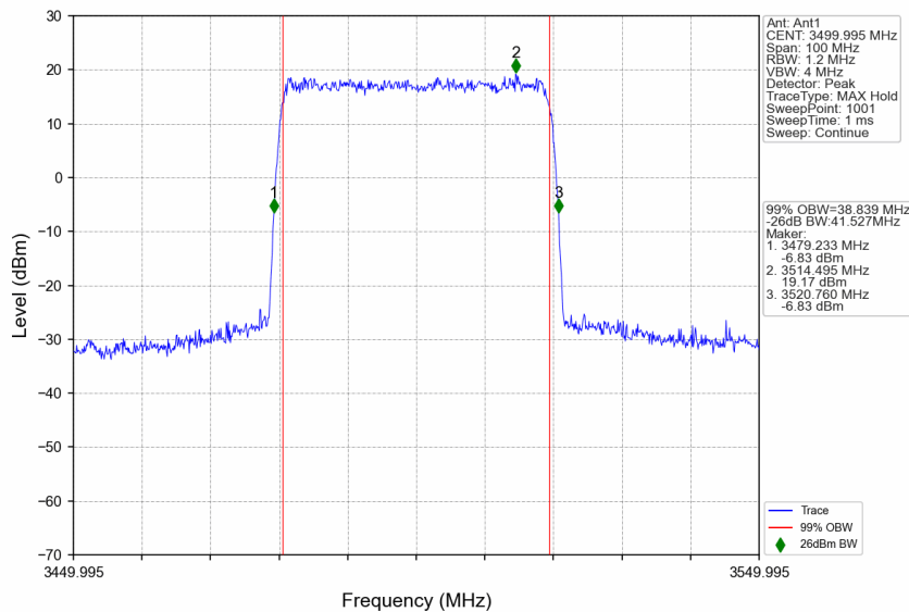
n77d_15kHz_SISO_NTNV_40MHz_DFT-s-OFDM 16 QAM_3499.995MHz_Outer_Full
