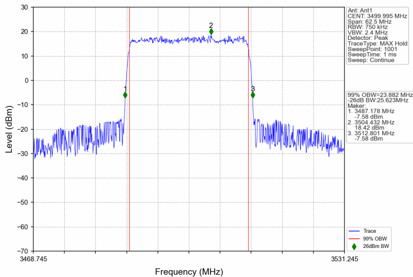
n77d_15kHz_SISO_NTNV_25MHz_CP-OFDM 16 QAM_3499.995MHz_Outer_Full
