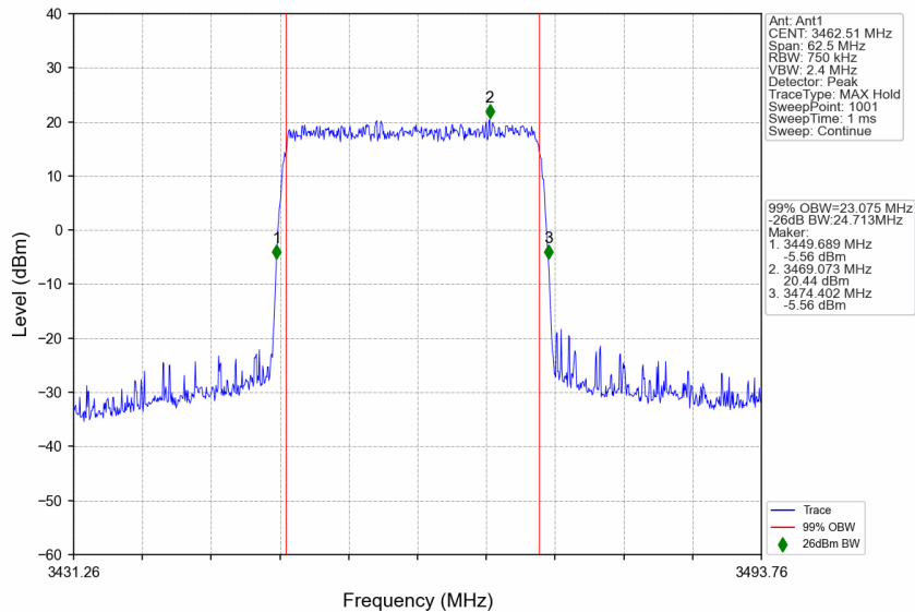
n77d_15kHz_SISO_NTNV_25MHz_DFT-s-OFDM QPSK_3462.51MHz_Outer_Full
