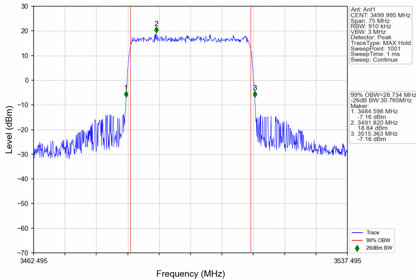
n77d_15kHz_SISO_NTNV_30MHz_CP-OFDM 16 QAM_3499.995MHz_Outer_Full
