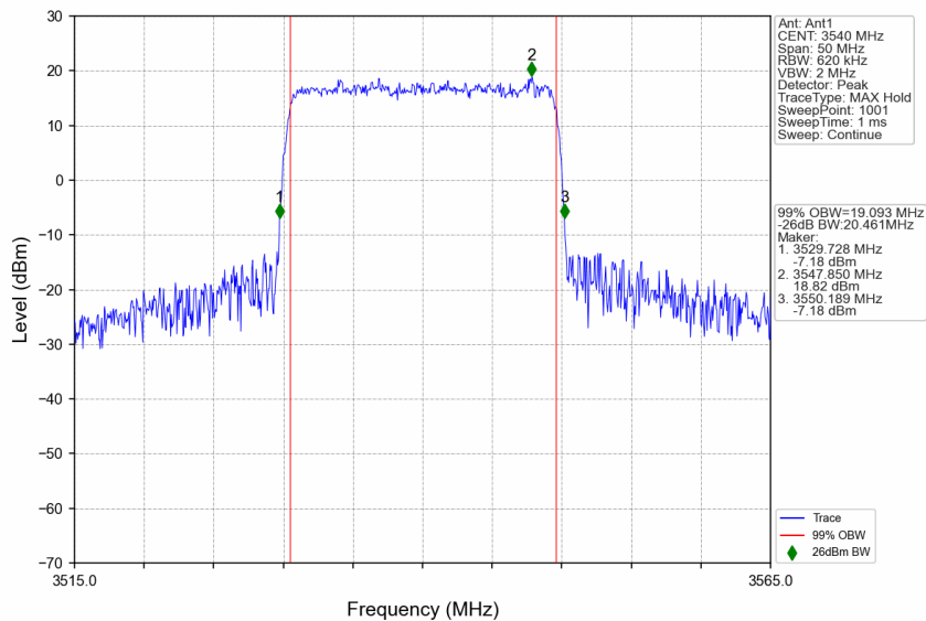
n77d_15kHz_SISO_NTNV_20MHz_CP-OFDM QPSK_3540MHz_Outer_Full
