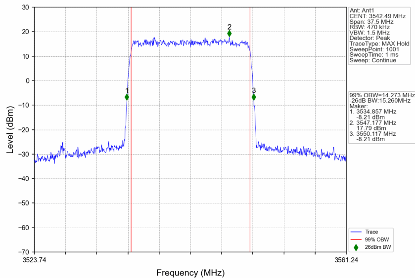
n77d_15kHz_SISO_NTNV_15MHz_CP-OFDM 64 QAM_3542.49MHz_Outer_Full
