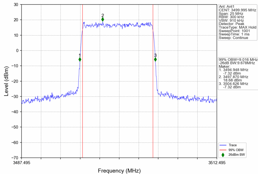
n77d_15kHz_SISO_NTNV_10MHz_DFT-s-OFDM 16 QAM_3499.995MHz_Outer_Full
