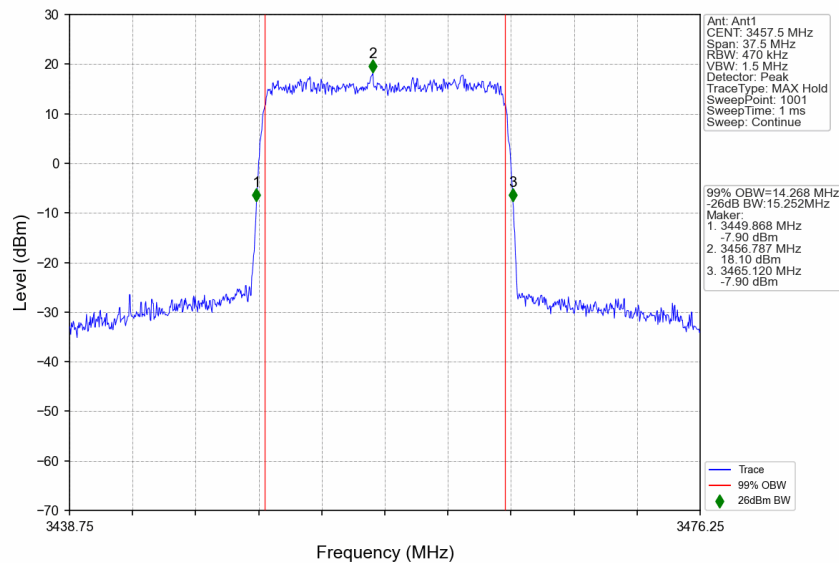
n77d_15kHz_SISO_NTNV_15MHz_CP-OFDM 64 QAM_3457.5MHz_Outer_Full
