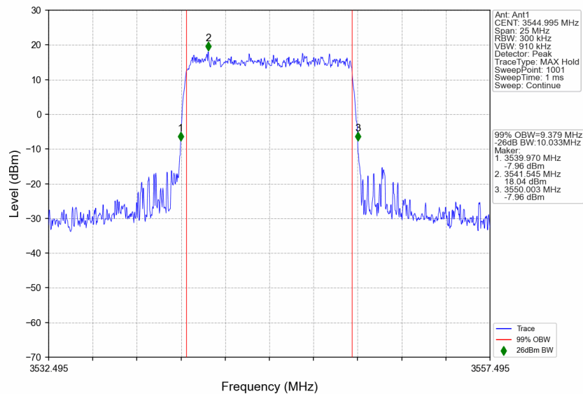
n77d_15kHz_SISO_NTNV_10MHz_CP-OFDM 64 QAM_3544.995MHz_Outer_Full
