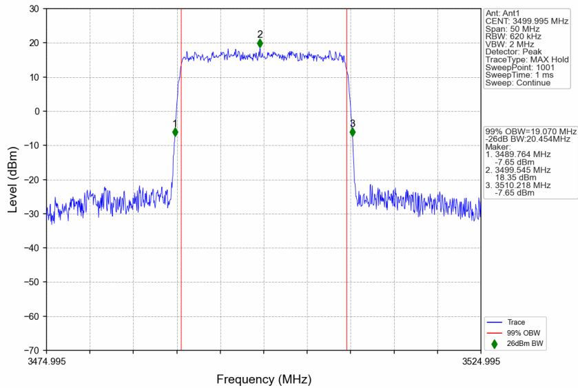
n77d_15kHz_SISO_NTNV_20MHz_CP-OFDM 16 QAM_3499.995MHz_Outer_Full
