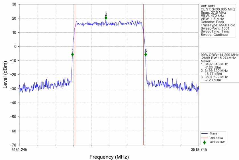
n77d_15kHz_SISO_NTNV_15MHz_CP-OFDM 16 QAM_3499.995MHz_Outer_Full
