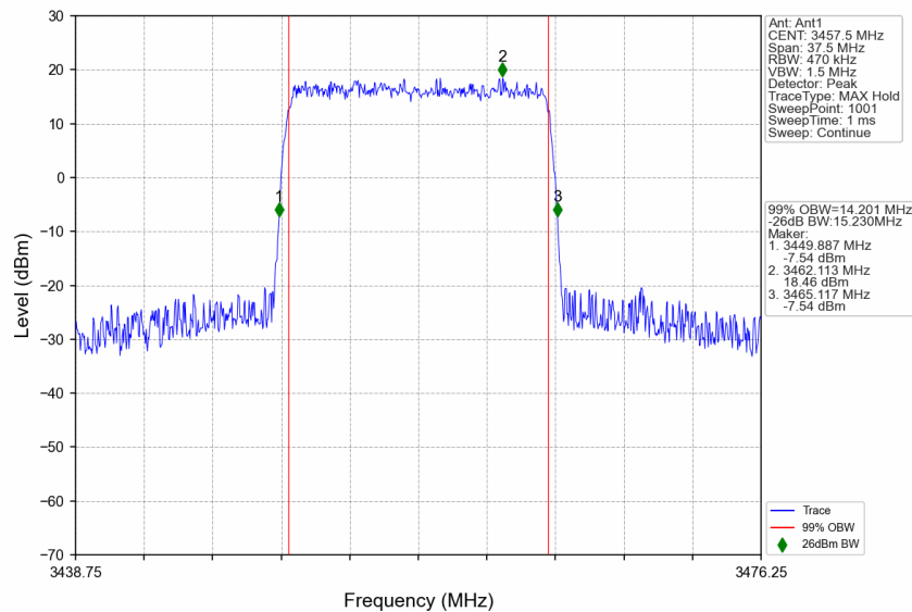
n77d_15kHz_SISO_NTNV_15MHz_CP-OFDM QPSK_3457.5MHz_Outer_Full
