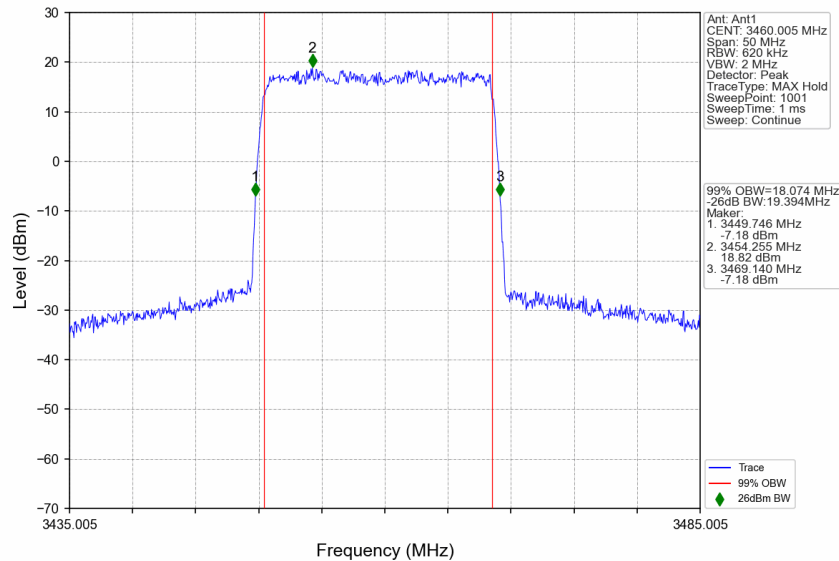
n77d_15kHz_SISO_NTNV_20MHz_DFT-s-OFDM 64 QAM_3460.005MHz_Outer_Full
