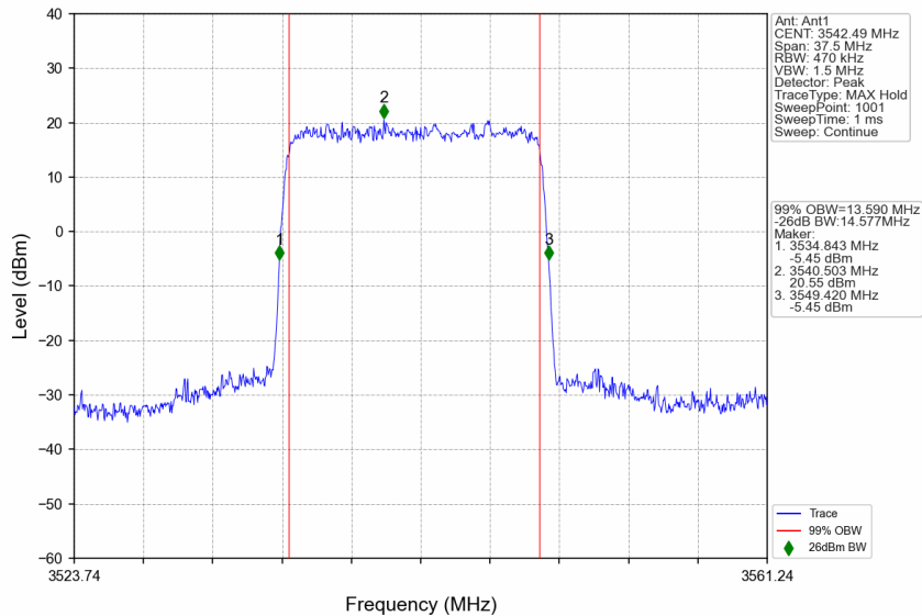
n77d_15kHz_SISO_NTNV_15MHz_DFT-s-OFDM QPSK_3542.49MHz_Outer_Full
