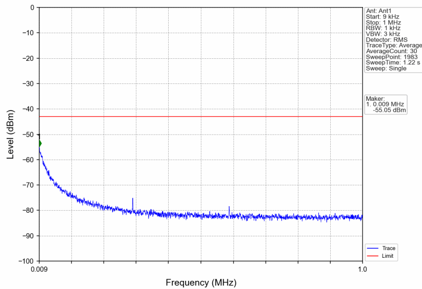
n66_30kHz_SISO_NTNV_40MHz_CP-OFDM QPSK_1760MHz_Edge_1RB_Right
