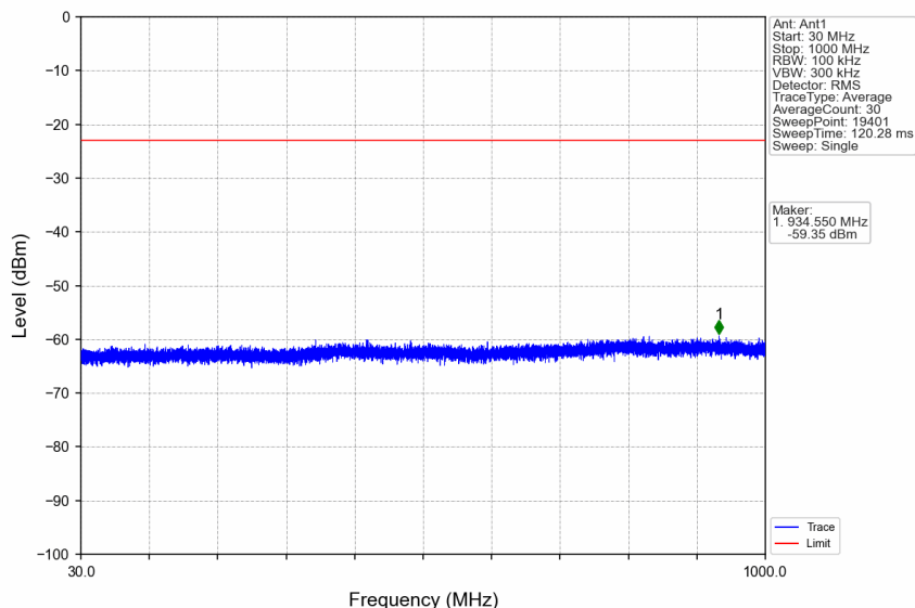
n66_30kHz_SISO_NTNV_40MHz_CP-OFDM QPSK_1730MHz_Edge_1RB_Left
