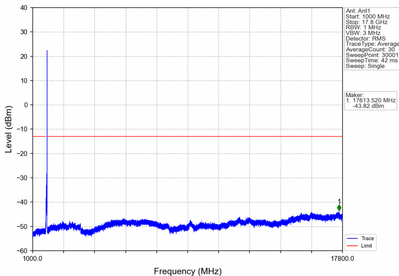
n66_30kHz_SISO_NTNV_40MHz_DFT-s-OFDM_QPSK_1760MHz_Edge_1RB_Right
