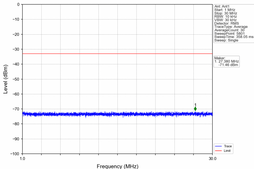
n66_30kHz_SISO_NTNV_40MHz_CP-OFDM QPSK_1745MHz_Edge_1RB_Left
