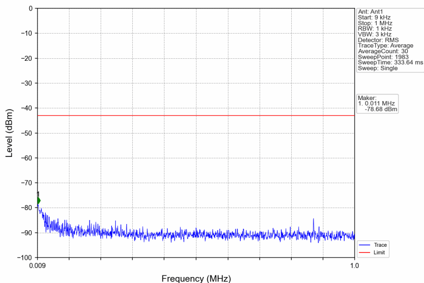
n66_30kHz_SISO_NTNV_35MHz_CP-OFDM QPSK_1762.5MHz_Edge_1RB_Right
