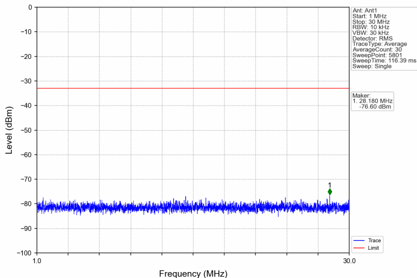
n66_30kHz_SISO_NTNV_35MHz_CP-OFDM QPSK_1745MHz_Edge_1RB_Left
