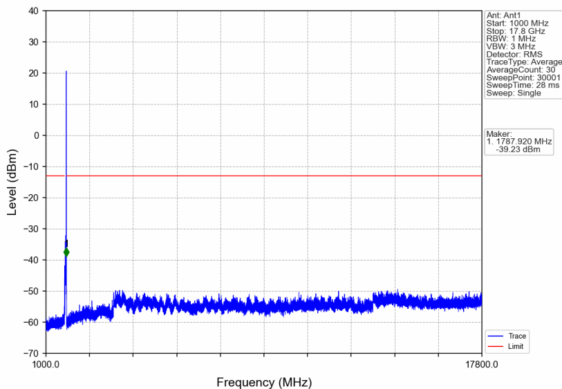
n66_30kHz_SISO_NTNV_35MHz_CP-OFDM QPSK_1762.5MHz_Edge_1RB_Right
