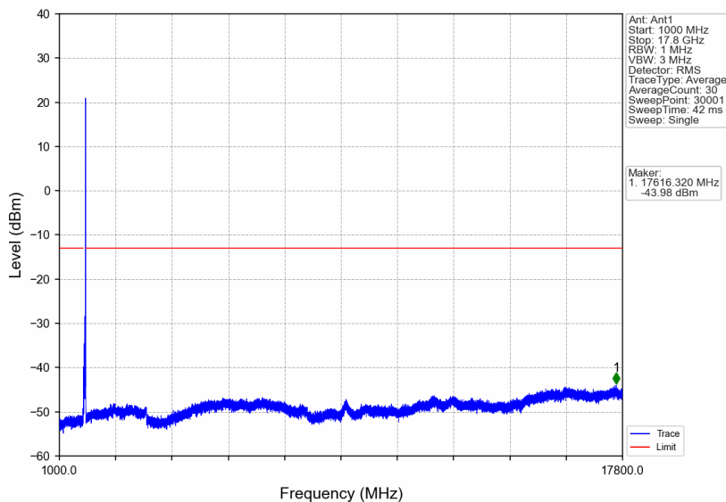
n66_30kHz_SISO_NTNV_40MHz_CP-OFDM QPSK_1760MHz_Edge_1RB_Right
