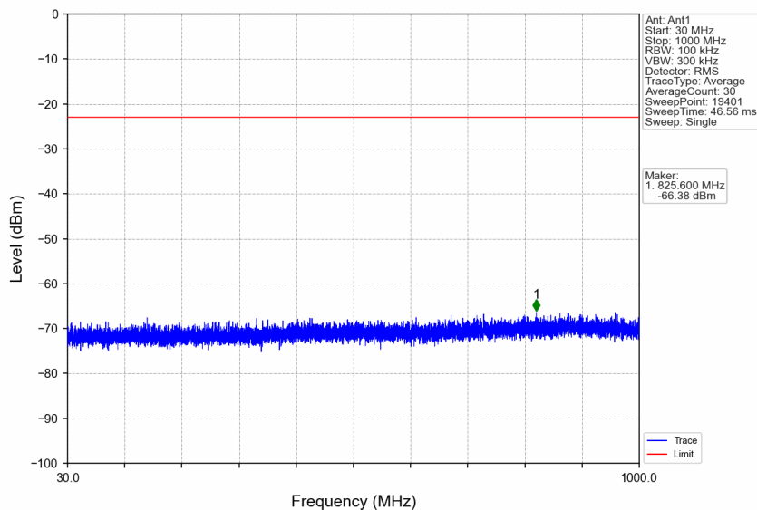
n66_30kHz_SISO_NTNV_35MHz_CP-OFDM QPSK_1745MHz_Edge_1RB_Left
