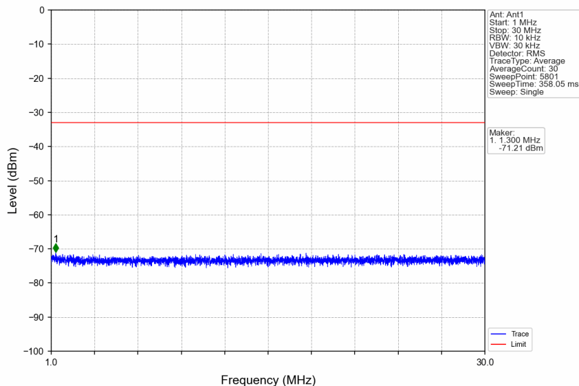
n66_30kHz_SISO_NTNV_40MHz_DFT-s-OFDM QPSK_1745MHz_Edge_1RB_Left
