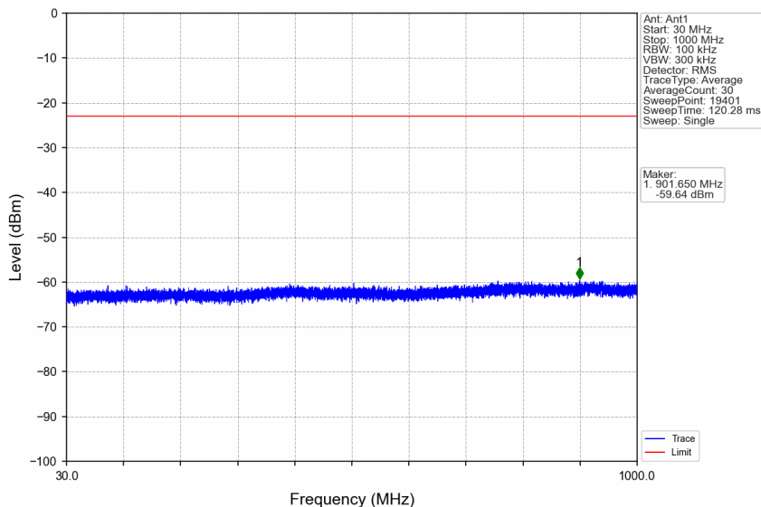
n66_30kHz_SISO_NTNV_40MHz_CP-OFDM QPSK_1760MHz_Edge_1RB_Right
