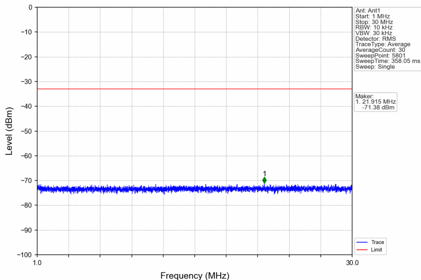
n66_30kHz_SISO_NTNV_40MHz_DFT-s-OFDM QPSK_1730MHz_Edge_1RB_Left
