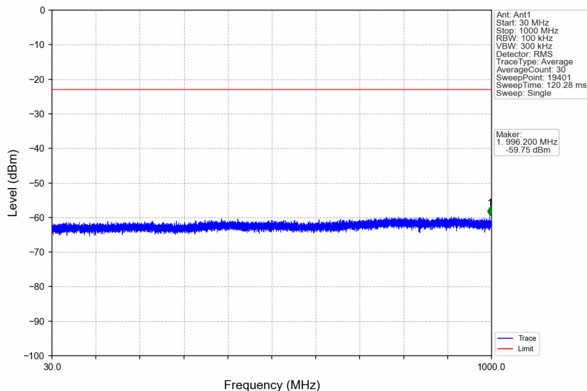
n66_30kHz_SISO_NTNV_40MHz_DFT-s-OFDM_QPSK_1760MHz_Edge_1RB_Right
