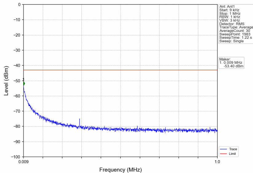
n66_30kHz_SISO_NTNV_40MHz_DFT-s-OFDM QPSK_1760MHz_Edge_1RB_Right
