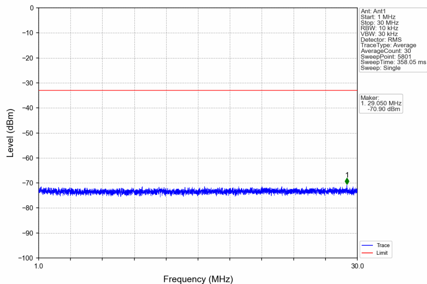
n66_30kHz_SISO_NTNV_40MHz_DFT-s-OFDM QPSK_1760MHz_Edge_1RB_Right
