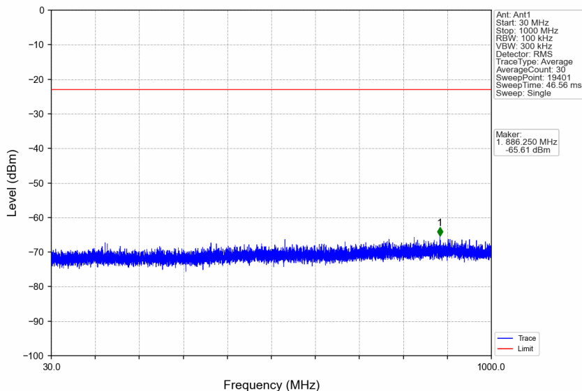
n66_30kHz_SISO_NTNV_35MHz_CP-OFDM QPSK_1762.5MHz_Edge_1RB_Right
