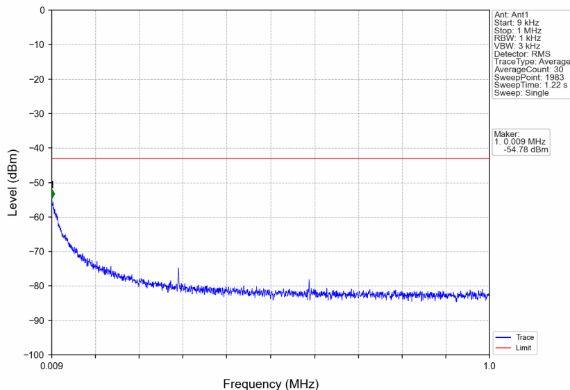
n66_30kHz_SISO_NTNV_30MHz_DFT-s-OFDM_QPSK_1765MHz_Edge_1RB_Right
