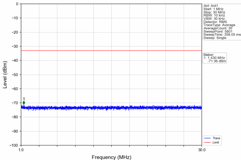
n66_30kHz_SISO_NTNV_30MHz_CP-OFDM QPSK_1765MHz_Edge_1RB_Right
