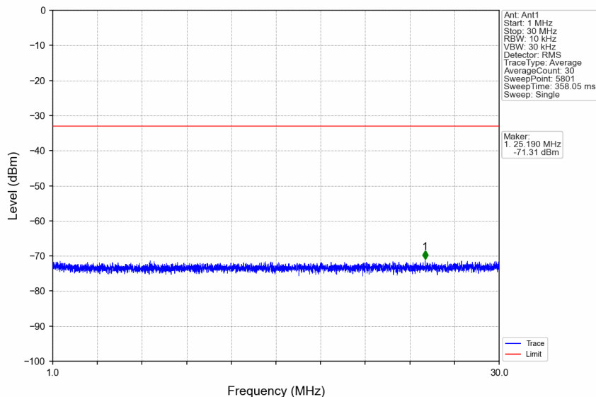
n66_30kHz_SISO_NTNV_30MHz_CP-OFDM QPSK_1745MHz_Edge_1RB_Left
