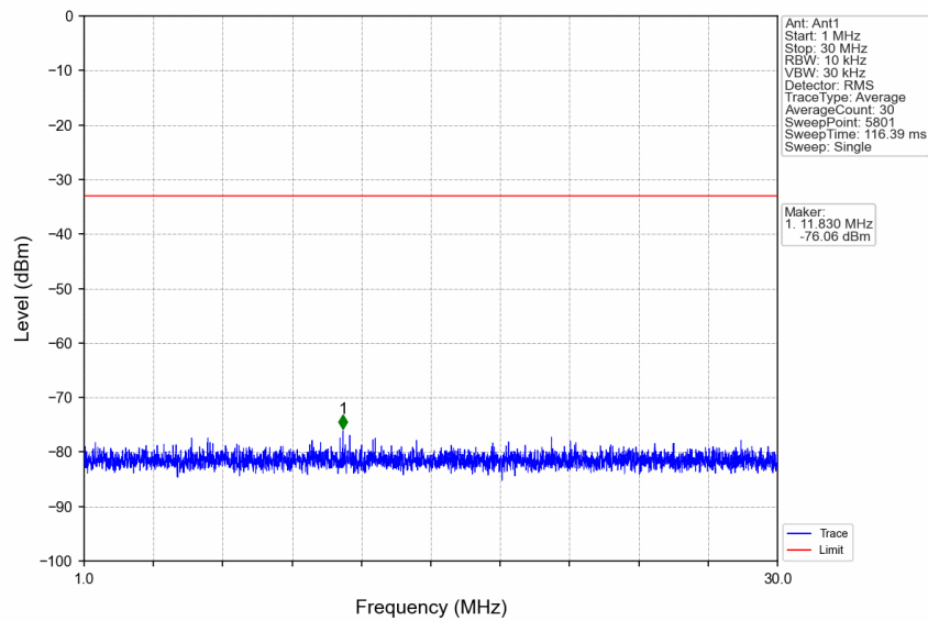
n66_30kHz_SISO_NTNV_35MHz_DFT-s-OFDM_QPSK_1727.5MHz_Edge_1RB_Left
