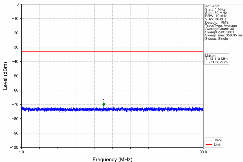
n66_30kHz_SISO_NTNV_30MHz_DFT-s-OFDM QPSK_1745MHz_Edge_1RB_Left
