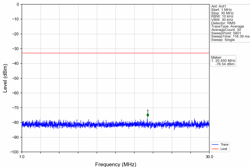
n66_30kHz_SISO_NTNV_35MHz_CP-OFDM QPSK_1727.5MHz_Edge_1RB_Left
