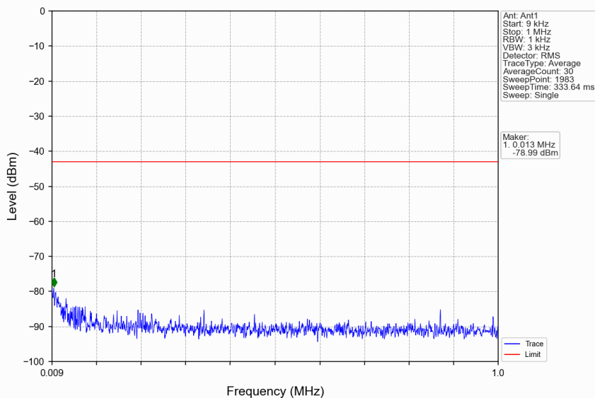
n66_30kHz_SISO_NTNV_35MHz_CP-OFDM QPSK_1745MHz_Edge_1RB_Left
