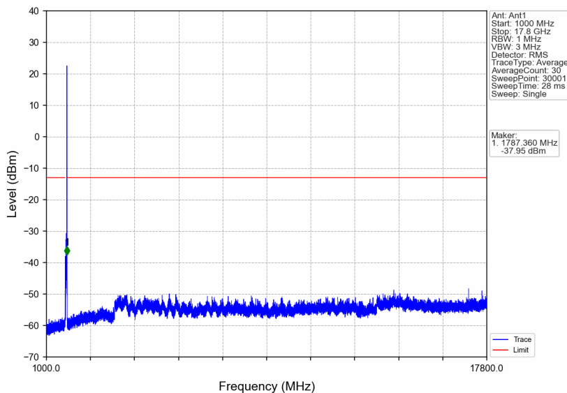
n66_30kHz_SISO_NTNV_35MHz_DFT-s-OFDM QPSK_1762.5MHz_Edge_1RB_Right
