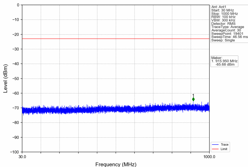
n66_30kHz_SISO_NTNV_35MHz_DFT-s-OFDM QPSK_1762.5MHz_Edge_1RB_Right
