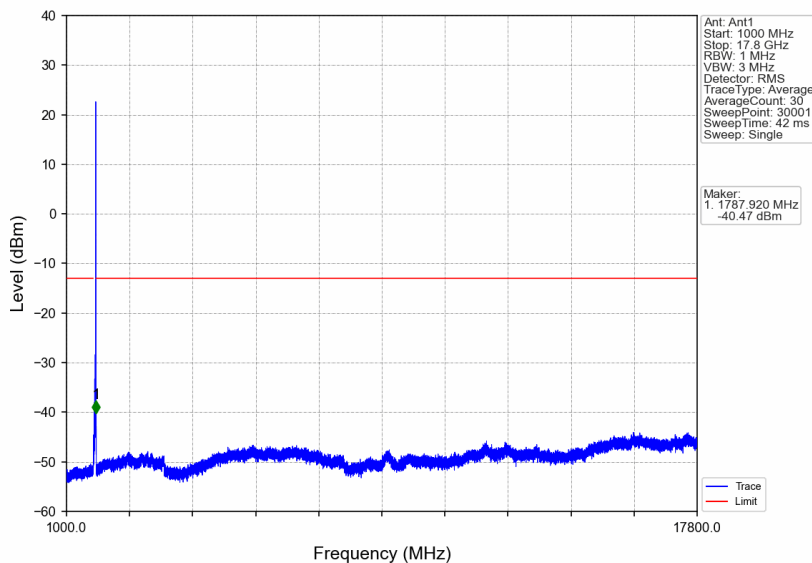
n66_30kHz_SISO_NTNV_30MHz_DFT-s-OFDM QPSK_1765MHz_Edge_1RB_Right
