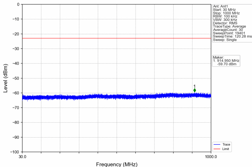
n66_30kHz_SISO_NTNV_30MHz_DFT-s-OFDM QPSK_1765MHz_Edge_1RB_Right
