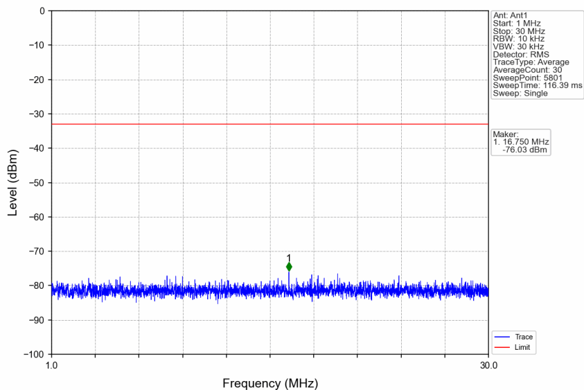
n66_30kHz_SISO_NTNV_35MHz_DFT-s-OFDM QPSK_1762.5MHz_Edge_1RB_Right
