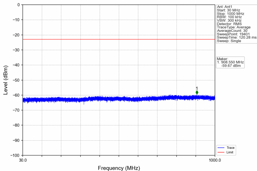
n66_30kHz_SISO_NTNV_30MHz_CP-OFDM QPSK_1725MHz_Edge_1RB_Left
