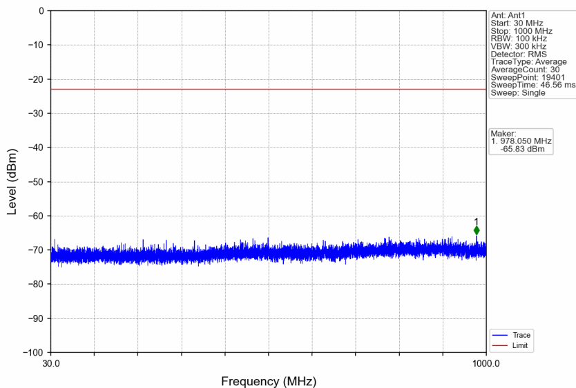
n66_30kHz_SISO_NTNV_35MHz_CP-OFDM QPSK_1727.5MHz_Edge_1RB_Left
