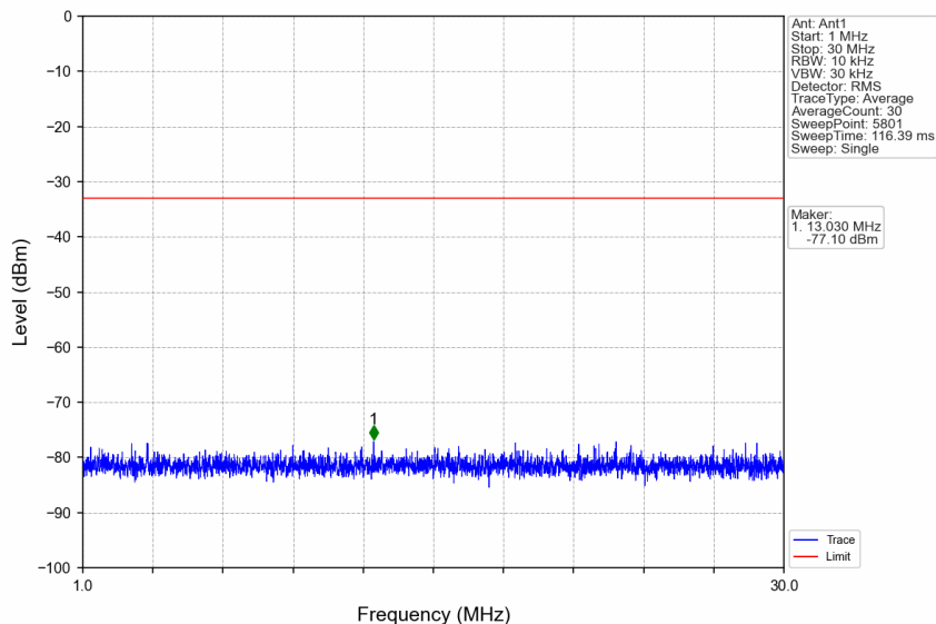
n66_30kHz_SISO_NTNV_35MHz_DFT-s-OFDM QPSK_1745MHz_Edge_1RB_Left
