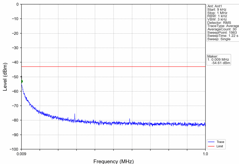
n66_30kHz_SISO_NTNV_30MHz_CP-OFDM QPSK_1765MHz_Edge_1RB_Right
