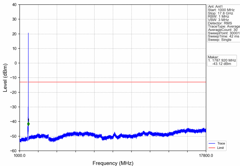
n66_30kHz_SISO_NTNV_30MHz_CP-OFDM QPSK_1765MHz_Edge_1RB_Right
