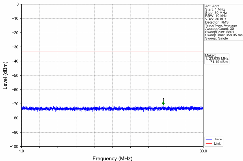
n66_30kHz_SISO_NTNV_30MHz_DFT-s-OFDM QPSK_1725MHz_Edge_1RB_Left
