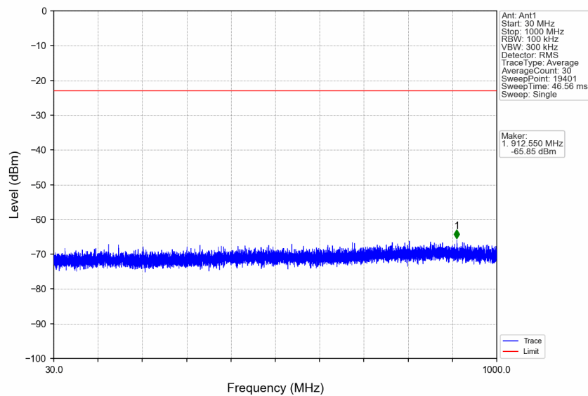
n66_30kHz_SISO_NTNV_35MHz_DFT-s-OFDM_QPSK_1727.5MHz_Edge_1RB_Left
