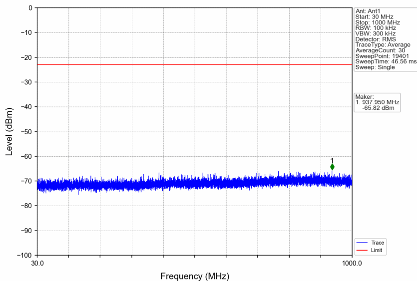
n66_30kHz_SISO_NTNV_35MHz_DFT-s-OFDM QPSK_1745MHz_Edge_1RB_Left
