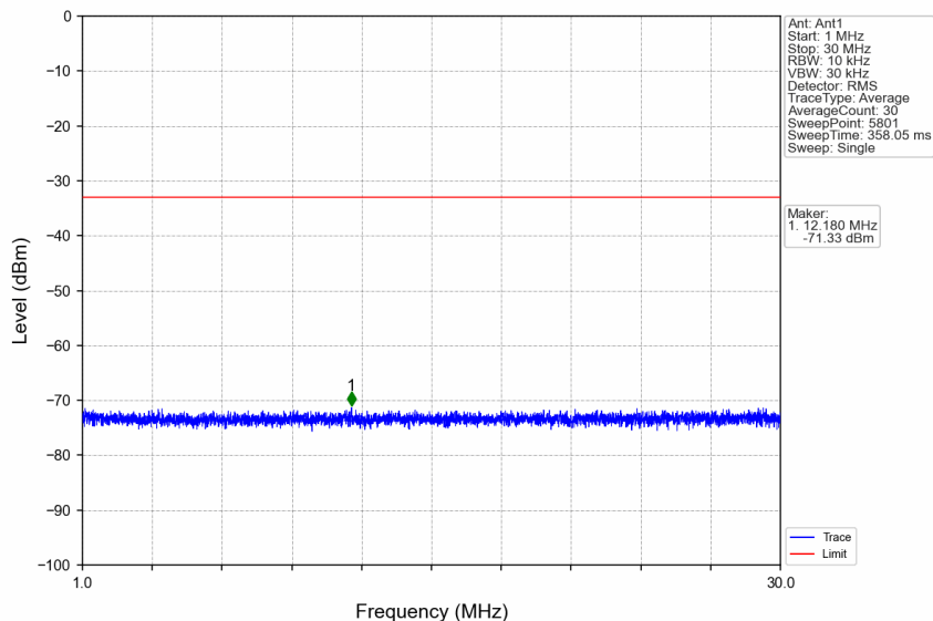
n66_30kHz_SISO_NTNV_30MHz_CP-OFDM QPSK_1725MHz_Edge_1RB_Left
