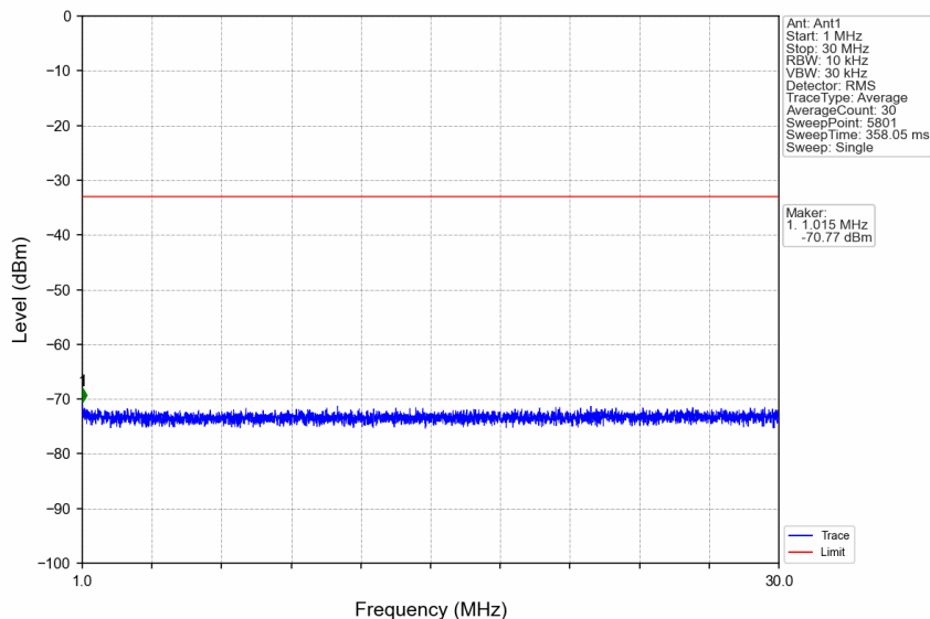
n66_30kHz_SISO_NTNV_25MHz_DFT-s-OFDM QPSK_1722.5MHz_Edge_1RB_Left
