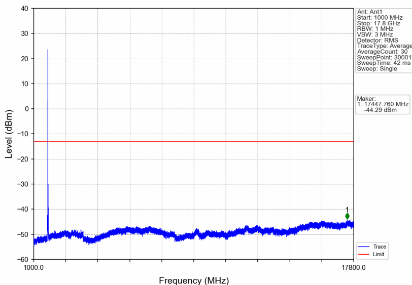
n66_30kHz_SISO_NTNV_25MHz_DFT-s-OFDM PI/2 BPSK_1767.5MHz_Edge_1RB_Right
