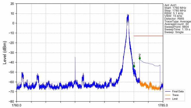
n66_30kHz_SISO_NTNV_20MHz_DFT-s-OFDM QPSK_1770MHz_Edge_1RB_Right
