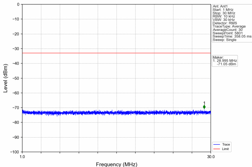
n66_30kHz_SISO_NTNV_25MHz_CP-OFDM QPSK_1745MHz_Edge_1RB_Left
