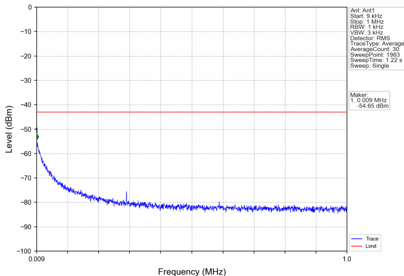
n66_30kHz_SISO_NTNV_20MHz_CP-OFDM QPSK_1770MHz_Edge_1RB_Right
