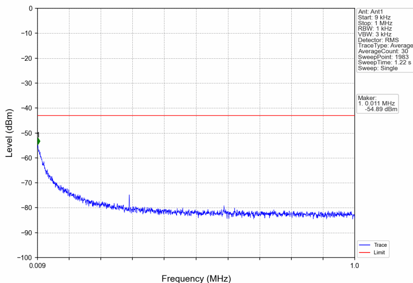
n66_30kHz_SISO_NTNV_25MHz_CP-OFDM QPSK_1767.5MHz_Edge_1RB_Right
