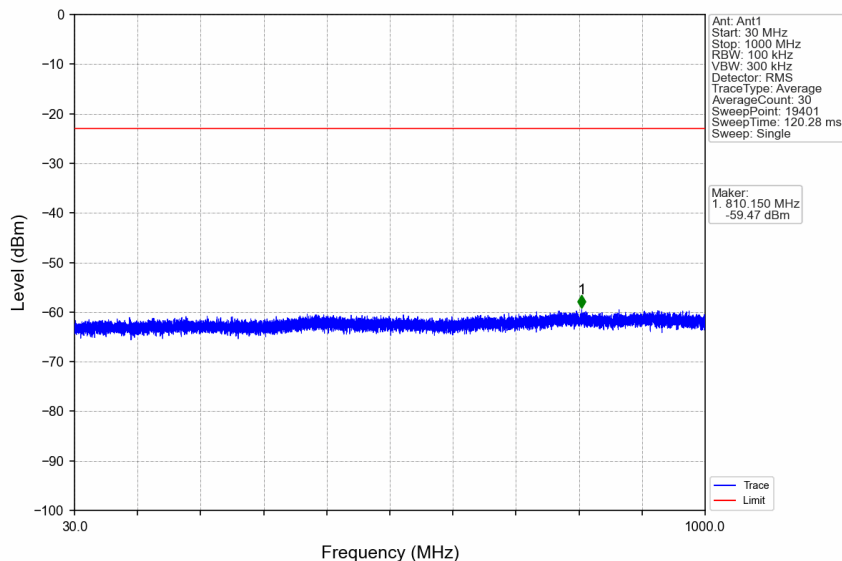
n66_30kHz_SISO_NTNV_20MHz_CP-OFDM QPSK_1770MHz_Edge_1RB_Right
