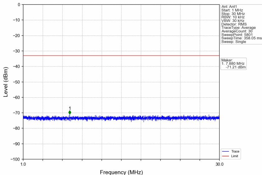
n66_30kHz_SISO_NTNV_20MHz_DFT-s-OFDM QPSK_1745MHz_Edge_1RB_Left
