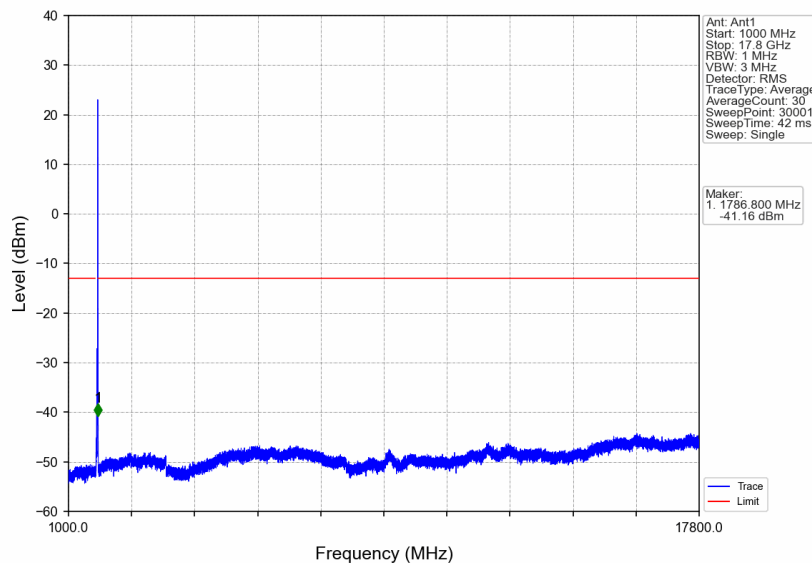
n66_30kHz_SISO_NTNV_25MHz_DFT-s-OFDM QPSK_1767.5MHz_Edge_1RB_Right
