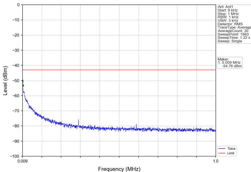
n66_30kHz_SISO_NTNV_25MHz_CP-OFDM QPSK_1745MHz_Edge_1RB_Left
