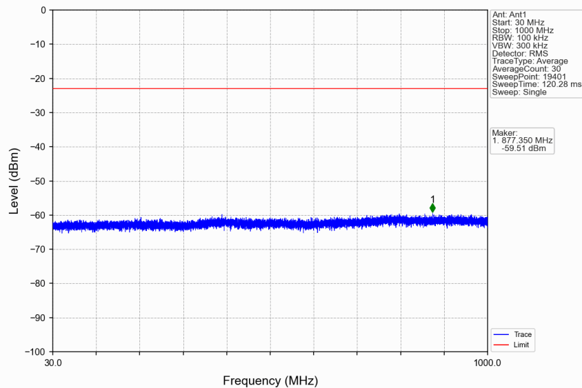
n66_30kHz_SISO_NTNV_25MHz_DFT-s-OFDM QPSK_1767.5MHz_Edge_1RB_Right
