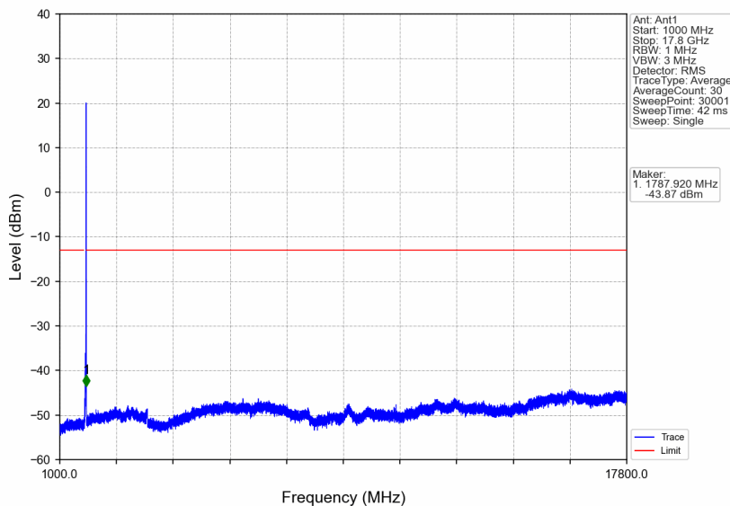
n66_30kHz_SISO_NTNV_20MHz_CP-OFDM QPSK_1770MHz_Edge_1RB_Right
