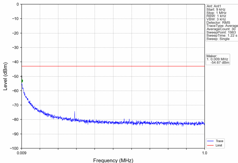
n66_30kHz_SISO_NTNV_20MHz_DFT-s-OFDM QPSK_1770MHz_Edge_1RB_Right
