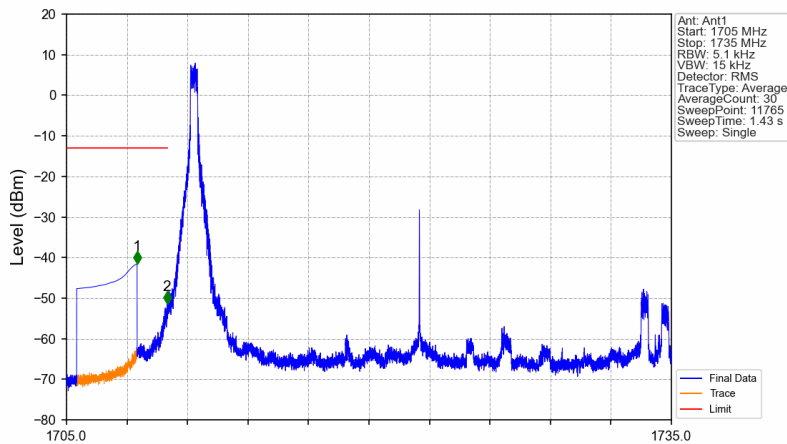
n66_30kHz_SISO_NTNV_25MHz_CP-OFDM QPSK_1722.5MHz_Inner_1RB_Left
