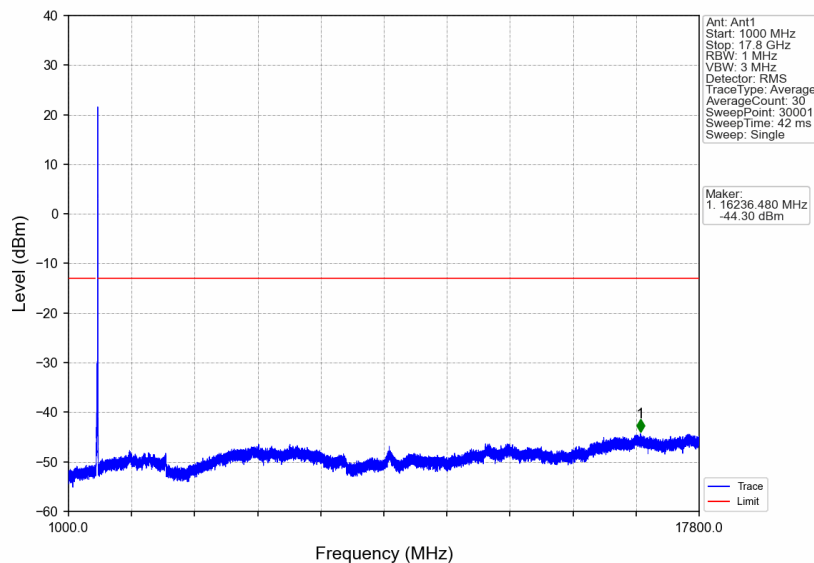
n66_30kHz_SISO_NTNV_25MHz_CP-OFDM QPSK_1767.5MHz_Edge_1RB_Right
