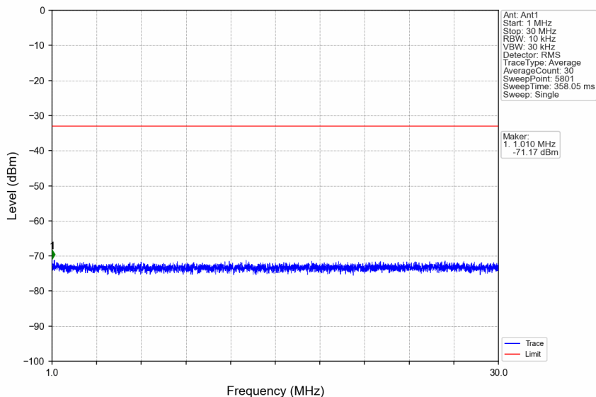
n66_30kHz_SISO_NTNV_25MHz_DFT-s-OFDM QPSK_1745MHz_Edge_1RB_Left
