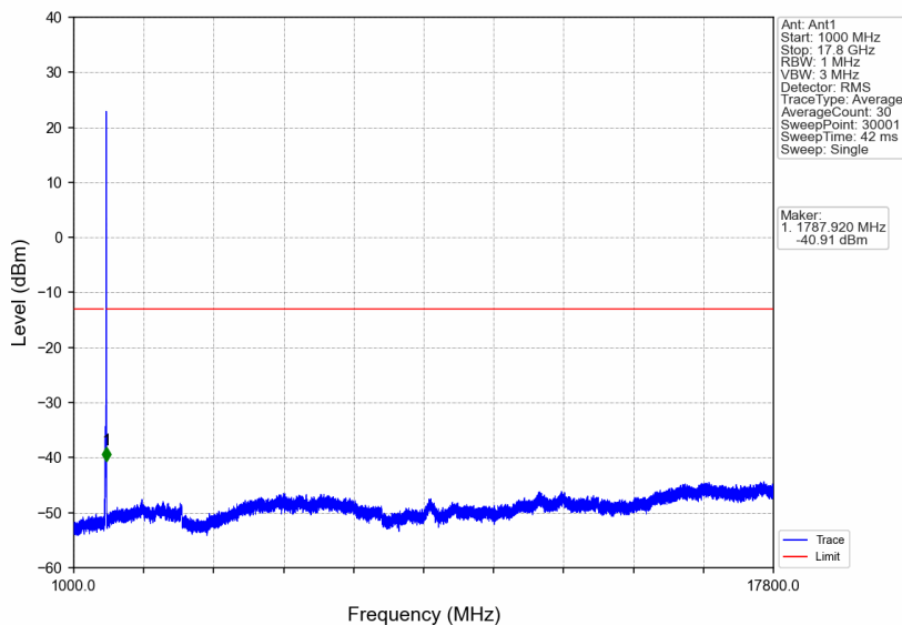
n66_30kHz_SISO_NTNV_20MHz_DFT-s-OFDM_QPSK_1770MHz_Edge_1RB_Right
