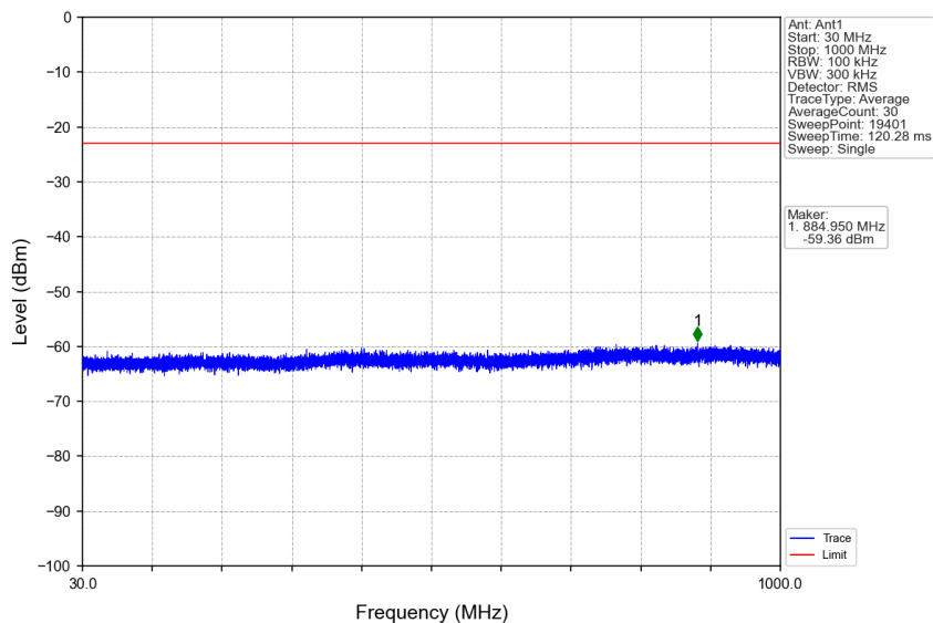
n66_30kHz_SISO_NTNV_25MHz_CP-OFDM QPSK_1722.5MHz_Edge_1RB_Left
