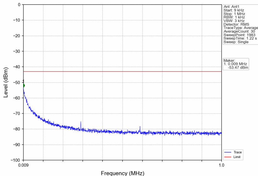
n66_30kHz_SISO_NTNV_25MHz_DFT-s-OFDM QPSK_1767.5MHz_Edge_1RB_Right
