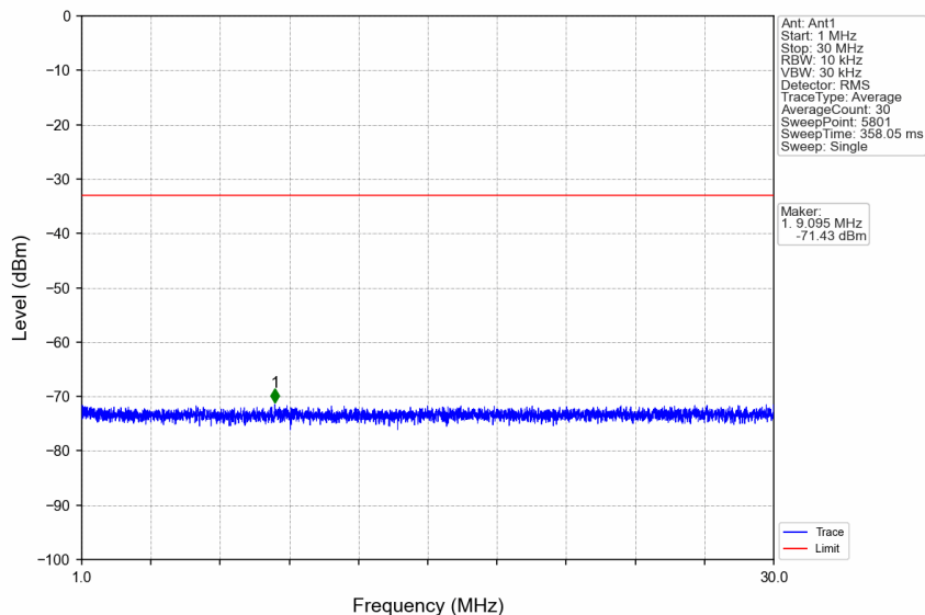
n66_30kHz_SISO_NTNV_25MHz_CP-OFDM QPSK_1722.5MHz_Edge_1RB_Left
