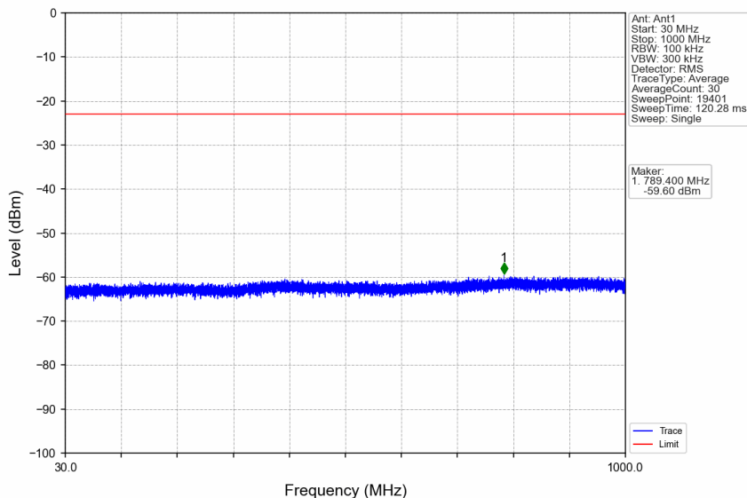
n66_30kHz_SISO_NTNV_20MHz_DFT-s-OFDM_QPSK_1770MHz_Edge_1RB_Right
