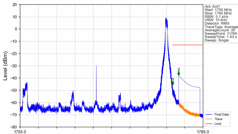
n66_30kHz_SISO_NTNV_25MHz_DFT-s-OFDM PI/2 BPSK_1767.5MHz_Edge_1RB_Right
