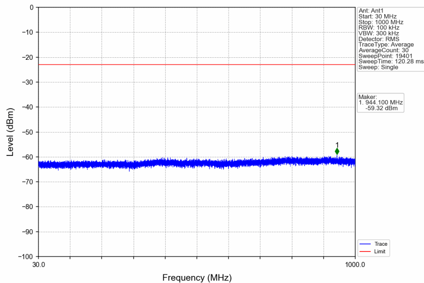
n66_30kHz_SISO_NTNV_25MHz_CP-OFDM QPSK_1767.5MHz_Edge_1RB_Right
