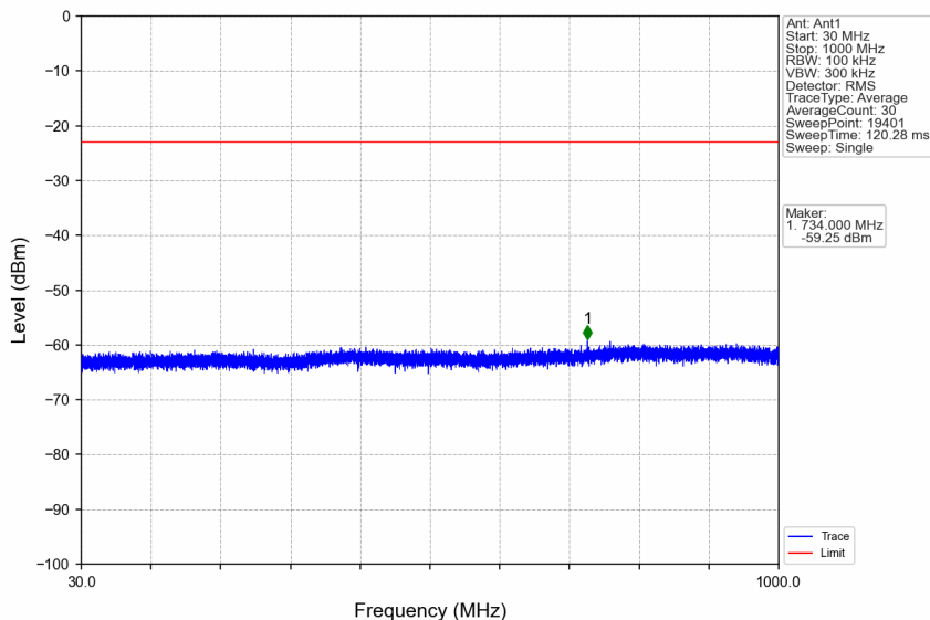
n66_30kHz_SISO_NTNV_10MHz_CP-OFDM QPSK_1775MHz_Edge_1RB_Right
