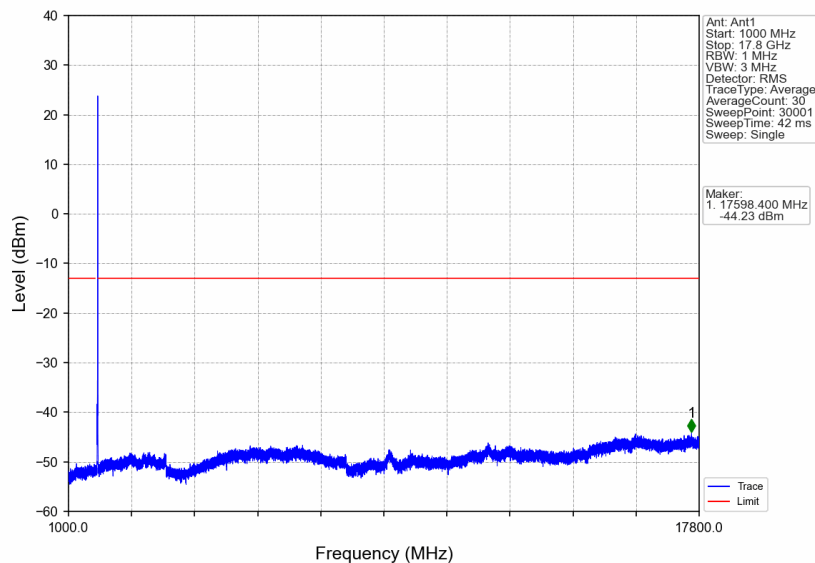
n66_30kHz_SISO_NTNV_10MHz_DFT-s-OFDM PI/2 BPSK_1775MHz_Edge_1RB_Right
