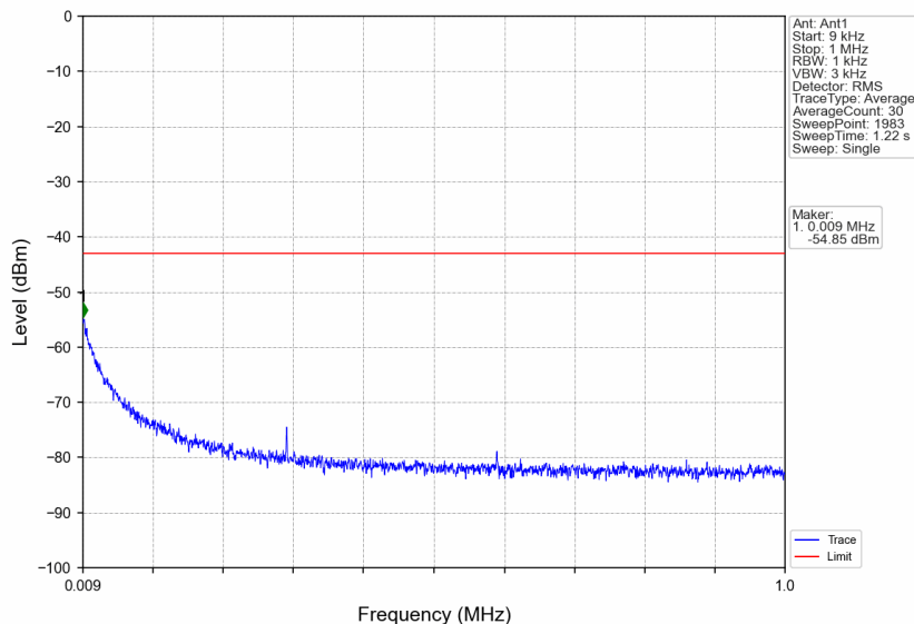
n66_30kHz_SISO_NTNV_10MHz_DFT-s-OFDM QPSK_1775MHz_Edge_1RB_Right
