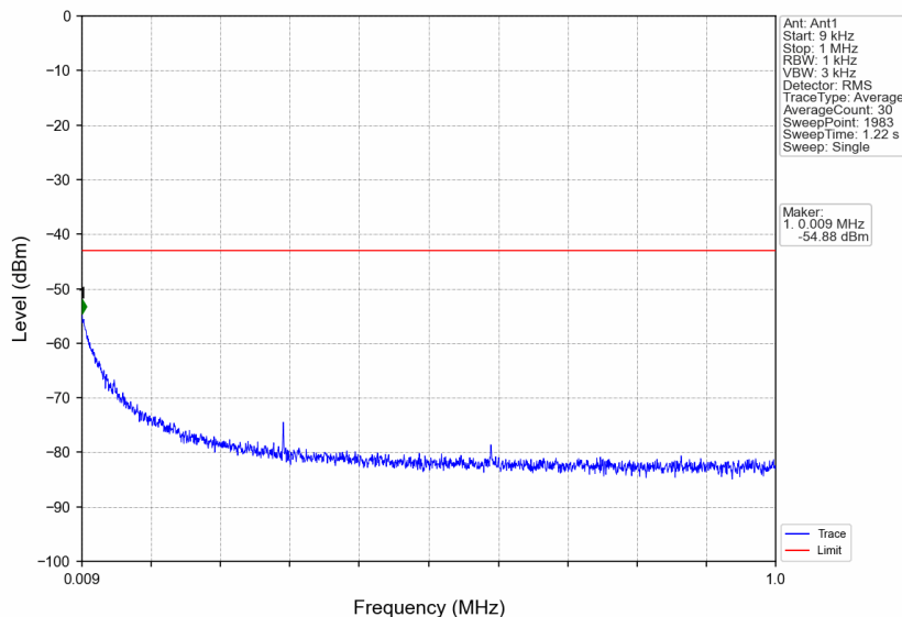
n66_30kHz_SISO_NTNV_10MHz_CP-OFDM QPSK_1775MHz_Edge_1RB_Right
