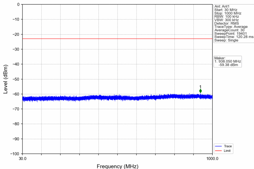
n66_30kHz_SISO_NTNV_15MHz_DFT-s-OFDM QPSK_1772.5MHz_Edge_1RB_Right
