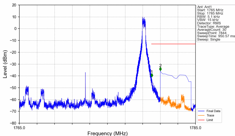
n66_30kHz_SISO_NTNV_15MHz_DFT-s-OFDM PI/2 BPSK_1772.5MHz_Edge_1RB_Right
