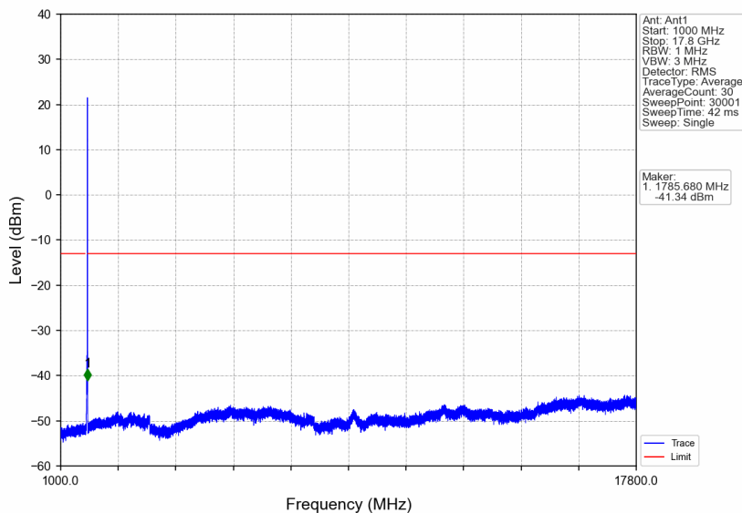
n66_30kHz_SISO_NTNV_15MHz_CP-OFDM QPSK_1772.5MHz_Edge_1RB_Right
