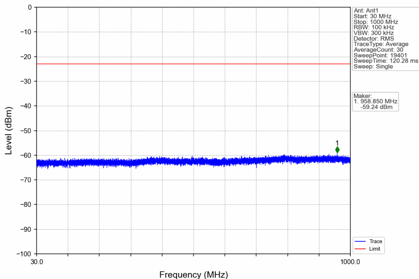
n66_30kHz_SISO_NTNV_15MHz_CP-OFDM QPSK_1772.5MHz_Edge_1RB_Right
