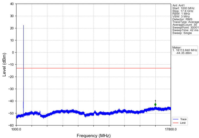
n66_30kHz_SISO_NTNV_10MHz_CP-OFDM QPSK_1775MHz_Edge_1RB_Right
