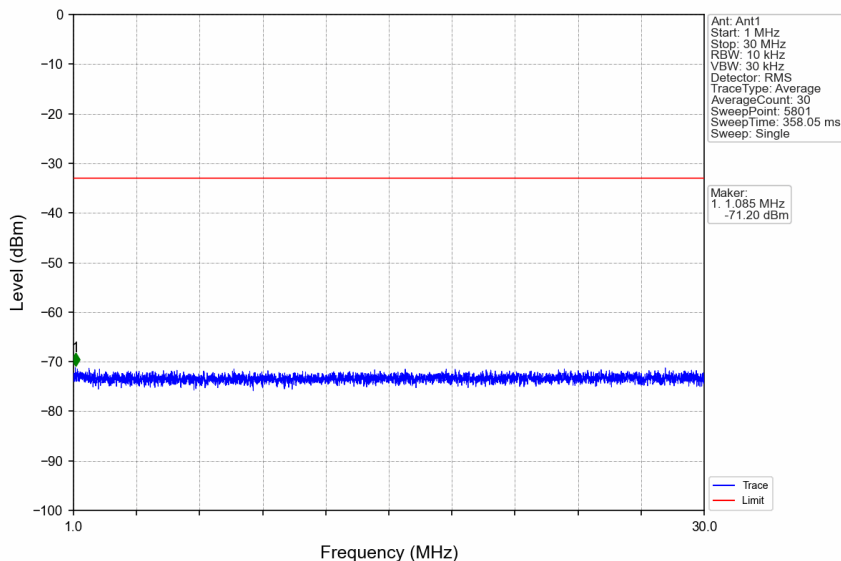
n66_30kHz_SISO_NTNV_15MHz_DFT-s-OFDM QPSK_1745MHz_Edge_1RB_Left
