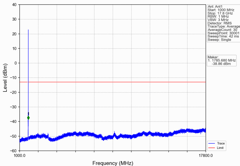
n66_30kHz_SISO_NTNV_15MHz_DFT-s-OFDM QPSK_1772.5MHz_Edge_1RB_Right
