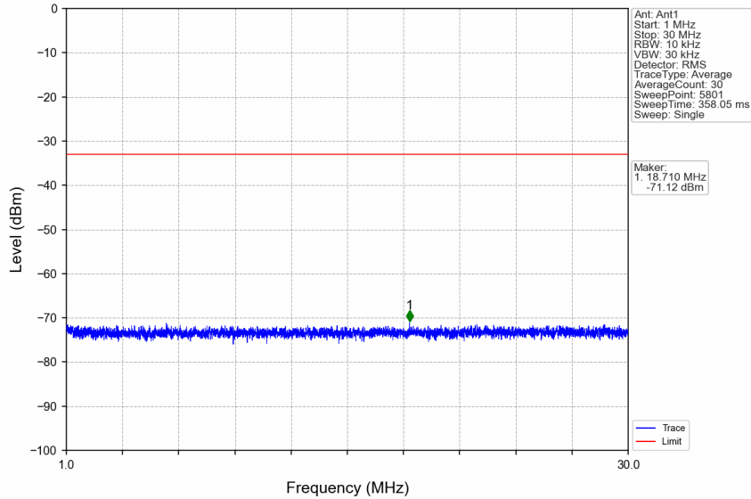
n66_30kHz_SISO_NTNV_15MHz_DFT-s-OFDM_QPSK_1717.5MHz_Edge_1RB_Left
