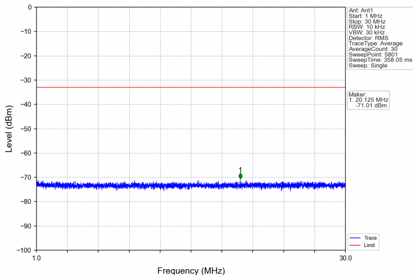
n66_30kHz_SISO_NTNV_10MHz_CP-OFDM QPSK_1715MHz_Edge_1RB_Left
