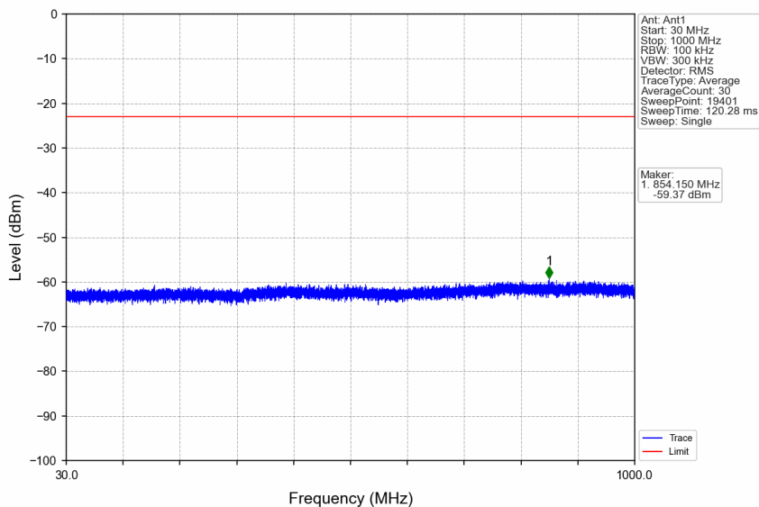
n66_30kHz_SISO_NTNV_15MHz_CP-OFDM QPSK_1717.5MHz_Edge_1RB_Left
