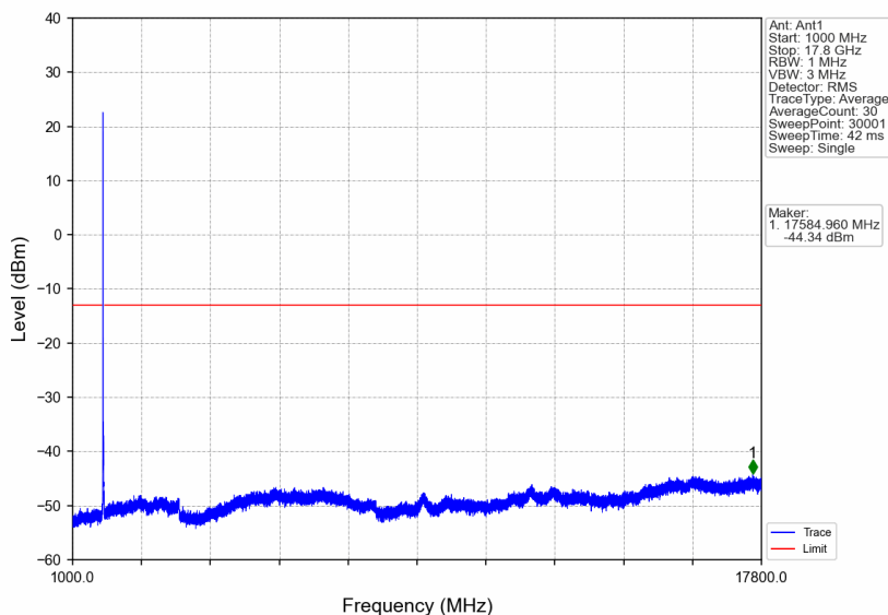
n66_30kHz_SISO_NTNV_15MHz_DFT-s-OFDM PI/2 BPSK_1772.5MHz_Edge_1RB_Right
