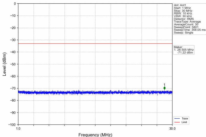
n66_30kHz_SISO_NTNV_10MHz_CP-OFDM QPSK_1745MHz_Edge_1RB_Left
