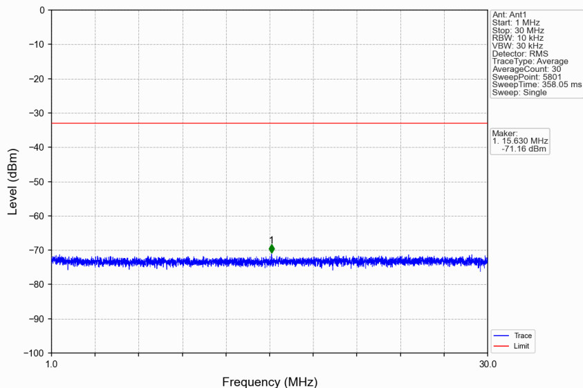
n66_30kHz_SISO_NTNV_10MHz_DFT-s-OFDM QPSK_1715MHz_Edge_1RB_Left
