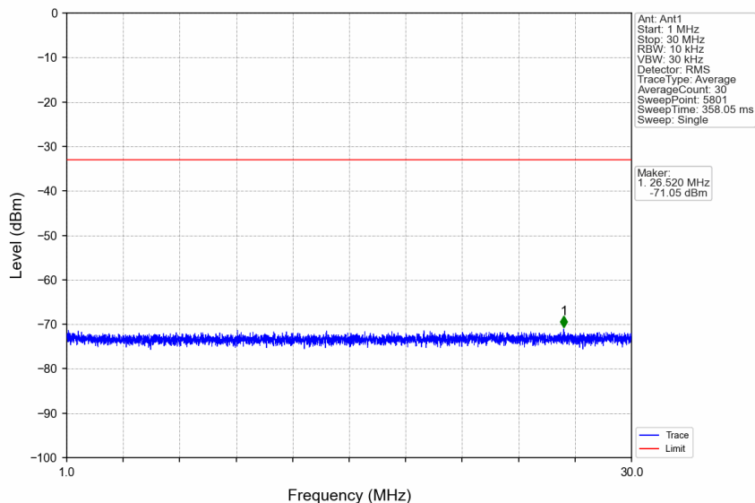
n66_30kHz_SISO_NTNV_10MHz_DFT-s-OFDM QPSK_1745MHz_Edge_1RB_Left
