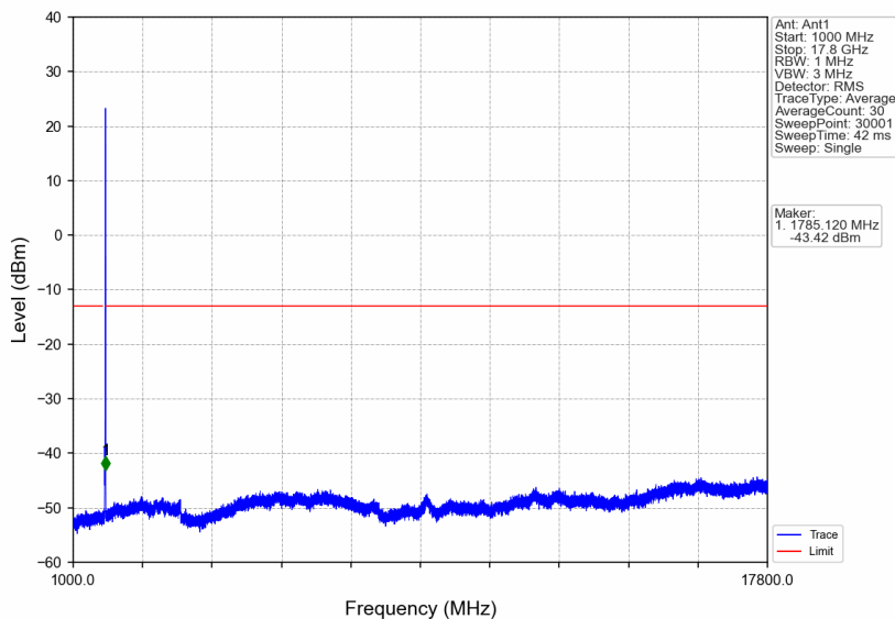
n66_30kHz_SISO_NTNV_10MHz_DFT-s-OFDM_QPSK_1775MHz_Edge_1RB_Right
