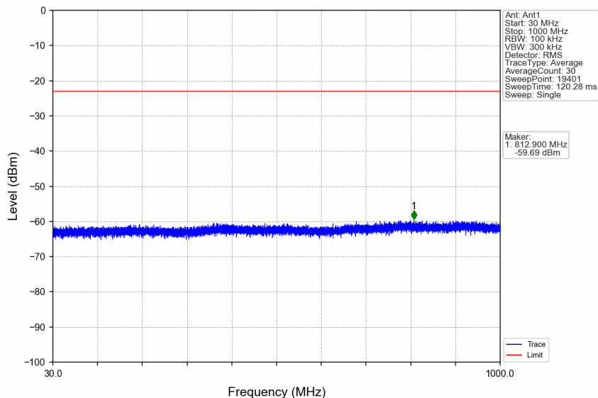
n66_30kHz_SISO_NTNV_10MHz_DFT-s-OFDM_QPSK_1775MHz_Edge_1RB_Right
