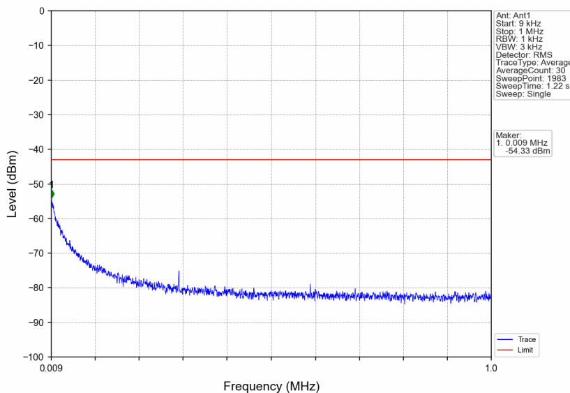
n66_30kHz_SISO_NTNV_15MHz_CP-OFDM QPSK_1745MHz_Edge_1RB_Left
