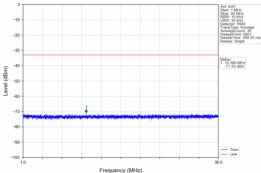
n66_30kHz_SISO_NTNV_15MHz_CP-OFDM QPSK_1745MHz_Edge_1RB_Left
