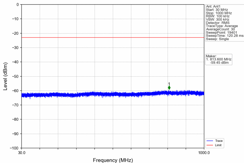
n66_30kHz_SISO_NTNV_10MHz_CP-OFDM QPSK_1715MHz_Edge_1RB_Left
