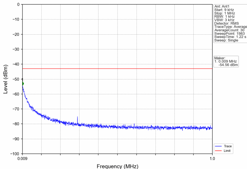
n66_30kHz_SISO_NTNV_15MHz_DFT-s-OFDM QPSK_1772.5MHz_Edge_1RB_Right
