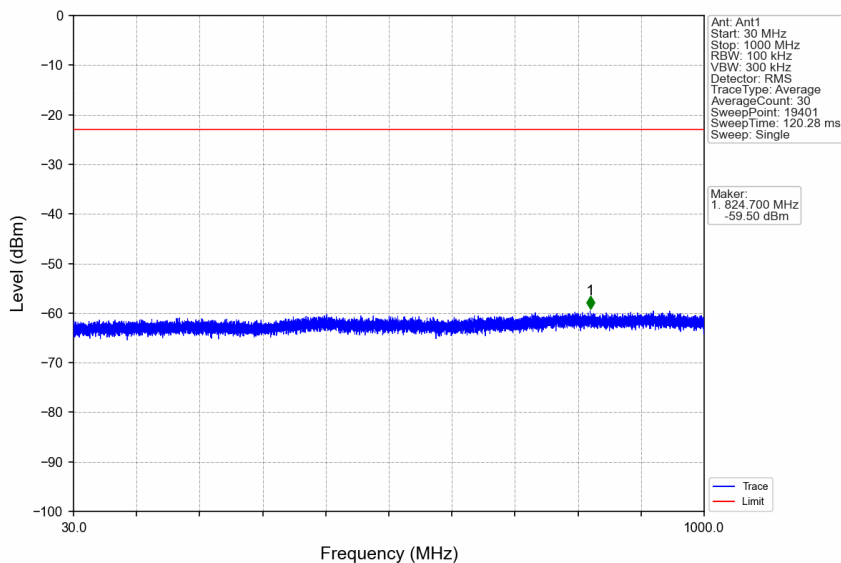
n66_30kHz_SISO_NTNV_15MHz_DFT-s-OFDM QPSK_1745MHz_Edge_1RB_Left
