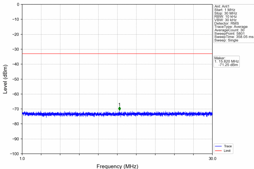
n66_30kHz_SISO_NTNV_15MHz_CP-OFDM QPSK_1717.5MHz_Edge_1RB_Left
